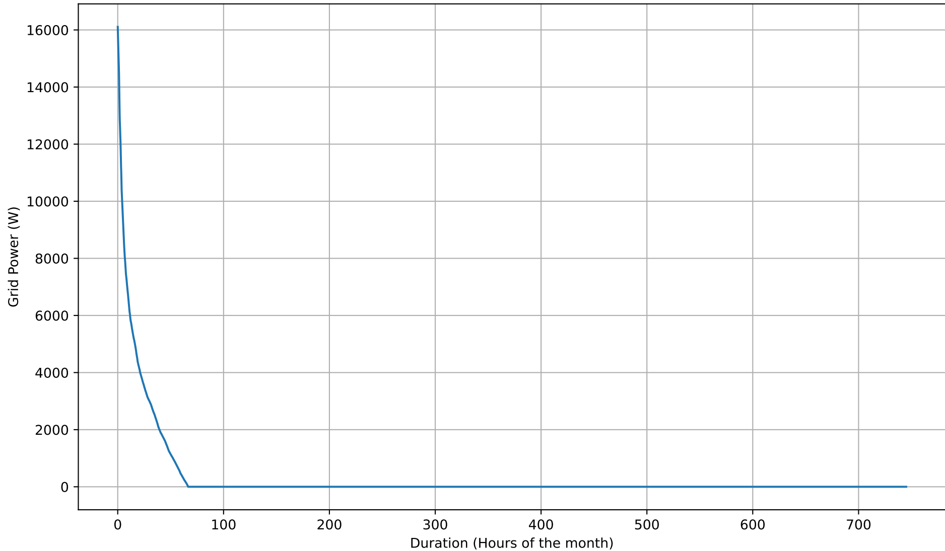
Grid Export Duration Curve - 15kWh - Oct
