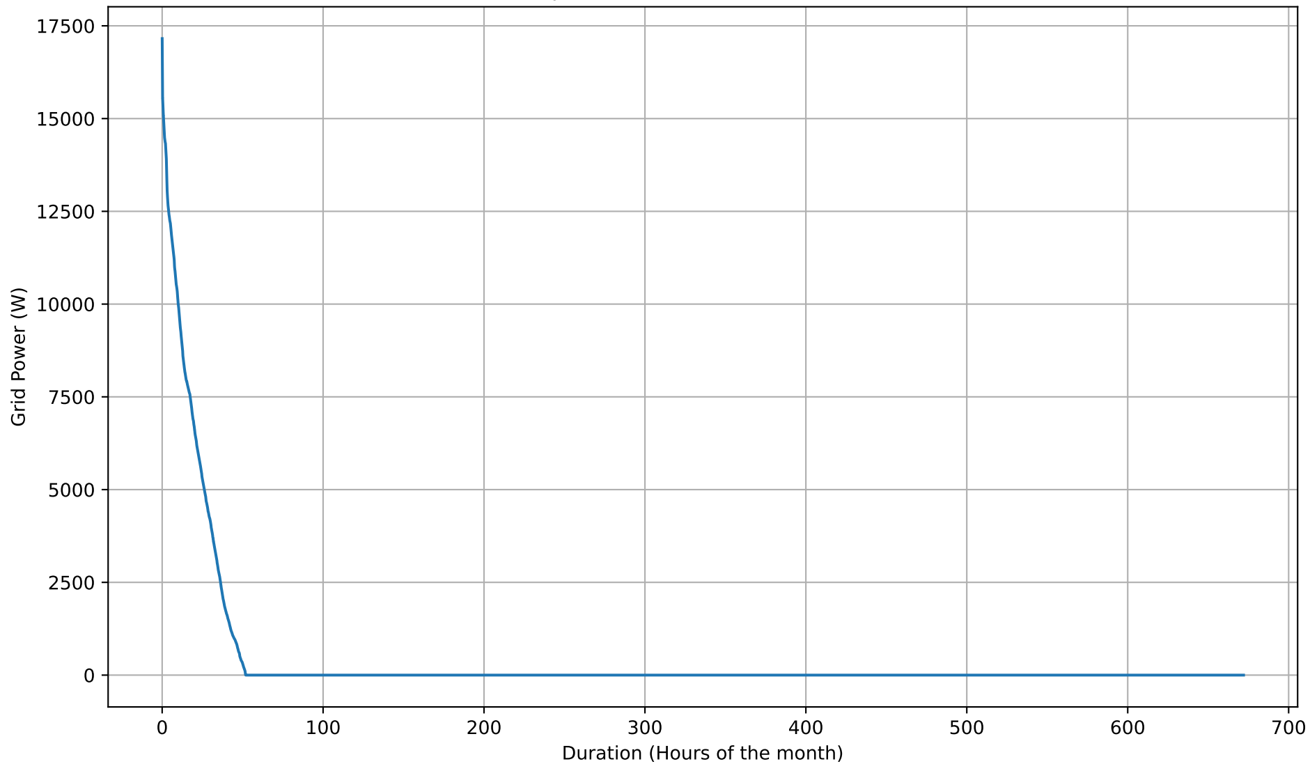
Grid Export Duration Curve - 15kWh - Feb
