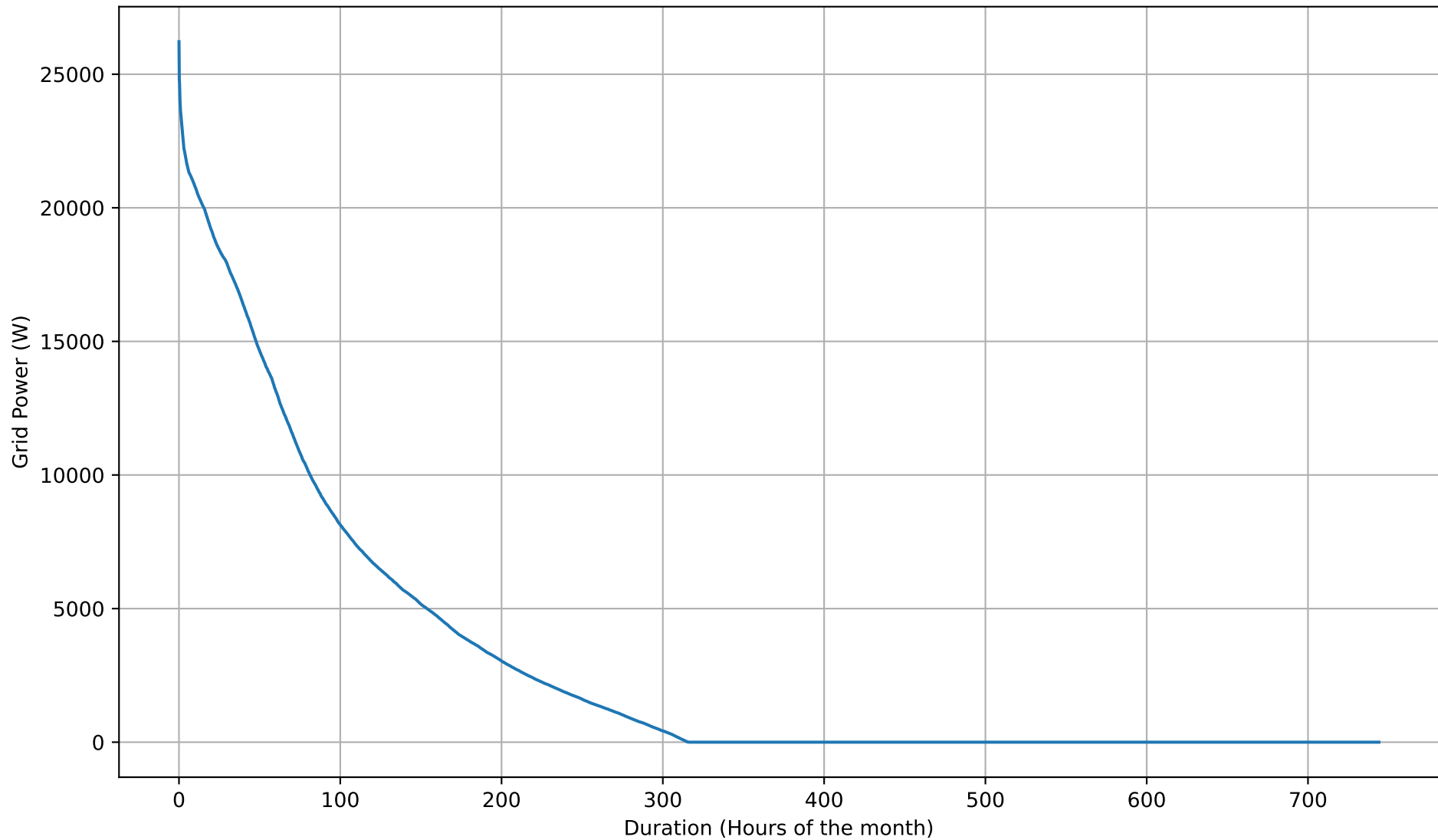
Grid Export Duration Curve - 15kWh - Jul
