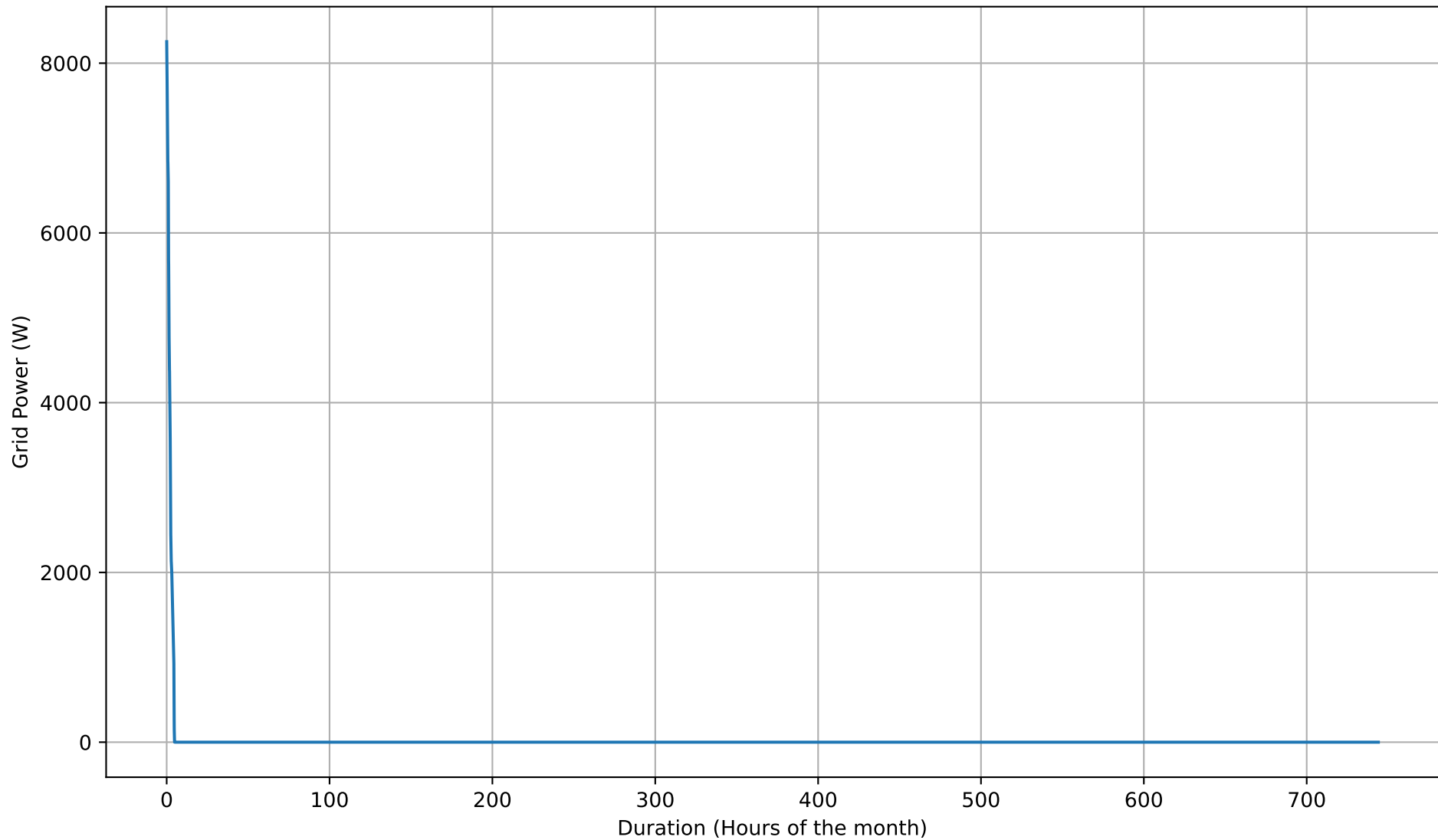
Grid Export Duration Curve - 15kWh - Jan
