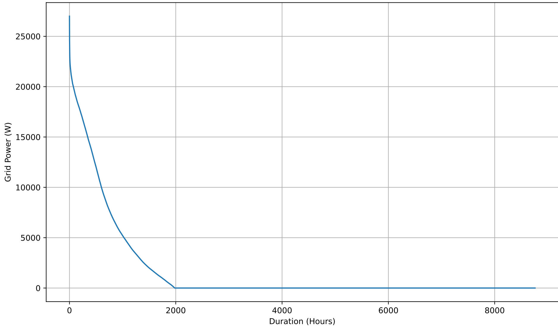
Yearly Grid Export Duration Curve - 15kWh
