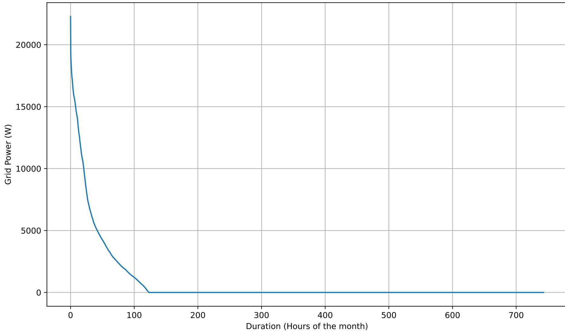
Grid Export Duration Curve - 15kWh - Mar
