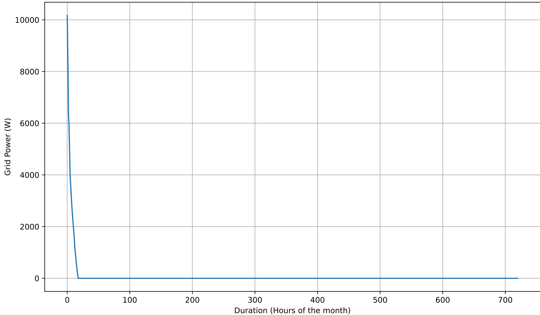
Grid Export Duration Curve - 15kWh - Nov
