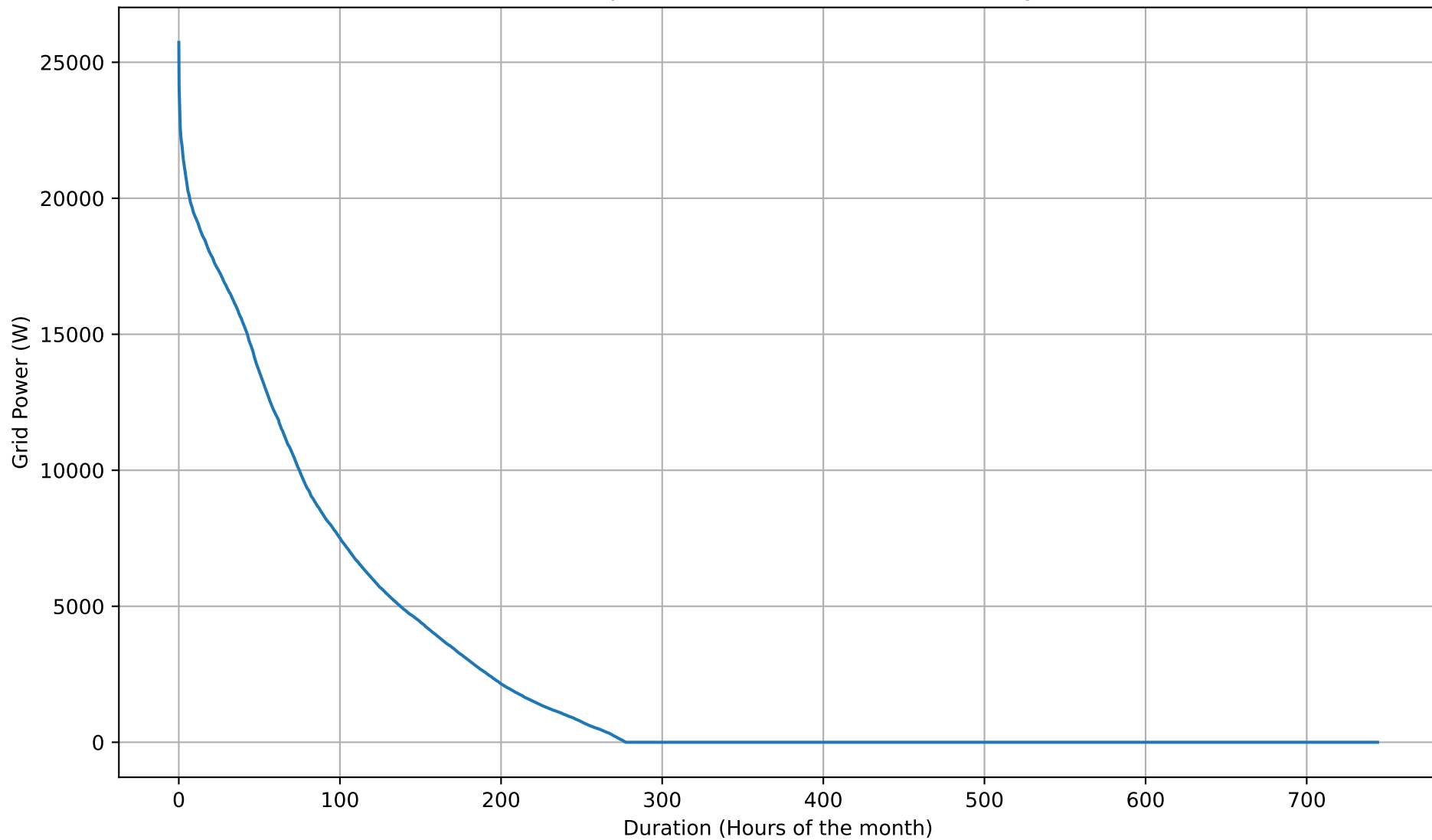
Grid Export Duration Curve - 15kWh - Aug
