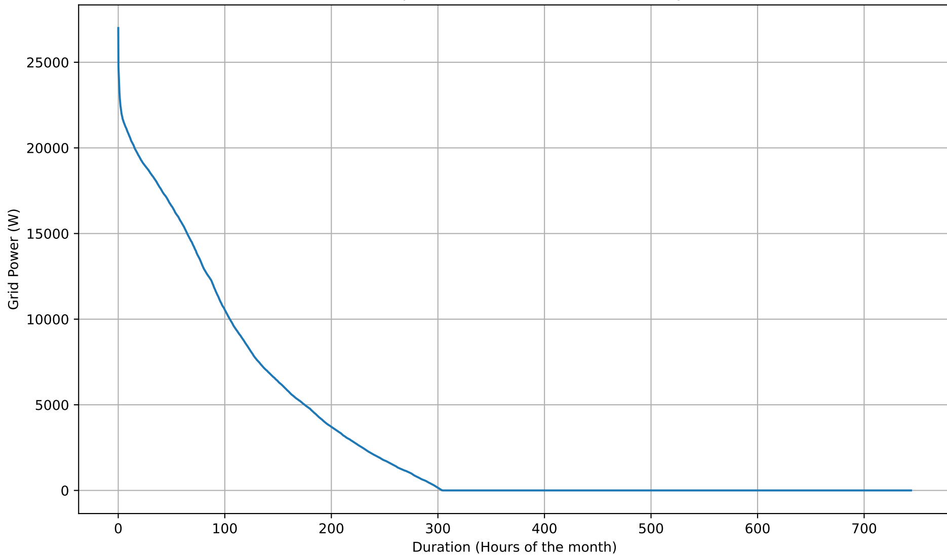
Grid Export Duration Curve - 15kWh - May
