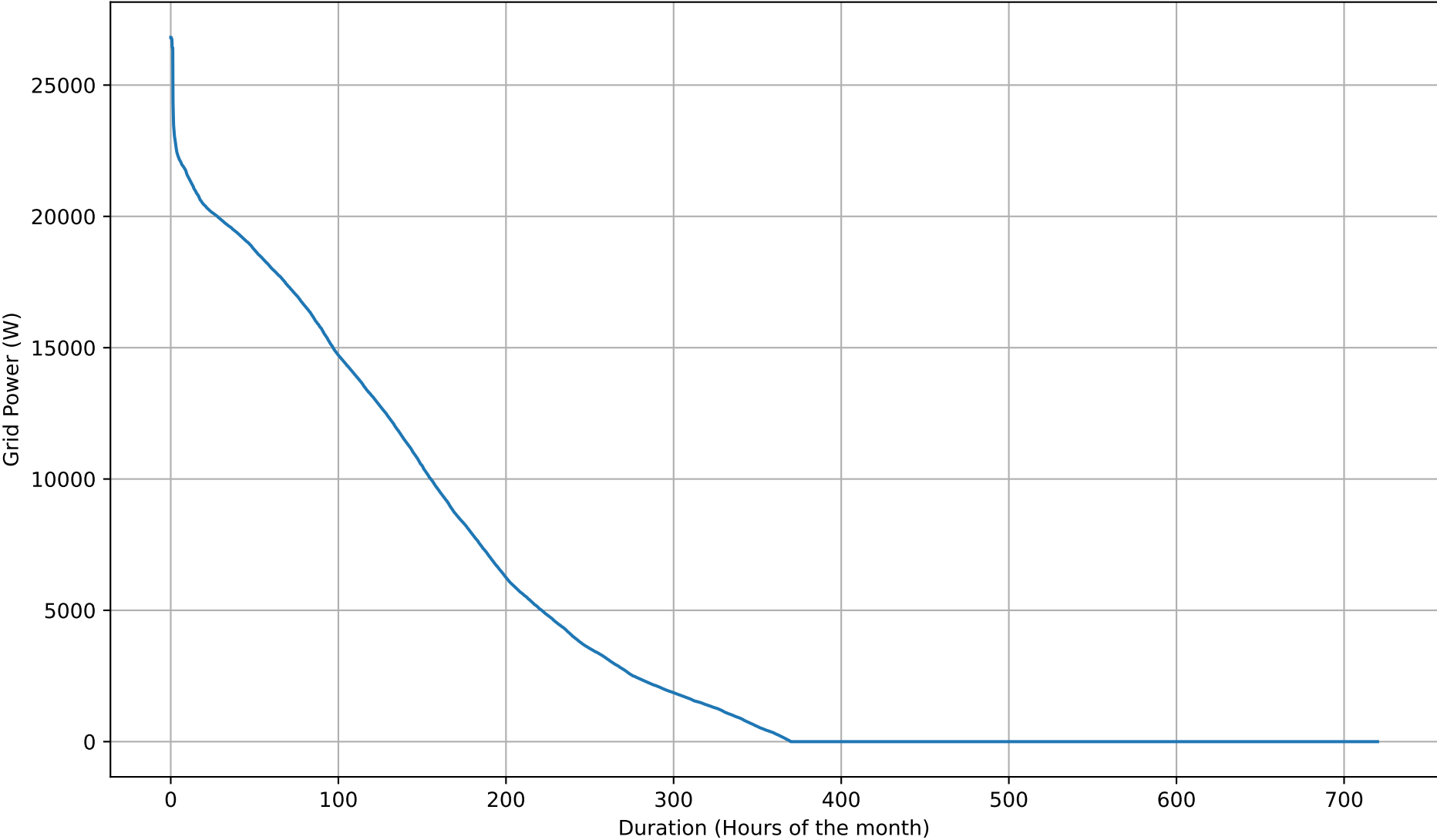
Grid Export Duration Curve - 15kWh - Jun
