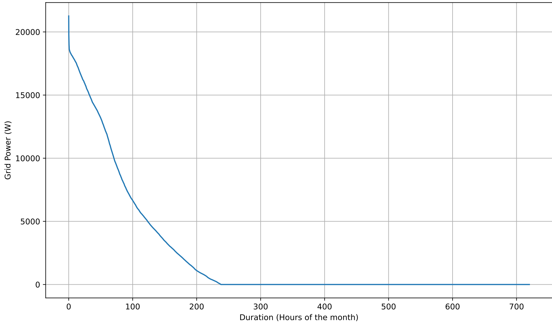
Grid Export Duration Curve - 15kWh - Sep
