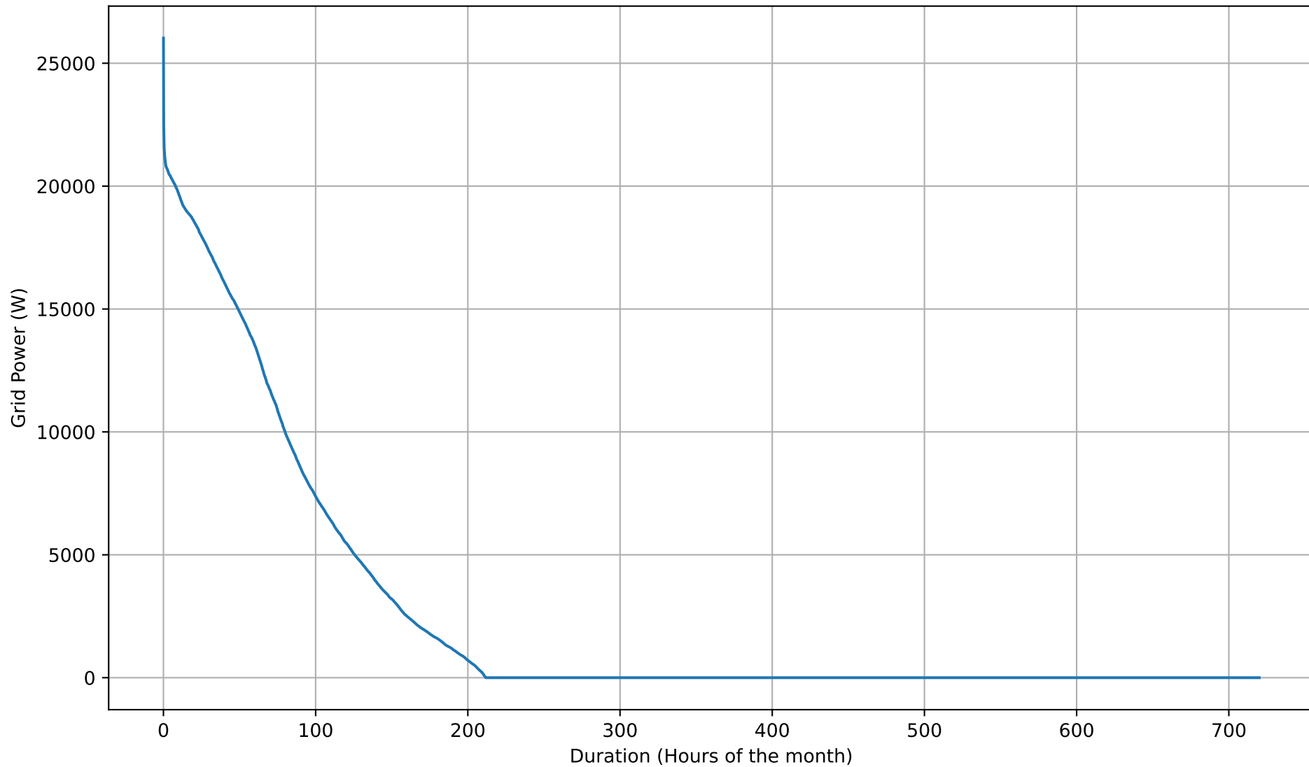
Grid Export Duration Curve - 15kWh - Apr
