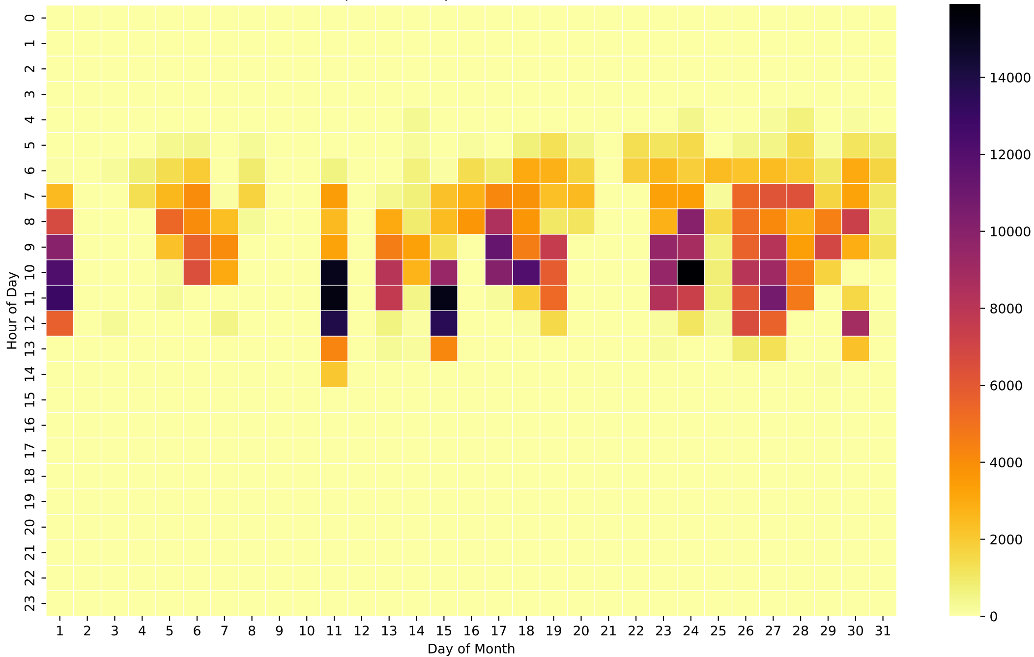
Grid Export Heatmap (Wh/Hour) - 15kWh - Mar
