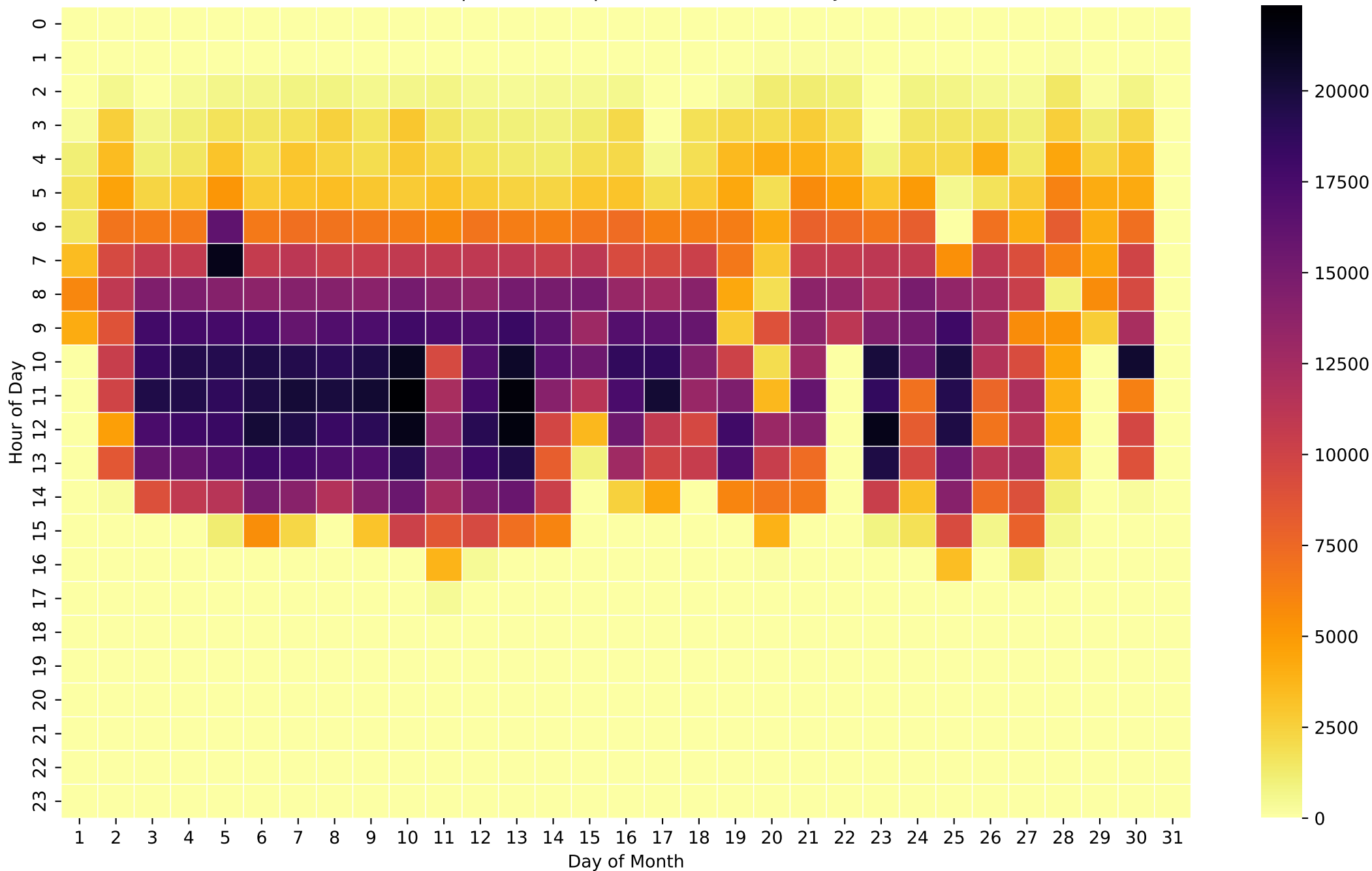
Grid Export Heatmap (Wh/Hour) - 15kWh - Jun
