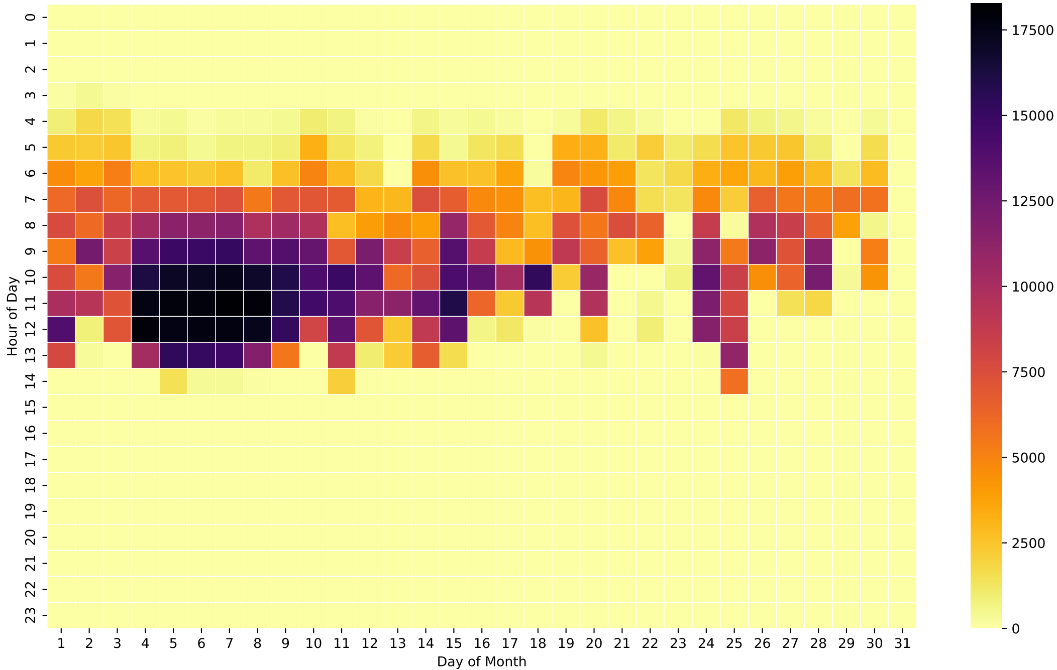
Grid Export Heatmap (Wh/Hour) - 15kWh - Sep
