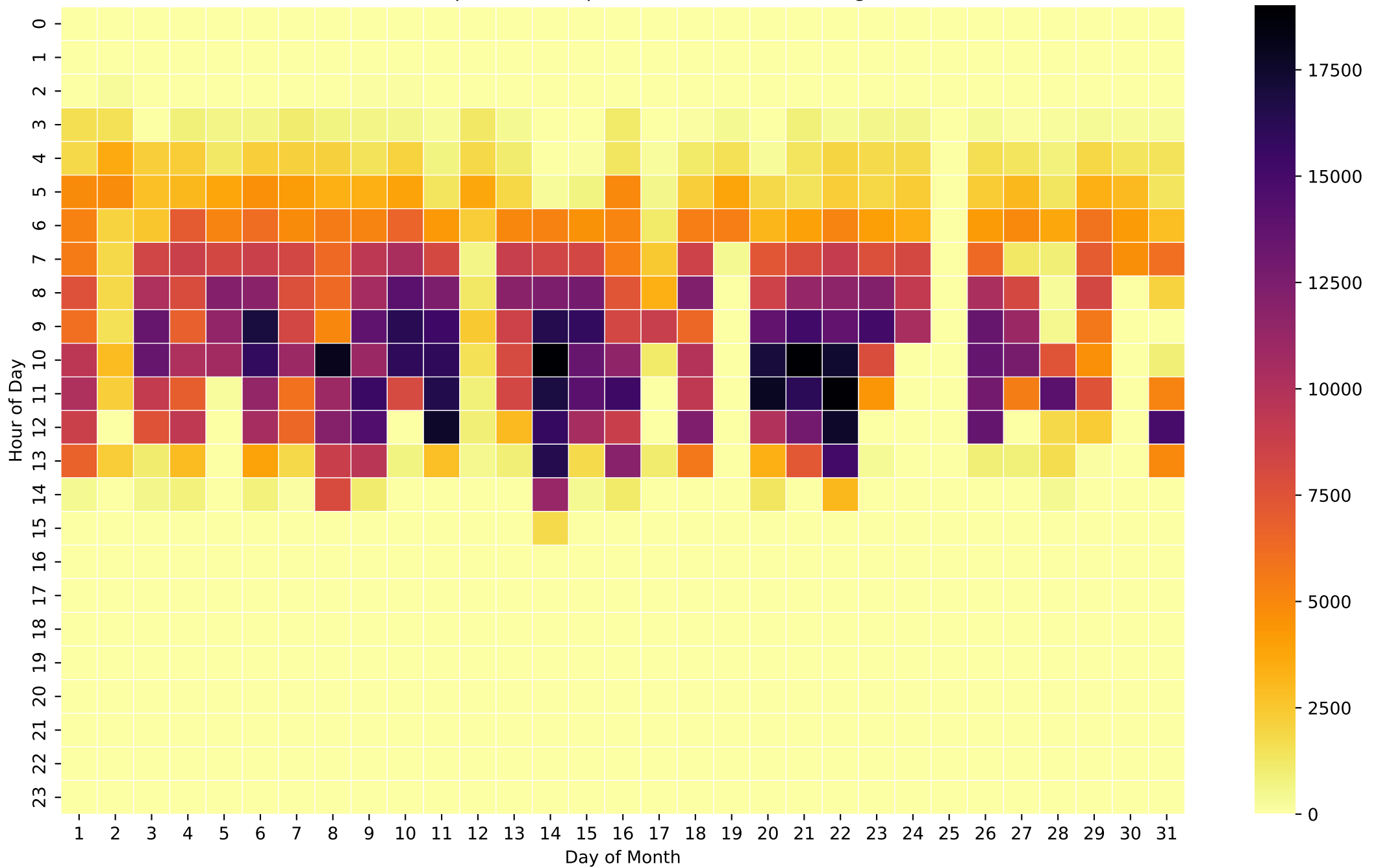
Grid Export Heatmap (Wh/Hour) - 15kWh - Aug
