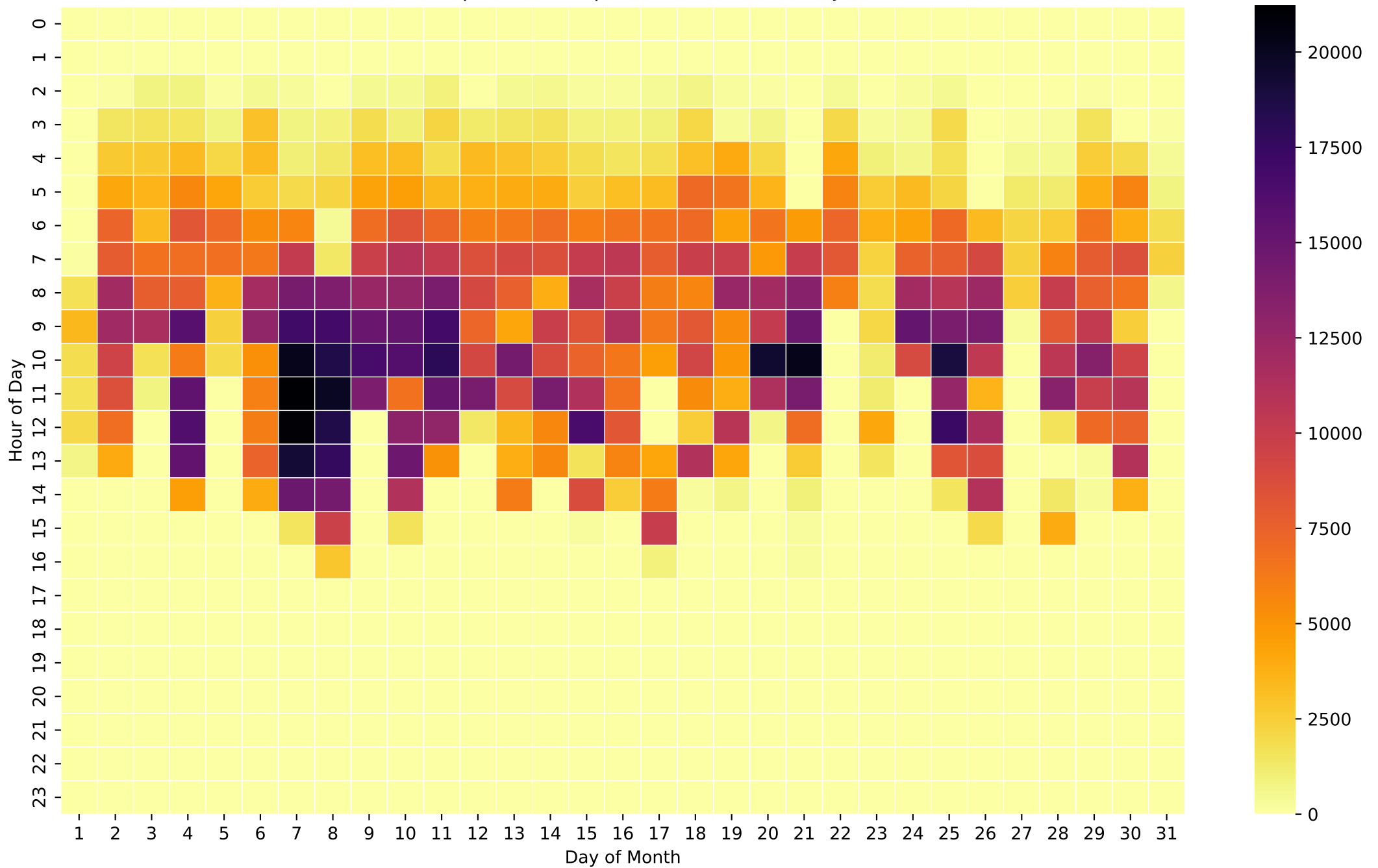
Grid Export Heatmap (Wh/Hour) - 15kWh - Jul
