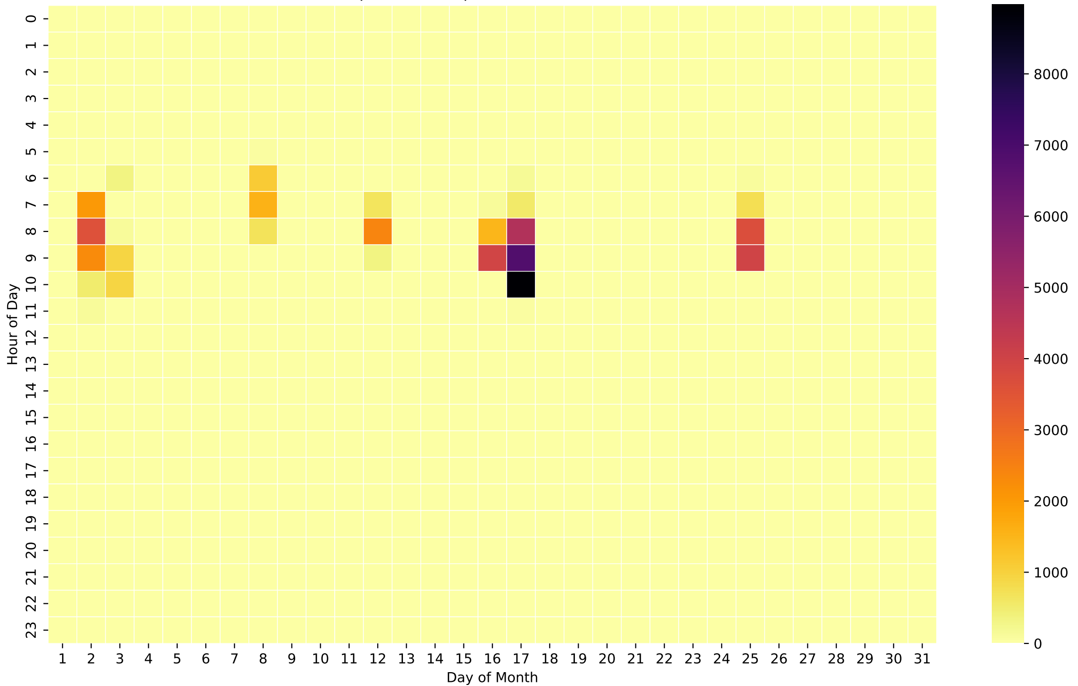
Grid Export Heatmap (Wh/Hour) - 15kWh - Nov
