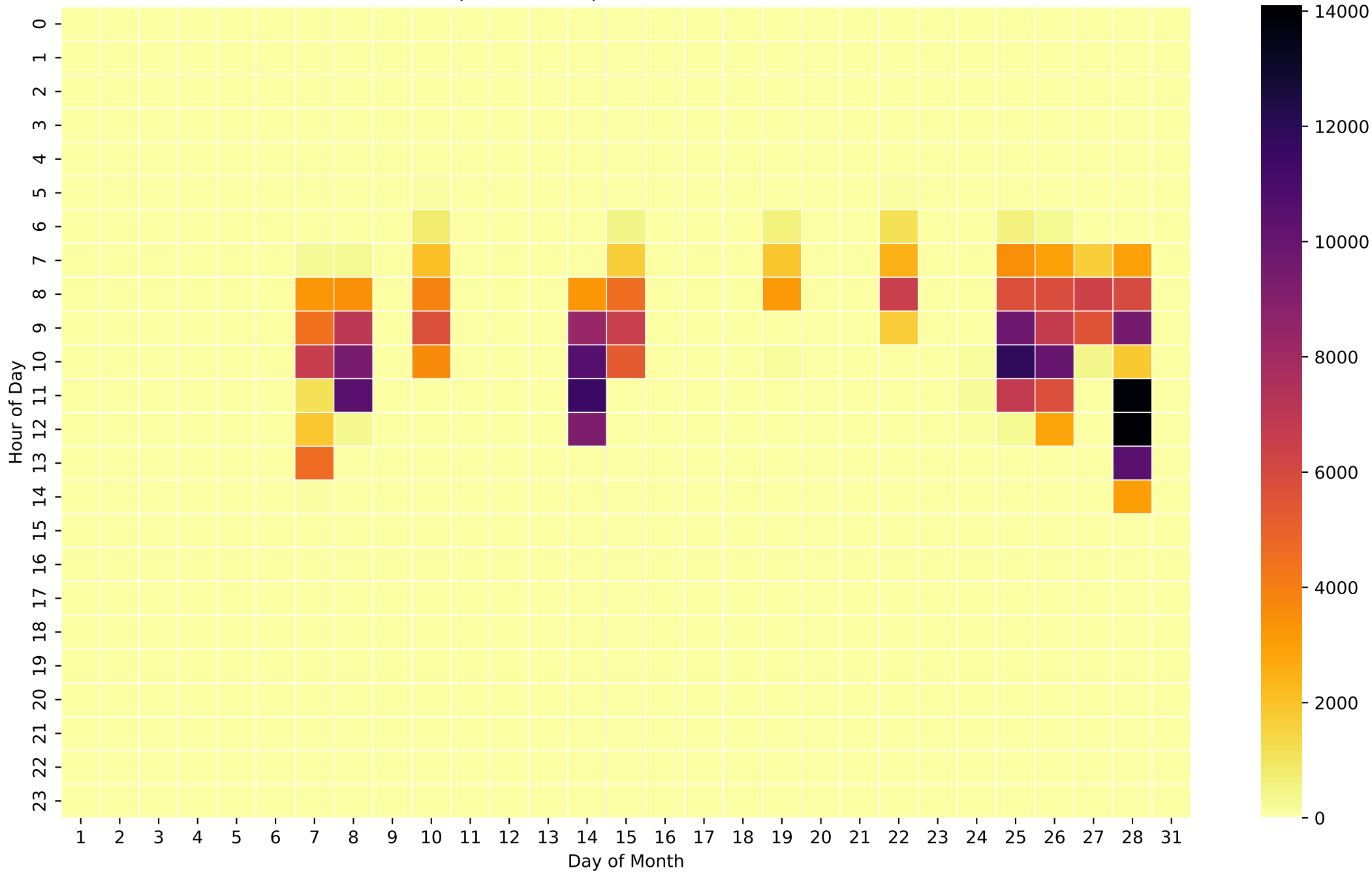
Grid Export Heatmap (Wh/Hour) - 15kWh - Feb
