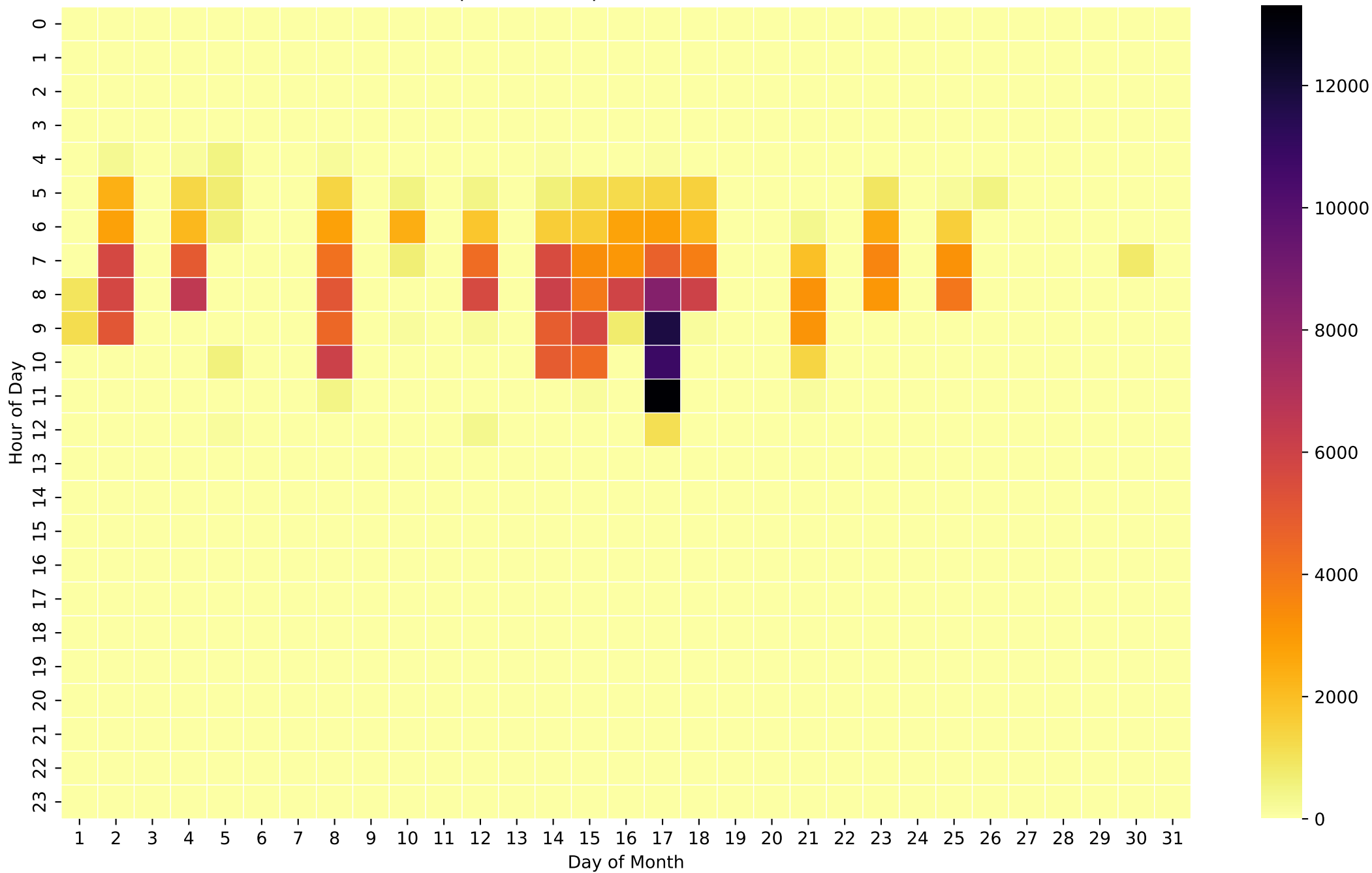
Grid Export Heatmap (Wh/Hour) - 15kWh - Oct
