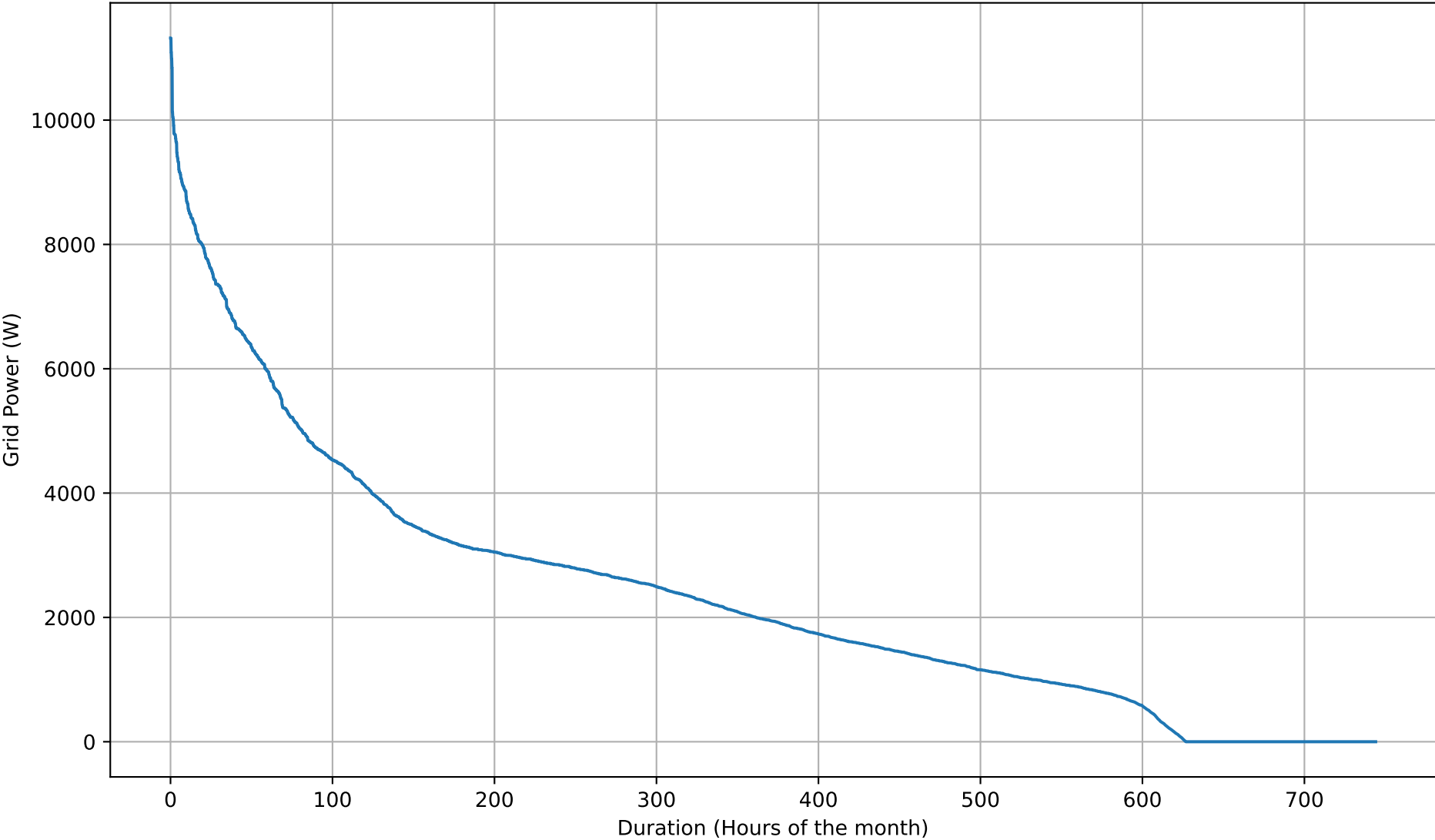
Grid Import Duration Curve - 15kWh - Jan
