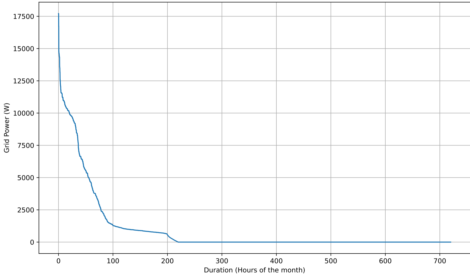
Grid Import Duration Curve - 15kWh - Sep
