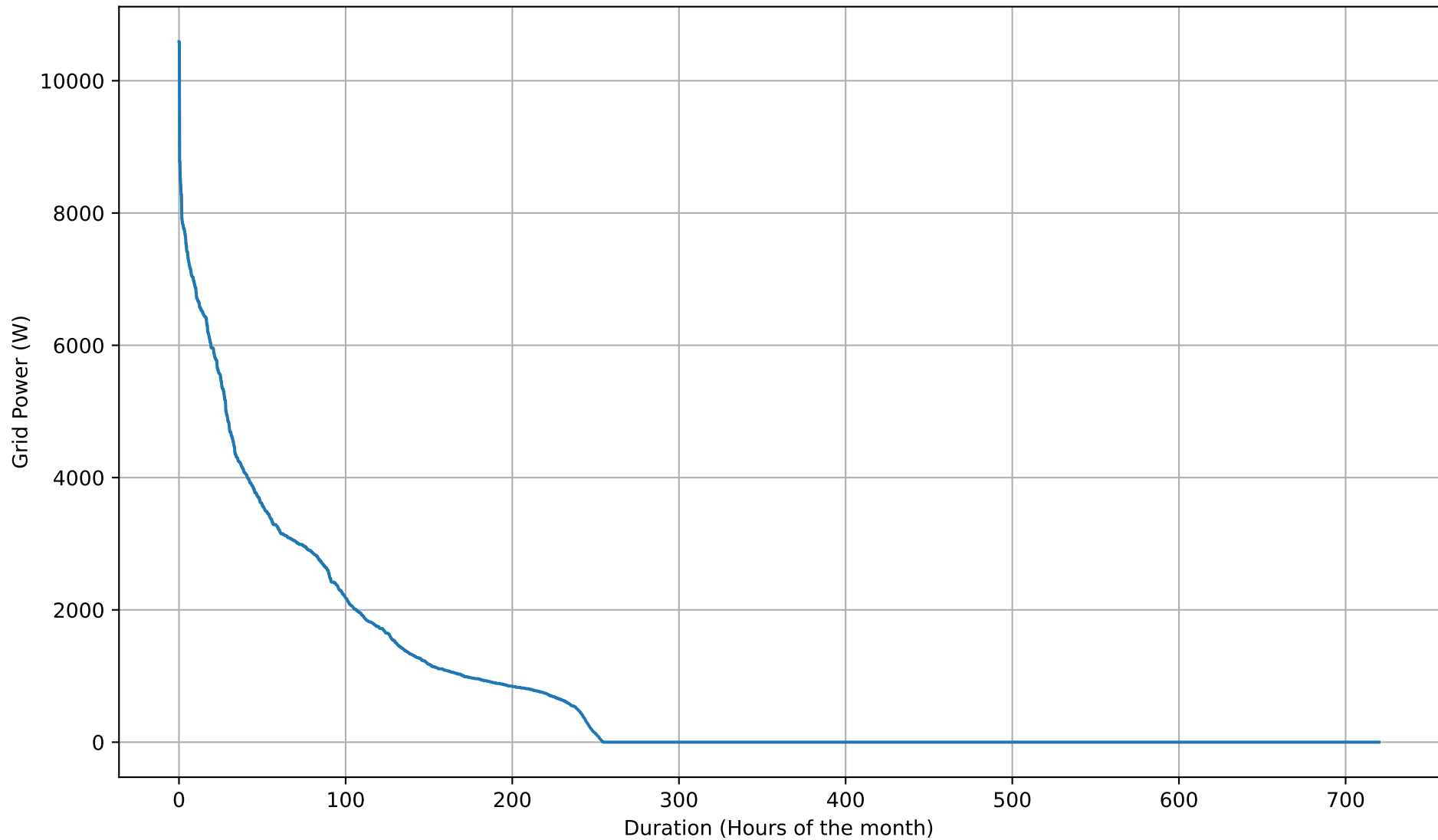
Grid Import Duration Curve - 15kWh - Apr
