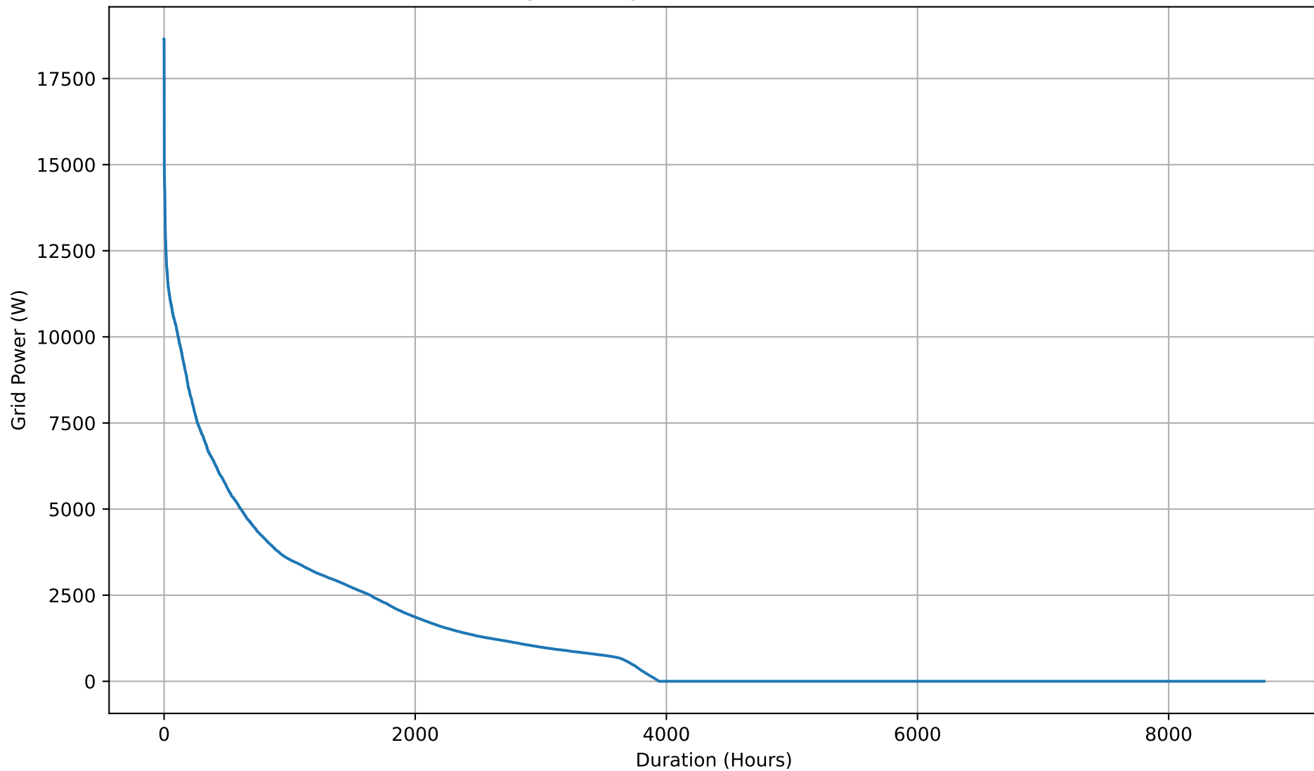
Yearly Grid Import Duration Curve - 15kWh
