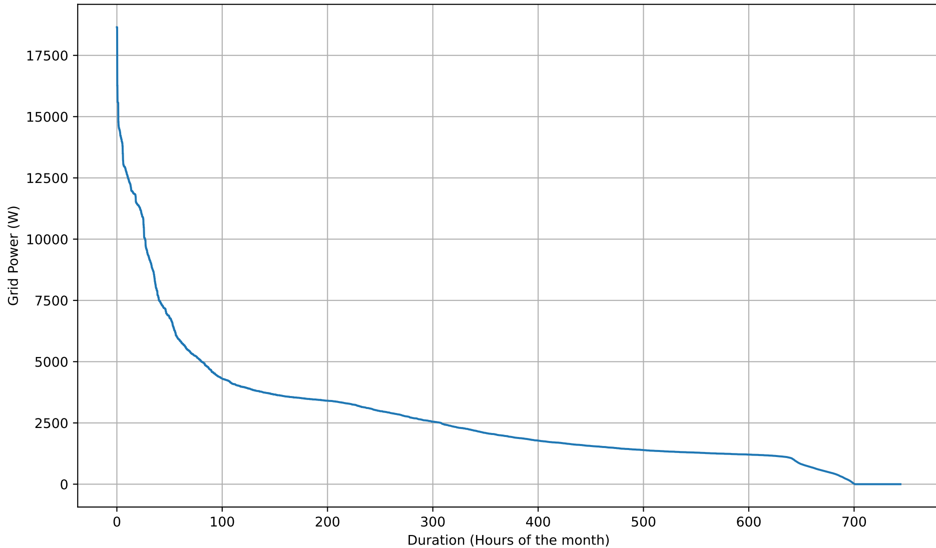
Grid Import Duration Curve - 15kWh - Dec
