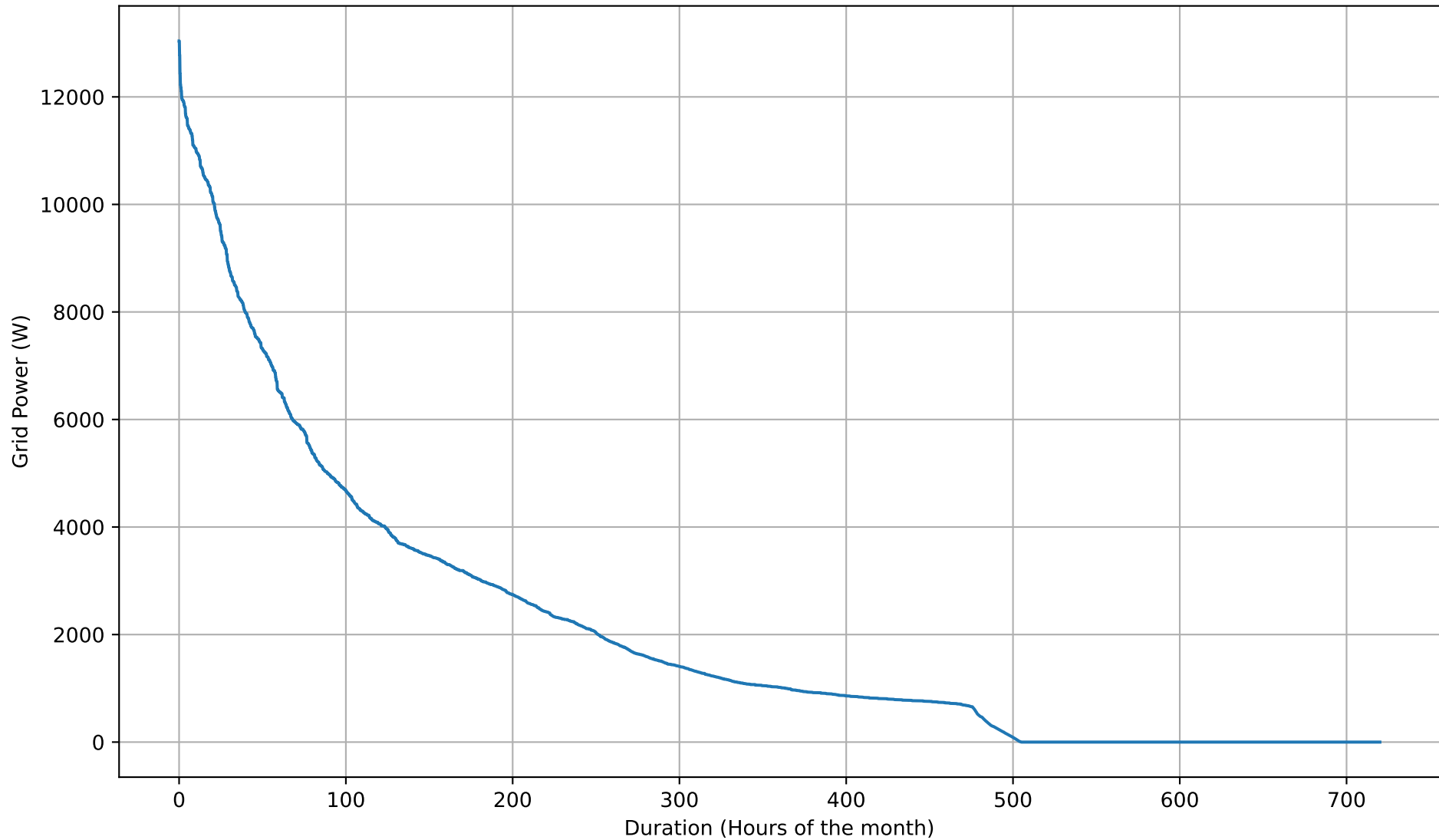
Grid Import Duration Curve - 15kWh - Nov
