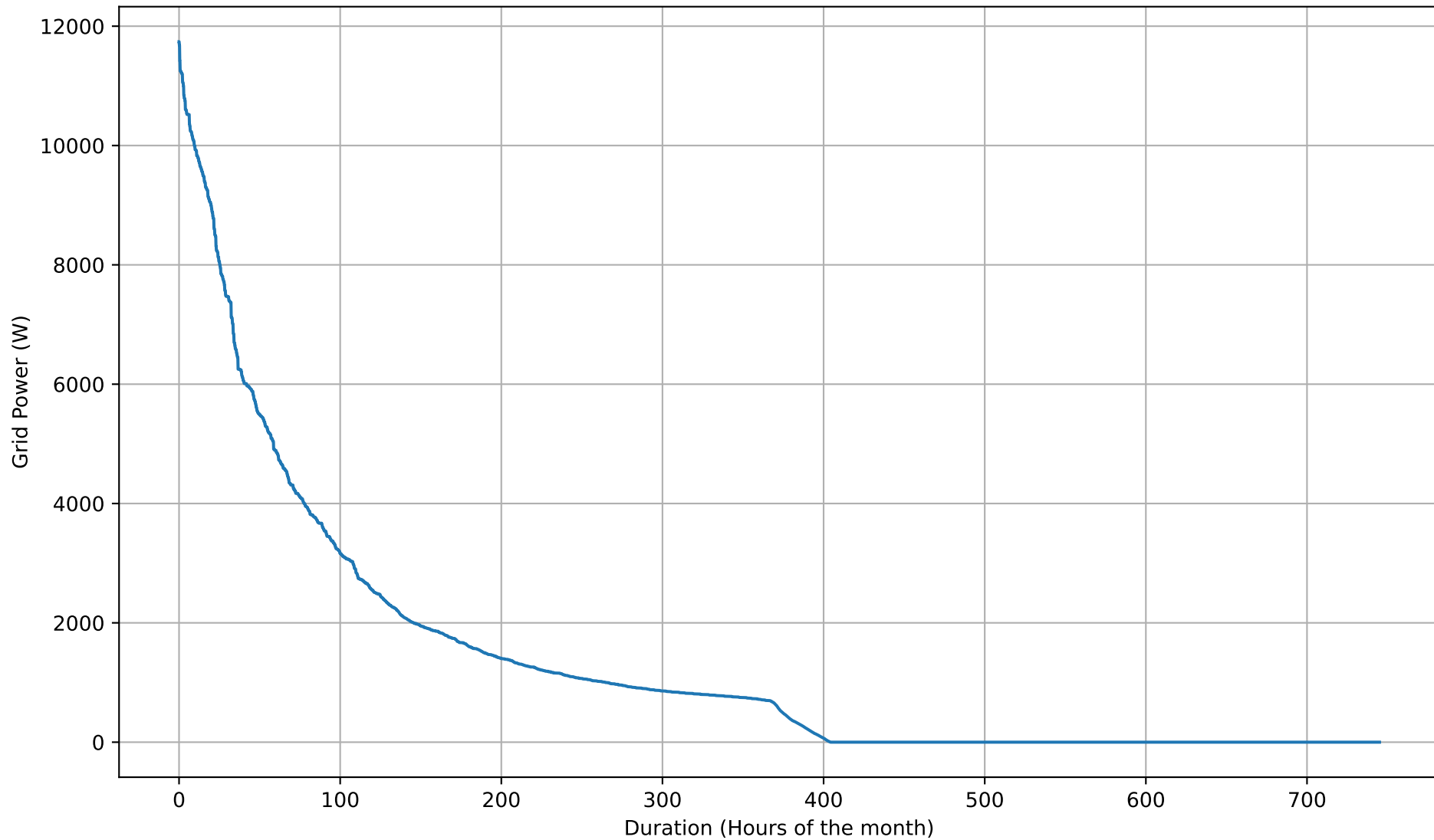
Grid Import Duration Curve - 15kWh - Oct
