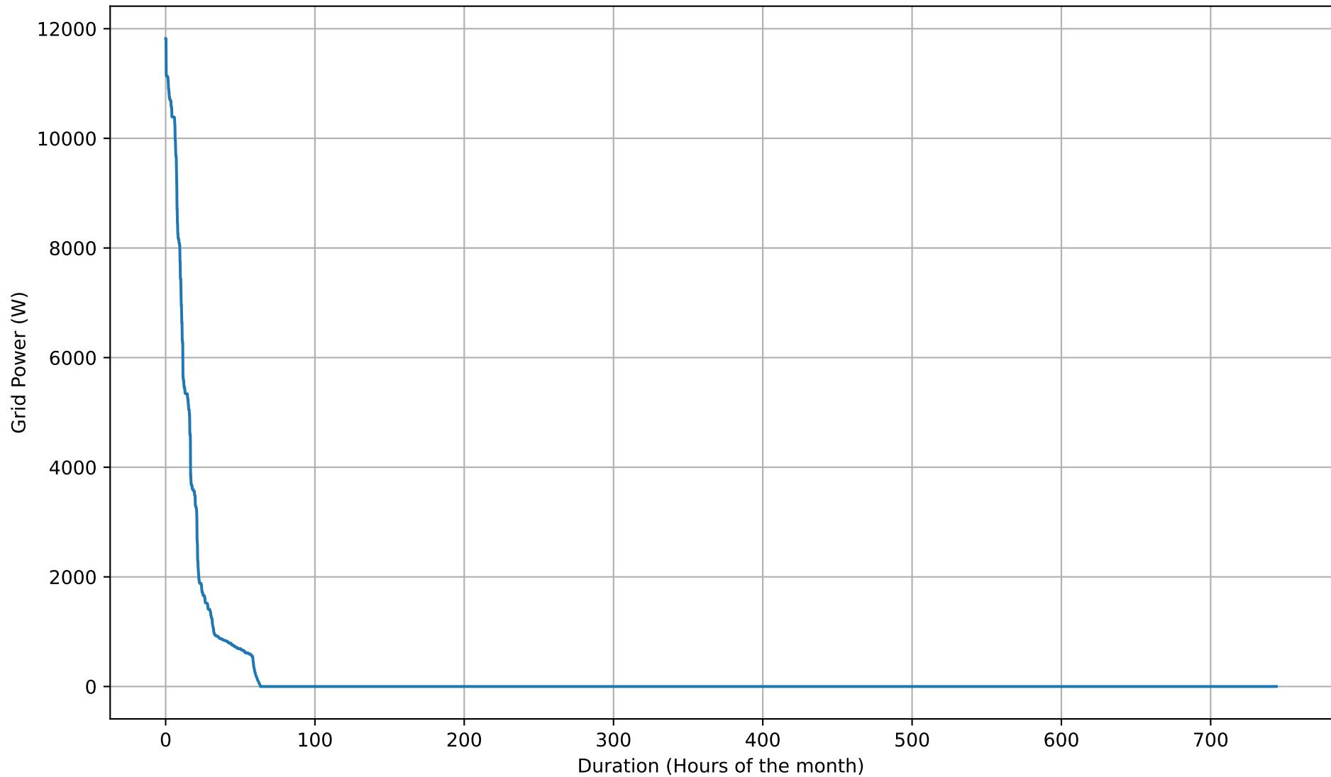
Grid Import Duration Curve - 15kWh - Jul
