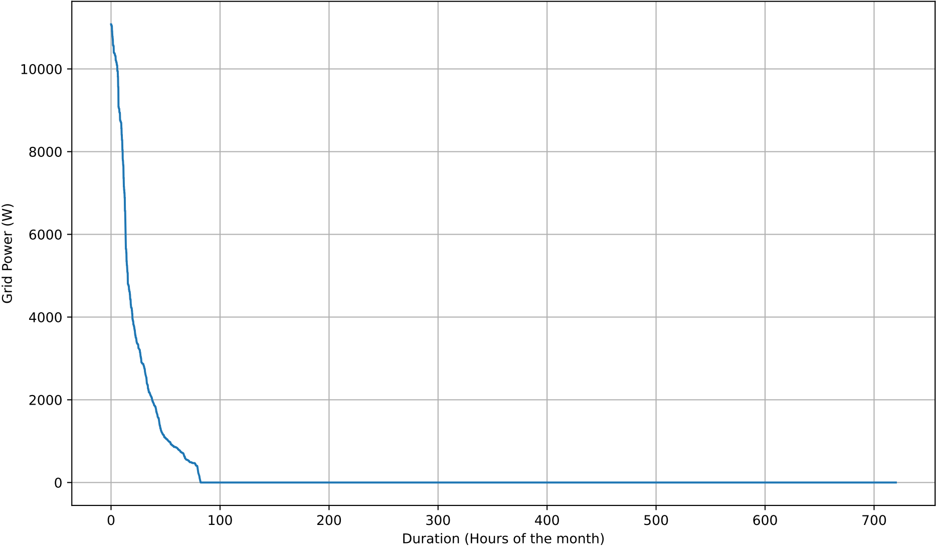
Grid Import Duration Curve - 15kWh - Jun
