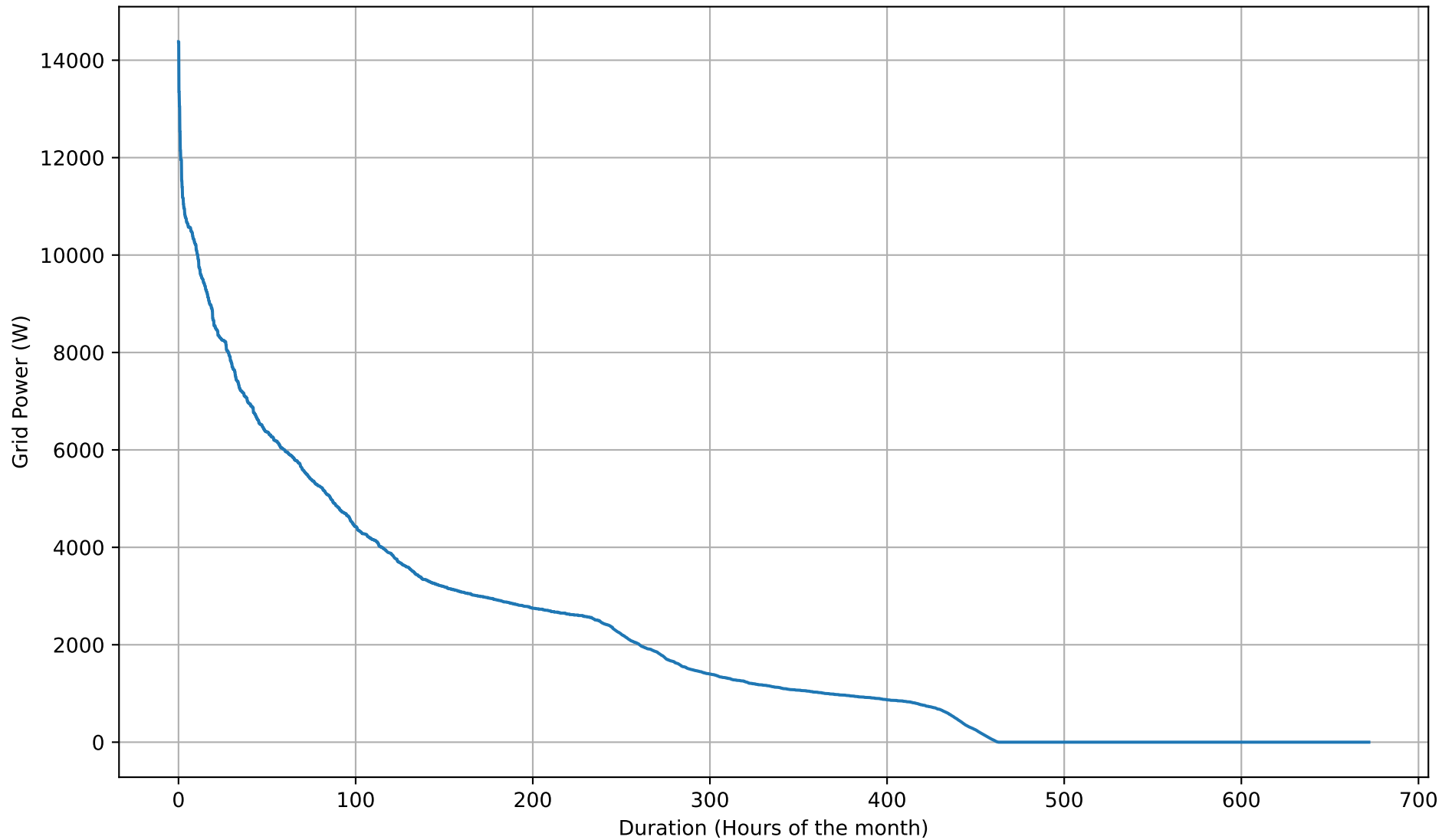
Grid Import Duration Curve - 15kWh - Feb
