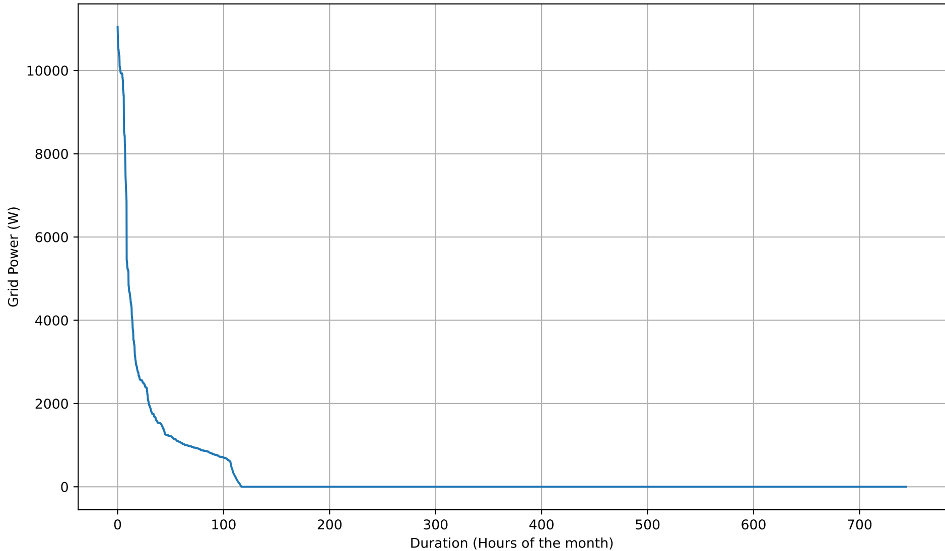
Grid Import Duration Curve - 15kWh - Aug
