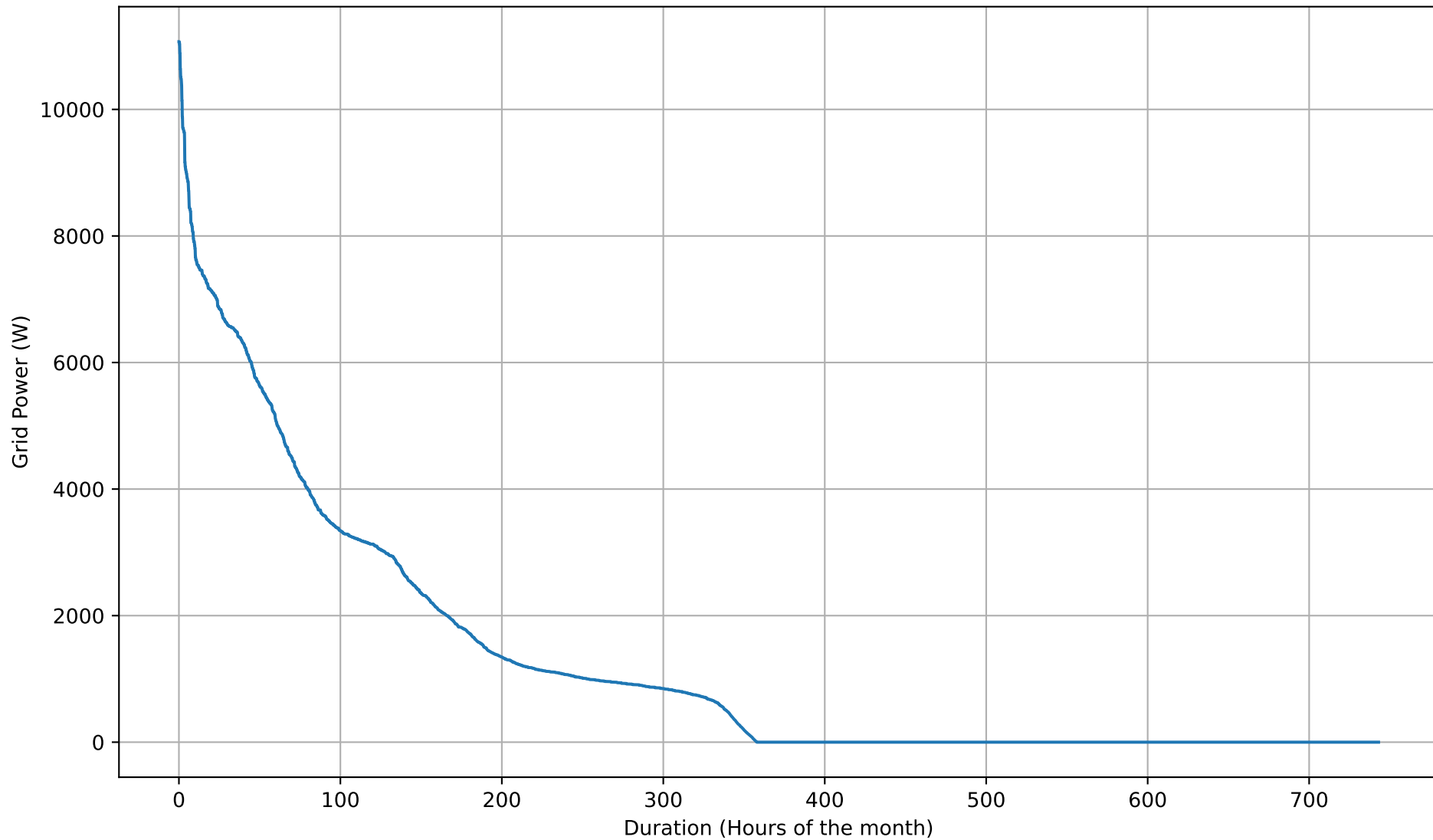
Grid Import Duration Curve - 15kWh - Mar
