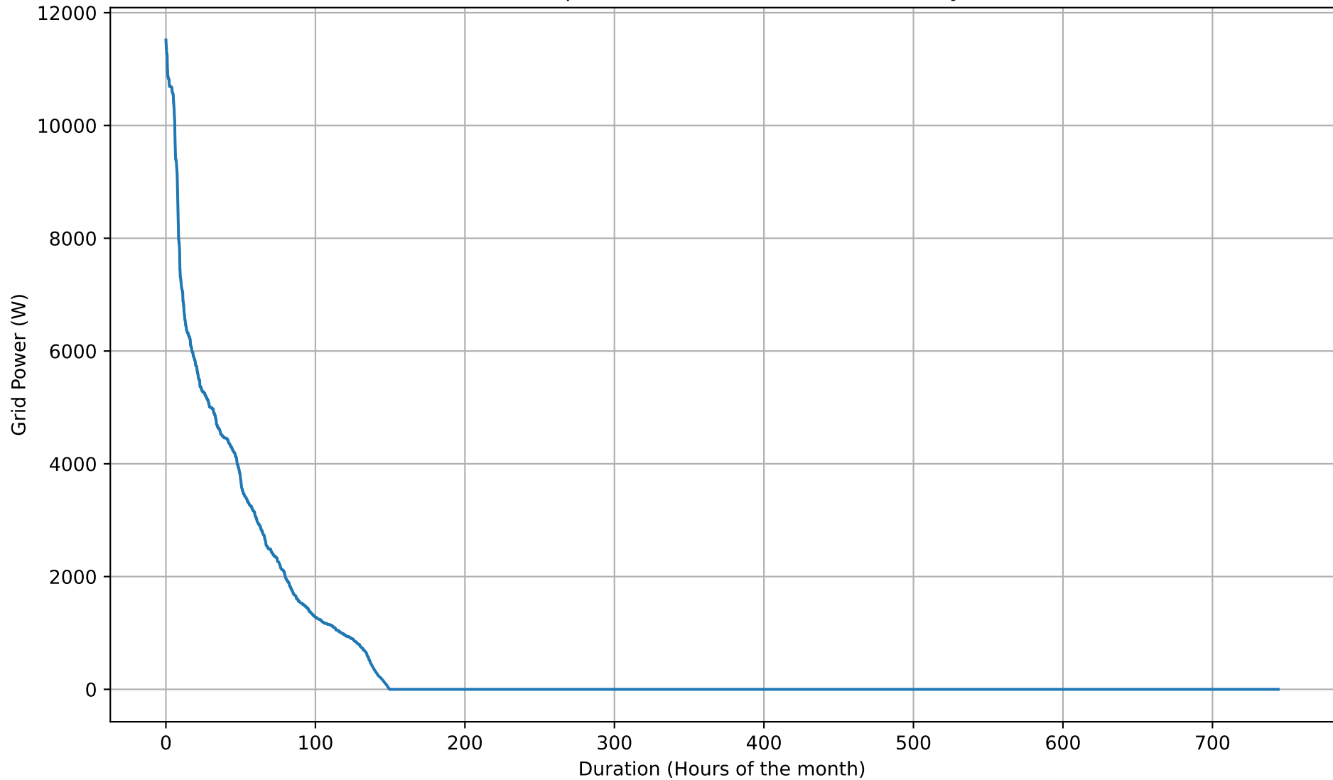
Grid Import Duration Curve - 15kWh - May
