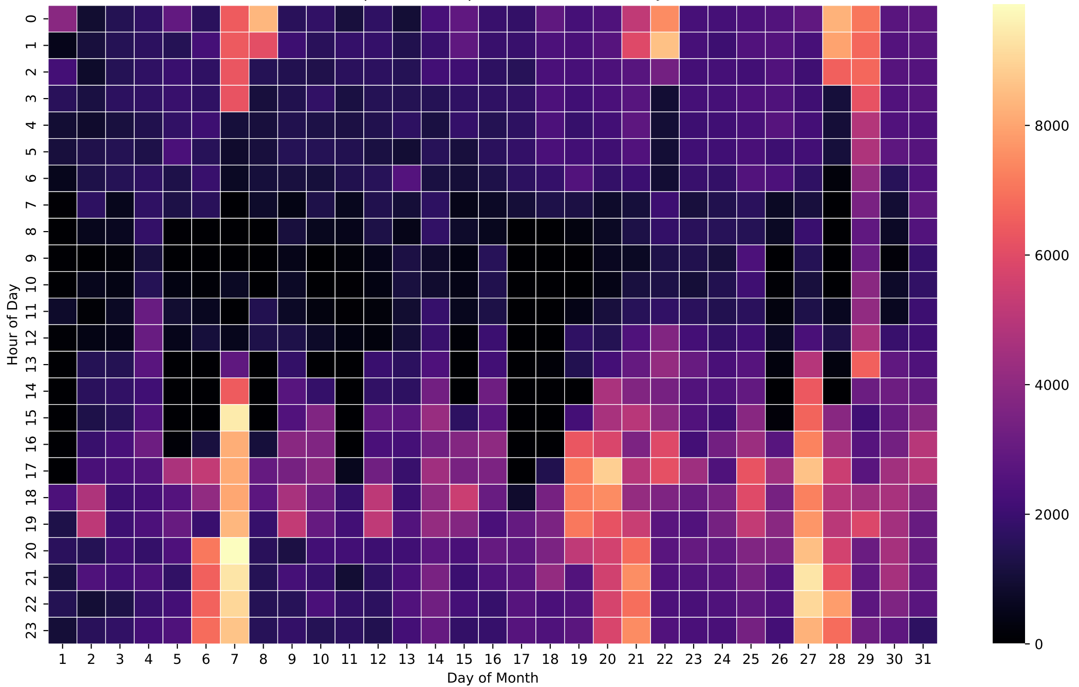
Grid Import Heatmap (Wh/Hour) - 15kWh - Jan
