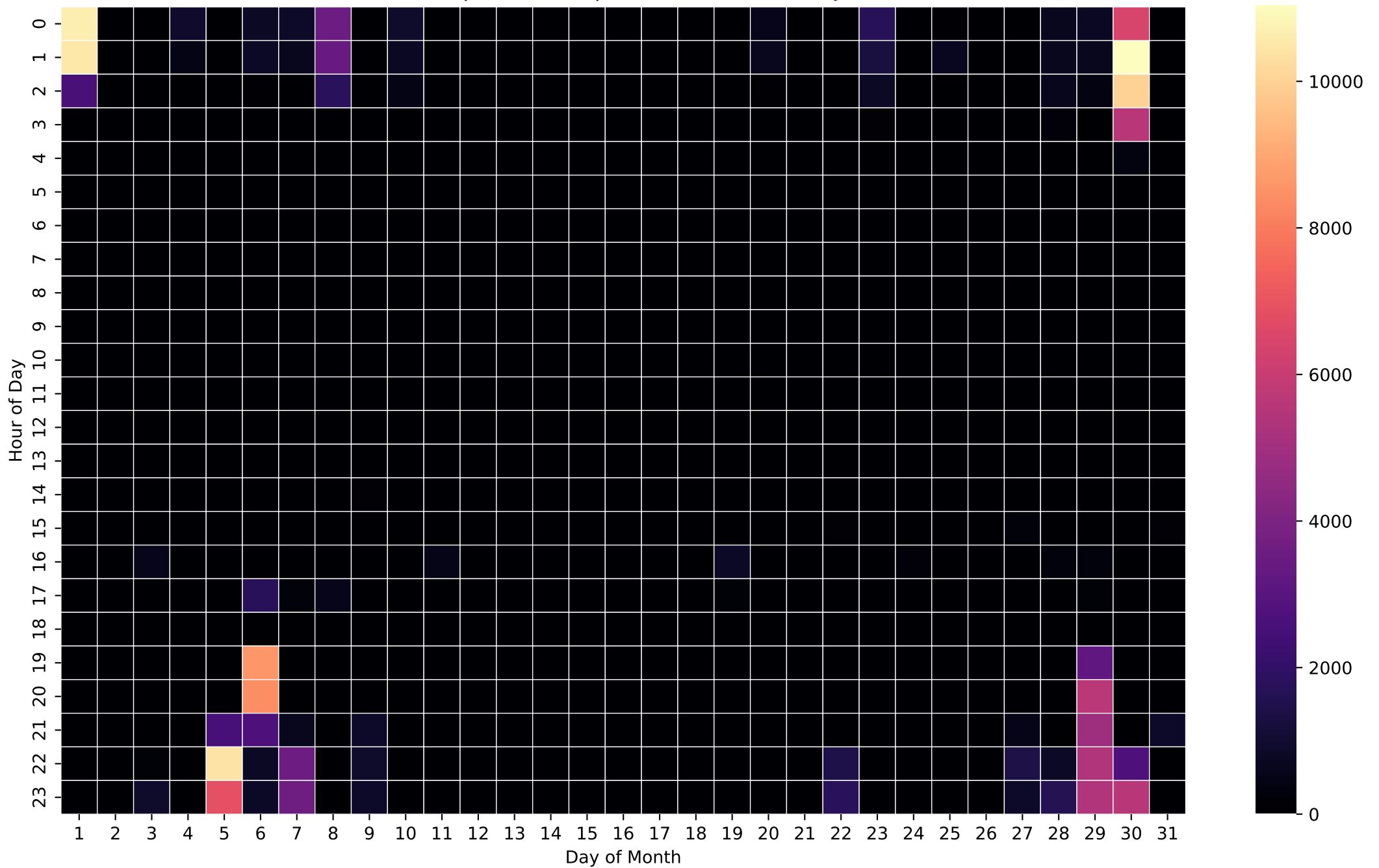
Grid Import Heatmap (Wh/Hour) - 15kWh - Jul
