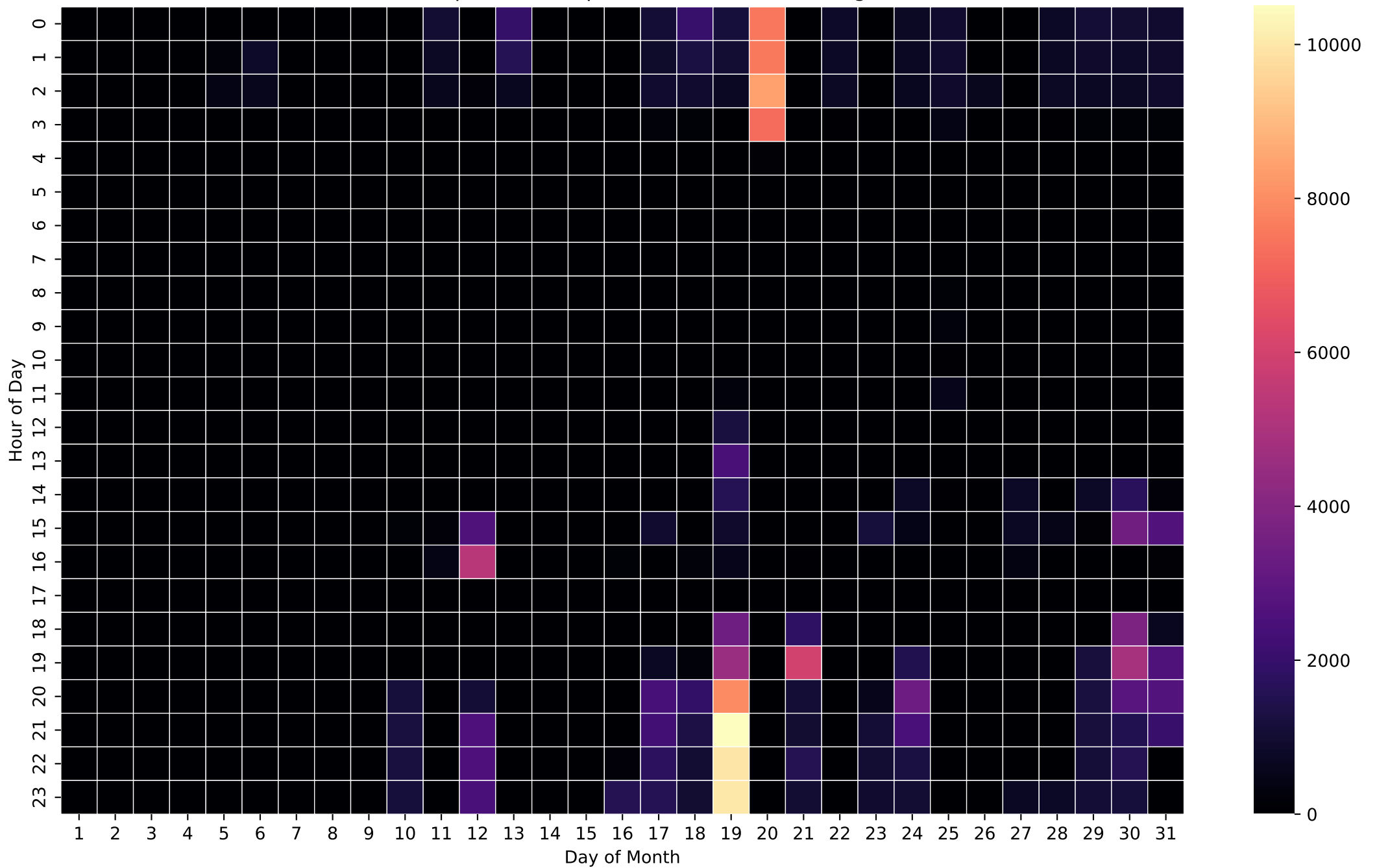
Grid Import Heatmap (Wh/Hour) - 15kWh - Aug
