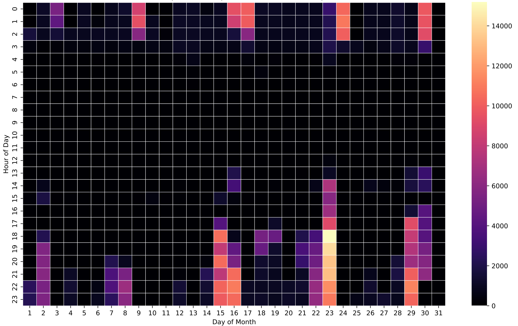
Grid Import Heatmap (Wh/Hour) - 15kWh - Sep
