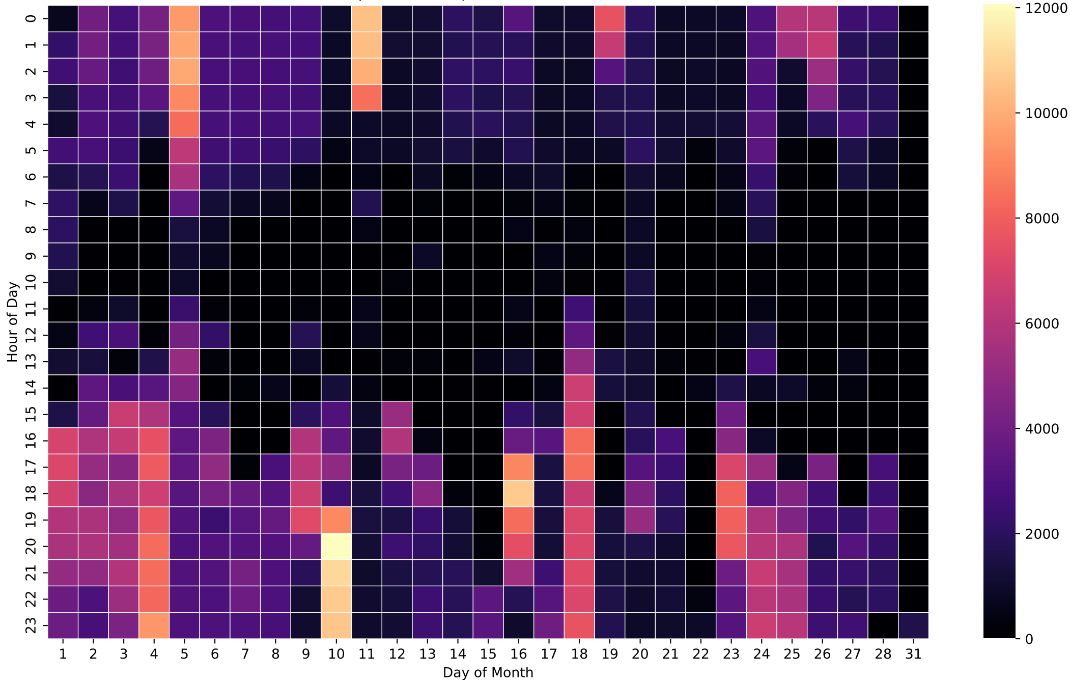
Grid Import Heatmap (Wh/Hour) - 15kWh - Feb
