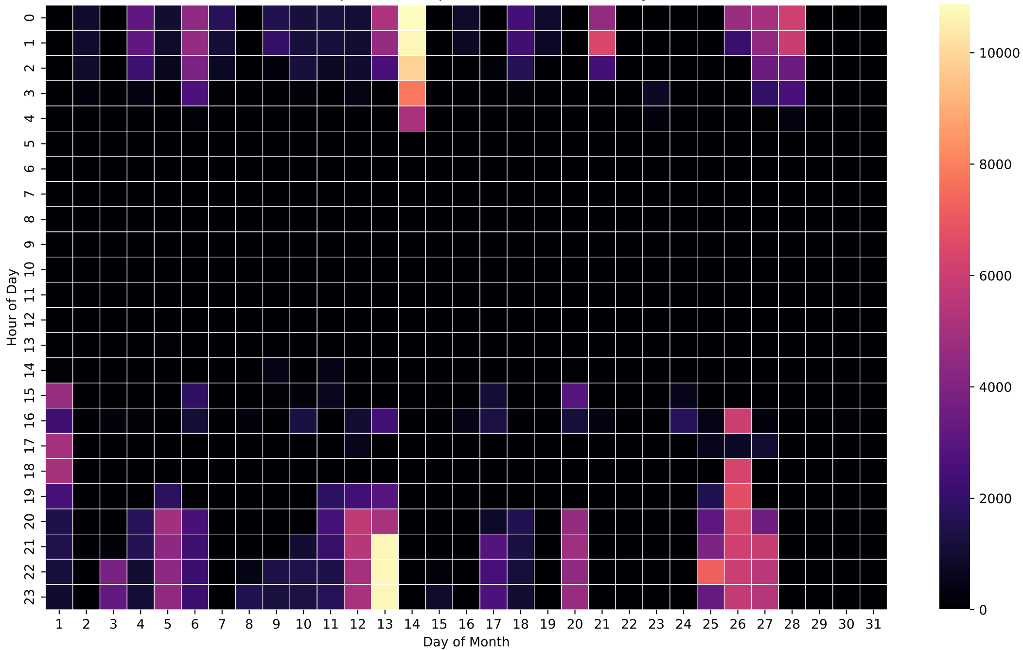
Grid Import Heatmap (Wh/Hour) - 15kWh - May
