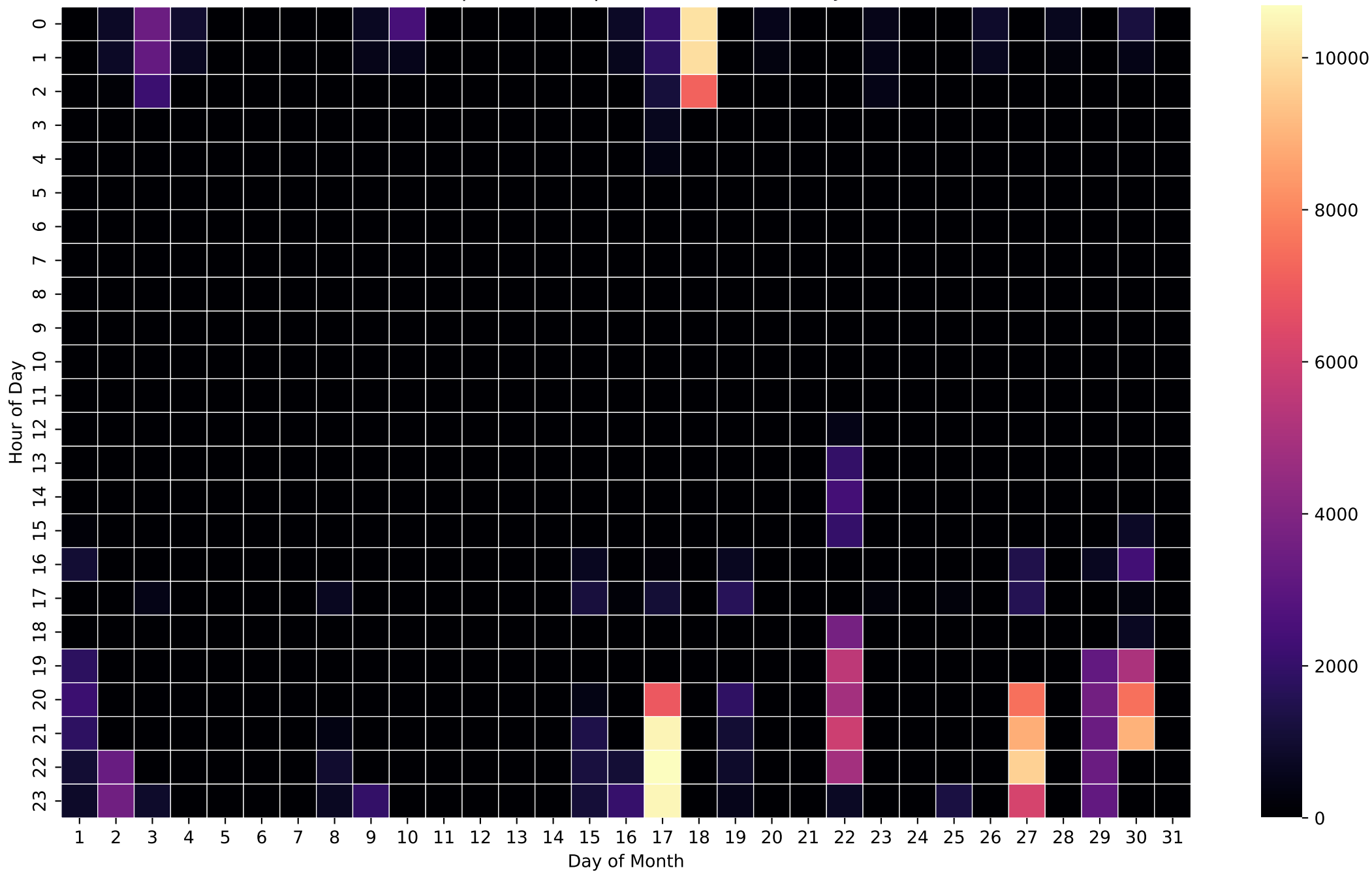
Grid Import Heatmap (Wh/Hour) - 15kWh - Jun
