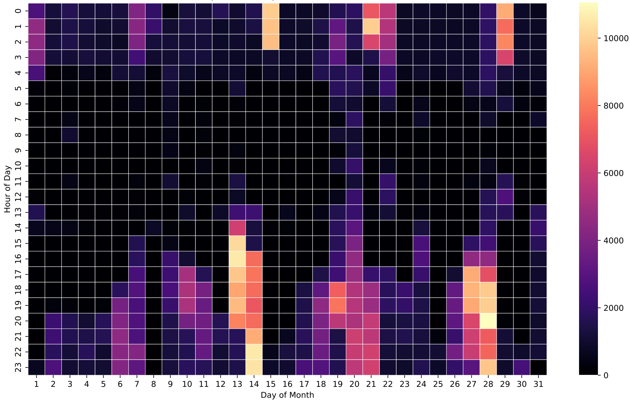
Grid Import Heatmap (Wh/Hour) - 15kWh - Oct
