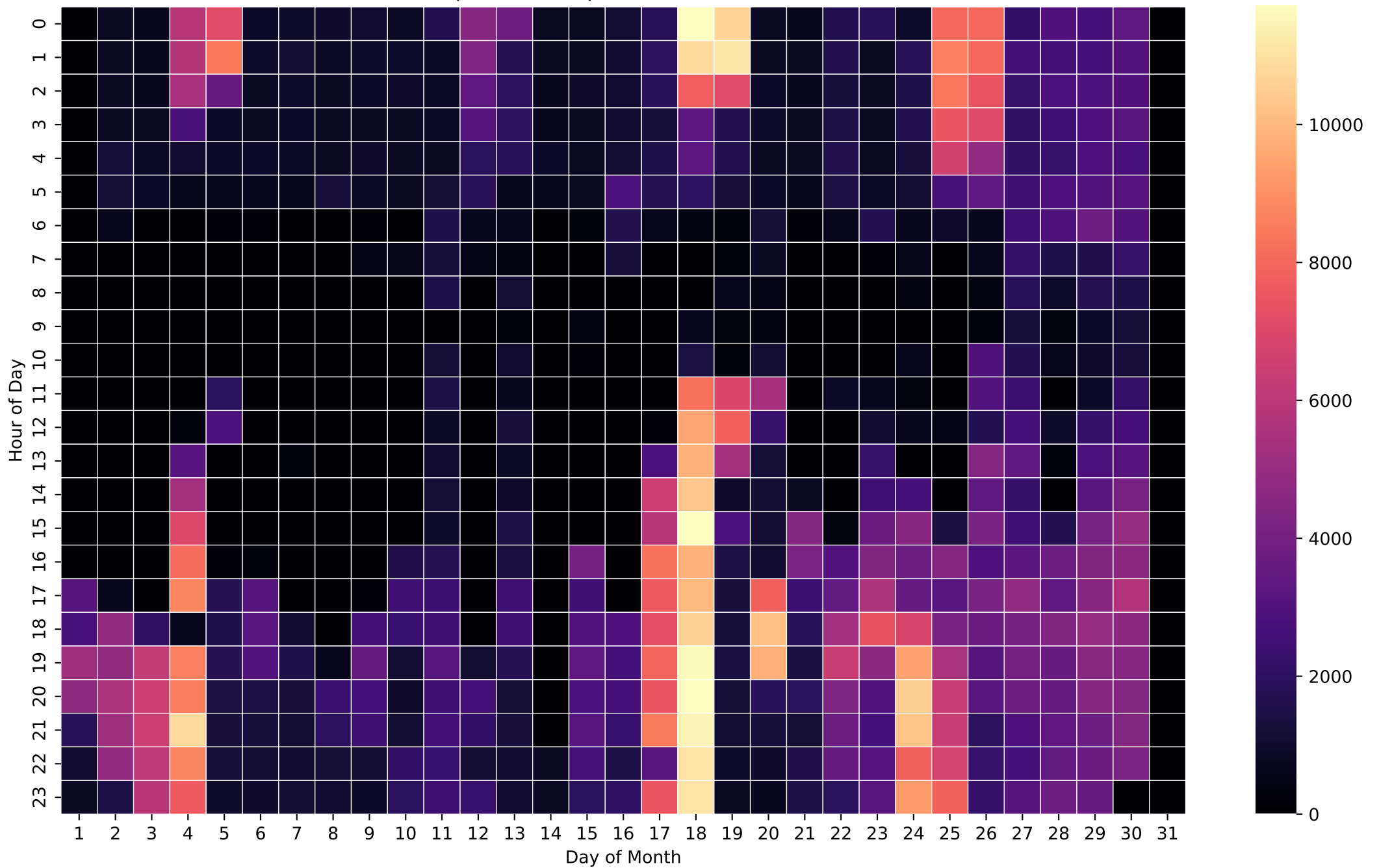
Grid Import Heatmap (Wh/Hour) - 15kWh - Nov
