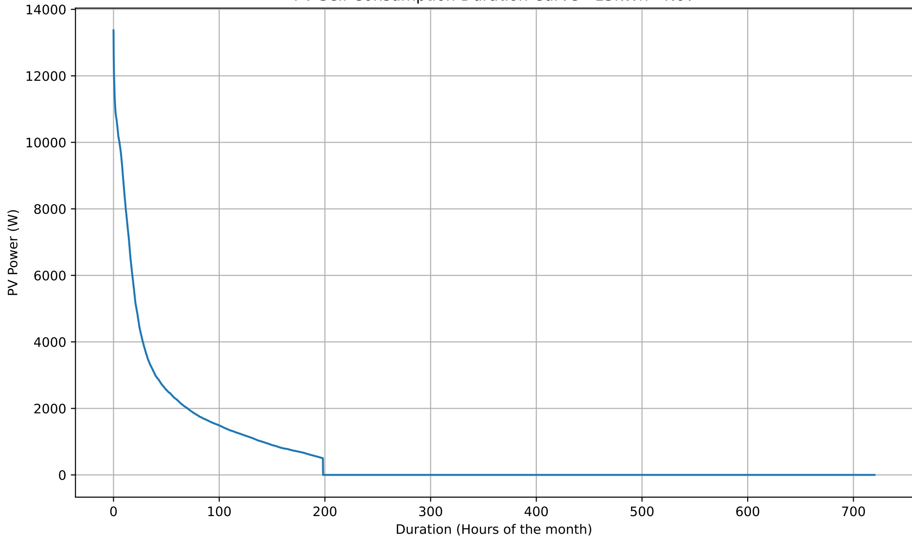
PV Self-Consumption Duration Curve - 15kWh - Nov
