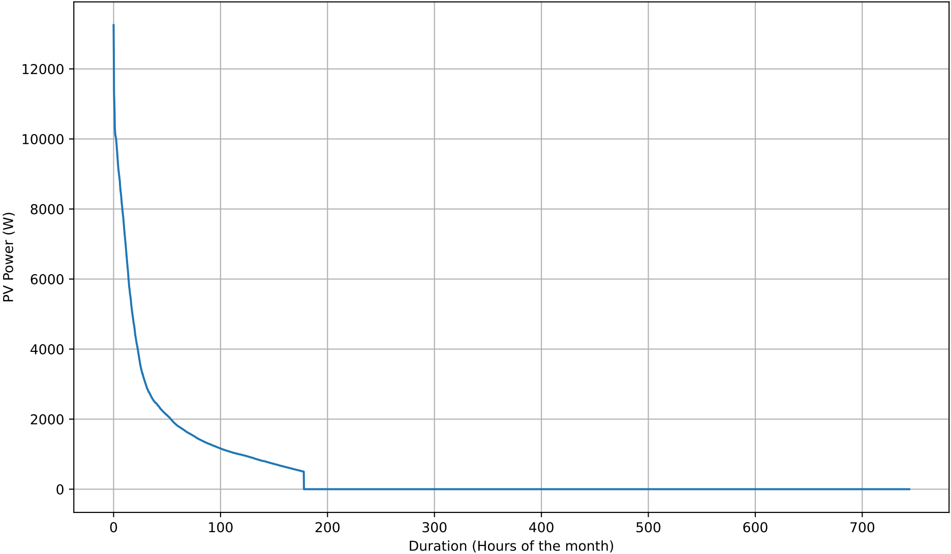
PV Self-Consumption Duration Curve - 15kWh - Jan
