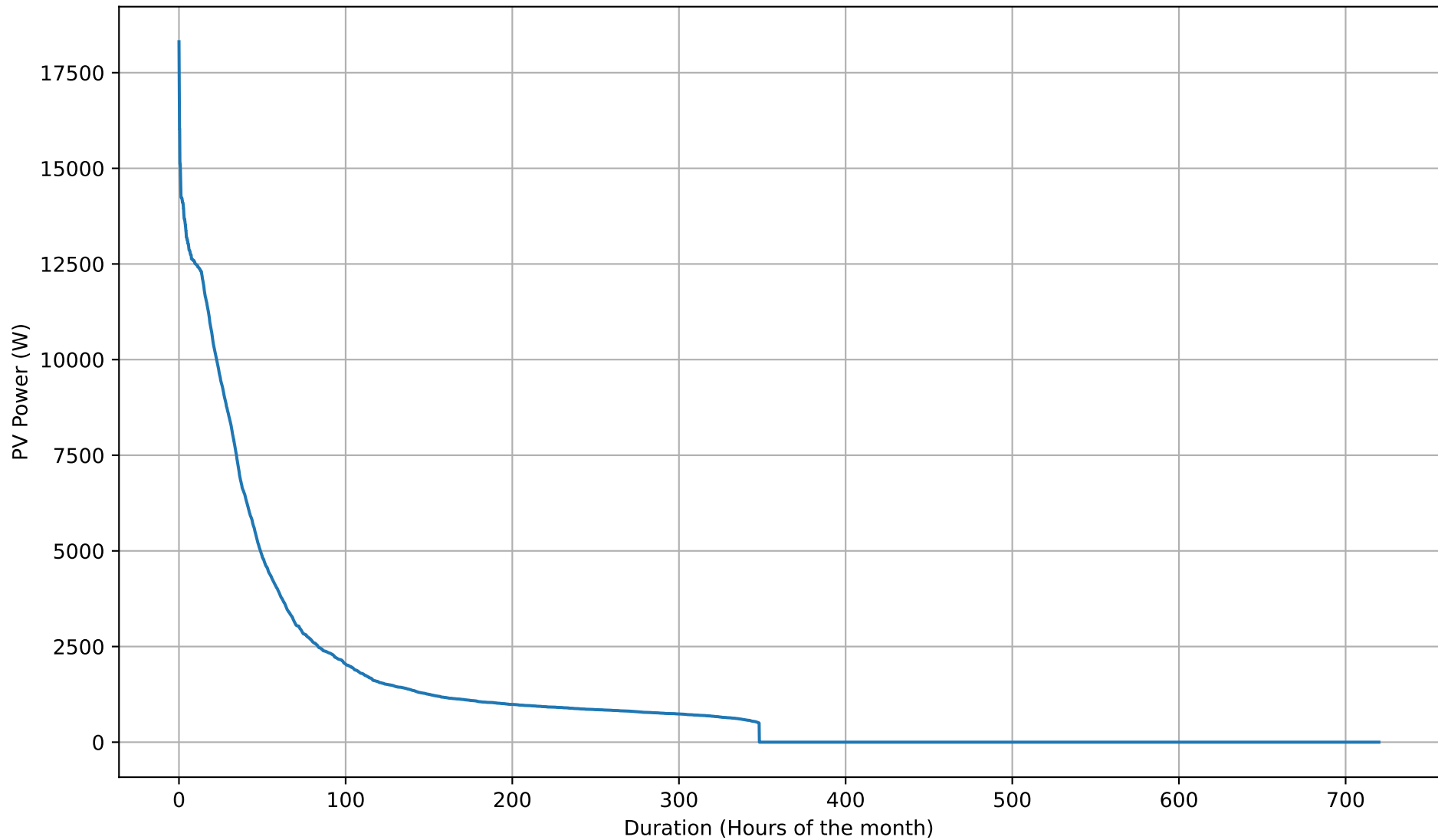
PV Self-Consumption Duration Curve - 15kWh - Sep
