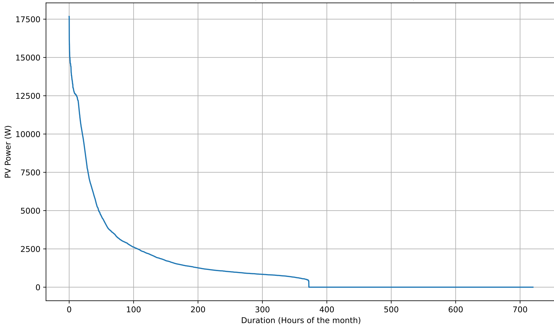
PV Self-Consumption Duration Curve - 15kWh - Apr
