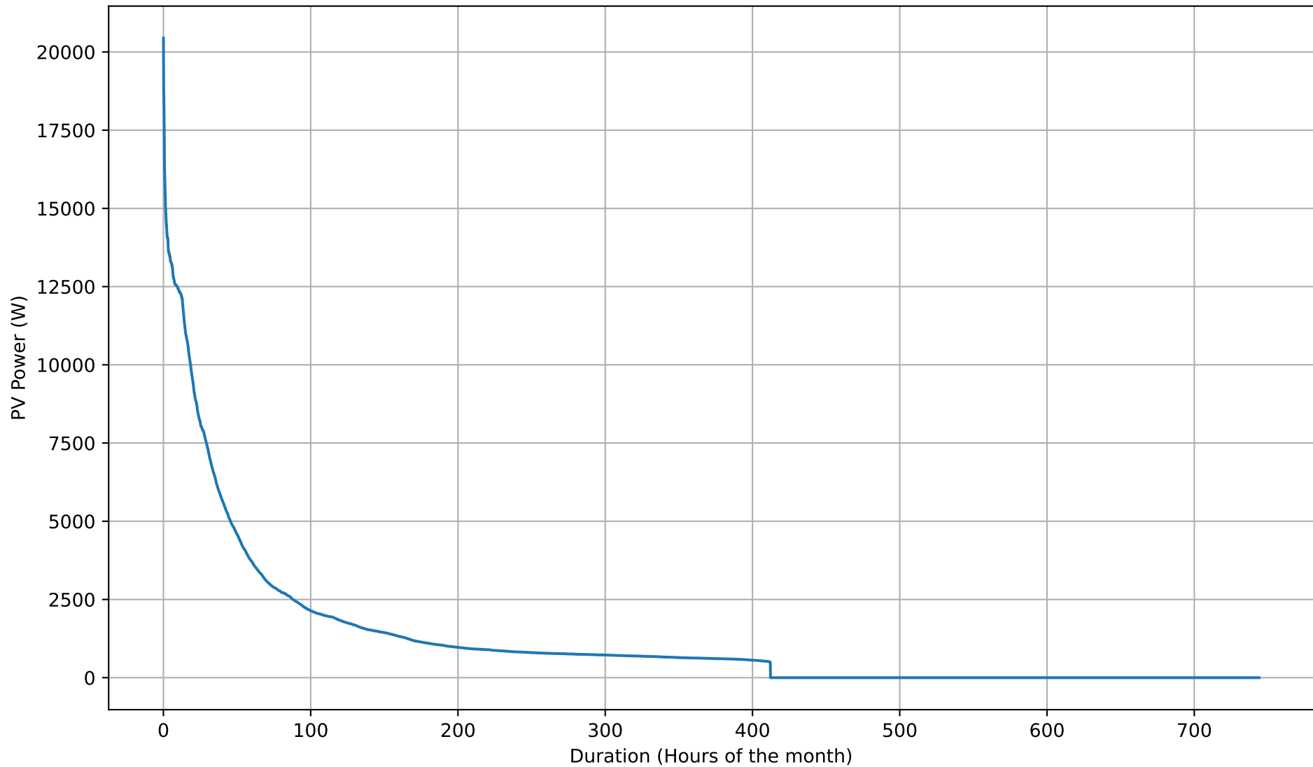
PV Self-Consumption Duration Curve - 15kWh - Aug
