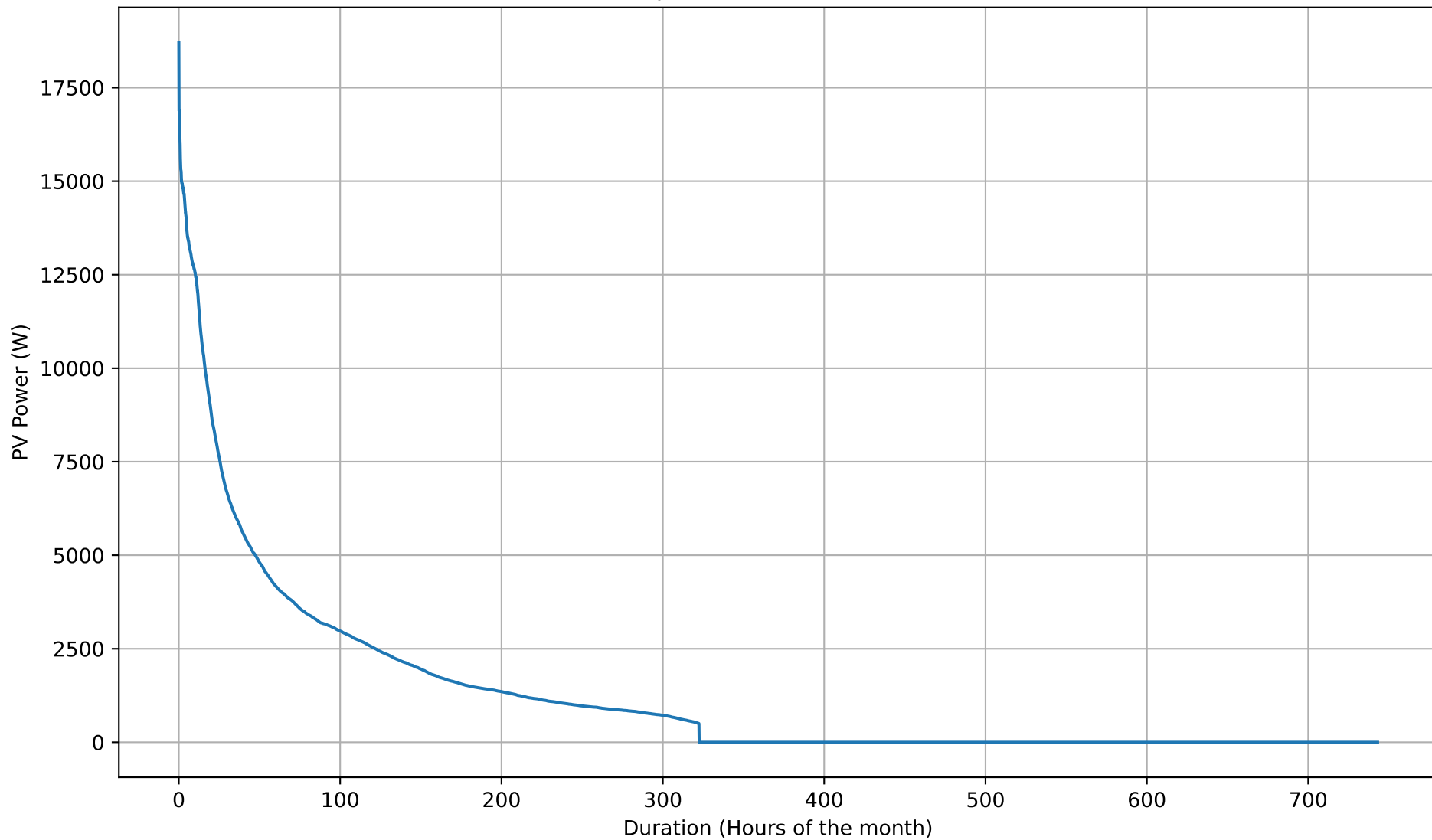
PV Self-Consumption Duration Curve - 15kWh - Mar
