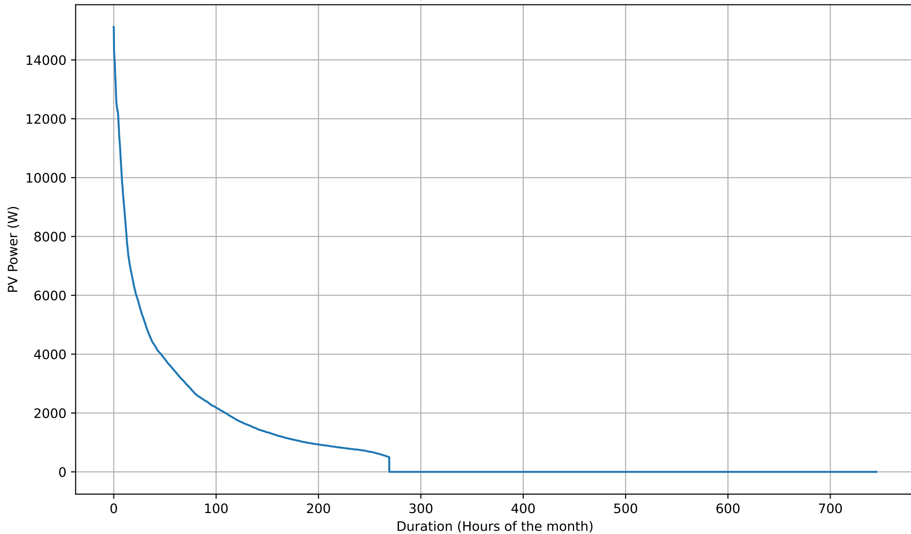
PV Self-Consumption Duration Curve - 15kWh - Oct
