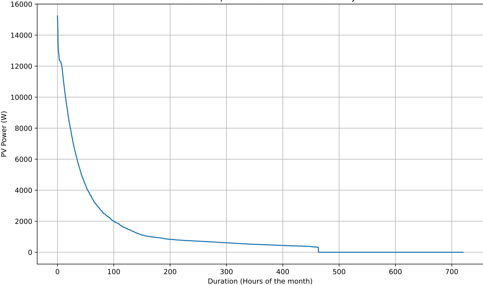
PV Self-Consumption Duration Curve - 15kWh - Jun
