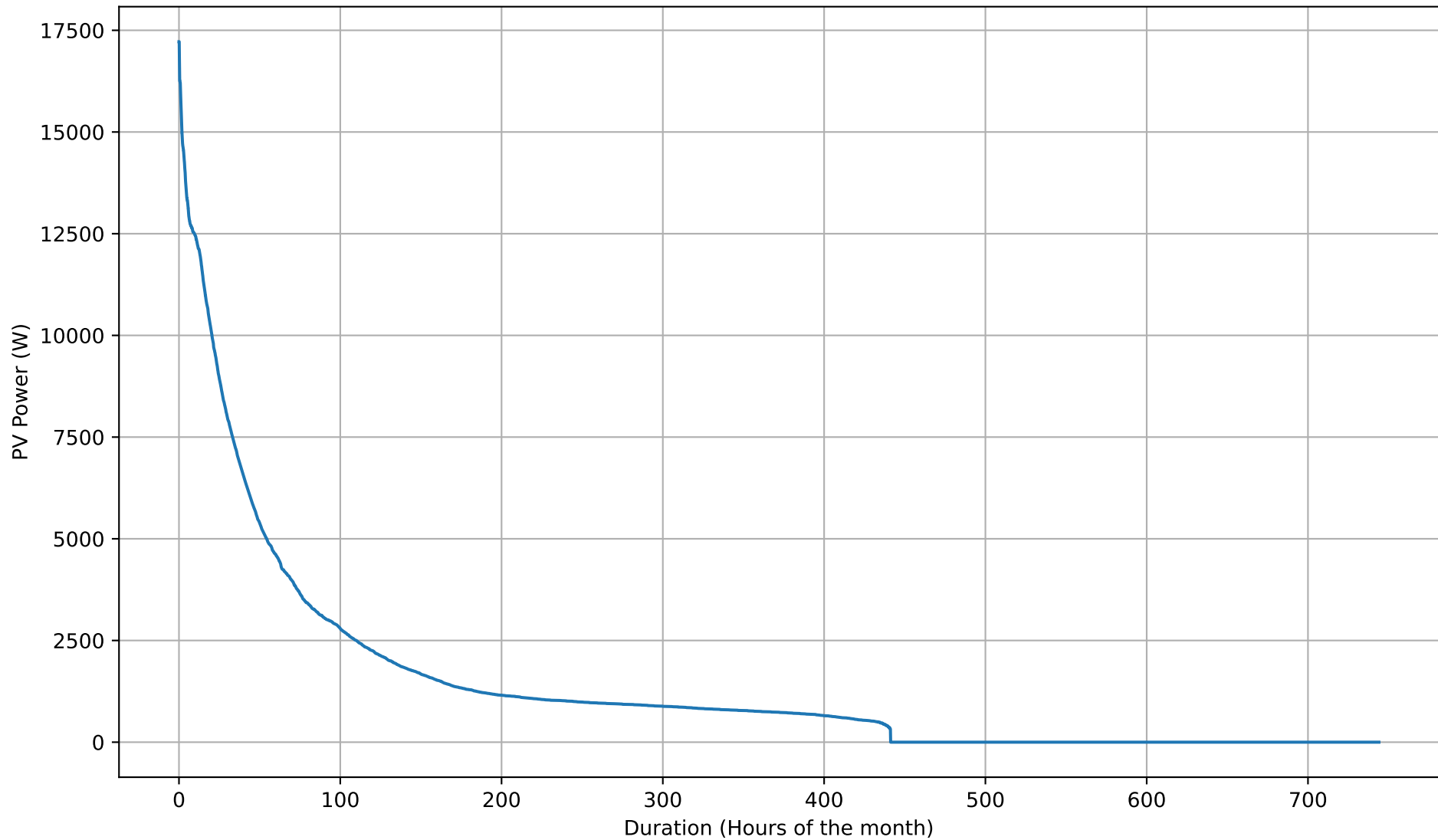
PV Self-Consumption Duration Curve - 15kWh - May
