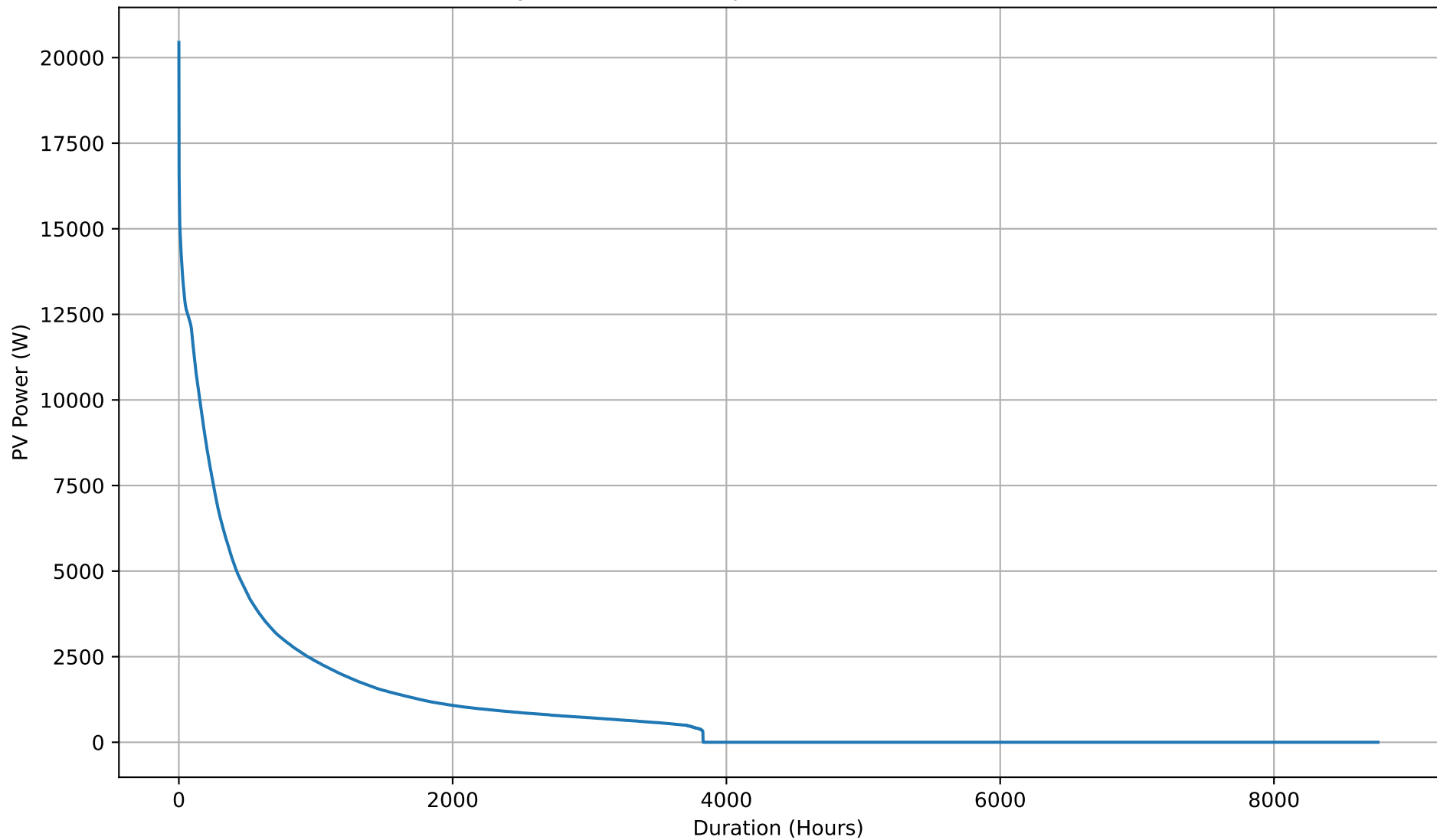
Yearly PV Self-Consumption Duration Curve - 15kWh
