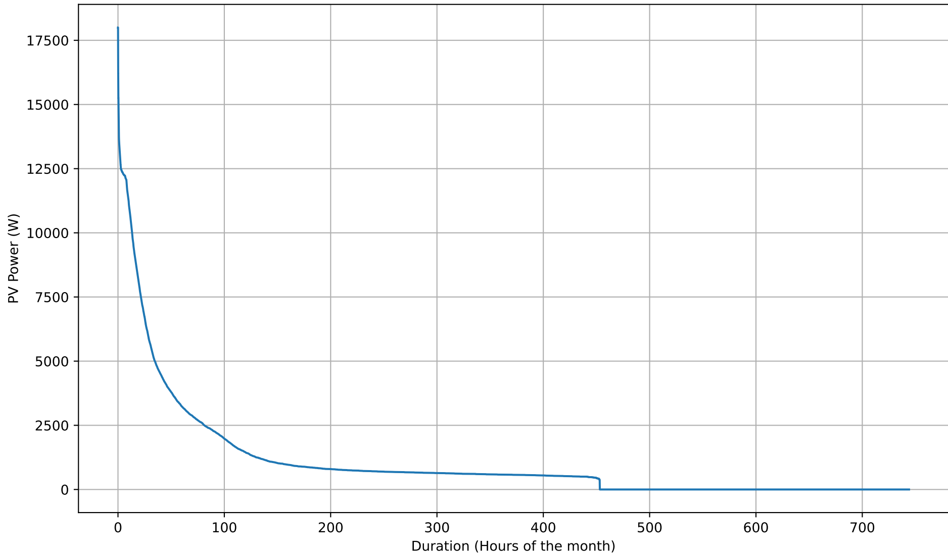
PV Self-Consumption Duration Curve - 15kWh - Jul
