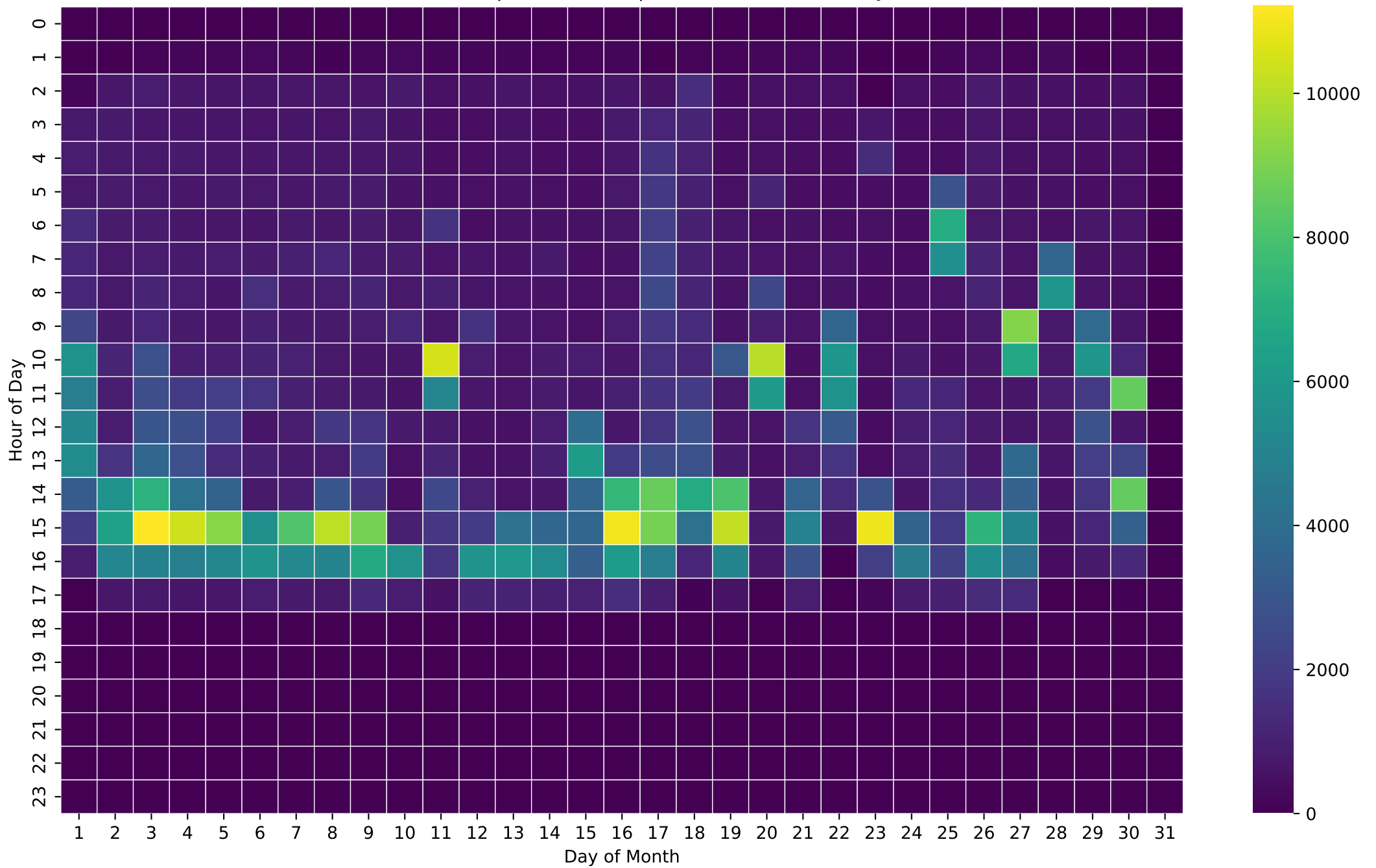
PV Self-Consumption Heatmap (Wh/Hour) - 15kWh - Jun
