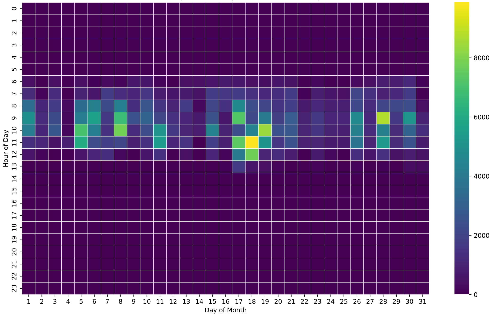
PV Self-Consumption Heatmap (Wh/Hour) - 15kWh - Jan
