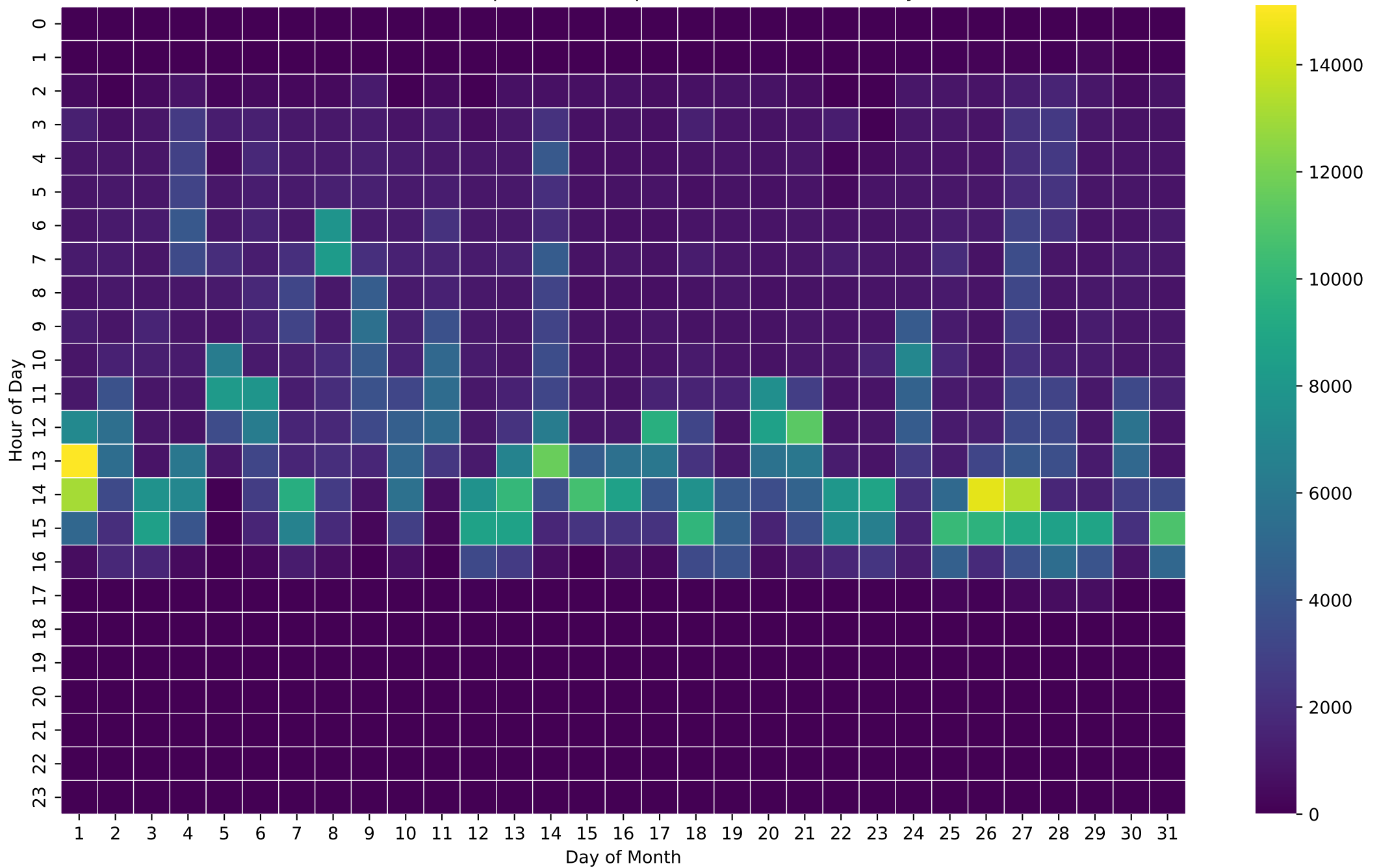
PV Self-Consumption Heatmap (Wh/Hour) - 15kWh - May
