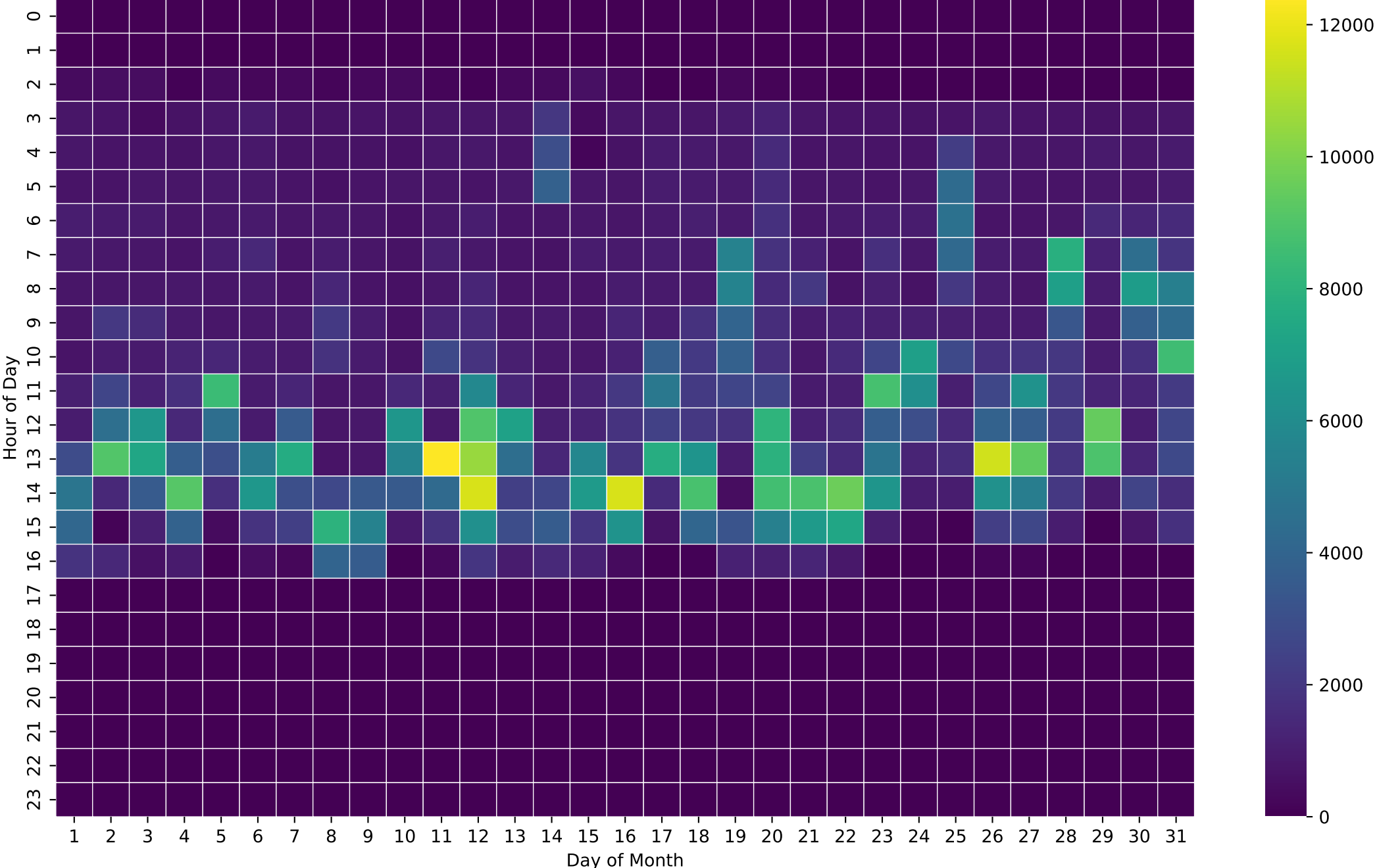
PV Self-Consumption Heatmap (Wh/Hour) - 15kWh - Aug
