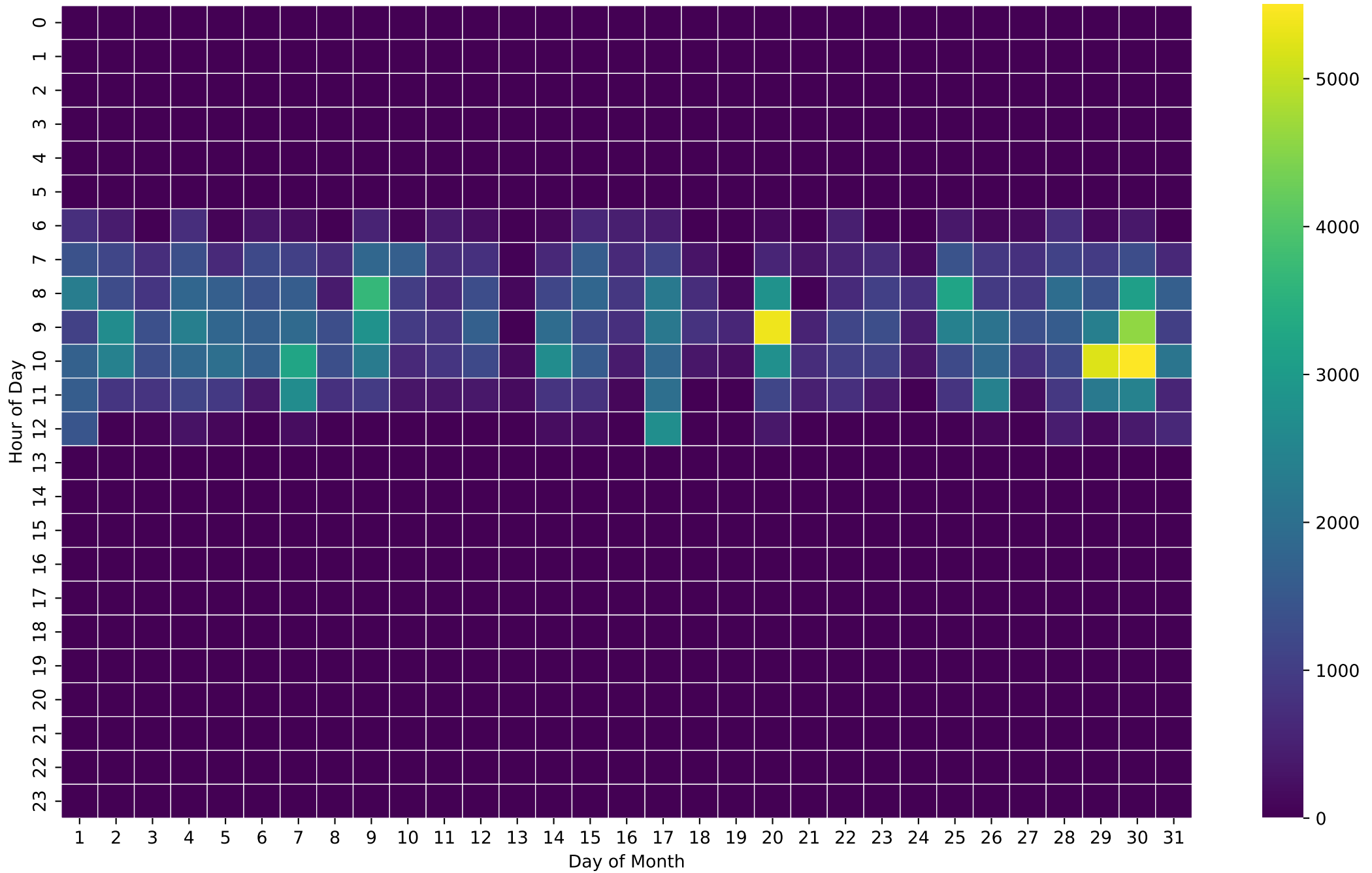
PV Self-Consumption Heatmap (Wh/Hour) - 15kWh - Dec
