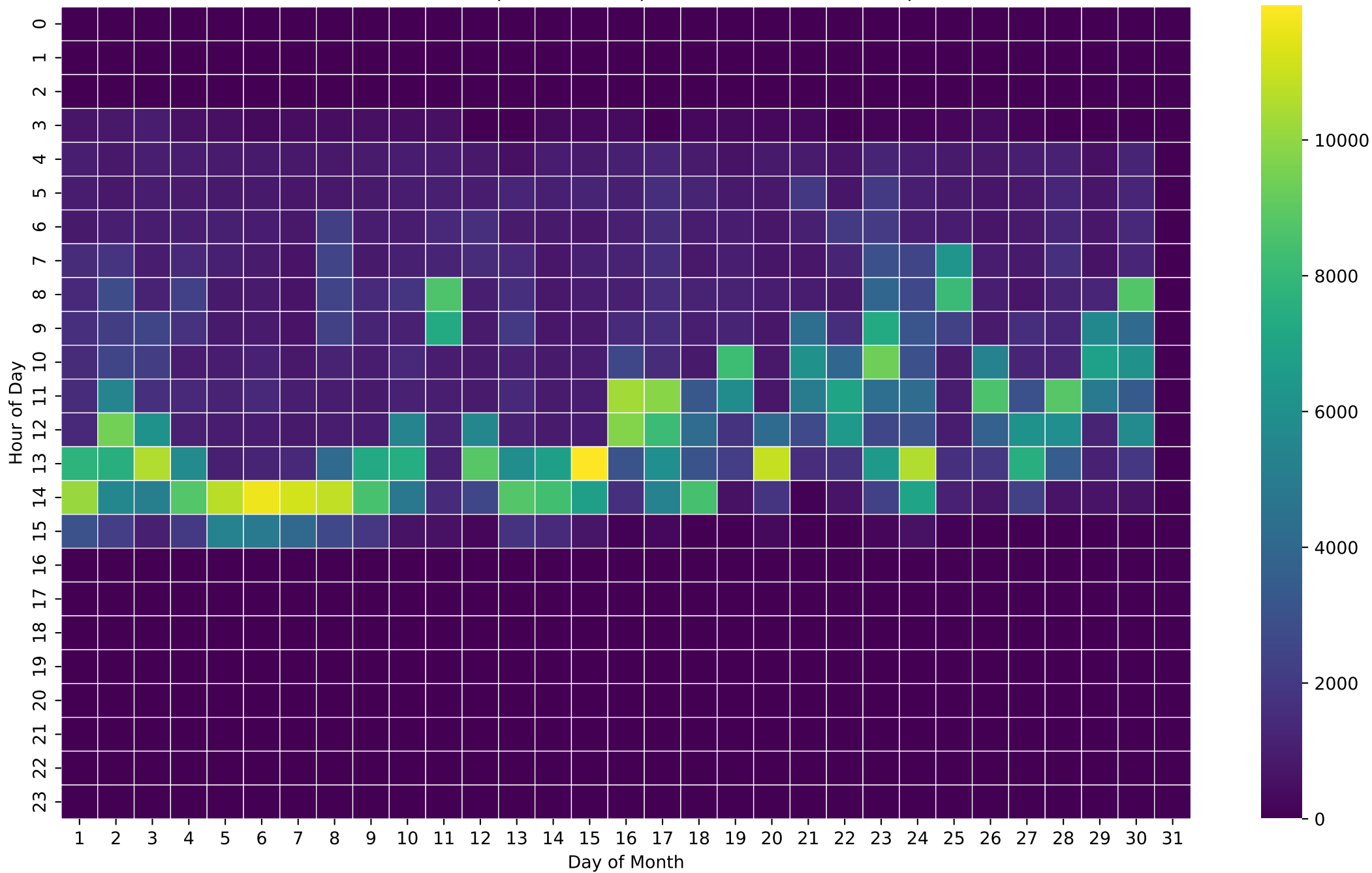
PV Self-Consumption Heatmap (Wh/Hour) - 15kWh - Sep
