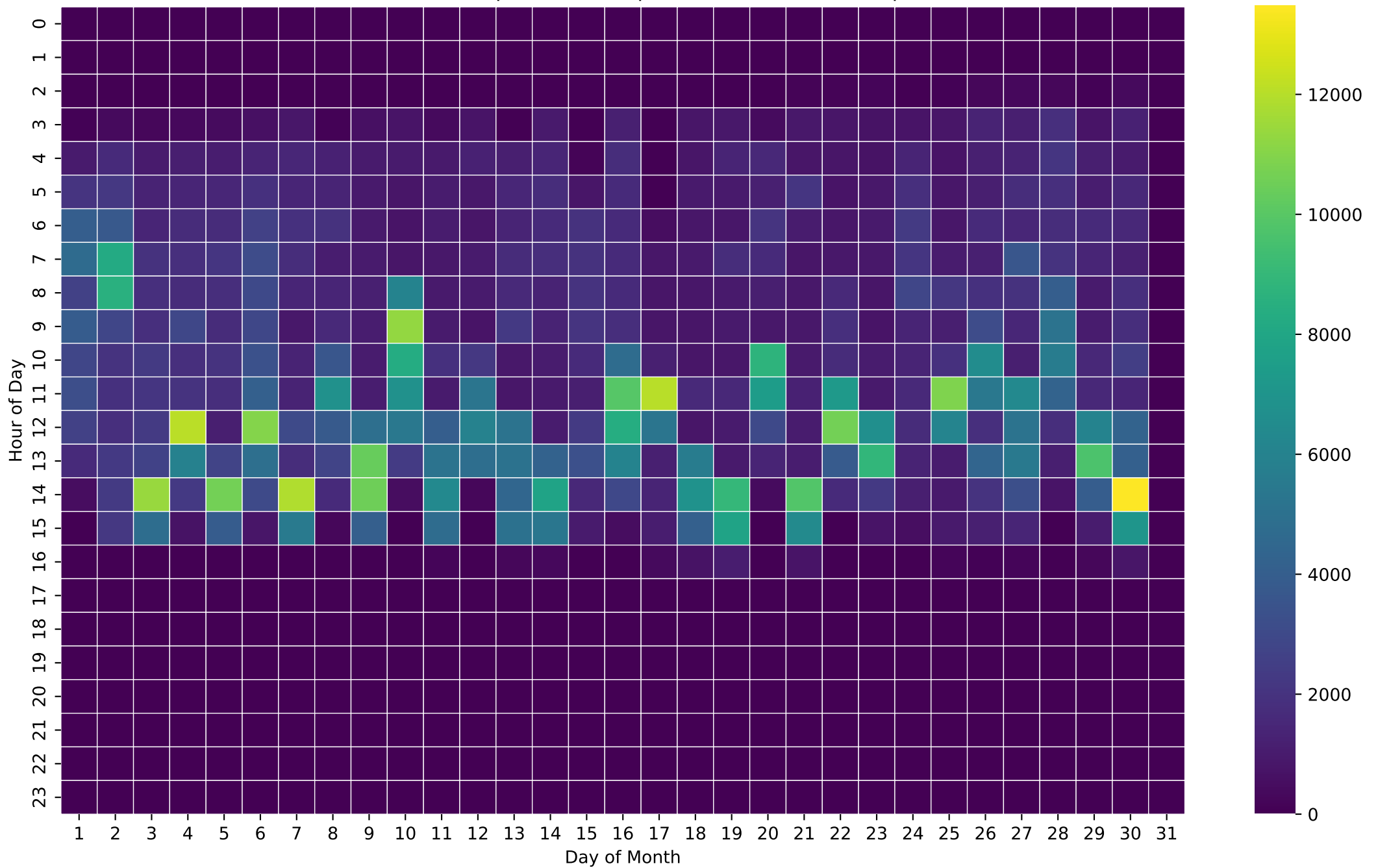
PV Self-Consumption Heatmap (Wh/Hour) - 15kWh - Apr
