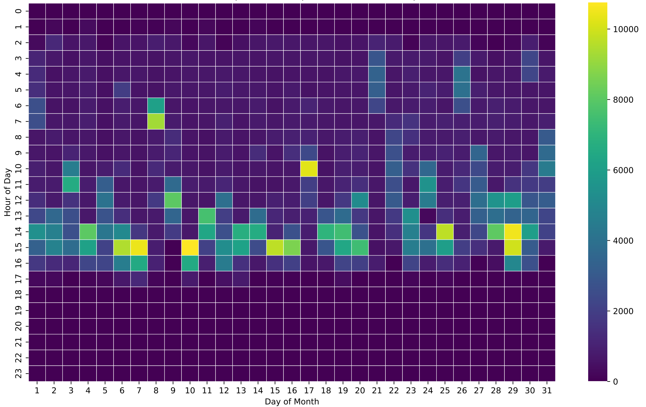
PV Self-Consumption Heatmap (Wh/Hour) - 15kWh - Jul
