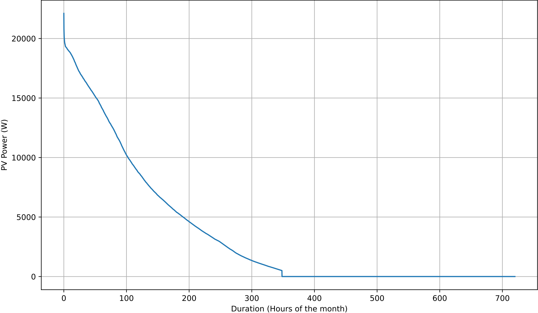
PV Production Duration Curve - 15kWh - Sep
