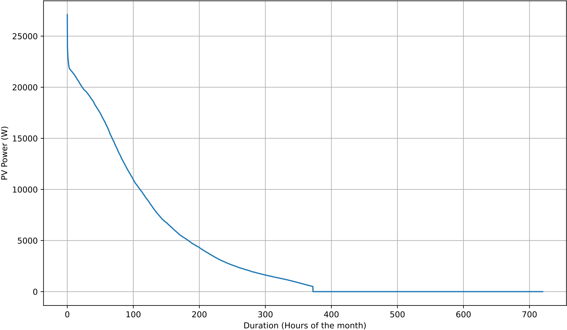
PV Production Duration Curve - 15kWh - Apr
