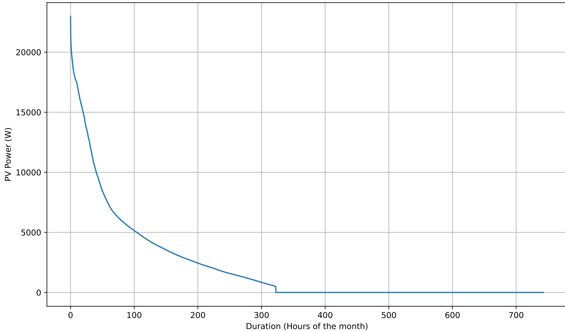
PV Production Duration Curve - 15kWh - Mar
