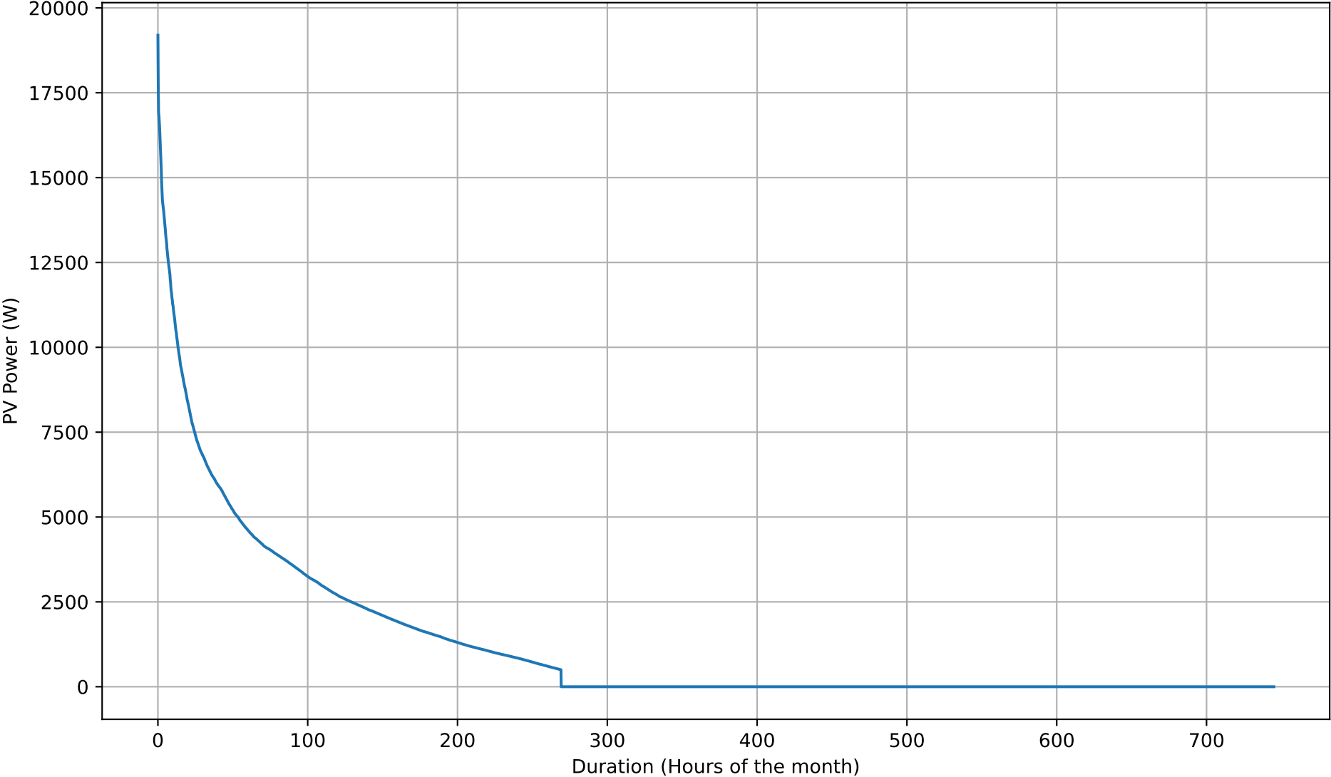
PV Production Duration Curve - 15kWh - Oct
