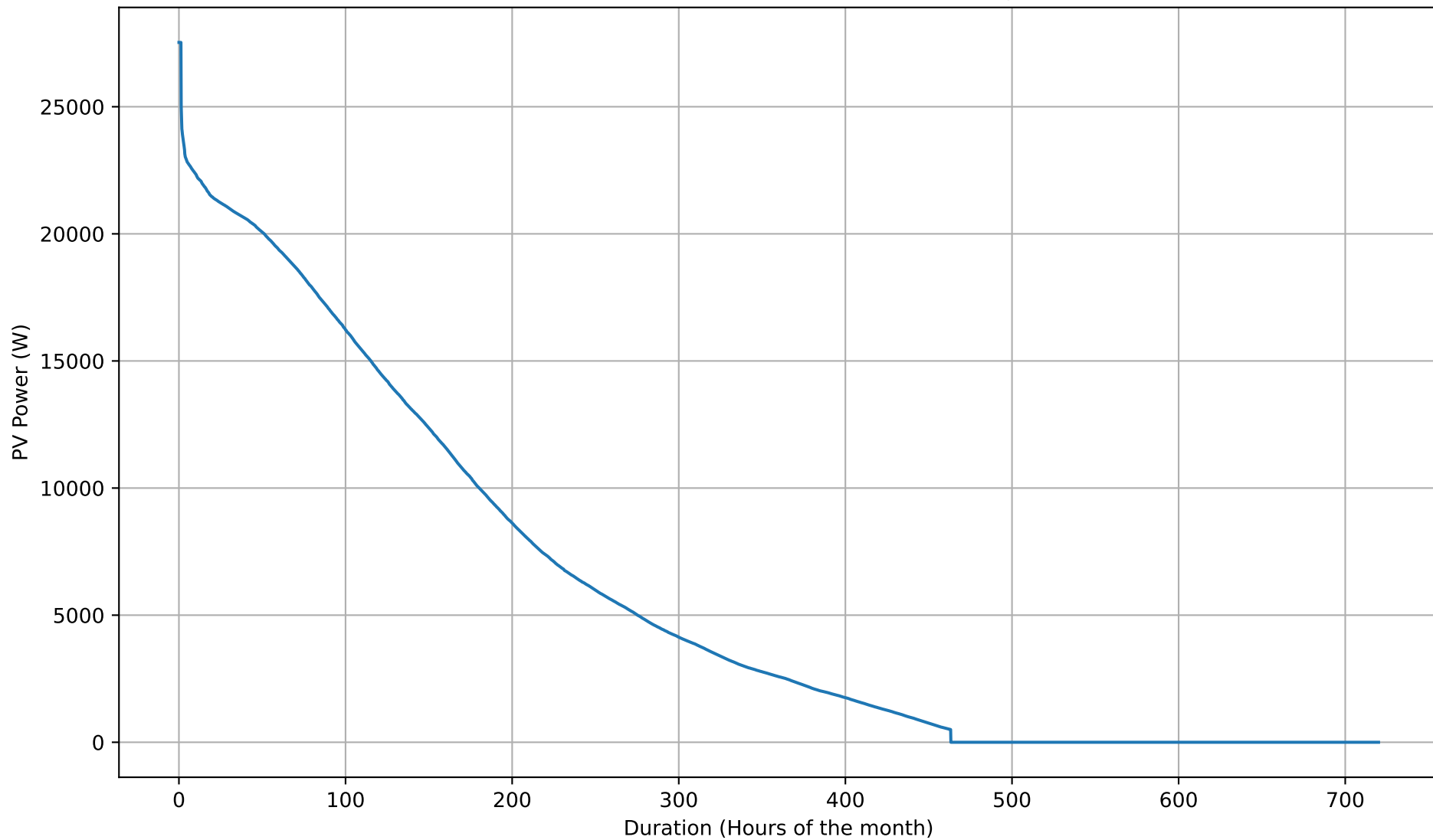
PV Production Duration Curve - 15kWh - Jun
