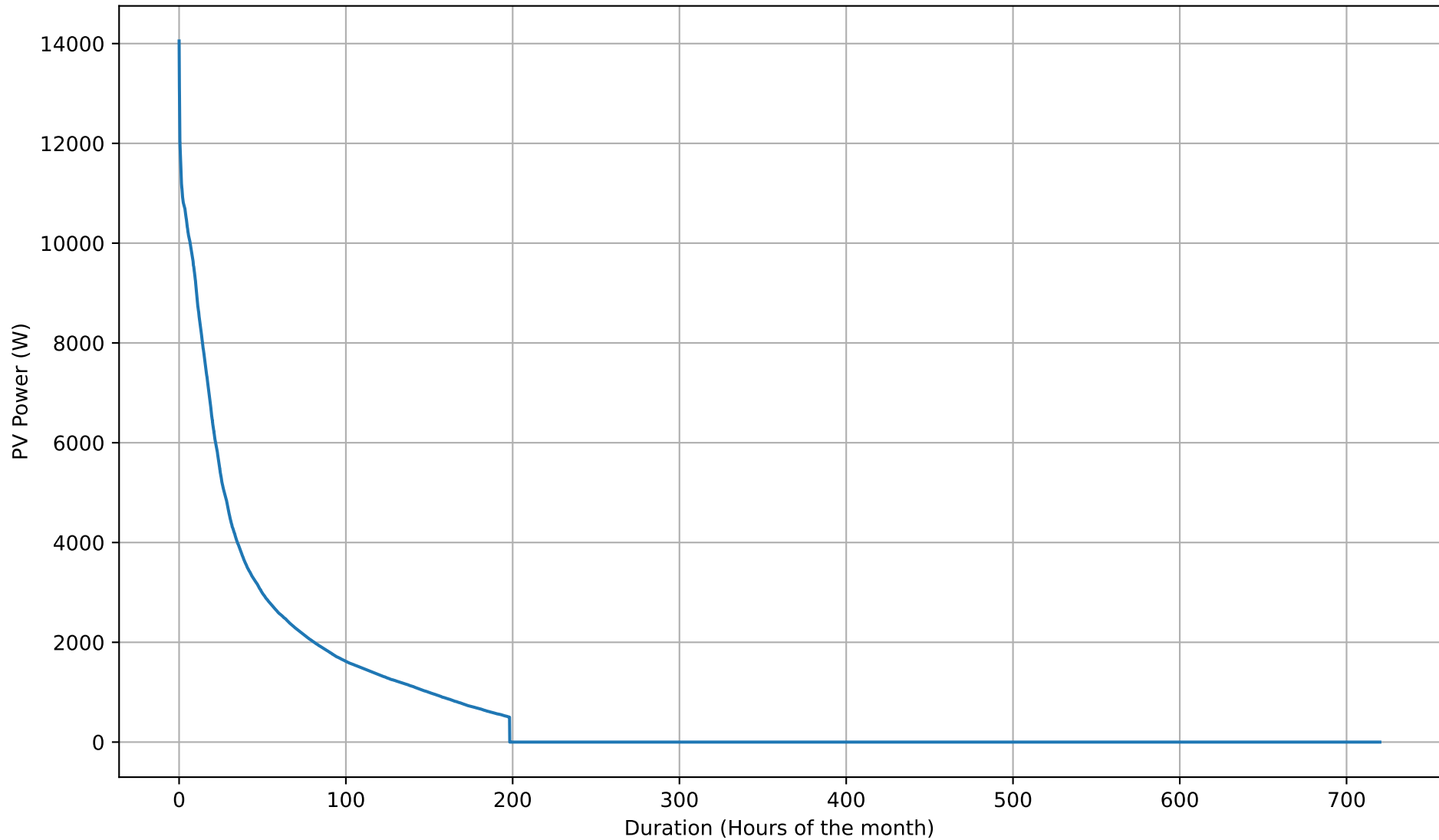
PV Production Duration Curve - 15kWh - Nov
