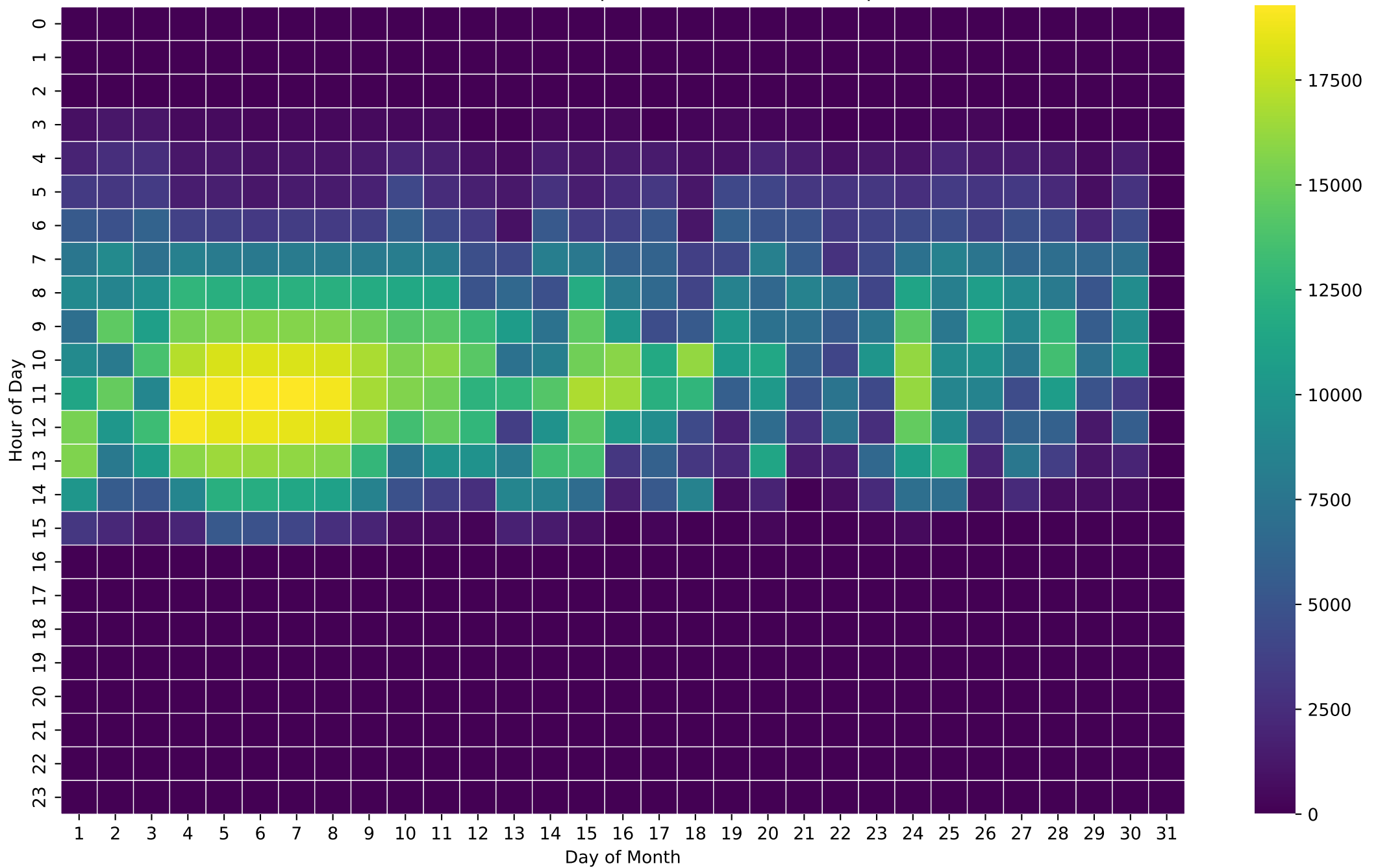
PV Production Heatmap (Wh/Hour) - 15kWh - Sep
