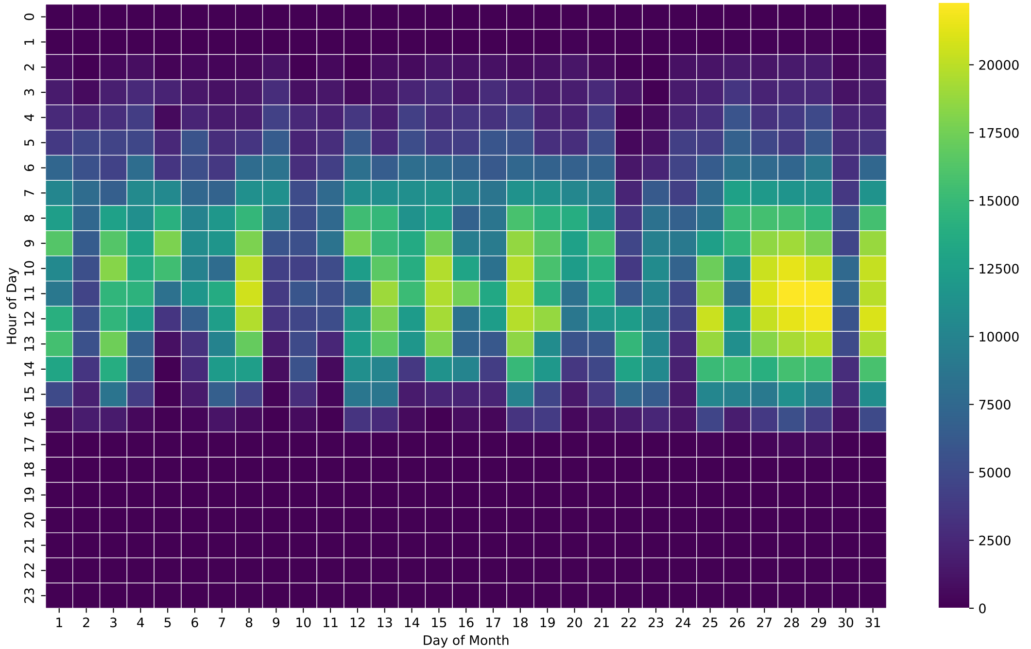
PV Production Heatmap (Wh/Hour) - 15kWh - May
