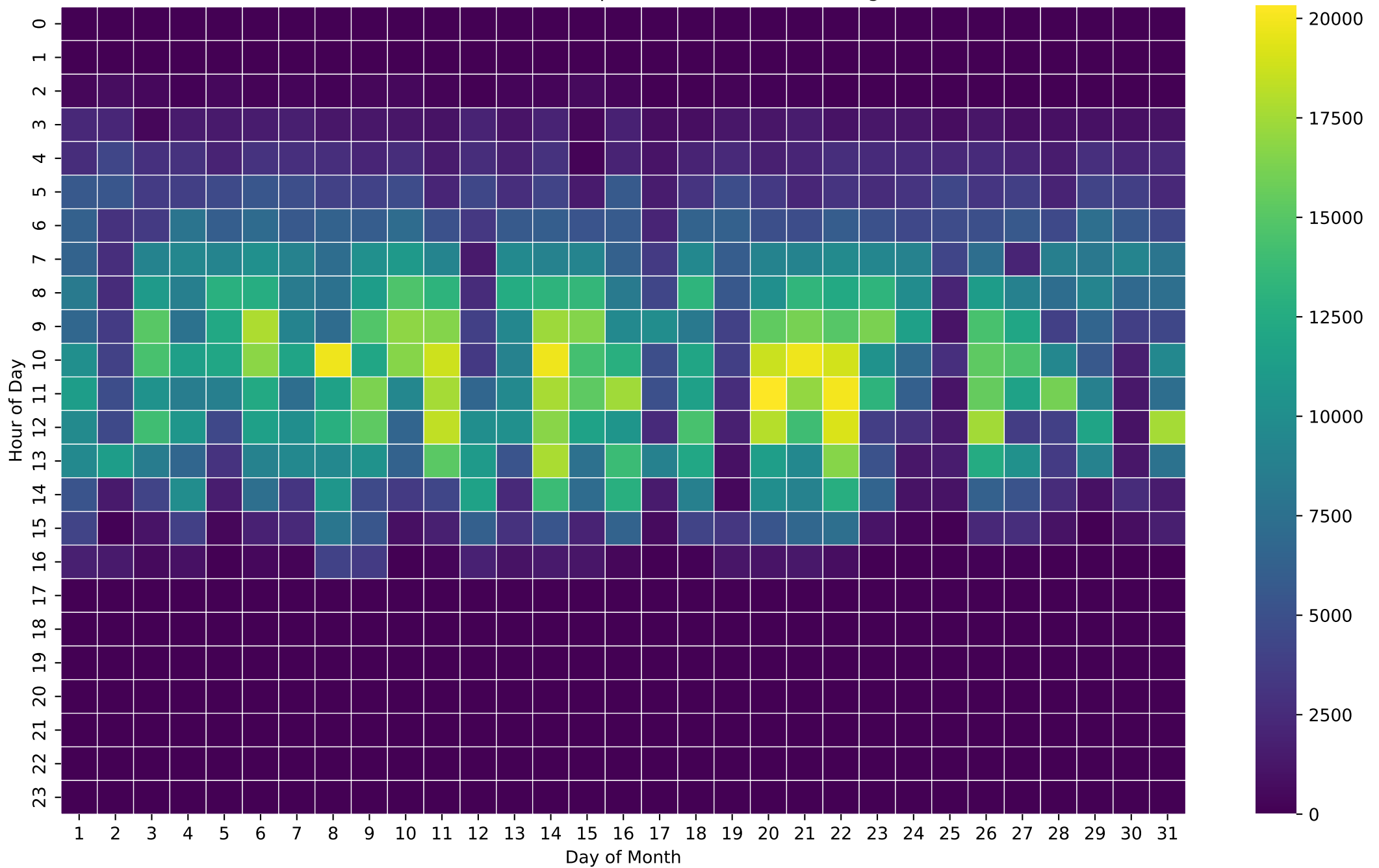
PV Production Heatmap (Wh/Hour) - 15kWh - Aug
