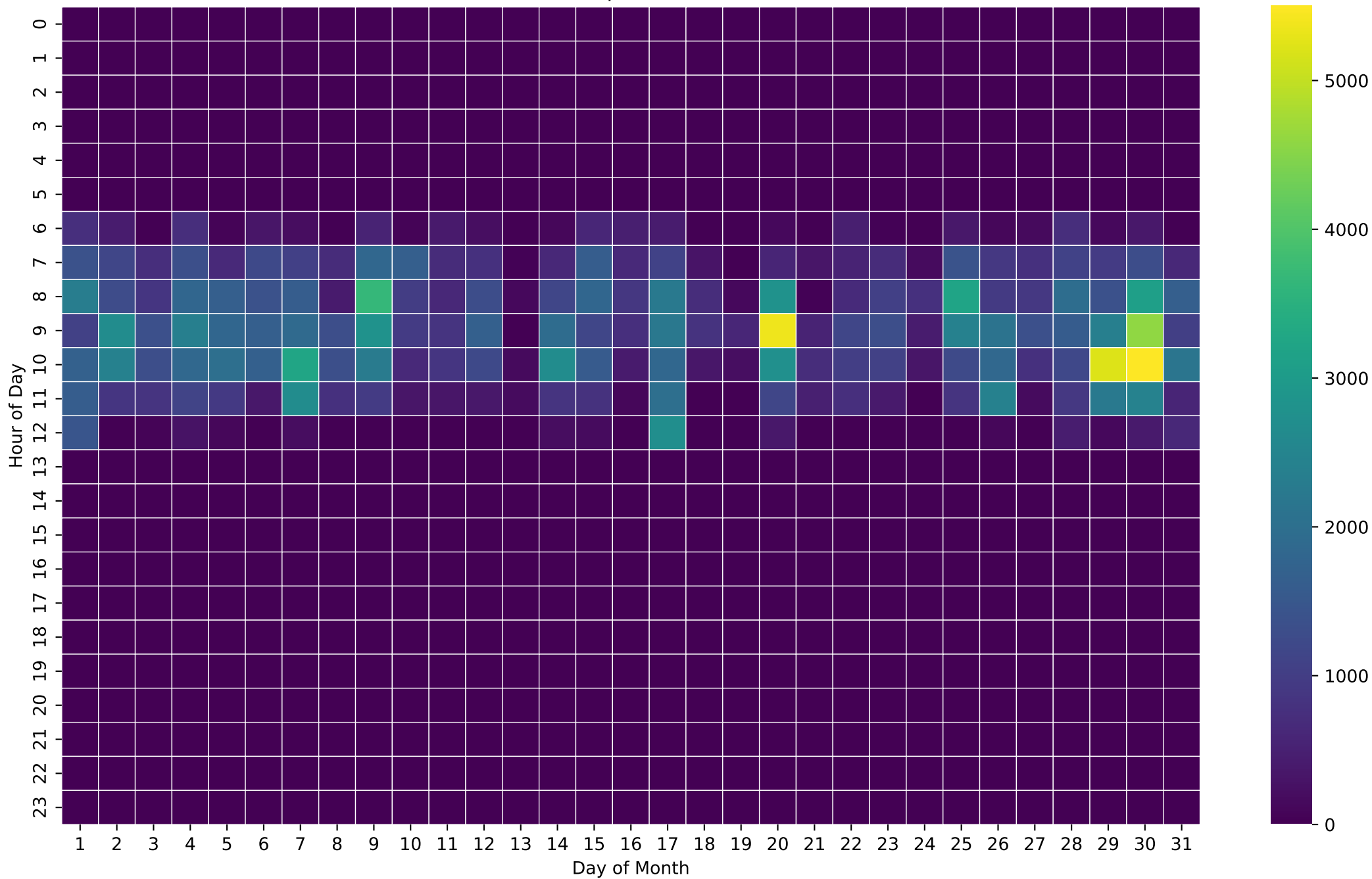
PV Production Heatmap (Wh/Hour) - 15kWh - Dec
