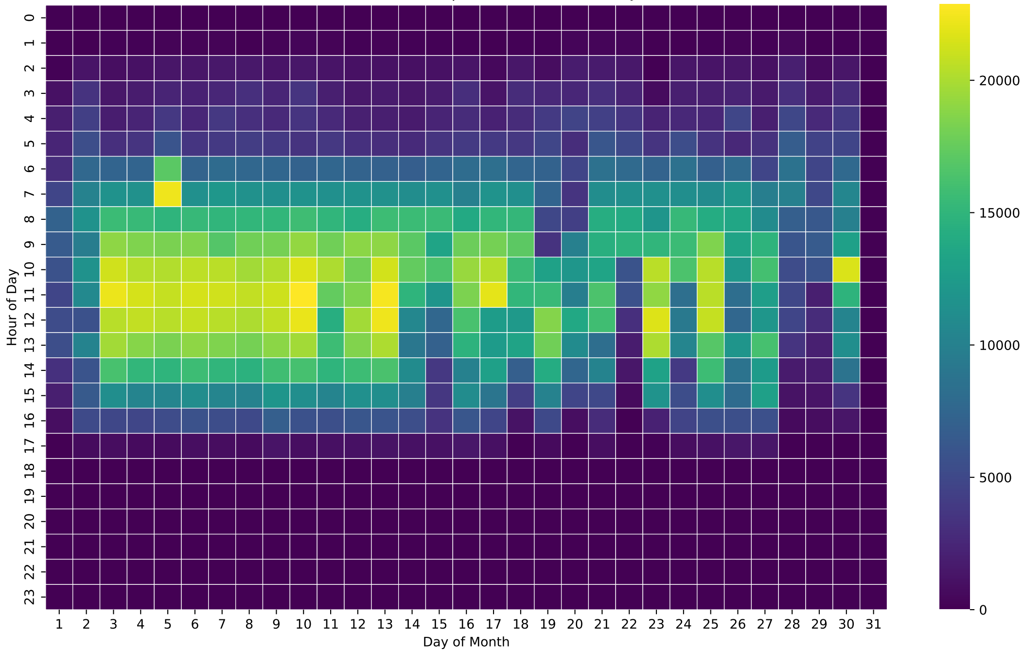
PV Production Heatmap (Wh/Hour) - 15kWh - Jun
