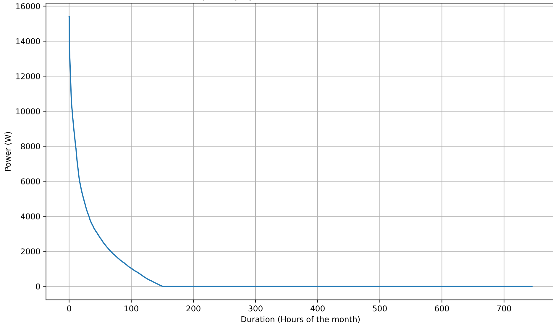
Battery Charging Power Duration Curve - 20kWh - Oct
