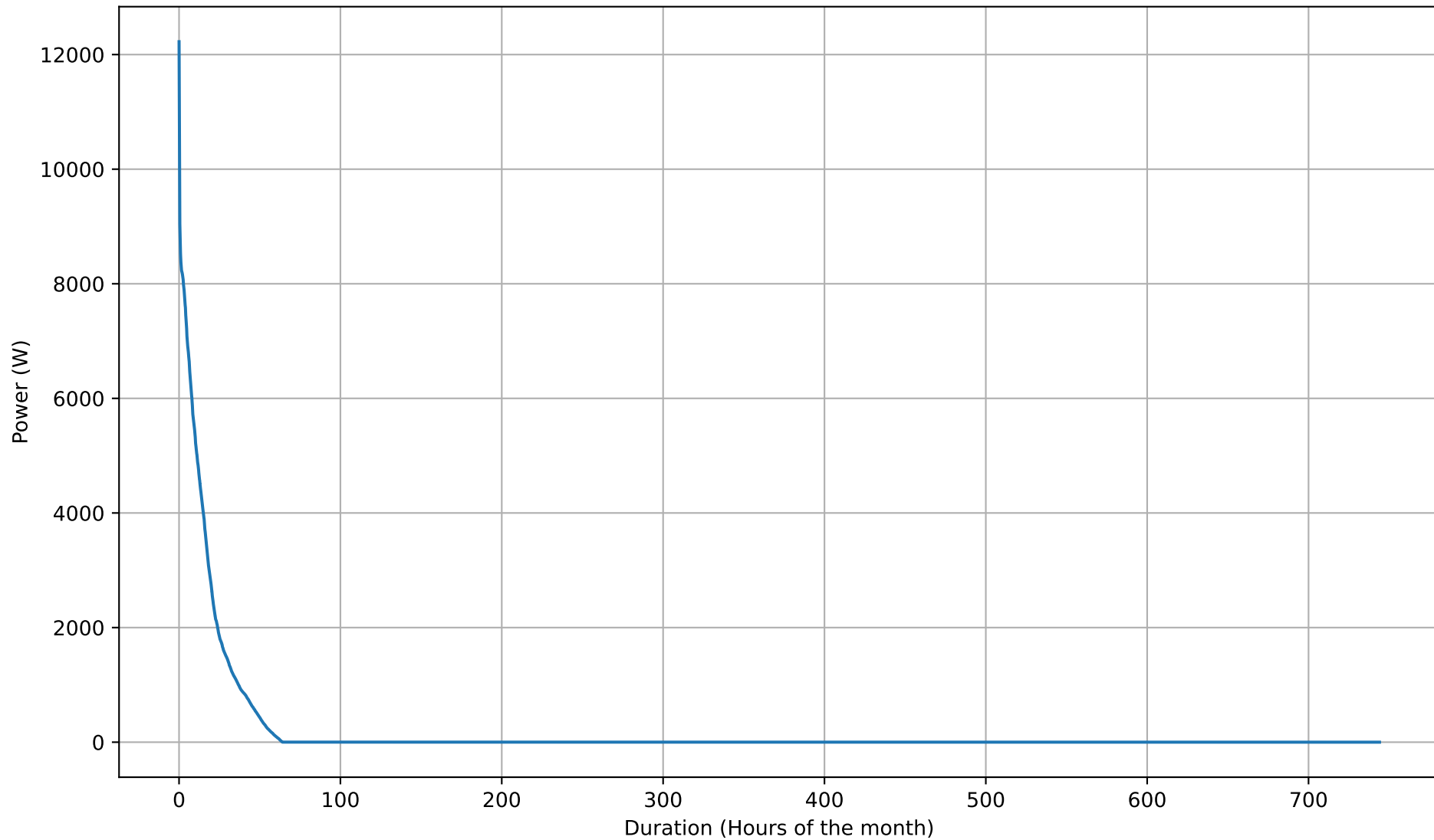
Battery Charging Power Duration Curve - 20kWh - Jan
