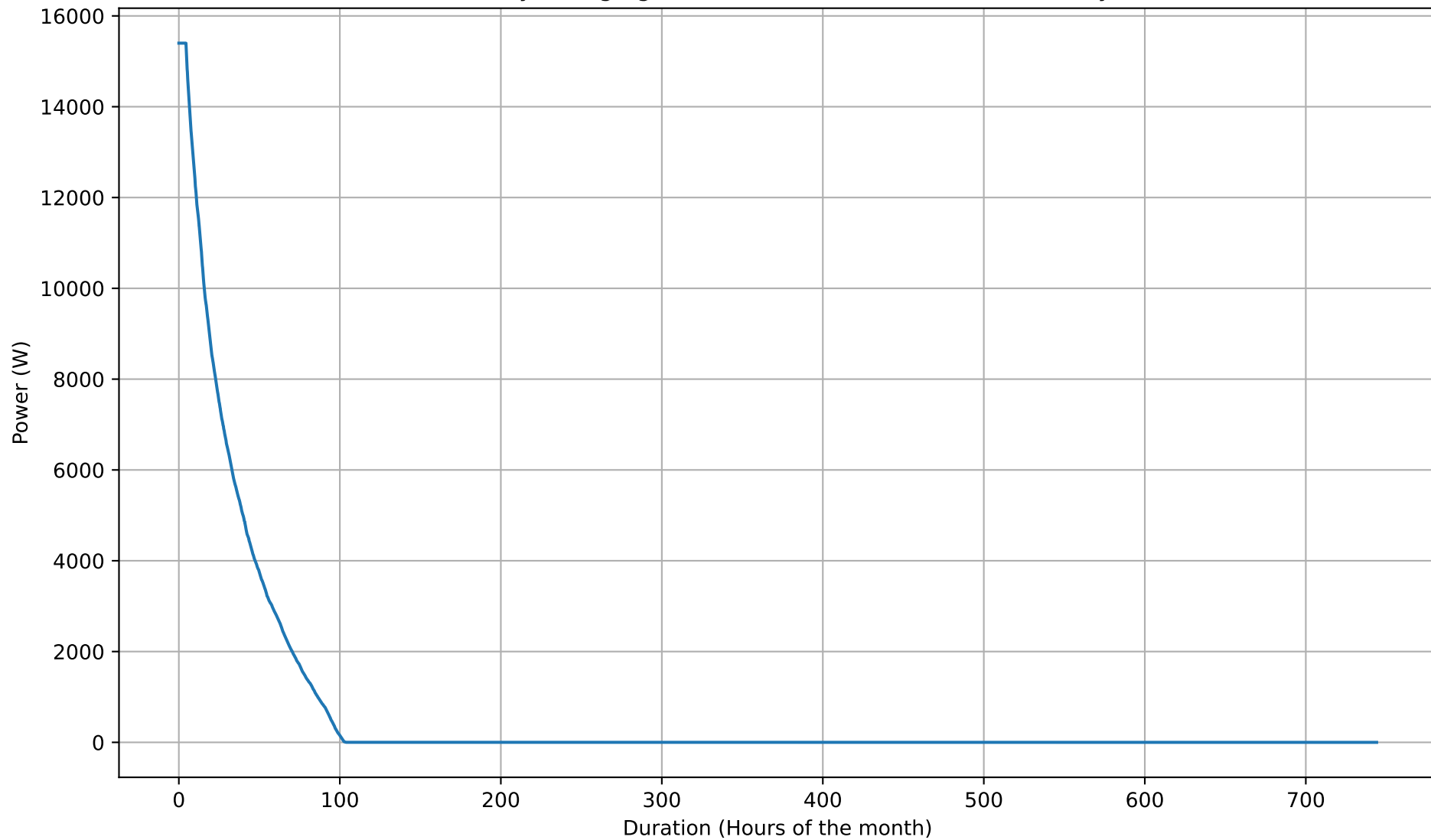
Battery Charging Power Duration Curve - 20kWh - May
