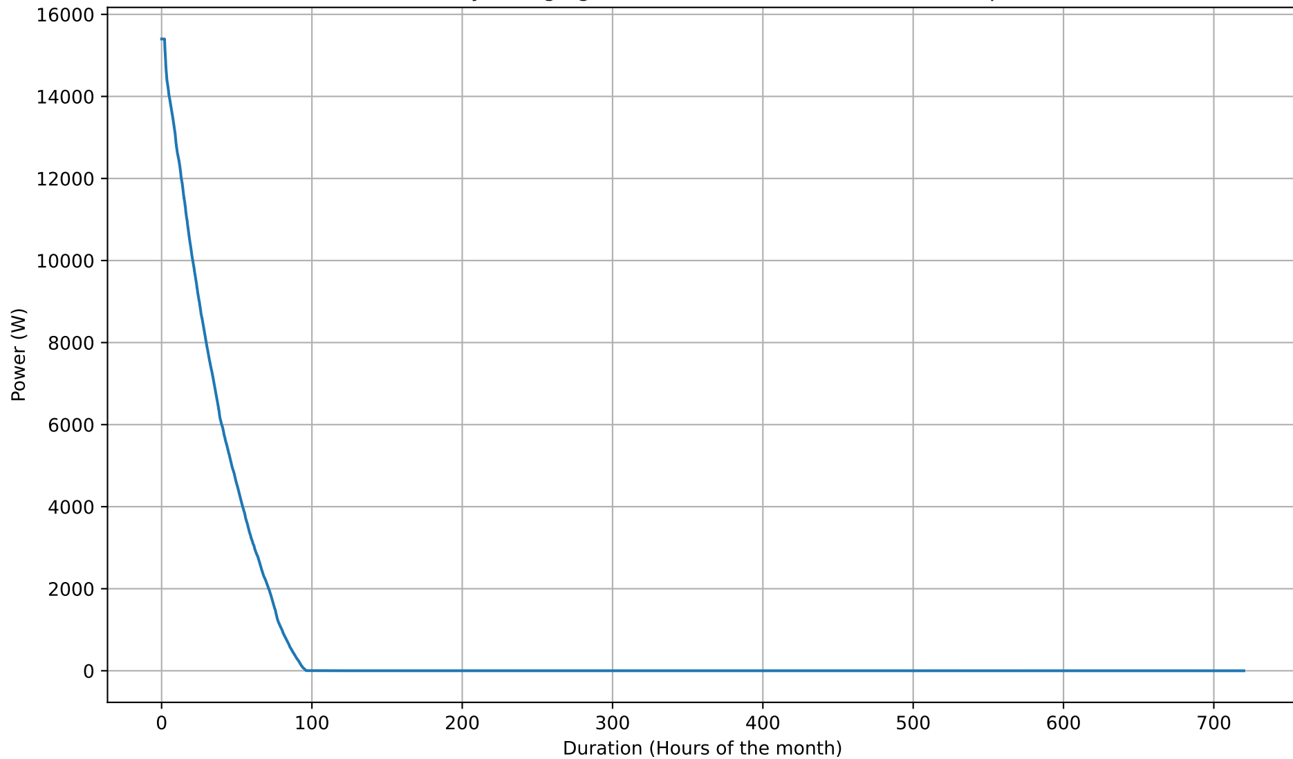
Battery Charging Power Duration Curve - 20kWh - Sep
