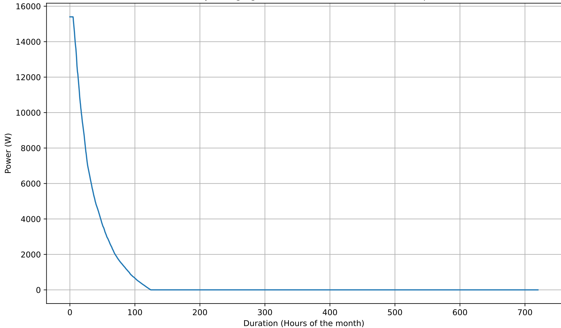
Battery Charging Power Duration Curve - 20kWh - Apr
