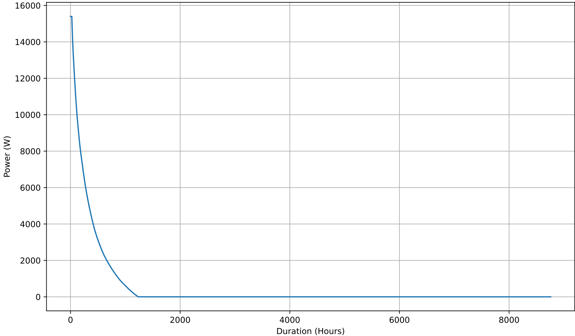
Yearly Battery Charging Power Duration Curve - 20kWh
