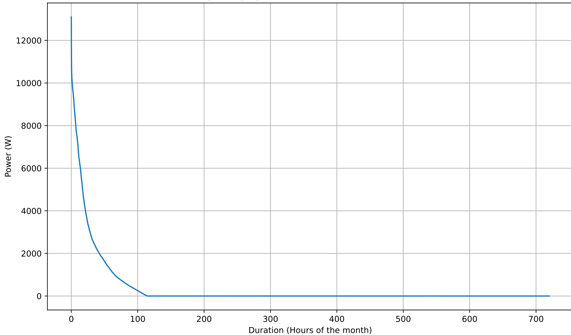
Battery Charging Power Duration Curve - 20kWh - Nov
