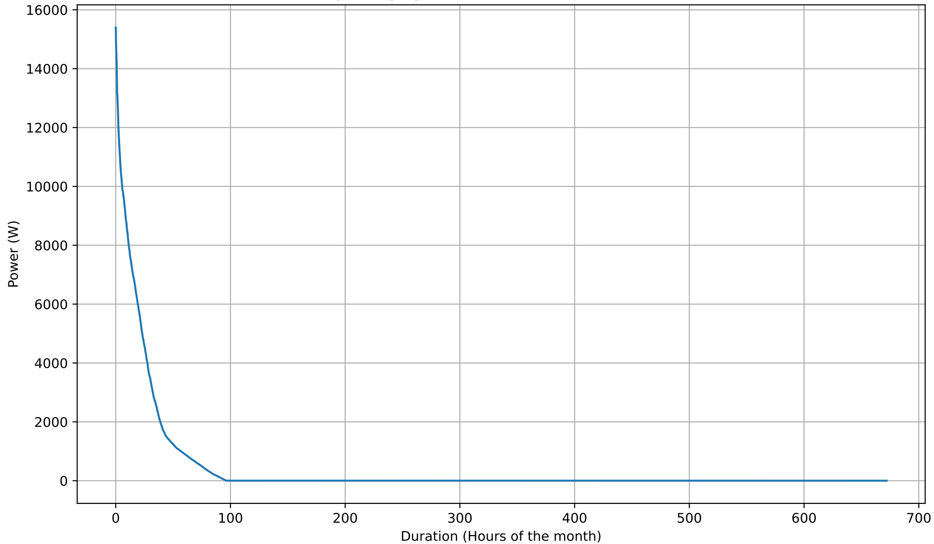
Battery Charging Power Duration Curve - 20kWh - Feb
