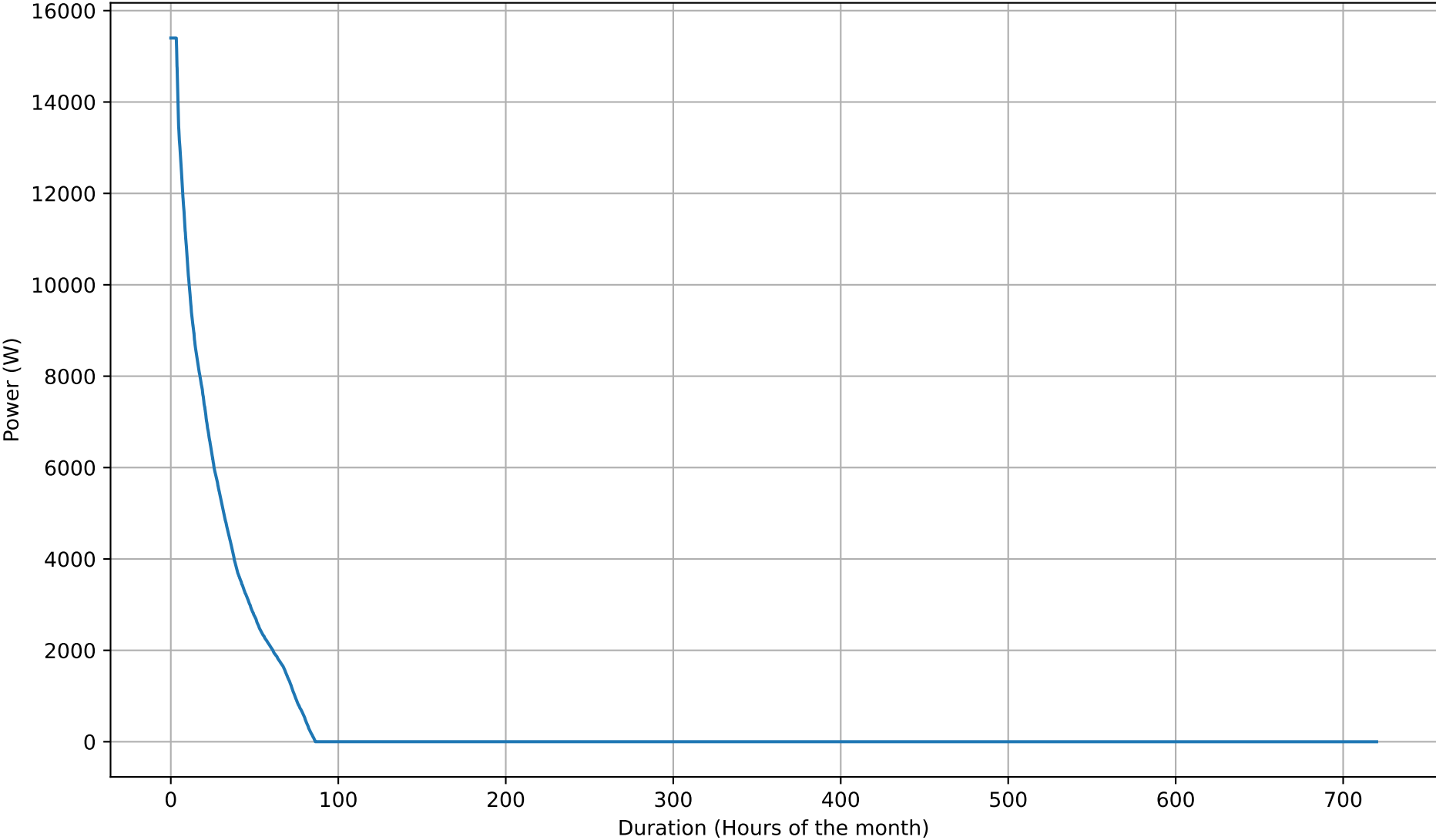
Battery Charging Power Duration Curve - 20kWh - Jun
