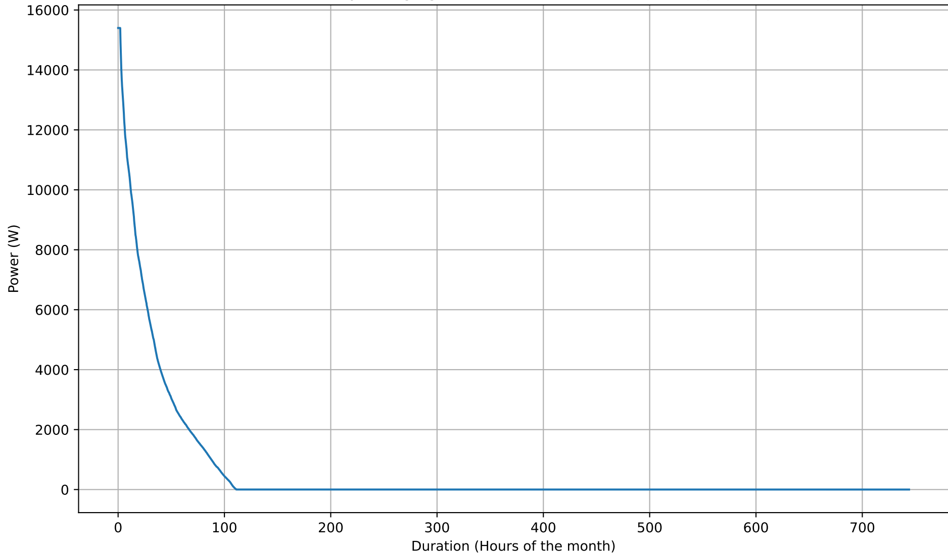
Battery Charging Power Duration Curve - 20kWh - Jul
