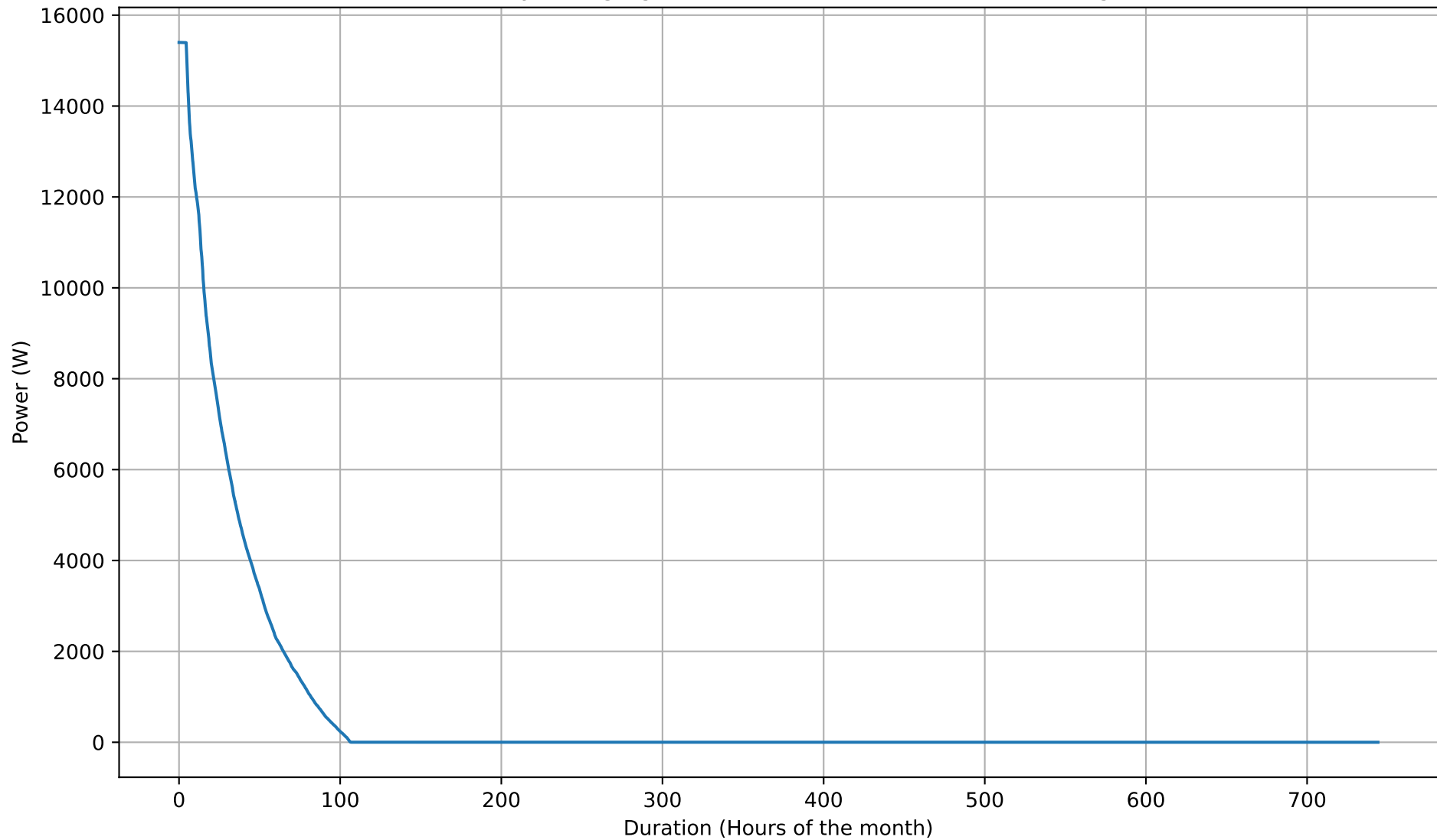
Battery Charging Power Duration Curve - 20kWh - Aug
