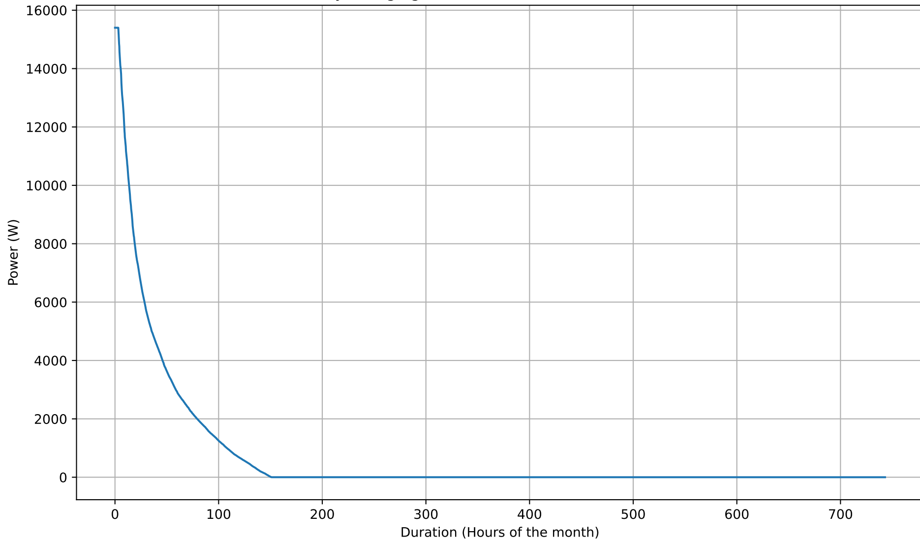
Battery Charging Power Duration Curve - 20kWh - Mar
