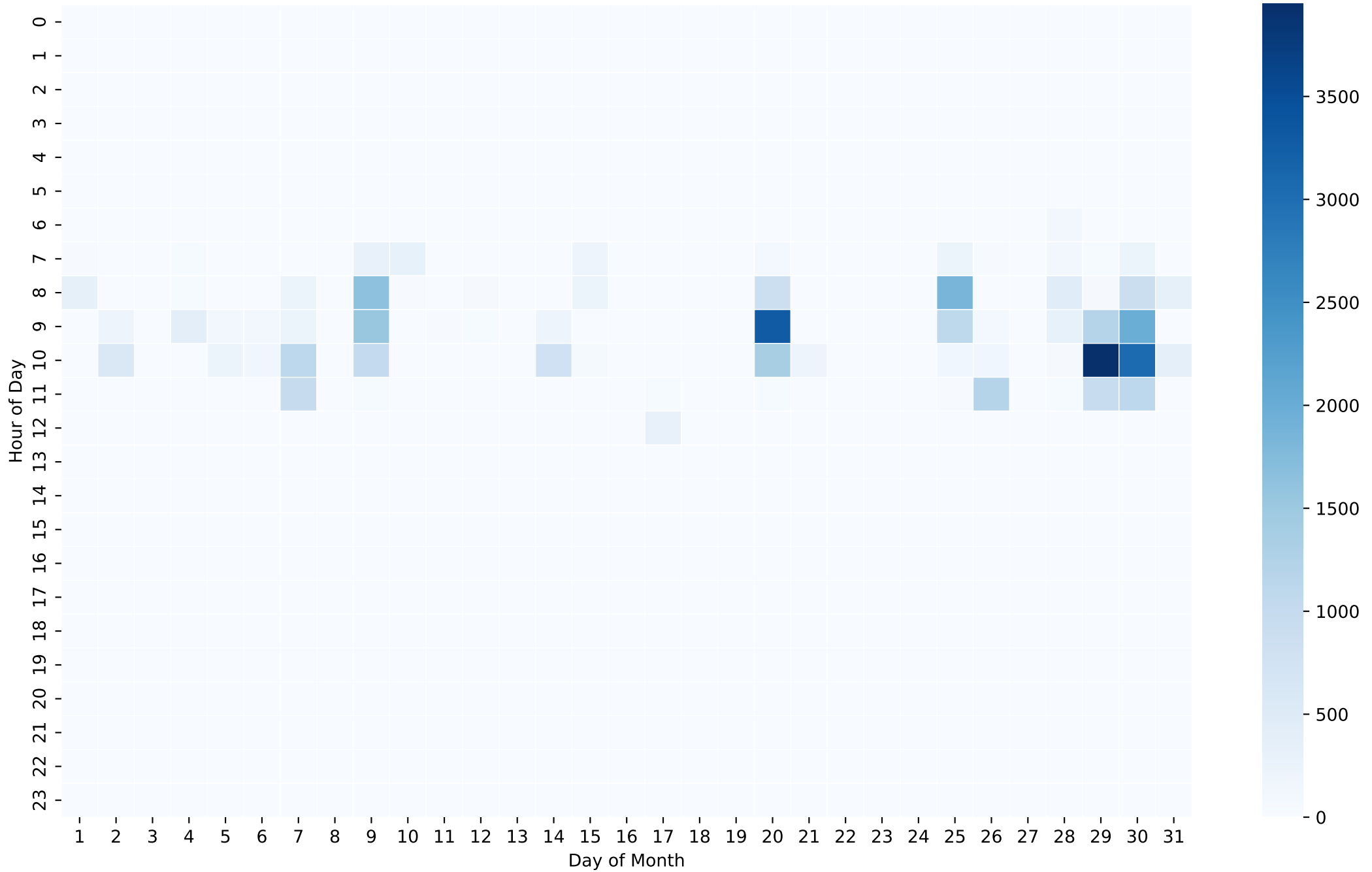
Battery Charging Power Heatmap (Wh/Hour) - 20kWh - Dec
