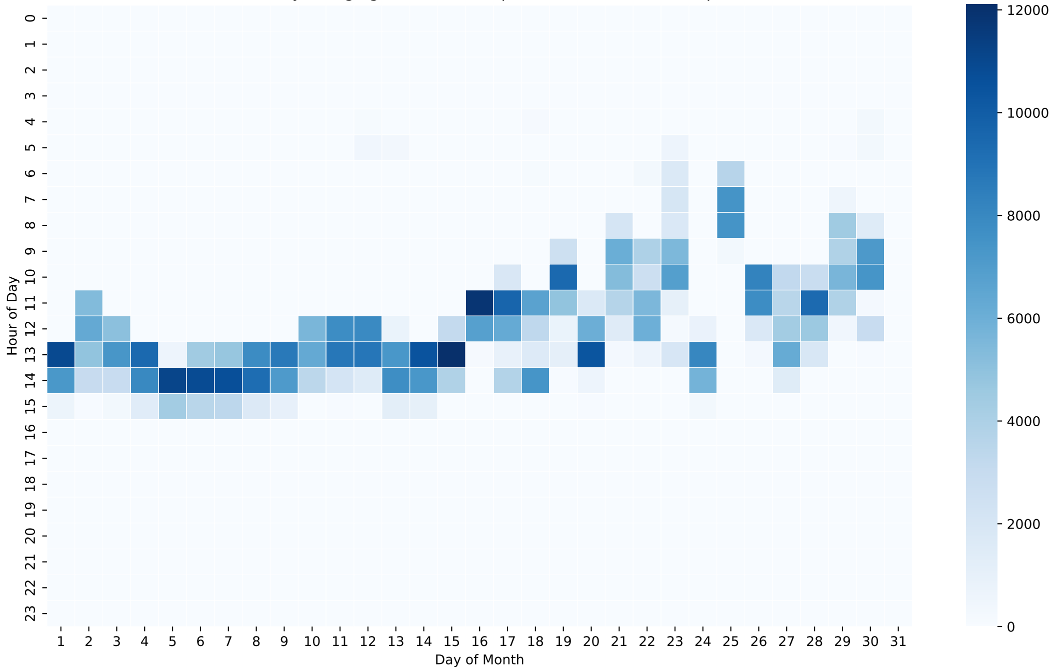
Battery Charging Power Heatmap (Wh/Hour) - 20kWh - Sep
