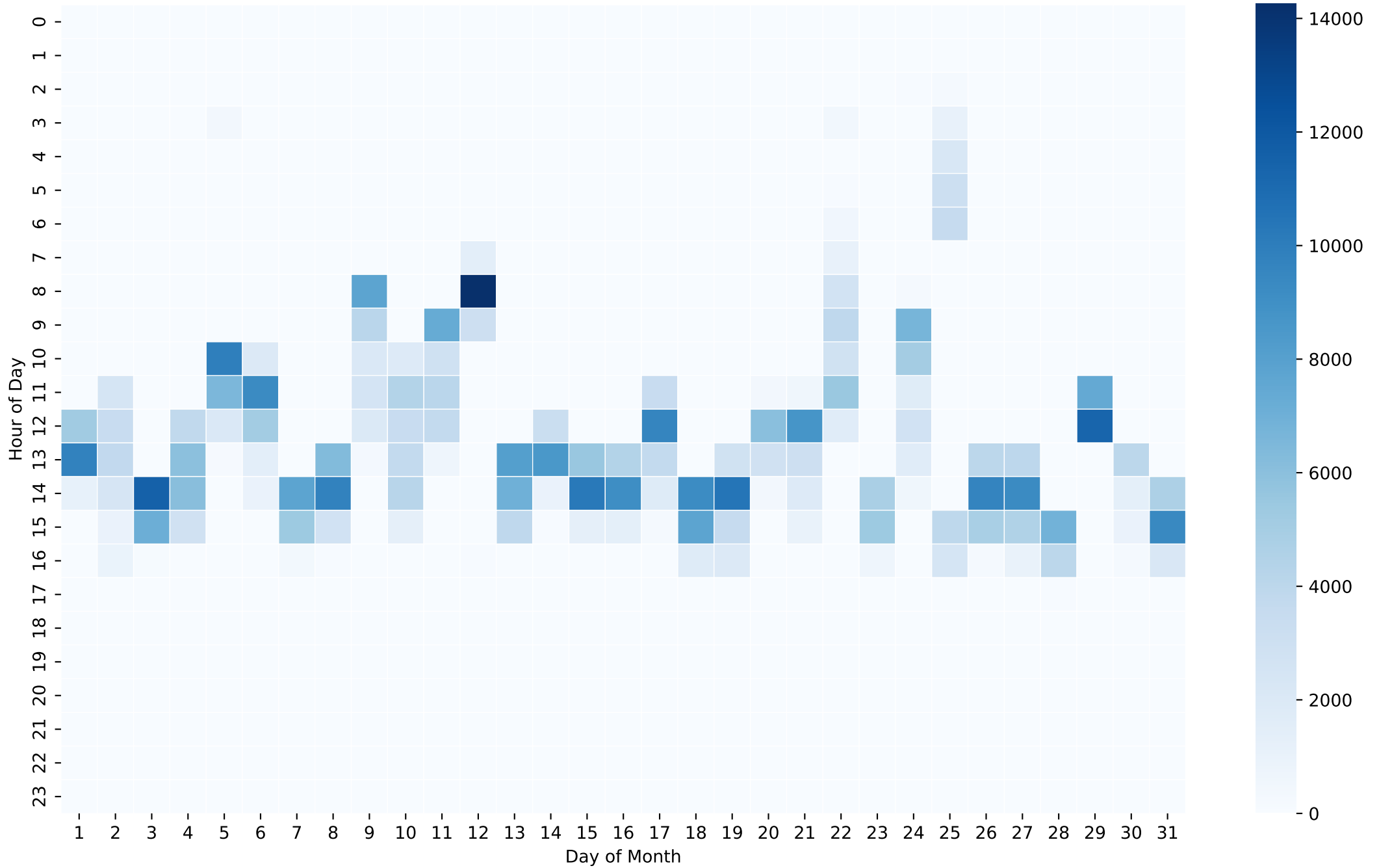
Battery Charging Power Heatmap (Wh/Hour) - 20kWh - May
