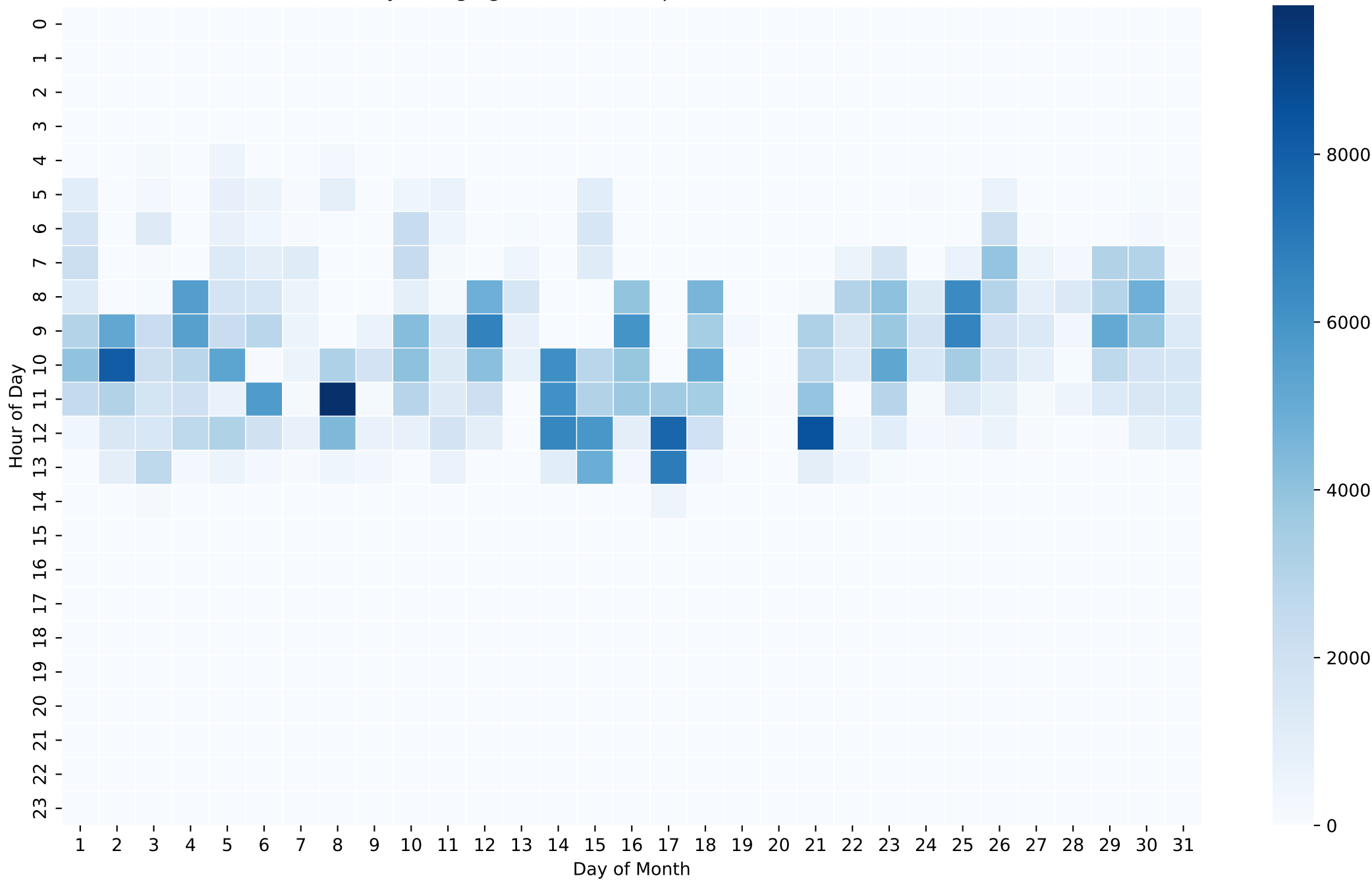
Battery Charging Power Heatmap (Wh/Hour) - 20kWh - Oct
