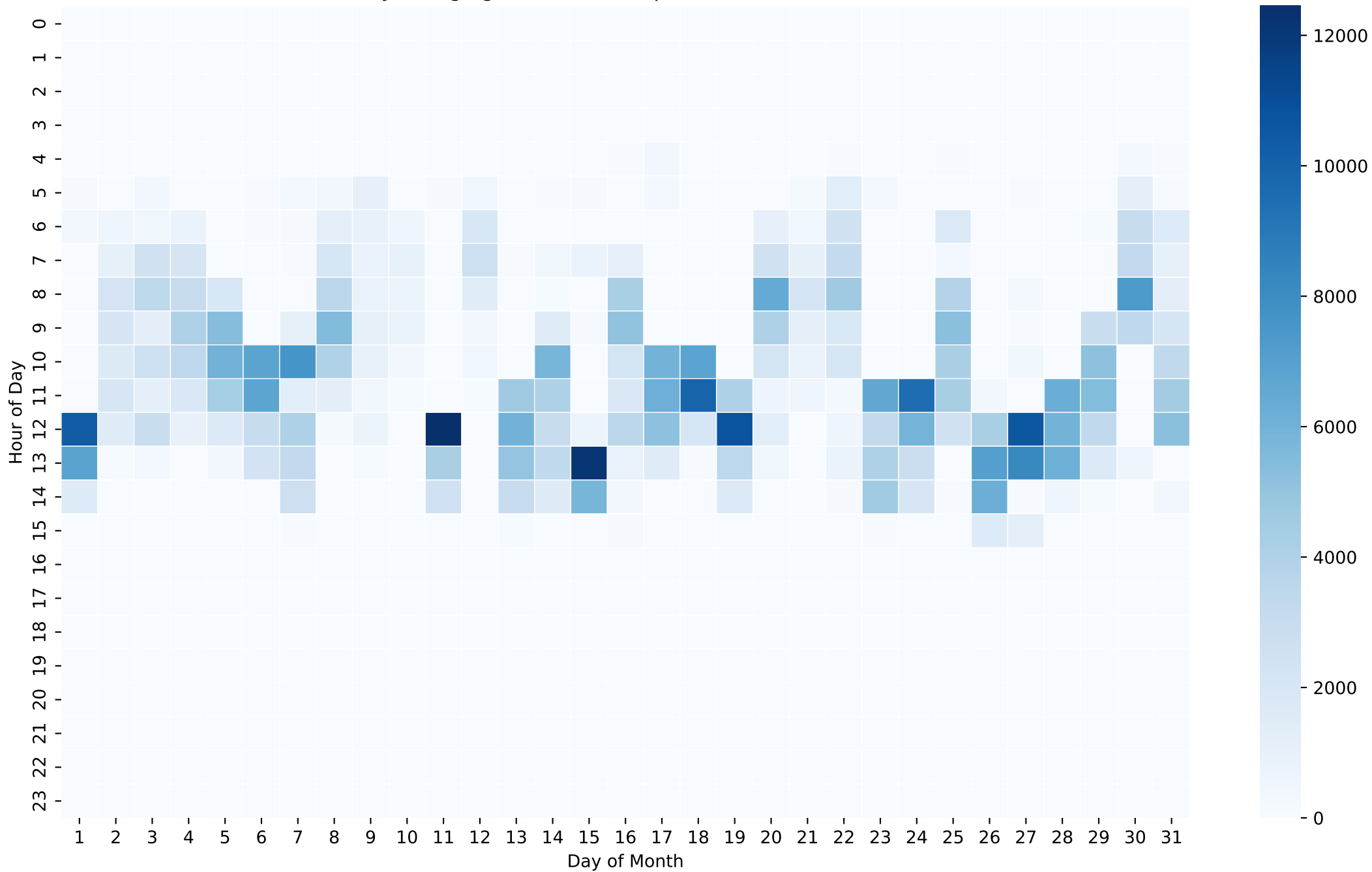
Battery Charging Power Heatmap (Wh/Hour) - 20kWh - Mar
