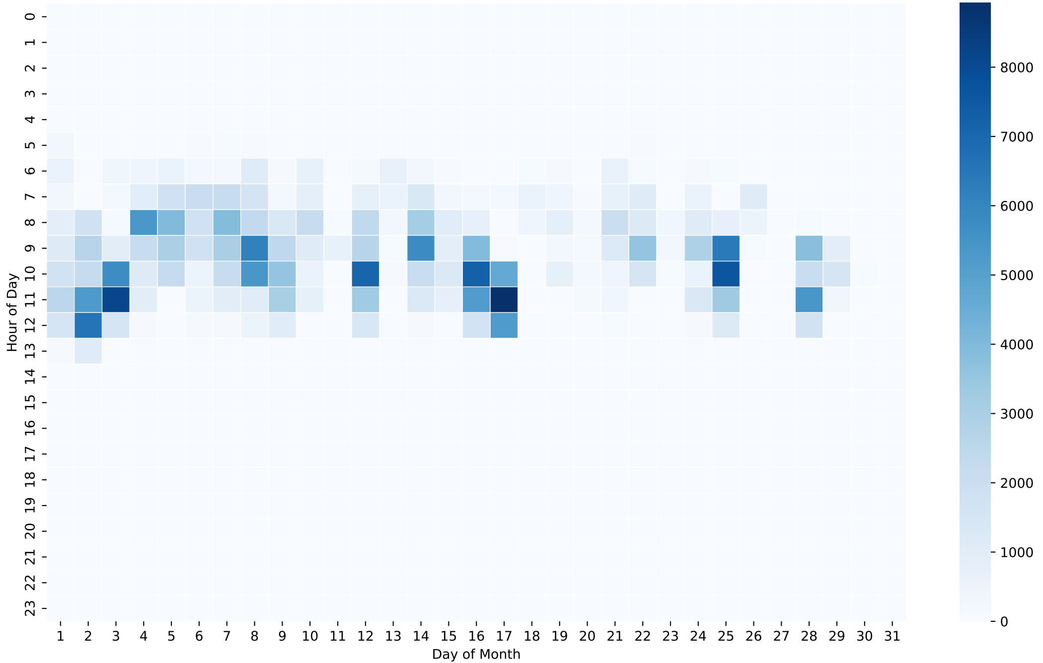
Battery Charging Power Heatmap (Wh/Hour) - 20kWh - Nov
