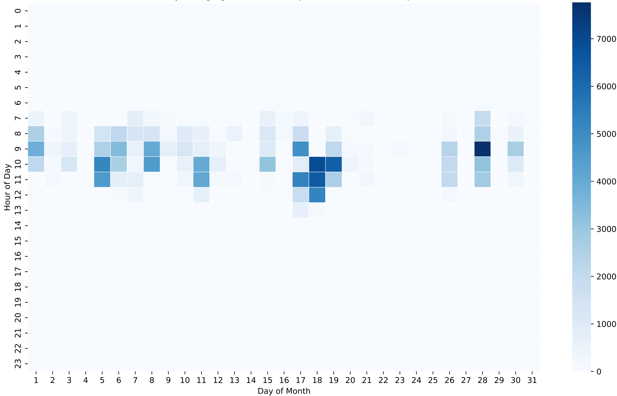
Battery Charging Power Heatmap (Wh/Hour) - 20kWh - Jan
