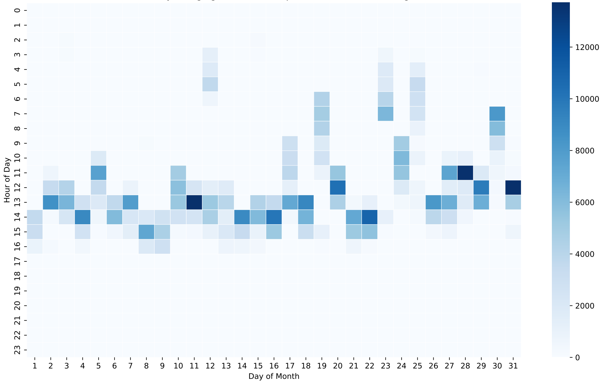
Battery Charging Power Heatmap (Wh/Hour) - 20kWh - Aug
