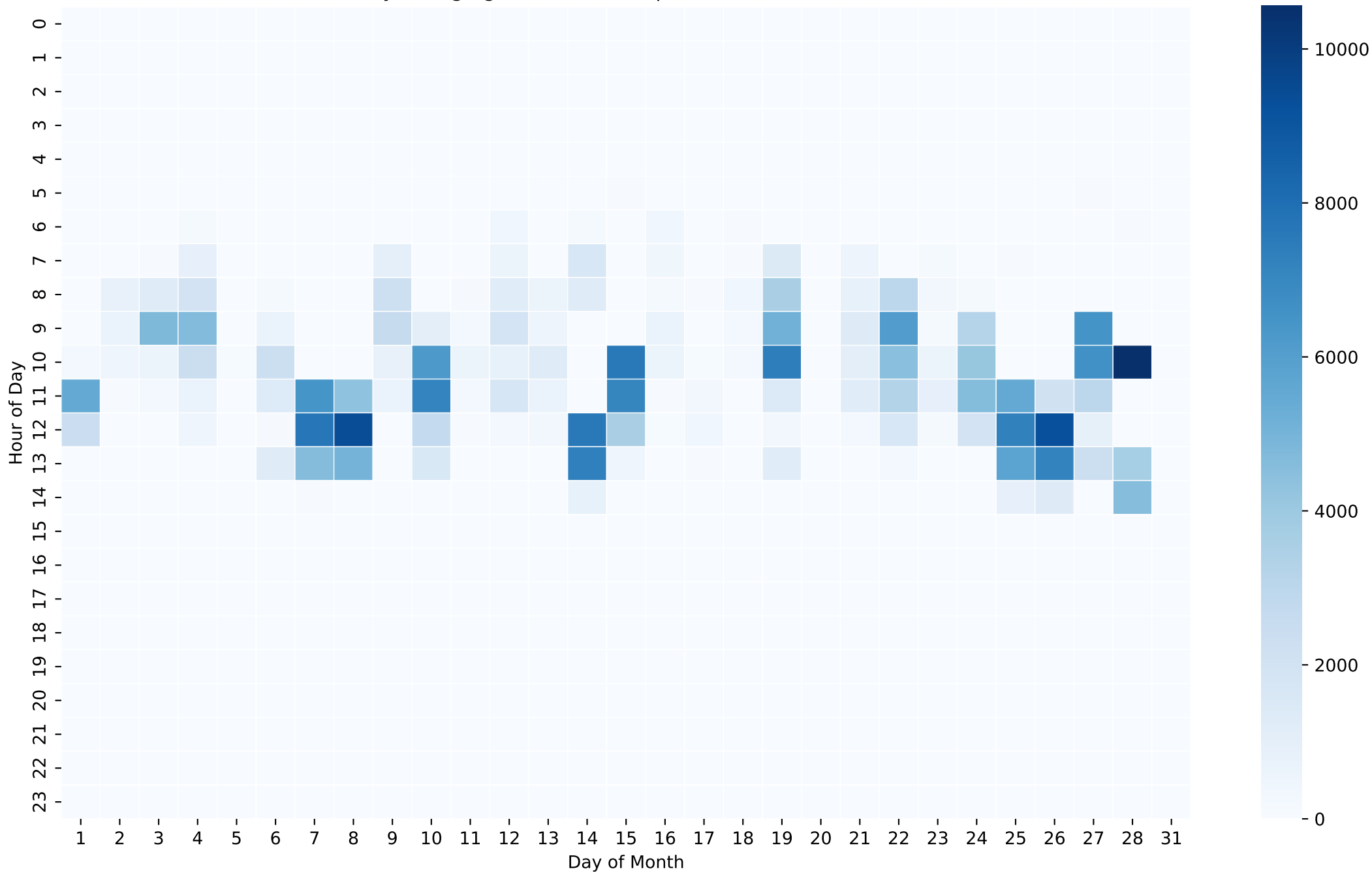
Battery Charging Power Heatmap (Wh/Hour) - 20kWh - Feb
