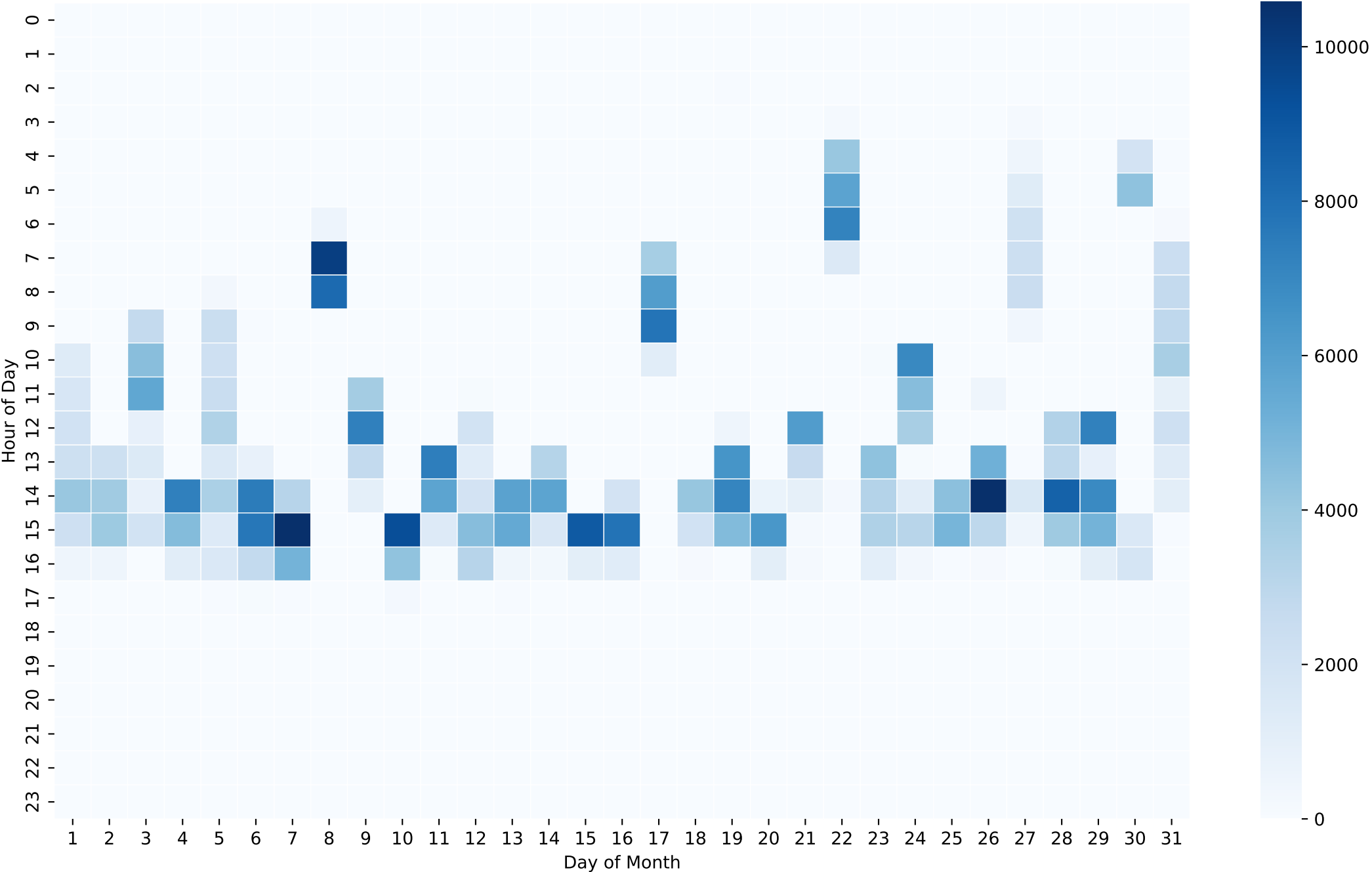
Battery Charging Power Heatmap (Wh/Hour) - 20kWh - Jul
