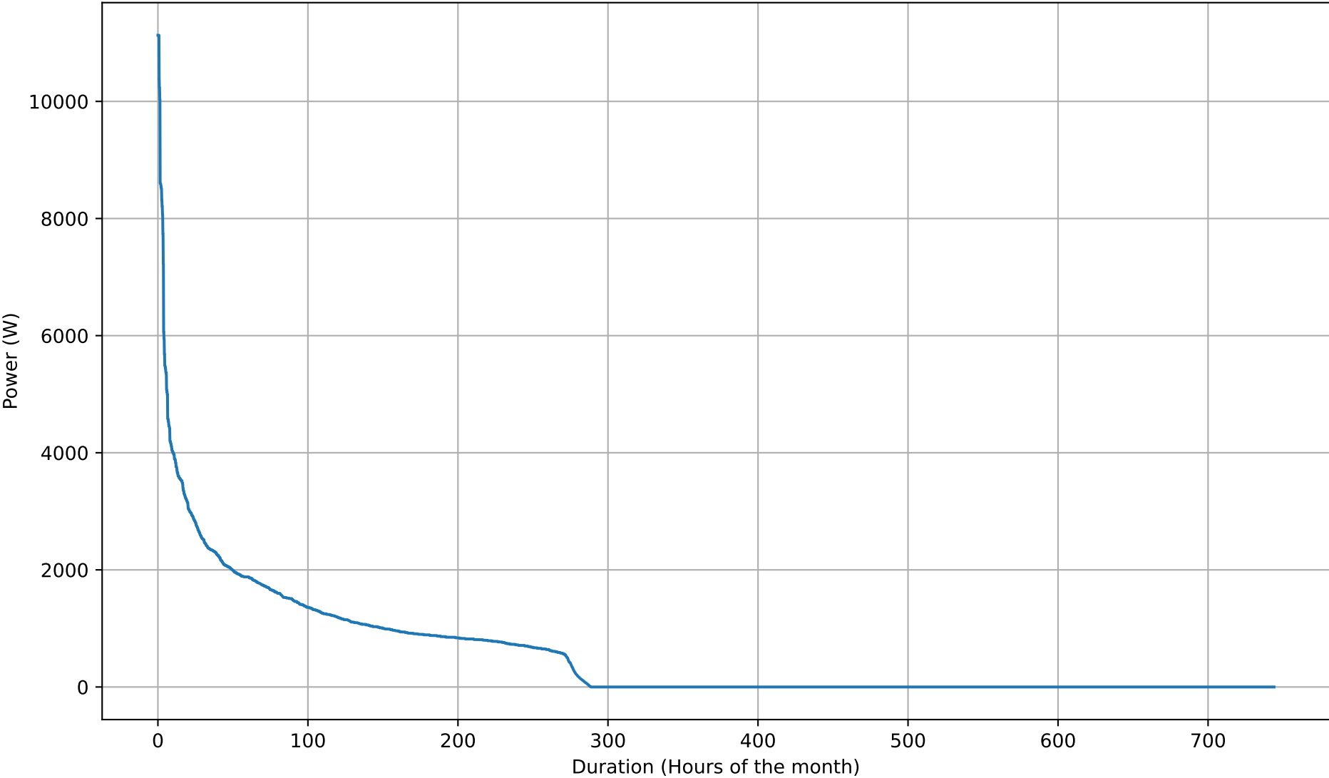
Battery Discharging Power Duration Curve - 20kWh - Jul
