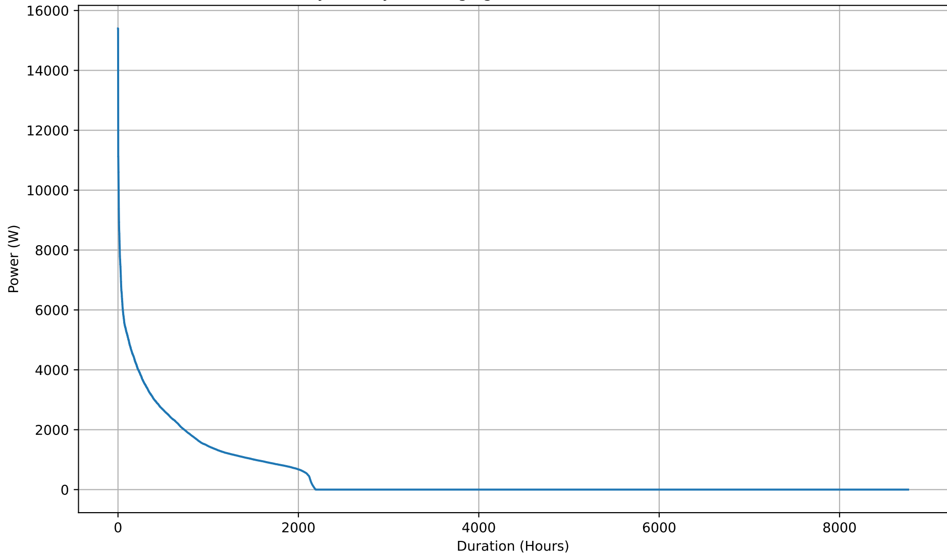
Yearly Battery Discharging Power Duration Curve - 20kWh
