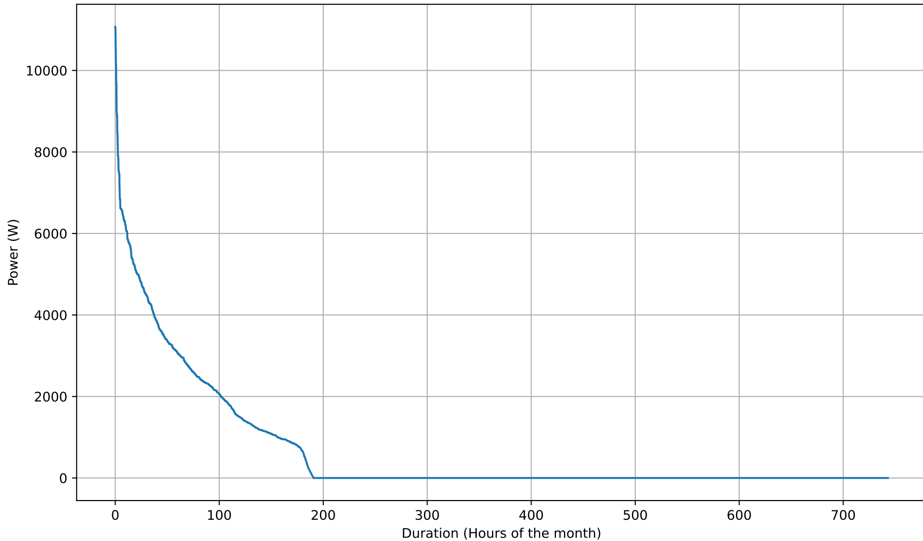
Battery Discharging Power Duration Curve - 20kWh - Mar
