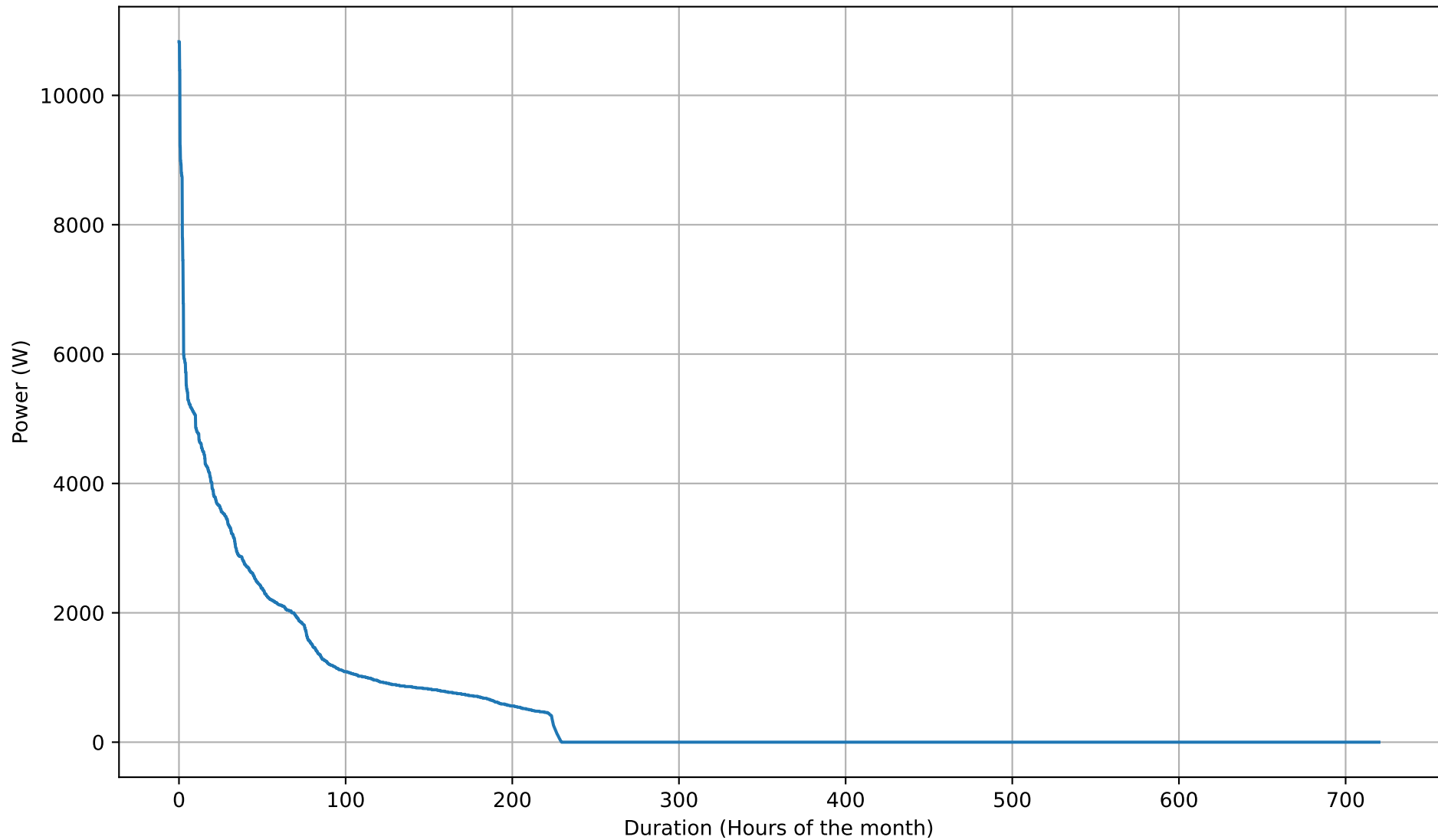
Battery Discharging Power Duration Curve - 20kWh - Jun
