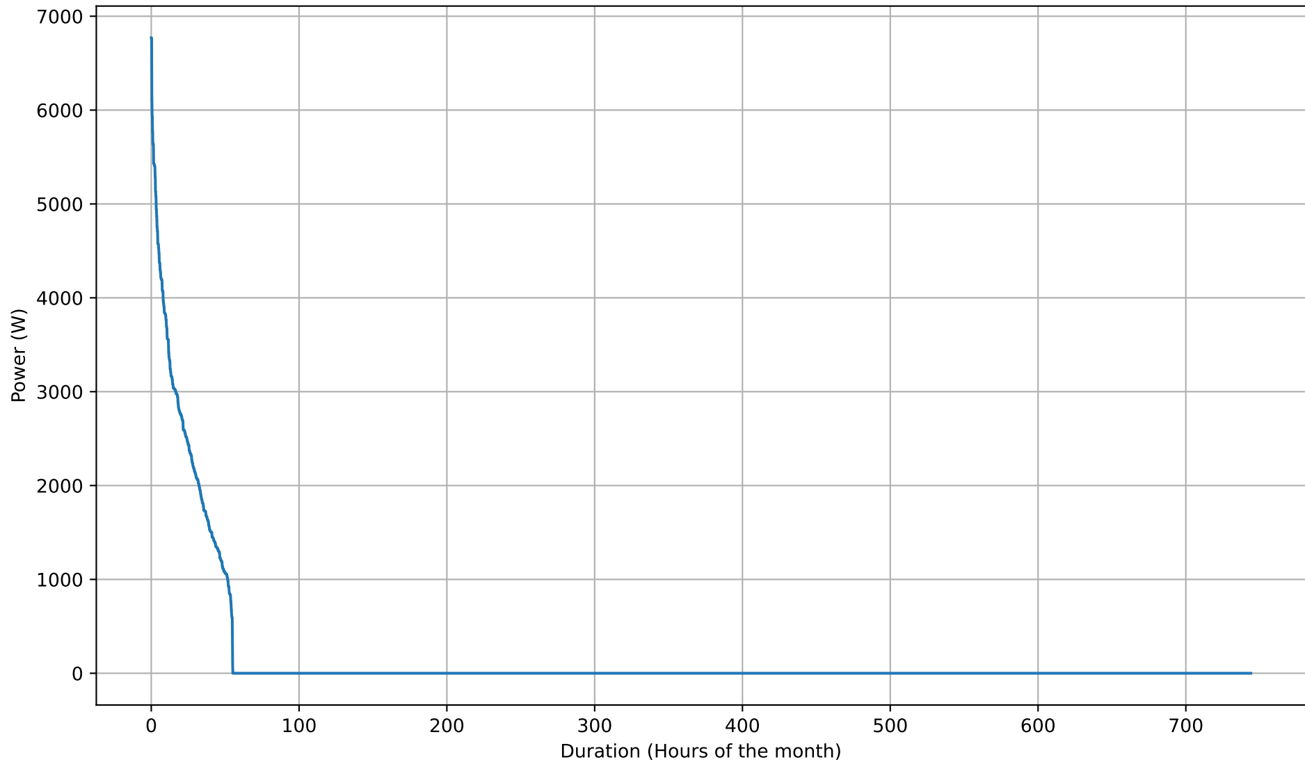
Battery Discharging Power Duration Curve - 20kWh - Jan
