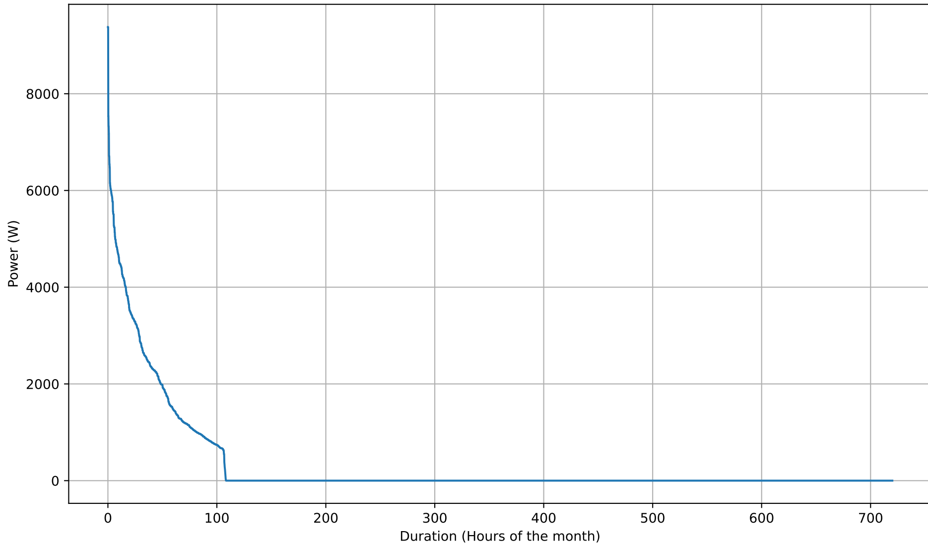
Battery Discharging Power Duration Curve - 20kWh - Nov
