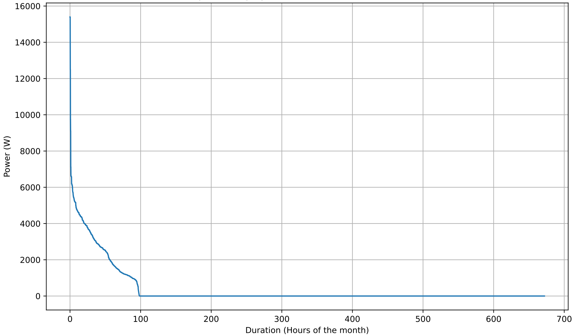
Battery Discharging Power Duration Curve - 20kWh - Feb
