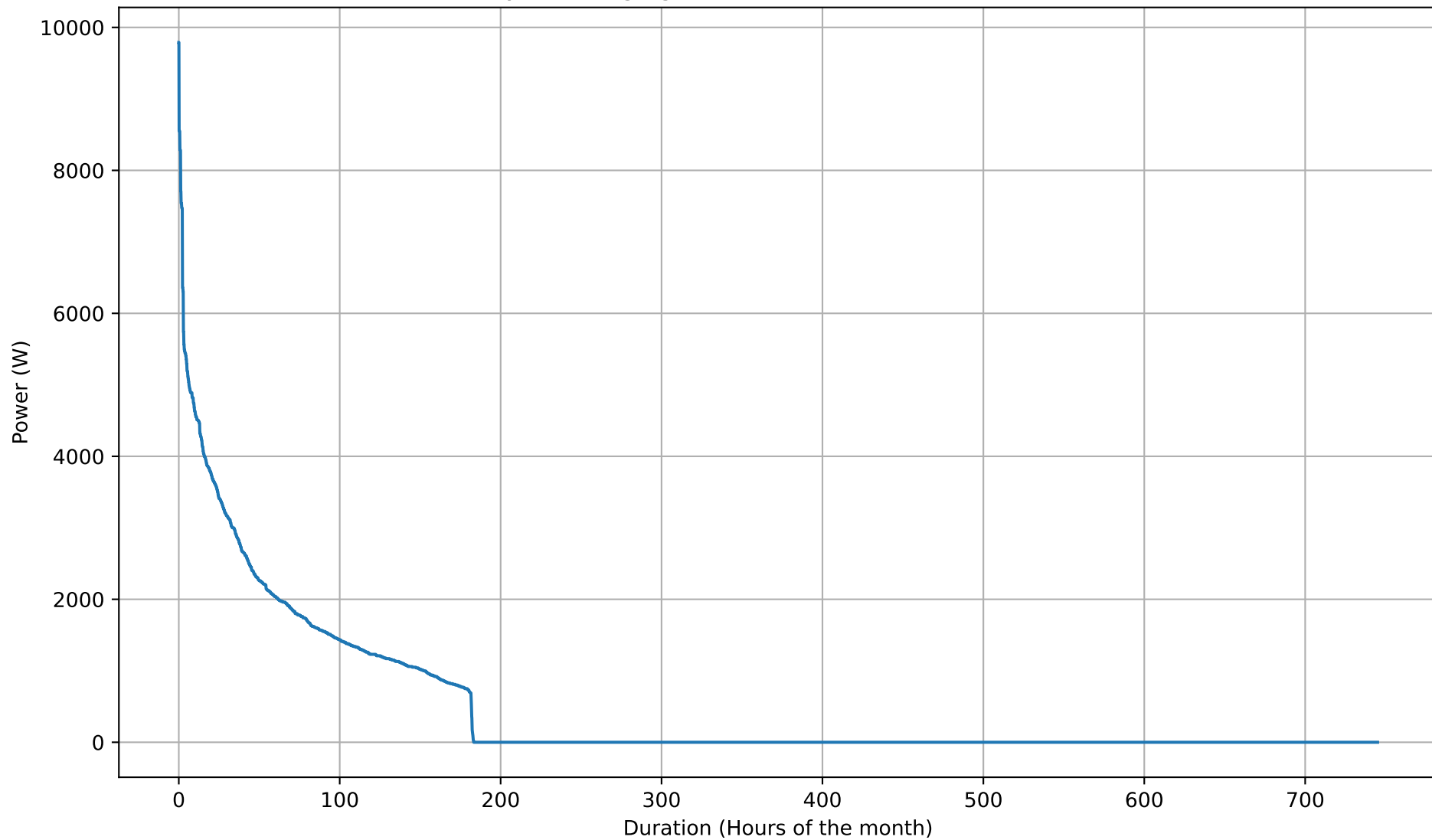
Battery Discharging Power Duration Curve - 20kWh - Oct
