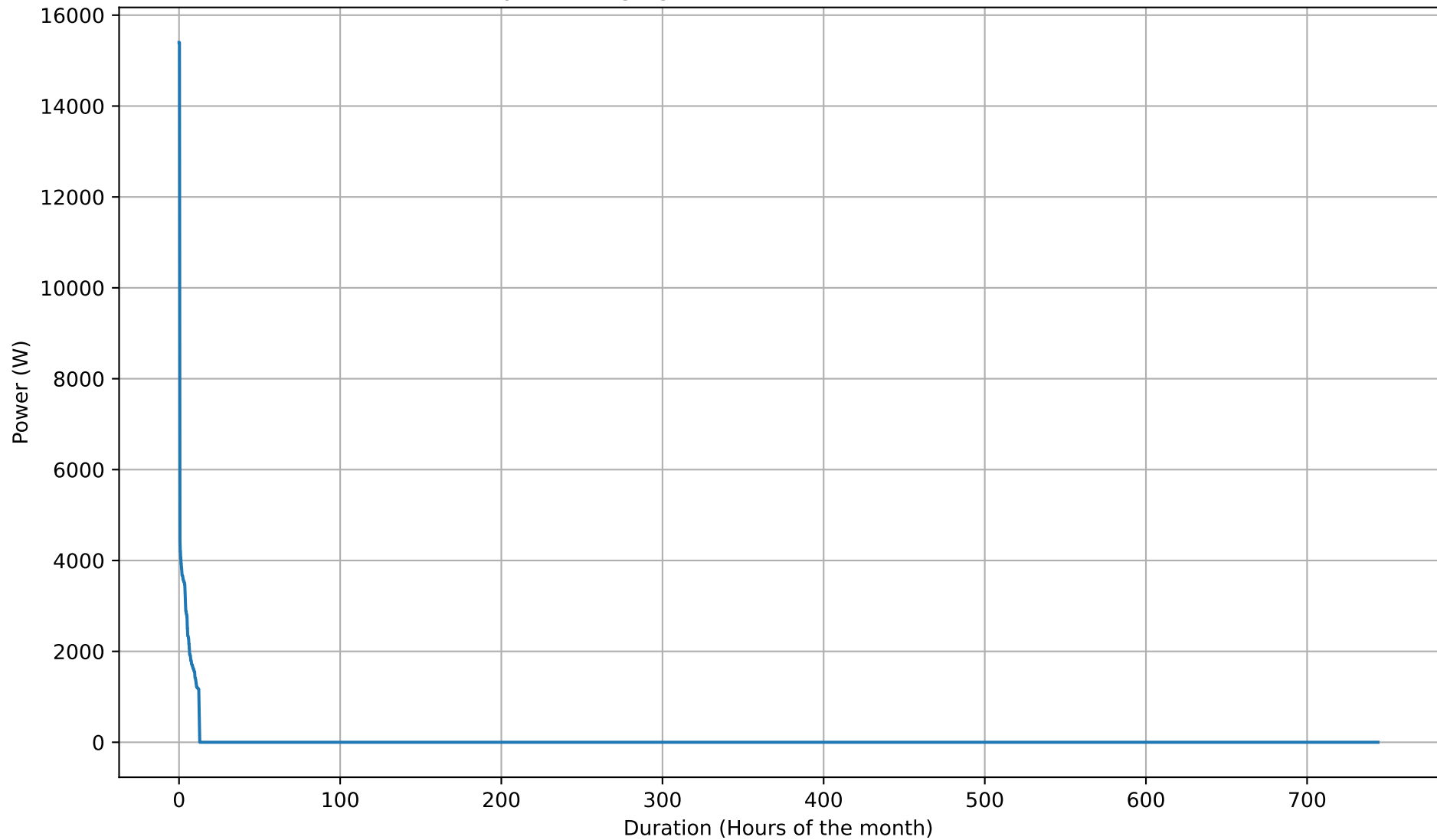
Battery Discharging Power Duration Curve - 20kWh - Dec
