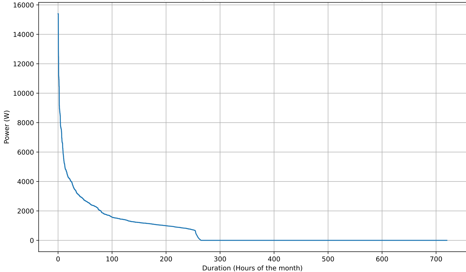
Battery Discharging Power Duration Curve - 20kWh - Sep
