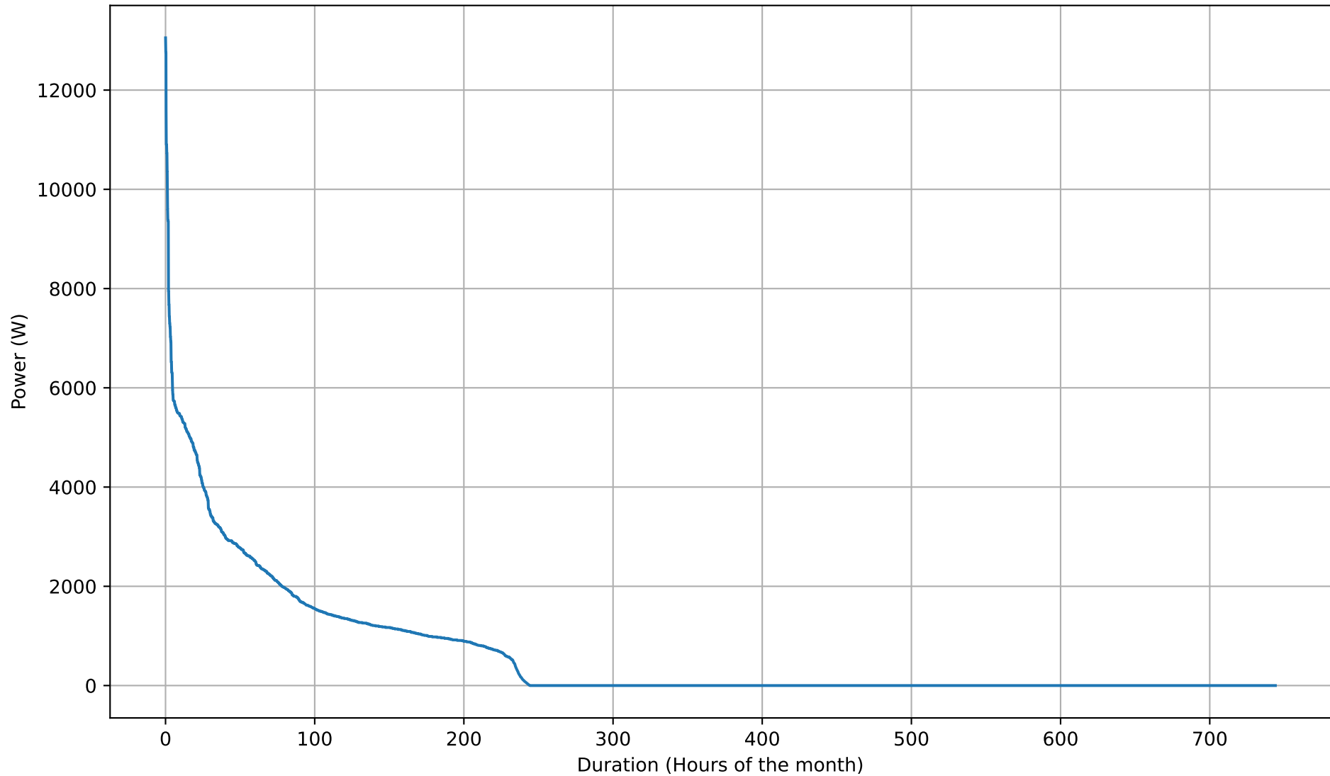
Battery Discharging Power Duration Curve - 20kWh - May
