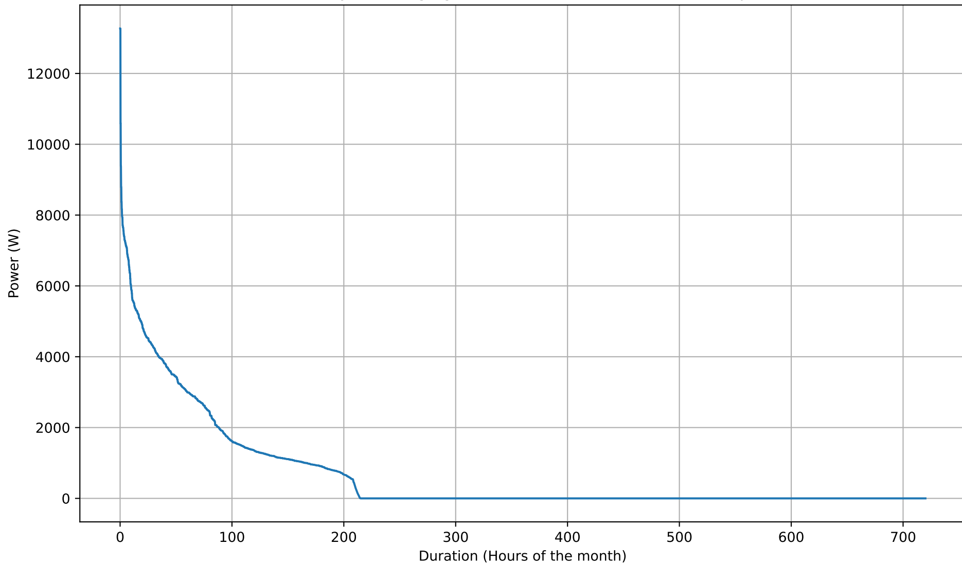
Battery Discharging Power Duration Curve - 20kWh - Apr
