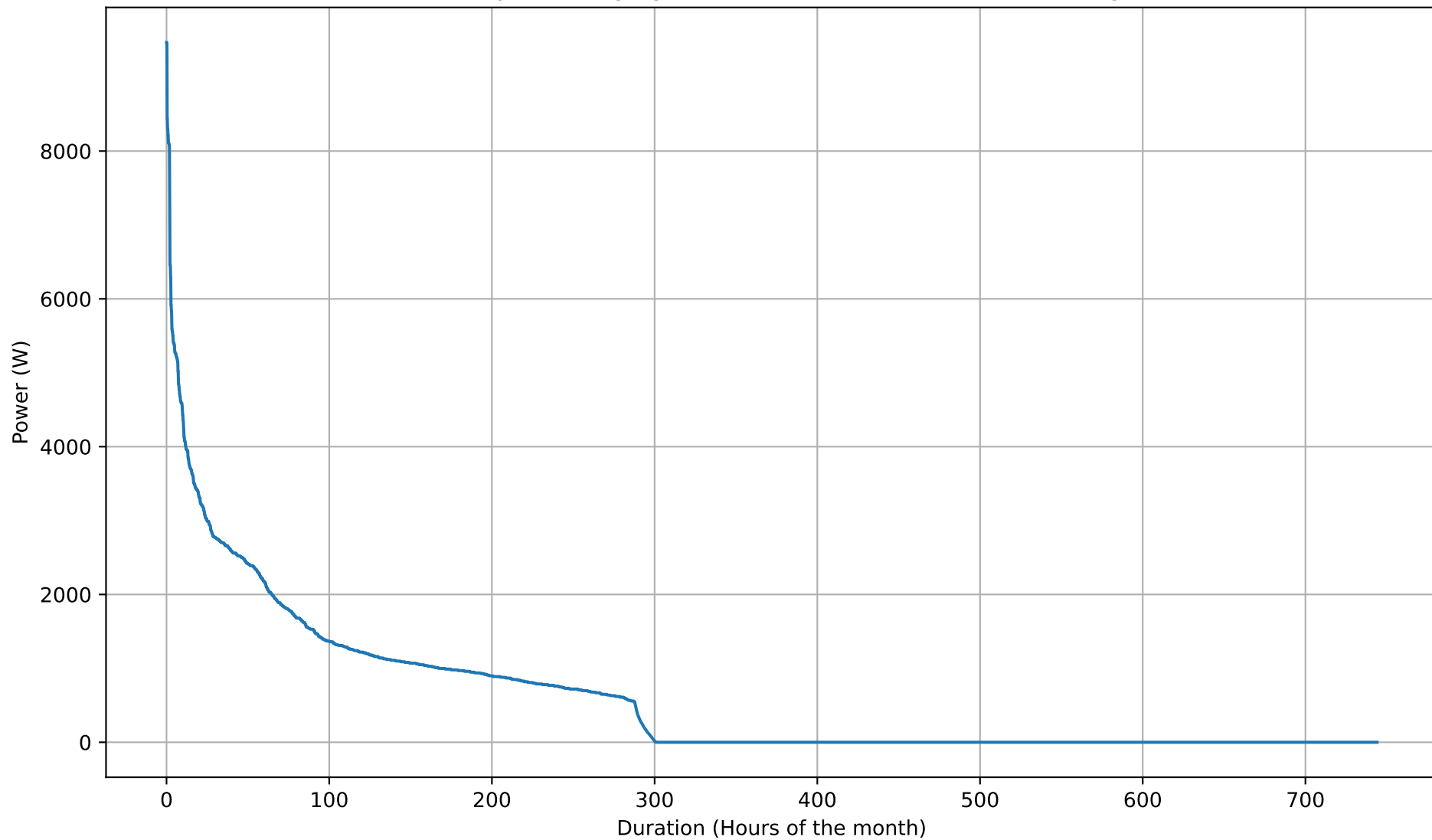
Battery Discharging Power Duration Curve - 20kWh - Aug
