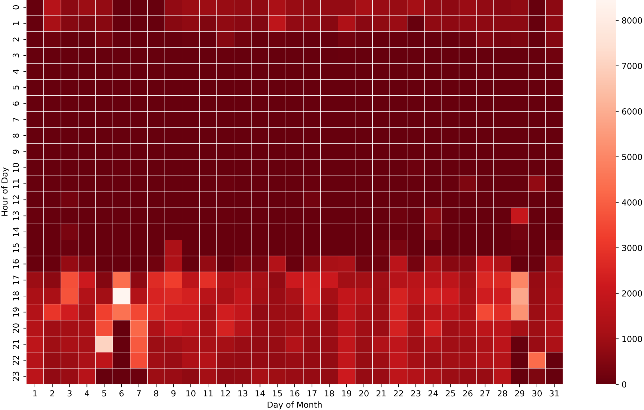
Battery Discharging Power Heatmap (Wh/Hour) - 20kWh - Jul
