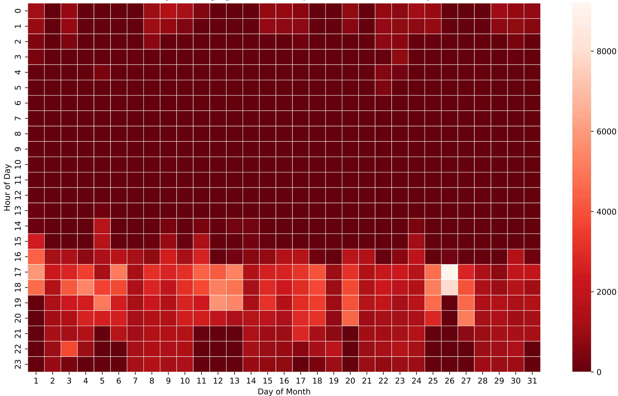
Battery Discharging Power Heatmap (Wh/Hour) - 20kWh - May
