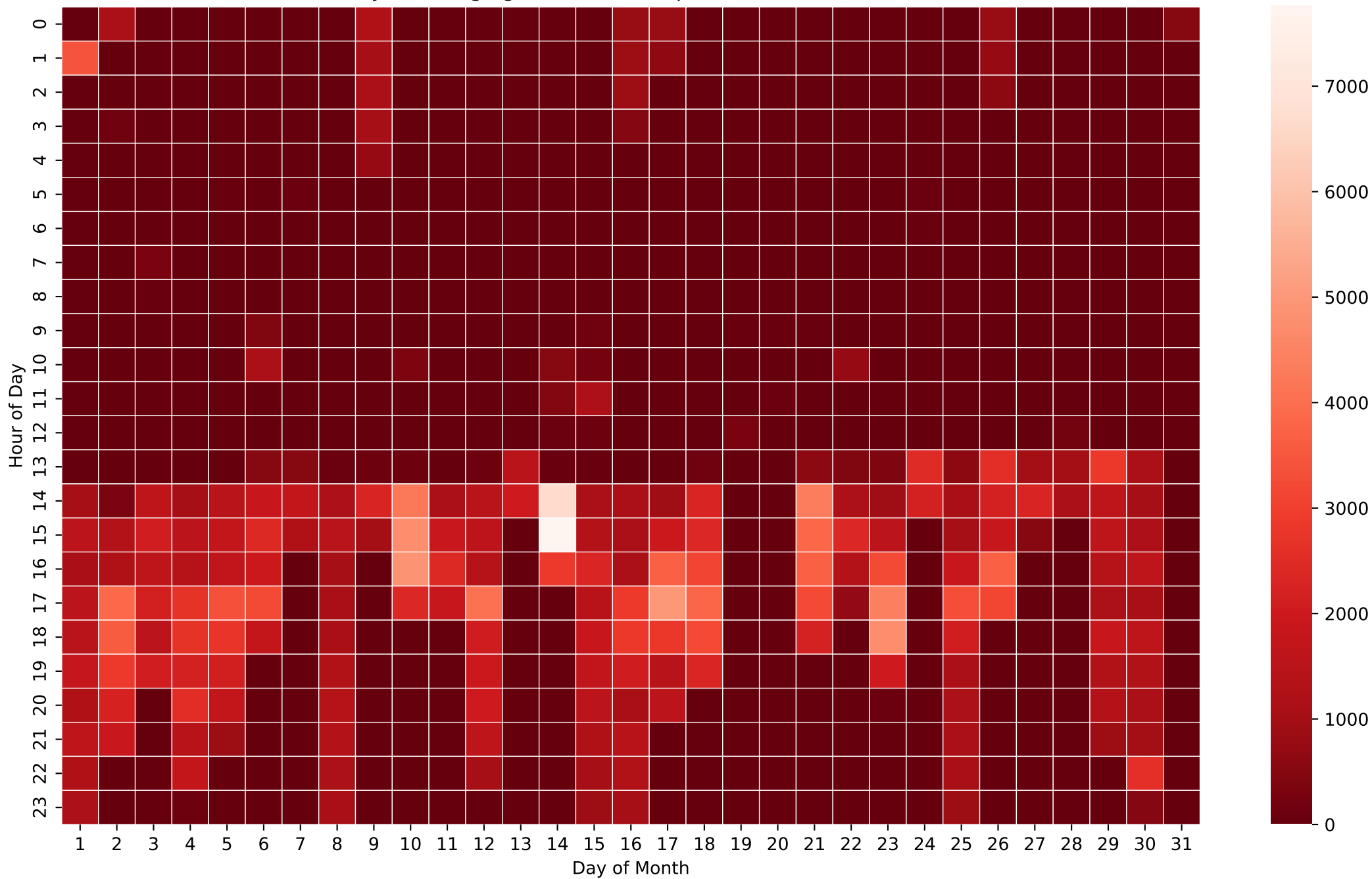
Battery Discharging Power Heatmap (Wh/Hour) - 20kWh - Oct
