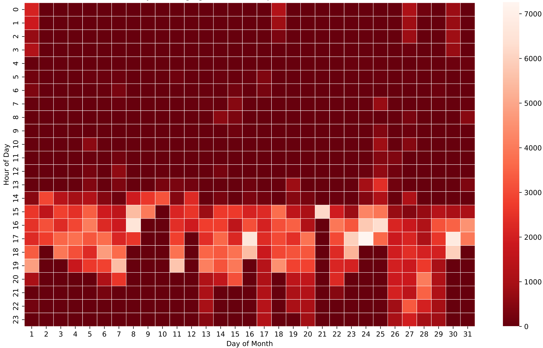
Battery Discharging Power Heatmap (Wh/Hour) - 20kWh - Mar
