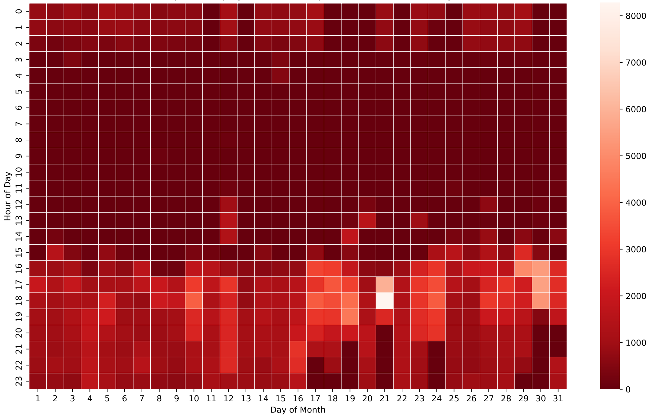
Battery Discharging Power Heatmap (Wh/Hour) - 20kWh - Aug
