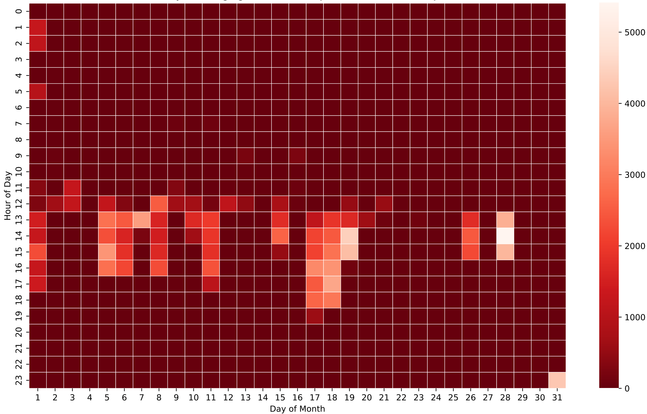
Battery Discharging Power Heatmap (Wh/Hour) - 20kWh - Jan
