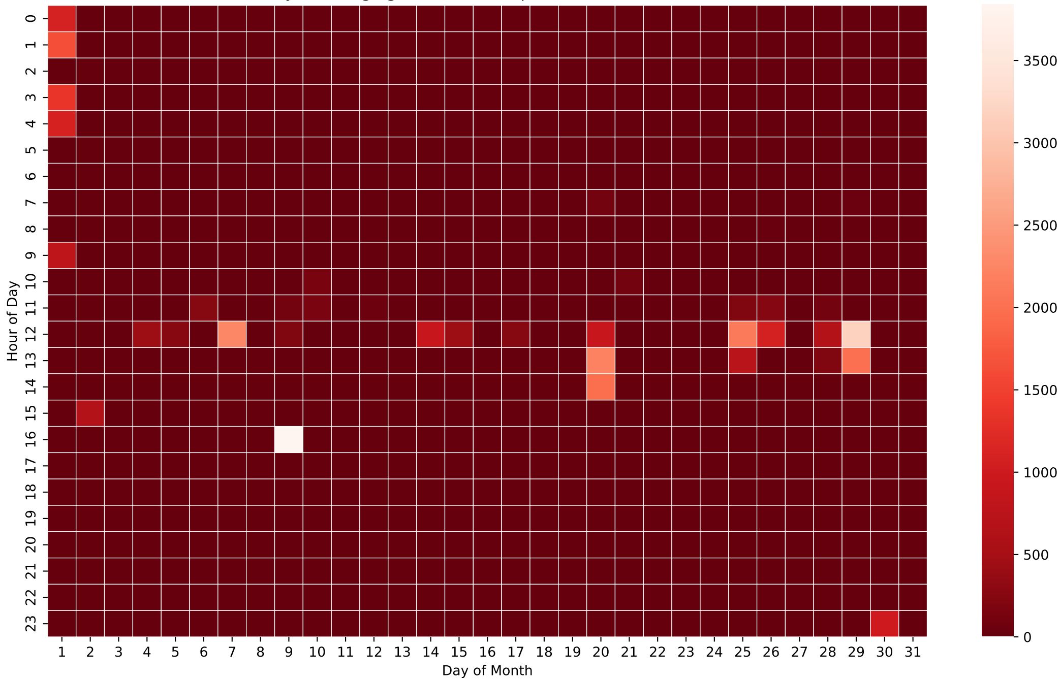
Battery Discharging Power Heatmap (Wh/Hour) - 20kWh - Dec
