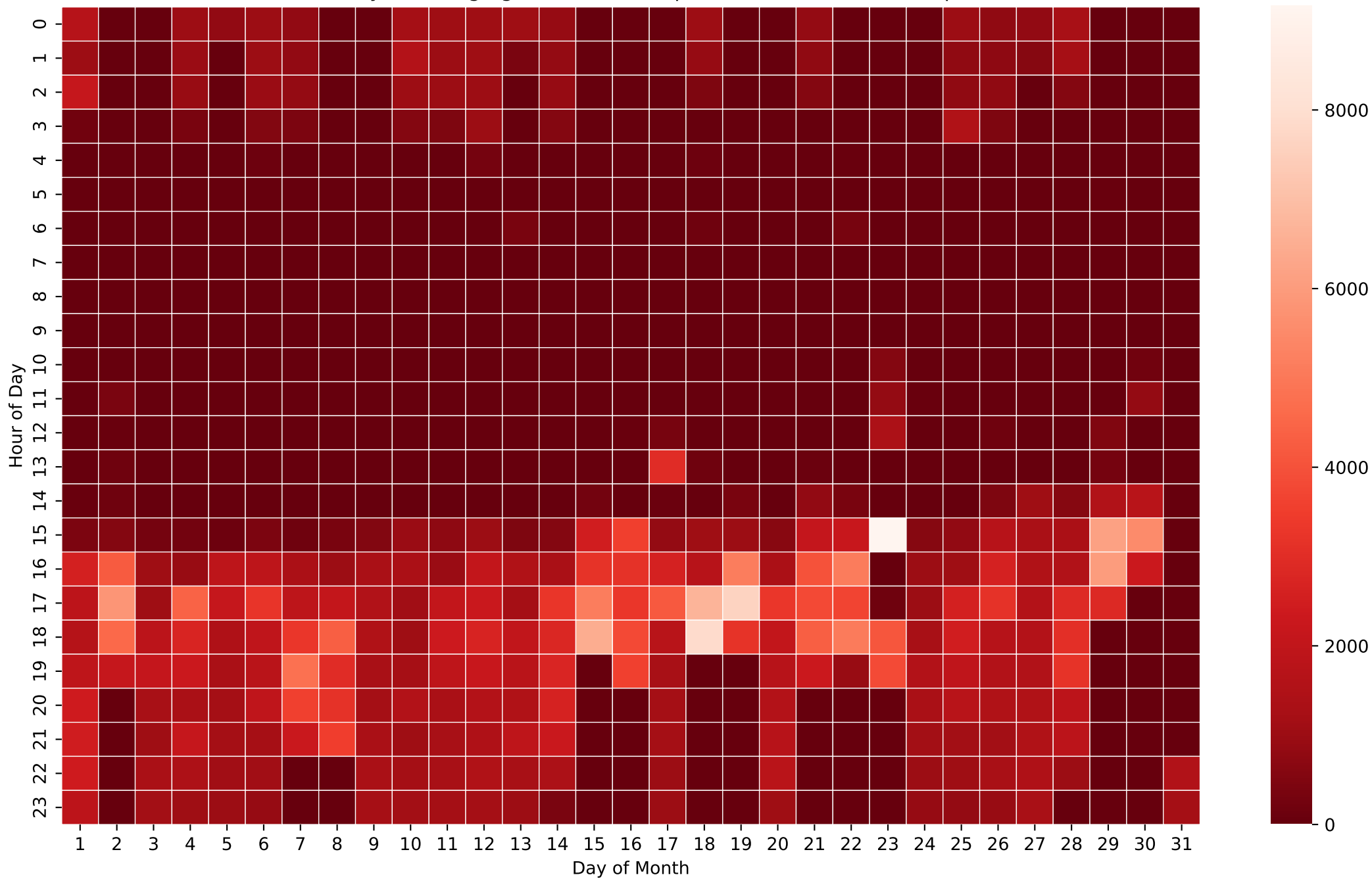
Battery Discharging Power Heatmap (Wh/Hour) - 20kWh - Sep
