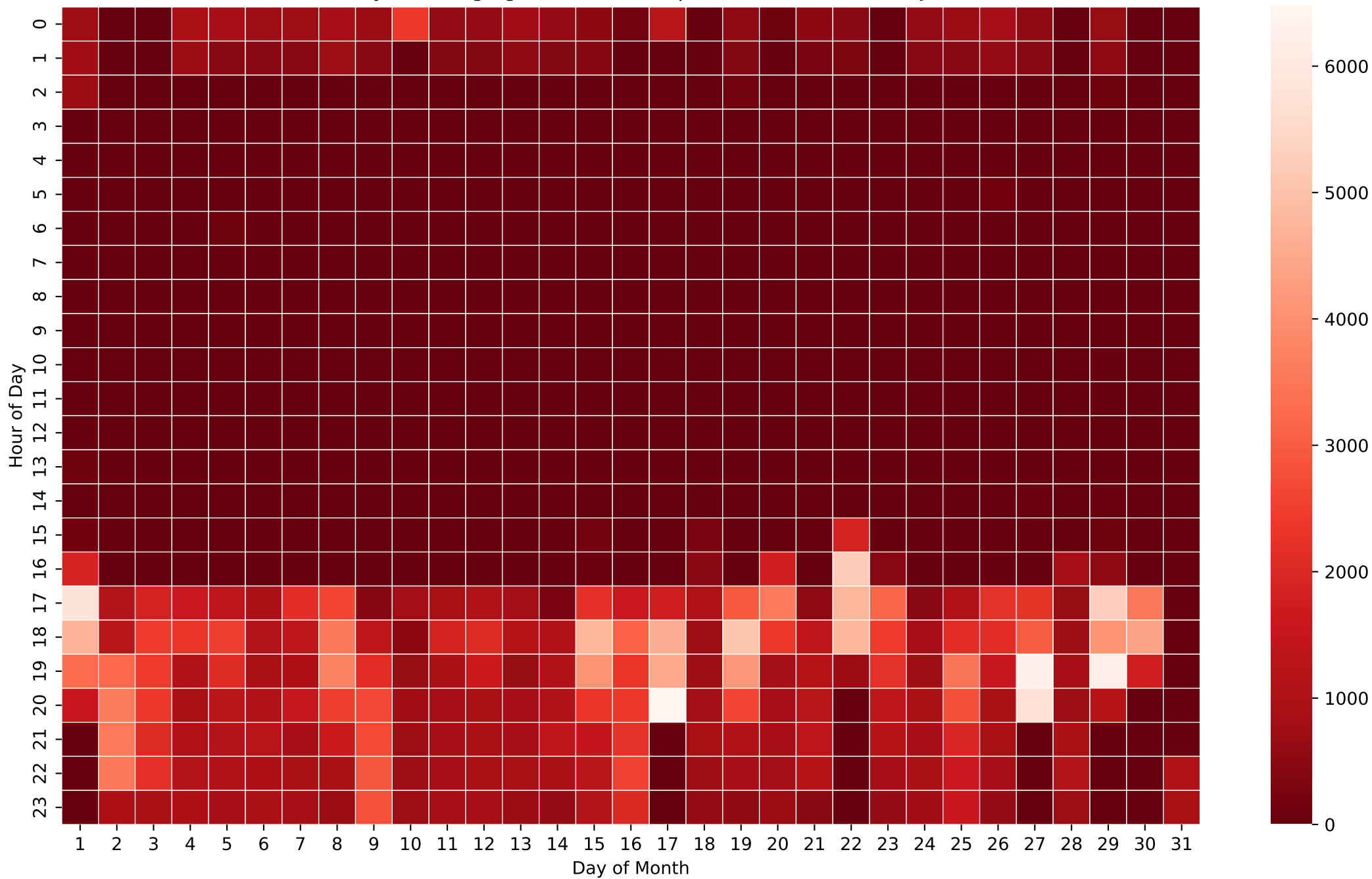
Battery Discharging Power Heatmap (Wh/Hour) - 20kWh - Jun
