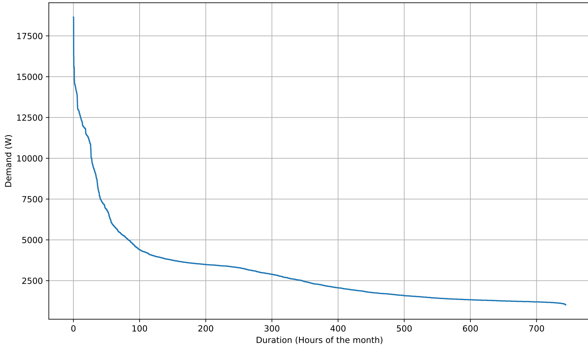
Electricity Demand Duration Curve - 20kWh - Dec
