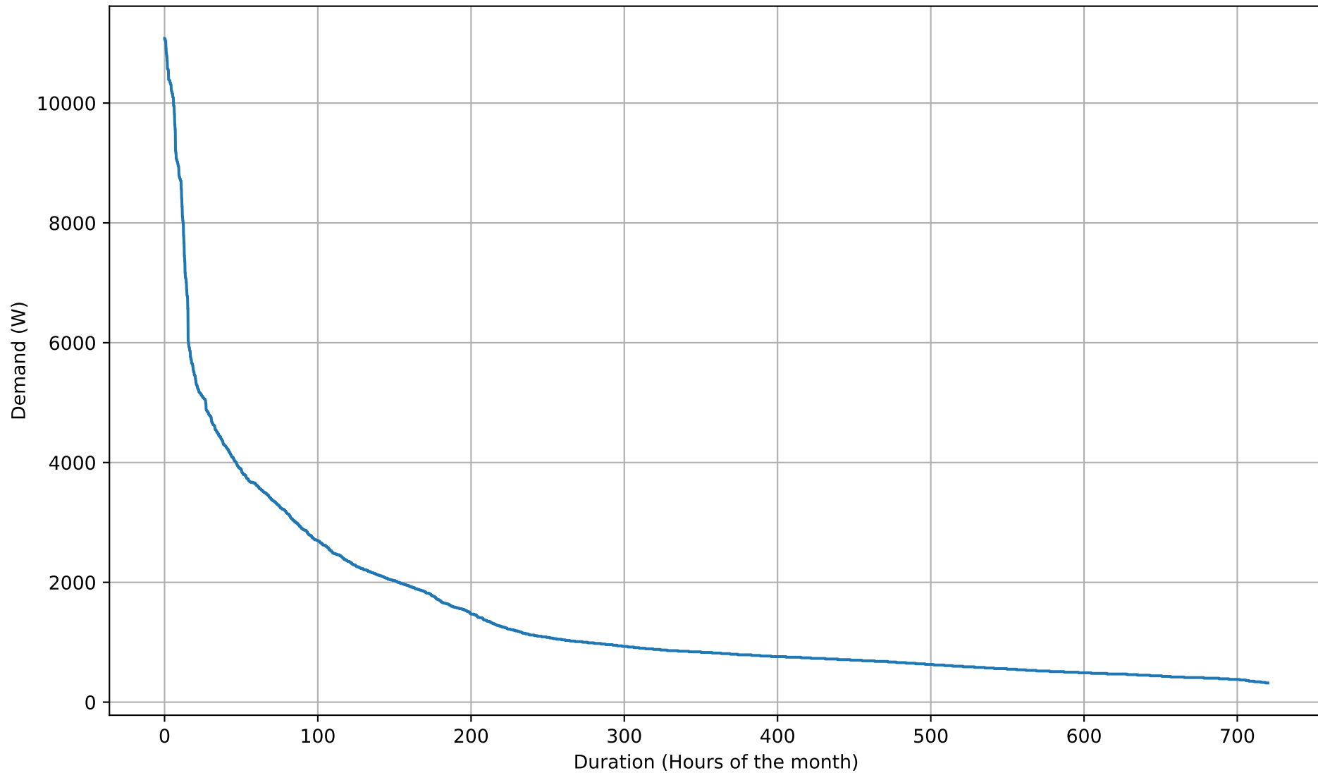
Electricity Demand Duration Curve - 20kWh - Jun
