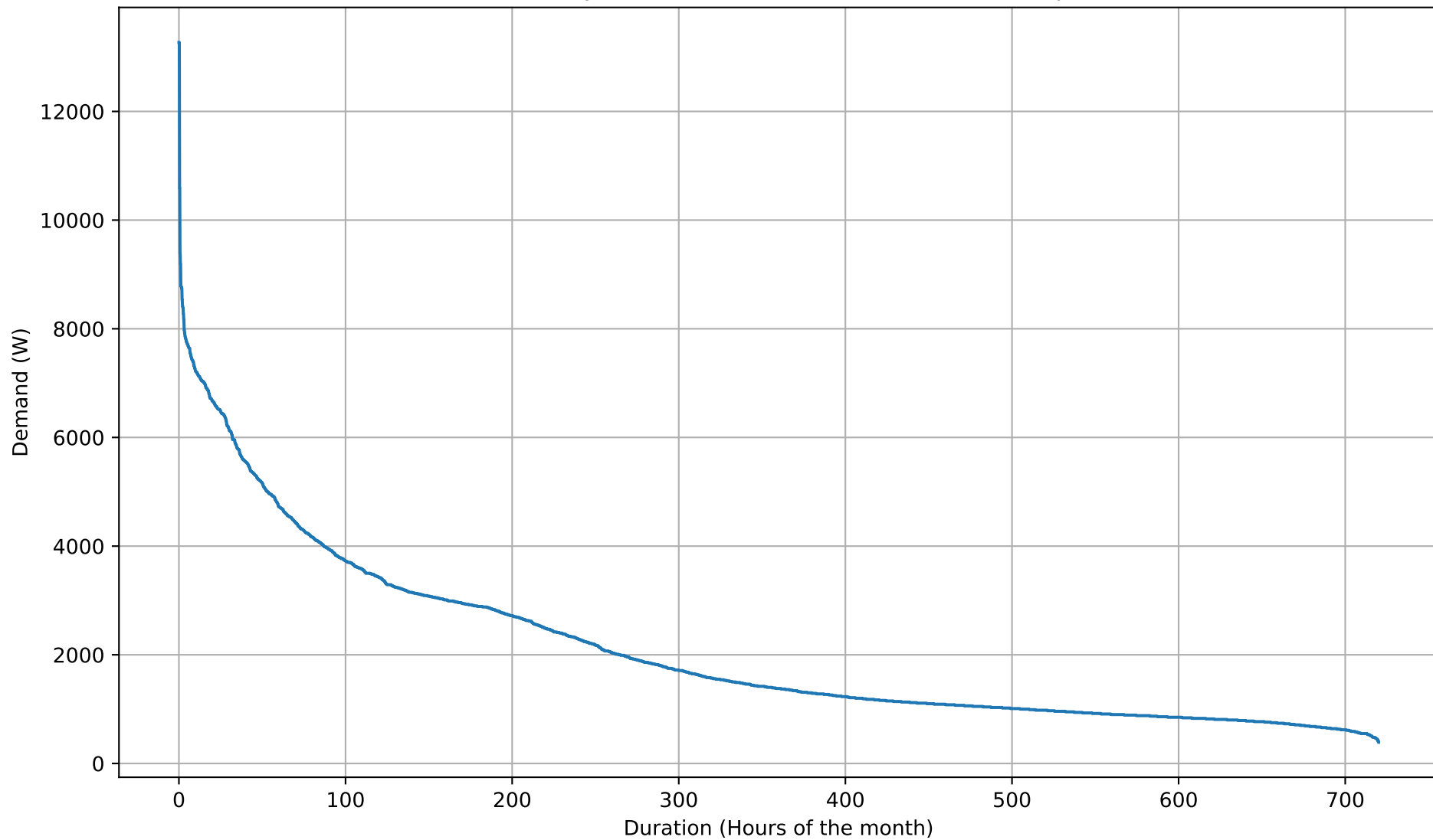
Electricity Demand Duration Curve - 20kWh - Apr
