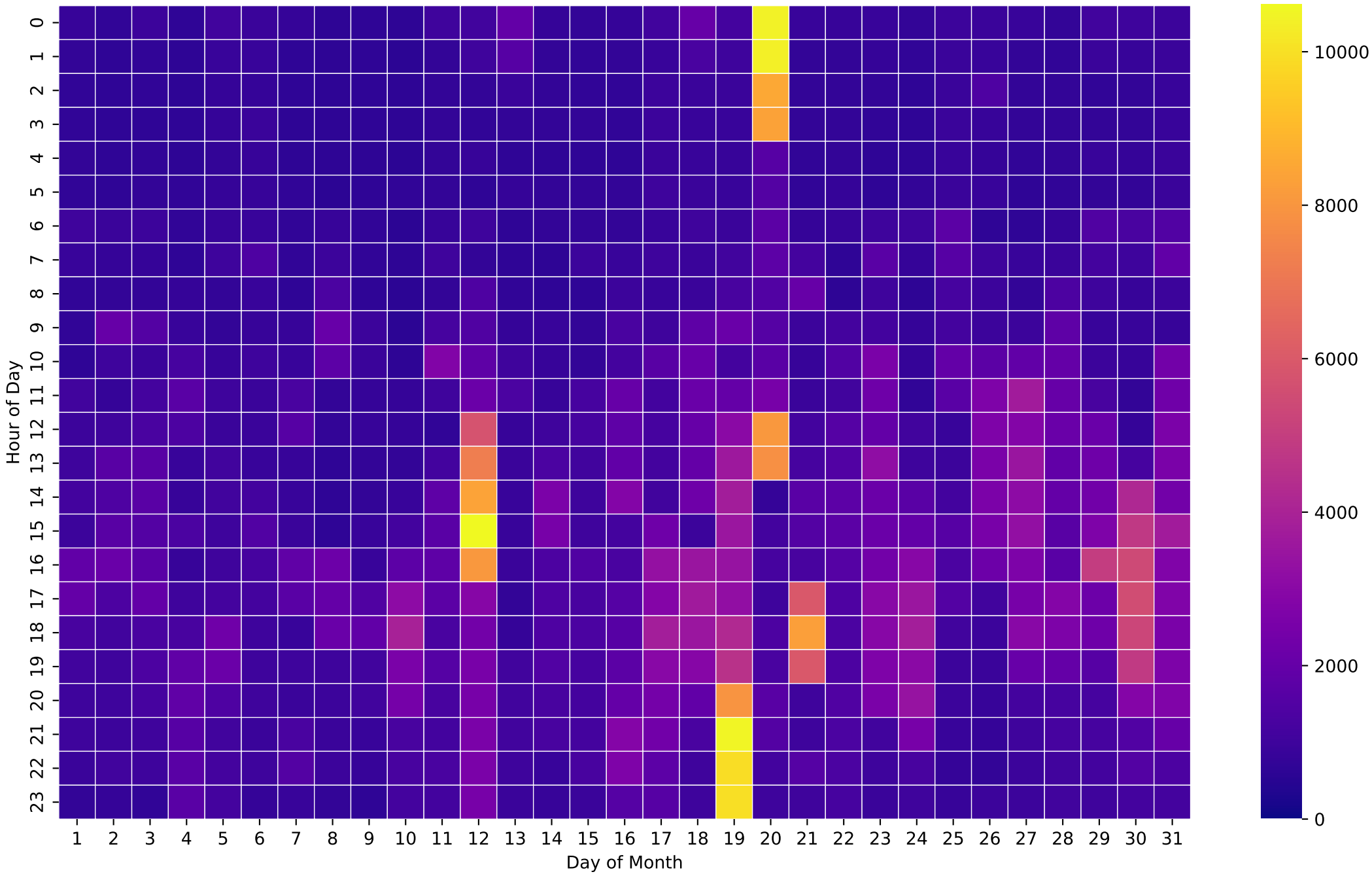
Electricity Demand Heatmap (Wh/Hour) - 20kWh - Aug
