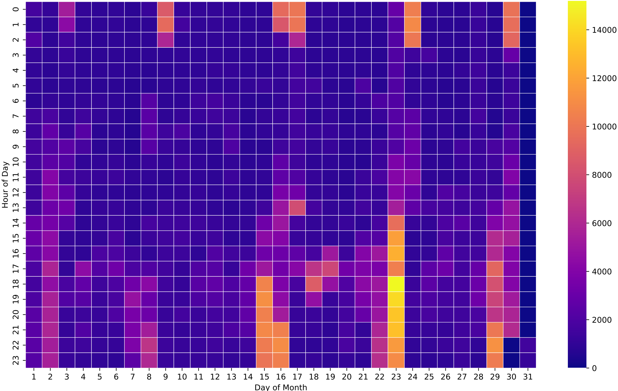
Electricity Demand Heatmap (Wh/Hour) - 20kWh - Sep
