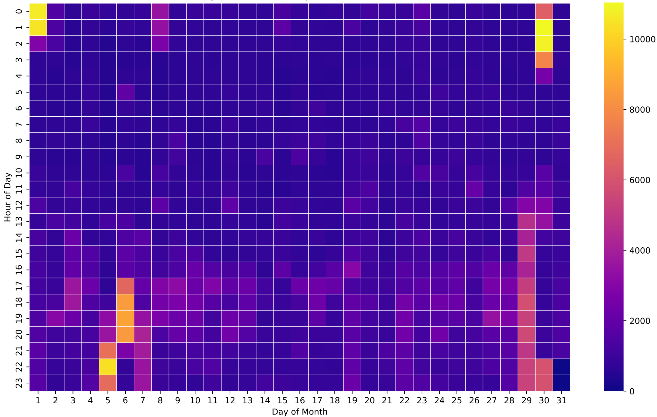
Electricity Demand Heatmap (Wh/Hour) - 20kWh - Jul
