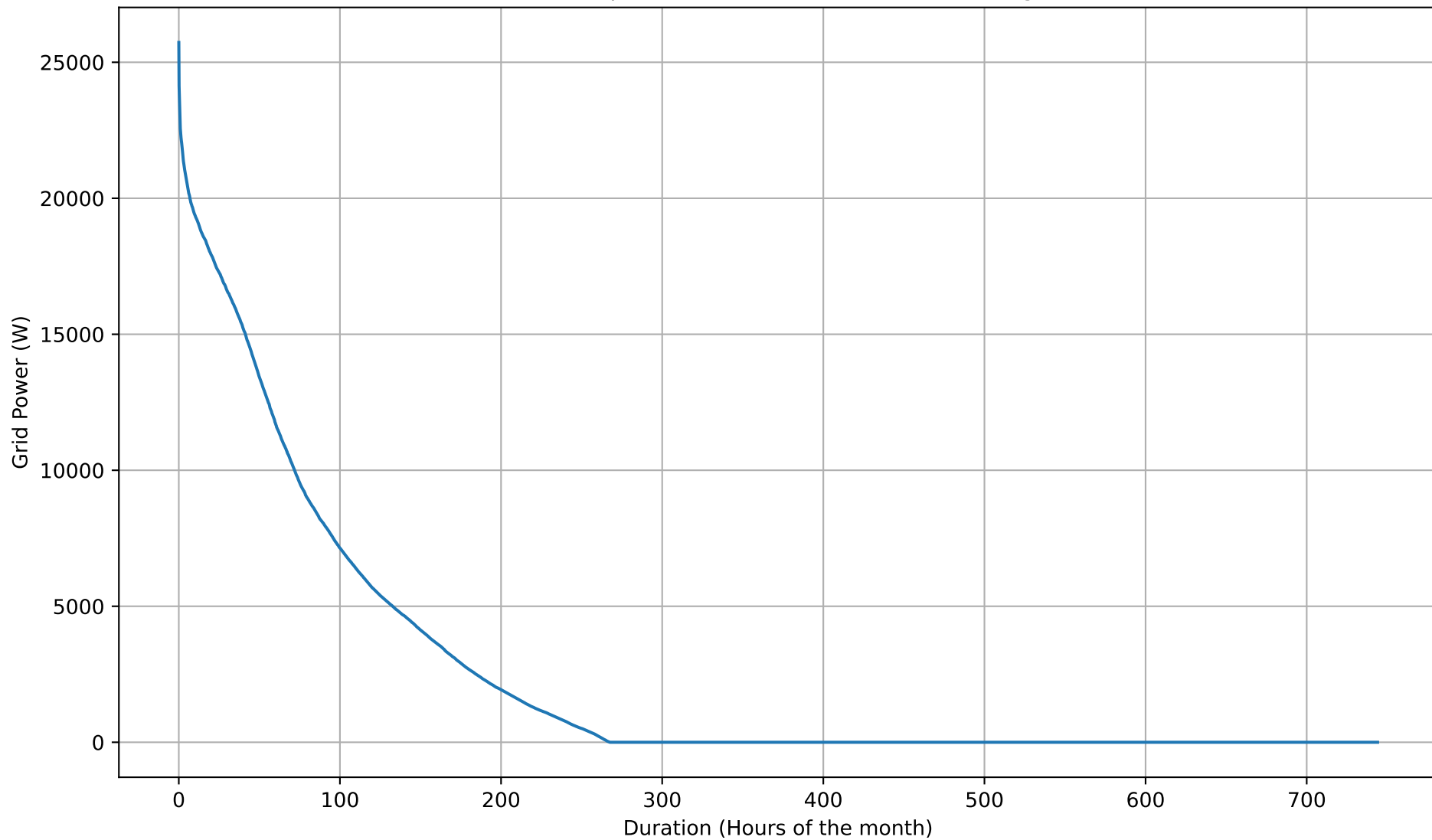
Grid Export Duration Curve - 20kWh - Aug
