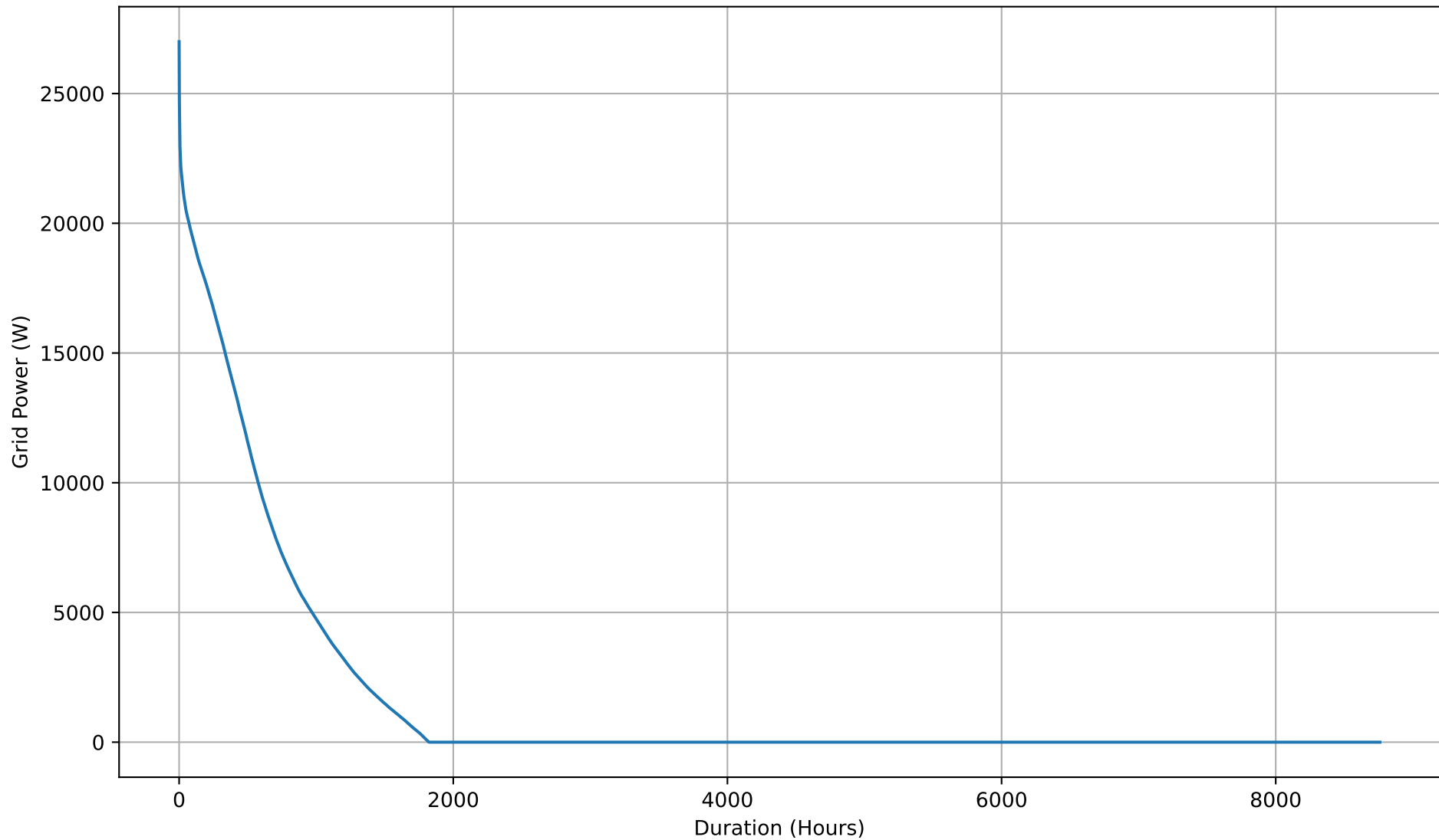
Yearly Grid Export Duration Curve - 20kWh
