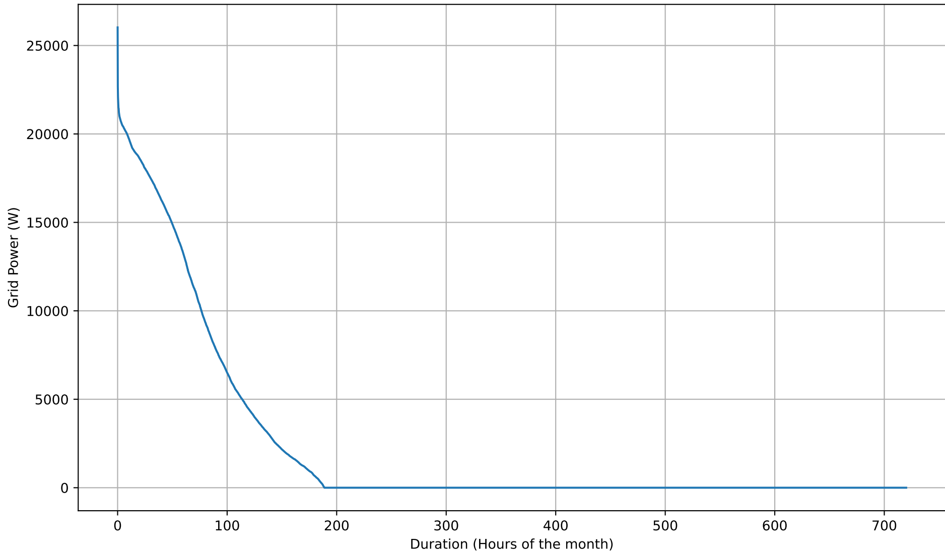
Grid Export Duration Curve - 20kWh - Apr
