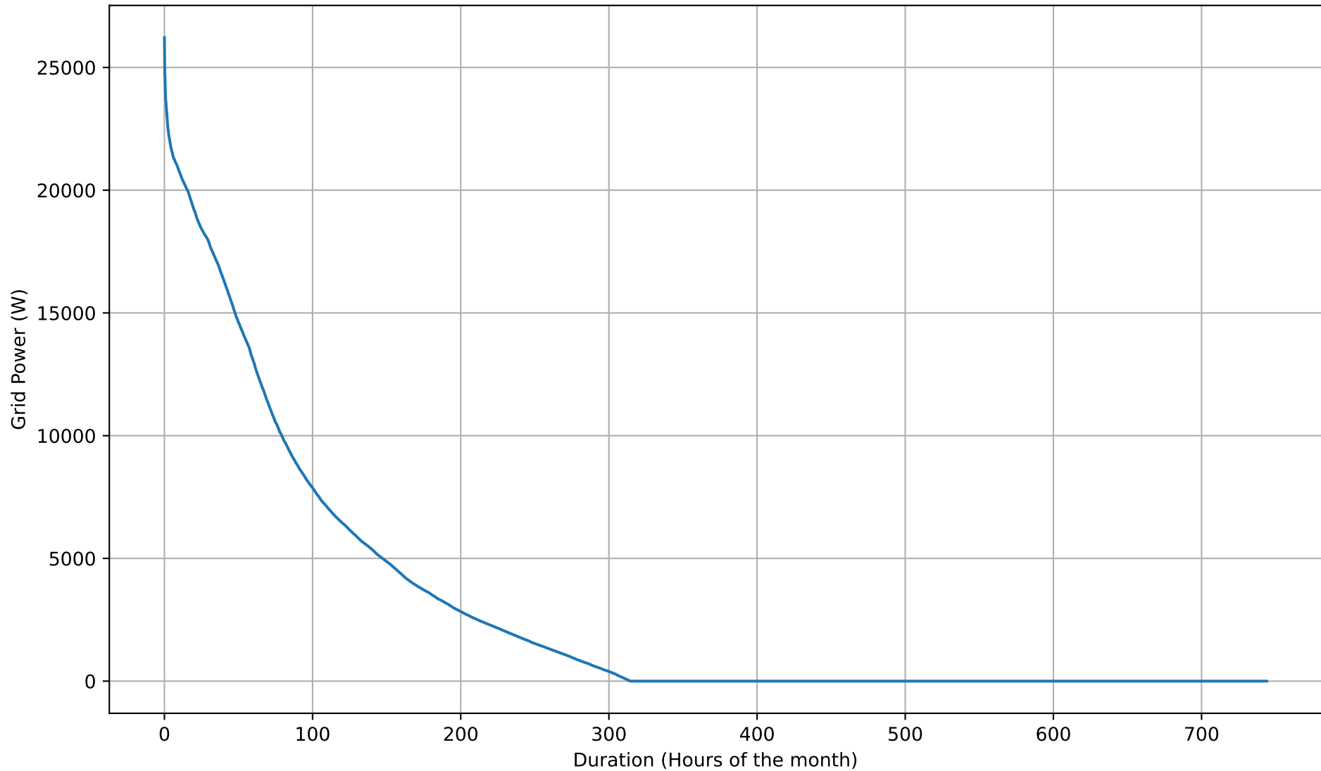
Grid Export Duration Curve - 20kWh - Jul
