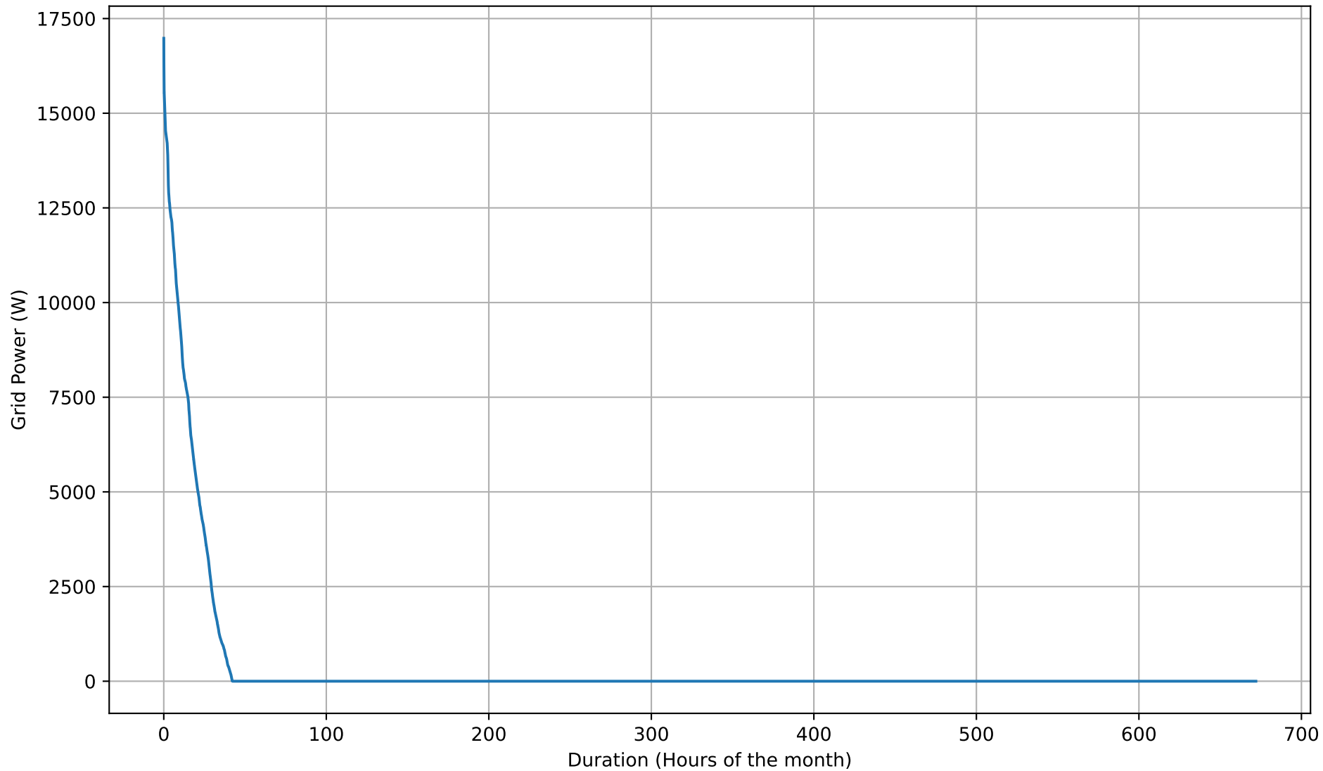
Grid Export Duration Curve - 20kWh - Feb
