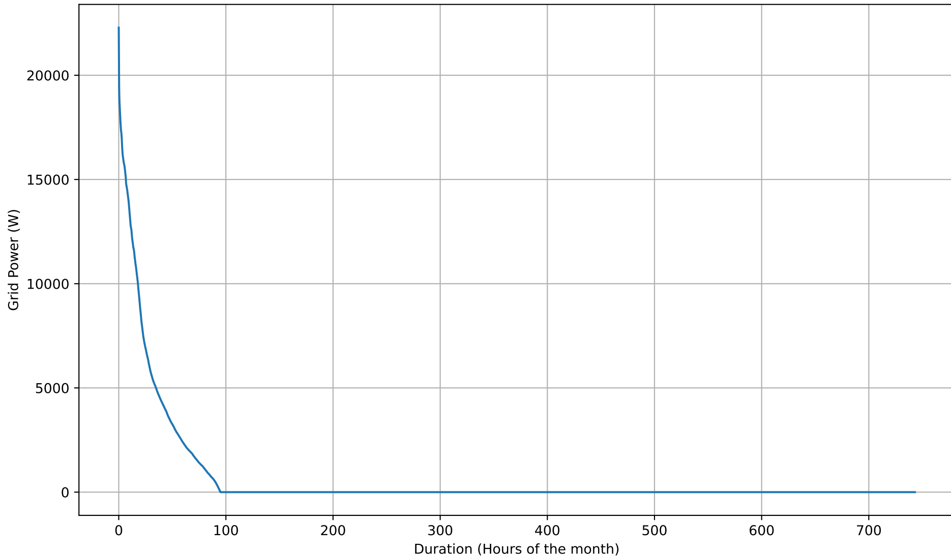
Grid Export Duration Curve - 20kWh - Mar
