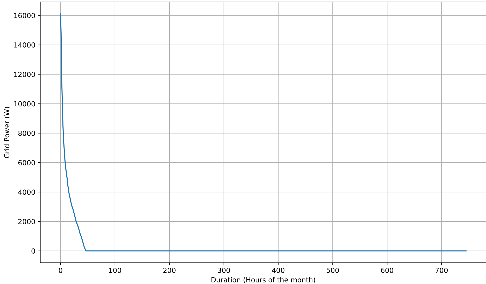
Grid Export Duration Curve - 20kWh - Oct
