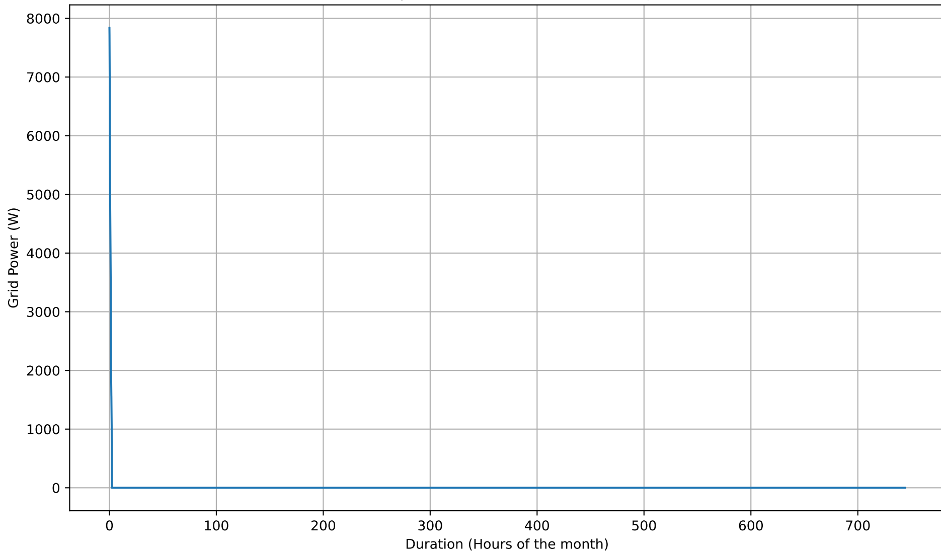
Grid Export Duration Curve - 20kWh - Jan
