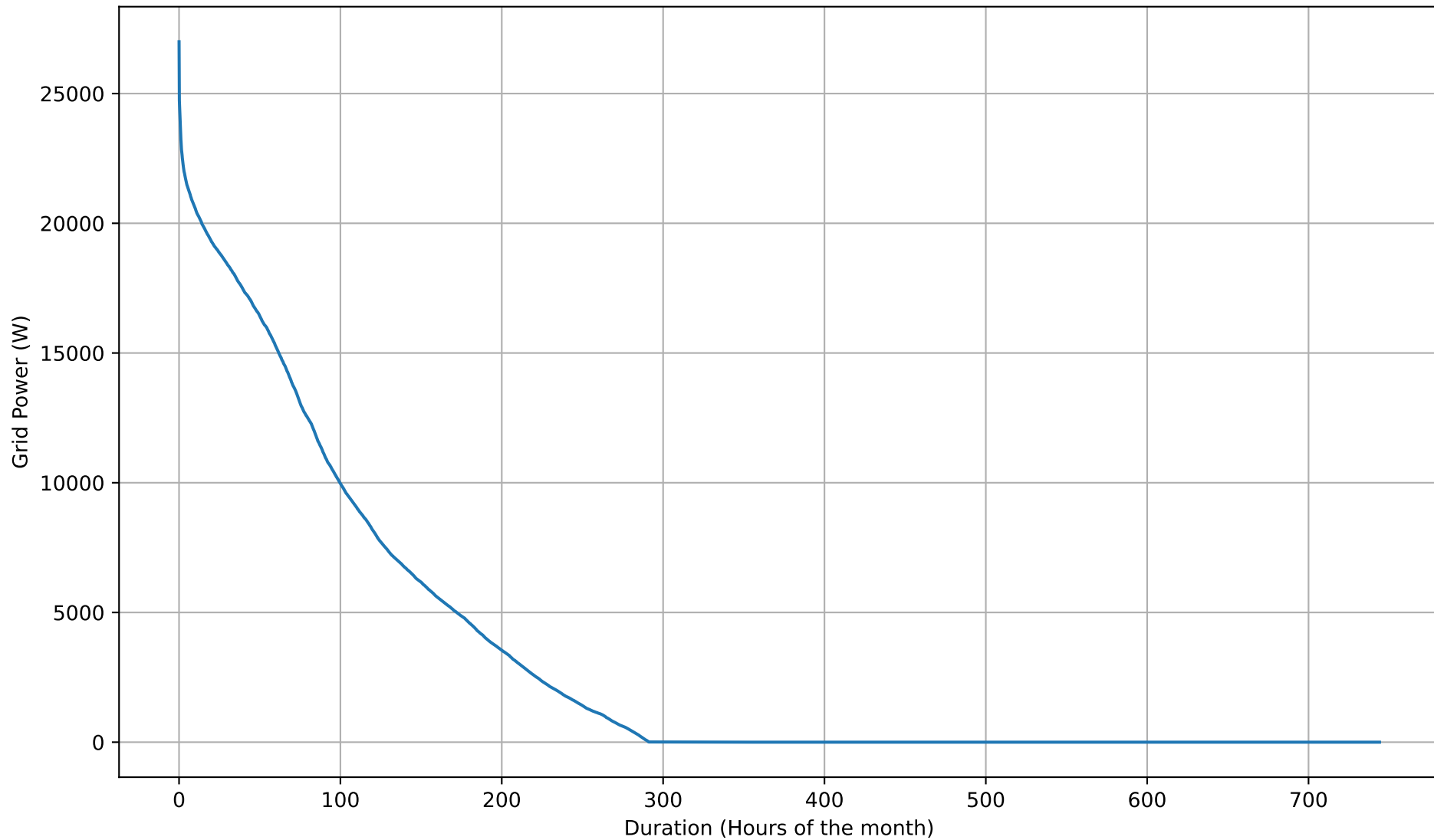
Grid Export Duration Curve - 20kWh - May
