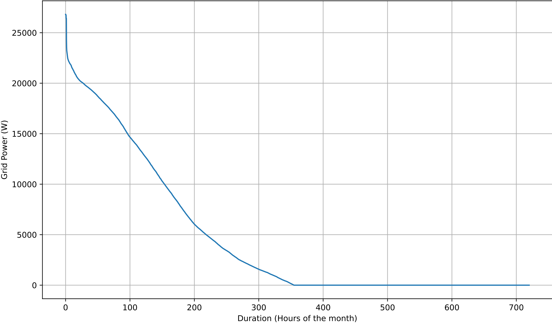
Grid Export Duration Curve - 20kWh - Jun
