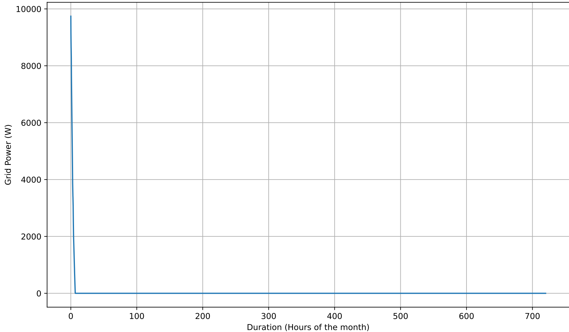
Grid Export Duration Curve - 20kWh - Nov
