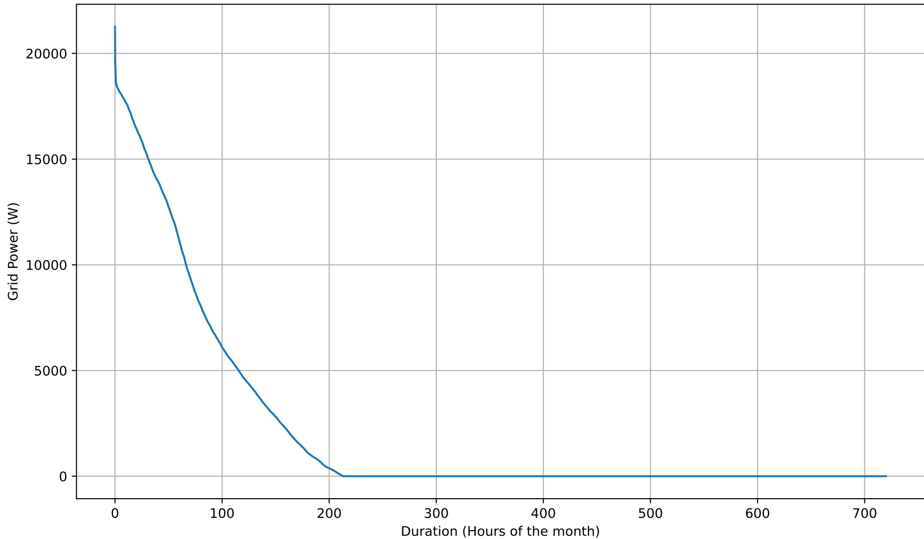
Grid Export Duration Curve - 20kWh - Sep
