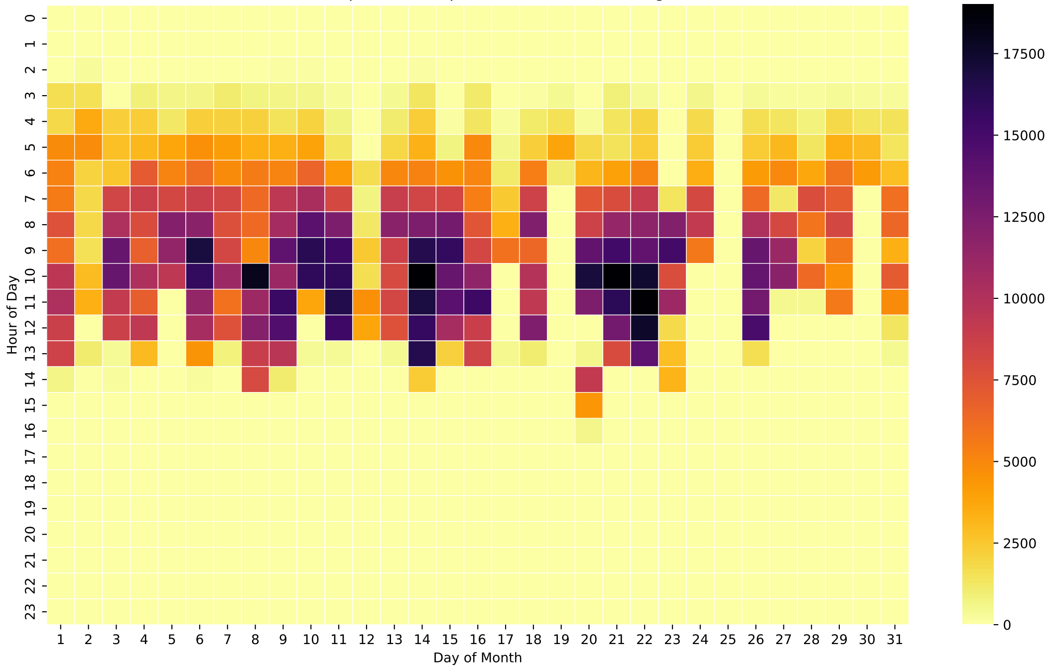
Grid Export Heatmap (Wh/Hour) - 20kWh - Aug
