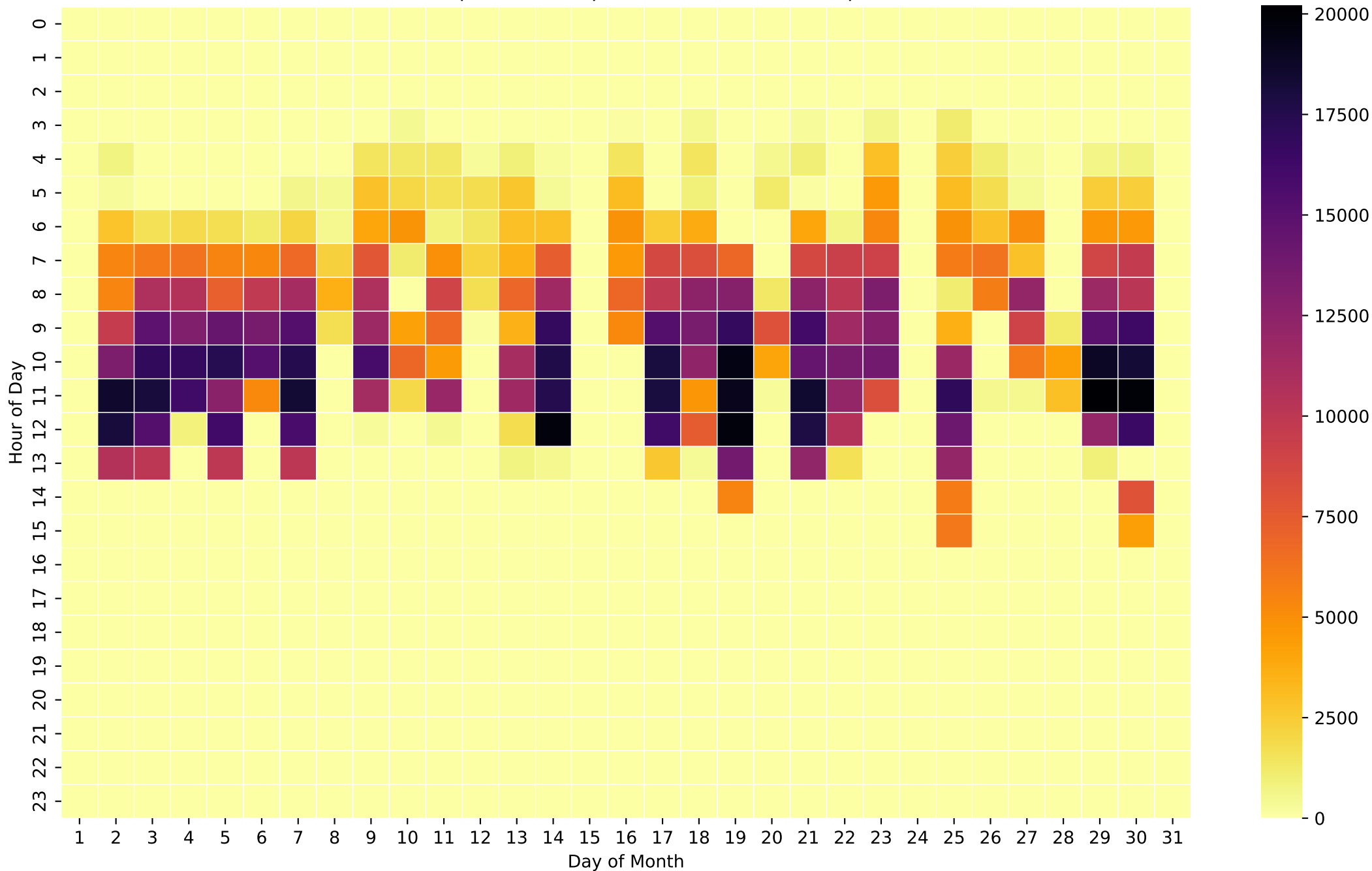
Grid Export Heatmap (Wh/Hour) - 20kWh - Apr
