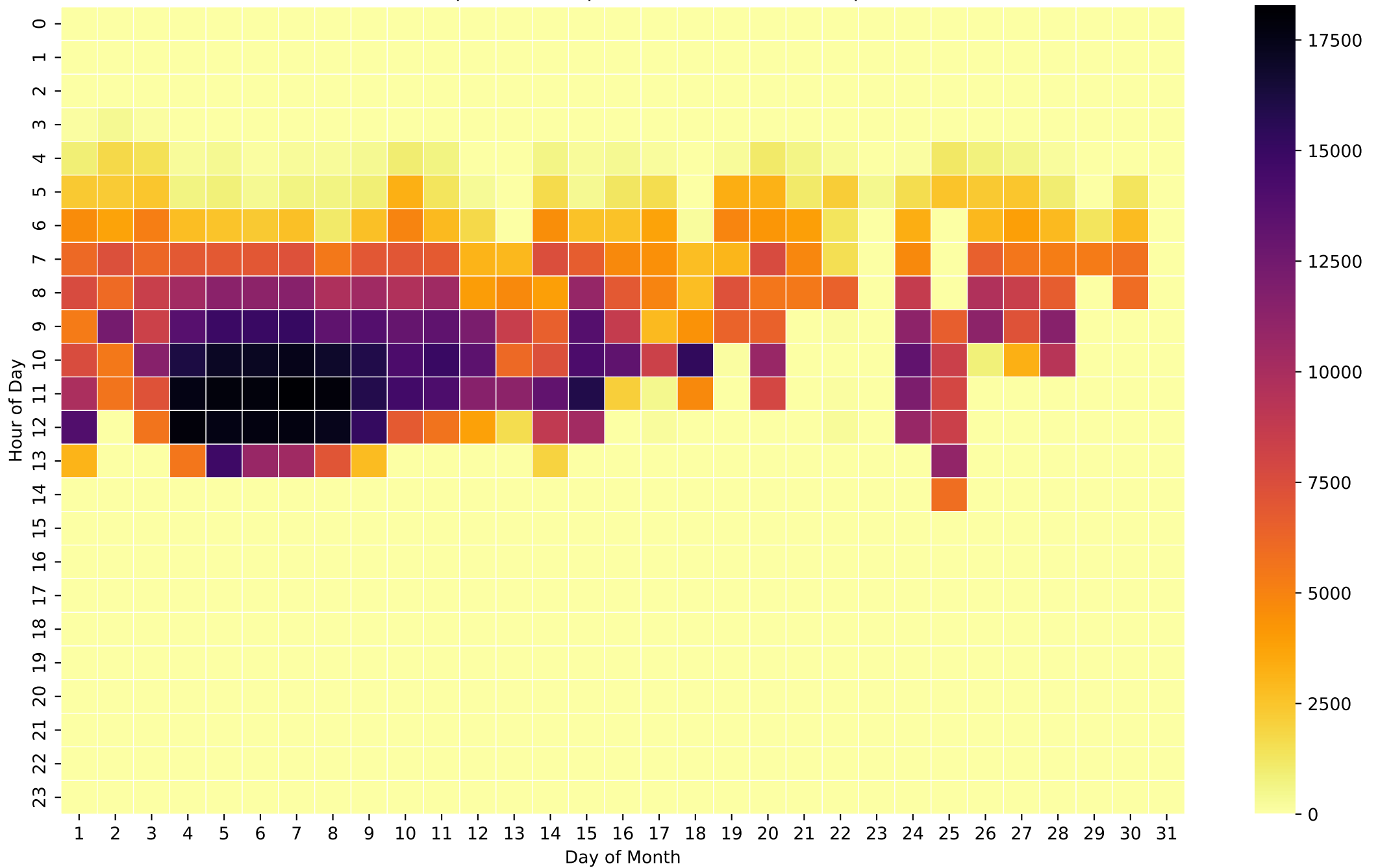
Grid Export Heatmap (Wh/Hour) - 20kWh - Sep
