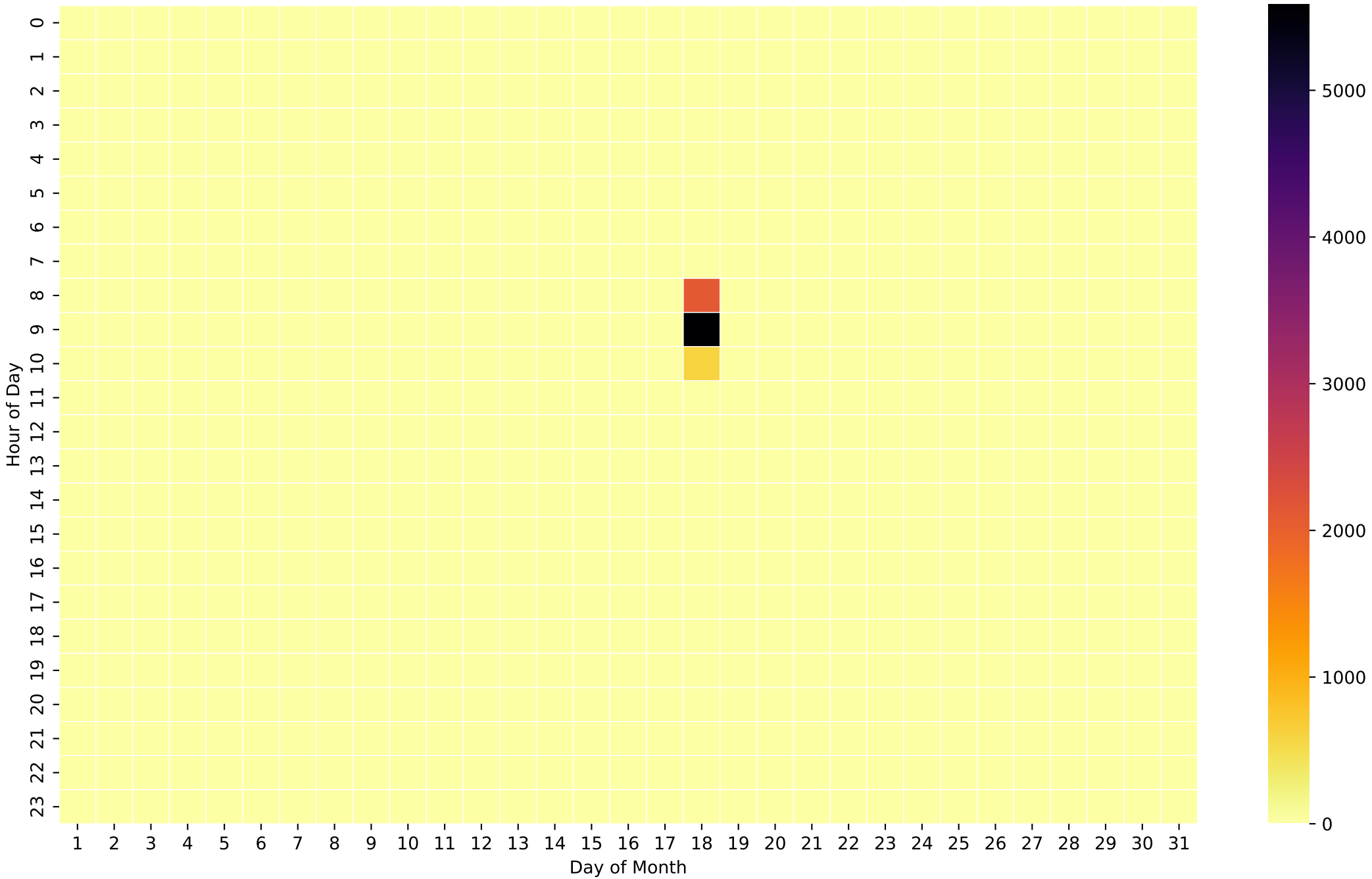
Grid Export Heatmap (Wh/Hour) - 20kWh - Jan
