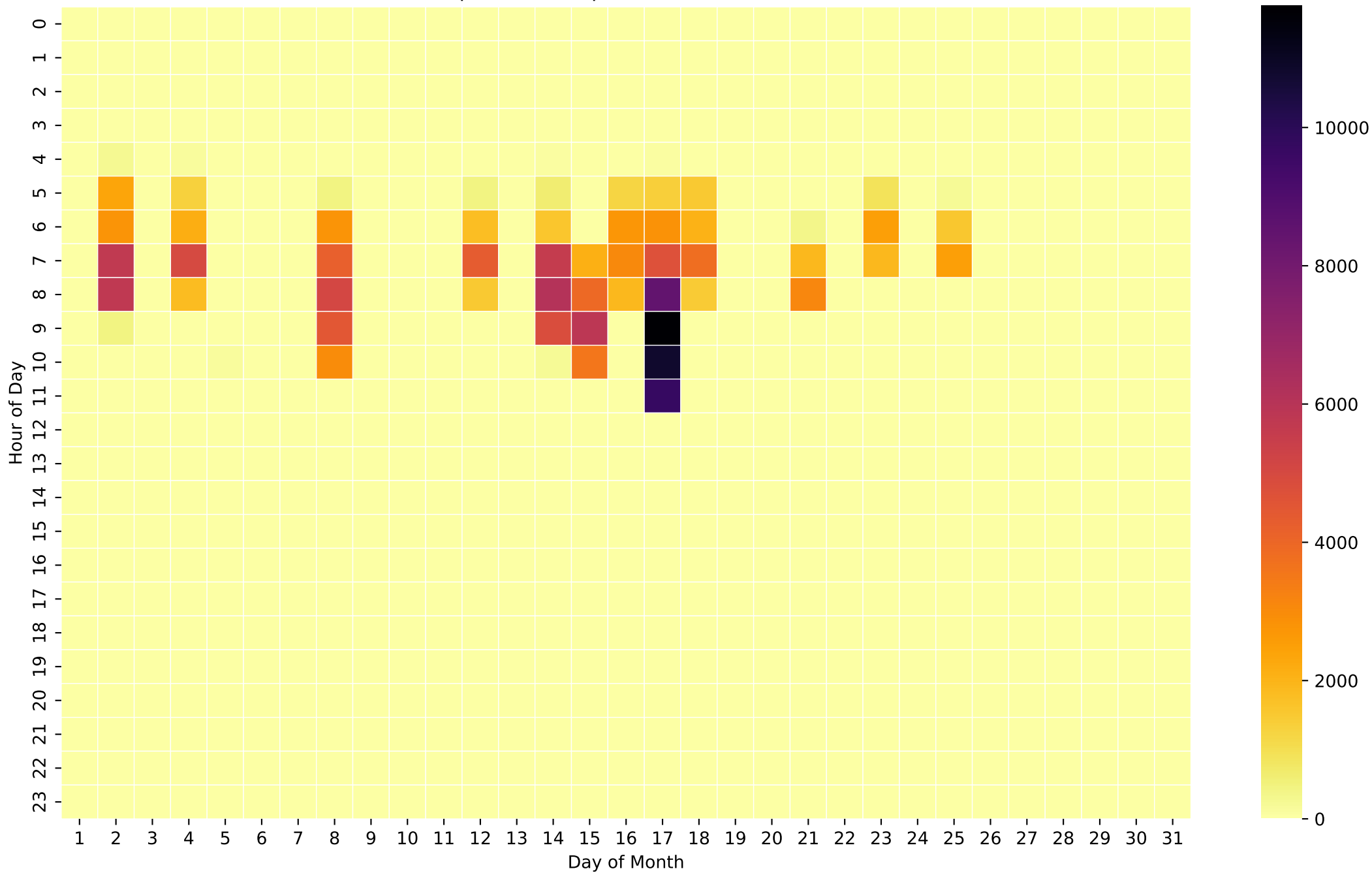
Grid Export Heatmap (Wh/Hour) - 20kWh - Oct
