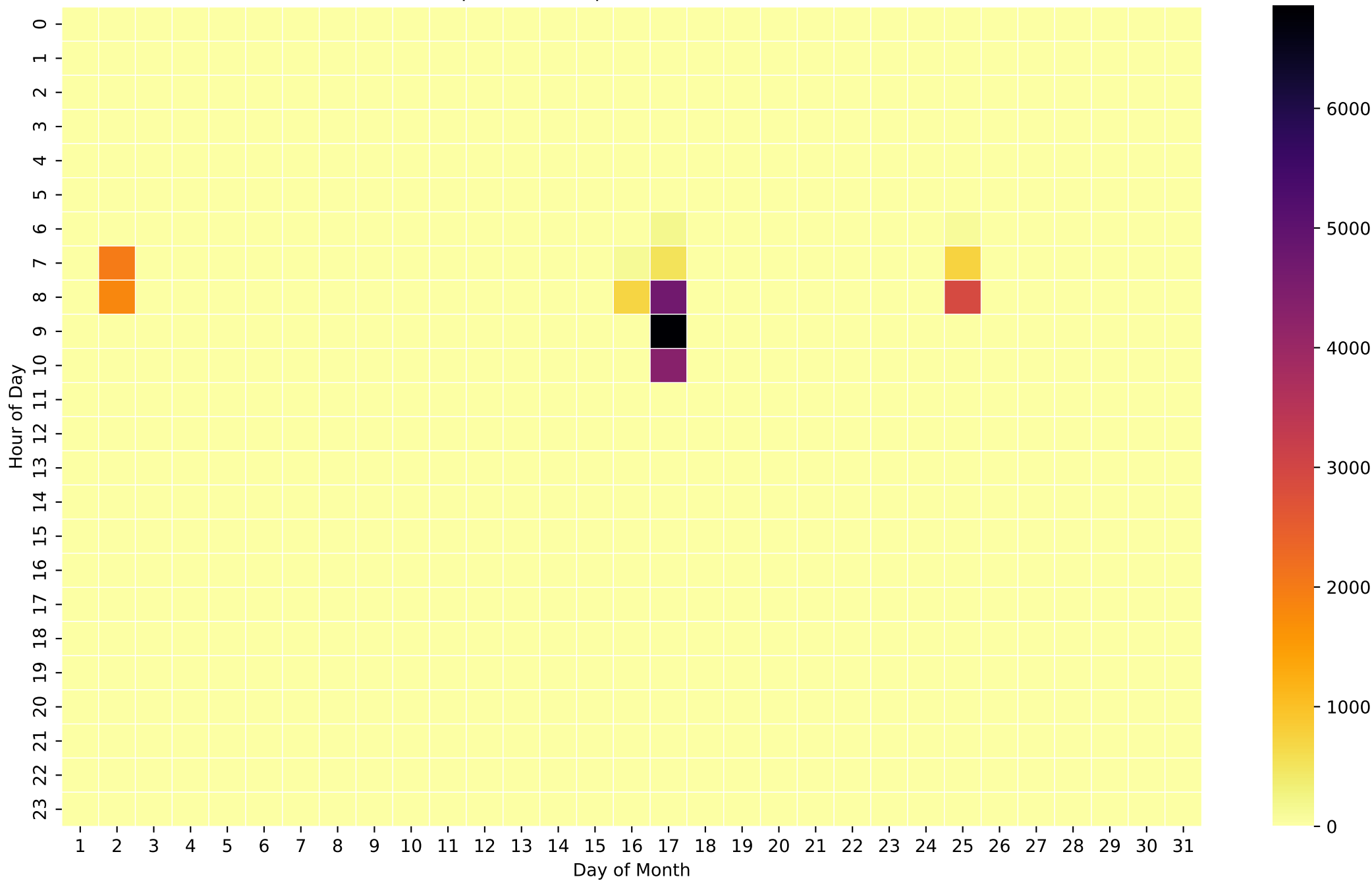
Grid Export Heatmap (Wh/Hour) - 20kWh - Nov
