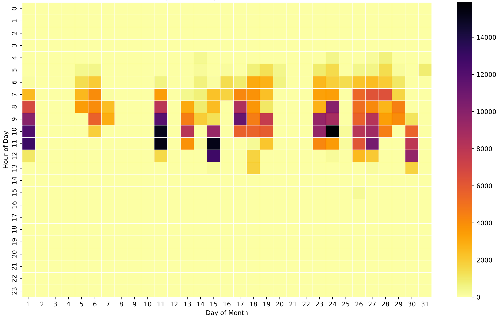
Grid Export Heatmap (Wh/Hour) - 20kWh - Mar
