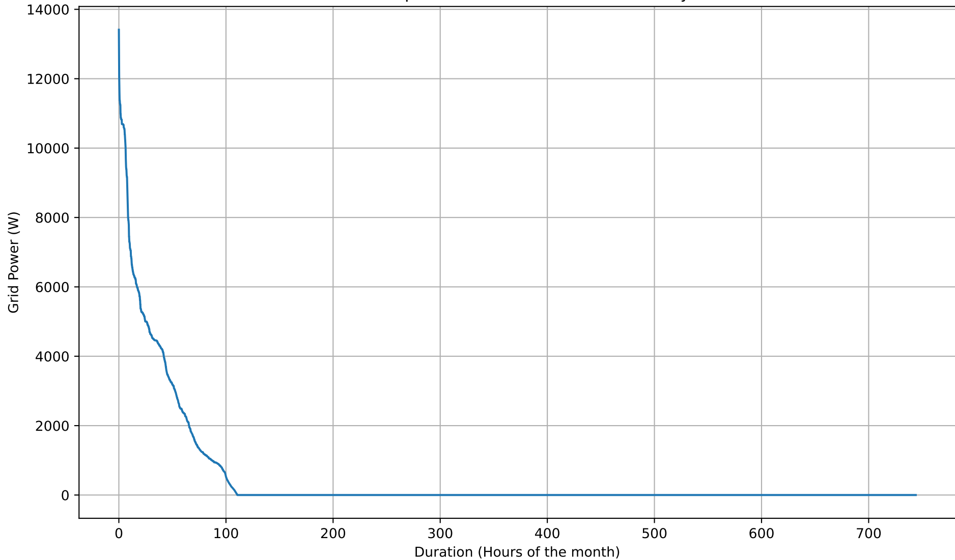
Grid Import Duration Curve - 20kWh - May
