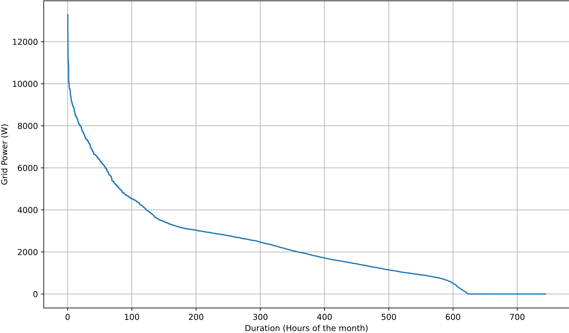
Grid Import Duration Curve - 20kWh - Jan
