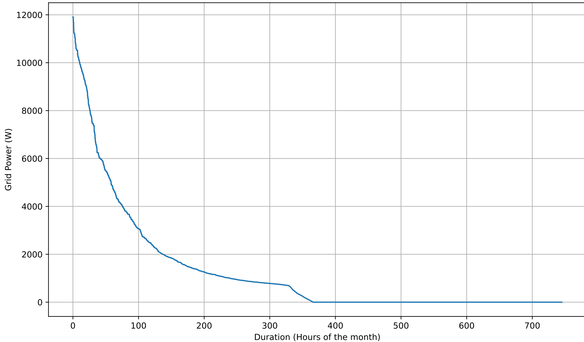
Grid Import Duration Curve - 20kWh - Oct
