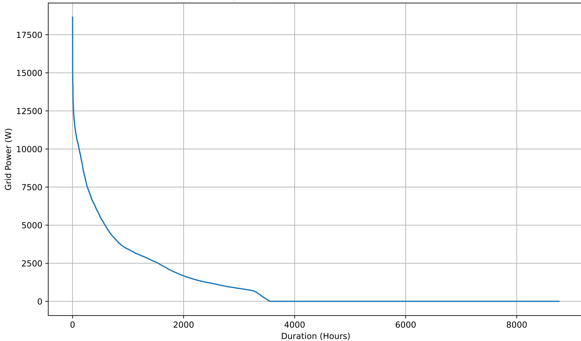
Yearly Grid Import Duration Curve - 20kWh
