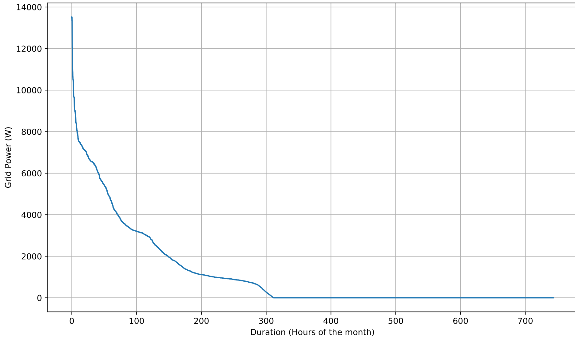
Grid Import Duration Curve - 20kWh - Mar
