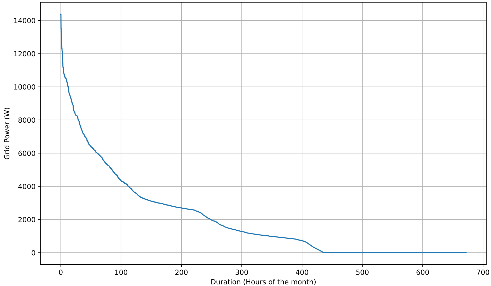
Grid Import Duration Curve - 20kWh - Feb
