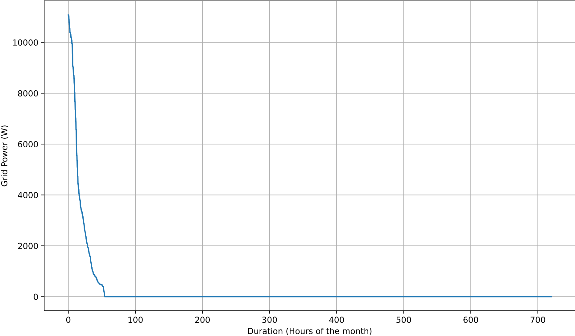
Grid Import Duration Curve - 20kWh - Jun
