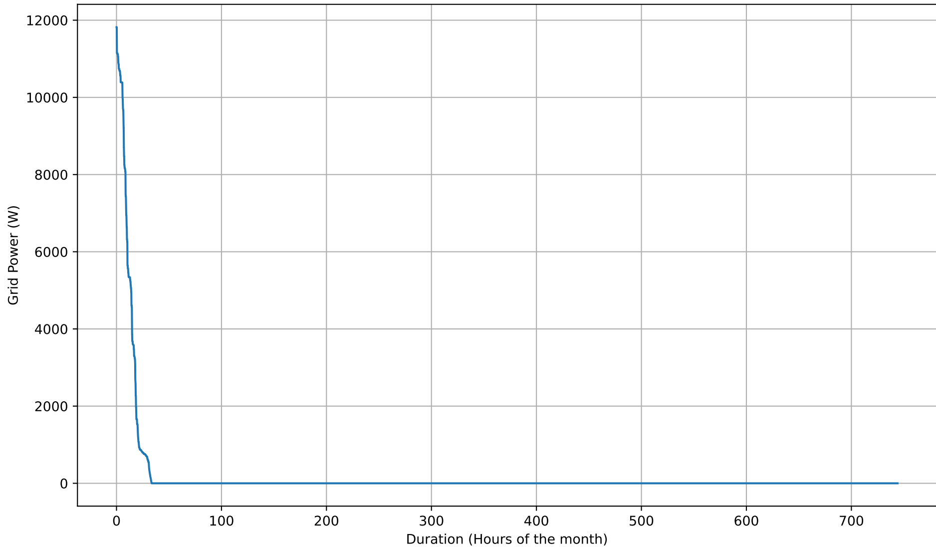
Grid Import Duration Curve - 20kWh - Jul
