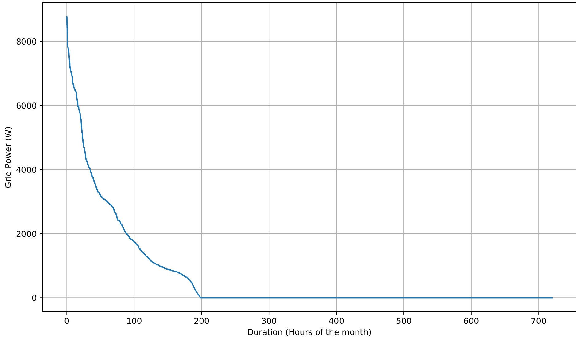
Grid Import Duration Curve - 20kWh - Apr
