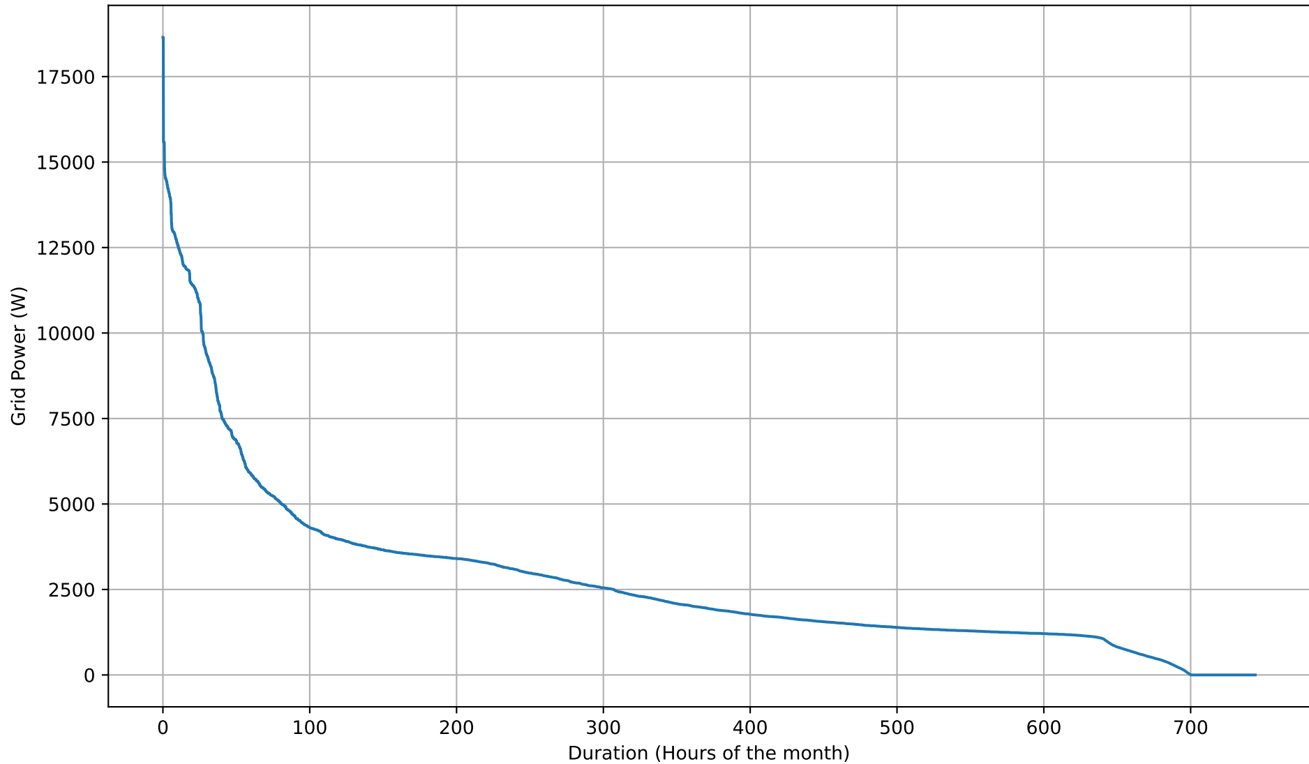
Grid Import Duration Curve - 20kWh - Dec
