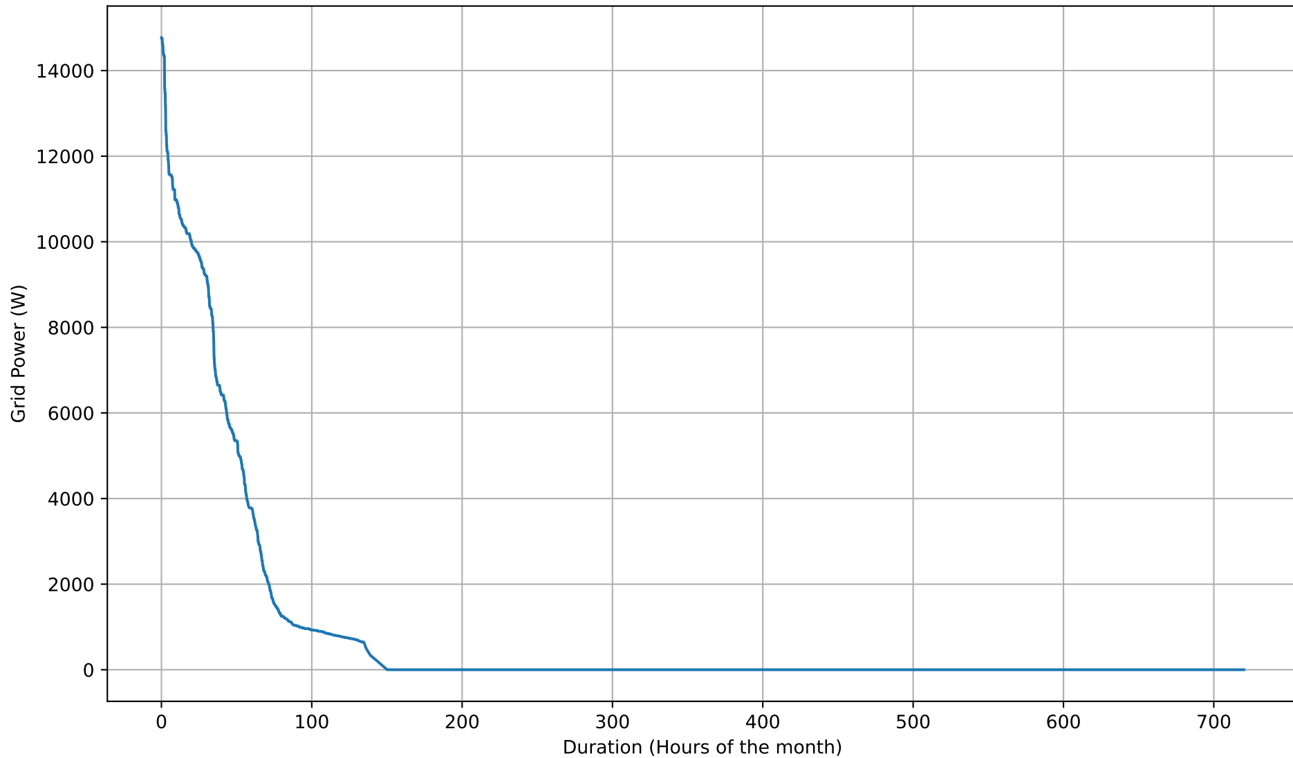
Grid Import Duration Curve - 20kWh - Sep
