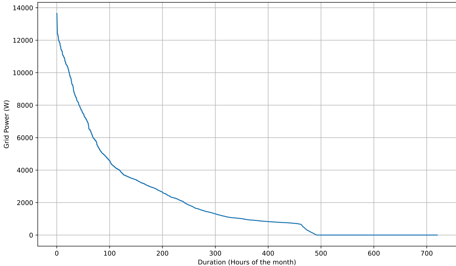
Grid Import Duration Curve - 20kWh - Nov
