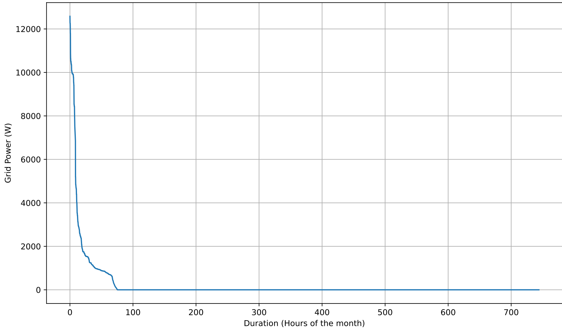
Grid Import Duration Curve - 20kWh - Aug
