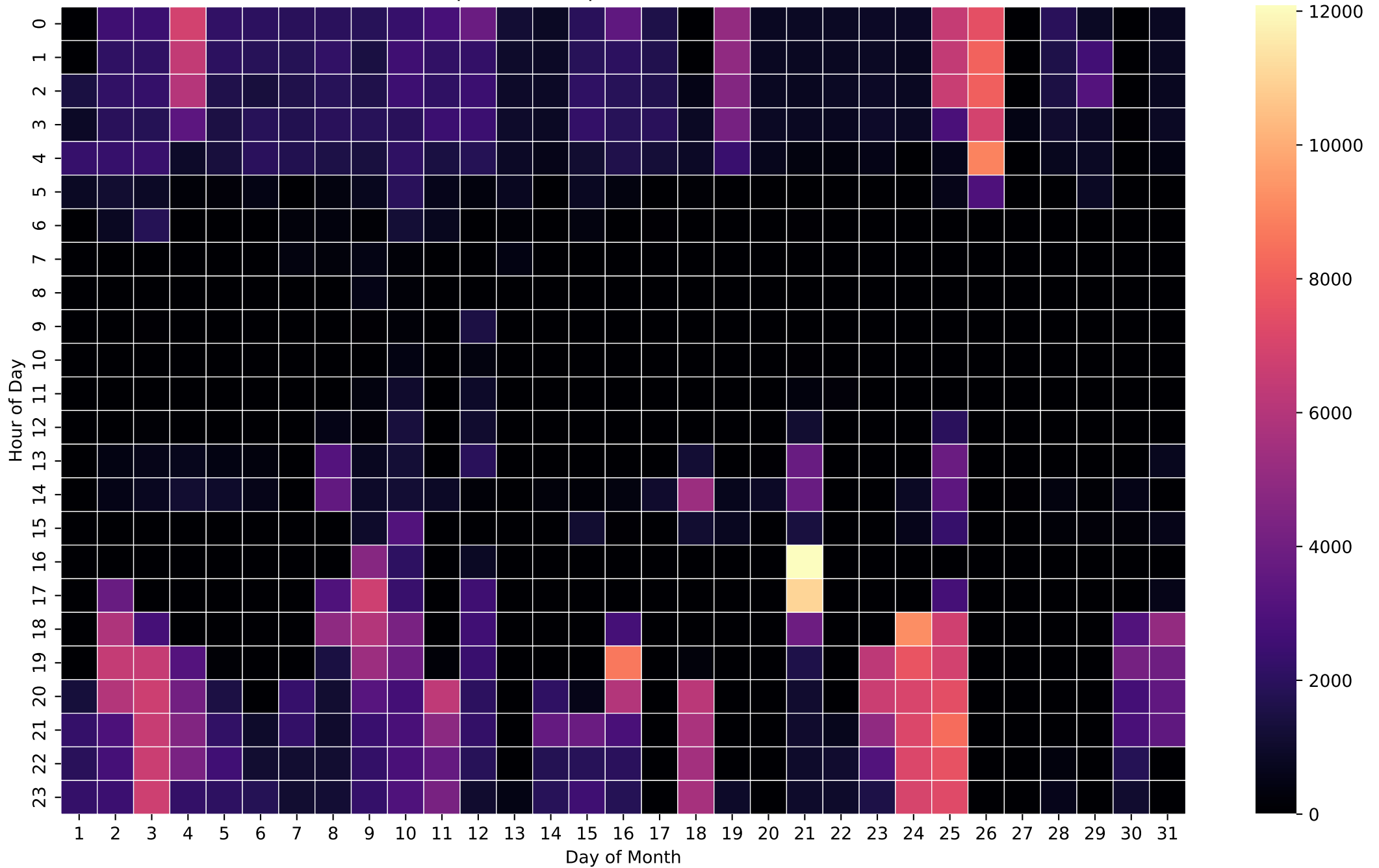
Grid Import Heatmap (Wh/Hour) - 20kWh - Mar
