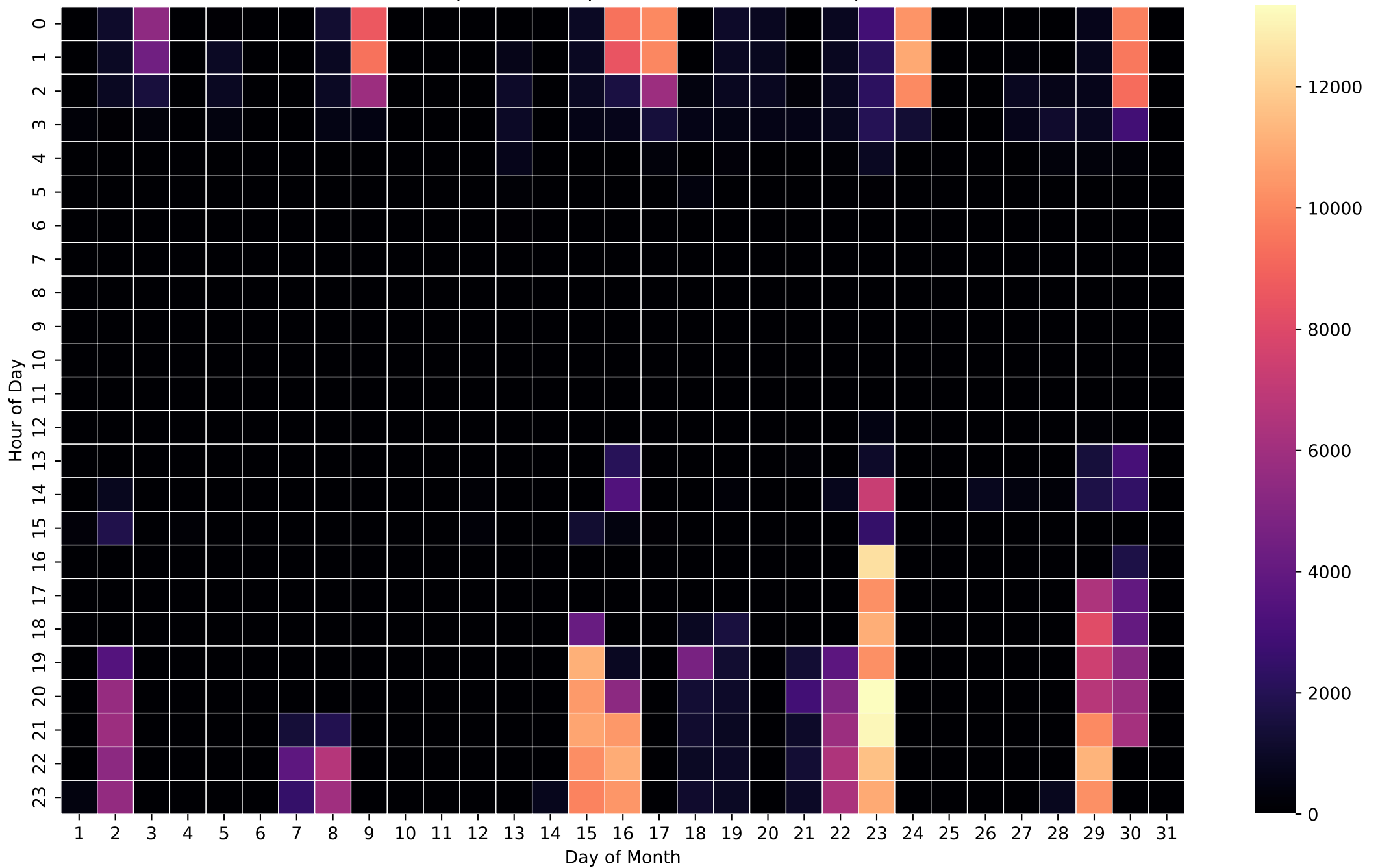
Grid Import Heatmap (Wh/Hour) - 20kWh - Sep
