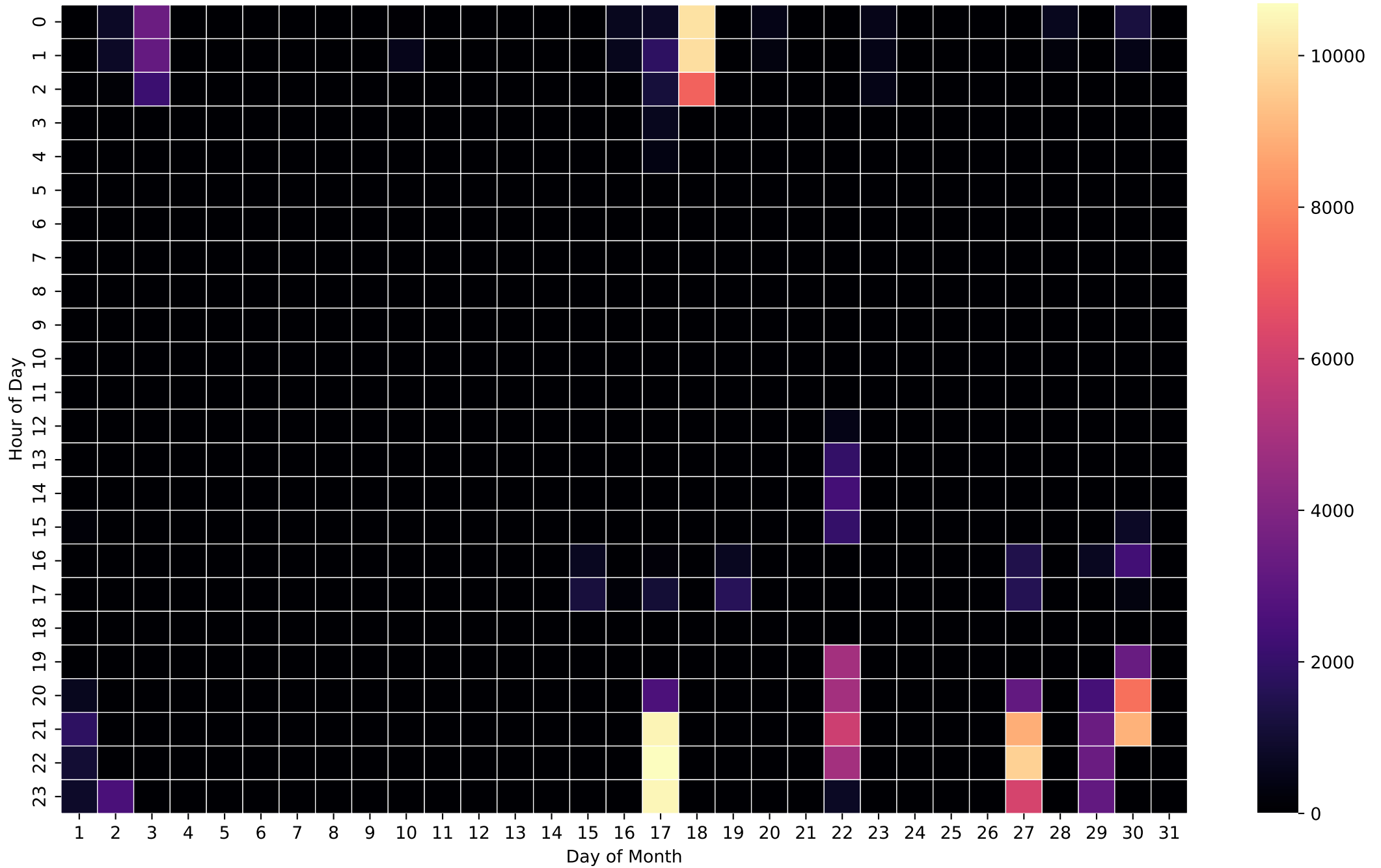
Grid Import Heatmap (Wh/Hour) - 20kWh - Jun
