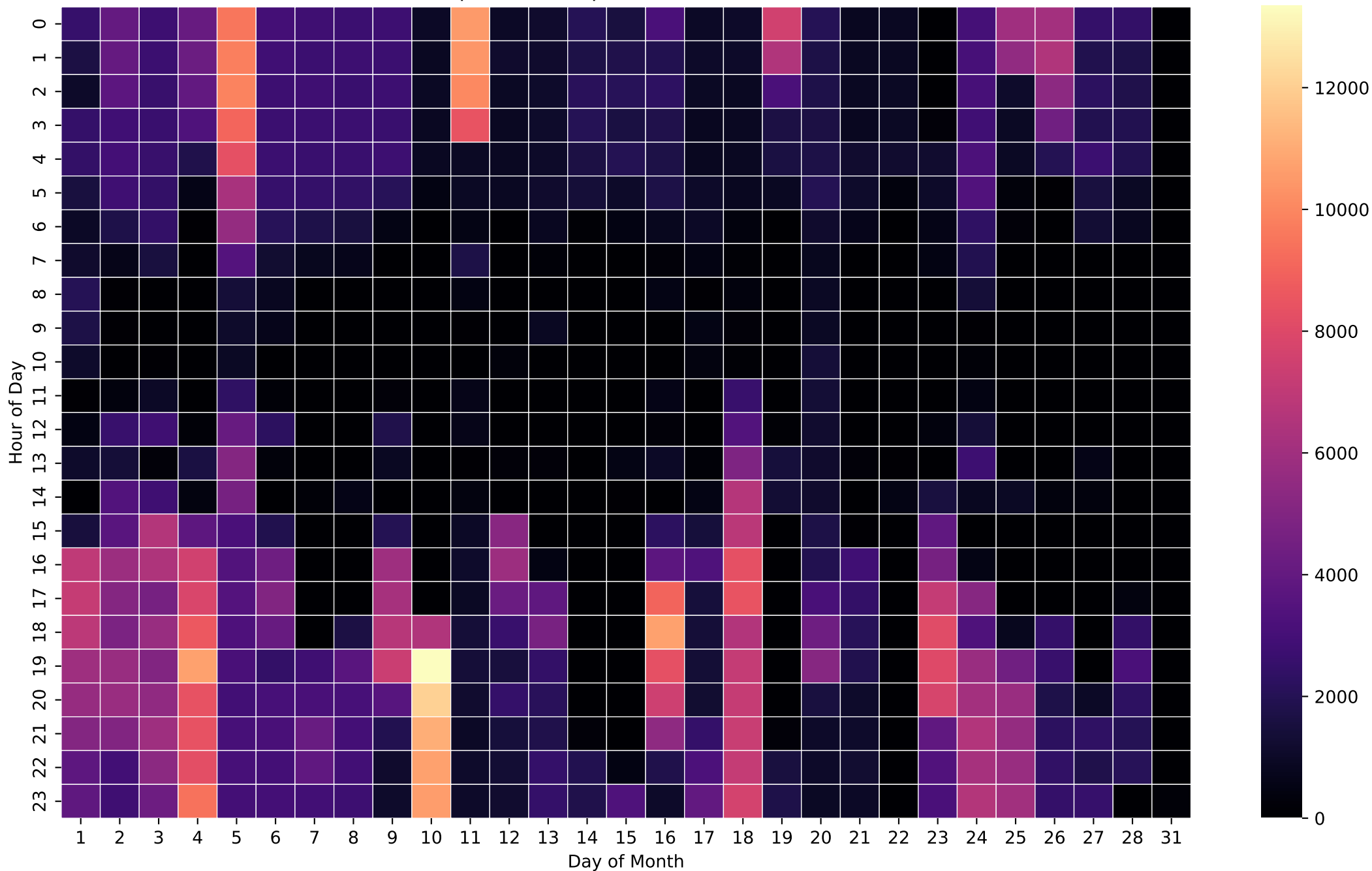
Grid Import Heatmap (Wh/Hour) - 20kWh - Feb
