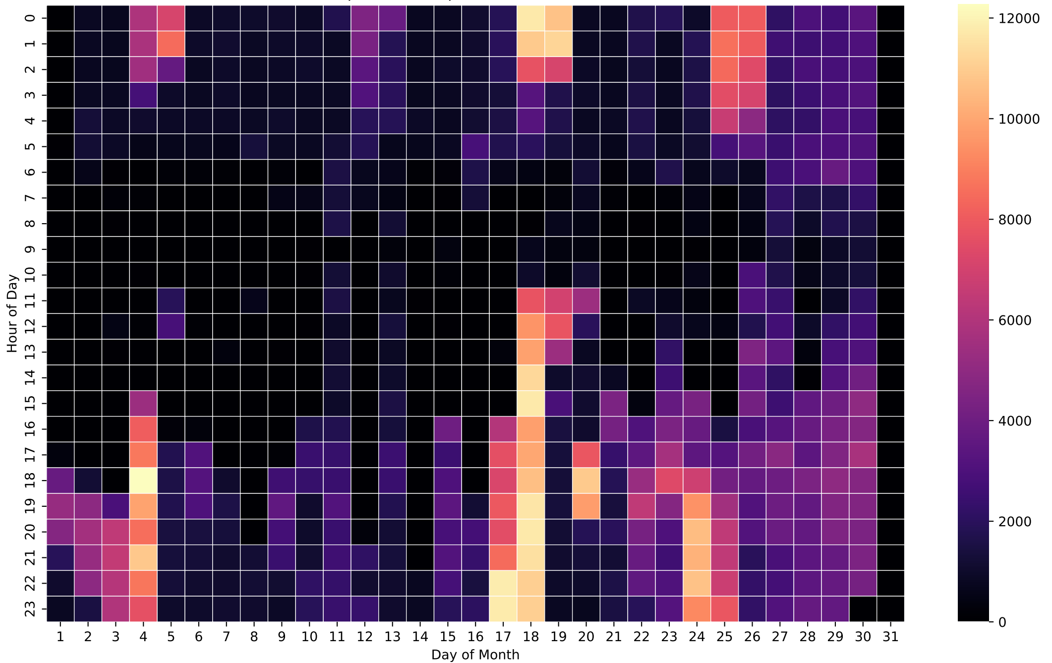
Grid Import Heatmap (Wh/Hour) - 20kWh - Nov
