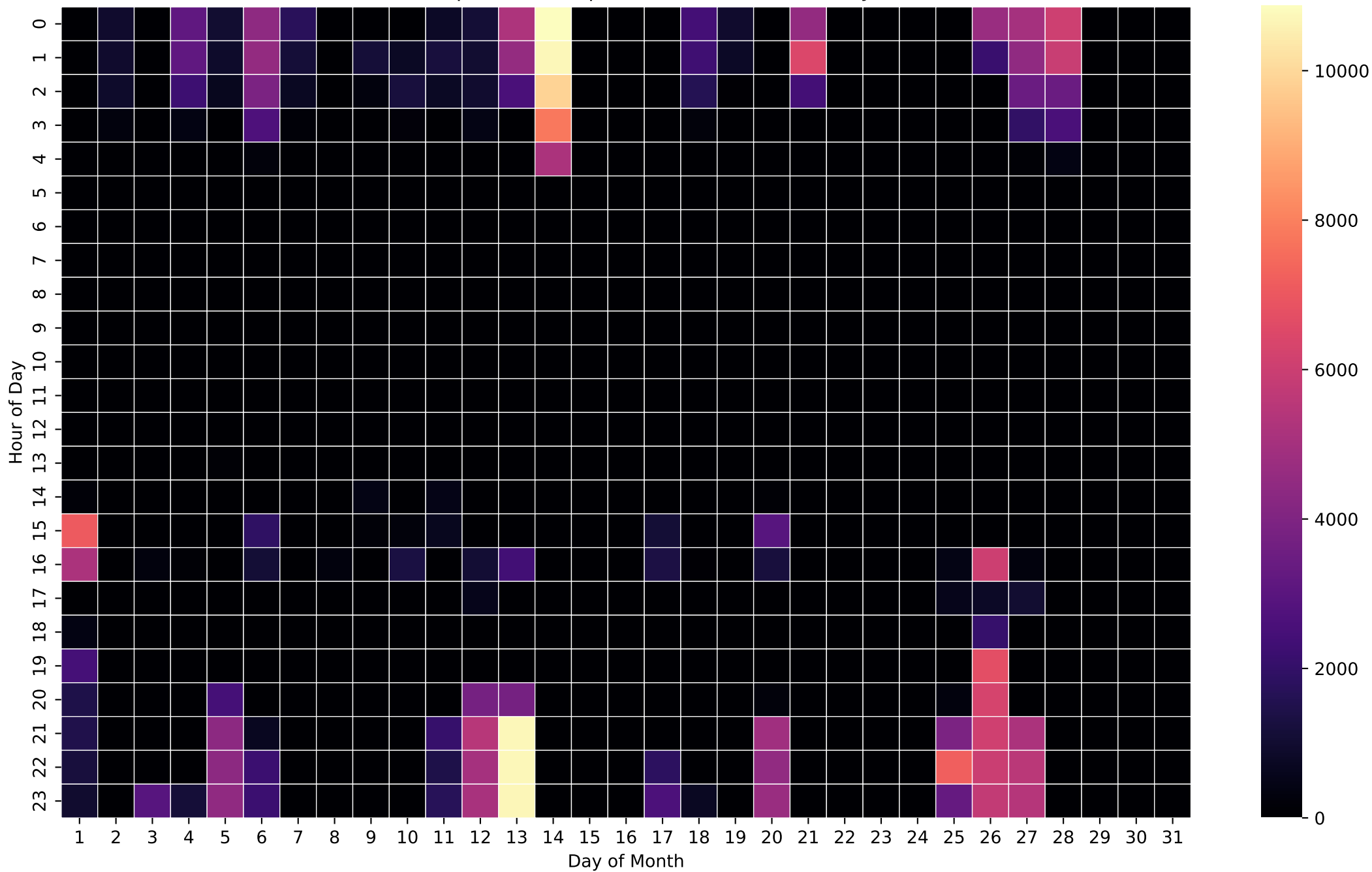
Grid Import Heatmap (Wh/Hour) - 20kWh - May
