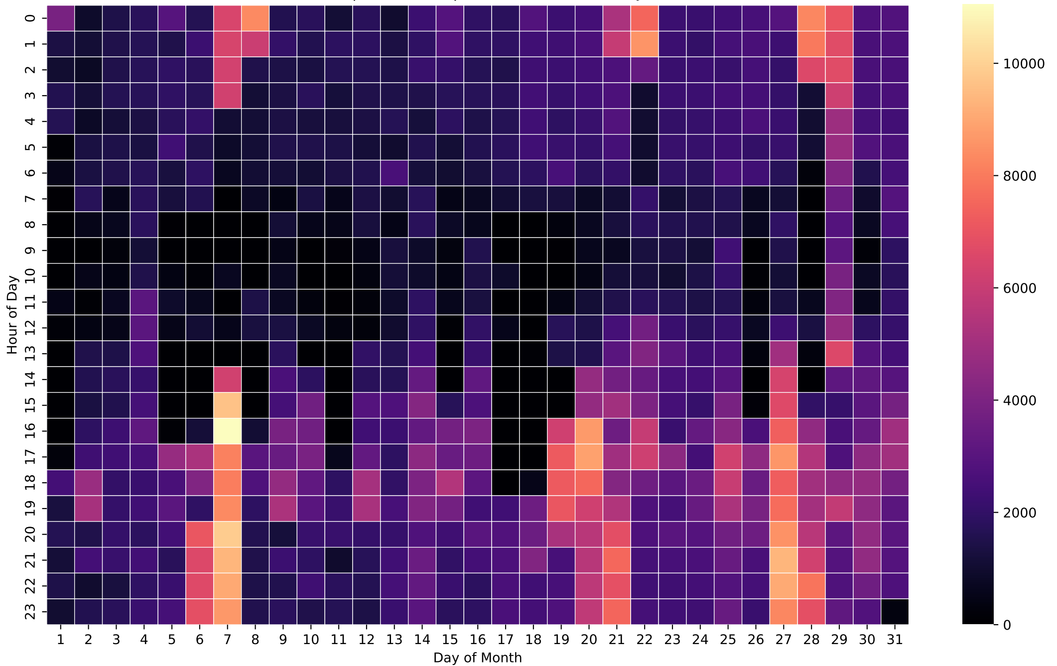
Grid Import Heatmap (Wh/Hour) - 20kWh - Jan
