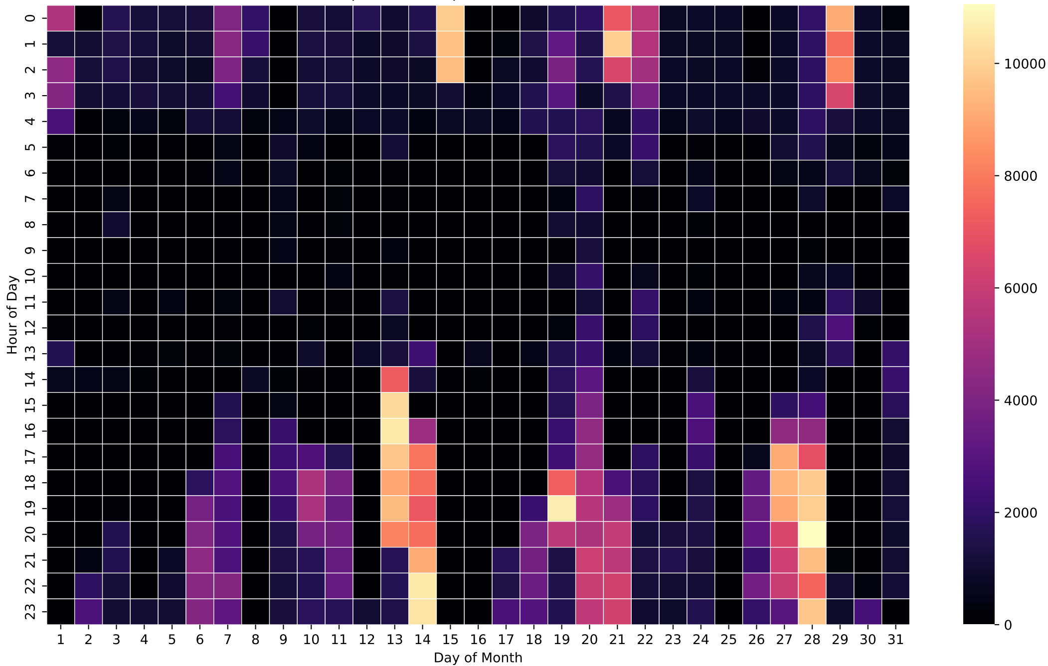
Grid Import Heatmap (Wh/Hour) - 20kWh - Oct
