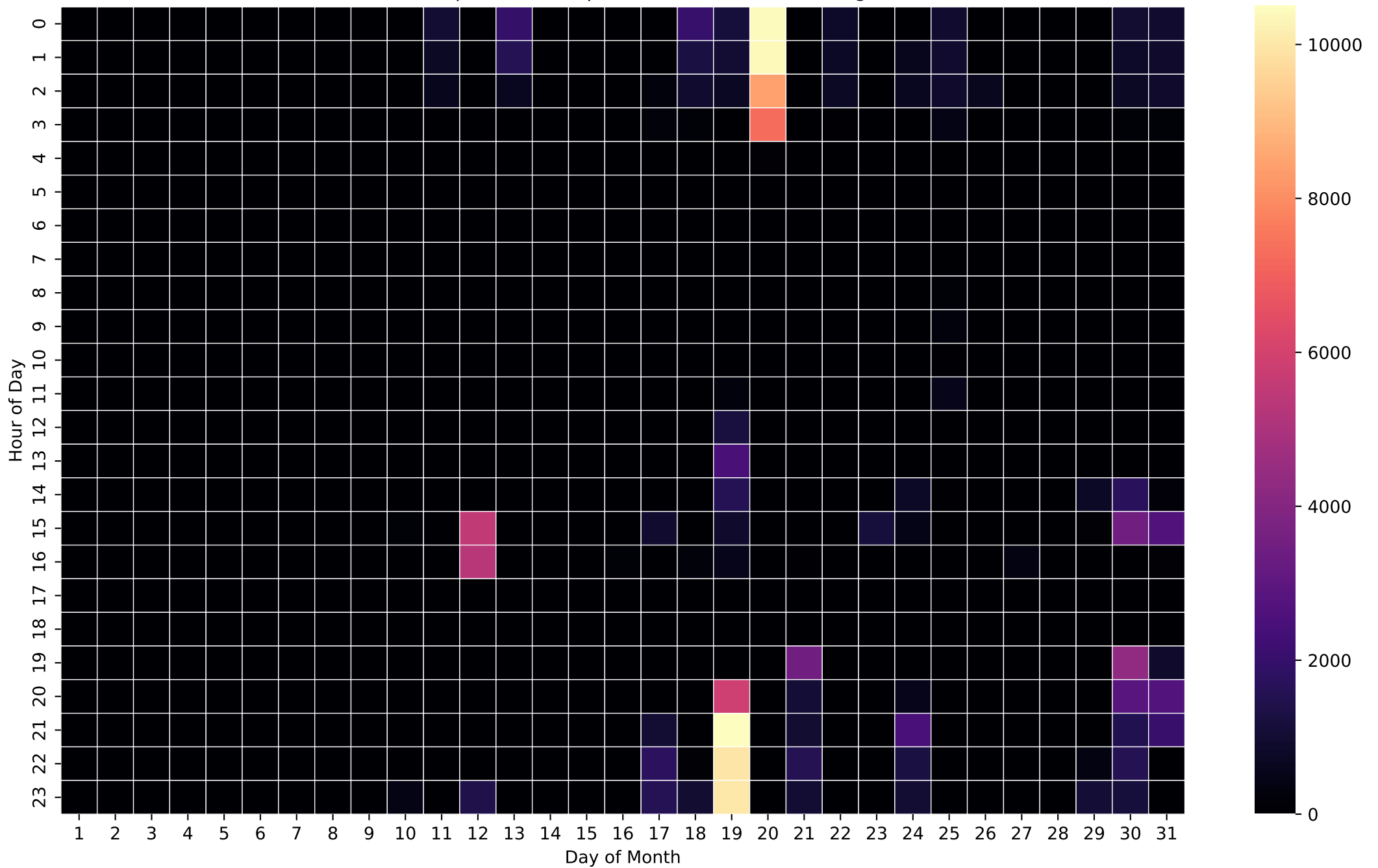
Grid Import Heatmap (Wh/Hour) - 20kWh - Aug
