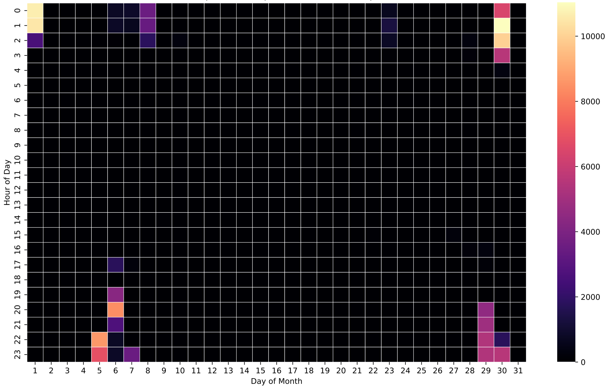
Grid Import Heatmap (Wh/Hour) - 20kWh - Jul
