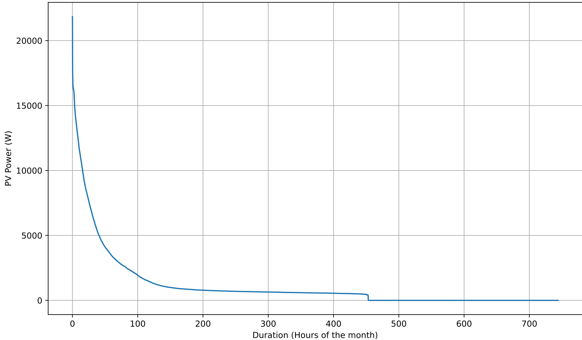
PV Self-Consumption Duration Curve - 20kWh - Jul
