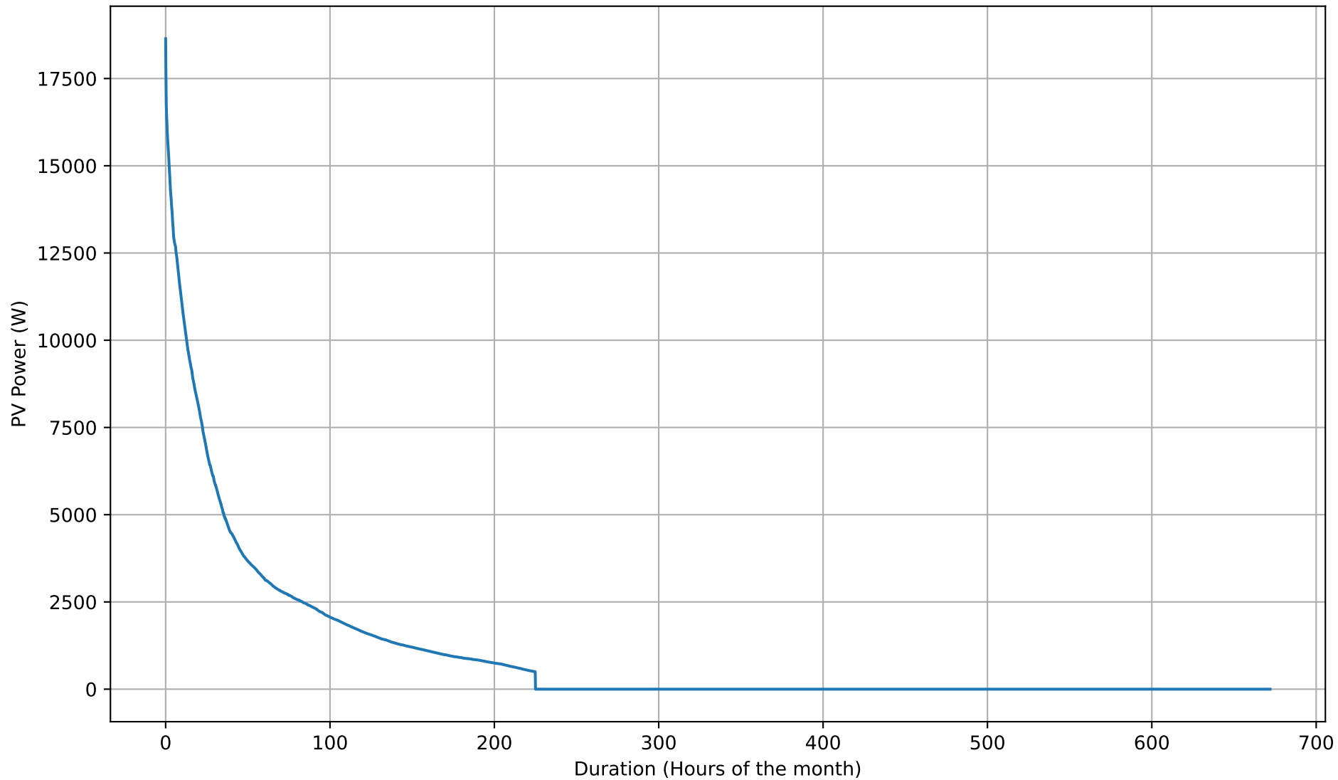
PV Self-Consumption Duration Curve - 20kWh - Feb
