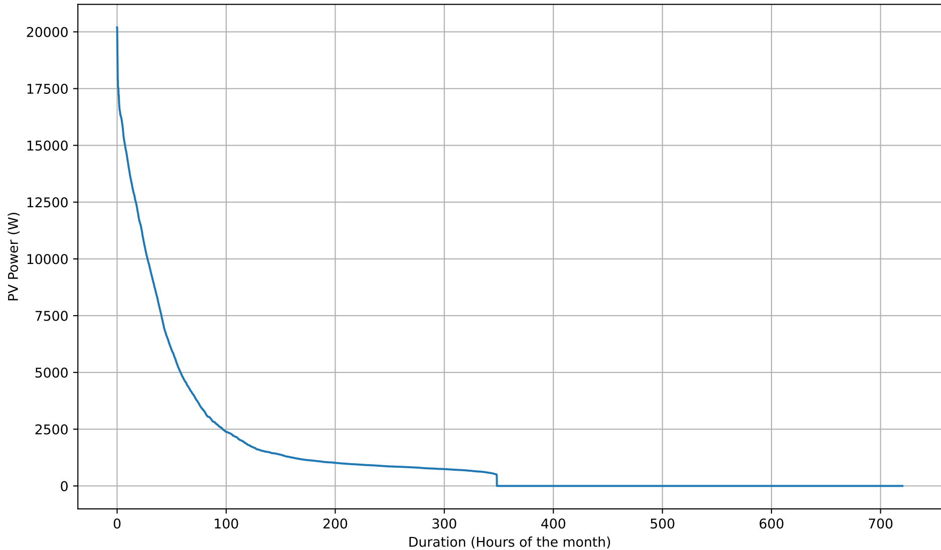
PV Self-Consumption Duration Curve - 20kWh - Sep
