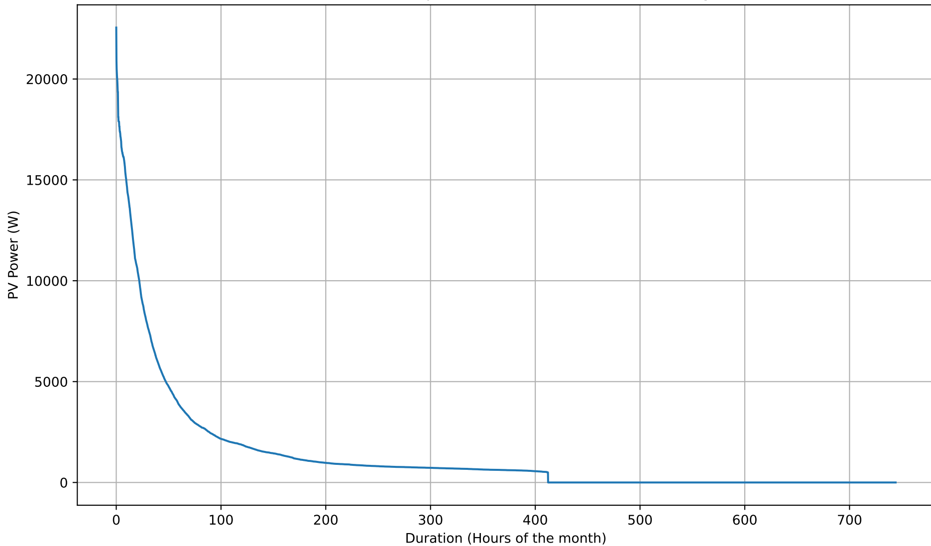
PV Self-Consumption Duration Curve - 20kWh - Aug
