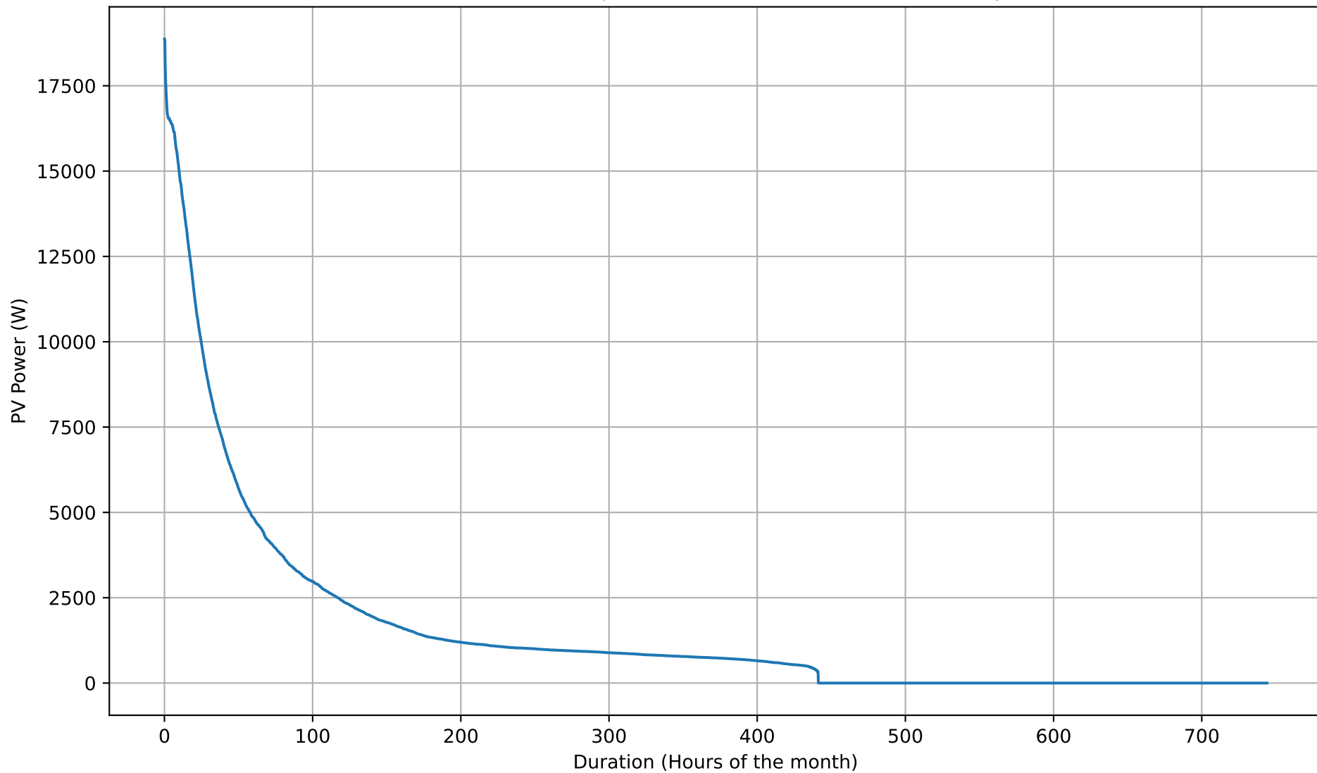
PV Self-Consumption Duration Curve - 20kWh - May
