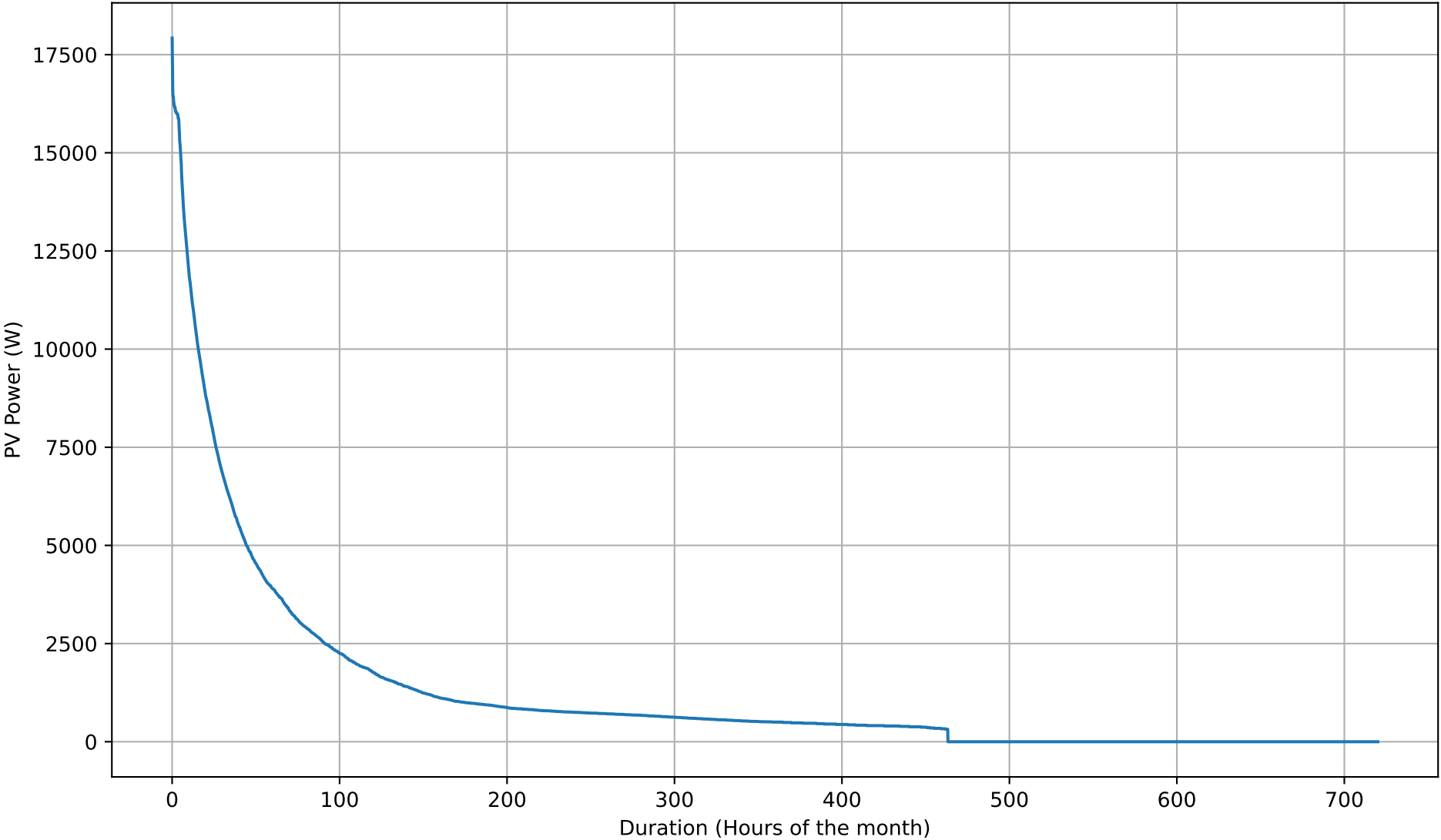
PV Self-Consumption Duration Curve - 20kWh - Jun
