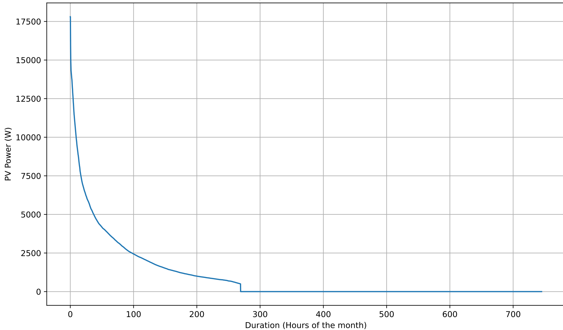
PV Self-Consumption Duration Curve - 20kWh - Oct
