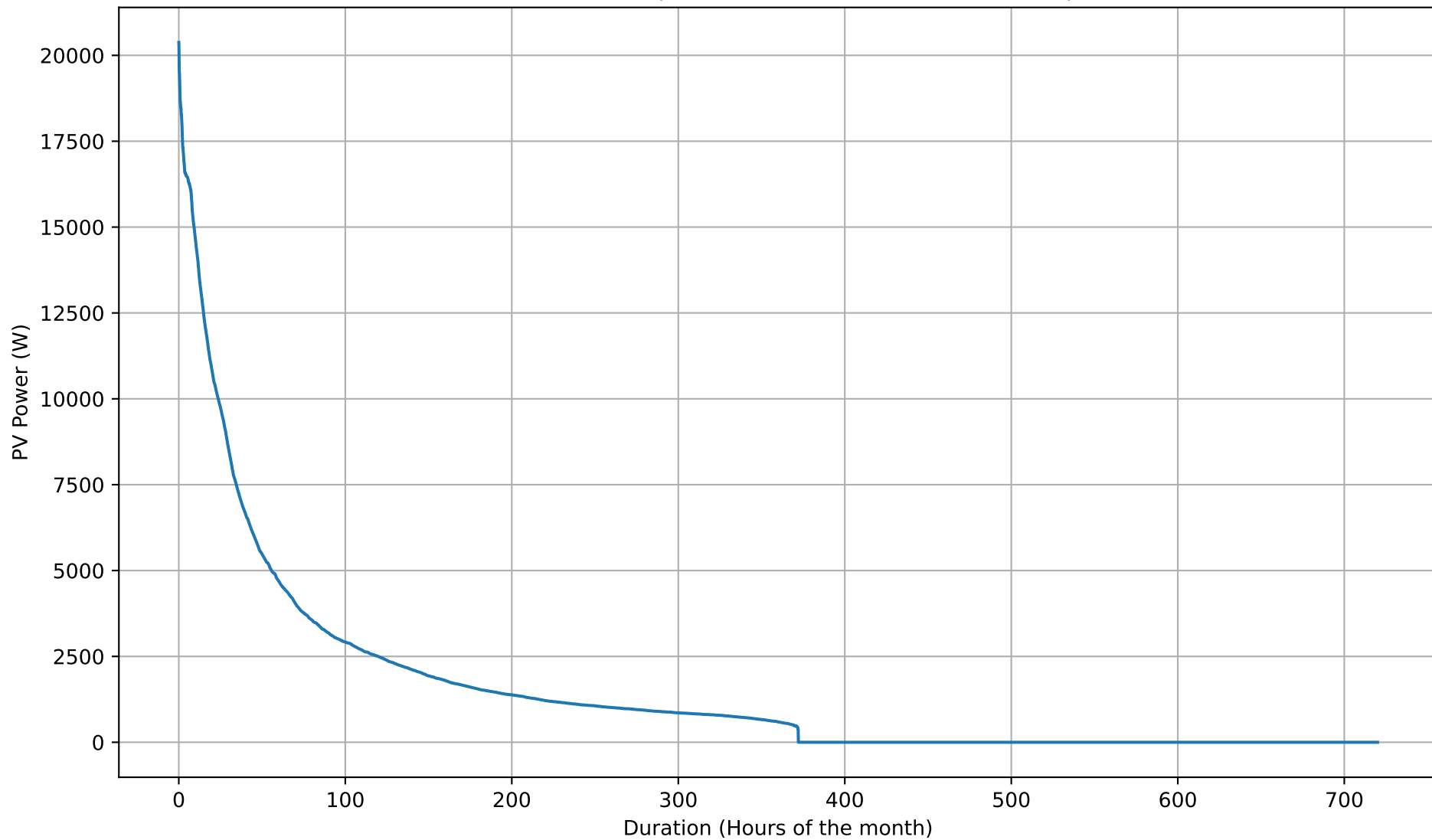
PV Self-Consumption Duration Curve - 20kWh - Apr
