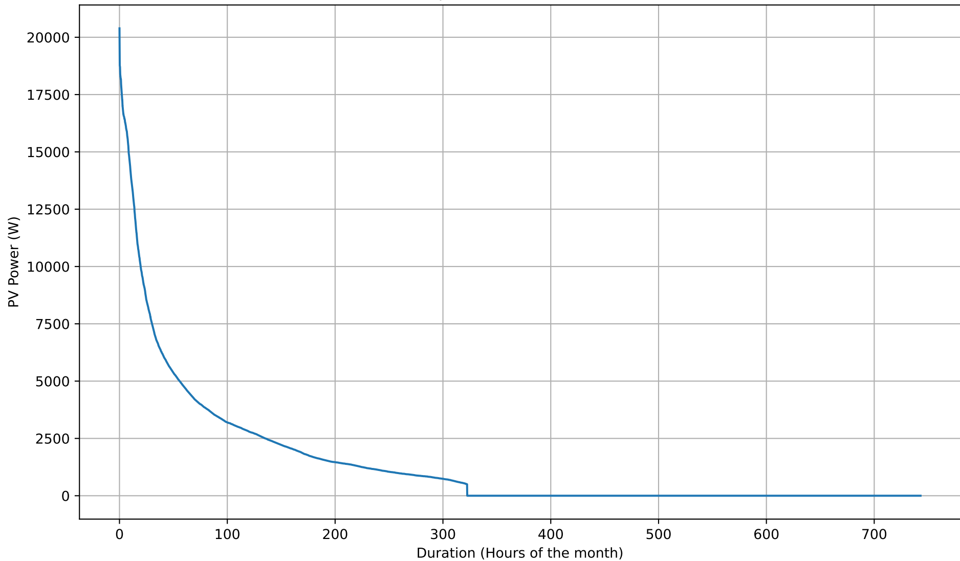
PV Self-Consumption Duration Curve - 20kWh - Mar
