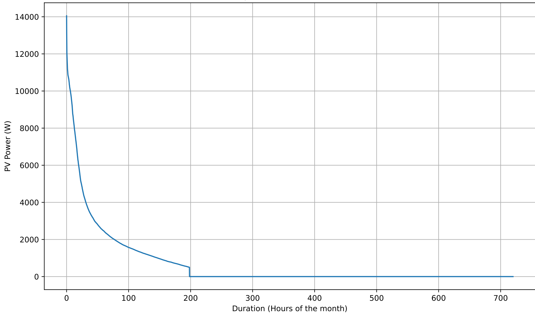
PV Self-Consumption Duration Curve - 20kWh - Nov
