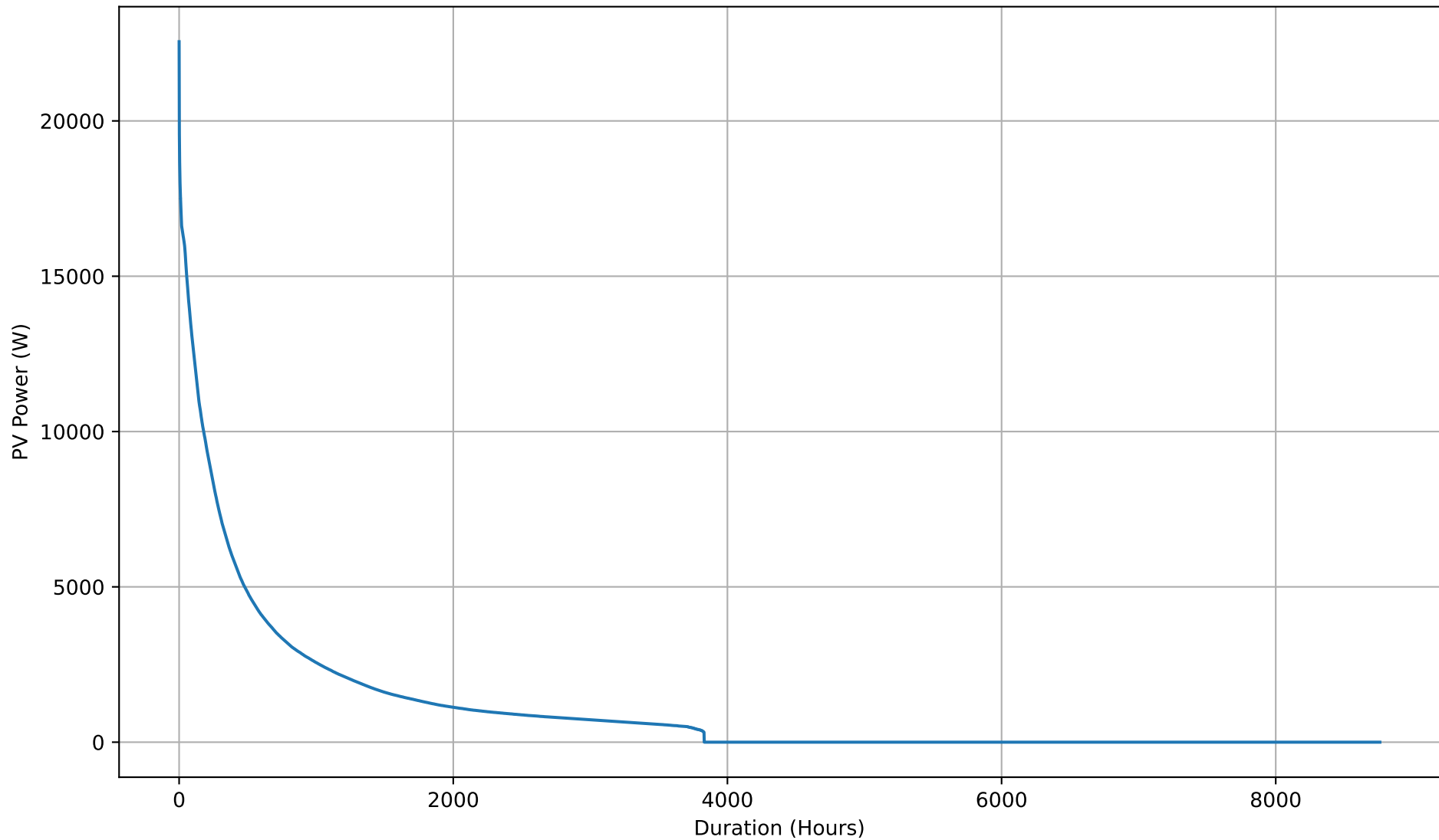
Yearly PV Self-Consumption Duration Curve - 20kWh
