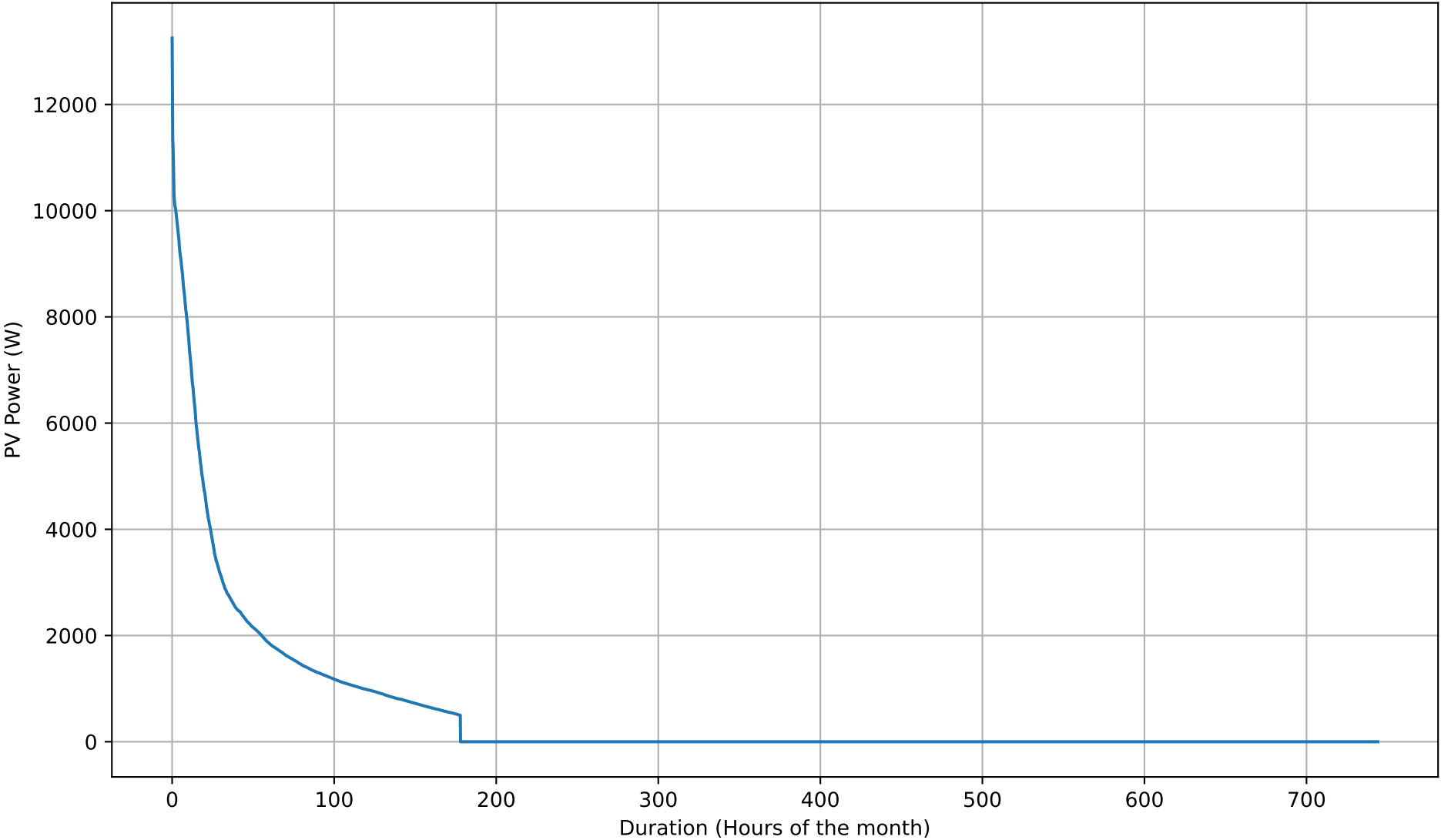
PV Self-Consumption Duration Curve - 20kWh - Jan
