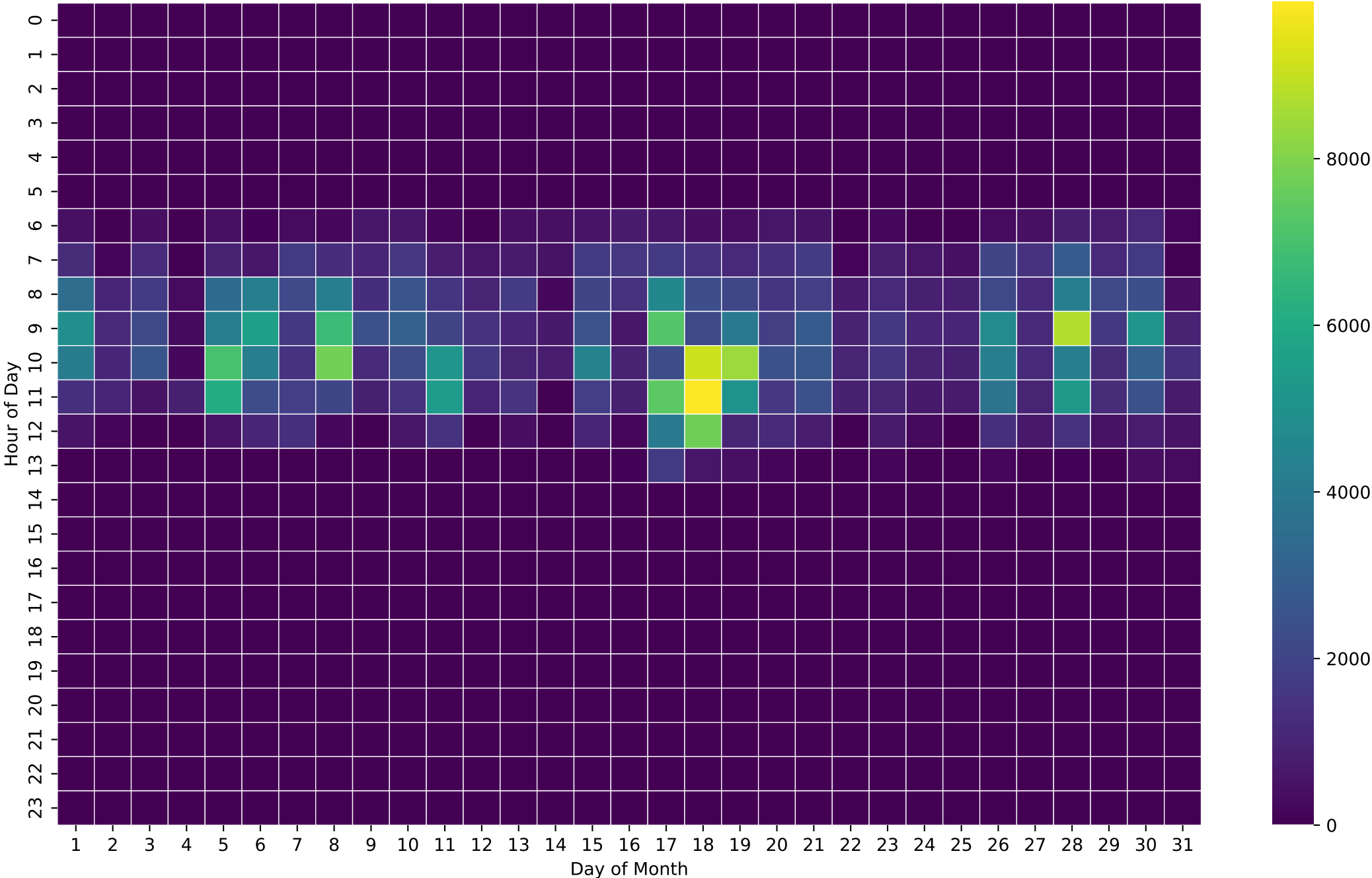
PV Self-Consumption Heatmap (Wh/Hour) - 20kWh - Jan
