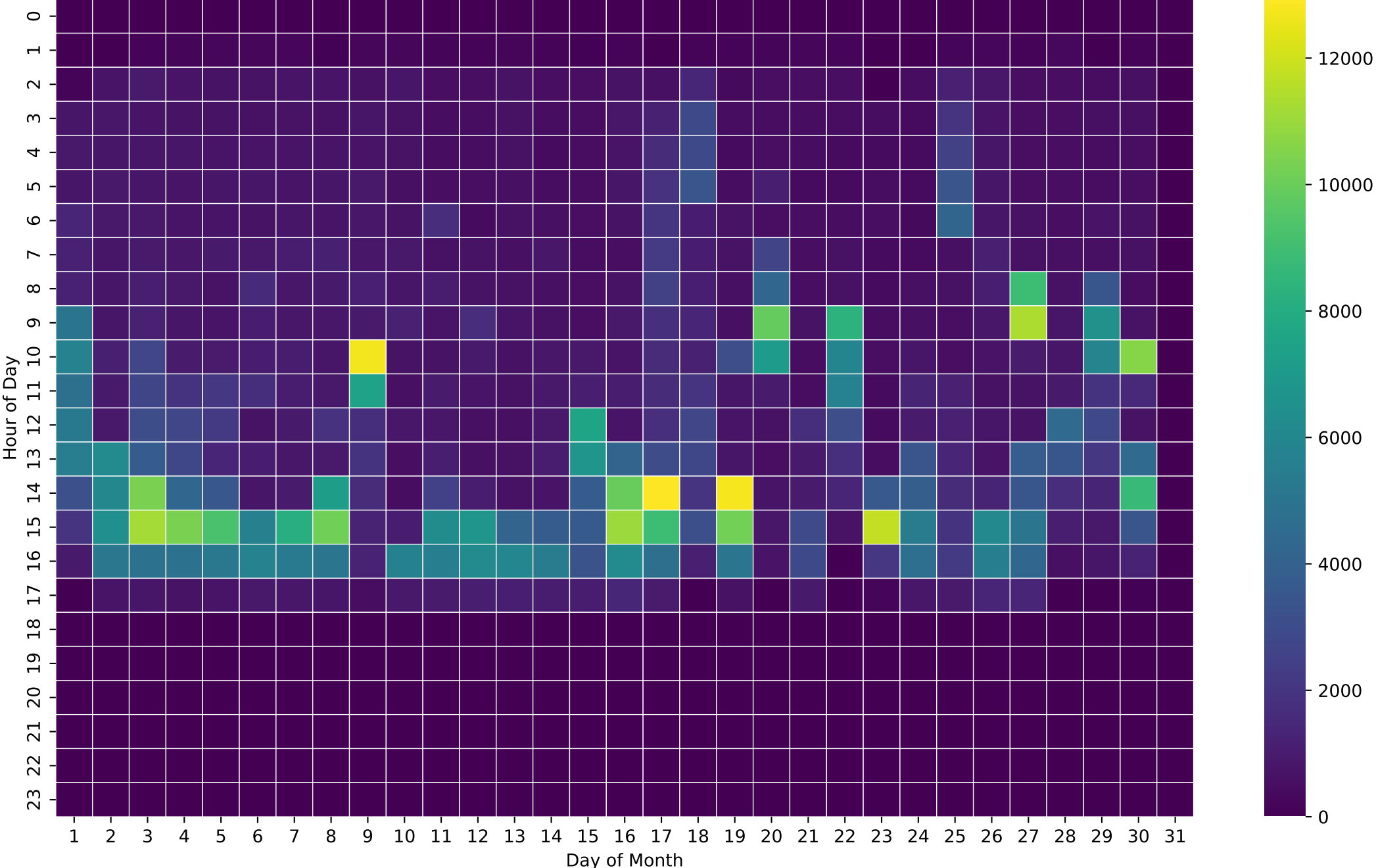
PV Self-Consumption Heatmap (Wh/Hour) - 20kWh - Jun
