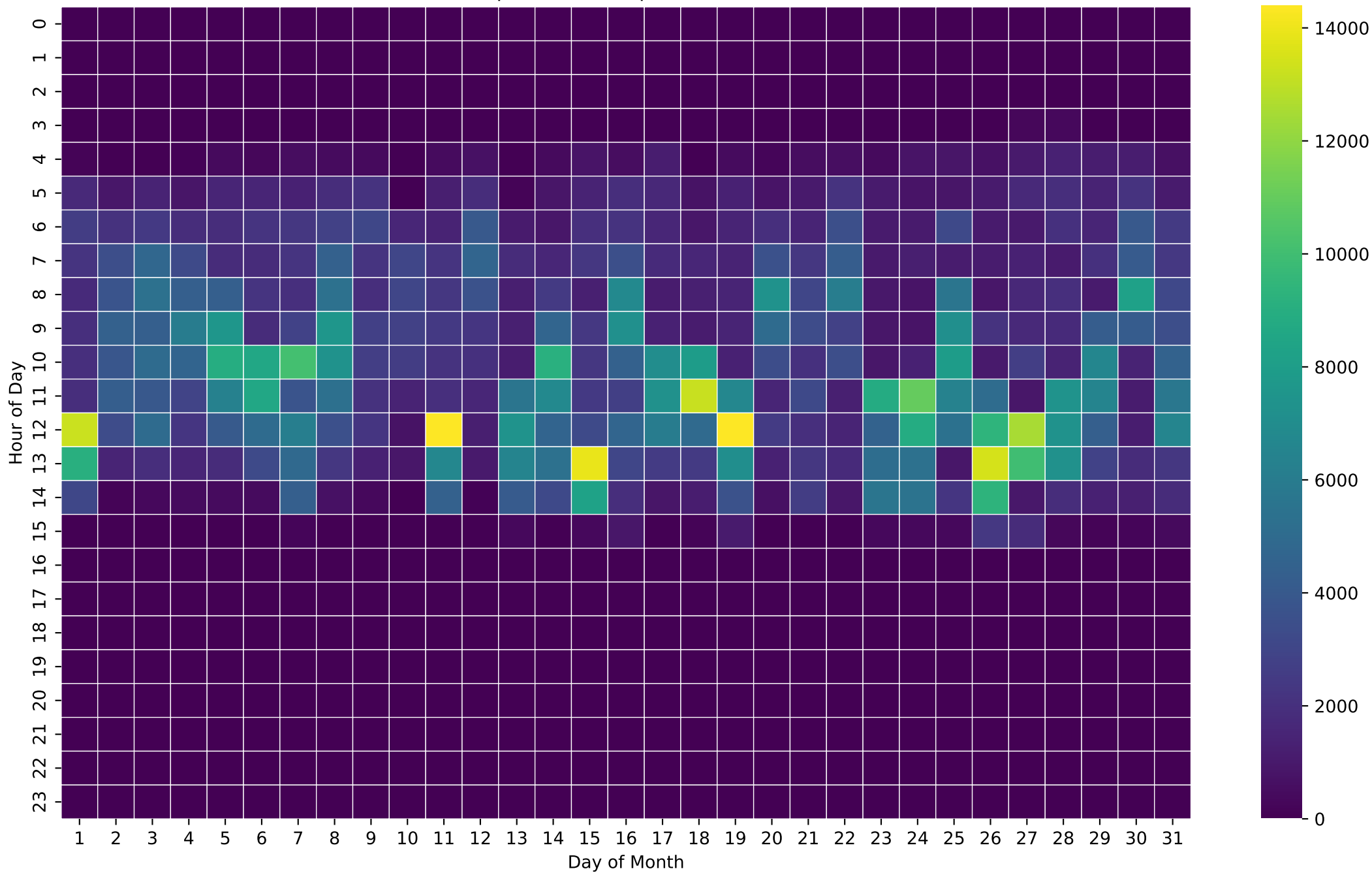
PV Self-Consumption Heatmap (Wh/Hour) - 20kWh - Mar
