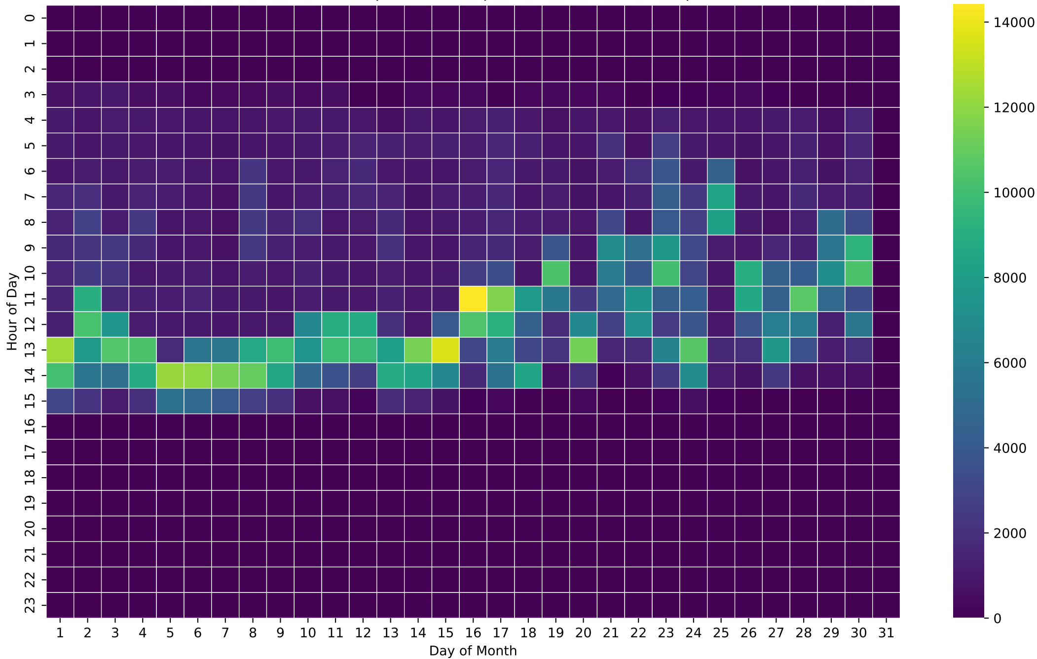
PV Self-Consumption Heatmap (Wh/Hour) - 20kWh - Sep
