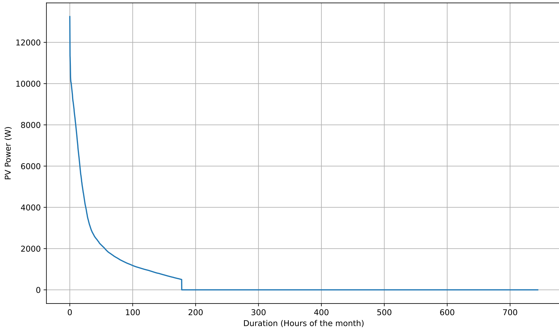
PV Production Duration Curve - 20kWh - Jan
