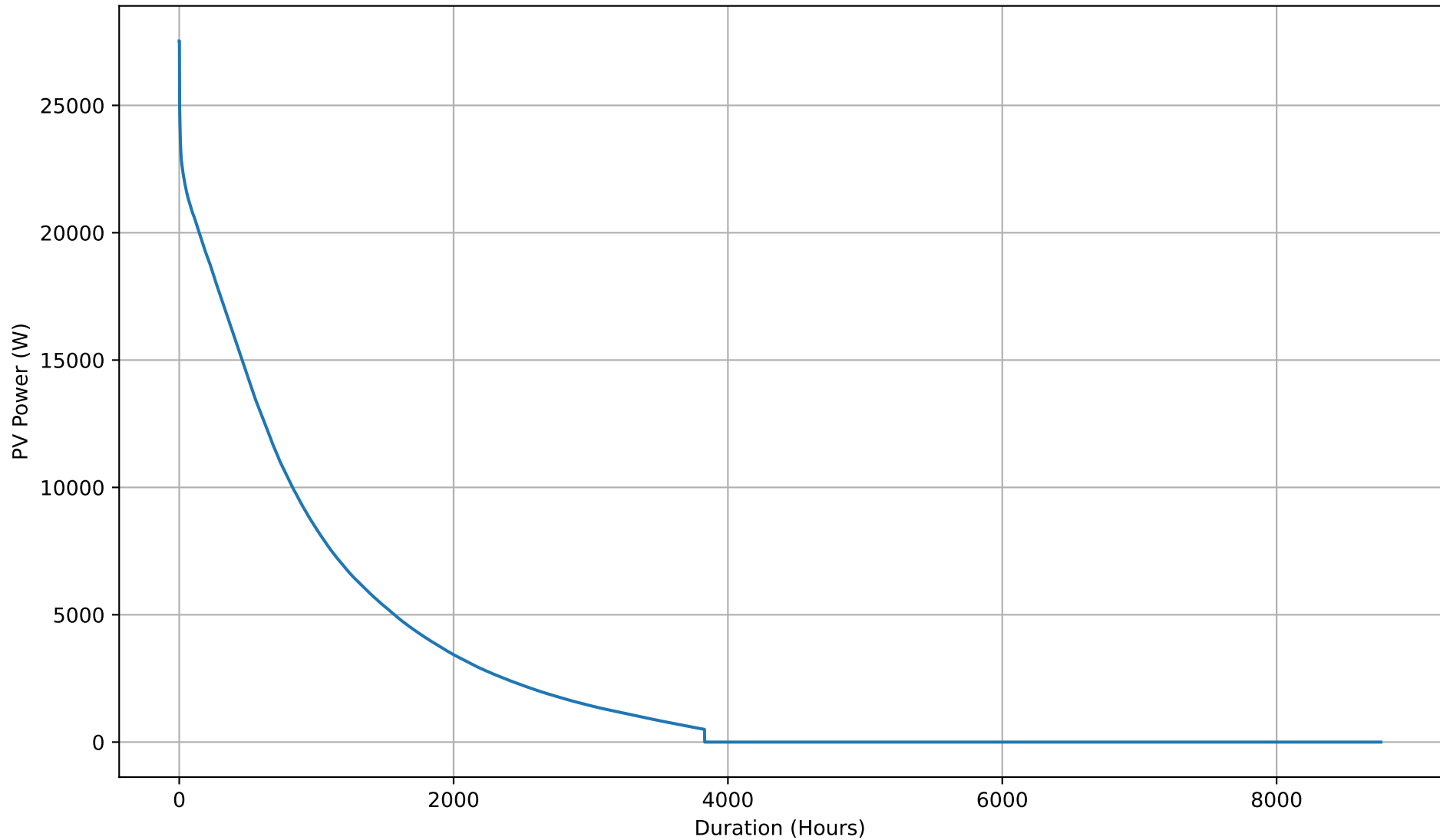
Yearly PV Production Duration Curve - 20kWh
