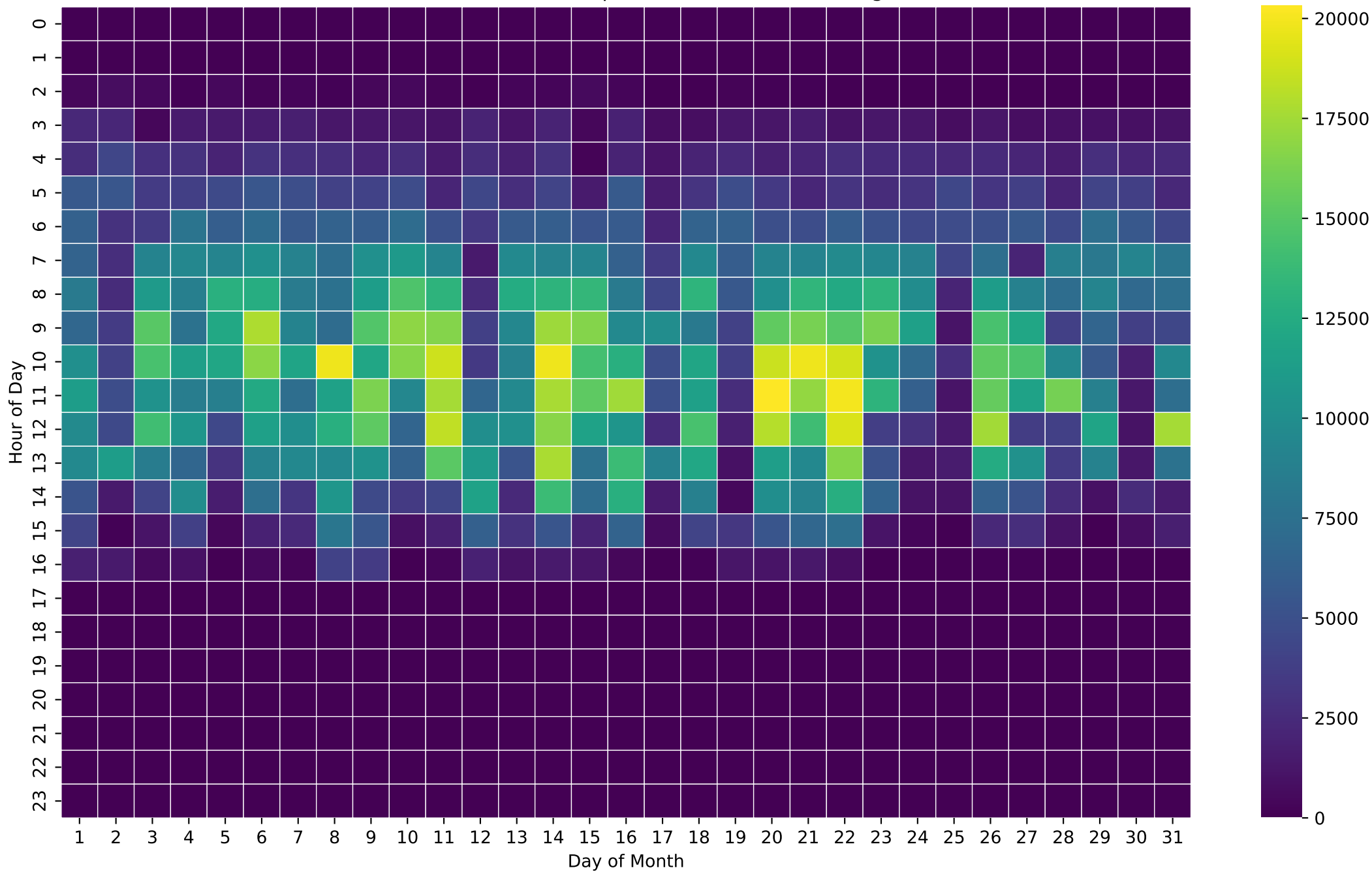
PV Production Heatmap (Wh/Hour) - 20kWh - Aug
