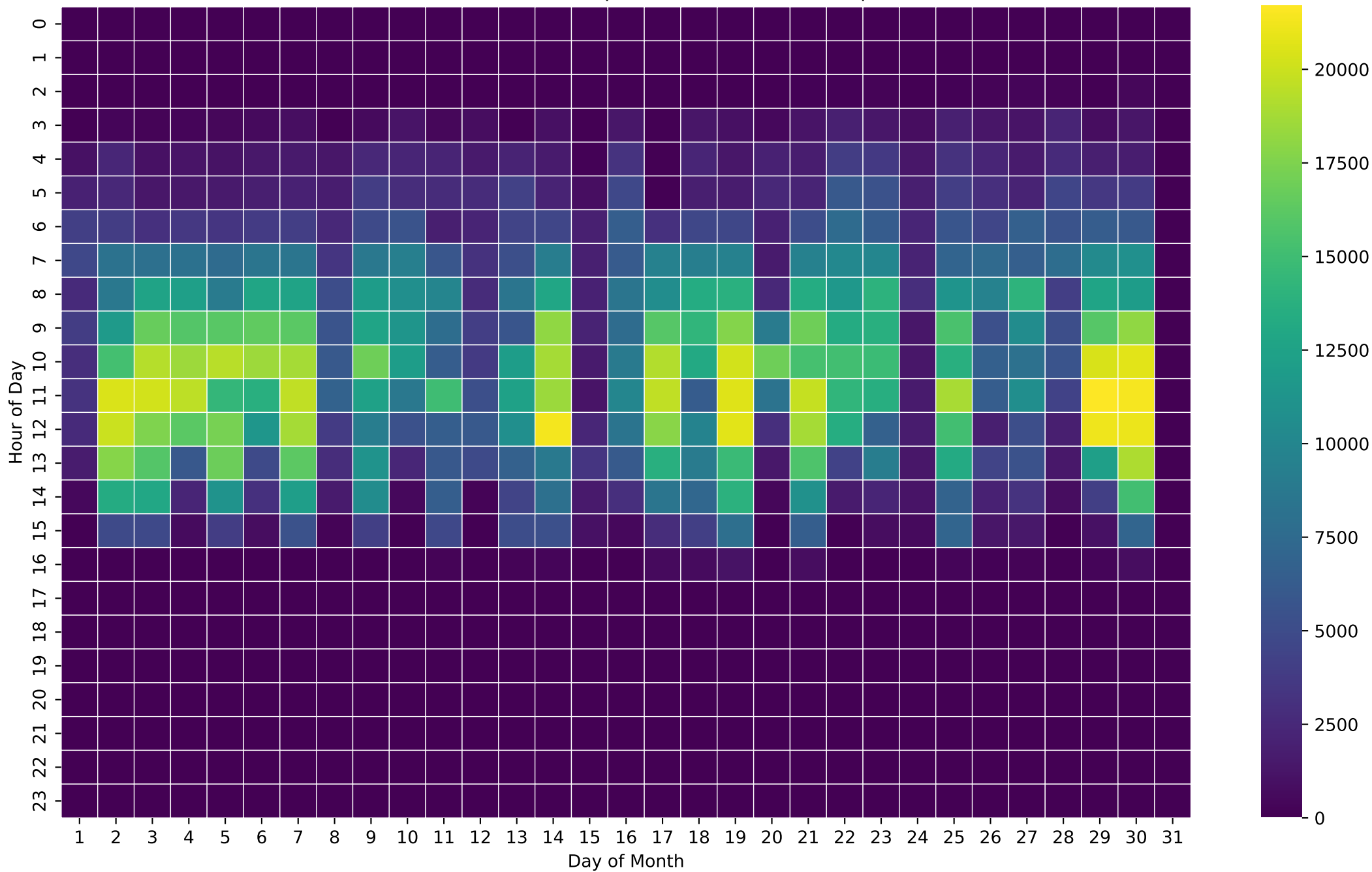
PV Production Heatmap (Wh/Hour) - 20kWh - Apr
