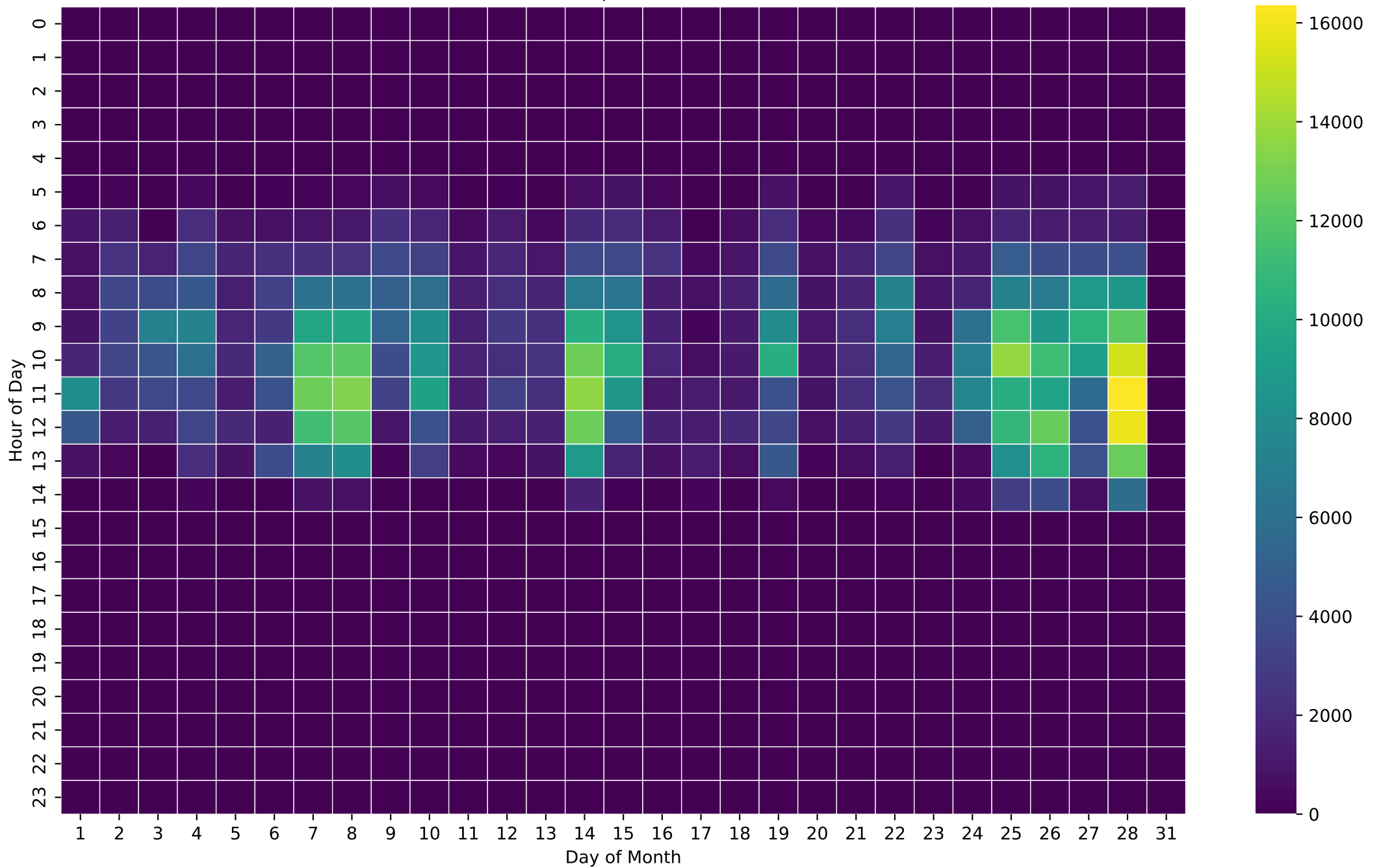
PV Production Heatmap (Wh/Hour) - 20kWh - Feb
