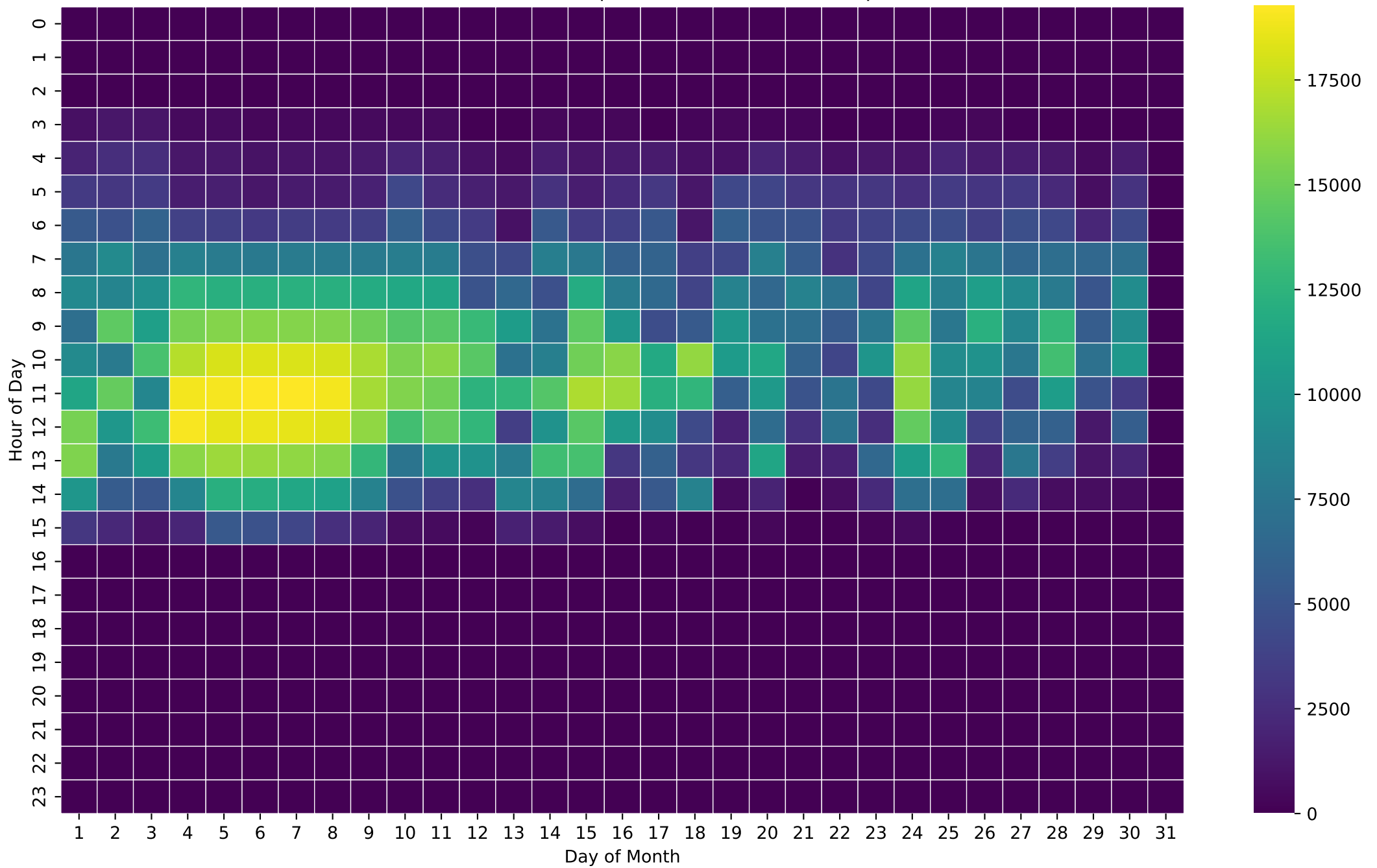
PV Production Heatmap (Wh/Hour) - 20kWh - Sep
