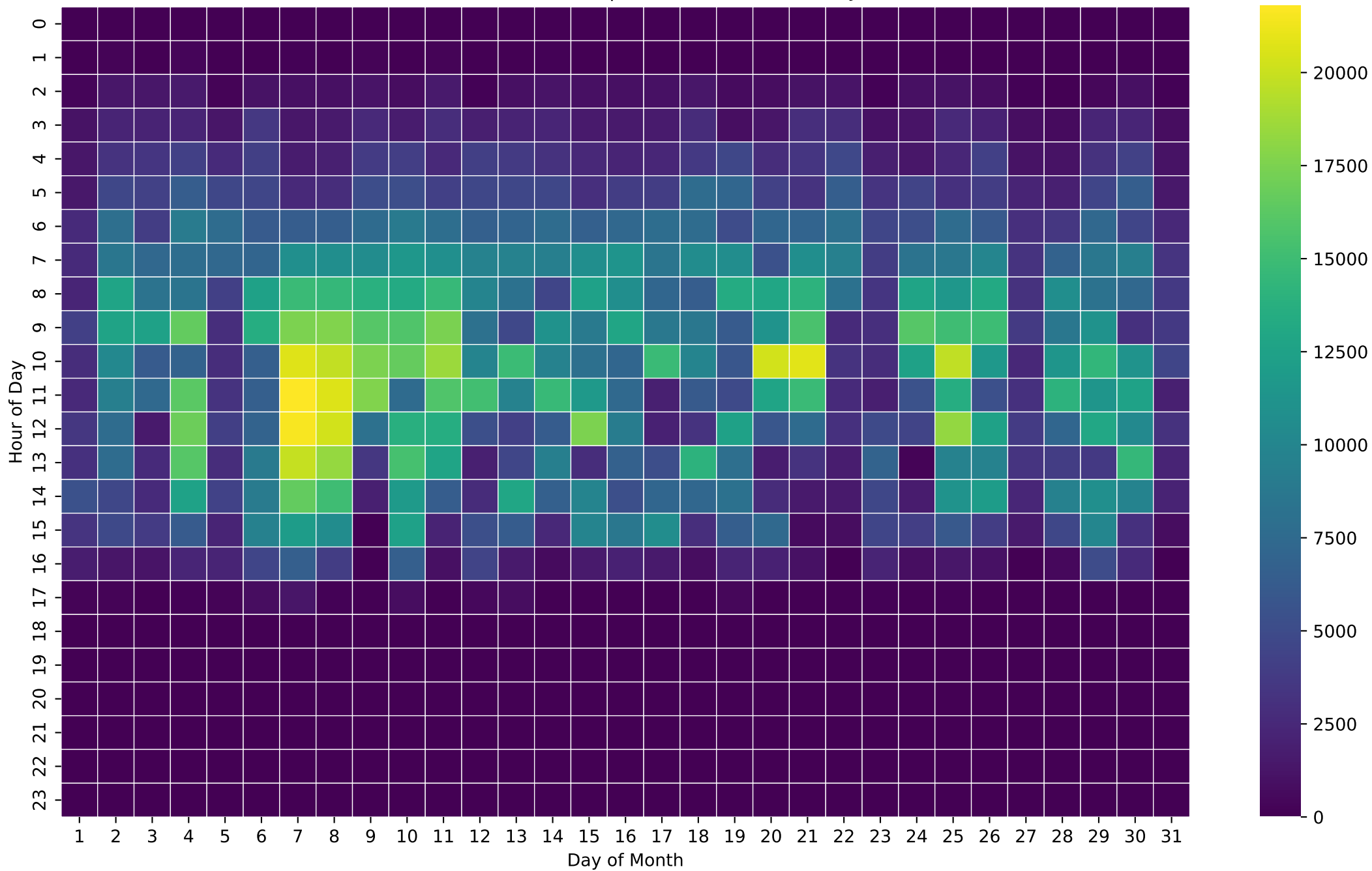
PV Production Heatmap (Wh/Hour) - 20kWh - Jul
