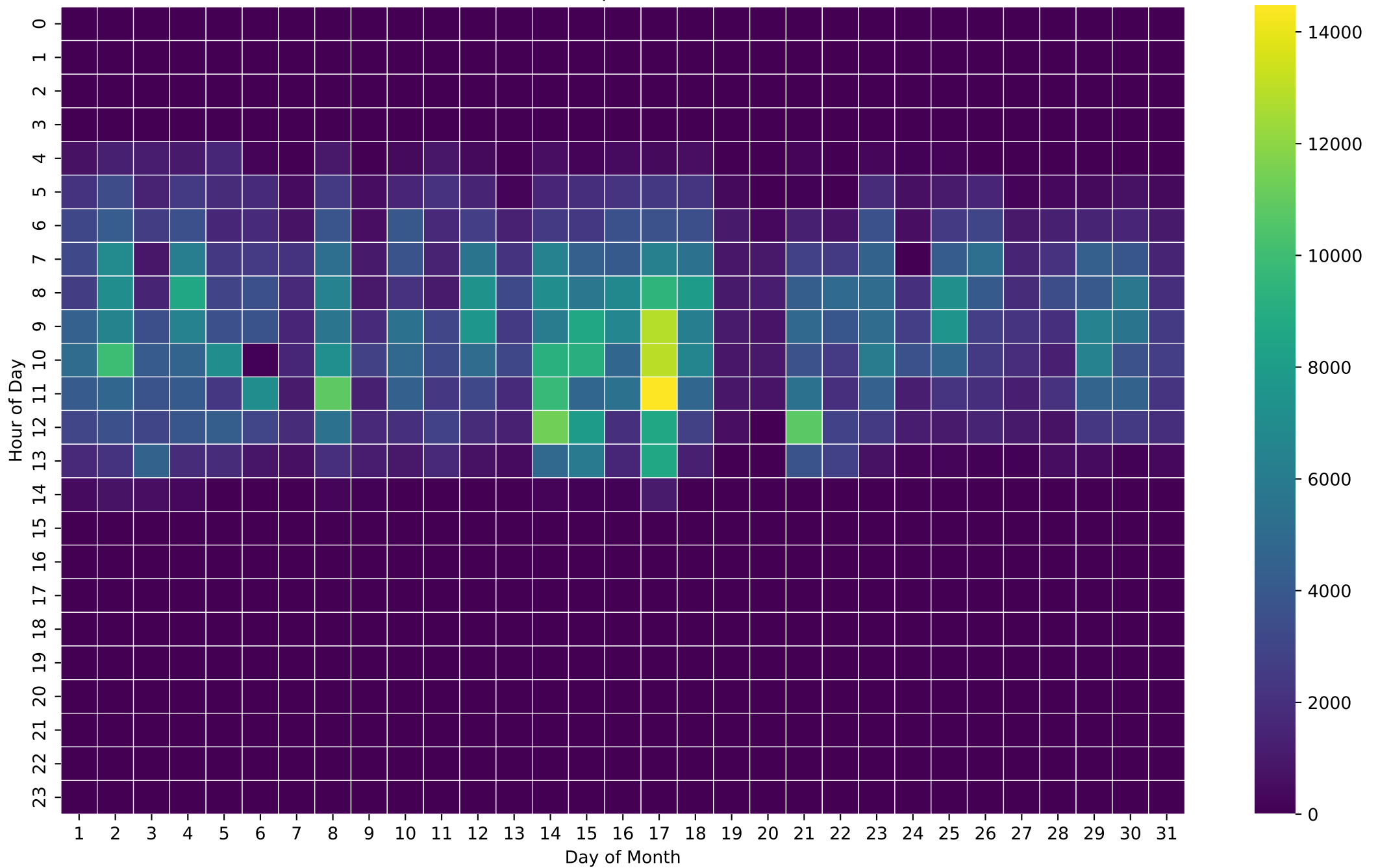
PV Production Heatmap (Wh/Hour) - 20kWh - Oct
