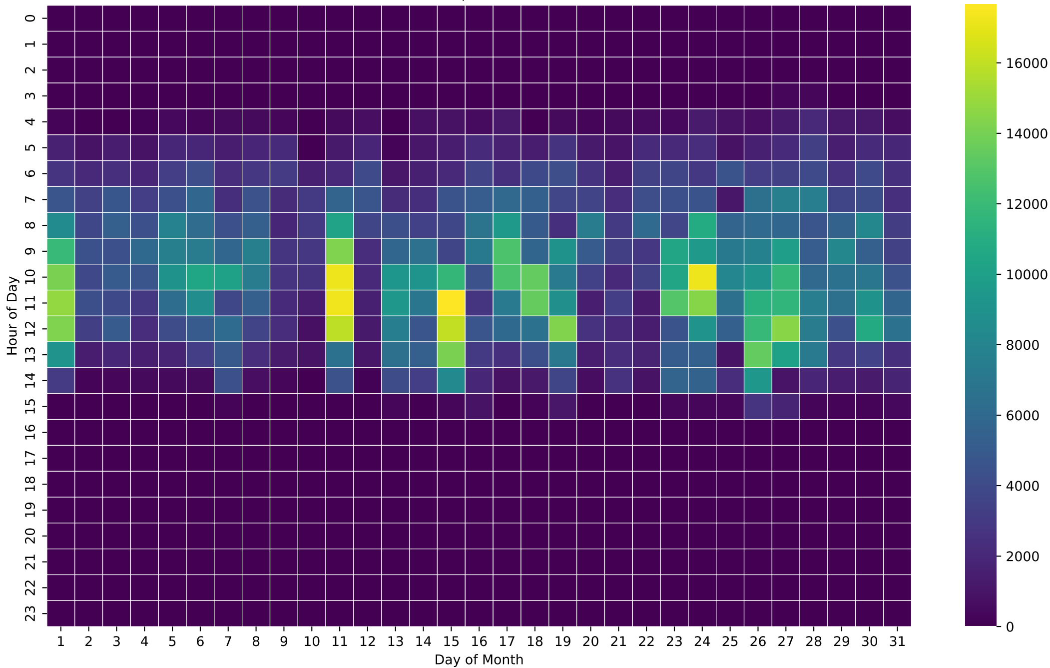
PV Production Heatmap (Wh/Hour) - 20kWh - Mar
