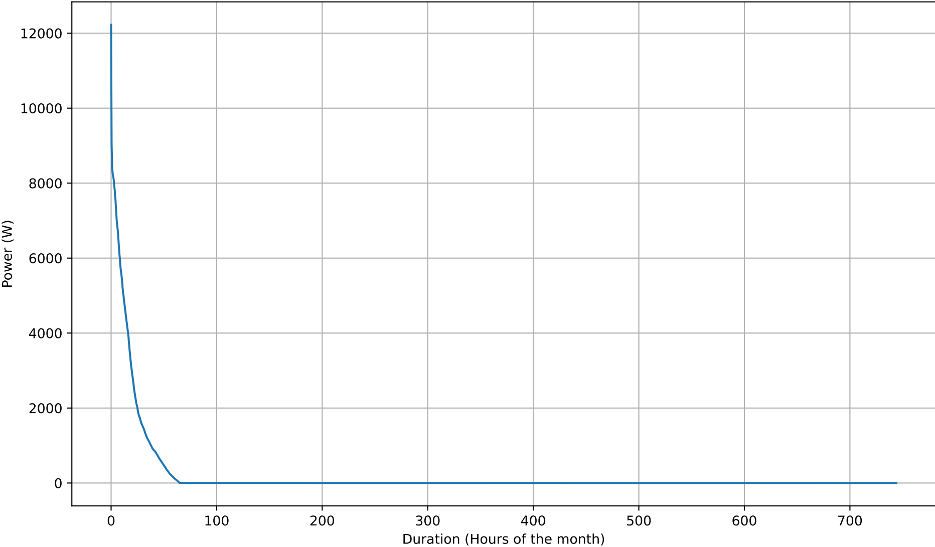
Battery Charging Power Duration Curve - 26kWh - Jan
