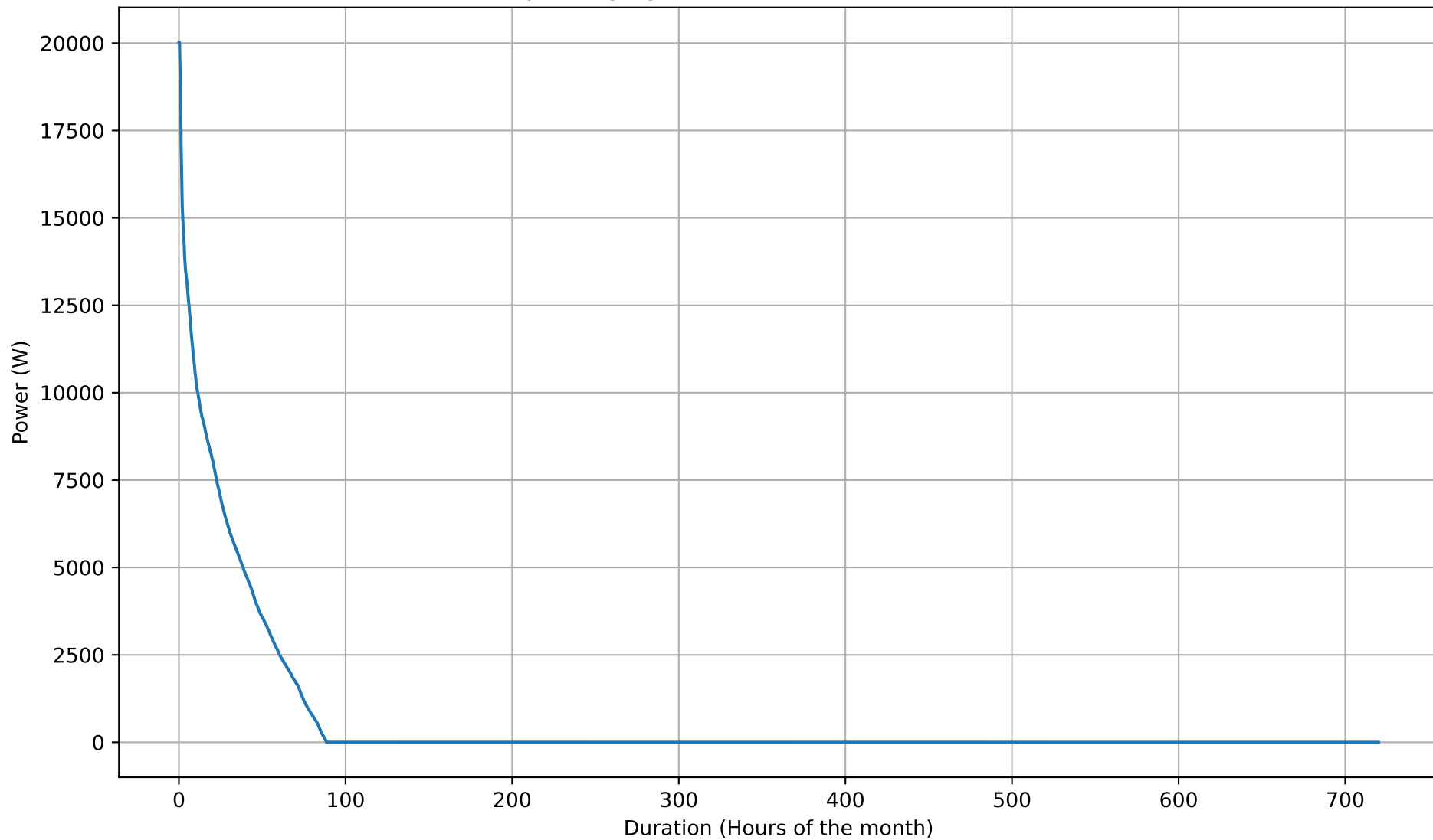
Battery Charging Power Duration Curve - 26kWh - Jun
