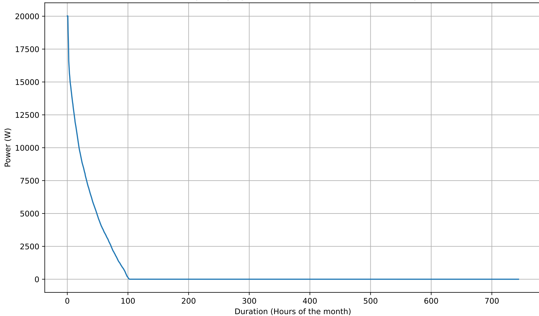
Battery Charging Power Duration Curve - 26kWh - May
