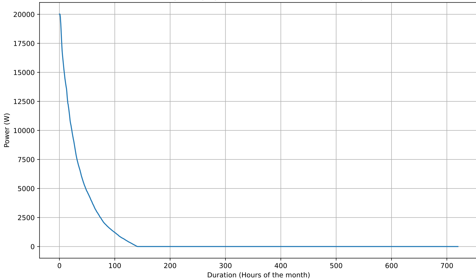
Battery Charging Power Duration Curve - 26kWh - Apr
