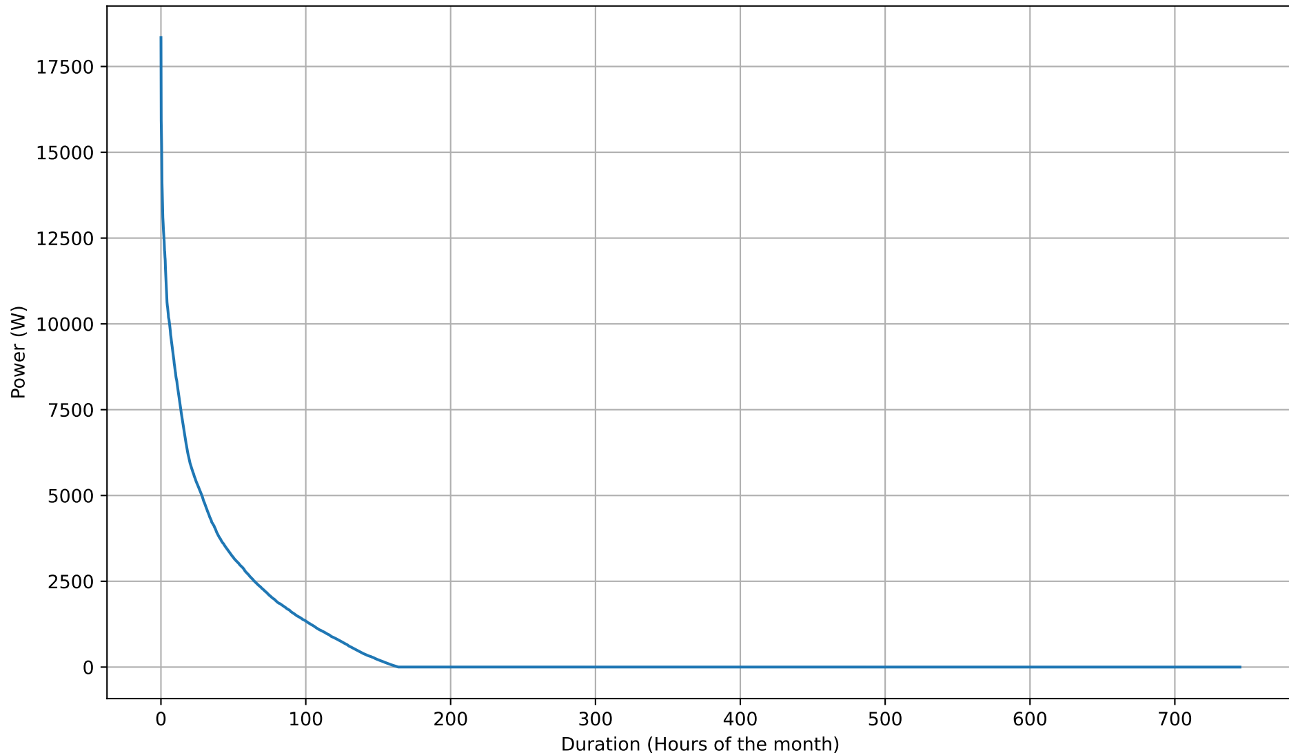
Battery Charging Power Duration Curve - 26kWh - Oct
