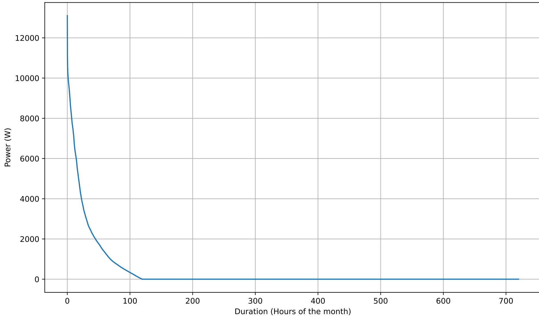
Battery Charging Power Duration Curve - 26kWh - Nov
