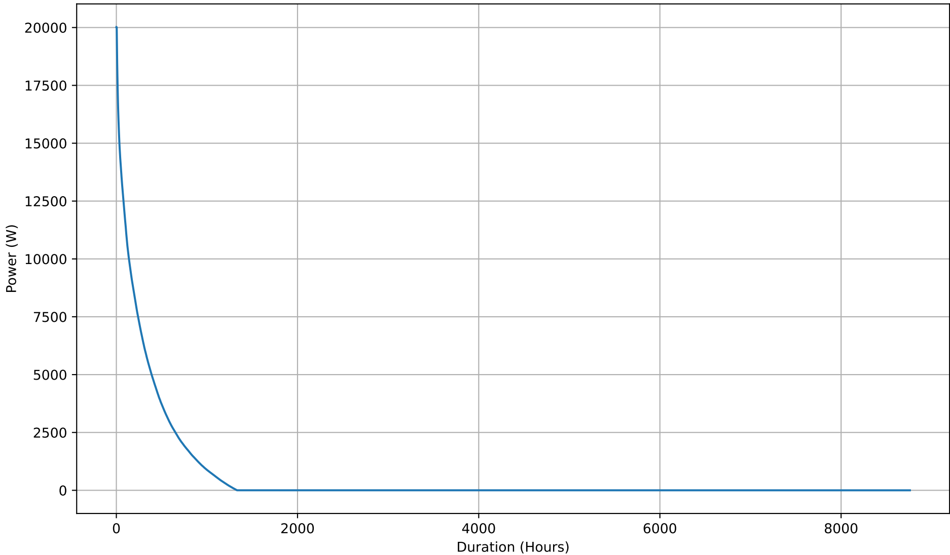
Yearly Battery Charging Power Duration Curve - 26kWh
