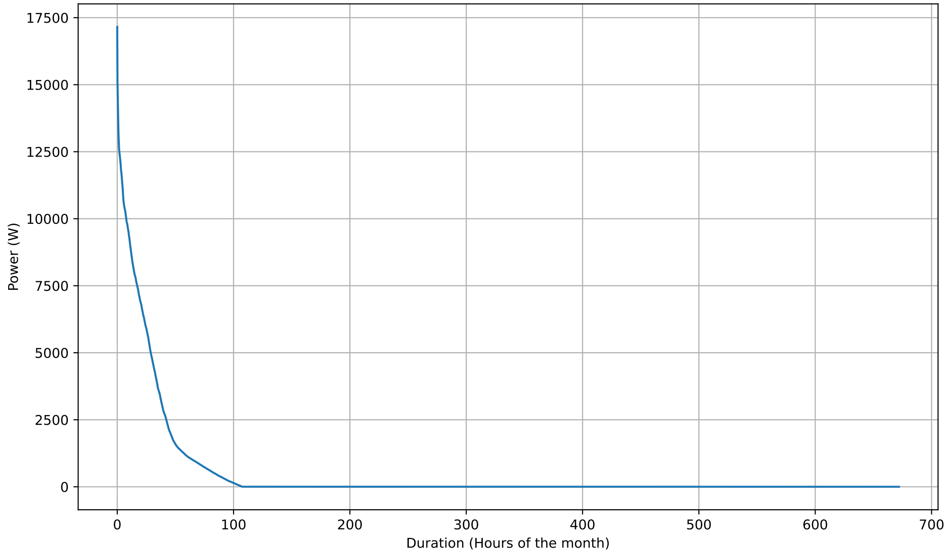
Battery Charging Power Duration Curve - 26kWh - Feb
