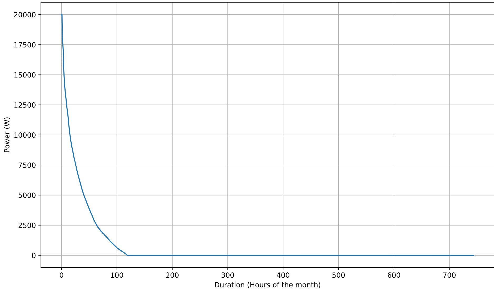
Battery Charging Power Duration Curve - 26kWh - Aug
