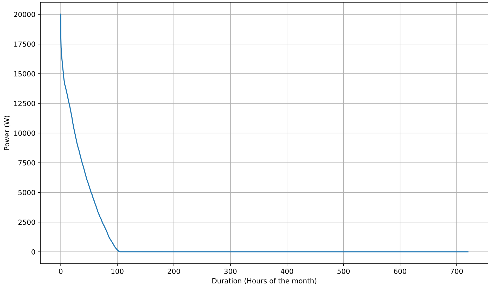
Battery Charging Power Duration Curve - 26kWh - Sep
