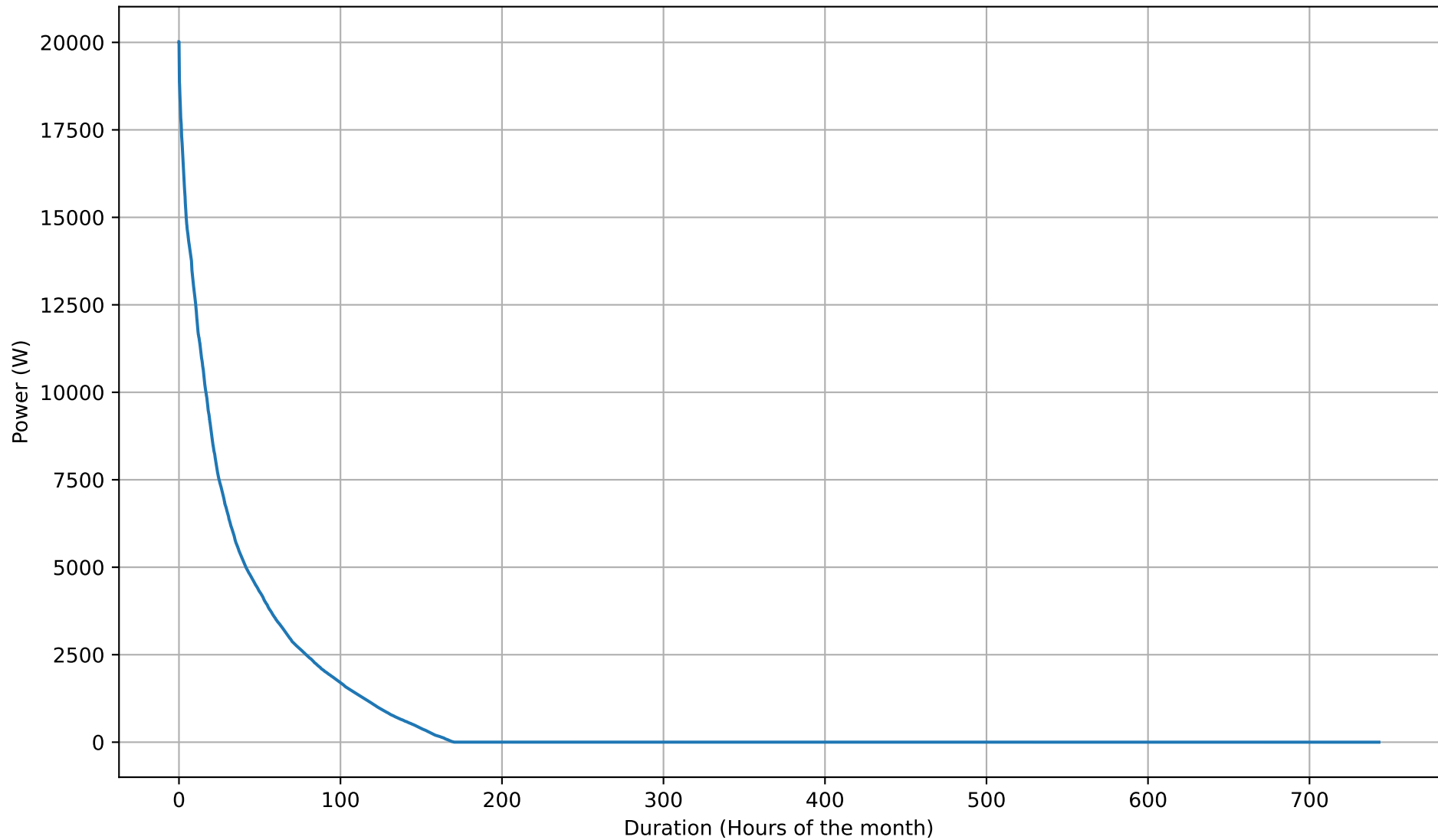
Battery Charging Power Duration Curve - 26kWh - Mar
