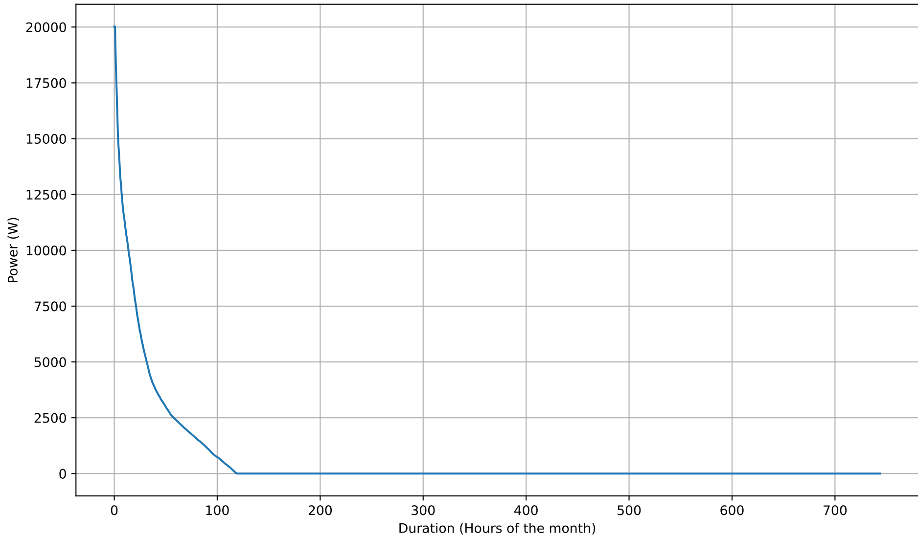
Battery Charging Power Duration Curve - 26kWh - Jul
