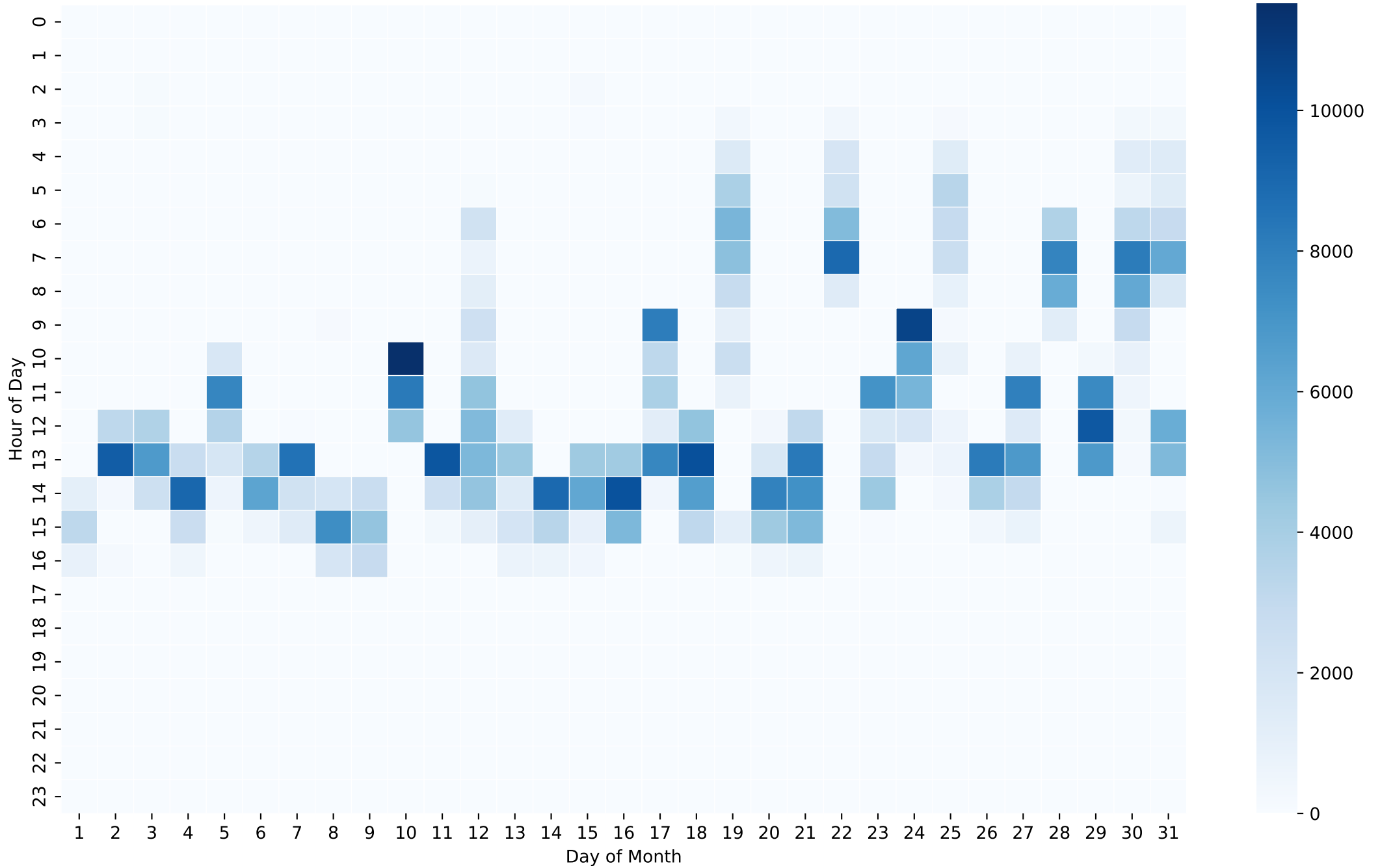
Battery Charging Power Heatmap (Wh/Hour) - 26kWh - Aug
