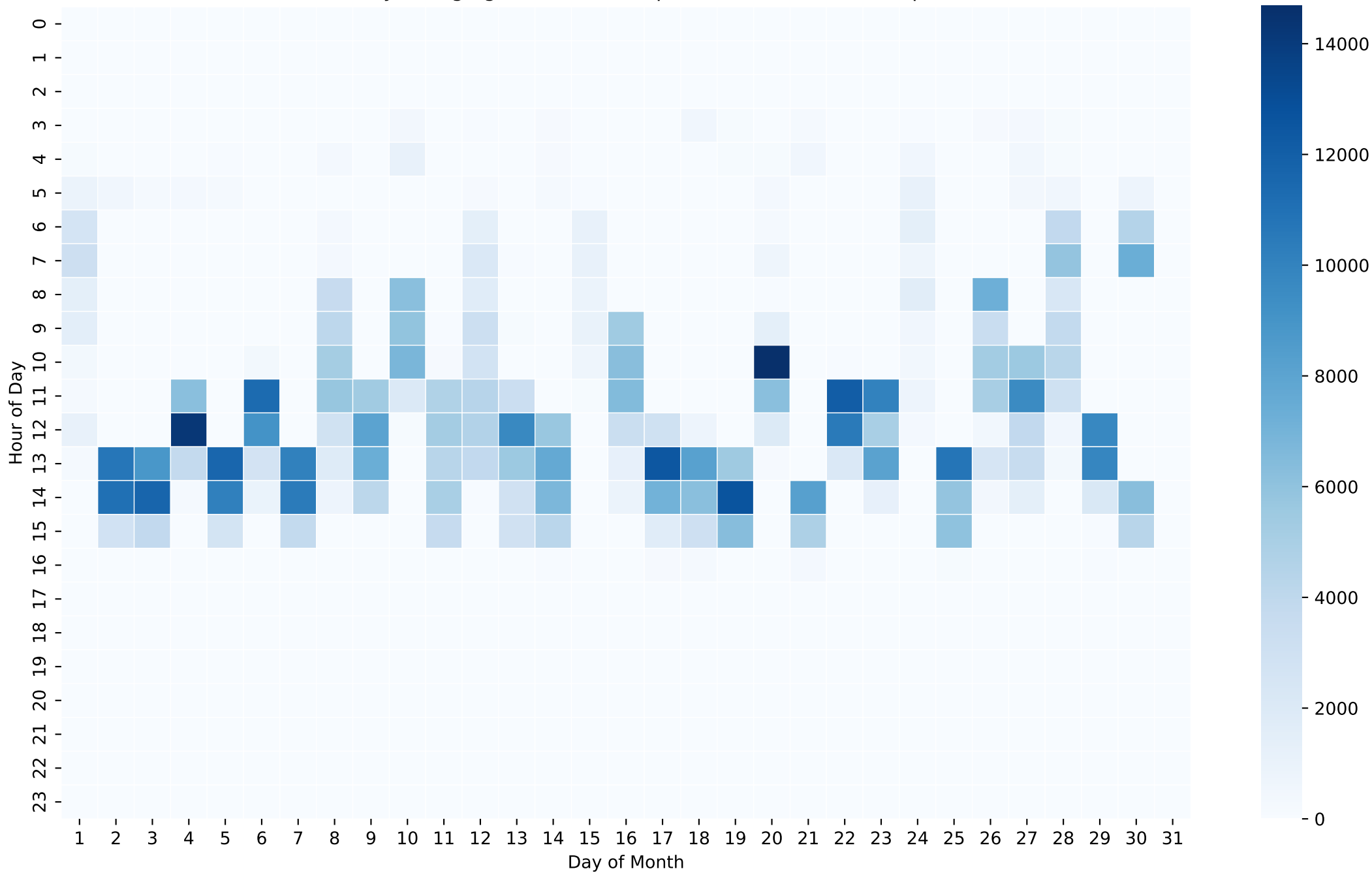
Battery Charging Power Heatmap (Wh/Hour) - 26kWh - Apr
