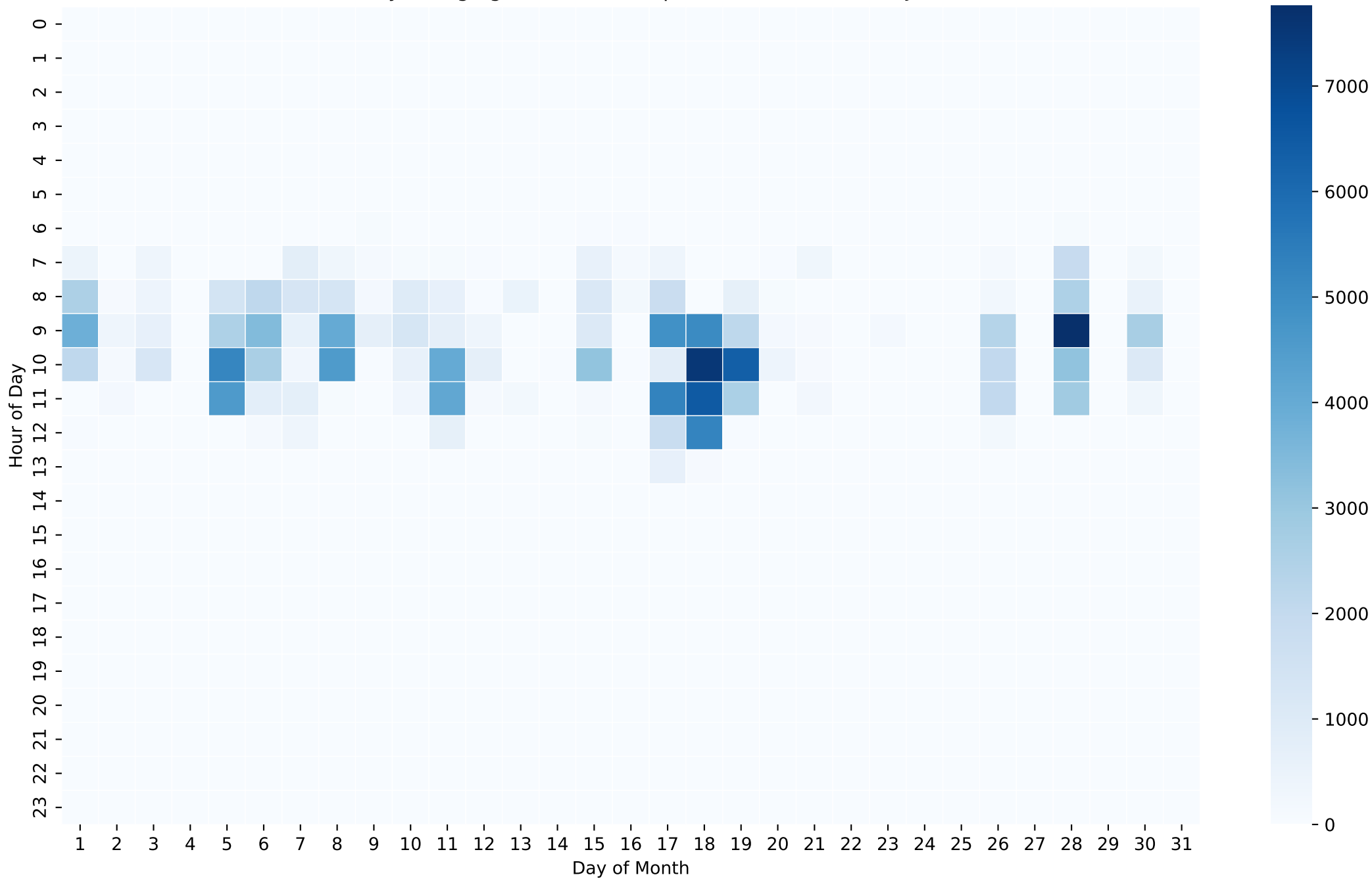
Battery Charging Power Heatmap (Wh/Hour) - 26kWh - Jan
