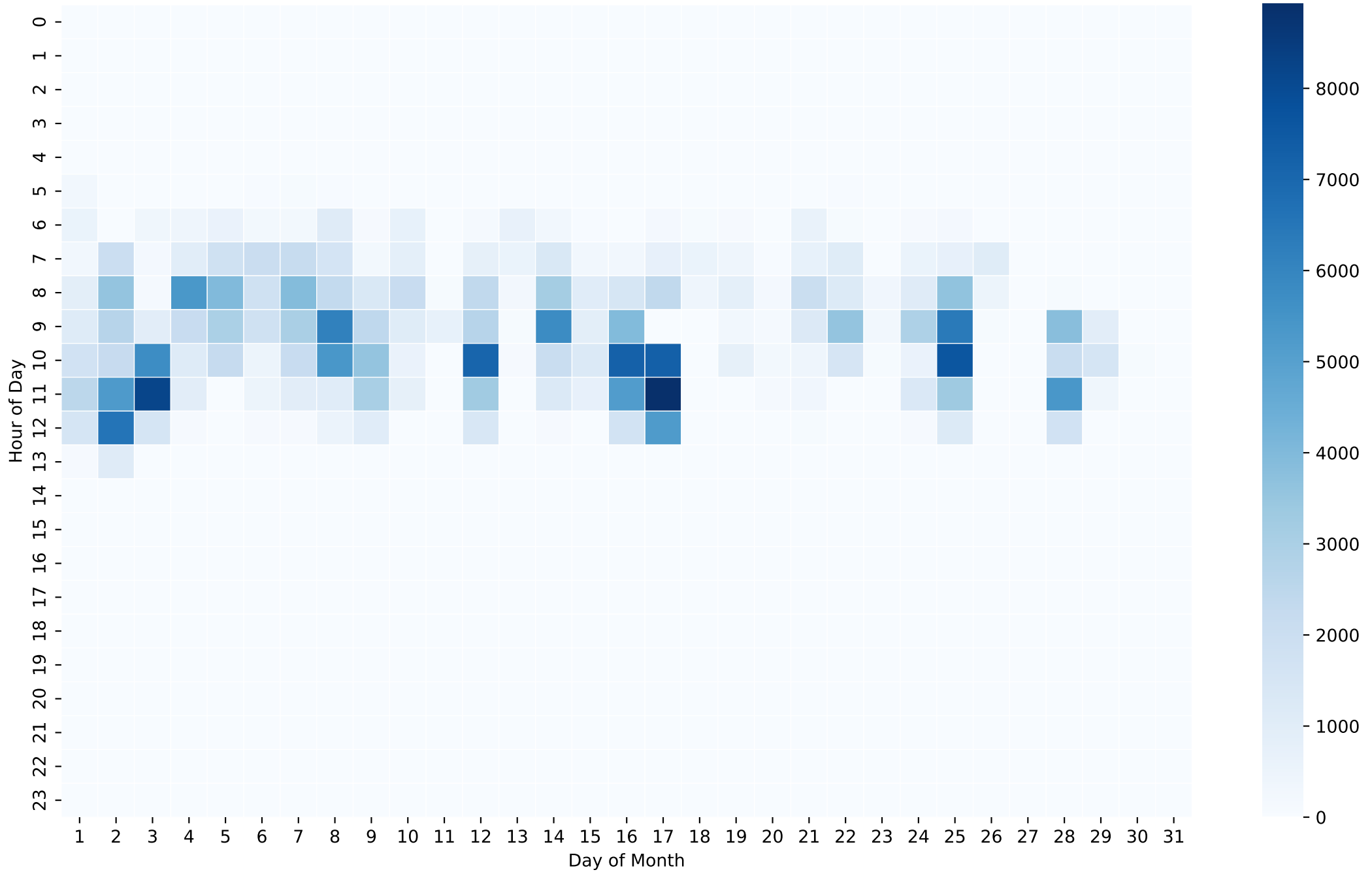
Battery Charging Power Heatmap (Wh/Hour) - 26kWh - Nov
