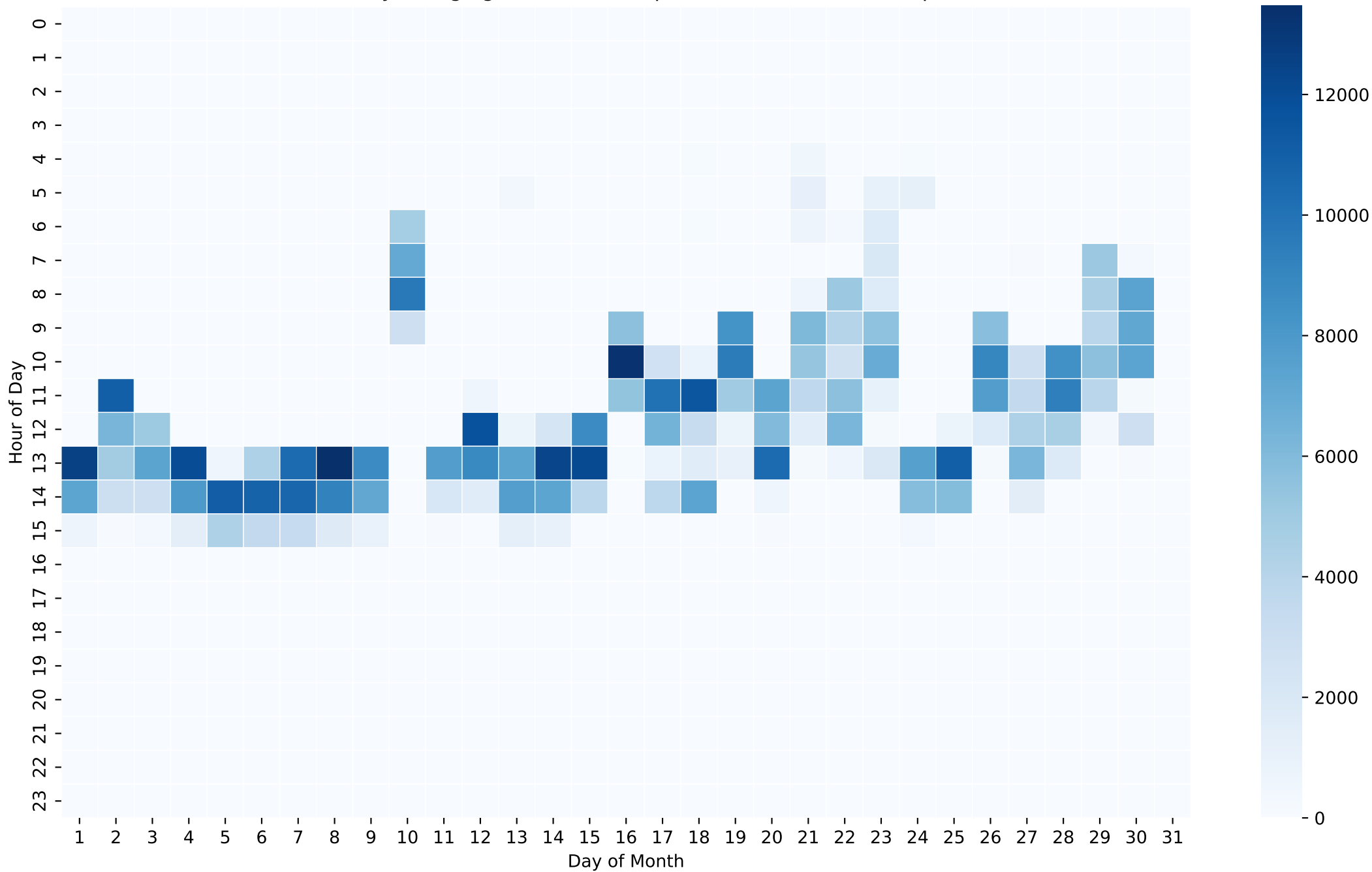
Battery Charging Power Heatmap (Wh/Hour) - 26kWh - Sep
