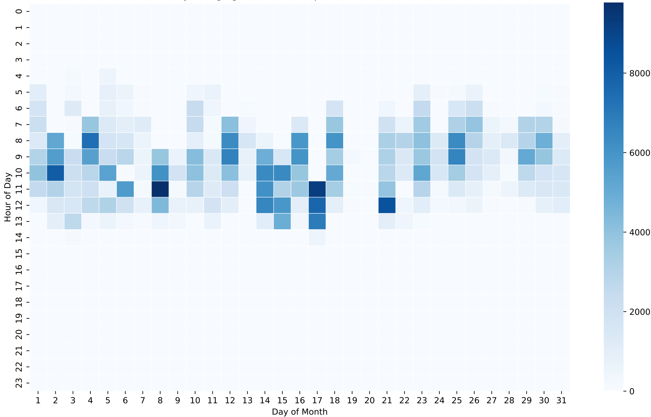
Battery Charging Power Heatmap (Wh/Hour) - 26kWh - Oct
