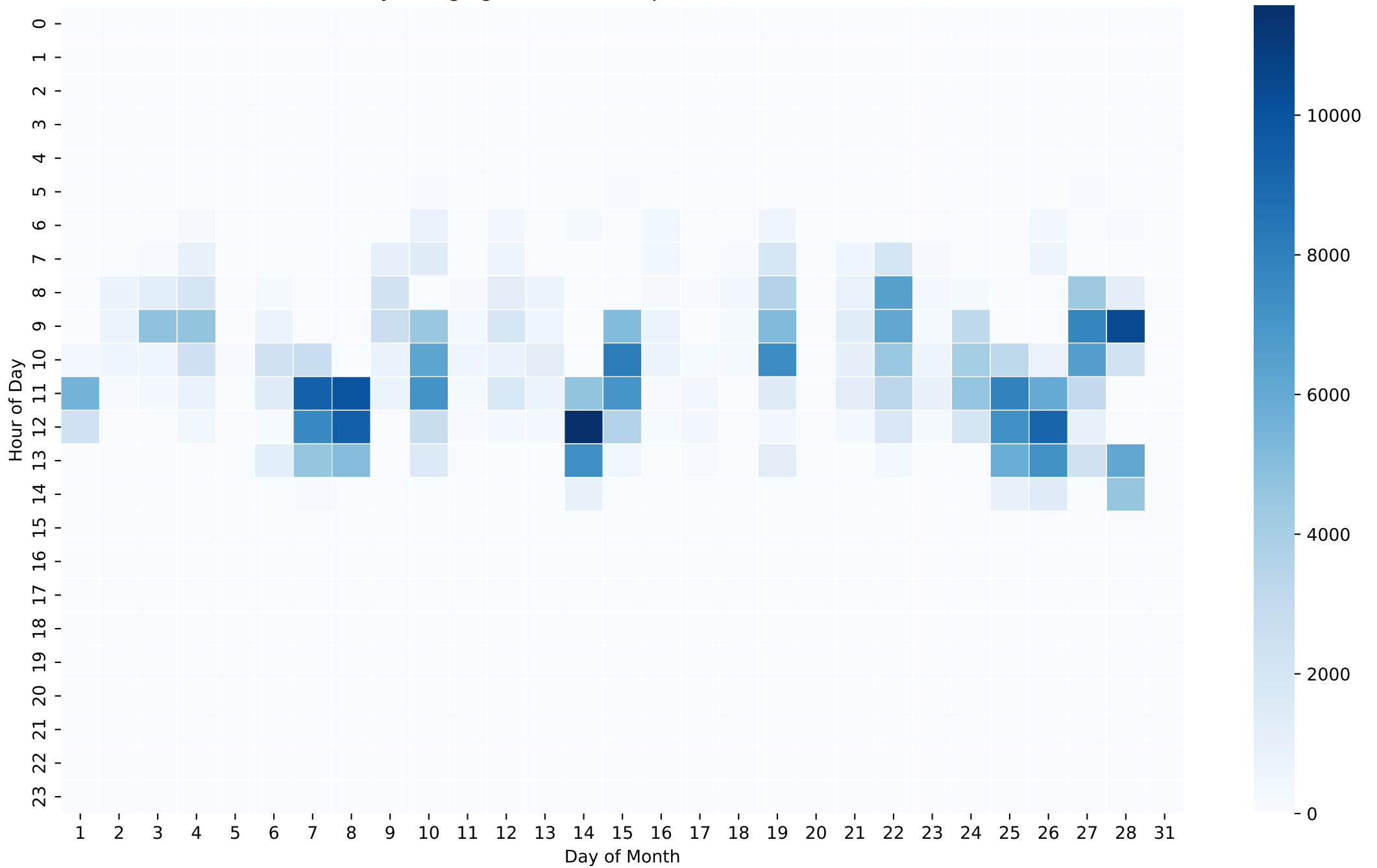
Battery Charging Power Heatmap (Wh/Hour) - 26kWh - Feb
