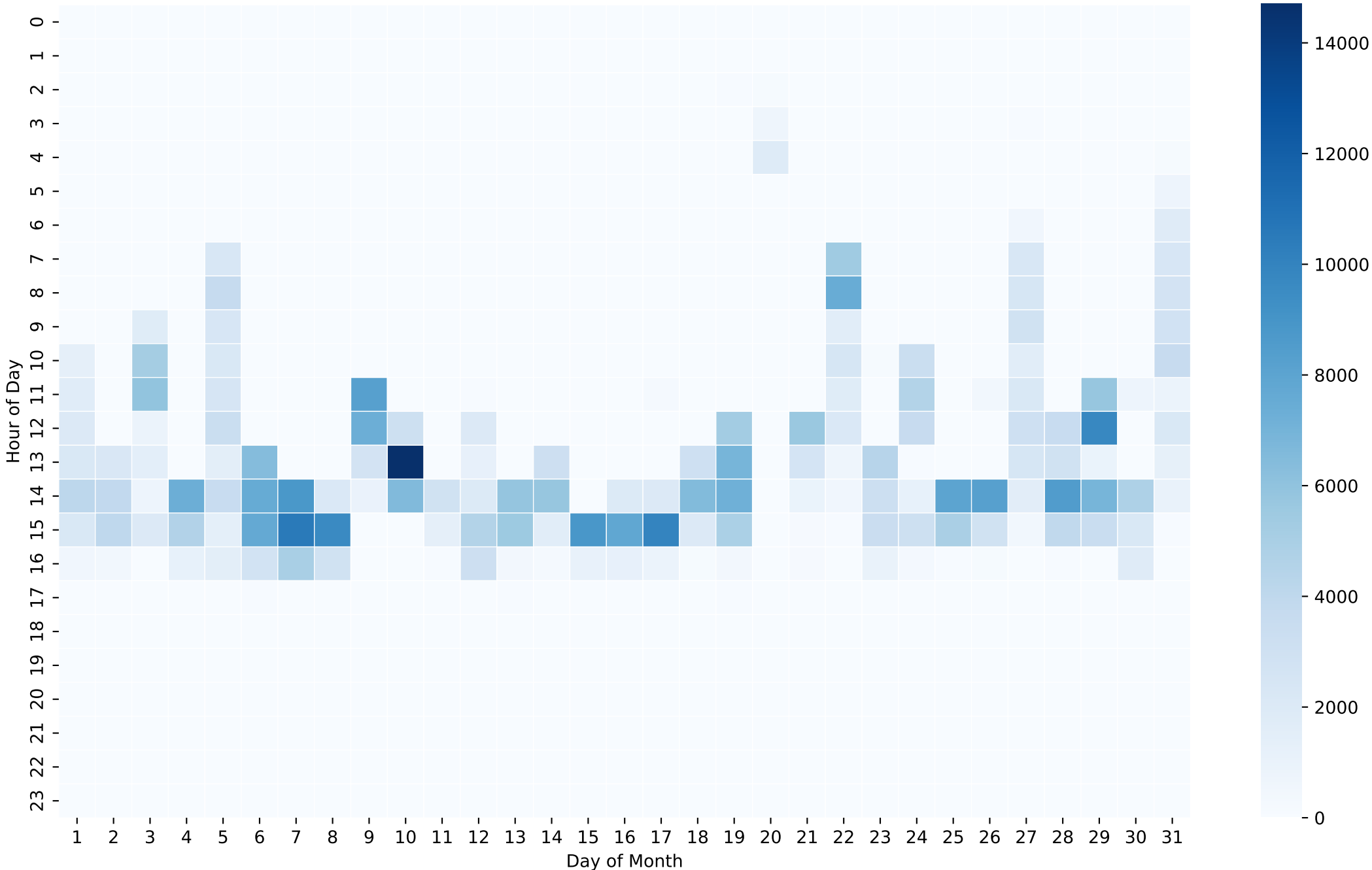
Battery Charging Power Heatmap (Wh/Hour) - 26kWh - Jul
