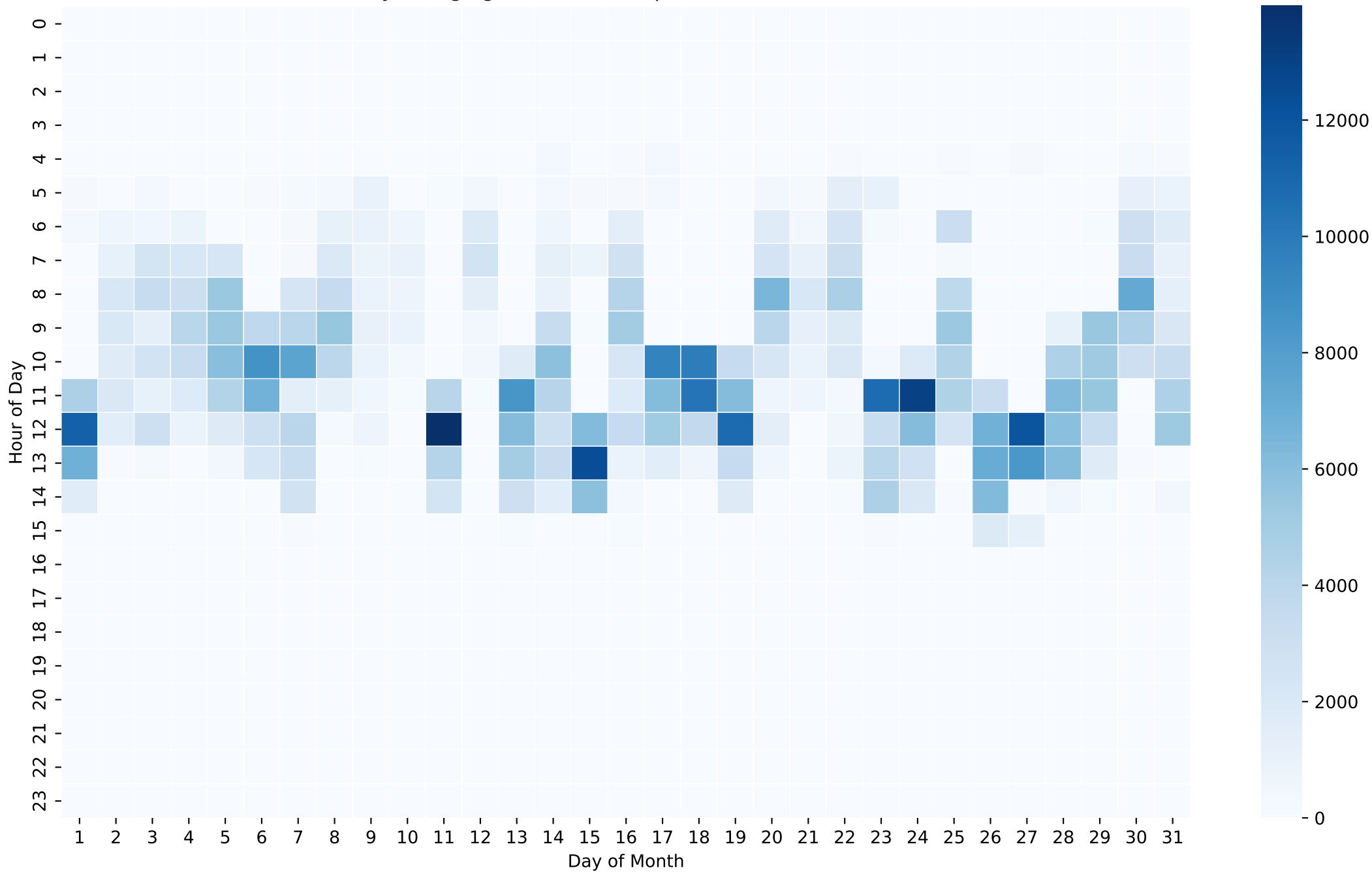
Battery Charging Power Heatmap (Wh/Hour) - 26kWh - Mar
