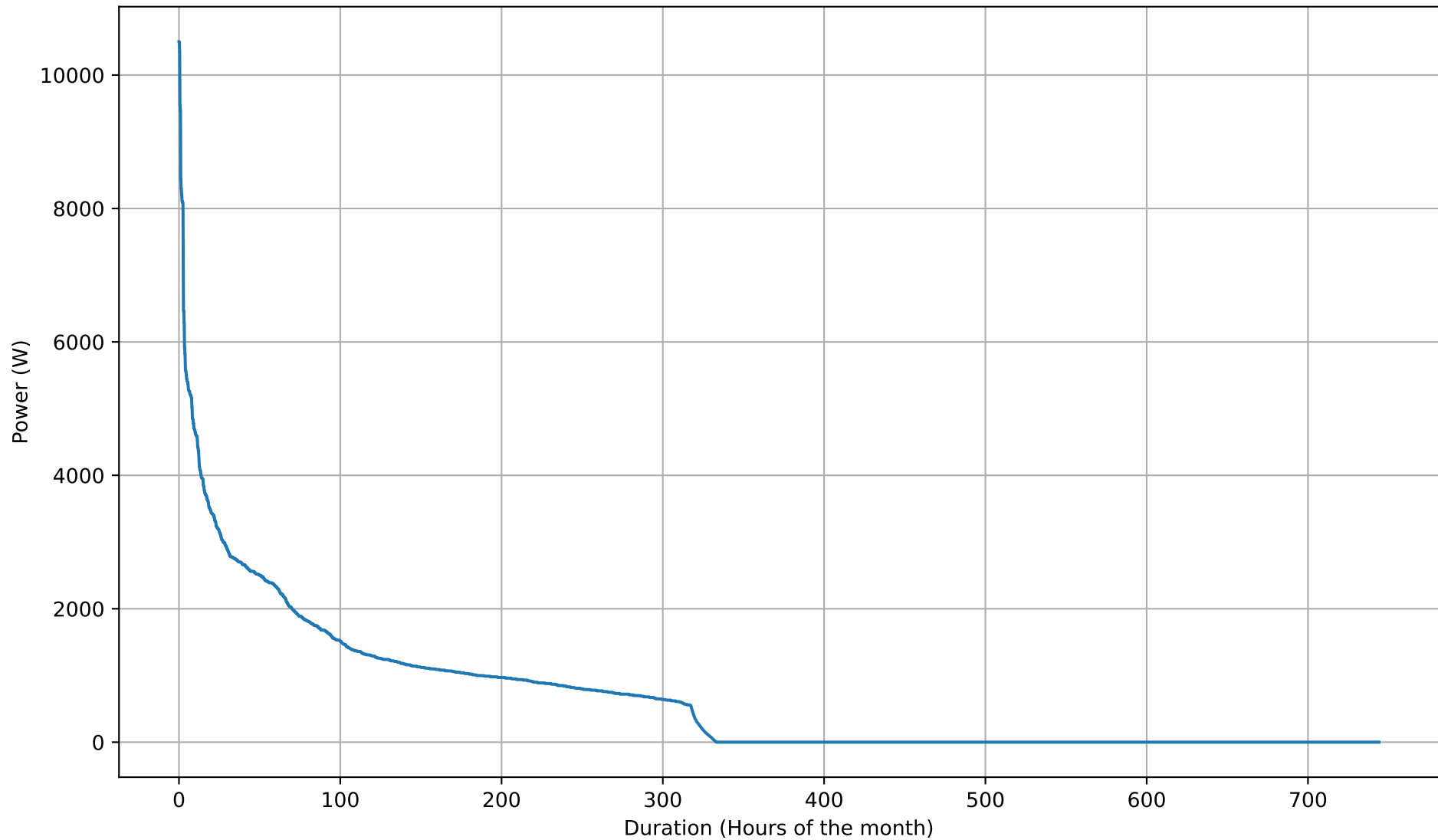
Battery Discharging Power Duration Curve - 26kWh - Aug
