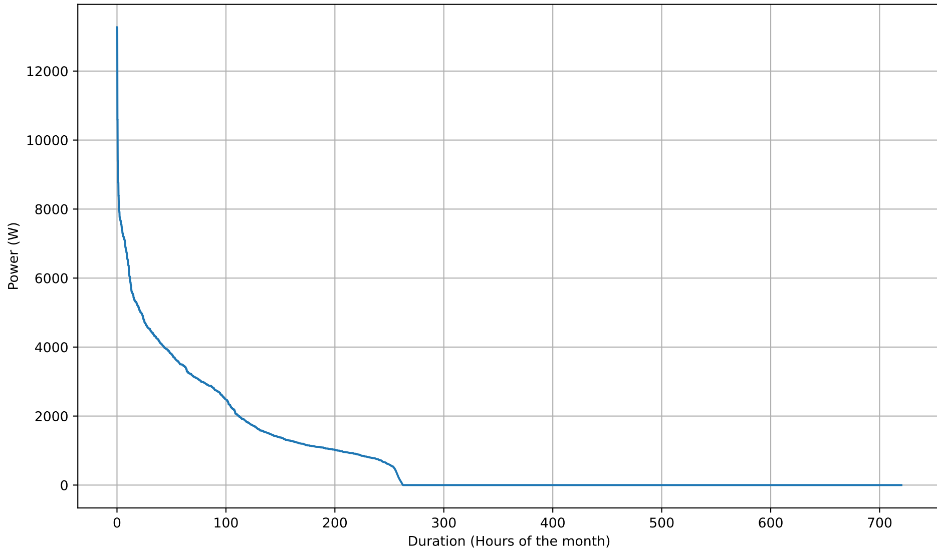
Battery Discharging Power Duration Curve - 26kWh - Apr
