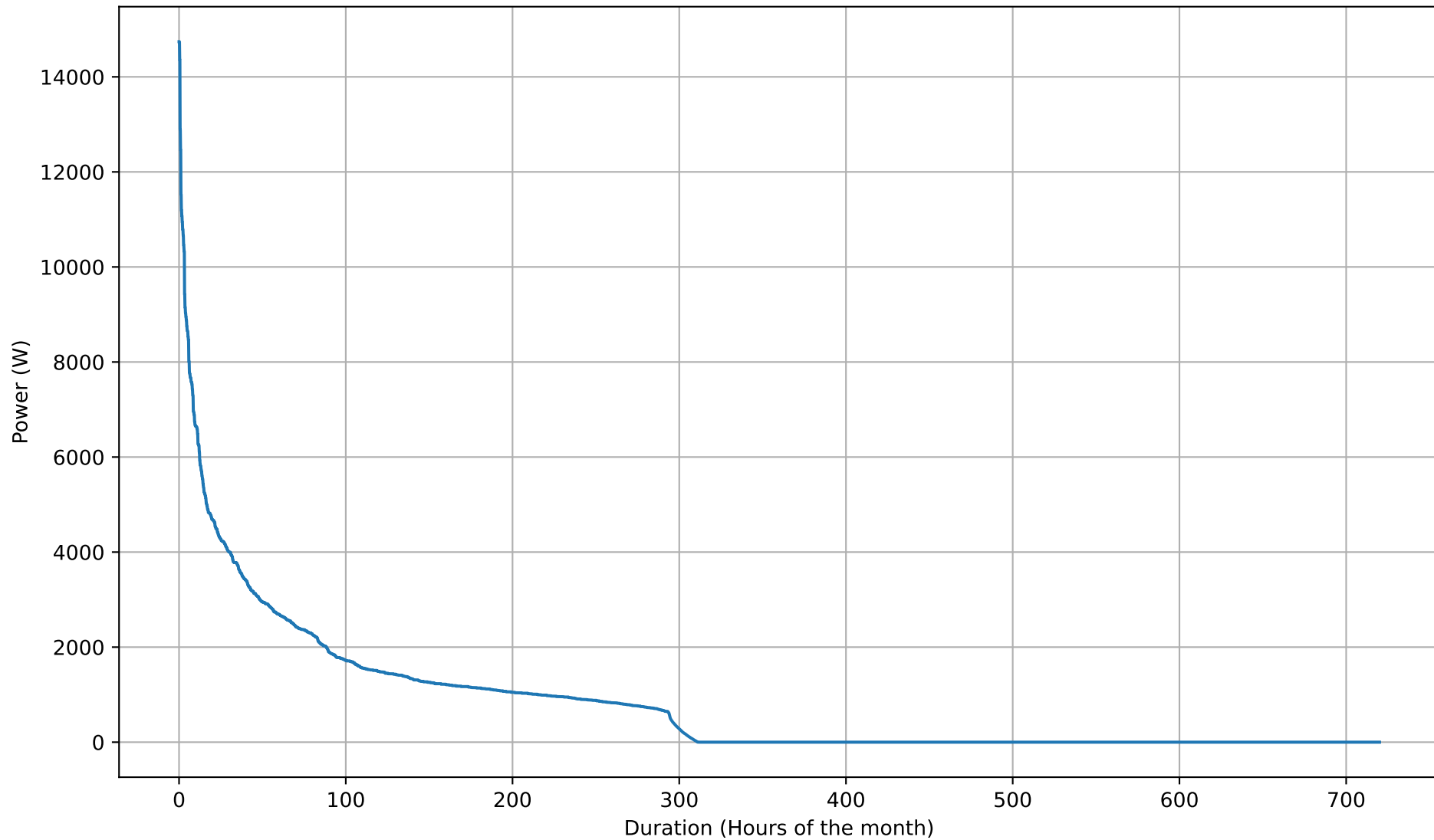
Battery Discharging Power Duration Curve - 26kWh - Sep
