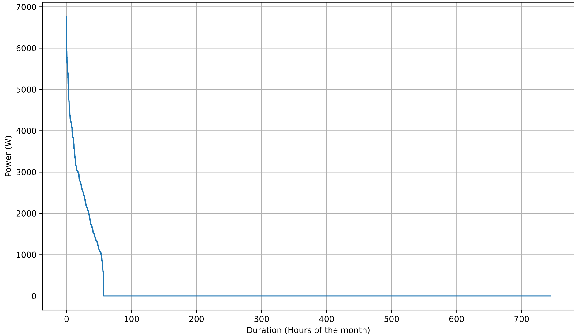
Battery Discharging Power Duration Curve - 26kWh - Jan
