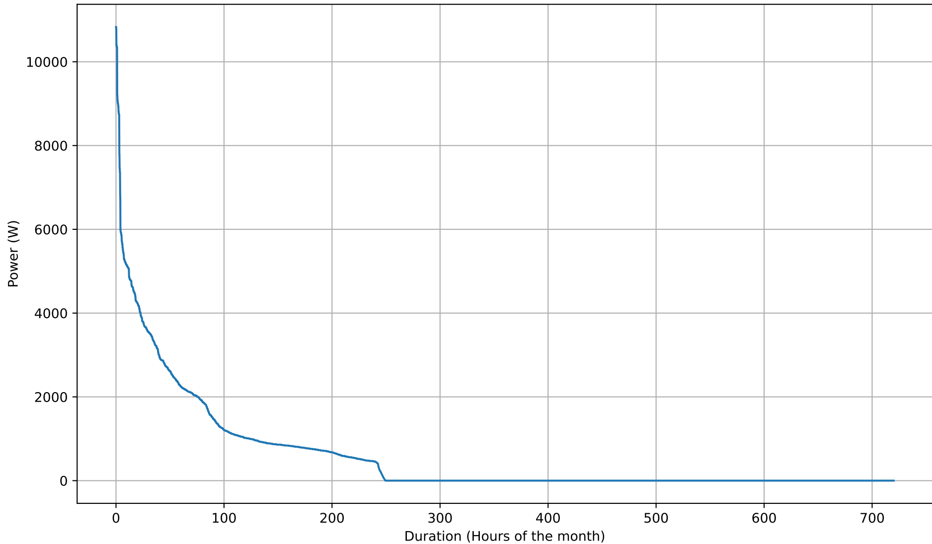
Battery Discharging Power Duration Curve - 26kWh - Jun
