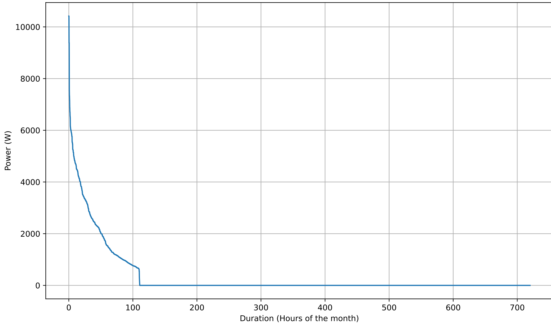
Battery Discharging Power Duration Curve - 26kWh - Nov
