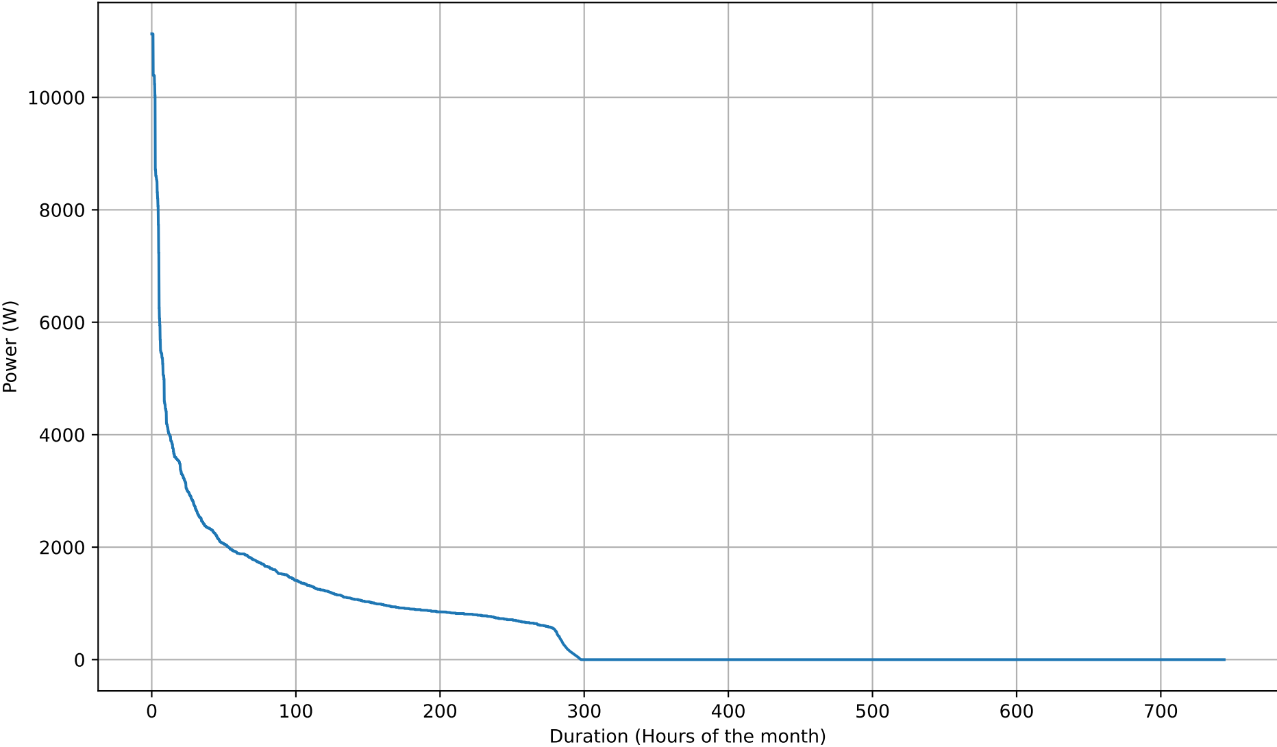
Battery Discharging Power Duration Curve - 26kWh - Jul
