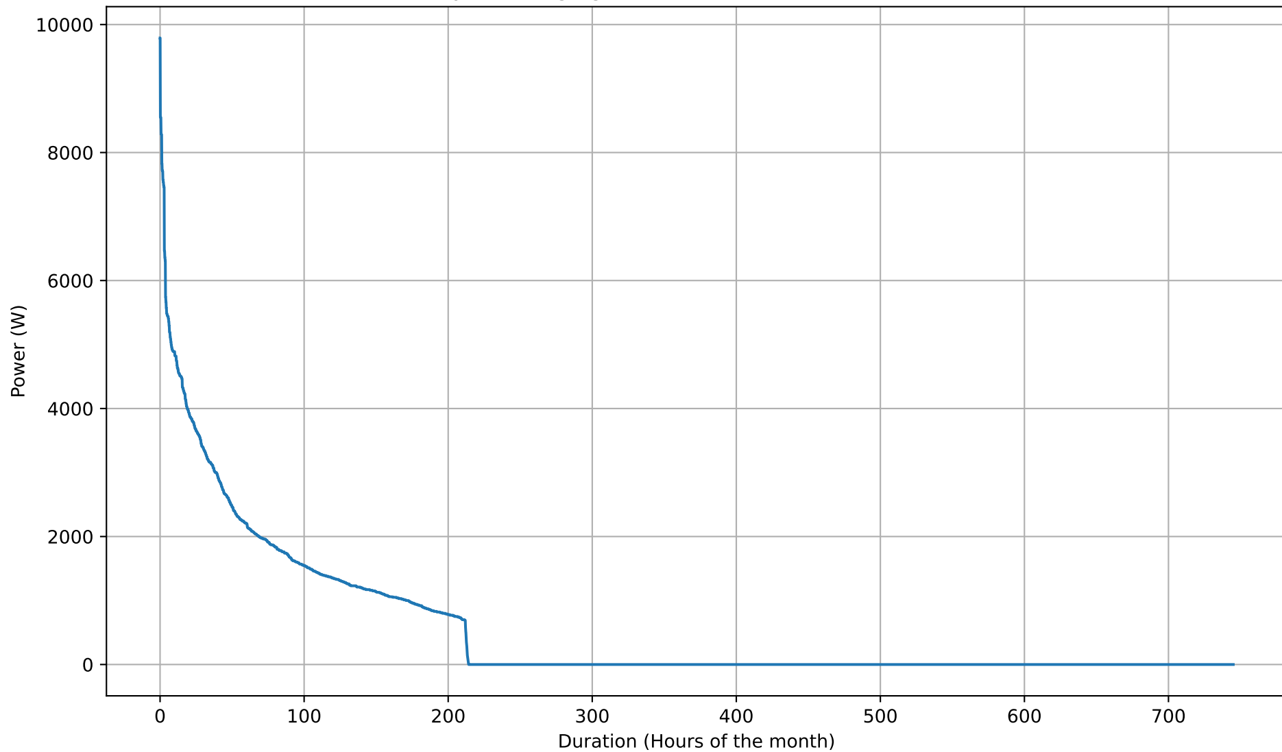
Battery Discharging Power Duration Curve - 26kWh - Oct
