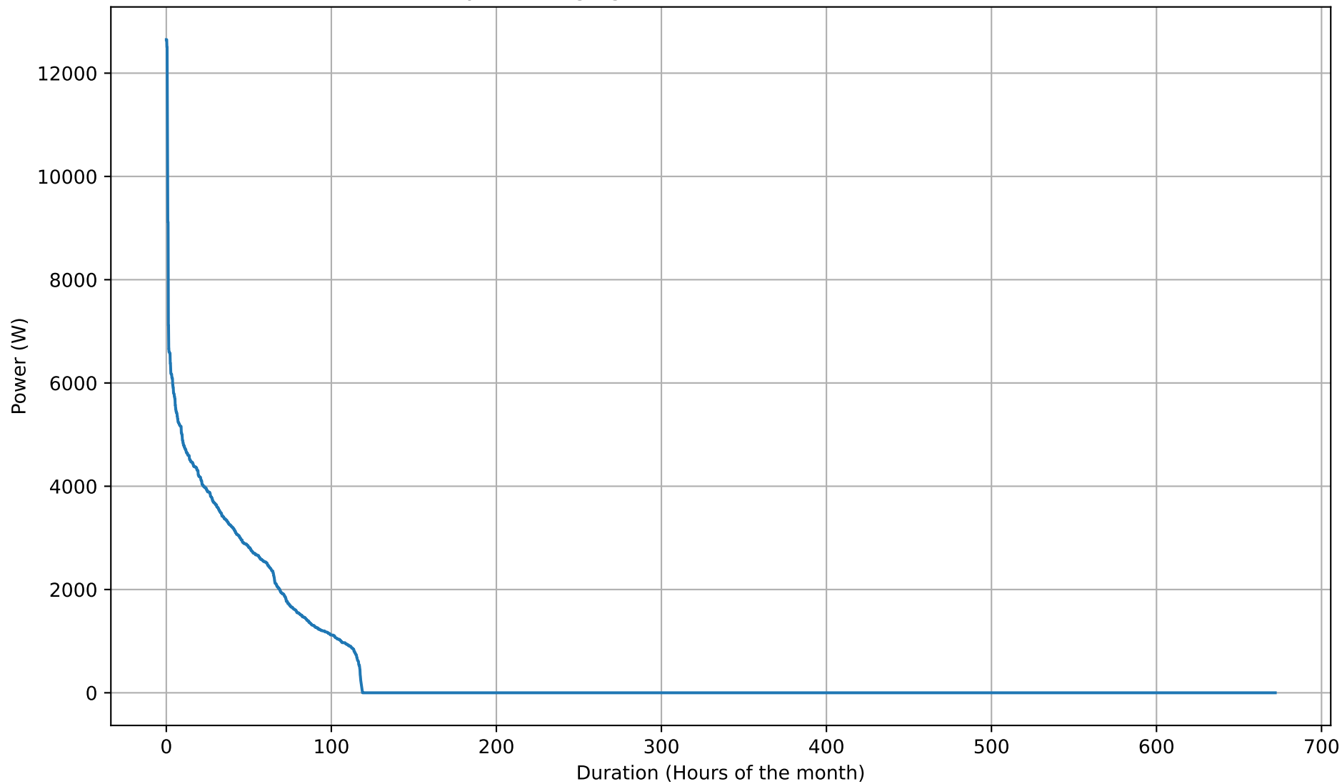
Battery Discharging Power Duration Curve - 26kWh - Feb
