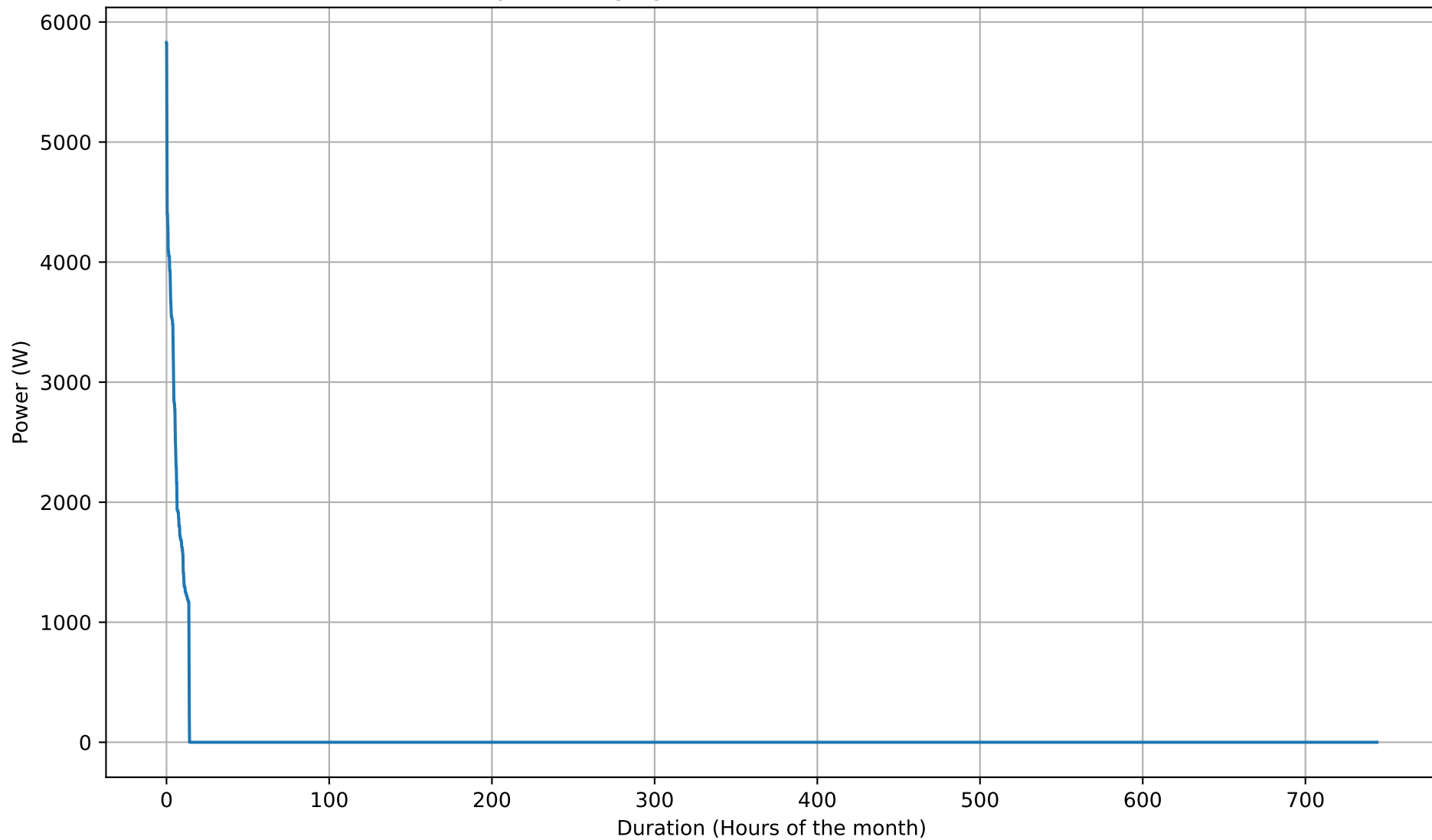
Battery Discharging Power Duration Curve - 26kWh - Dec
