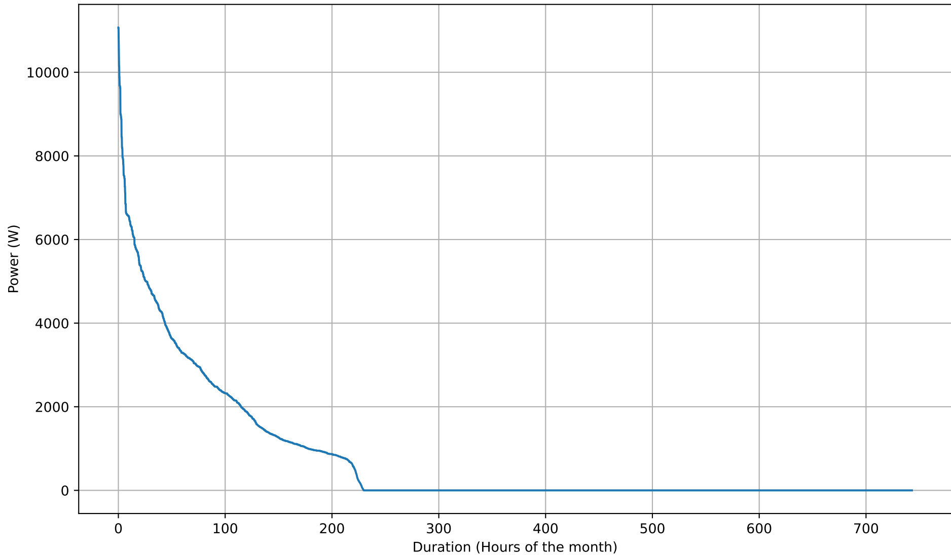
Battery Discharging Power Duration Curve - 26kWh - Mar
