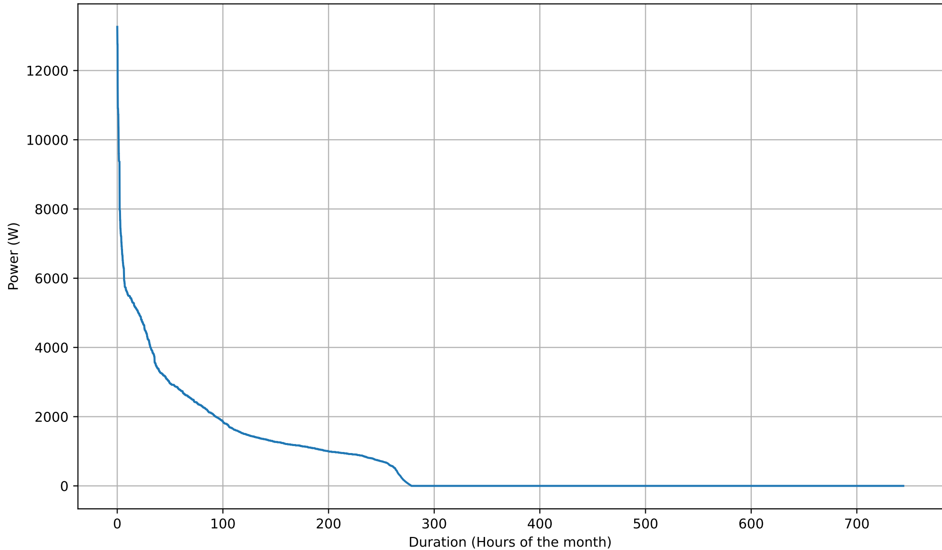
Battery Discharging Power Duration Curve - 26kWh - May
