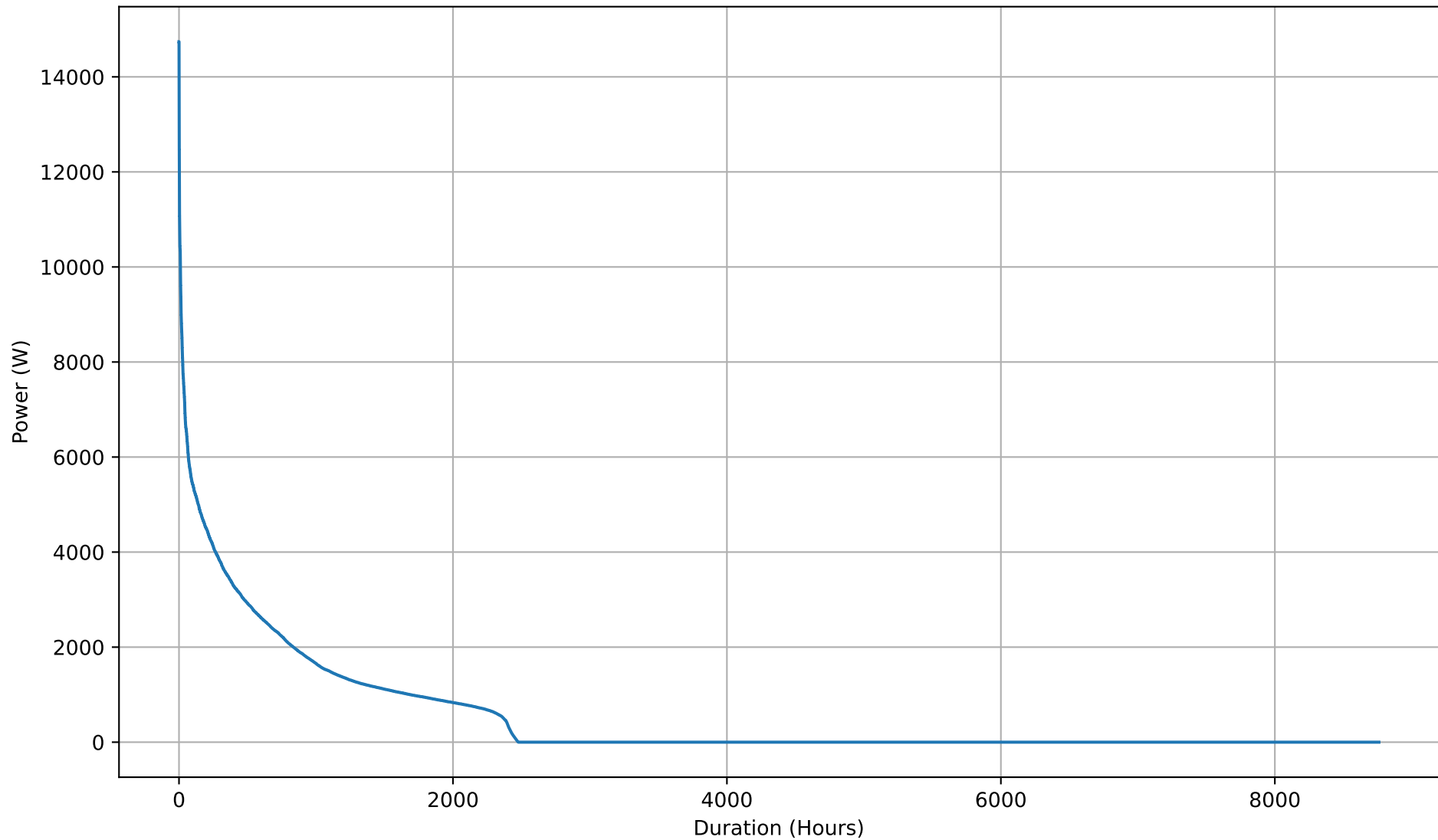
Yearly Battery Discharging Power Duration Curve - 26kWh
