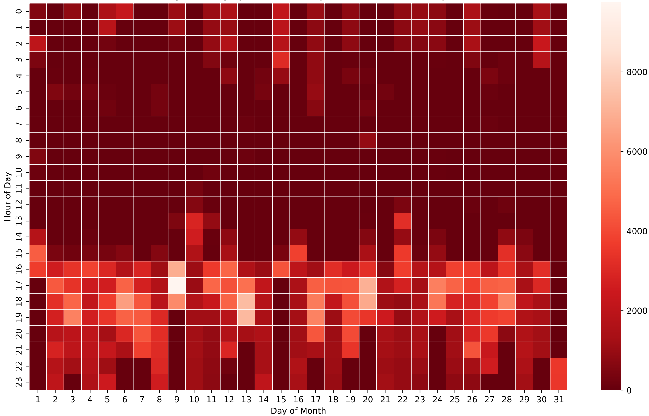
Battery Discharging Power Heatmap (Wh/Hour) - 26kWh - Apr
