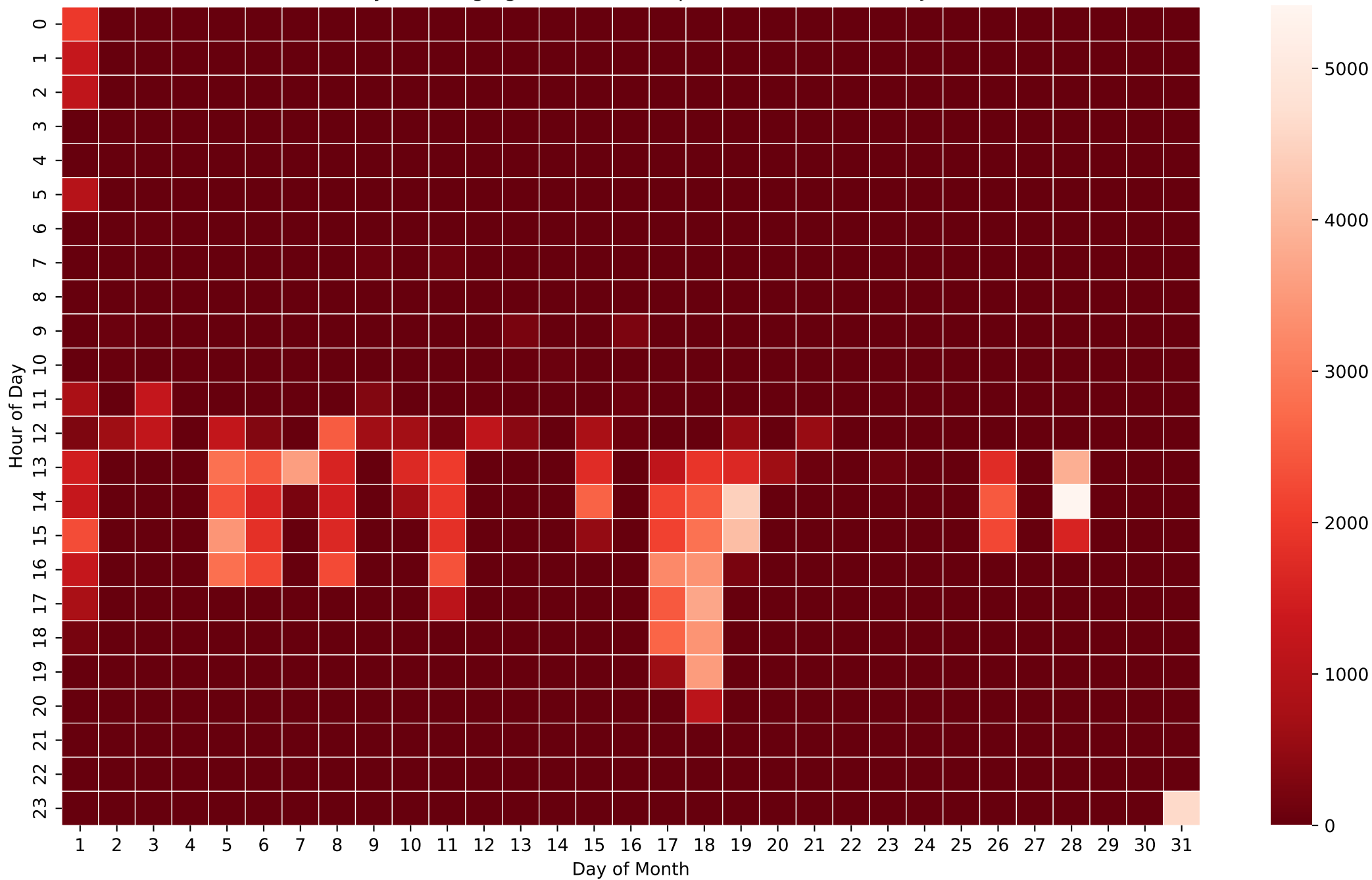
Battery Discharging Power Heatmap (Wh/Hour) - 26kWh - Jan
