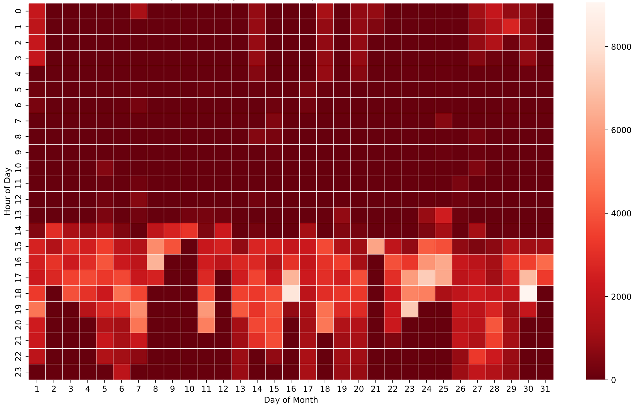
Battery Discharging Power Heatmap (Wh/Hour) - 26kWh - Mar
