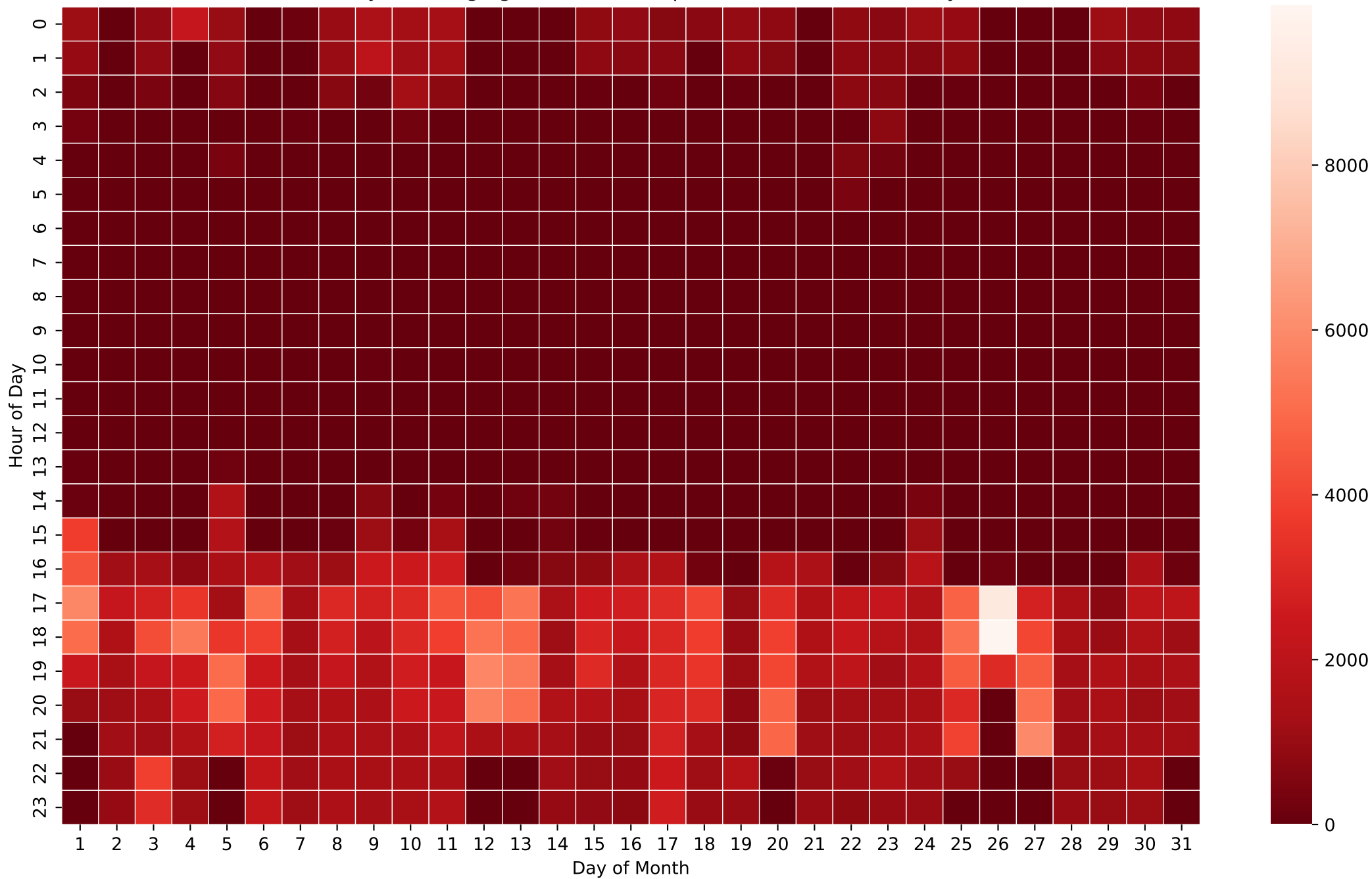
Battery Discharging Power Heatmap (Wh/Hour) - 26kWh - May
