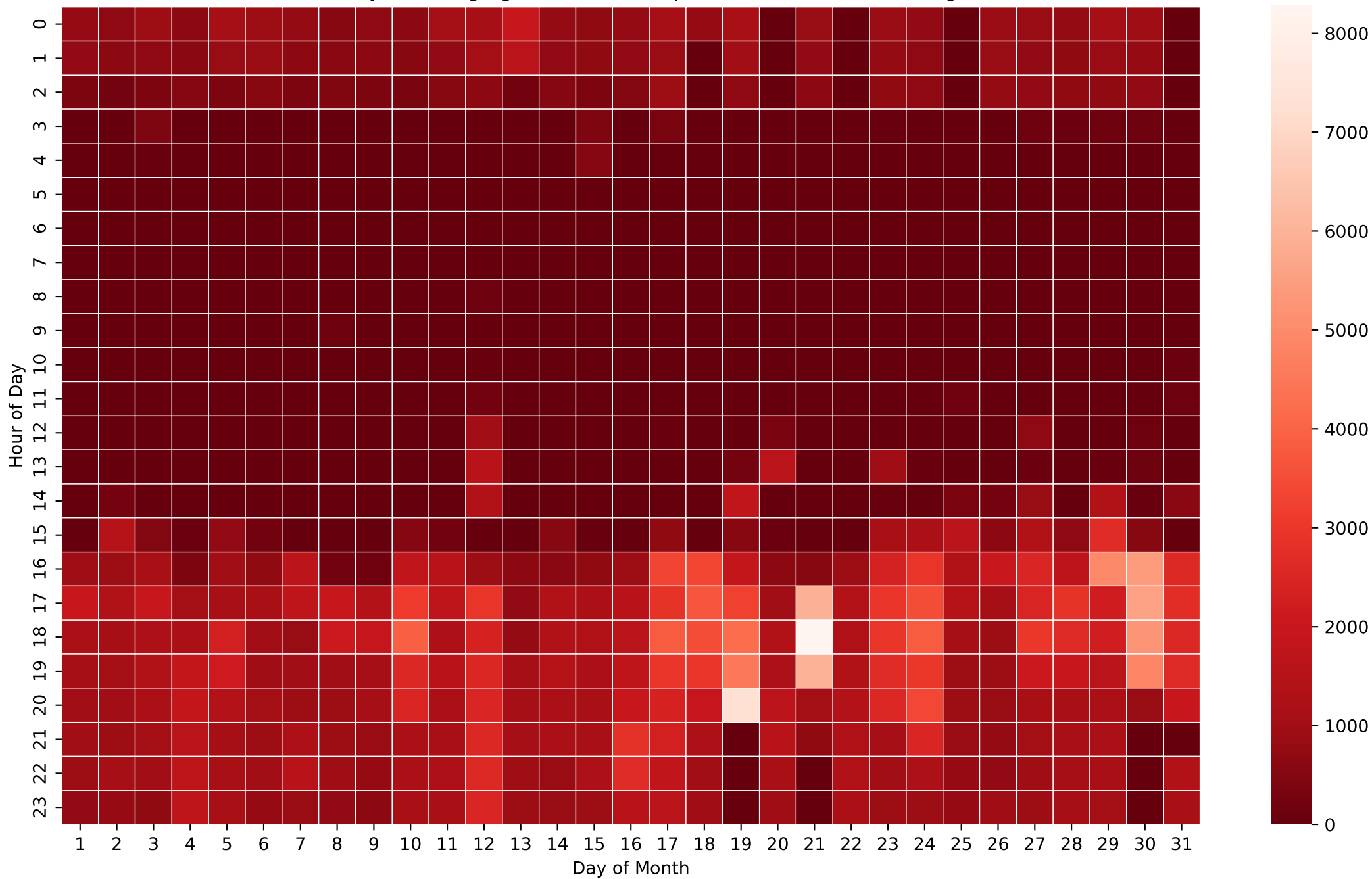
Battery Discharging Power Heatmap (Wh/Hour) - 26kWh - Aug
