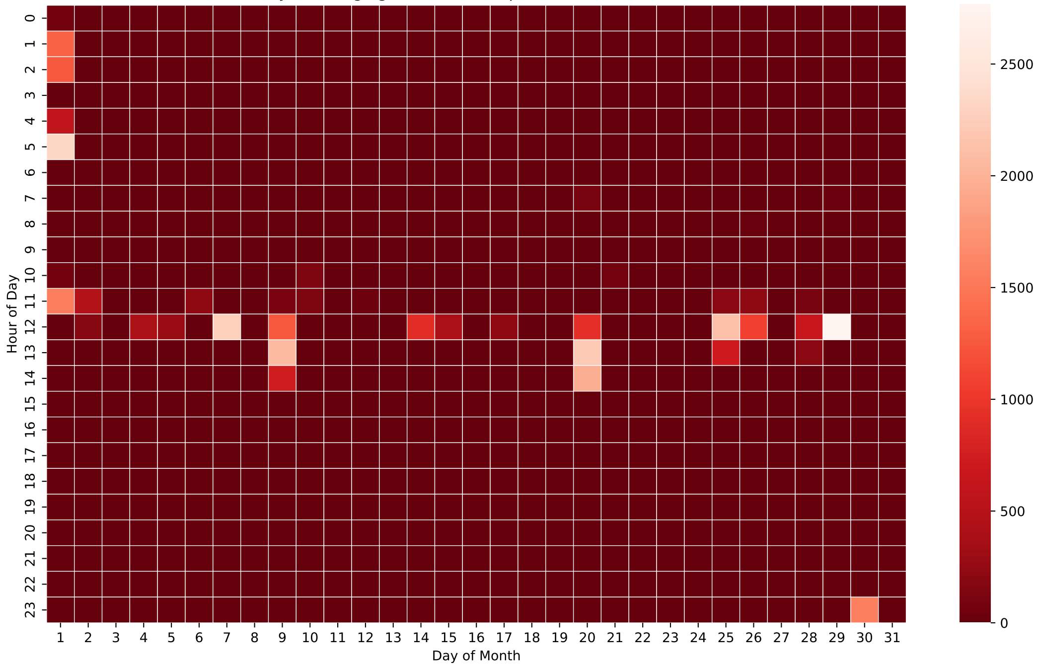
Battery Discharging Power Heatmap (Wh/Hour) - 26kWh - Dec
