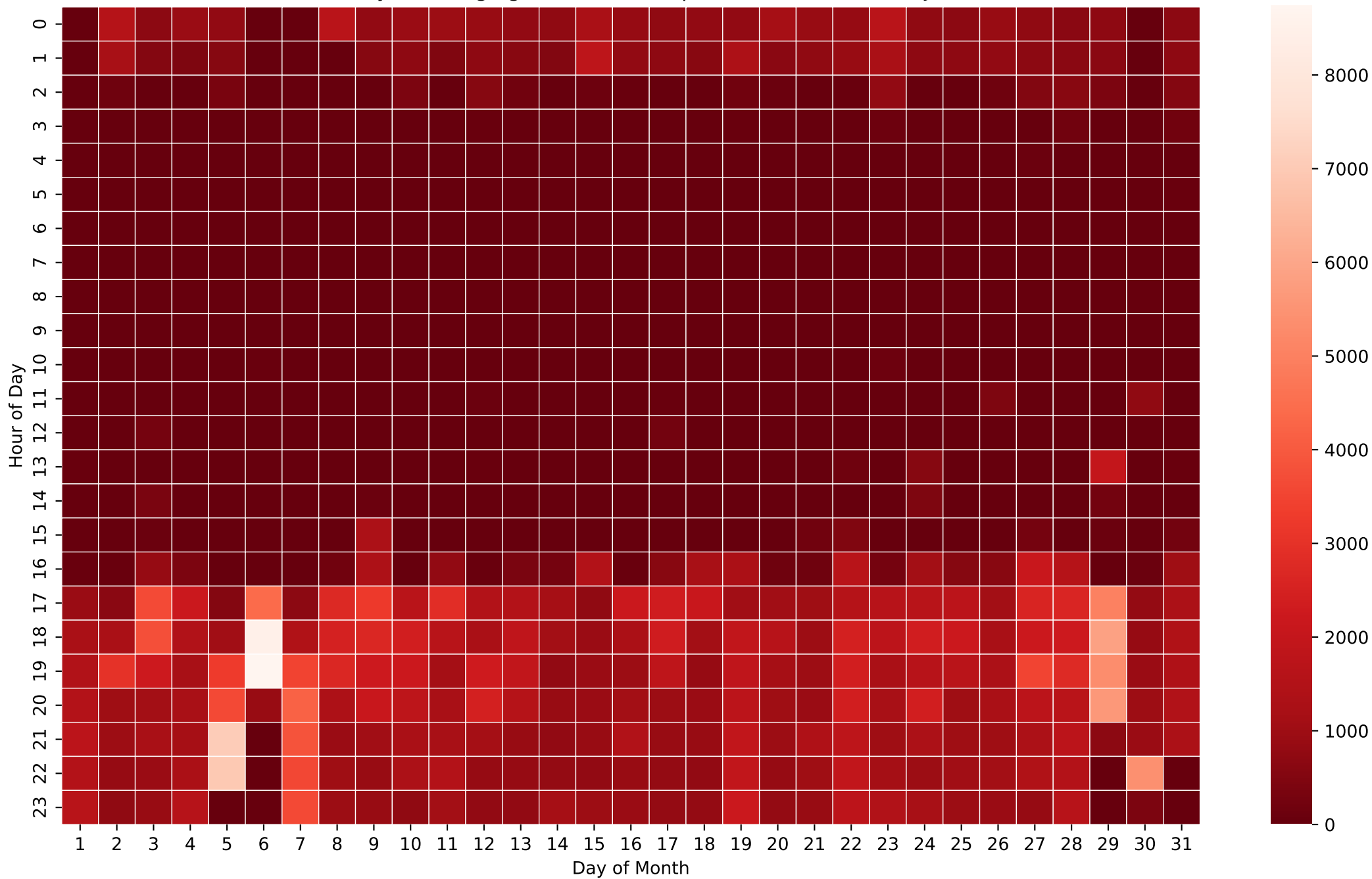
Battery Discharging Power Heatmap (Wh/Hour) - 26kWh - Jul
