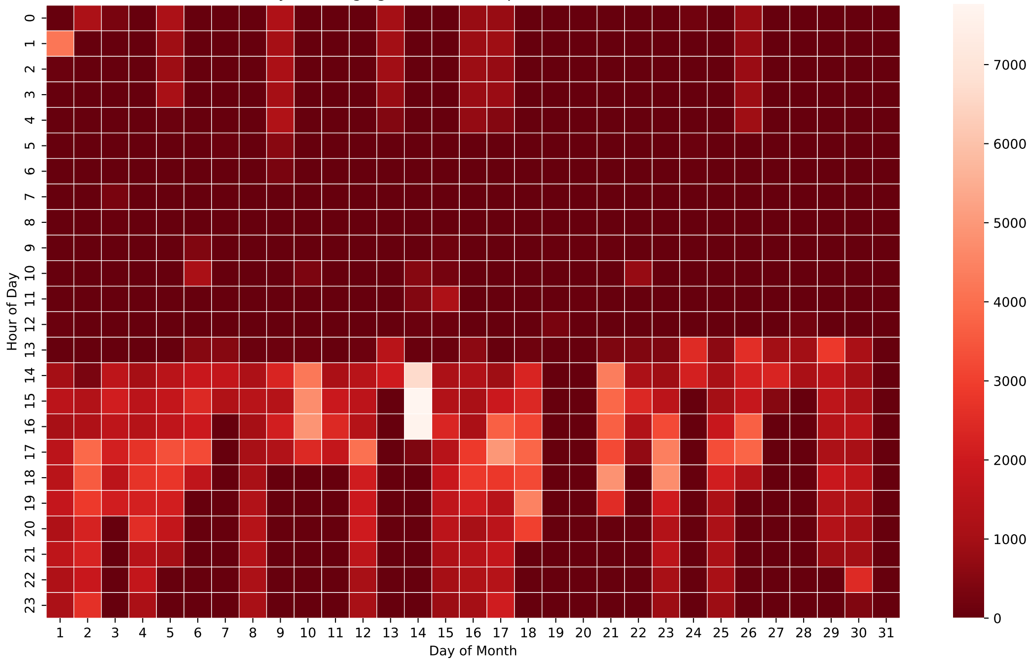
Battery Discharging Power Heatmap (Wh/Hour) - 26kWh - Oct
