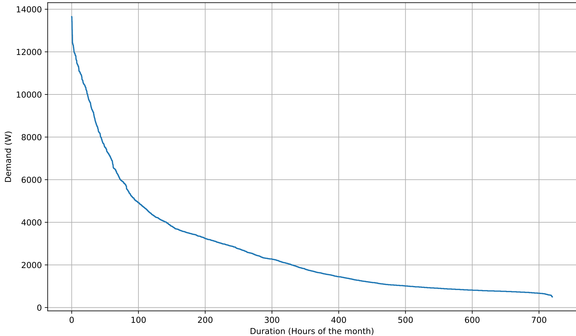
Electricity Demand Duration Curve - 26kWh - Nov
