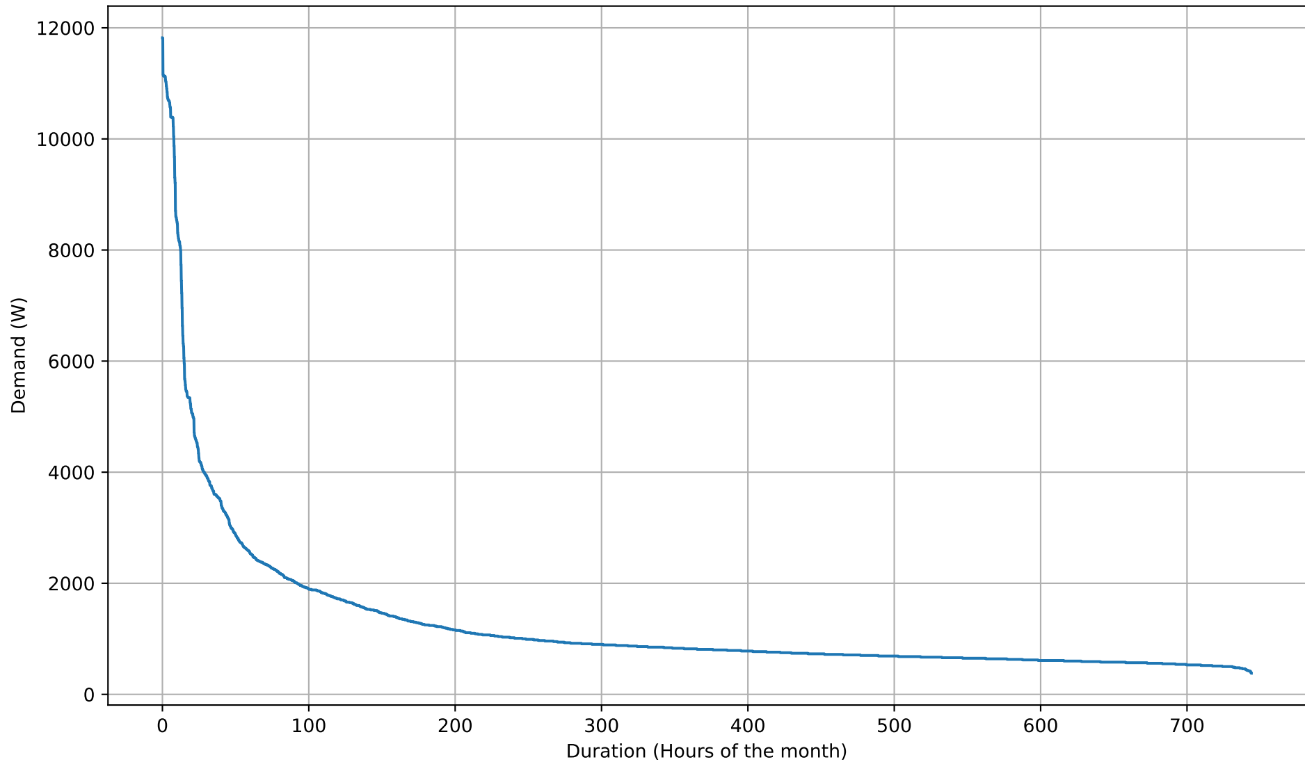
Electricity Demand Duration Curve - 26kWh - Jul
