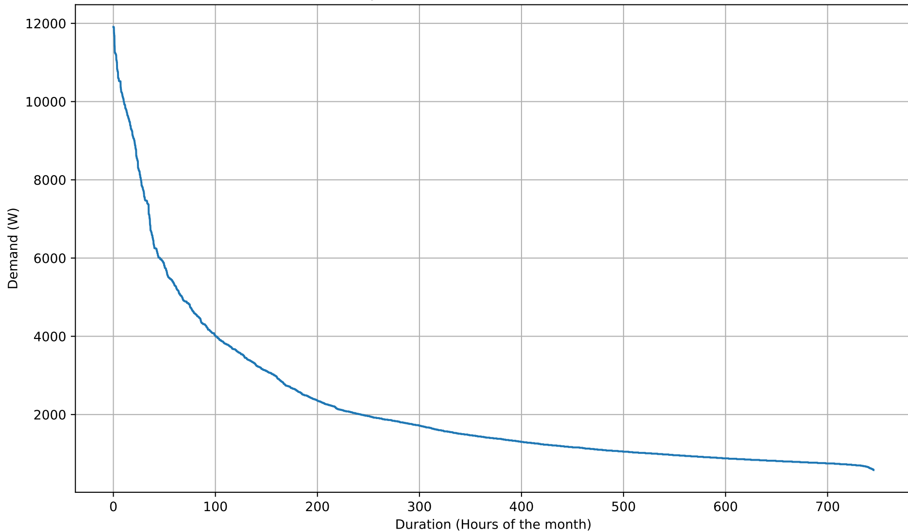
Electricity Demand Duration Curve - 26kWh - Oct
