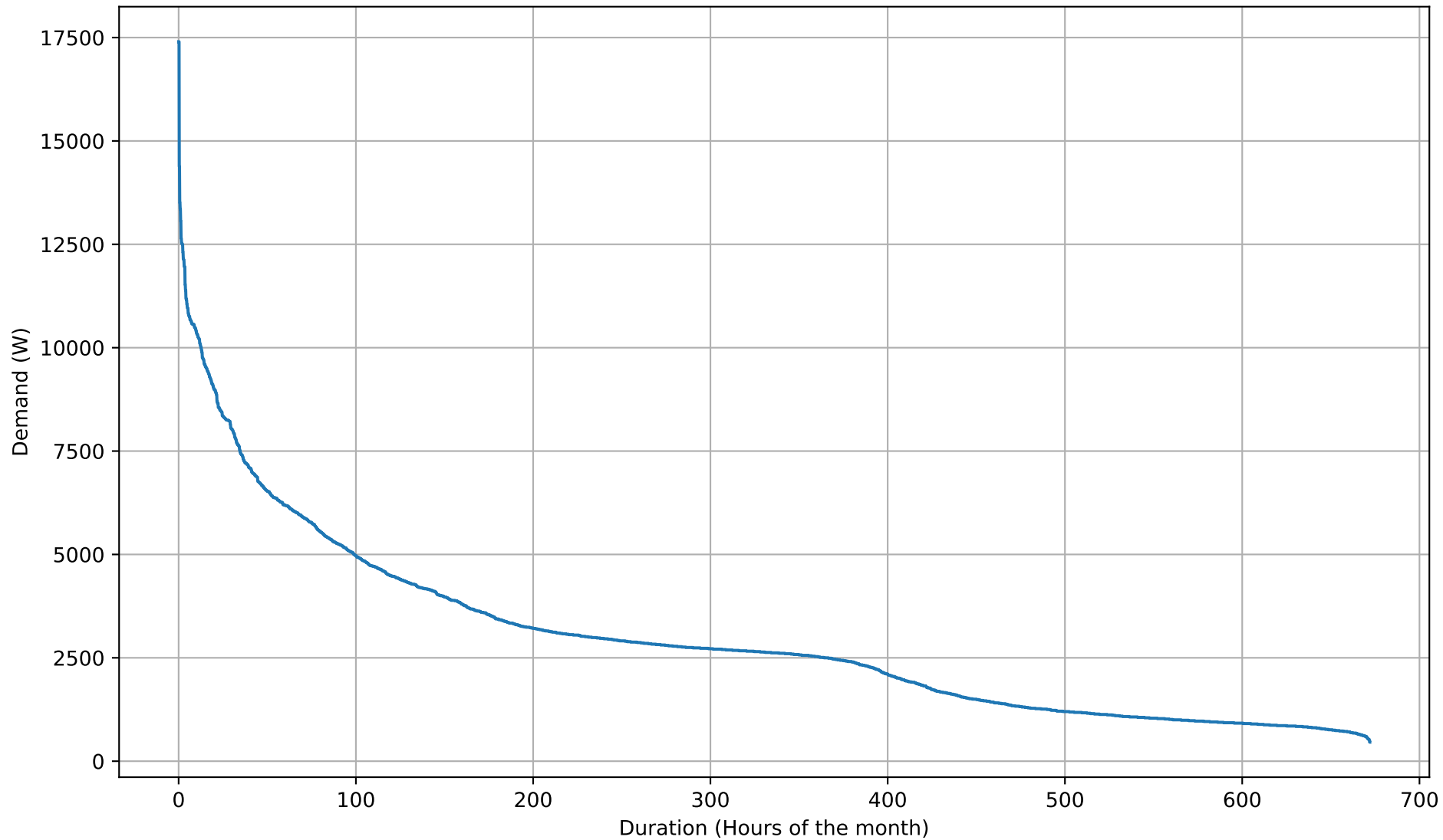
Electricity Demand Duration Curve - 26kWh - Feb
