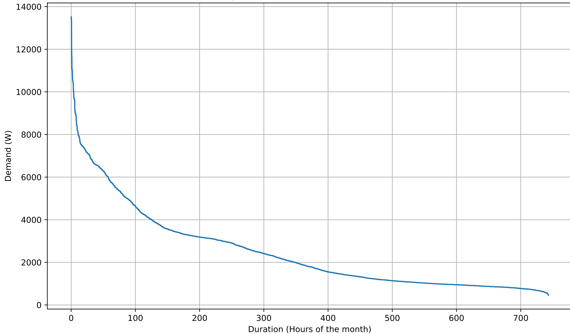
Electricity Demand Duration Curve - 26kWh - Mar
