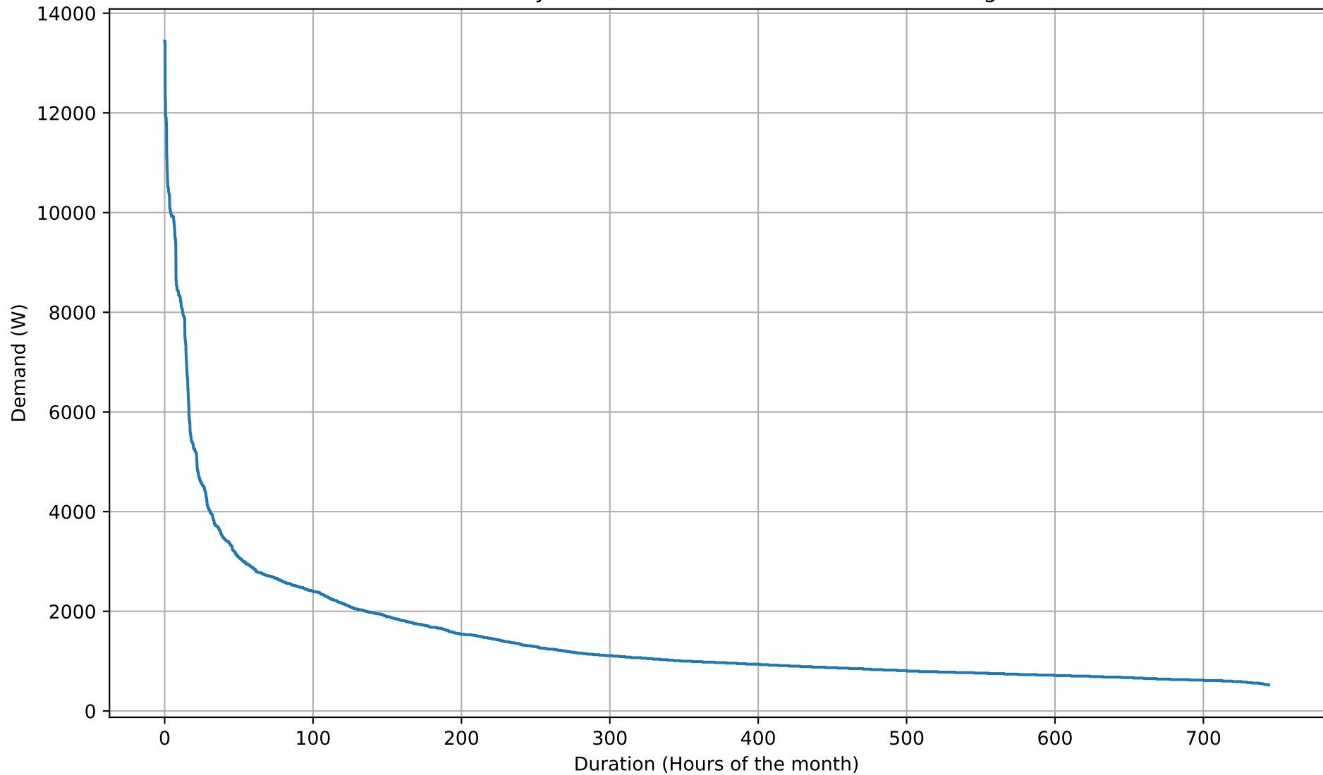
Electricity Demand Duration Curve - 26kWh - Aug
