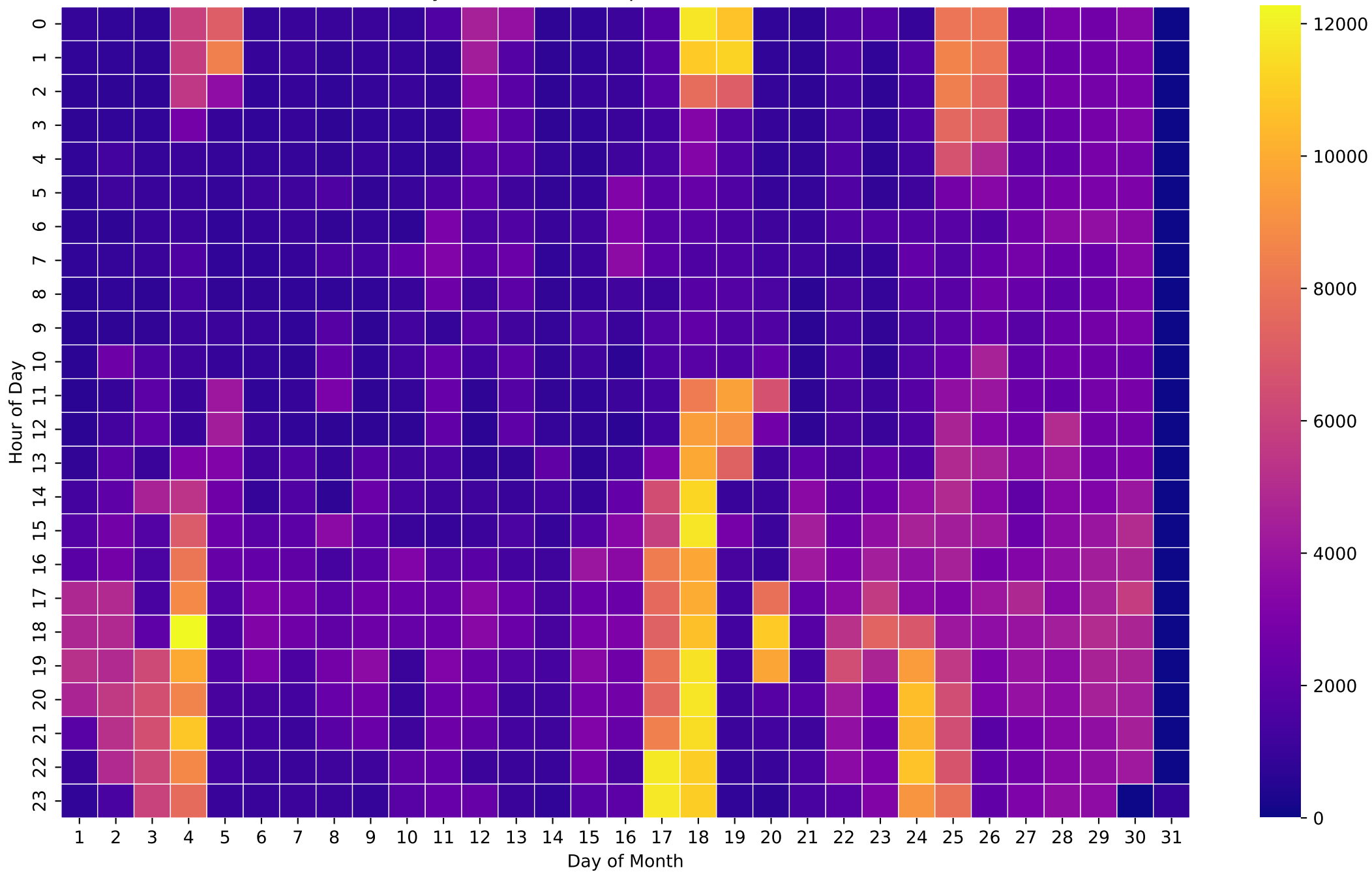
Electricity Demand Heatmap (Wh/Hour) - 26kWh - Nov
