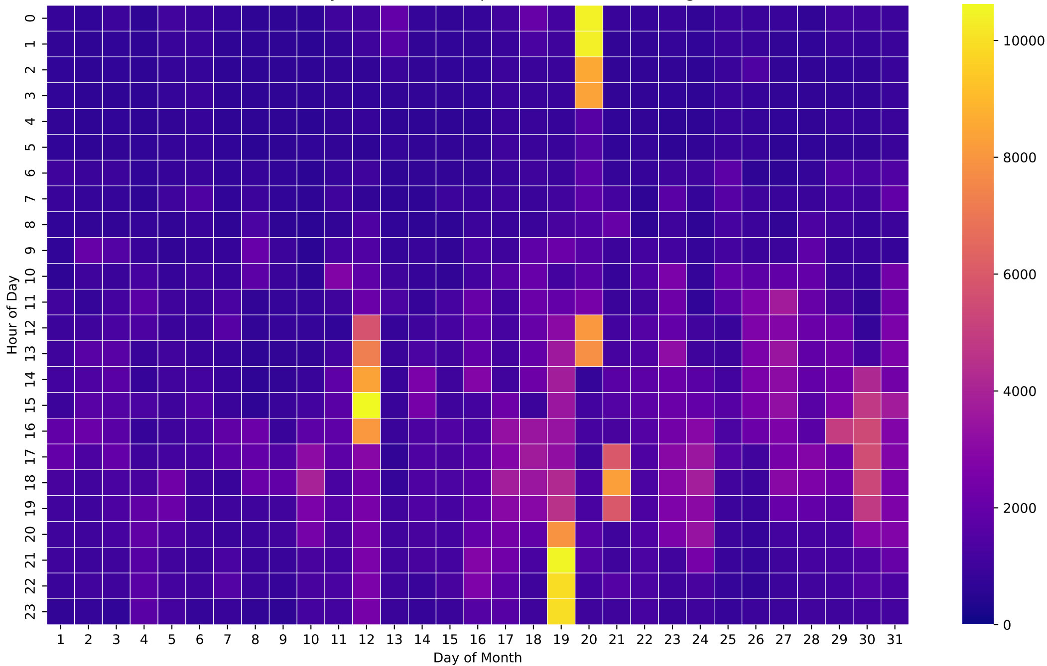
Electricity Demand Heatmap (Wh/Hour) - 26kWh - Aug
