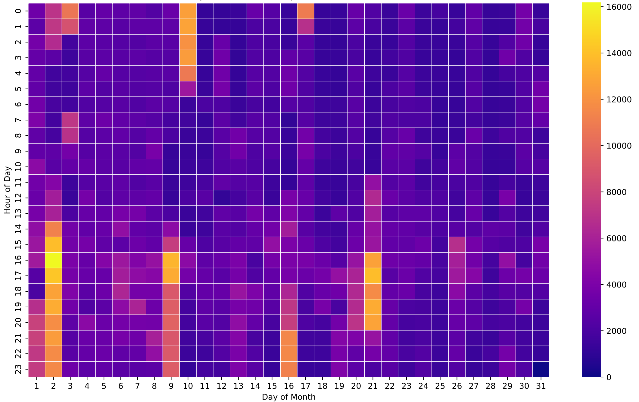
Electricity Demand Heatmap (Wh/Hour) - 26kWh - Dec
