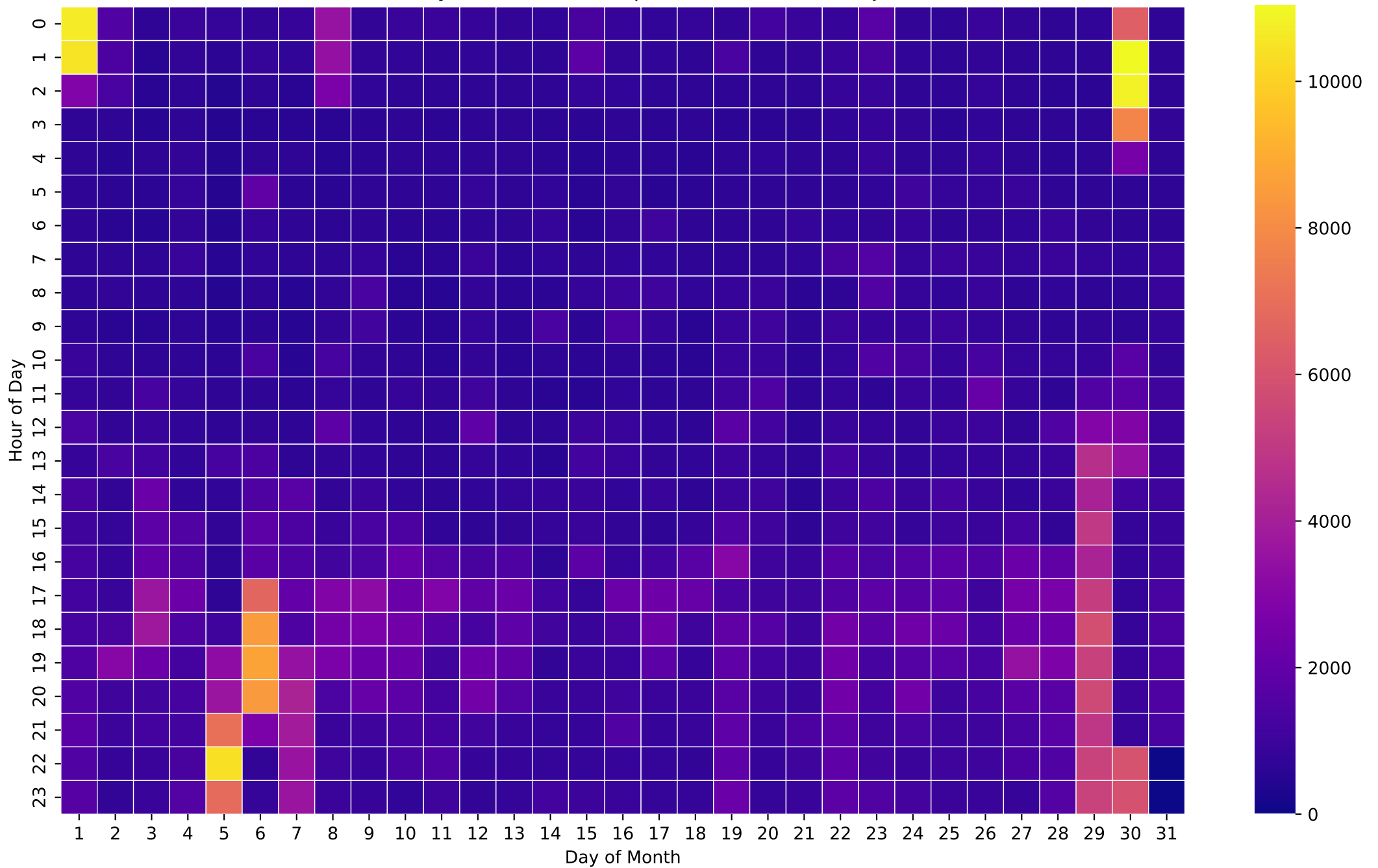
Electricity Demand Heatmap (Wh/Hour) - 26kWh - Jul
