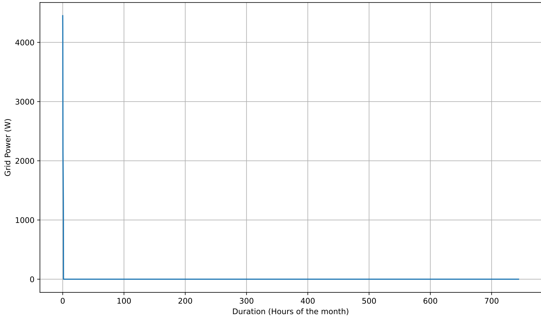
Grid Export Duration Curve - 26kWh - Jan
