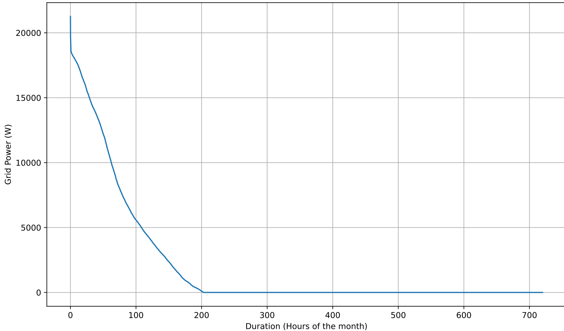
Grid Export Duration Curve - 26kWh - Sep
