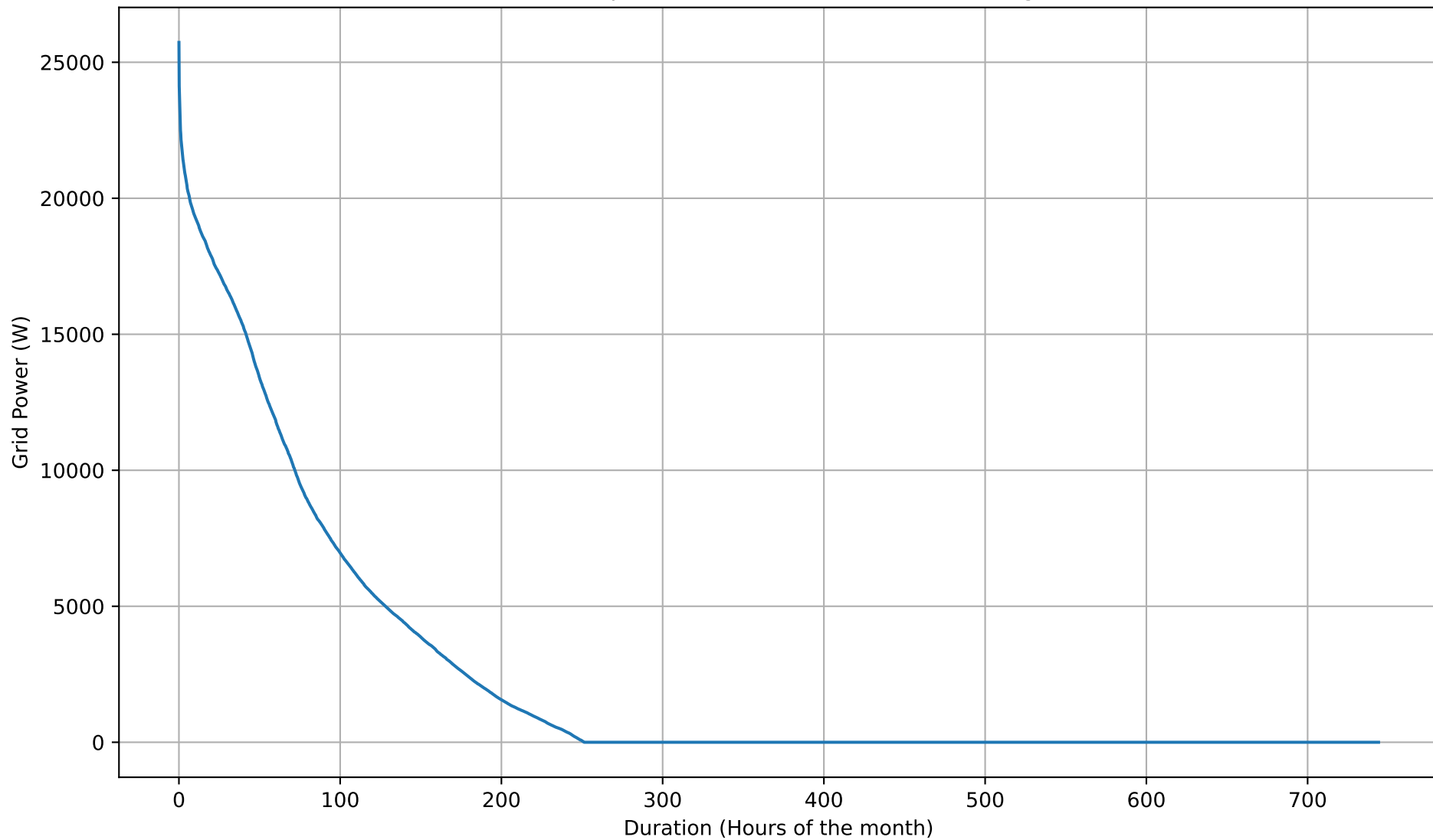
Grid Export Duration Curve - 26kWh - Aug
