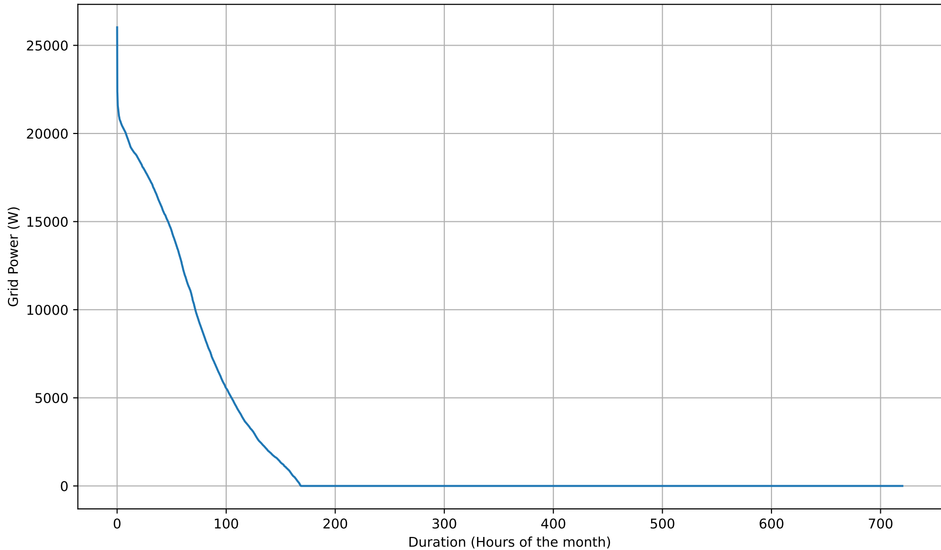
Grid Export Duration Curve - 26kWh - Apr
