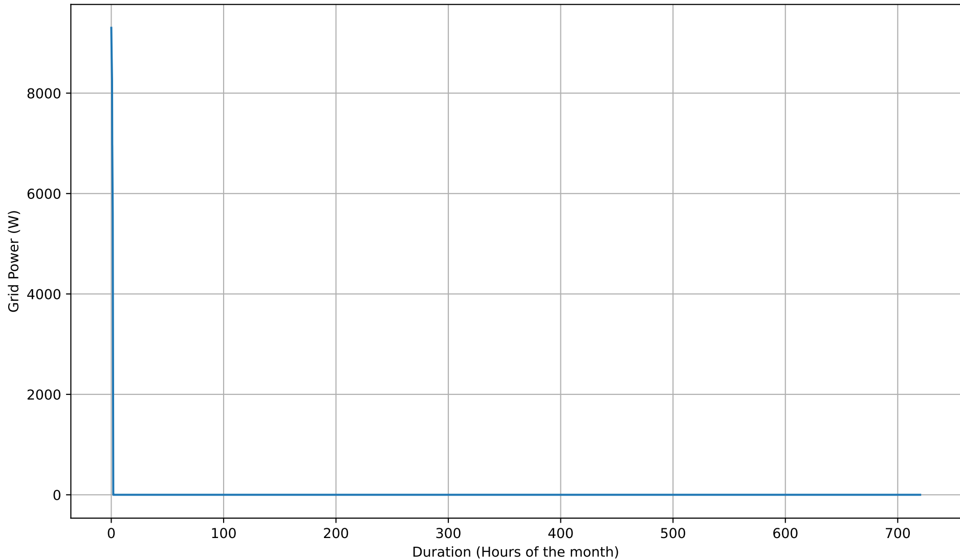
Grid Export Duration Curve - 26kWh - Nov
