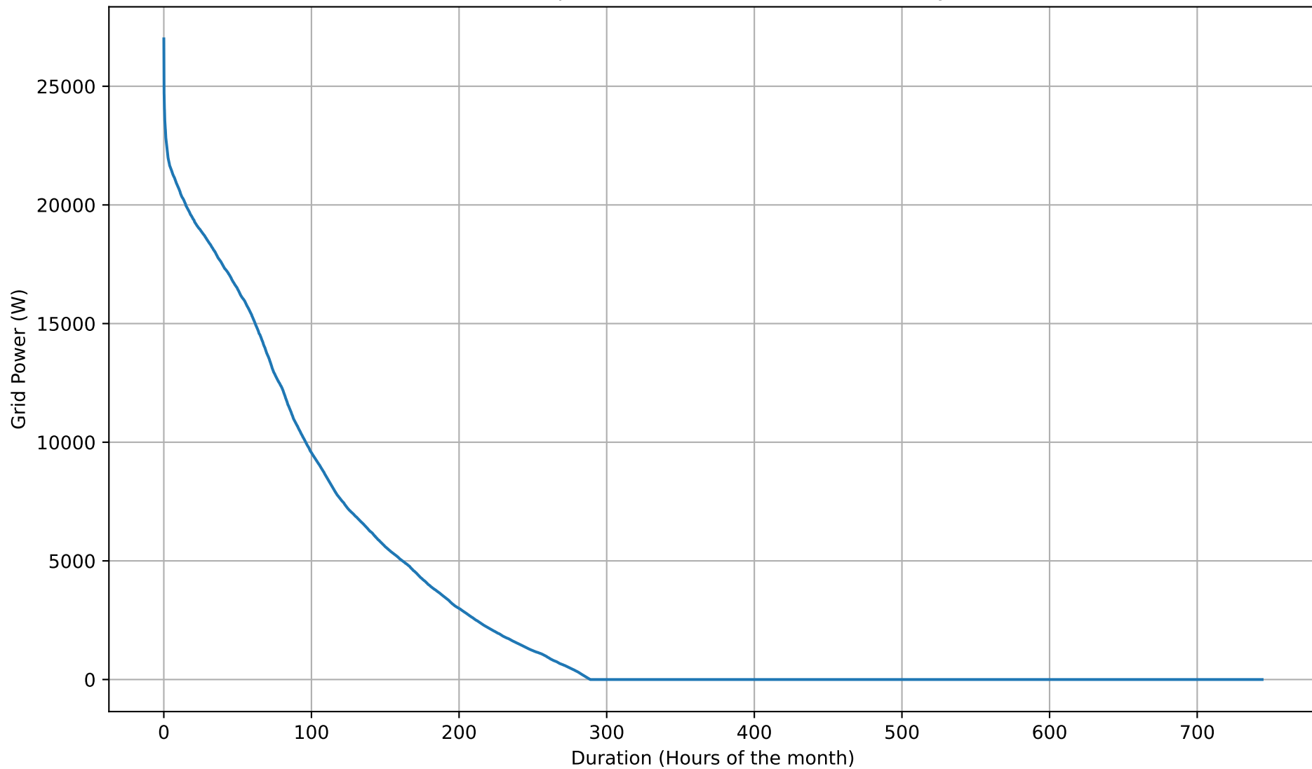
Grid Export Duration Curve - 26kWh - May
