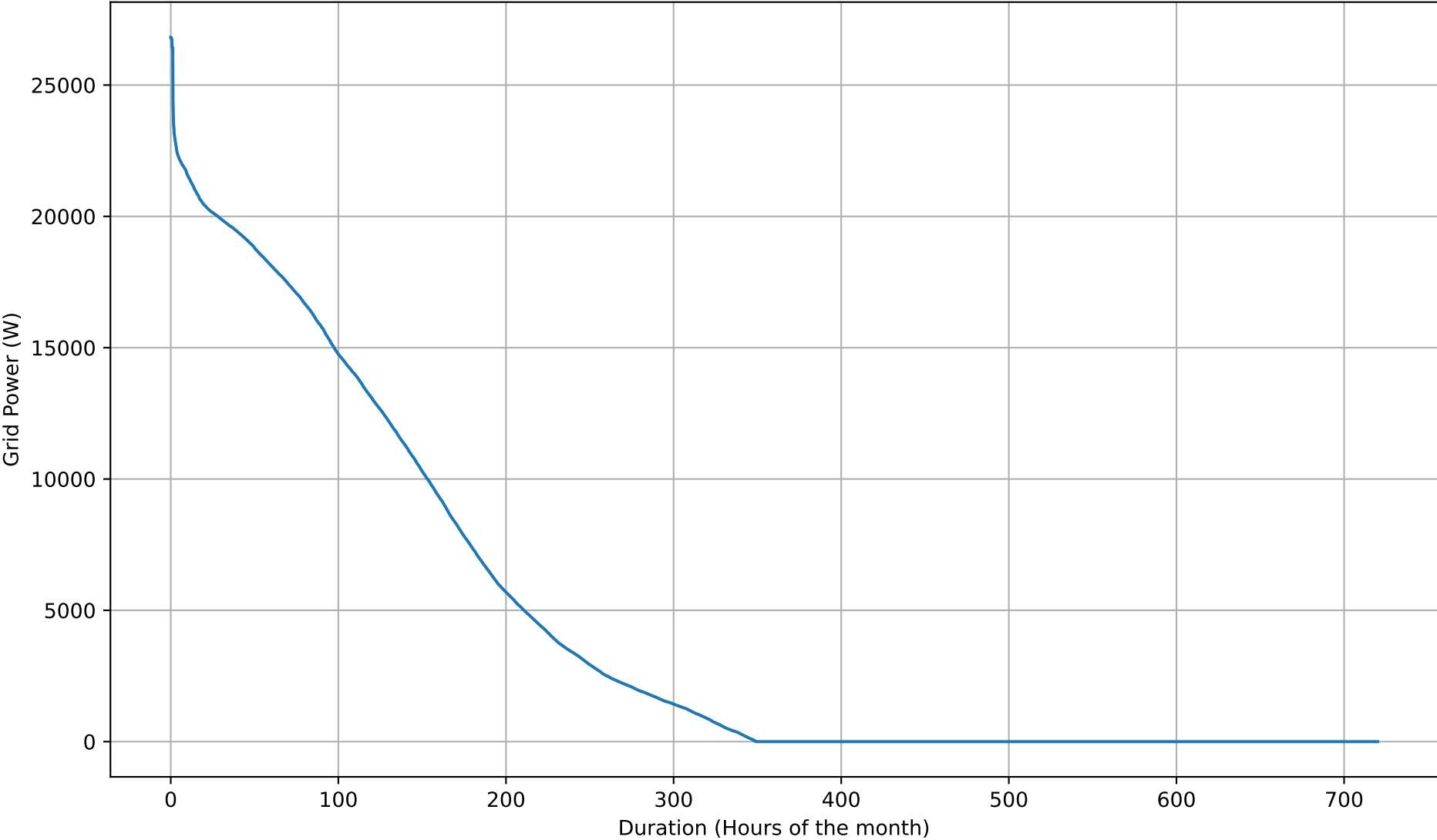
Grid Export Duration Curve - 26kWh - Jun
