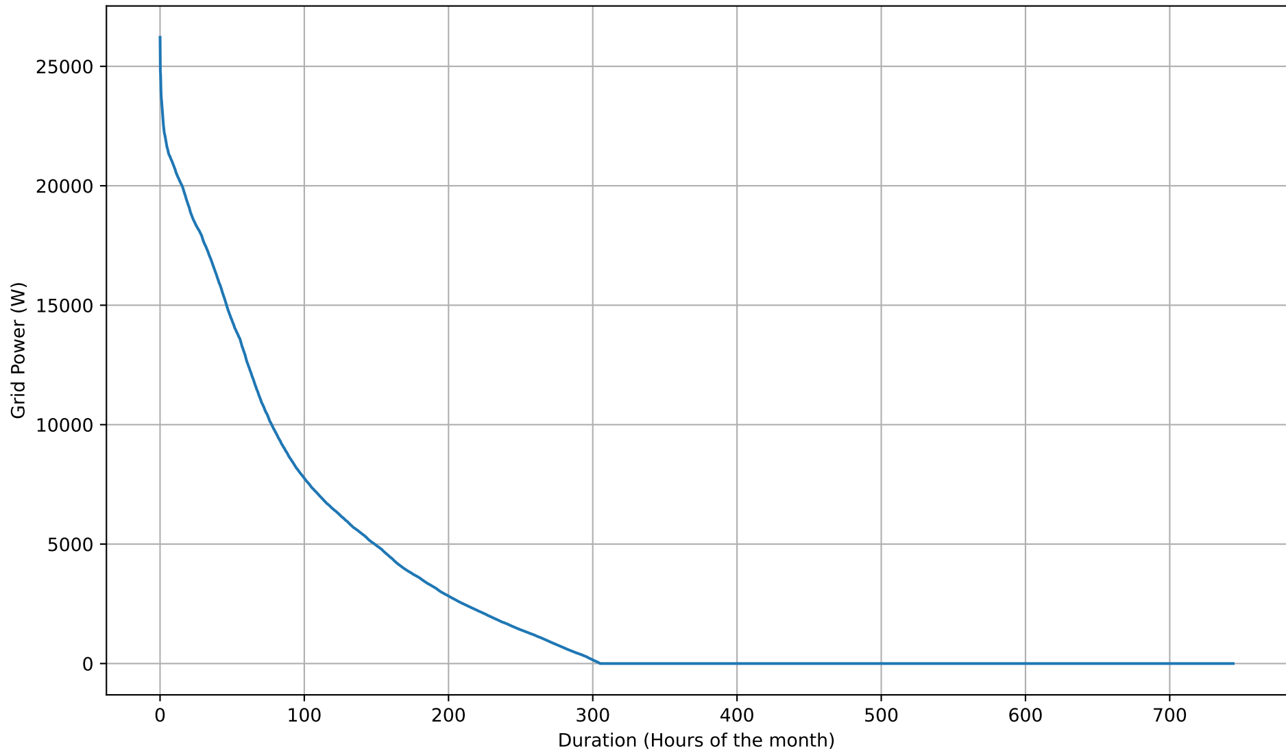
Grid Export Duration Curve - 26kWh - Jul
