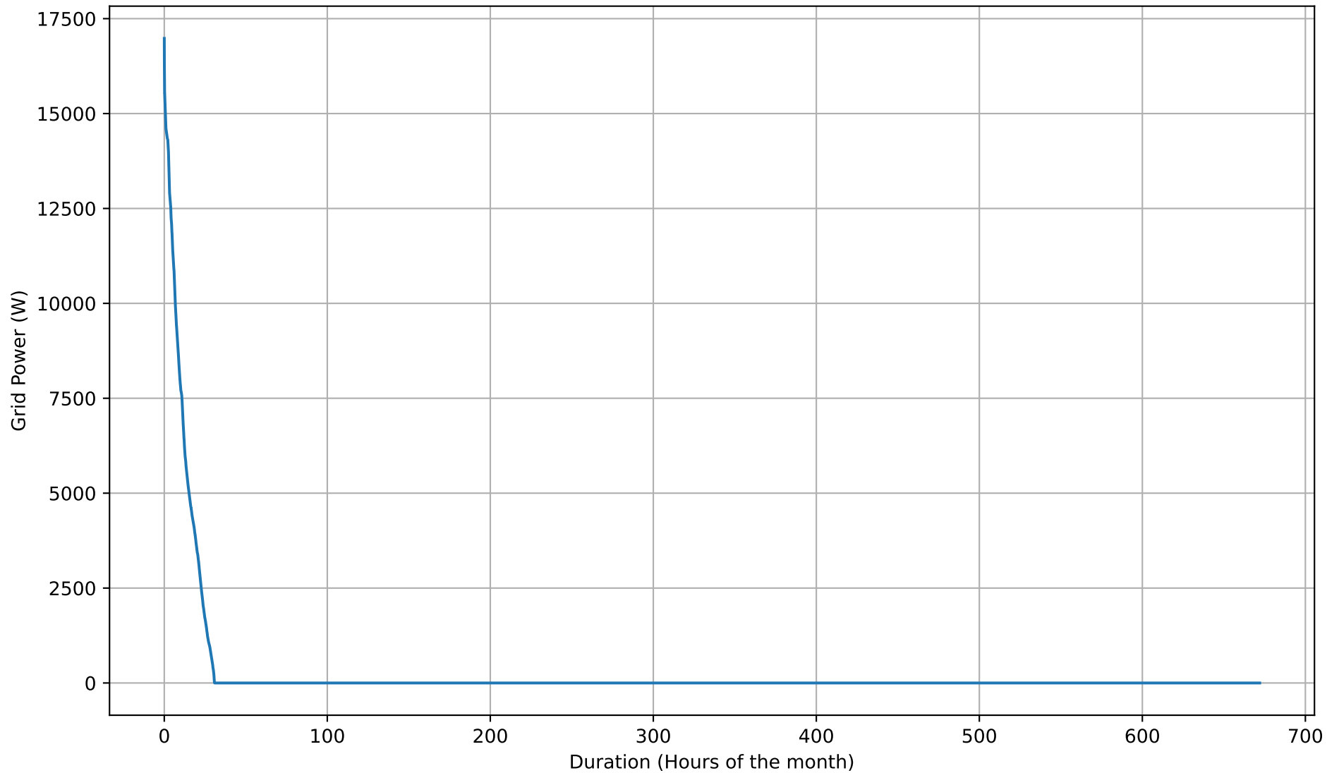
Grid Export Duration Curve - 26kWh - Feb
