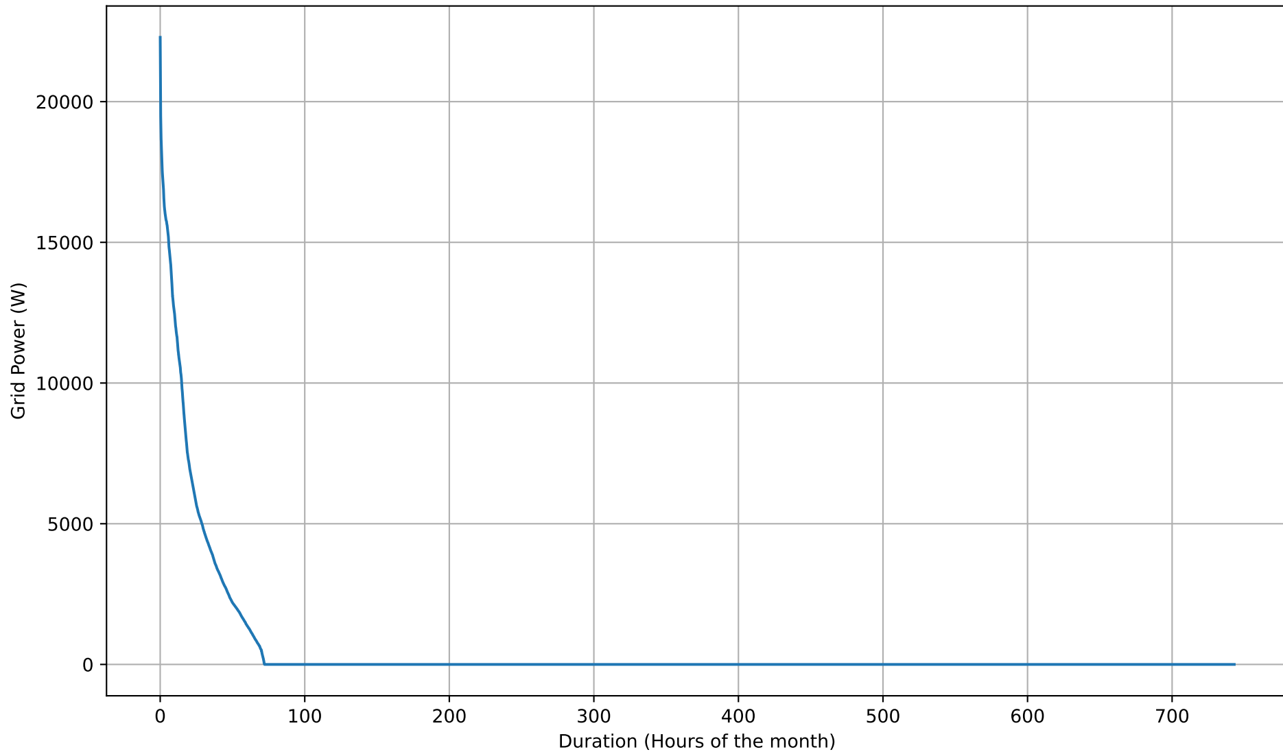
Grid Export Duration Curve - 26kWh - Mar
