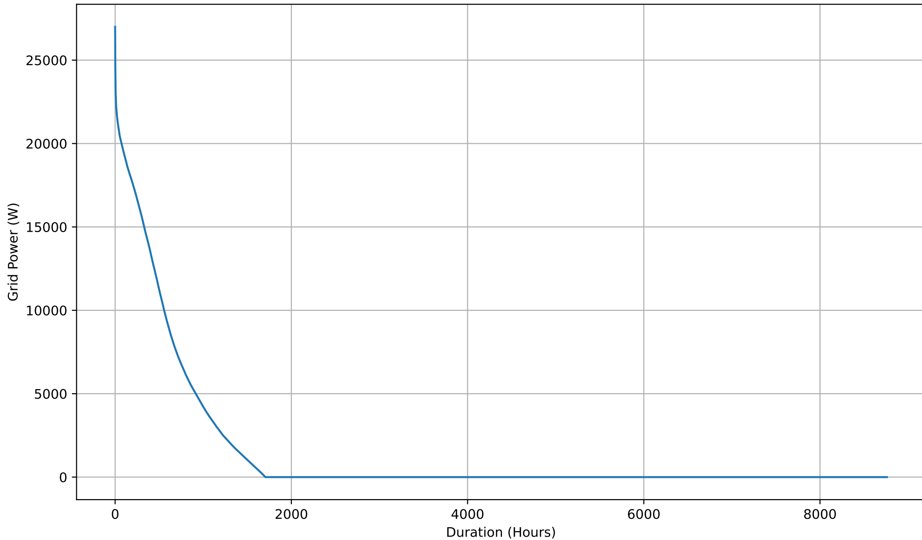
Yearly Grid Export Duration Curve - 26kWh
