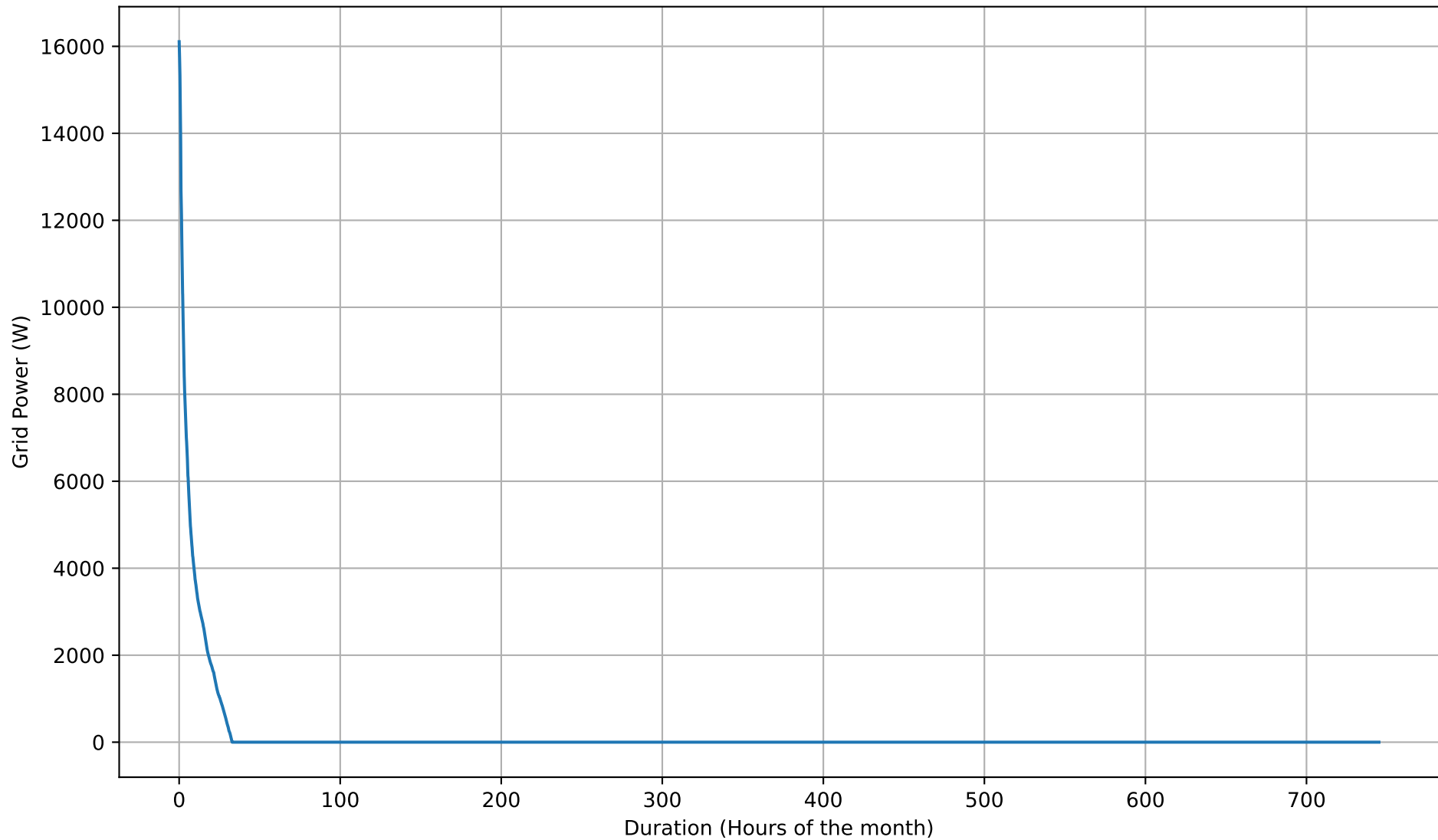
Grid Export Duration Curve - 26kWh - Oct
