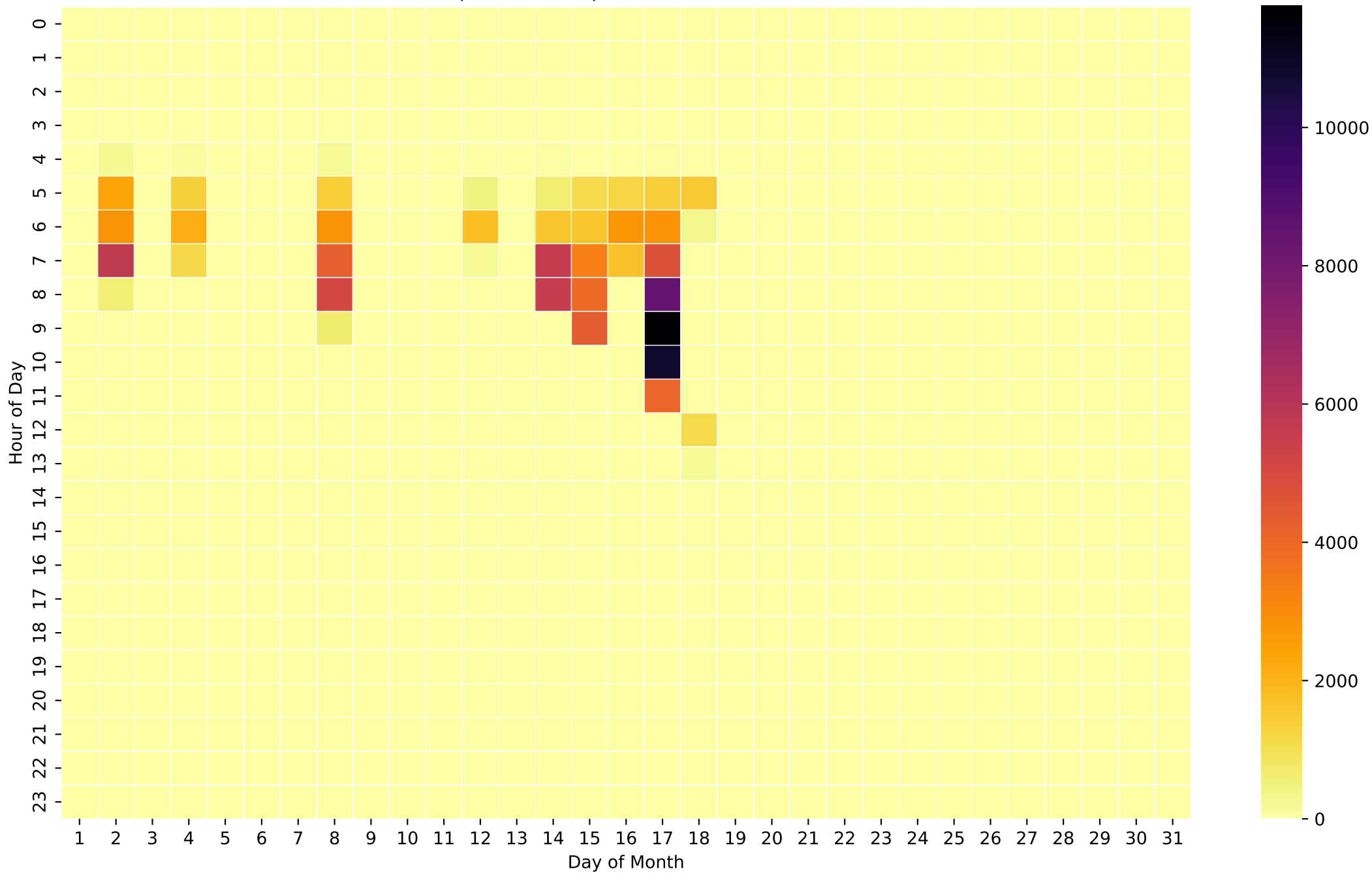
Grid Export Heatmap (Wh/Hour) - 26kWh - Oct
