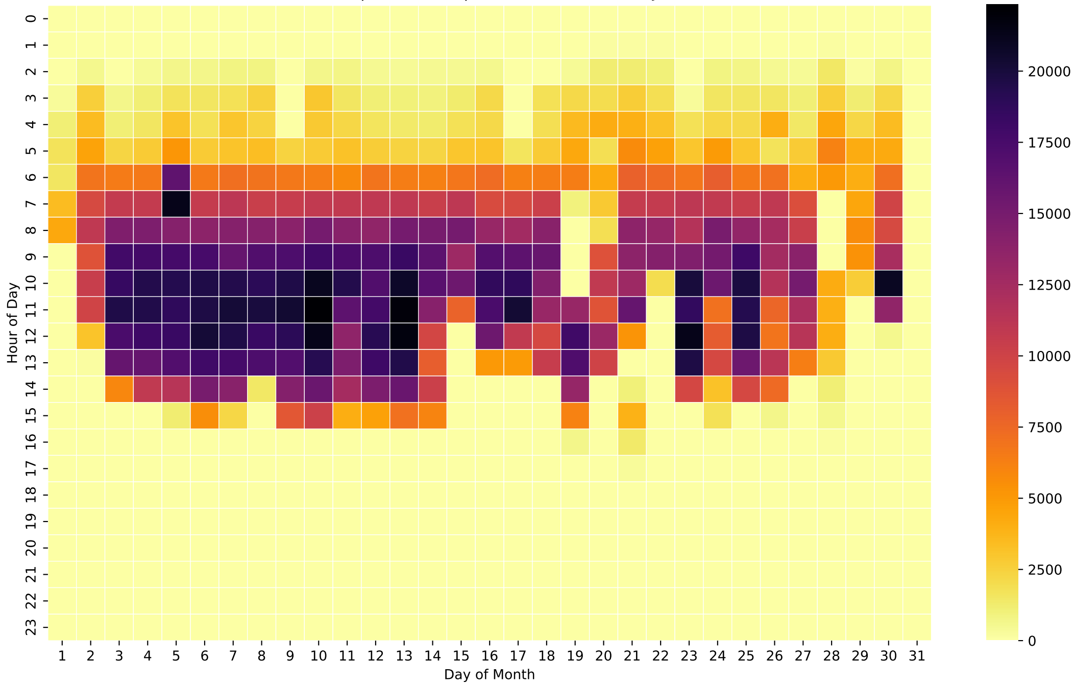
Grid Export Heatmap (Wh/Hour) - 26kWh - Jun
