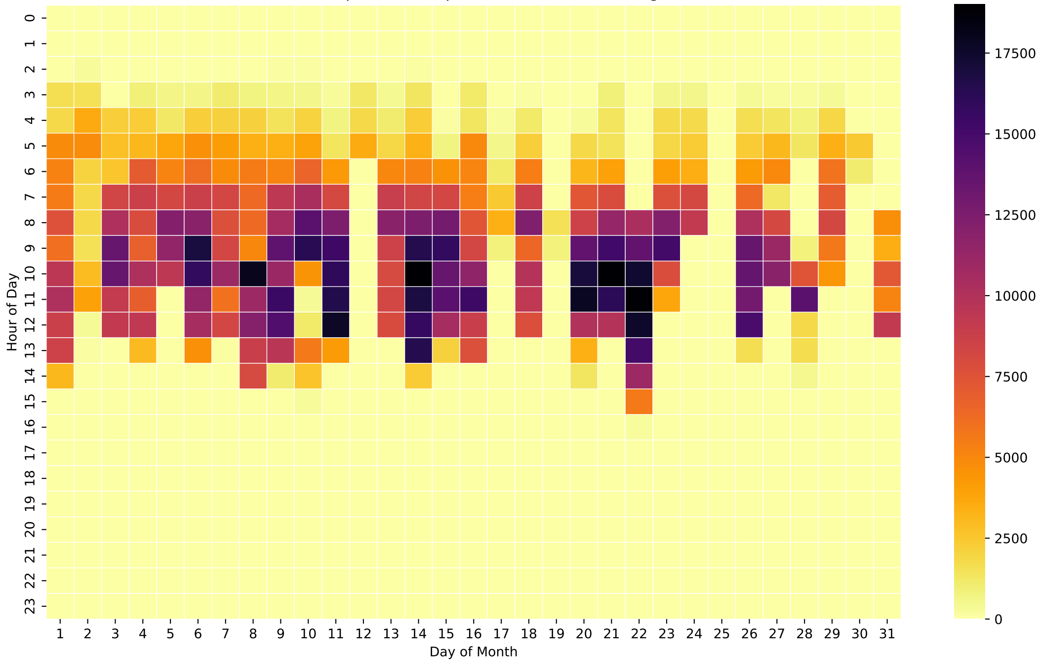
Grid Export Heatmap (Wh/Hour) - 26kWh - Aug
