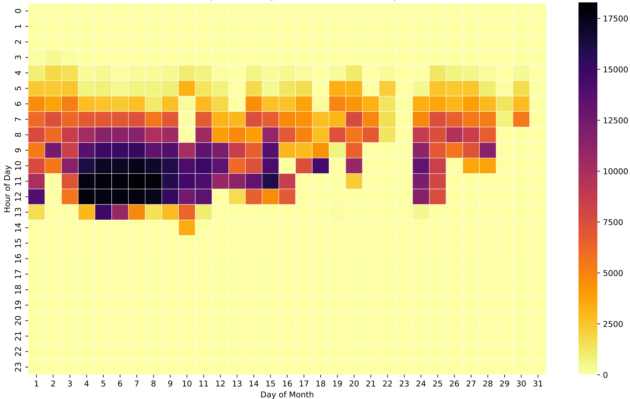
Grid Export Heatmap (Wh/Hour) - 26kWh - Sep
