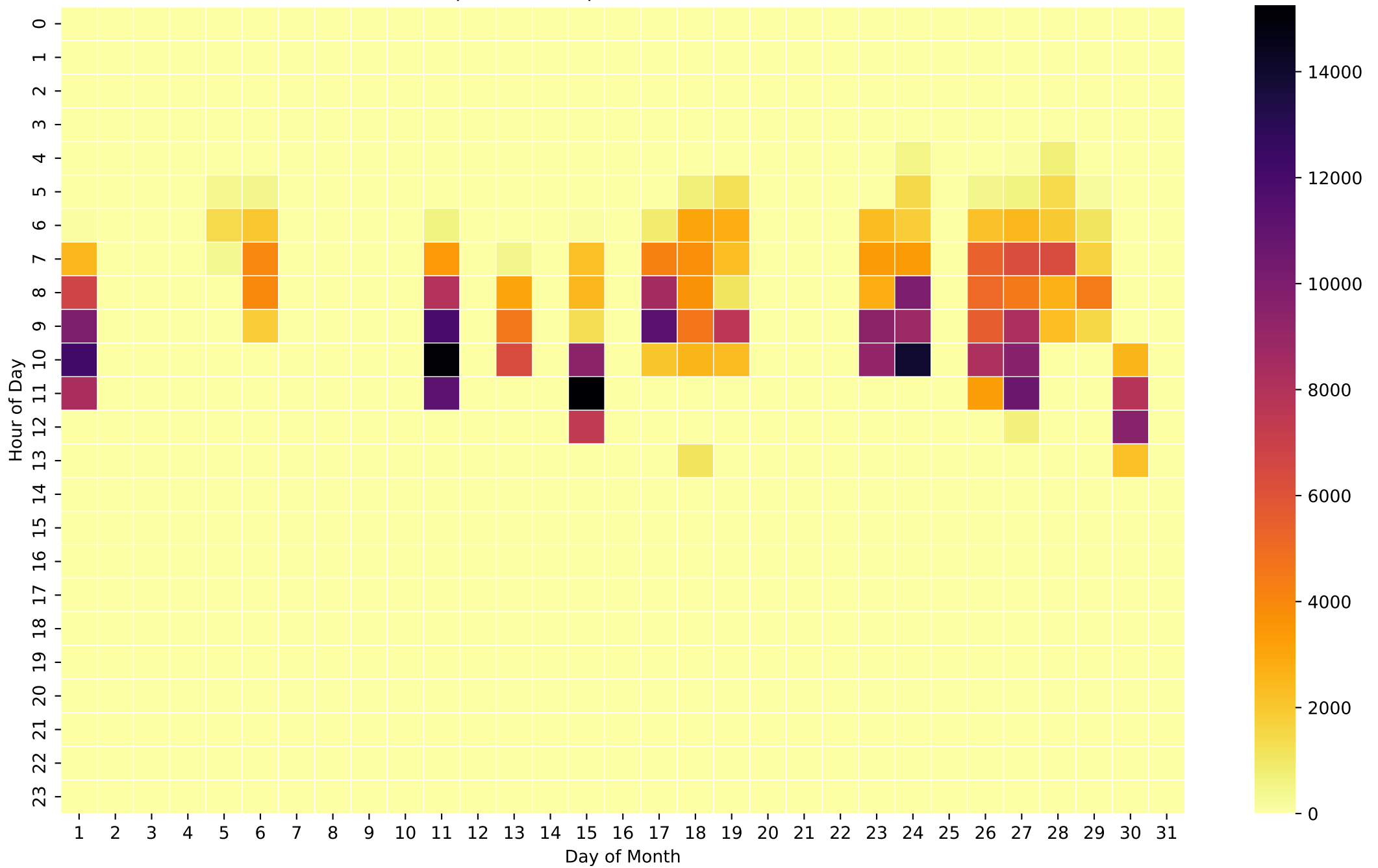
Grid Export Heatmap (Wh/Hour) - 26kWh - Mar
