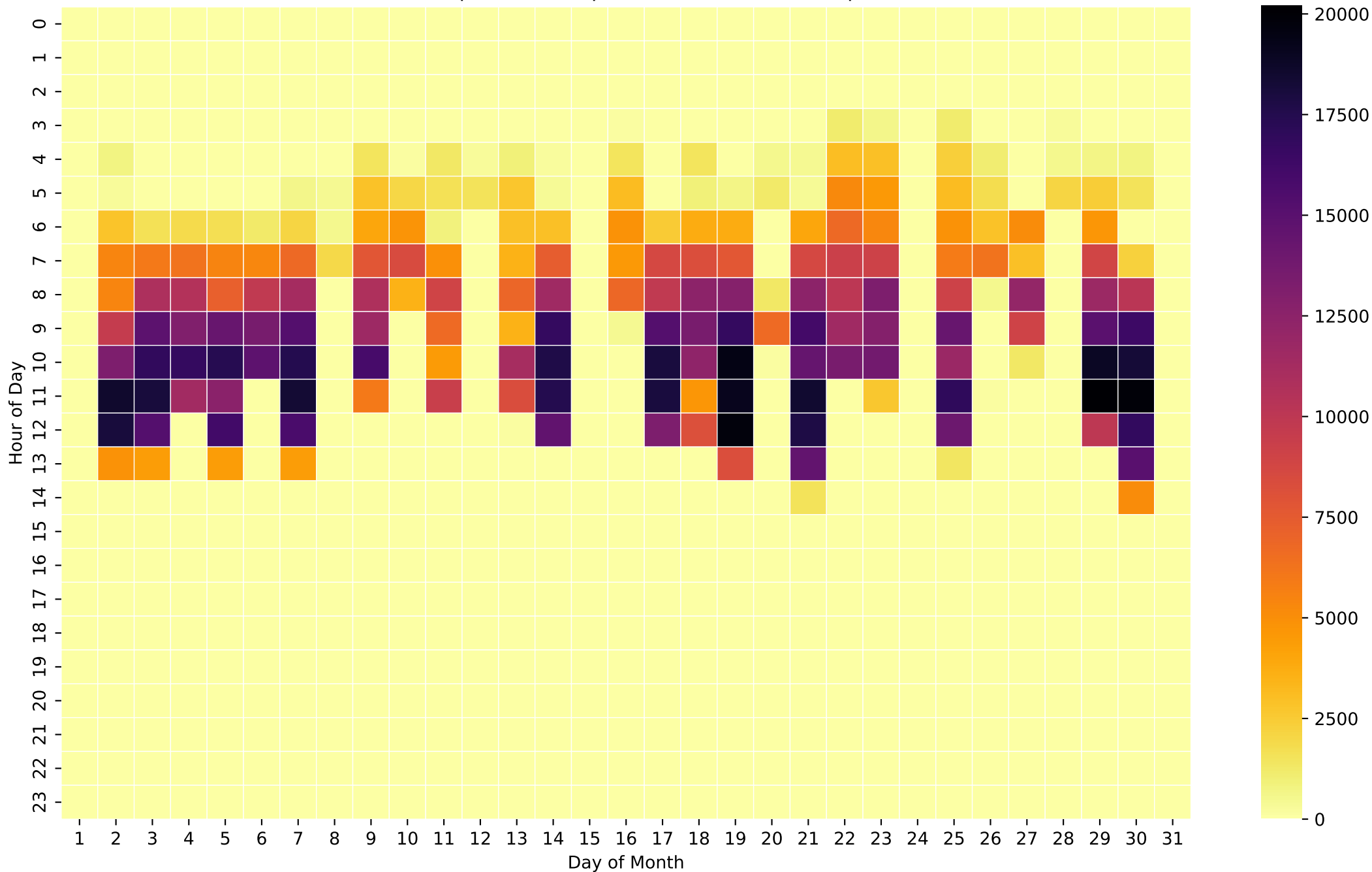
Grid Export Heatmap (Wh/Hour) - 26kWh - Apr
