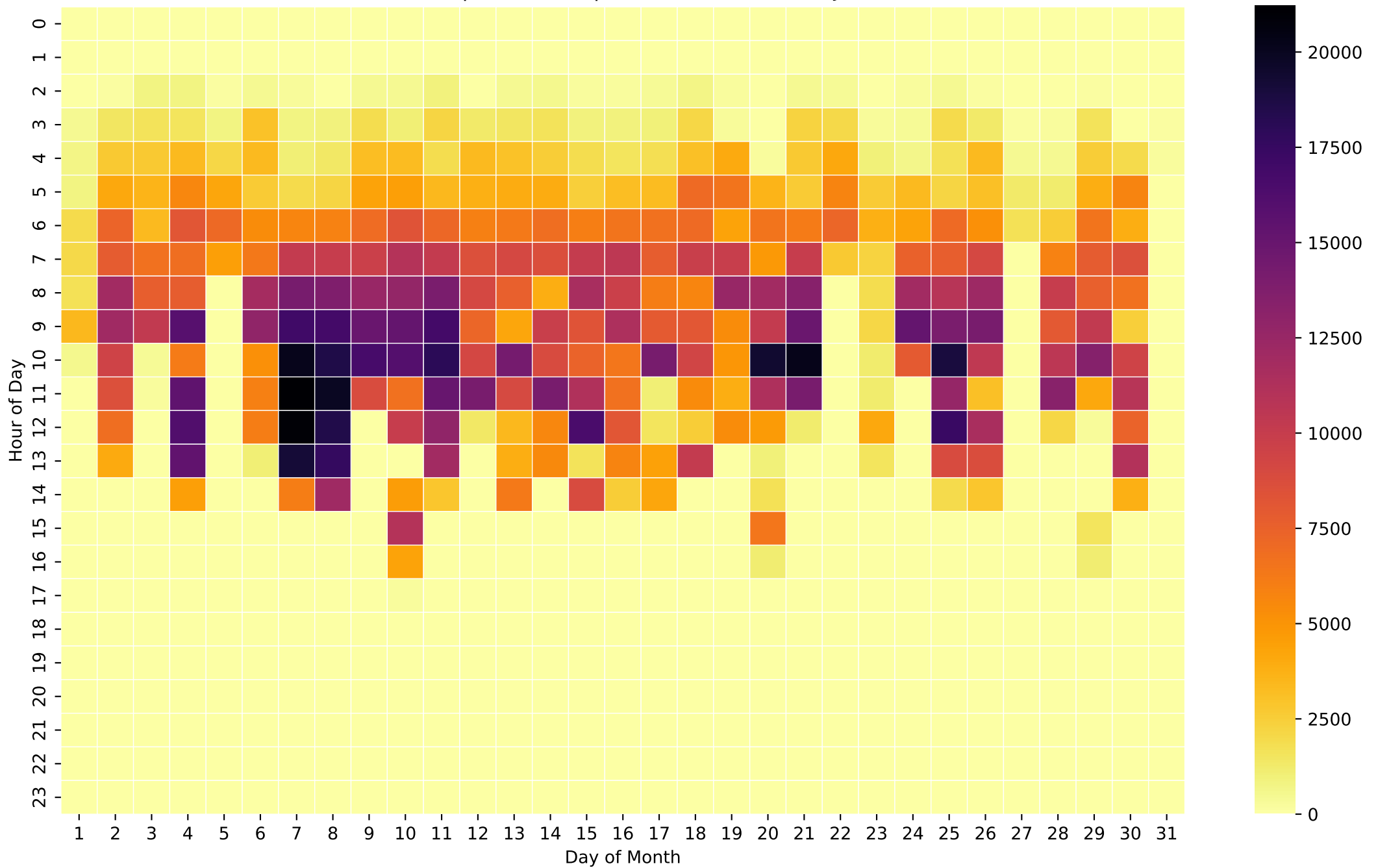
Grid Export Heatmap (Wh/Hour) - 26kWh - Jul
