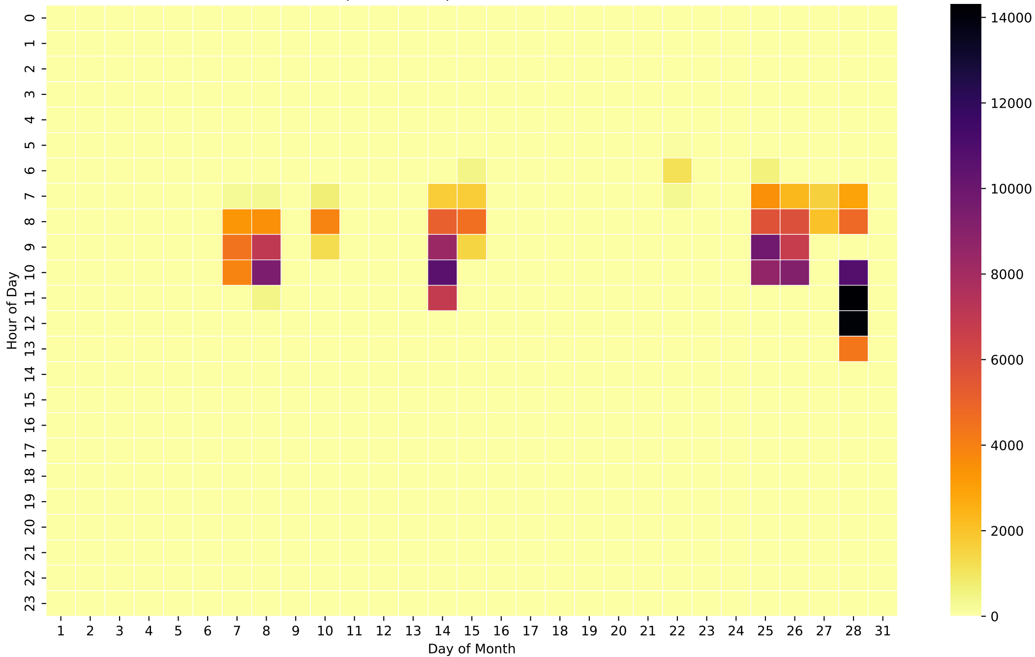
Grid Export Heatmap (Wh/Hour) - 26kWh - Feb
