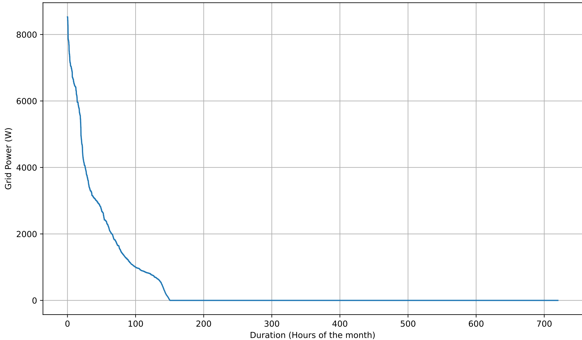
Grid Import Duration Curve - 26kWh - Apr
