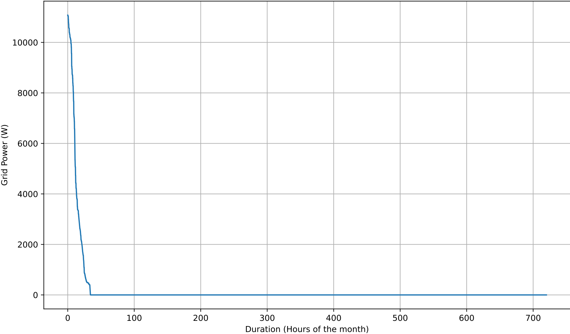
Grid Import Duration Curve - 26kWh - Jun
