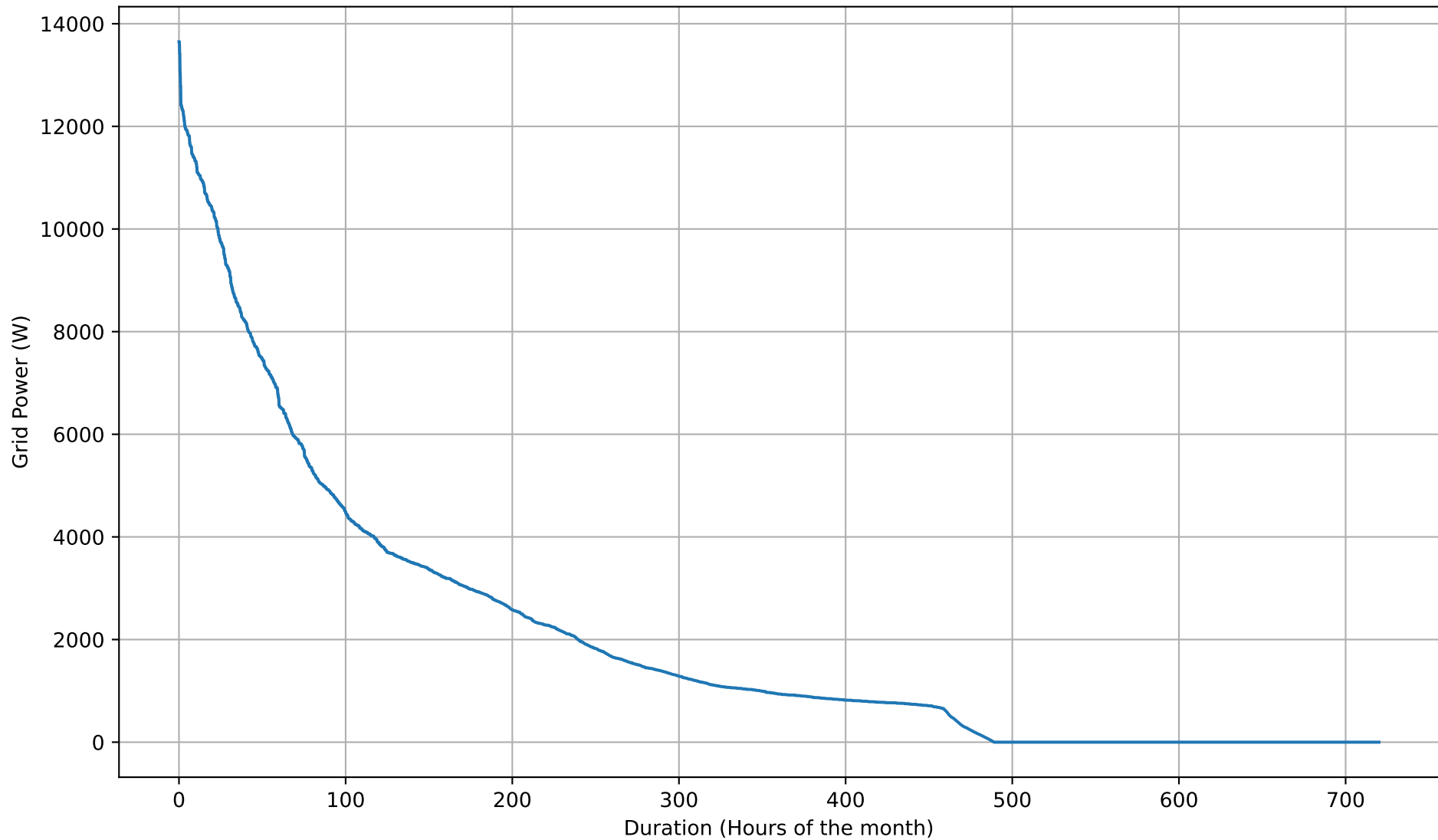
Grid Import Duration Curve - 26kWh - Nov
