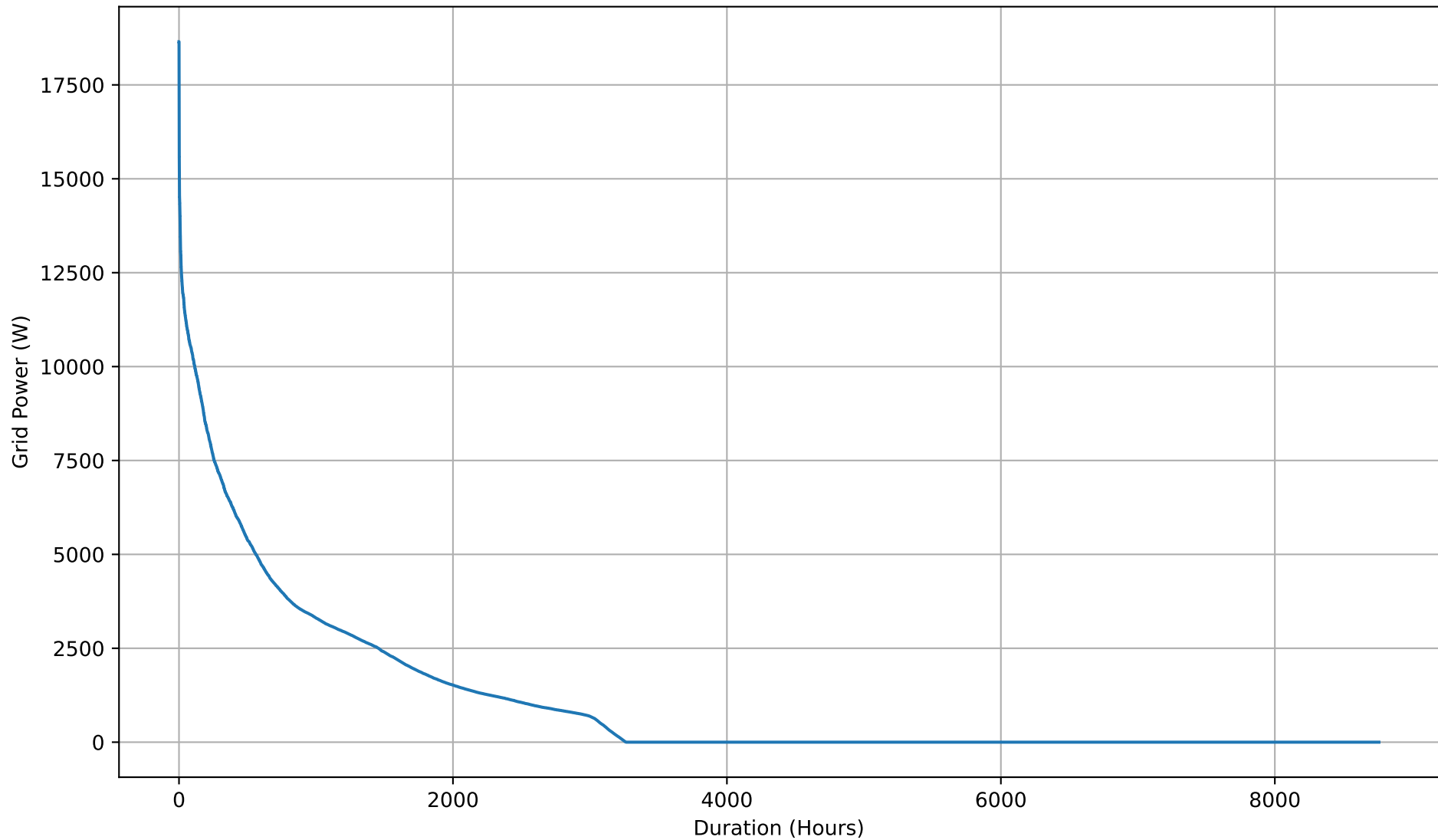
Yearly Grid Import Duration Curve - 26kWh
