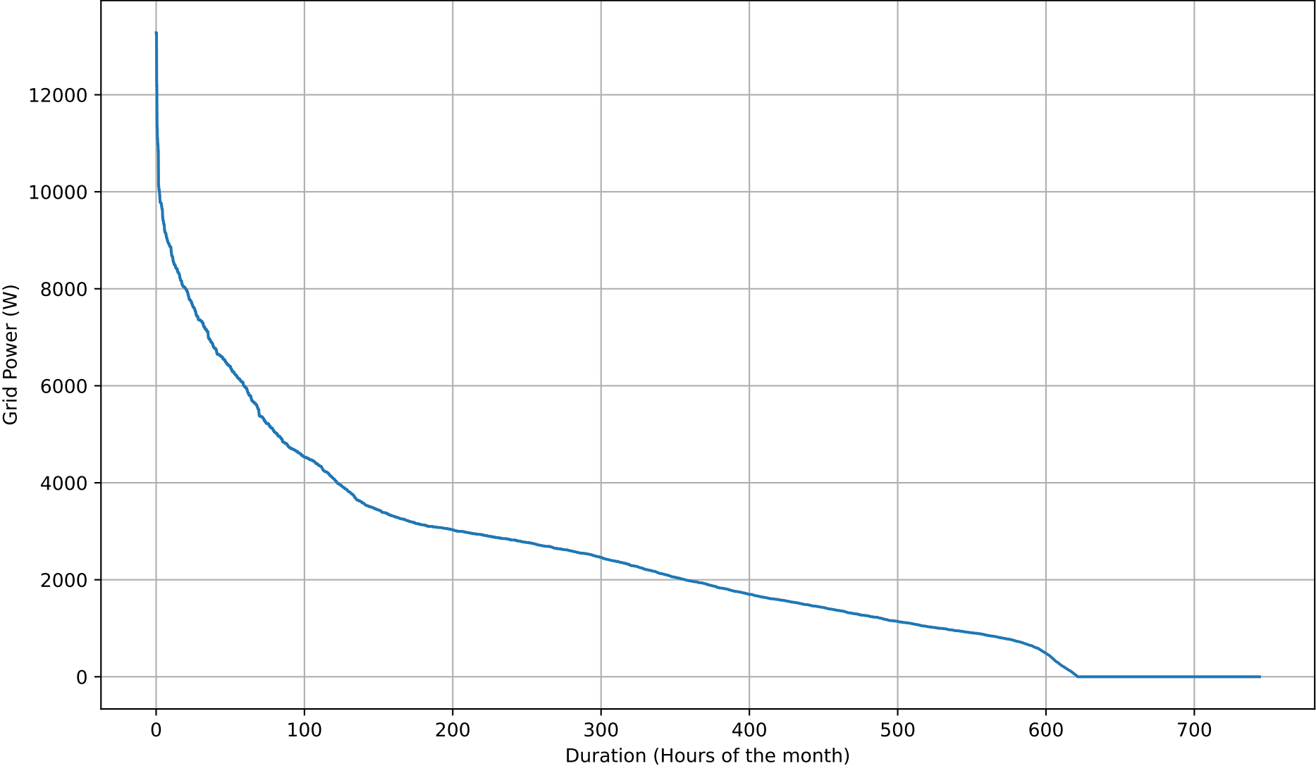
Grid Import Duration Curve - 26kWh - Jan
