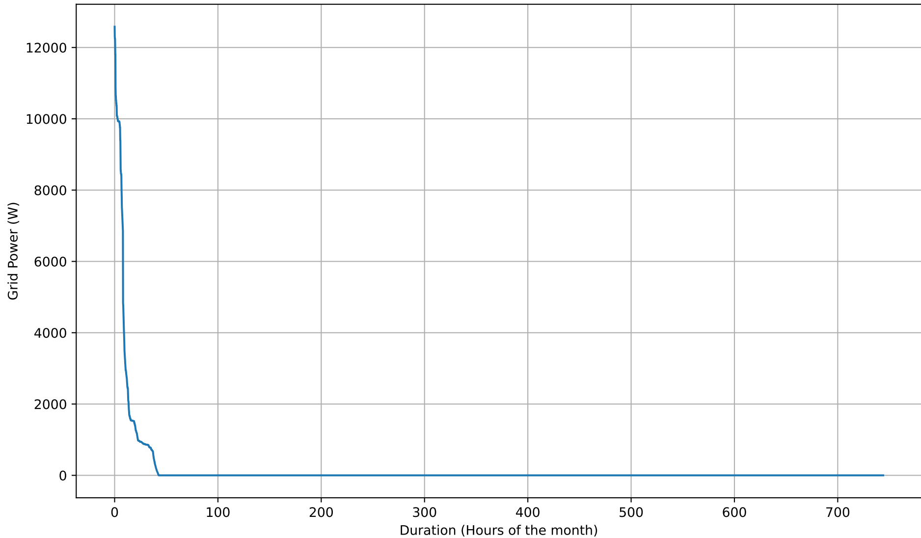
Grid Import Duration Curve - 26kWh - Aug
