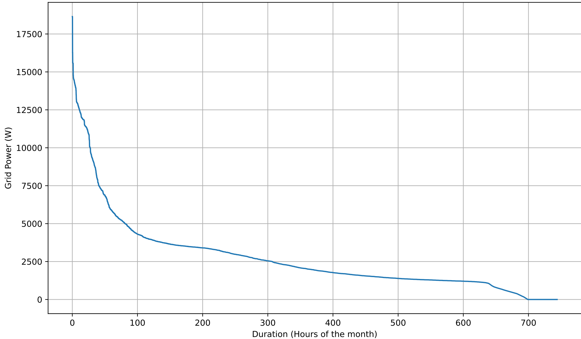
Grid Import Duration Curve - 26kWh - Dec
