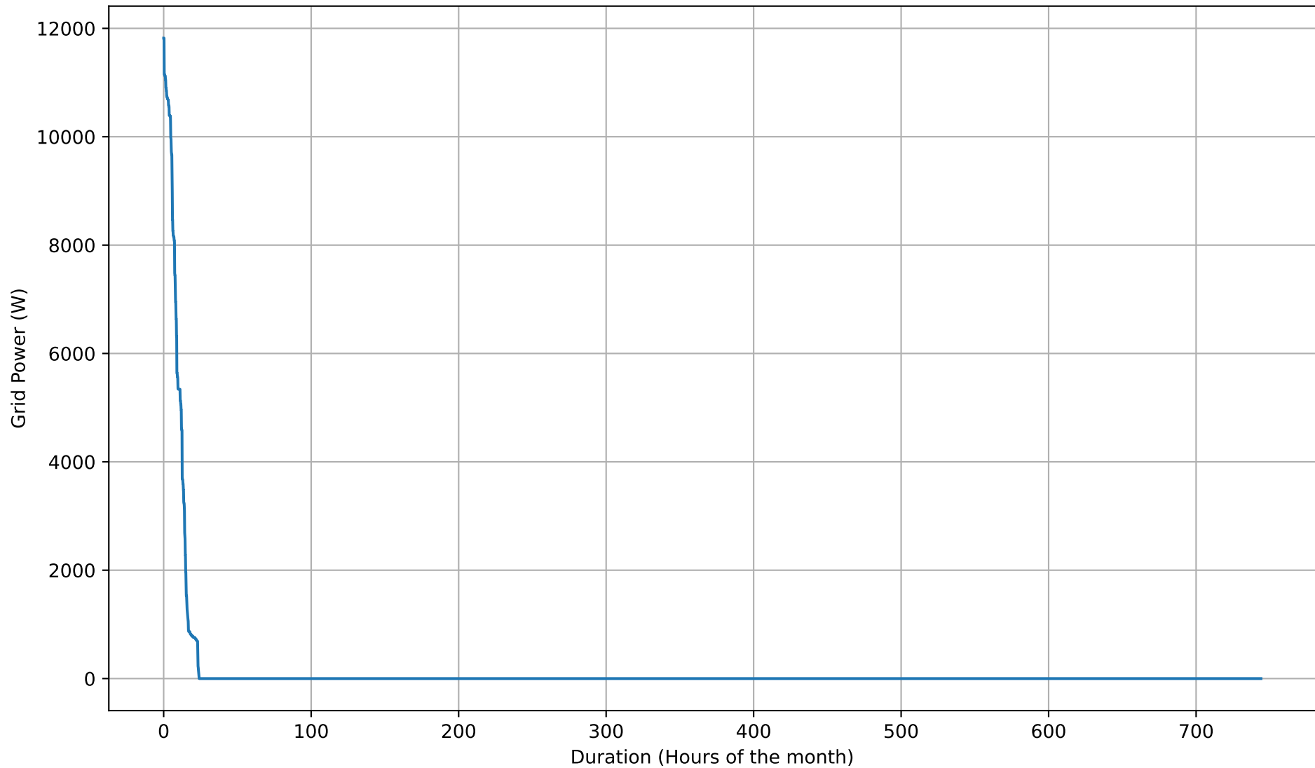
Grid Import Duration Curve - 26kWh - Jul
