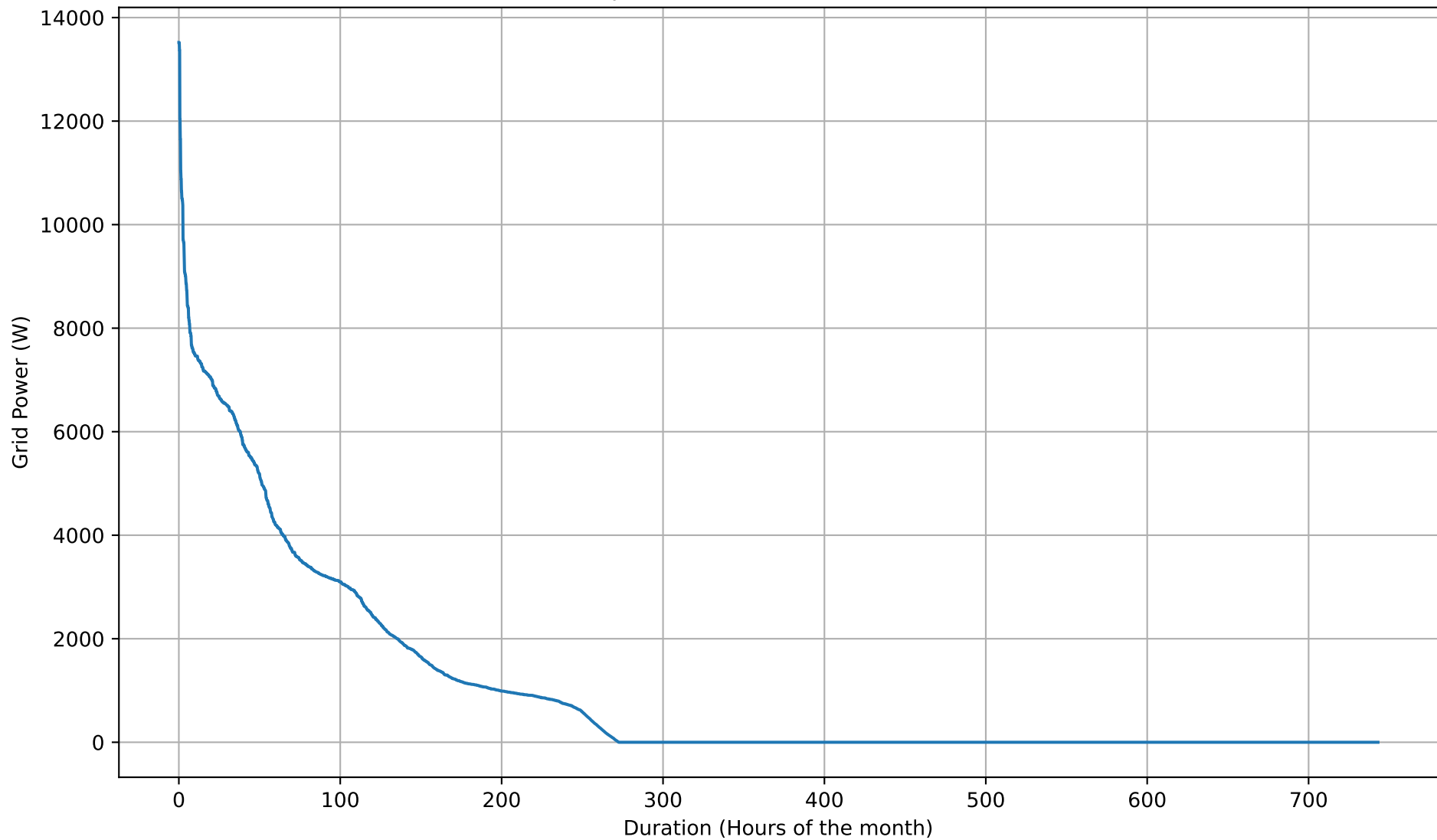
Grid Import Duration Curve - 26kWh - Mar
