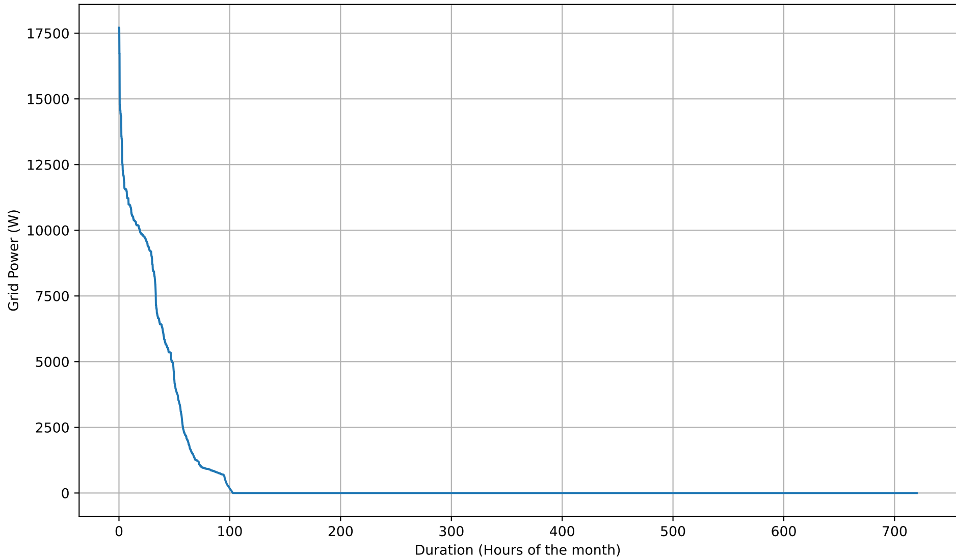
Grid Import Duration Curve - 26kWh - Sep
