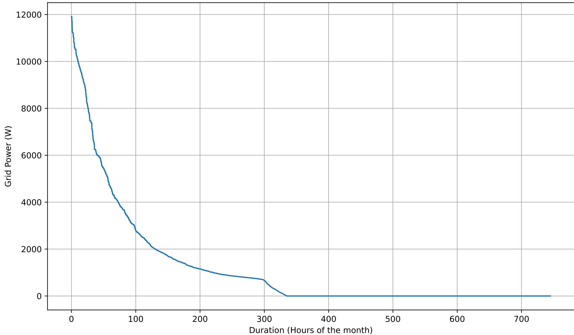
Grid Import Duration Curve - 26kWh - Oct
