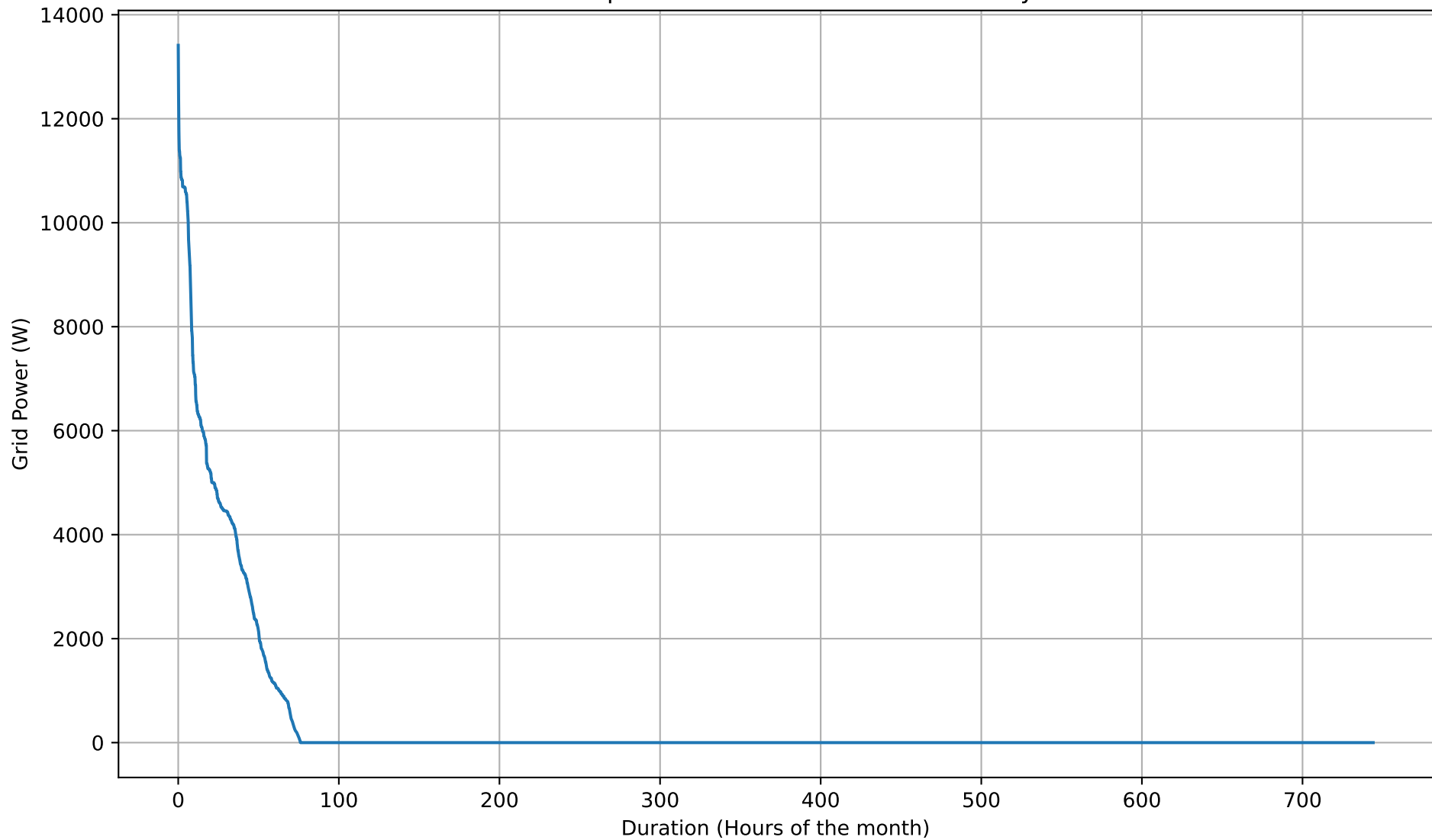
Grid Import Duration Curve - 26kWh - May
