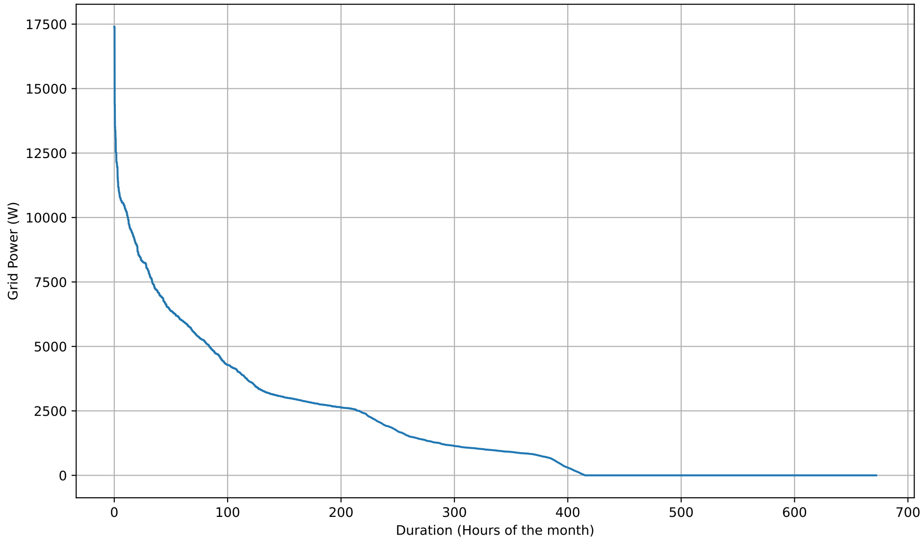
Grid Import Duration Curve - 26kWh - Feb
