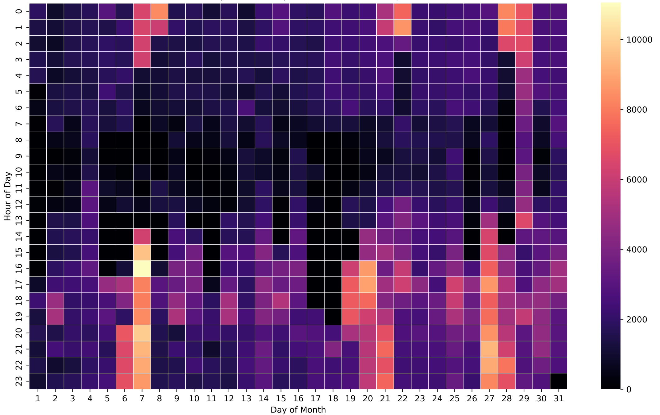
Grid Import Heatmap (Wh/Hour) - 26kWh - Jan
