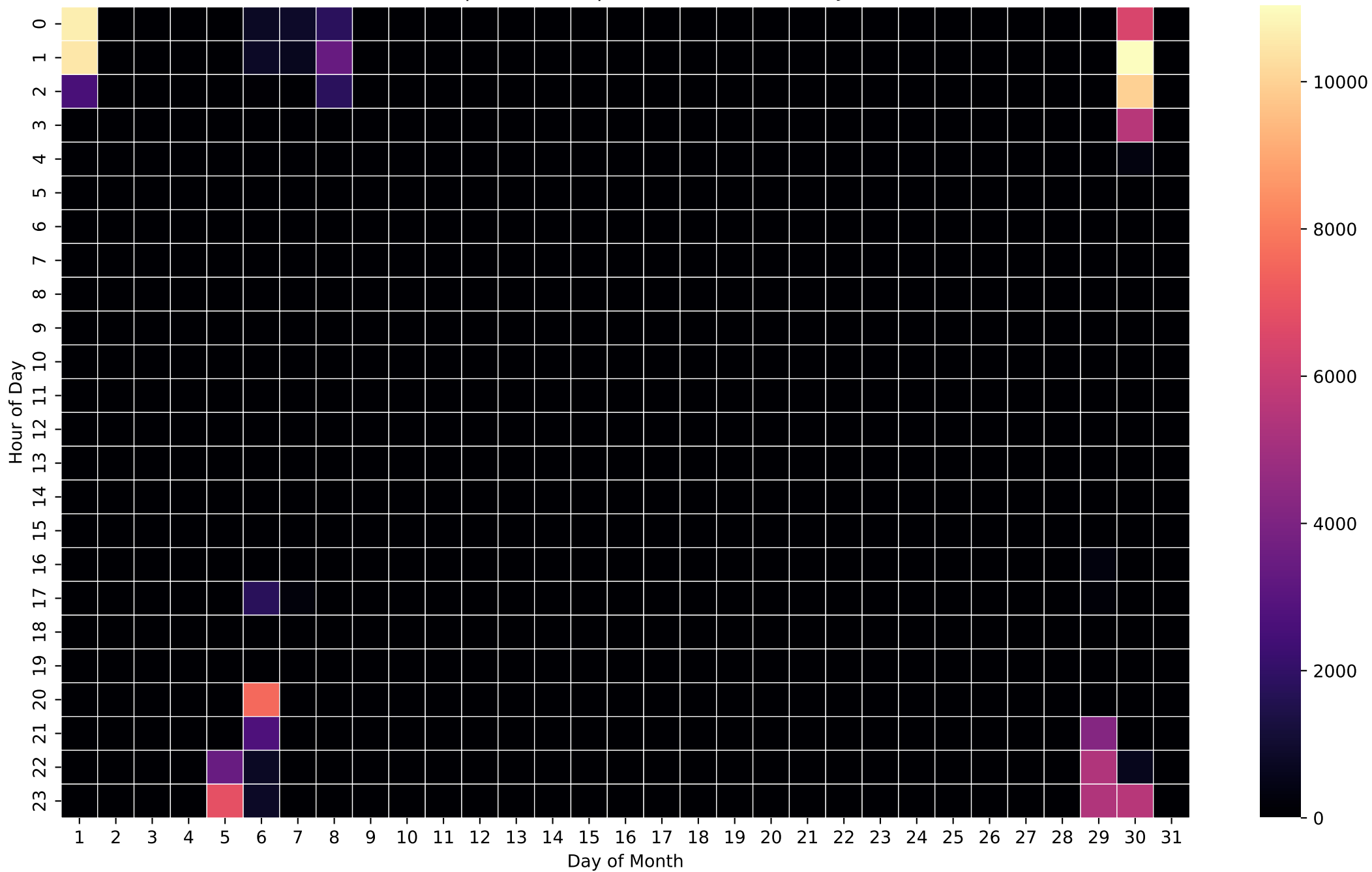
Grid Import Heatmap (Wh/Hour) - 26kWh - Jul
