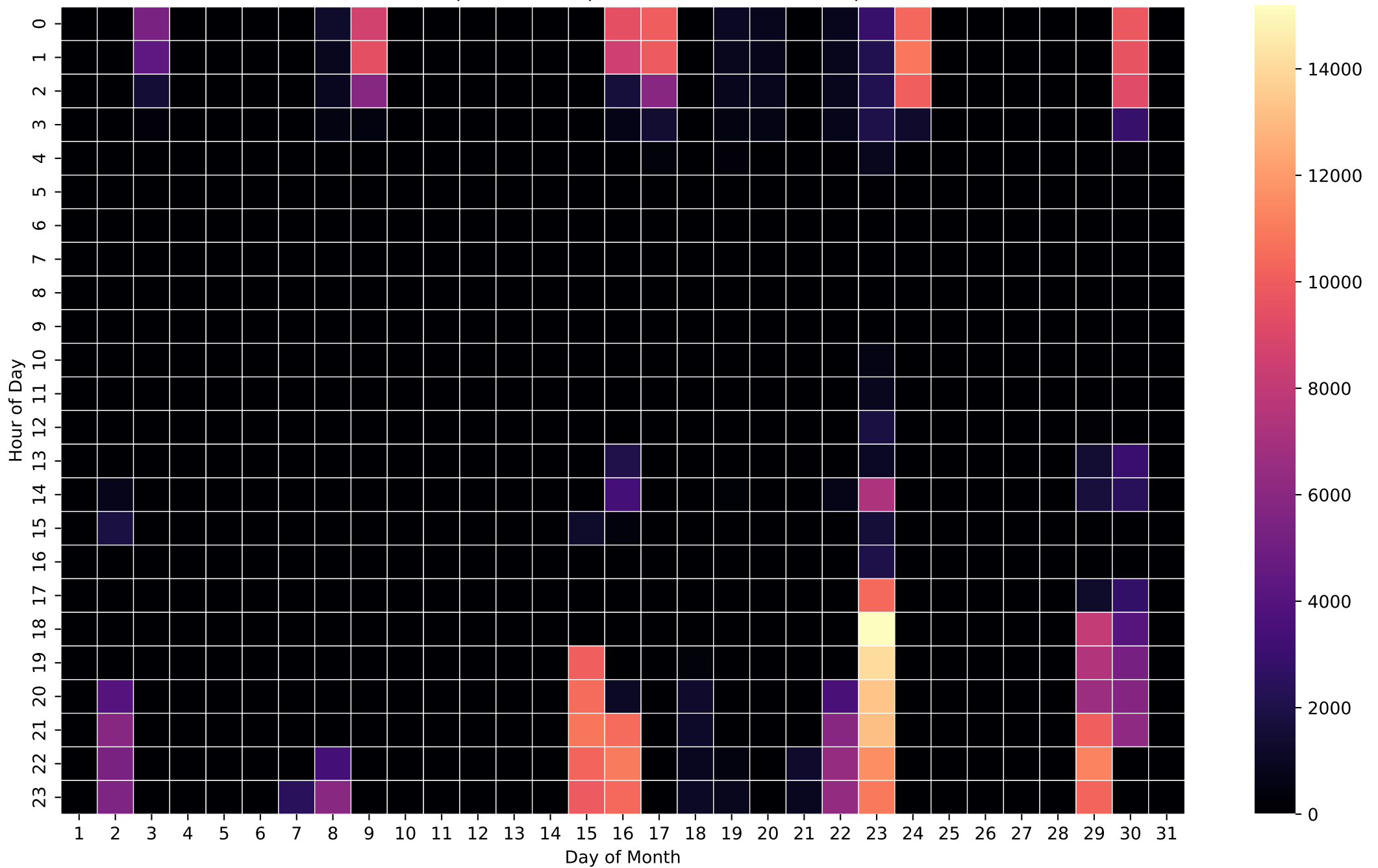
Grid Import Heatmap (Wh/Hour) - 26kWh - Sep
