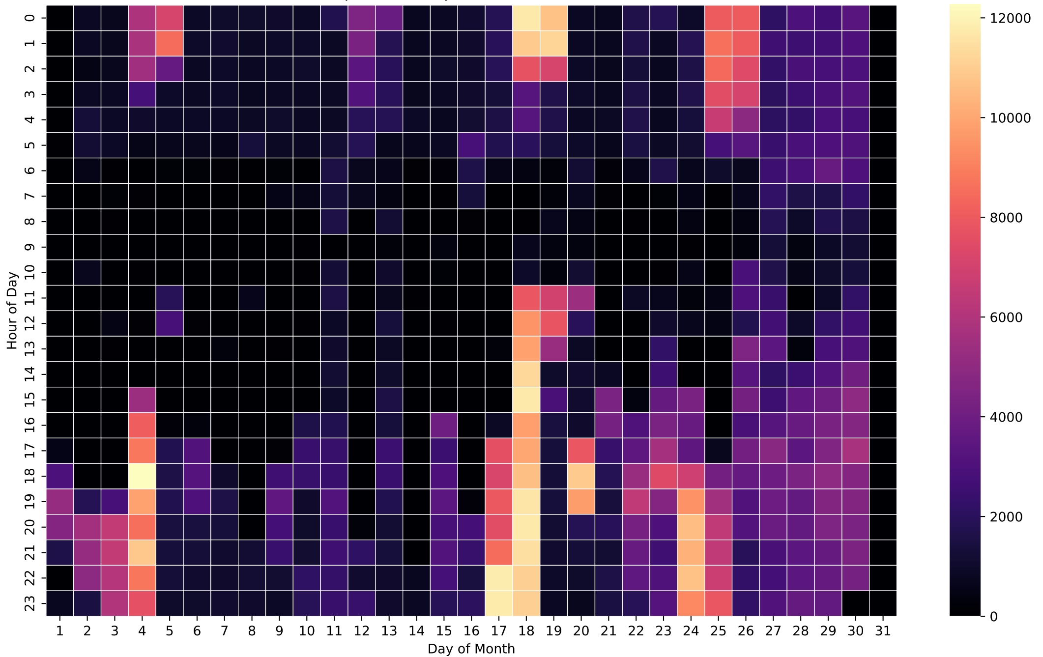
Grid Import Heatmap (Wh/Hour) - 26kWh - Nov
