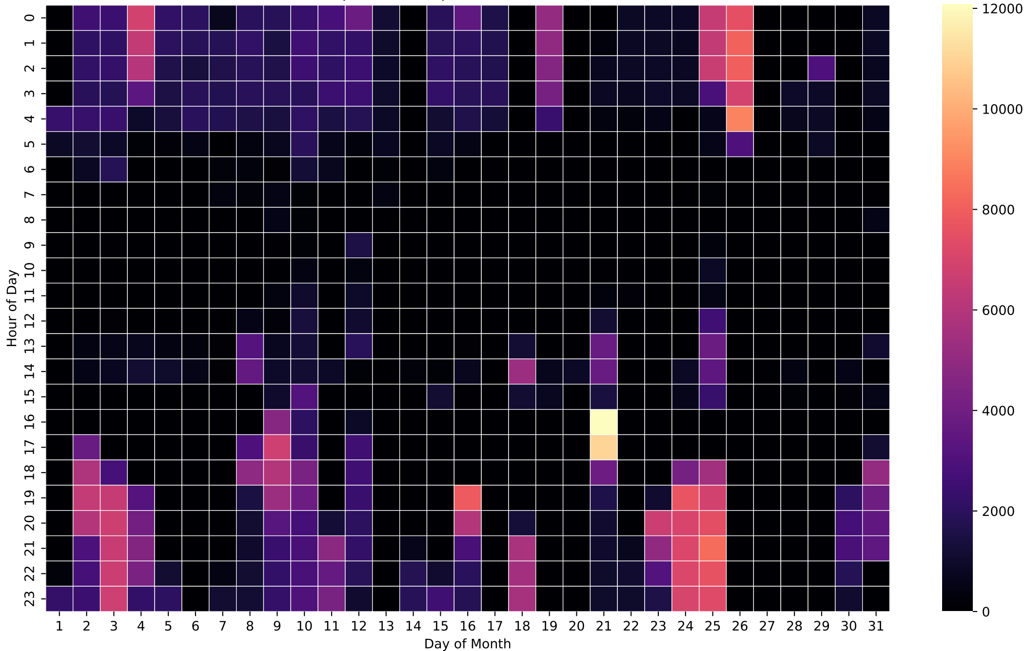
Grid Import Heatmap (Wh/Hour) - 26kWh - Mar
