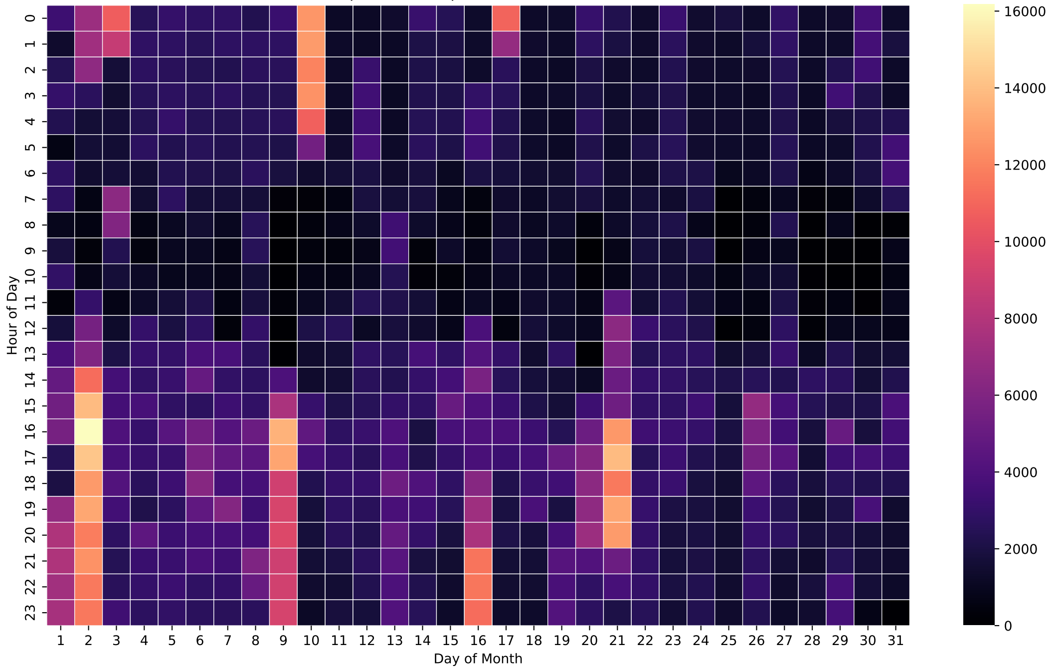
Grid Import Heatmap (Wh/Hour) - 26kWh - Dec
