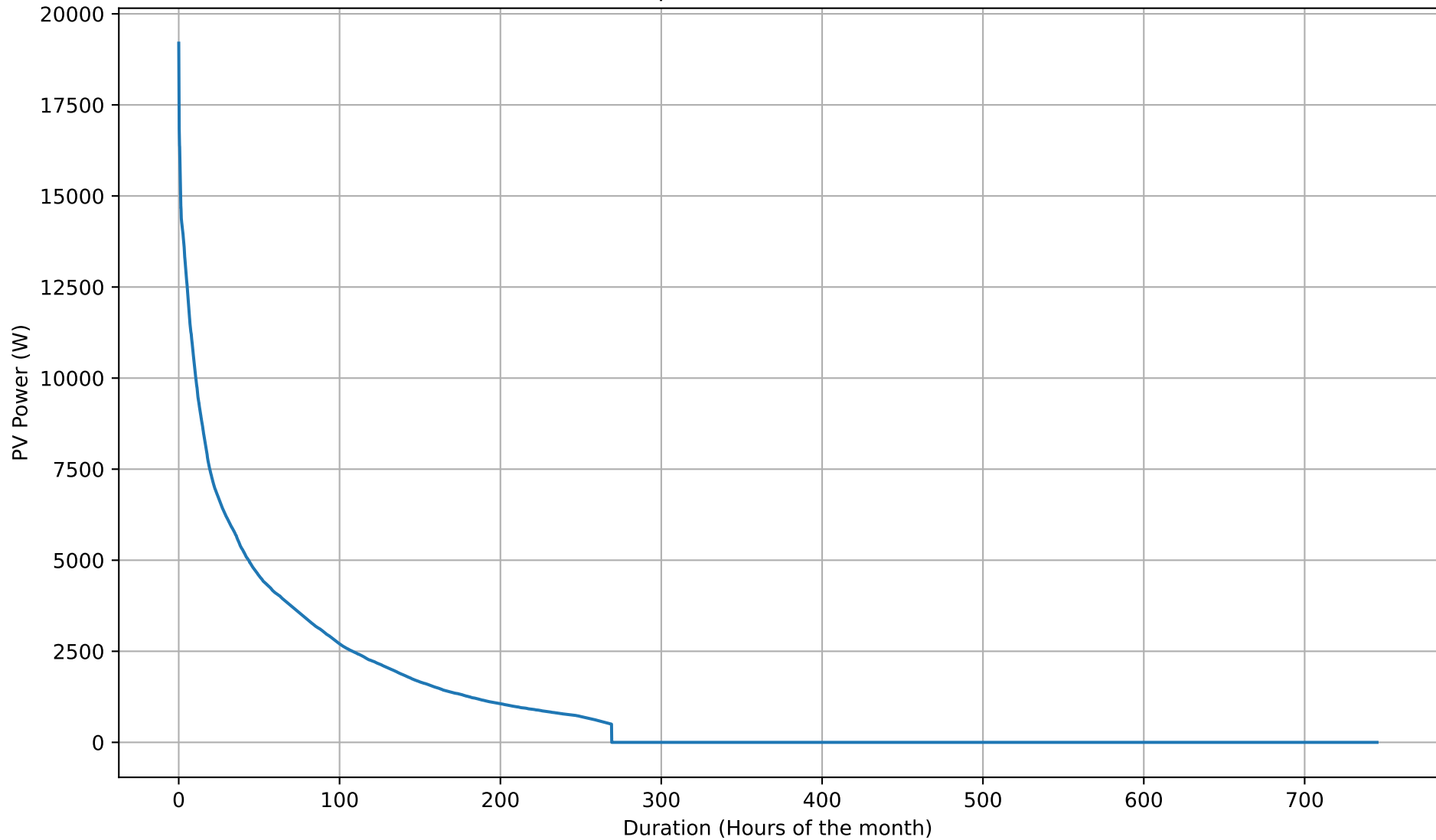
PV Self-Consumption Duration Curve - 26kWh - Oct
