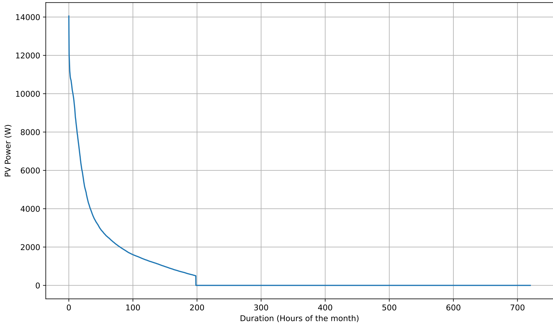
PV Self-Consumption Duration Curve - 26kWh - Nov
