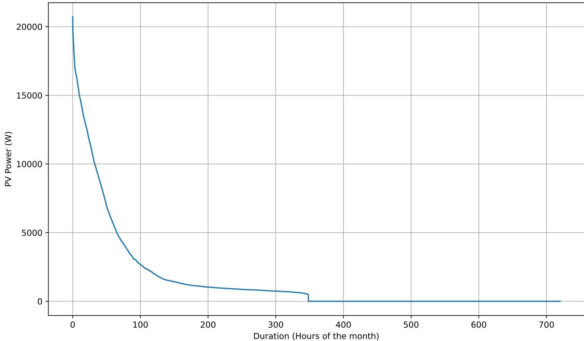
PV Self-Consumption Duration Curve - 26kWh - Sep
