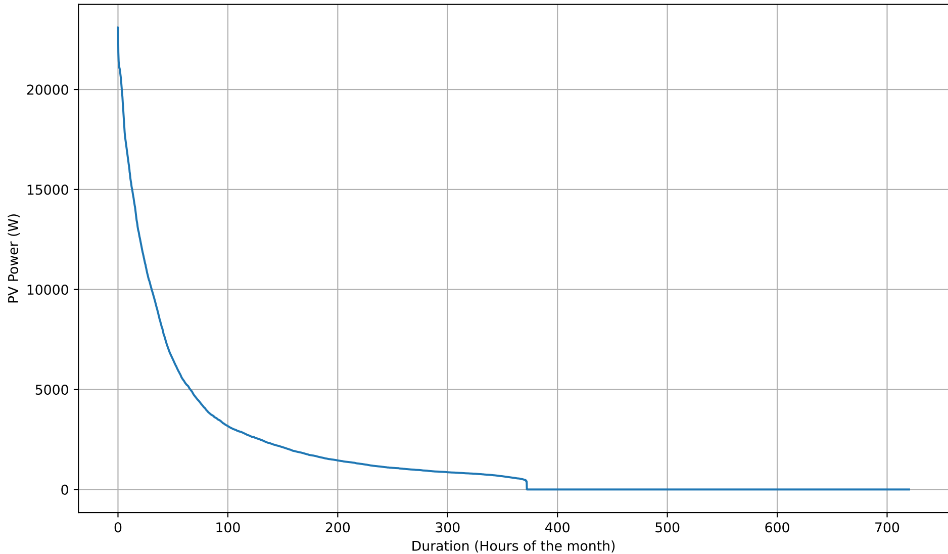
PV Self-Consumption Duration Curve - 26kWh - Apr
