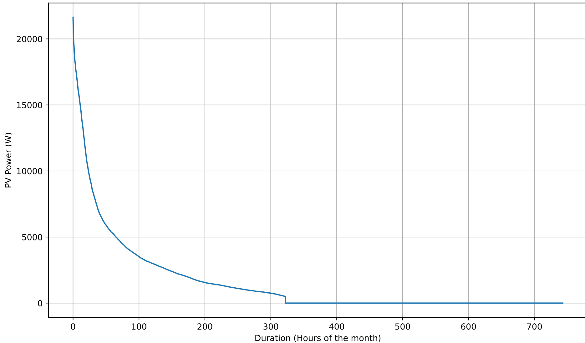
PV Self-Consumption Duration Curve - 26kWh - Mar
