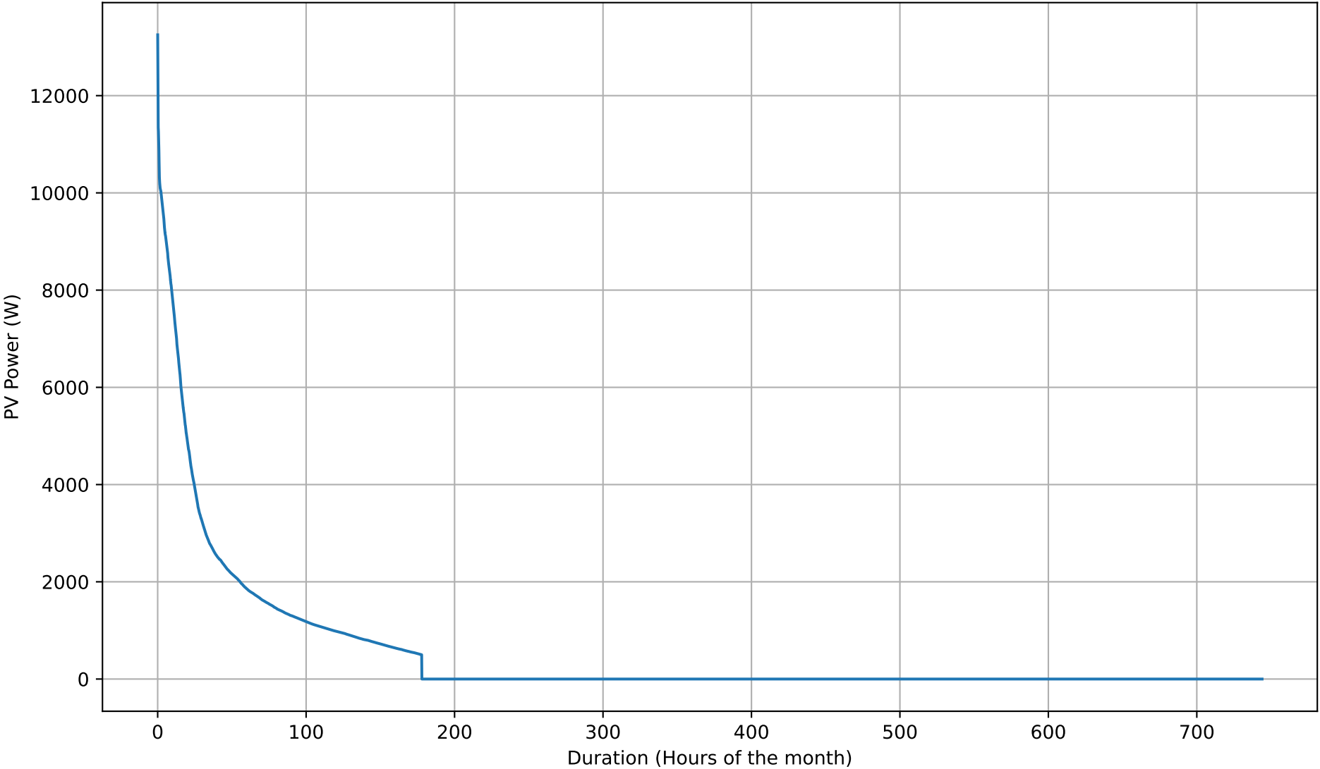
PV Self-Consumption Duration Curve - 26kWh - Jan
