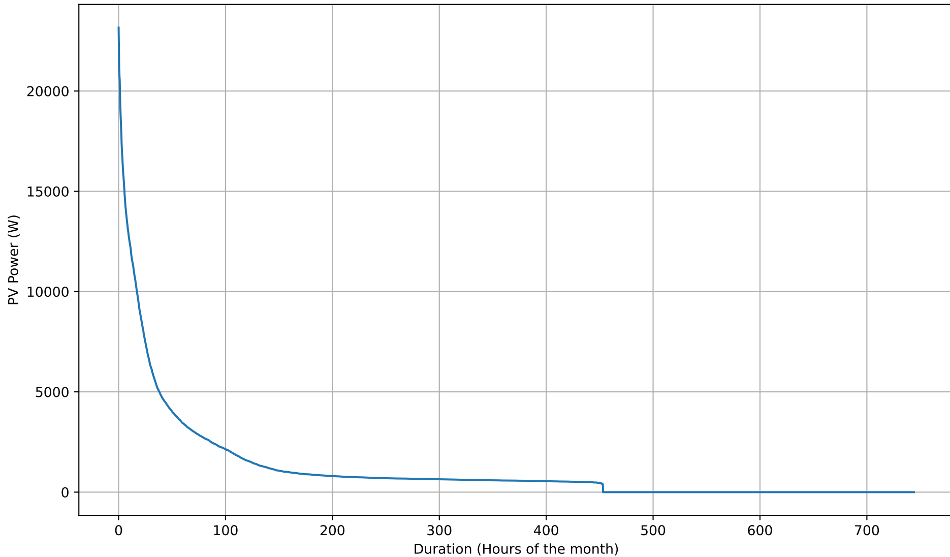
PV Self-Consumption Duration Curve - 26kWh - Jul
