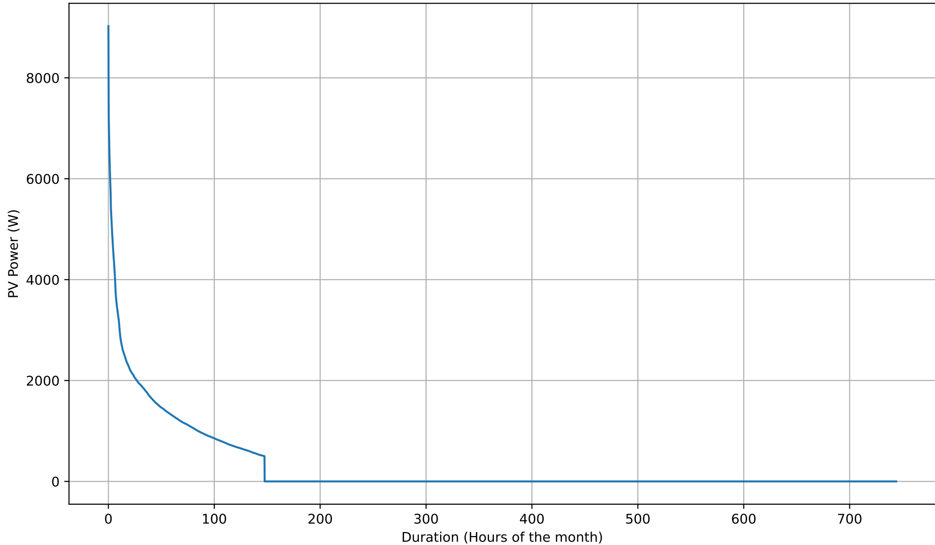
PV Self-Consumption Duration Curve - 26kWh - Dec
