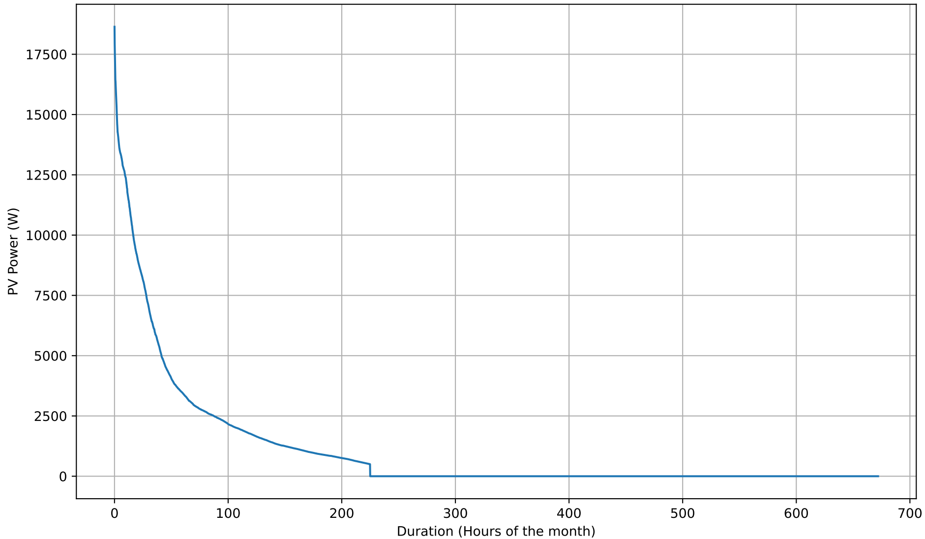
PV Self-Consumption Duration Curve - 26kWh - Feb
