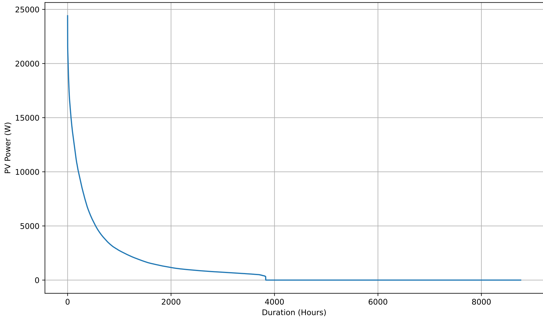
Yearly PV Self-Consumption Duration Curve - 26kWh
