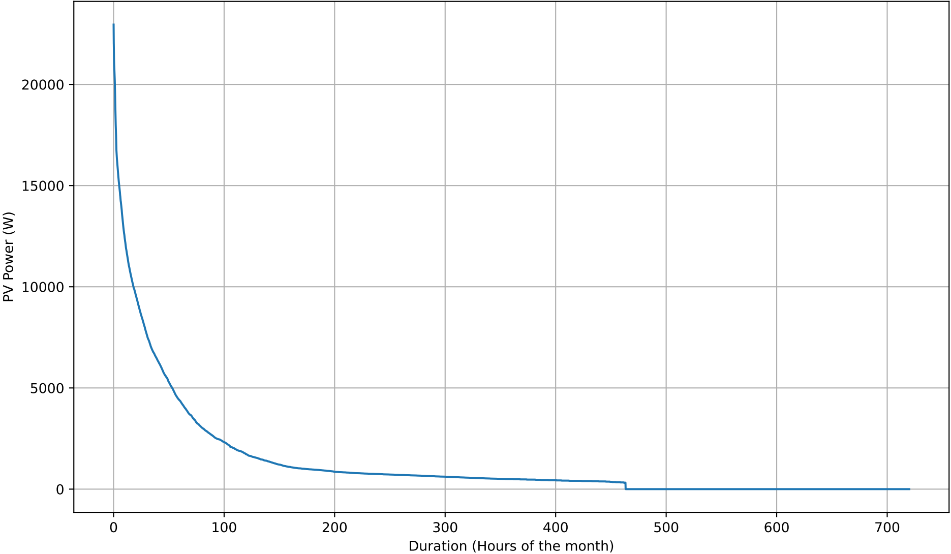
PV Self-Consumption Duration Curve - 26kWh - Jun
