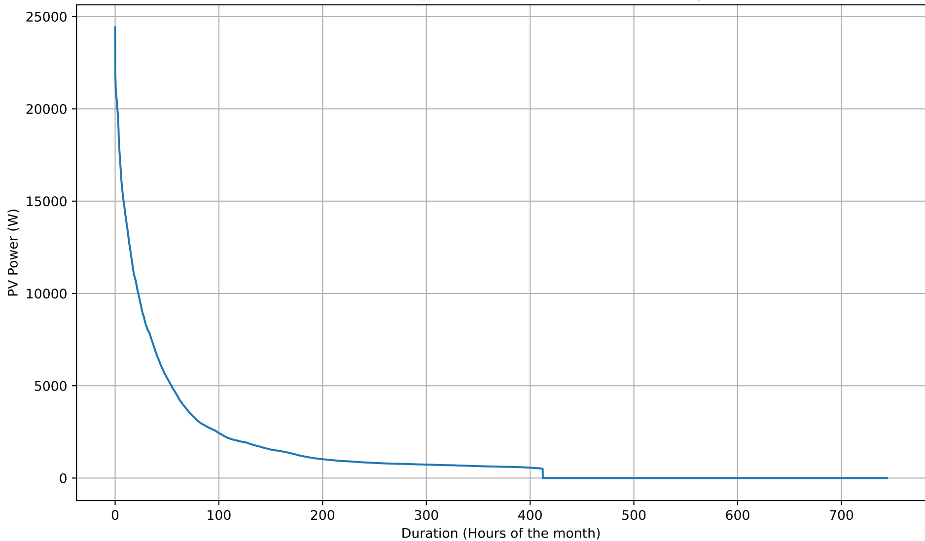
PV Self-Consumption Duration Curve - 26kWh - Aug
