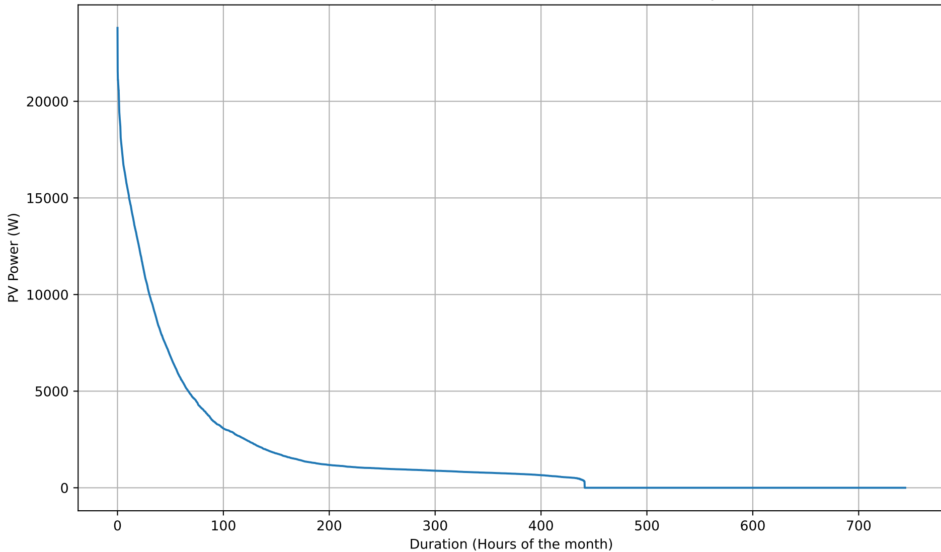
PV Self-Consumption Duration Curve - 26kWh - May
