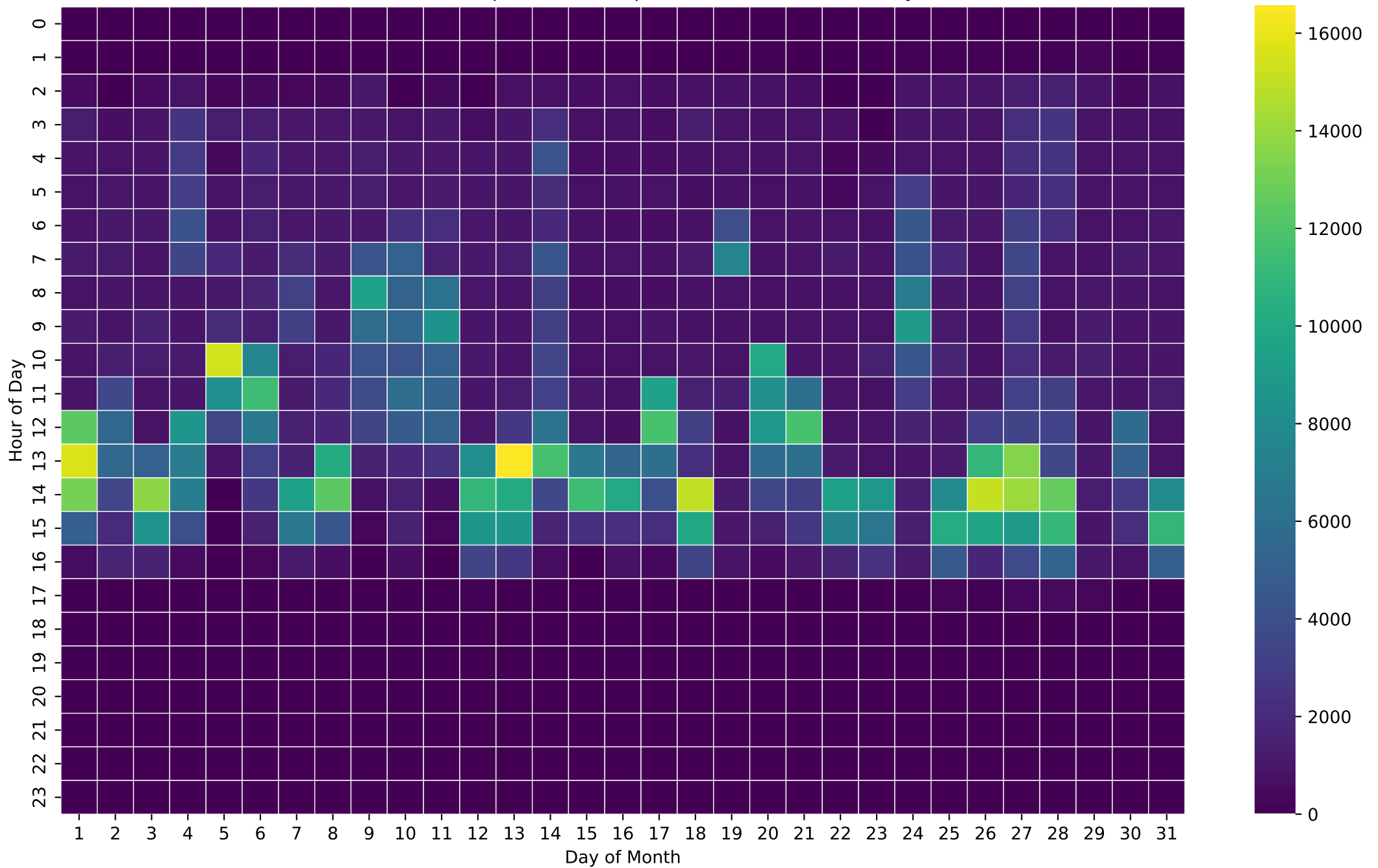
PV Self-Consumption Heatmap (Wh/Hour) - 26kWh - May
