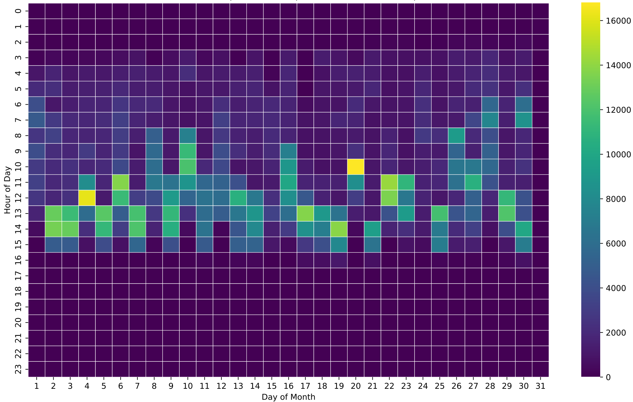
PV Self-Consumption Heatmap (Wh/Hour) - 26kWh - Apr
