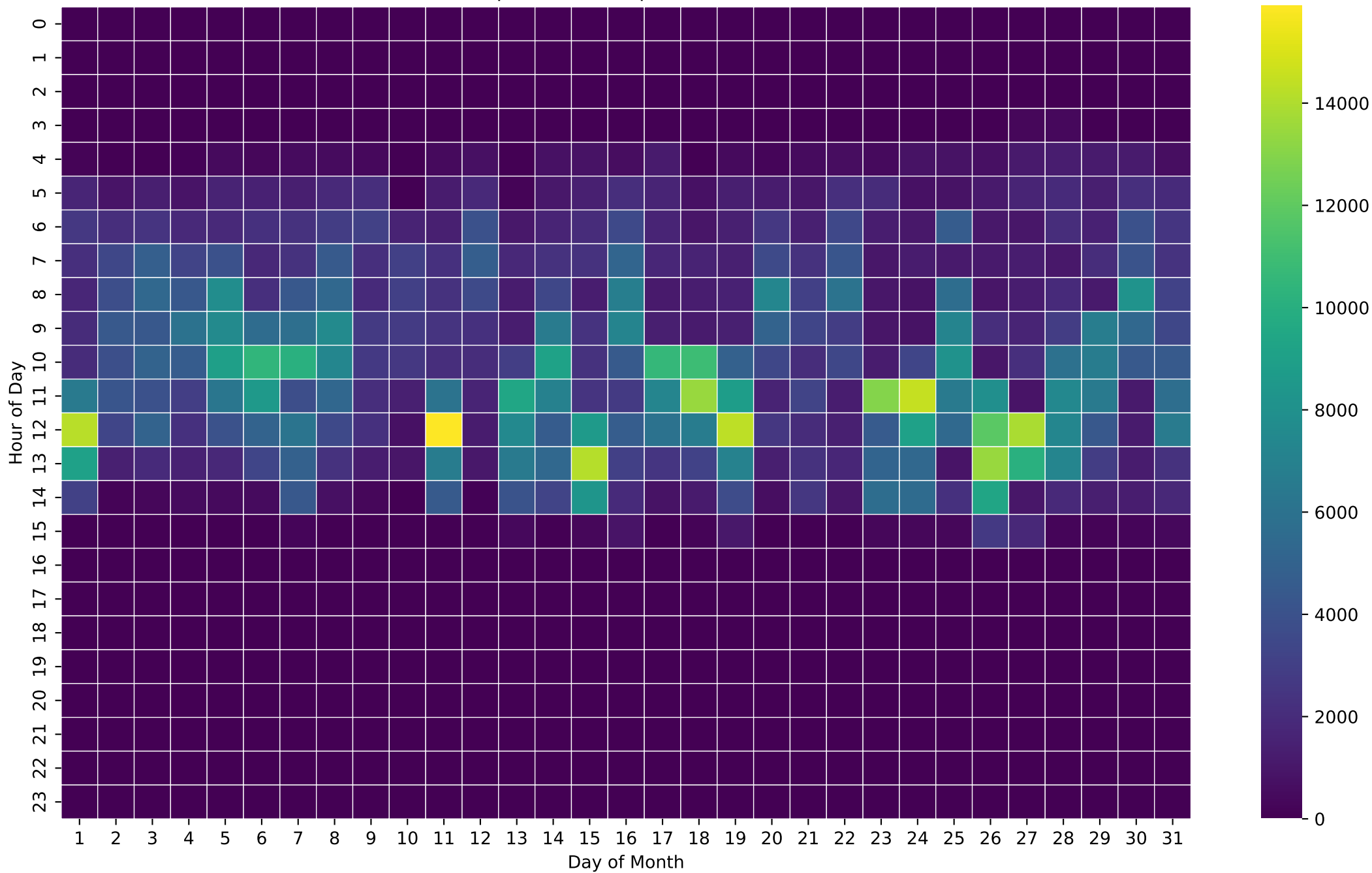
PV Self-Consumption Heatmap (Wh/Hour) - 26kWh - Mar
