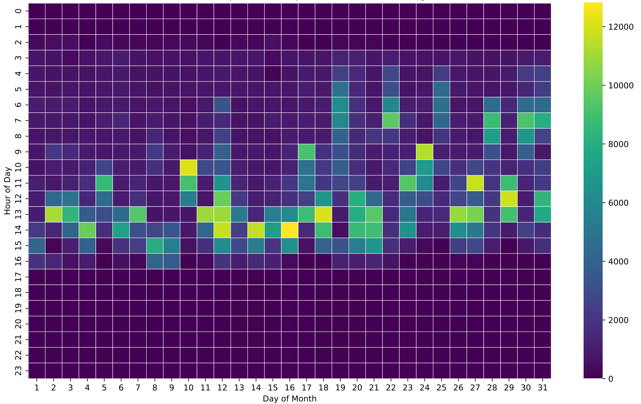
PV Self-Consumption Heatmap (Wh/Hour) - 26kWh - Aug
