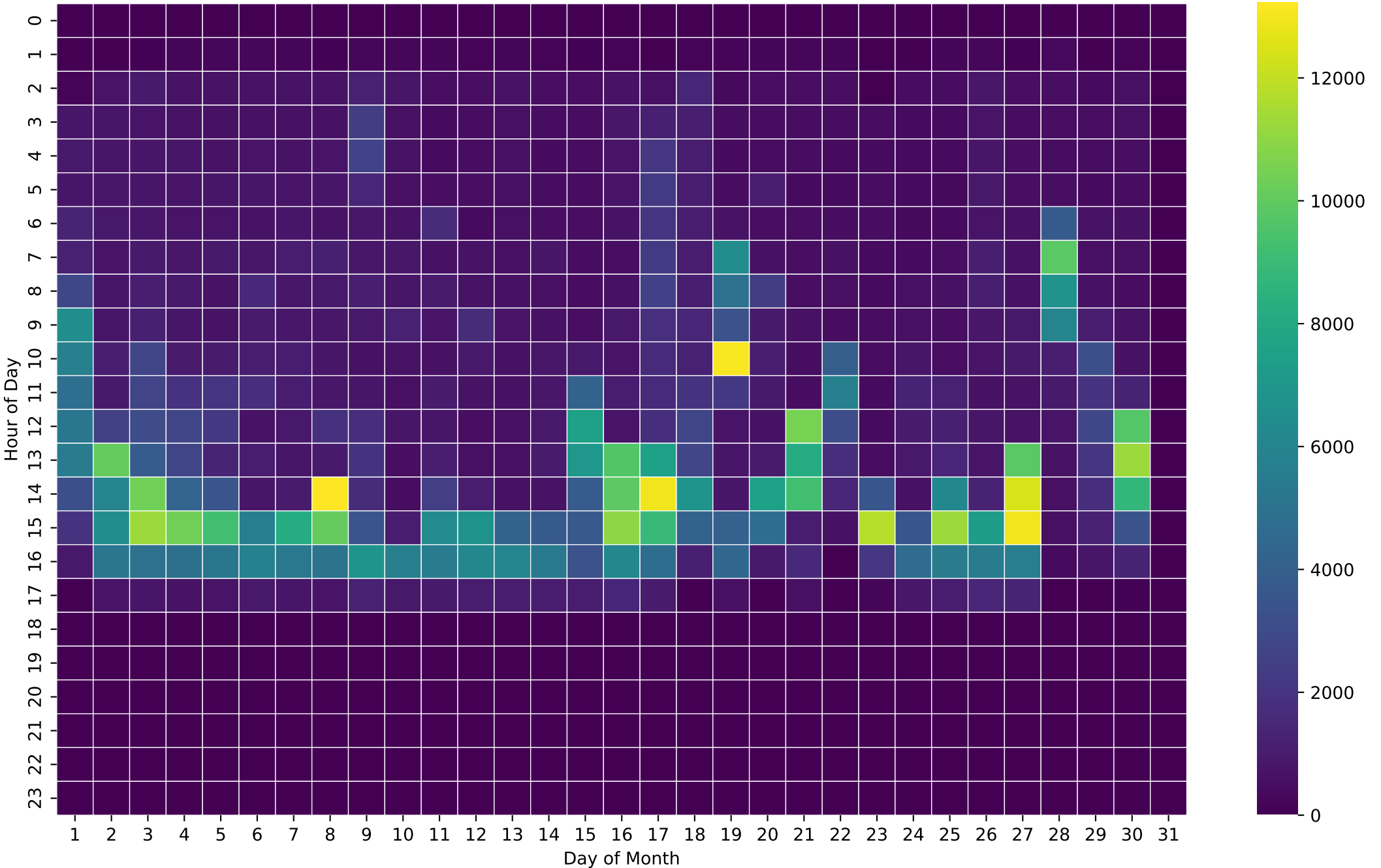
PV Self-Consumption Heatmap (Wh/Hour) - 26kWh - Jun
