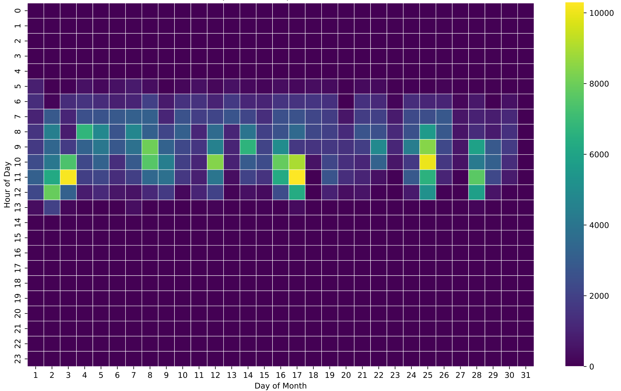
PV Self-Consumption Heatmap (Wh/Hour) - 26kWh - Nov
