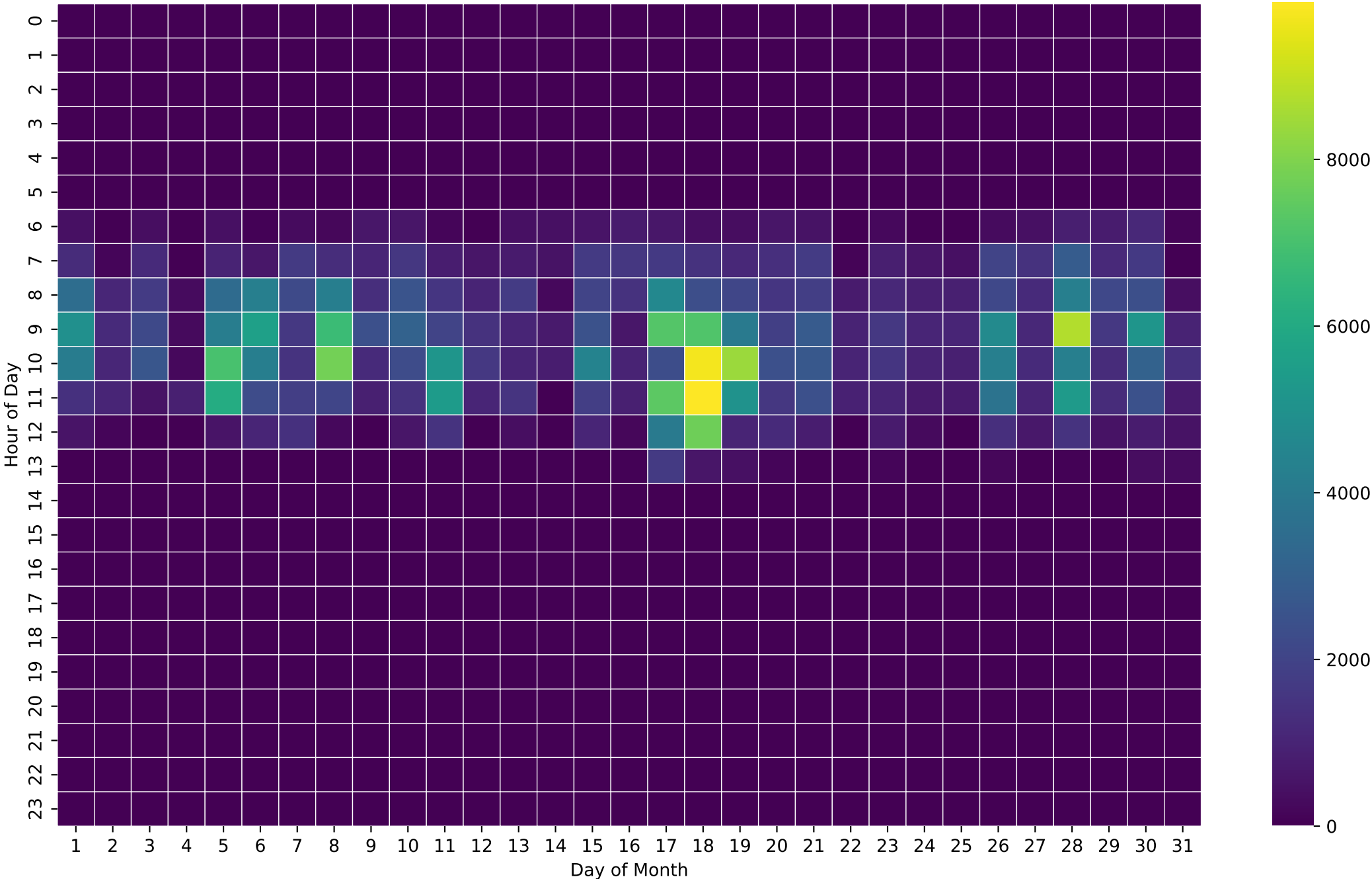
PV Self-Consumption Heatmap (Wh/Hour) - 26kWh - Jan
