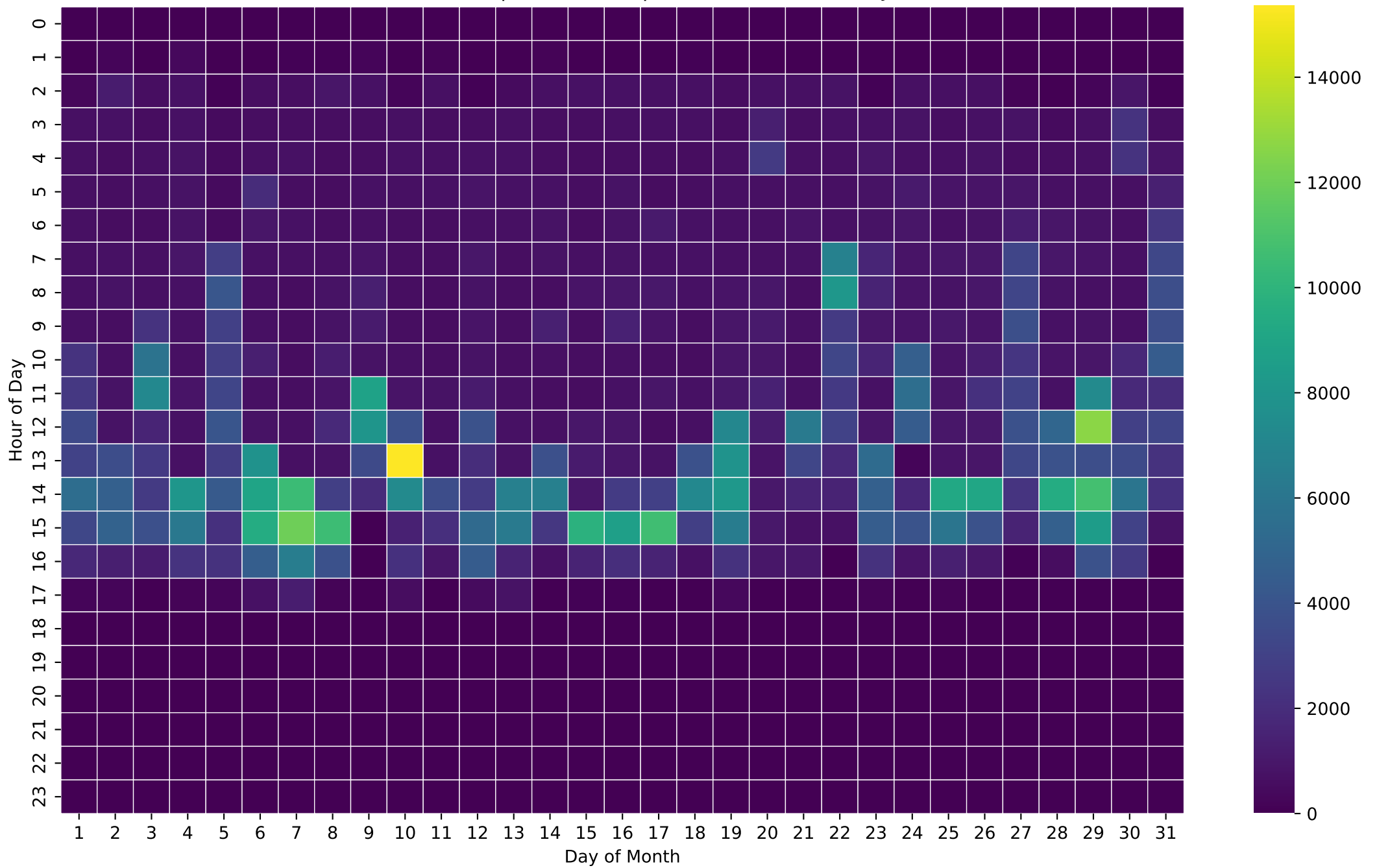
PV Self-Consumption Heatmap (Wh/Hour) - 26kWh - Jul
