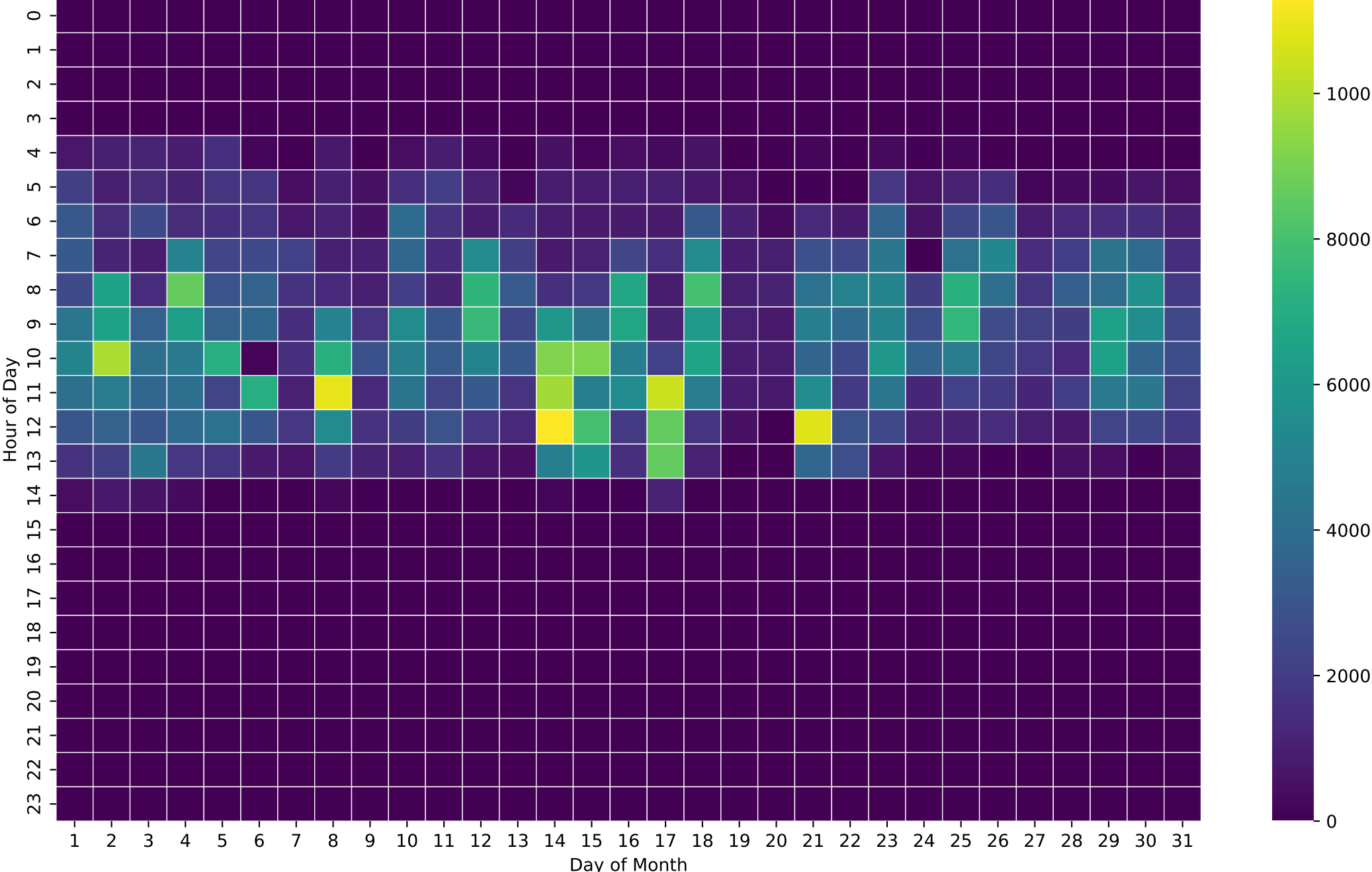
PV Self-Consumption Heatmap (Wh/Hour) - 26kWh - Oct
