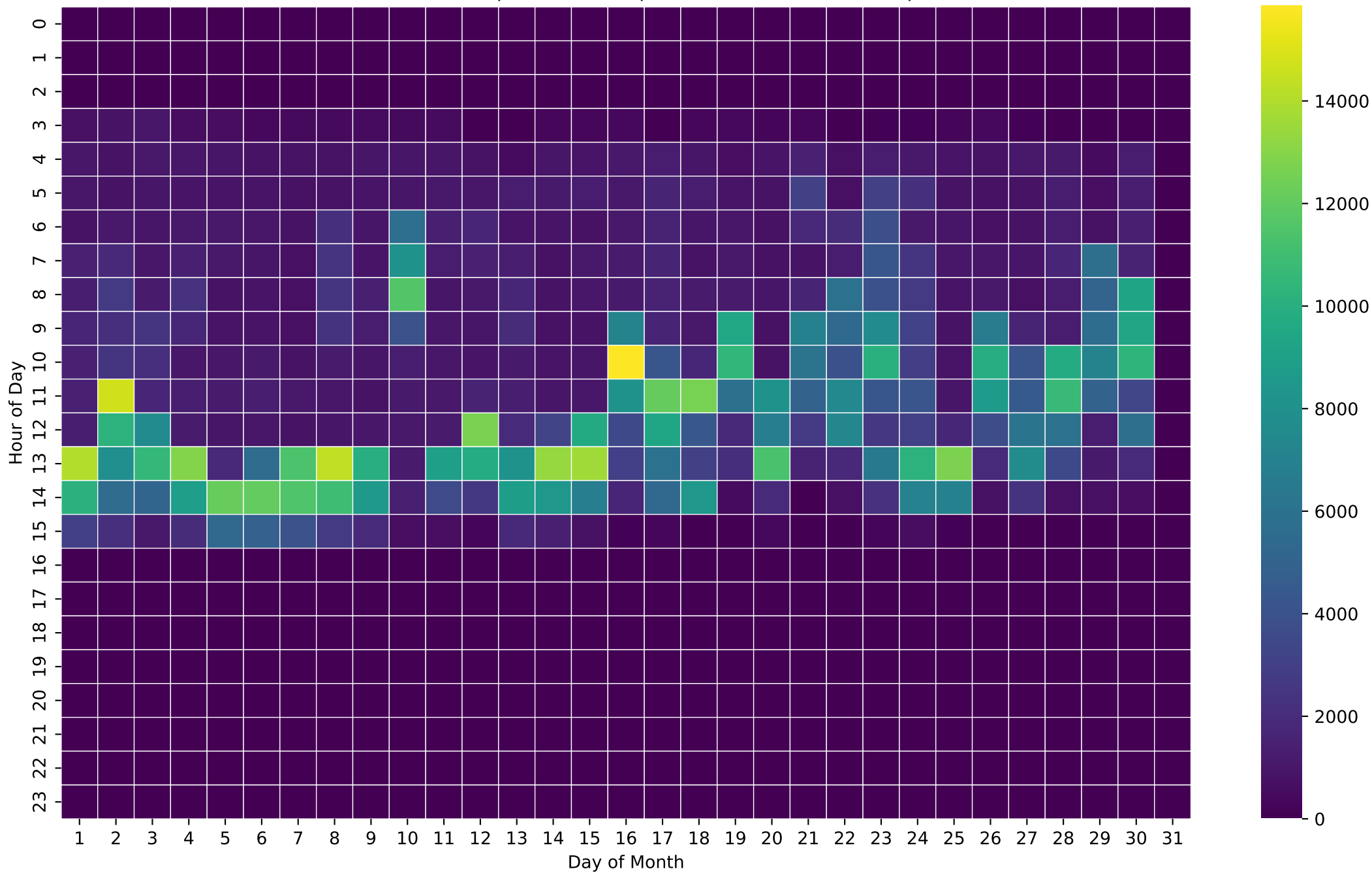
PV Self-Consumption Heatmap (Wh/Hour) - 26kWh - Sep
