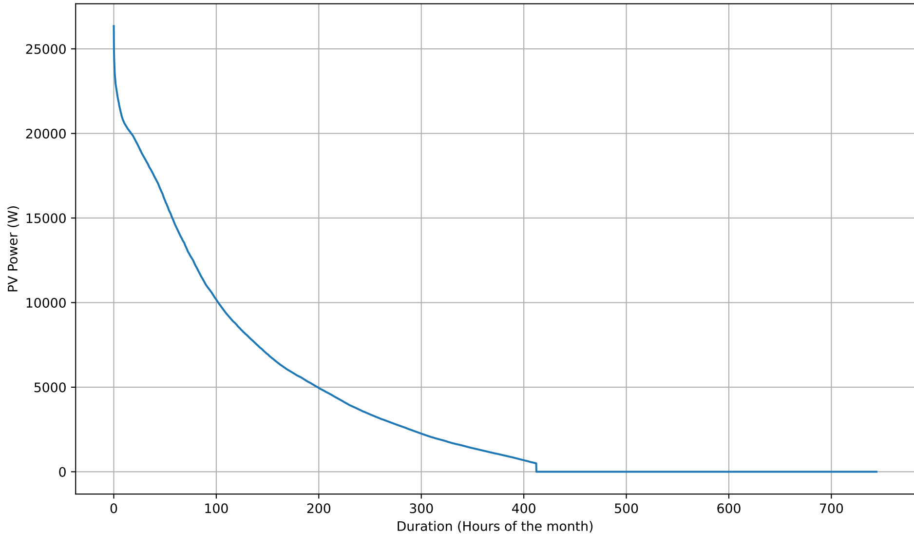
PV Production Duration Curve - 26kWh - Aug
