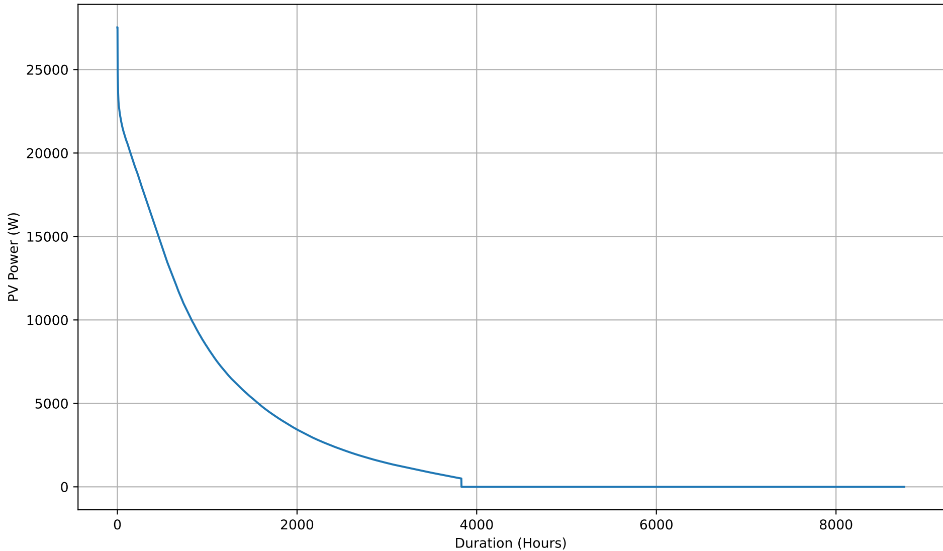
Yearly PV Production Duration Curve - 26kWh
