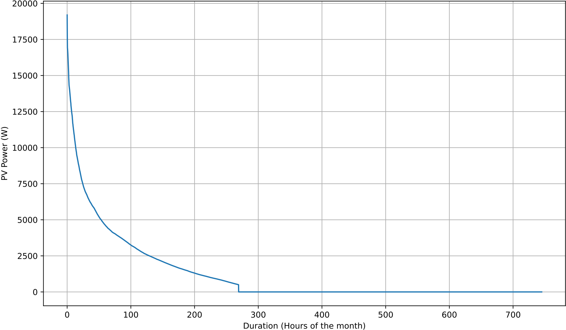
PV Production Duration Curve - 26kWh - Oct
