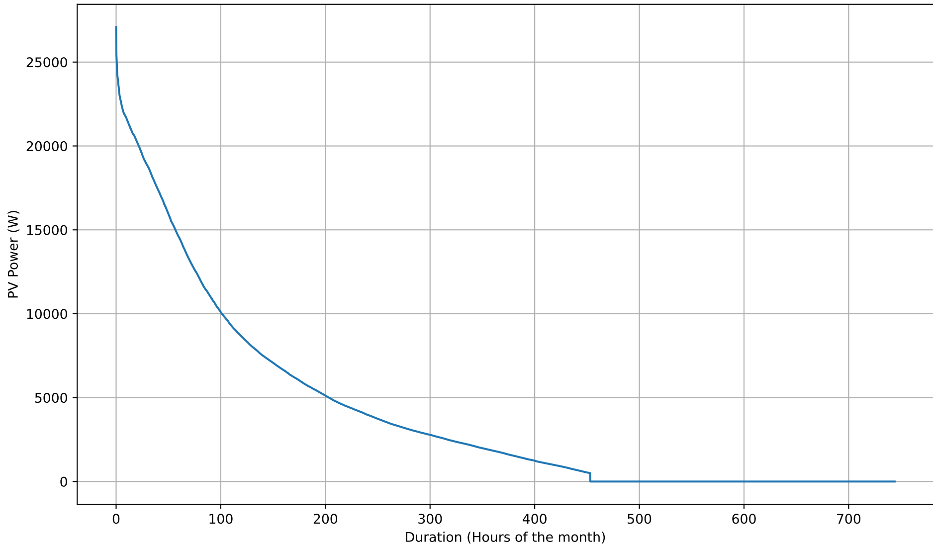
PV Production Duration Curve - 26kWh - Jul
