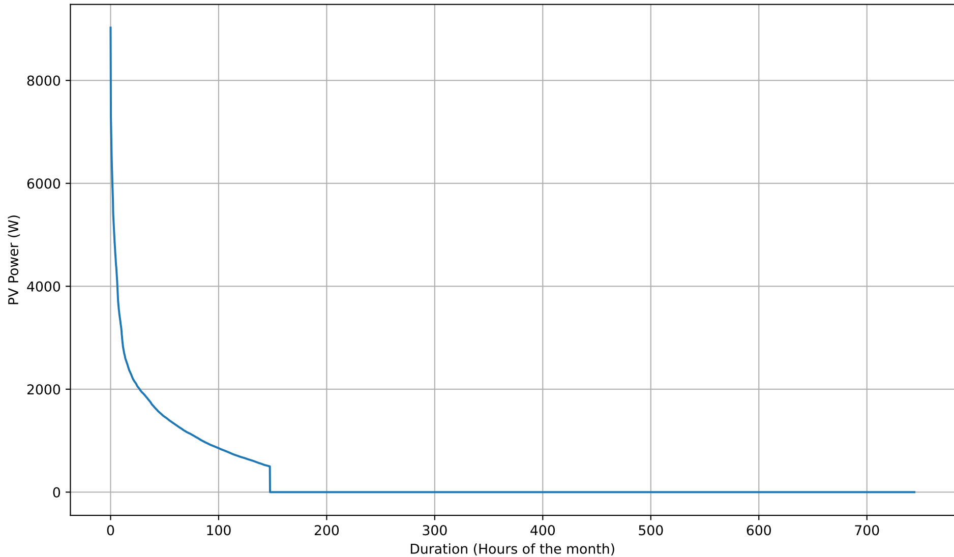
PV Production Duration Curve - 26kWh - Dec
