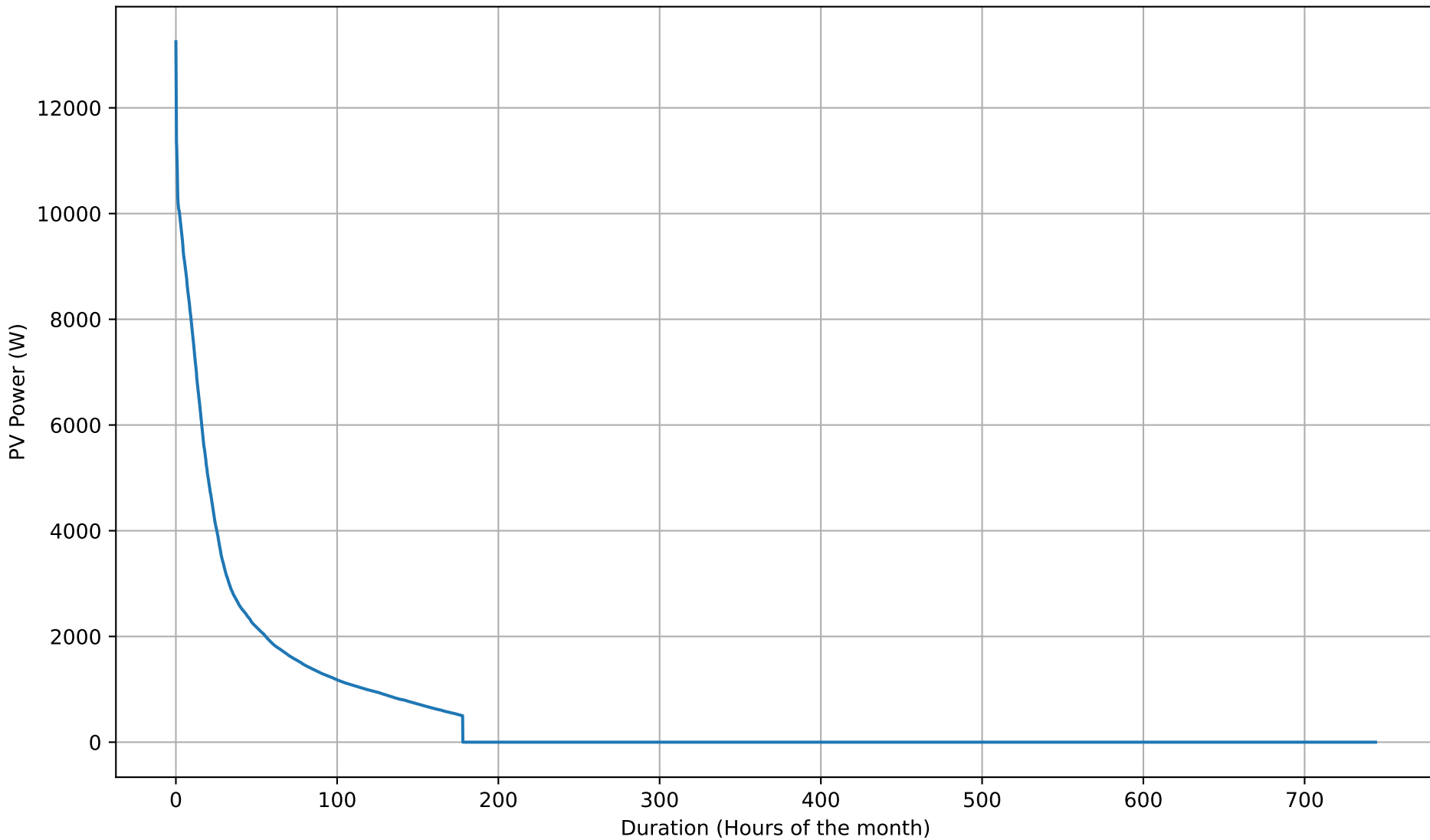
PV Production Duration Curve - 26kWh - Jan
