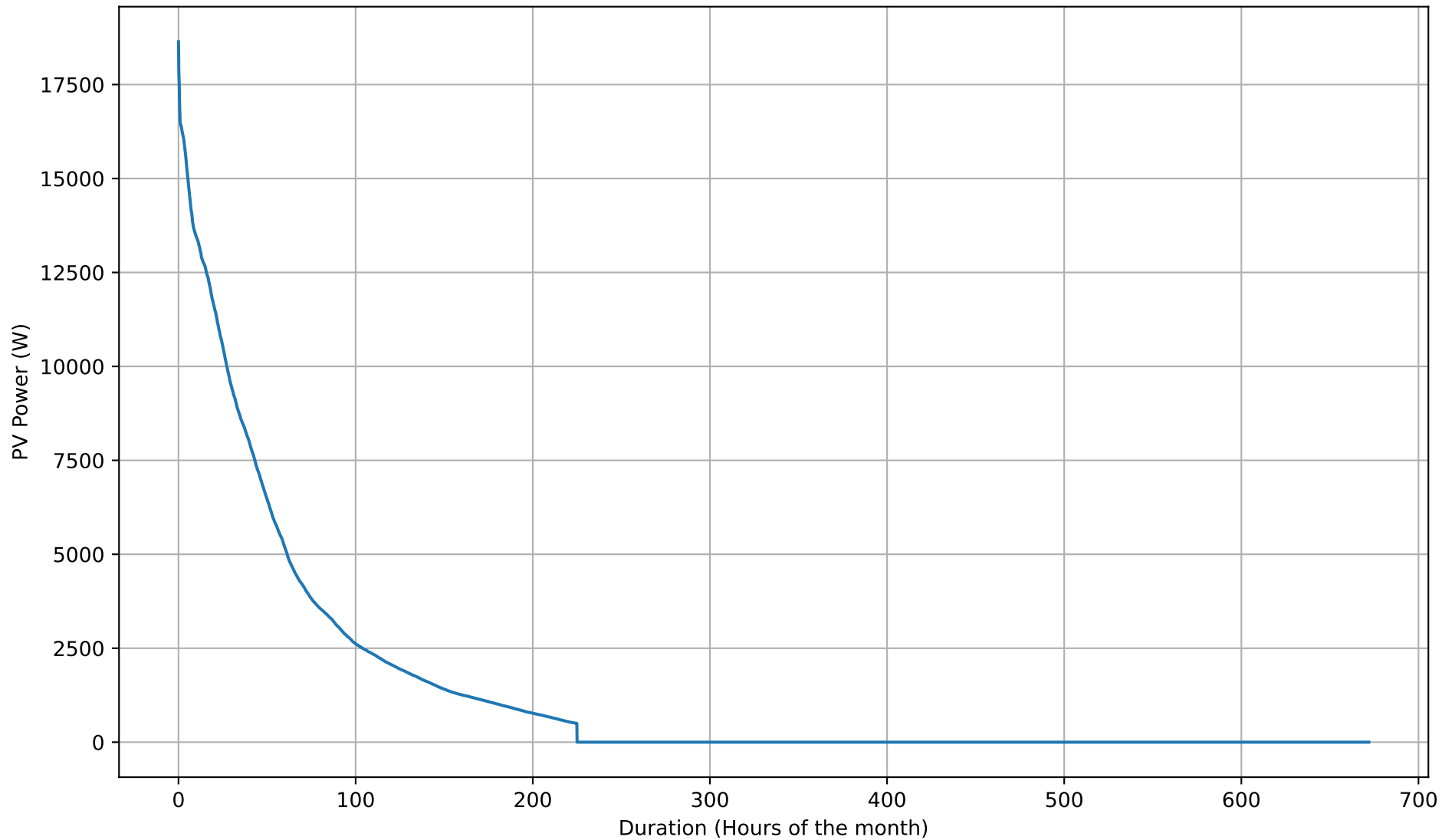
PV Production Duration Curve - 26kWh - Feb
