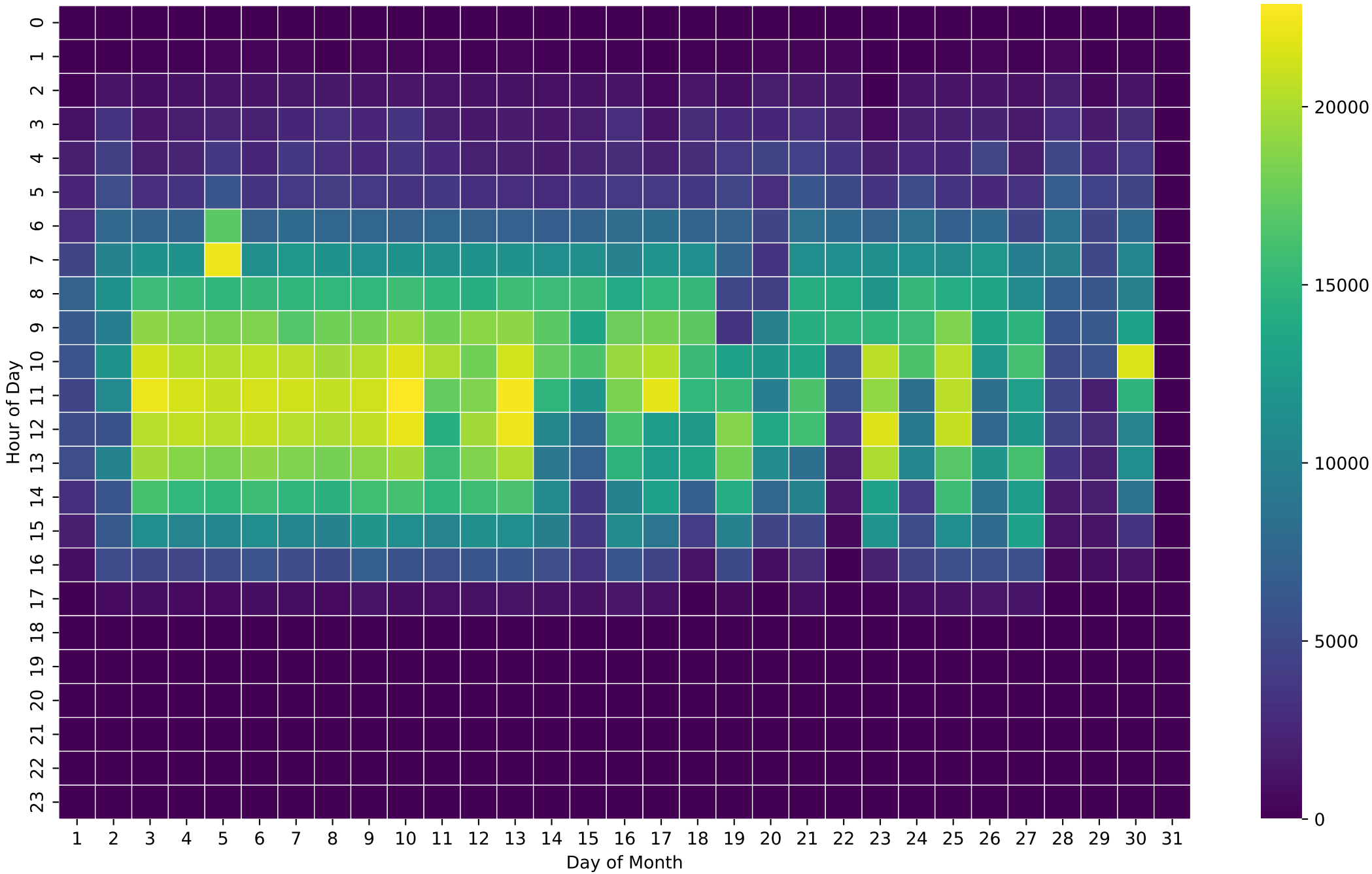
PV Production Heatmap (Wh/Hour) - 26kWh - Jun
