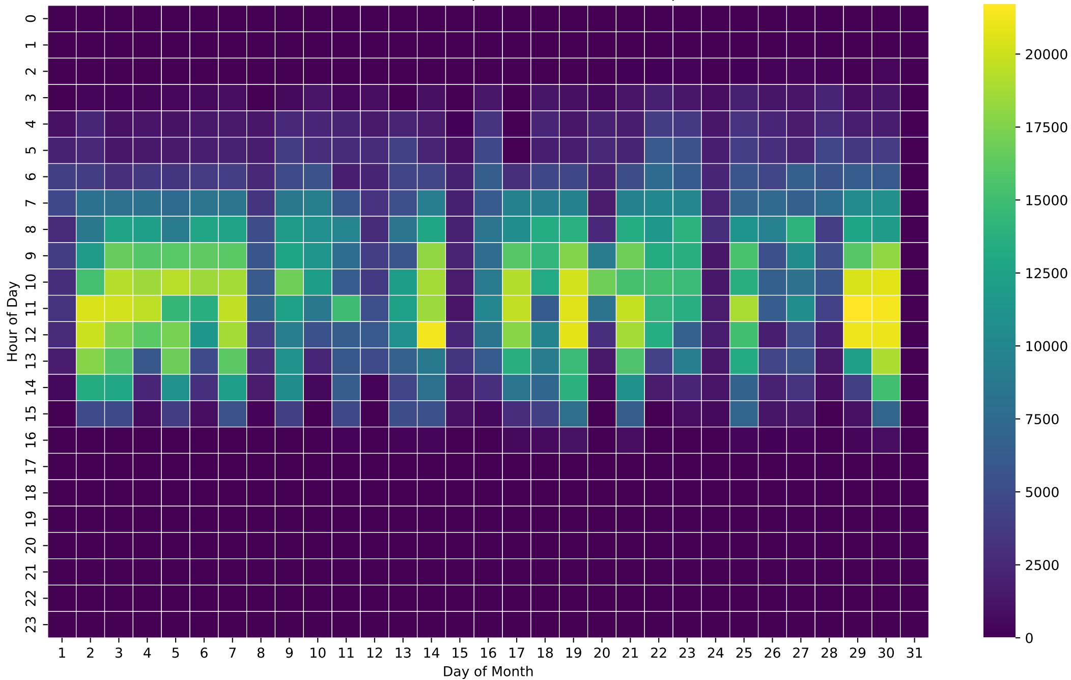
PV Production Heatmap (Wh/Hour) - 26kWh - Apr
