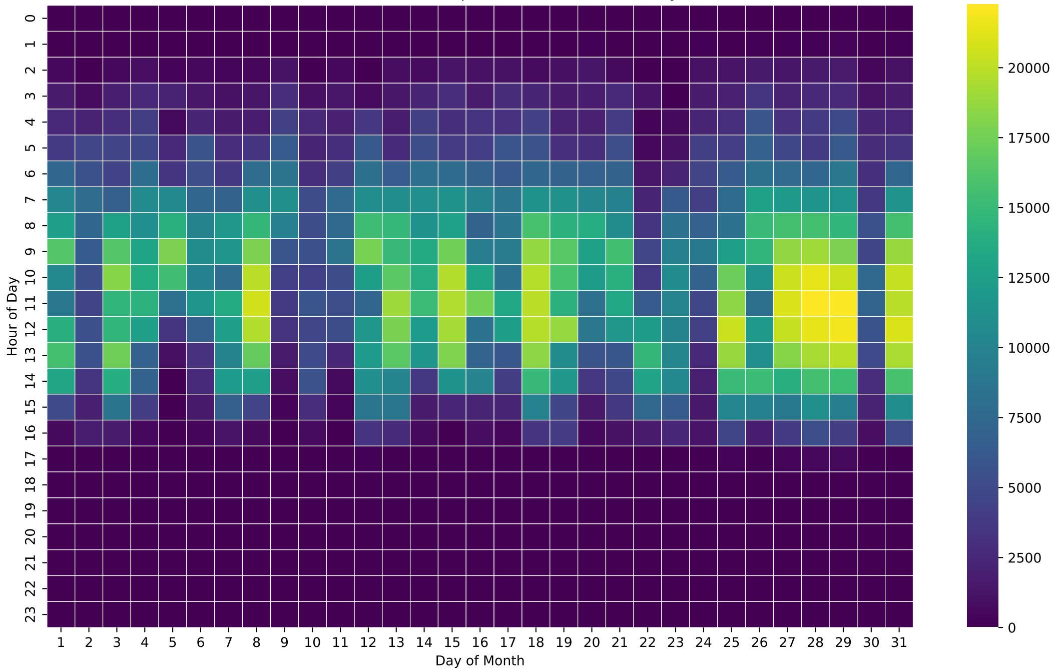
PV Production Heatmap (Wh/Hour) - 26kWh - May
