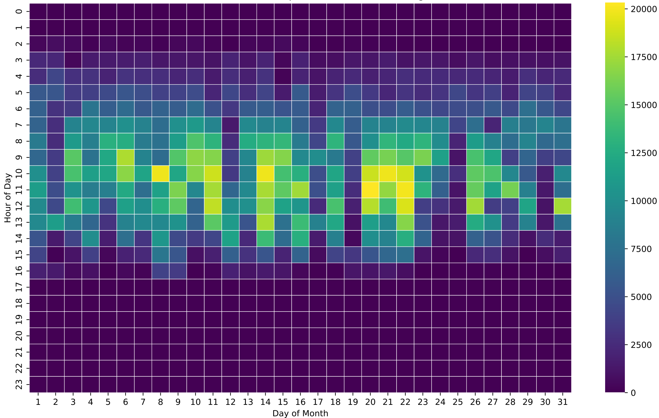
PV Production Heatmap (Wh/Hour) - 26kWh - Aug
