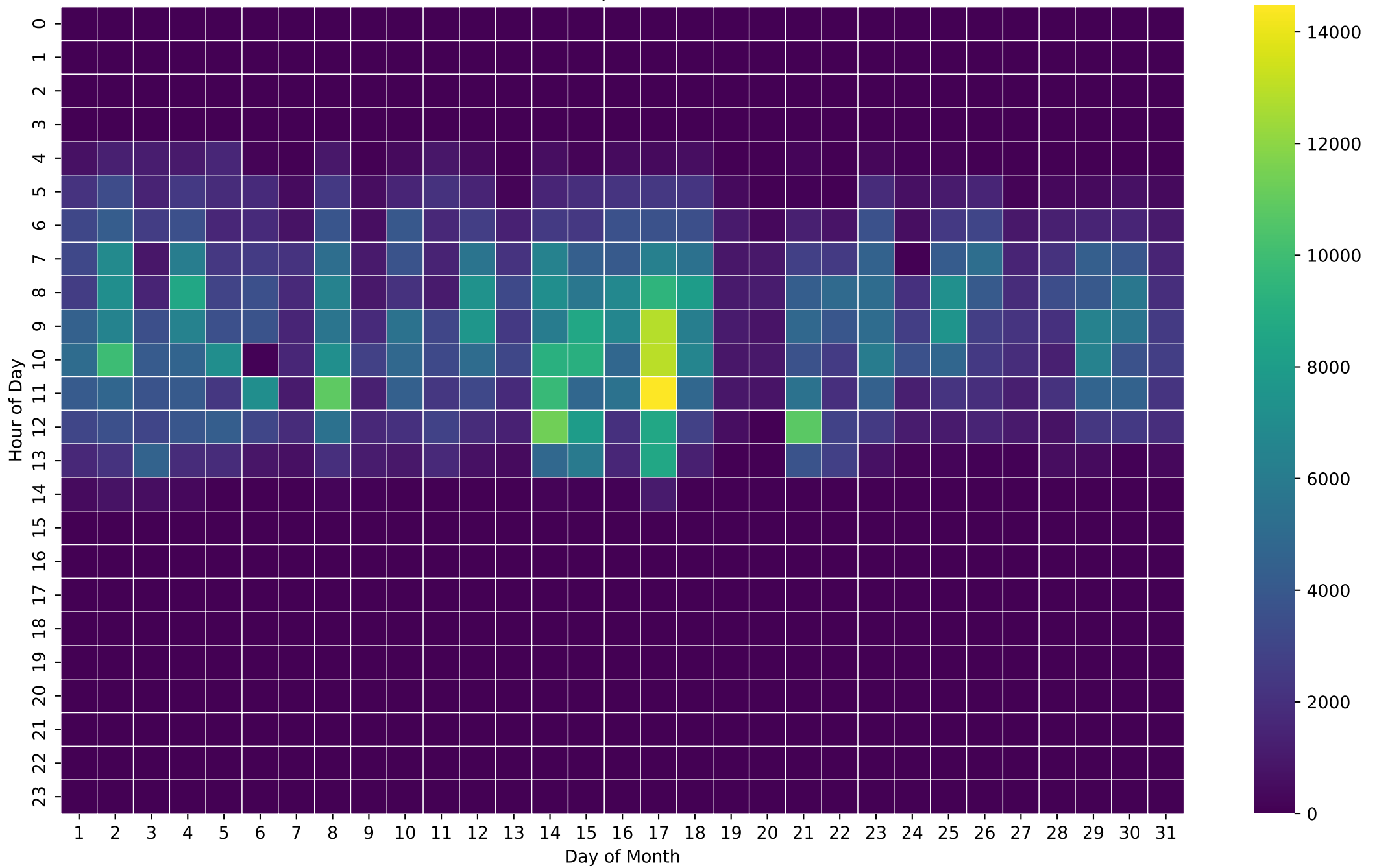
PV Production Heatmap (Wh/Hour) - 26kWh - Oct
