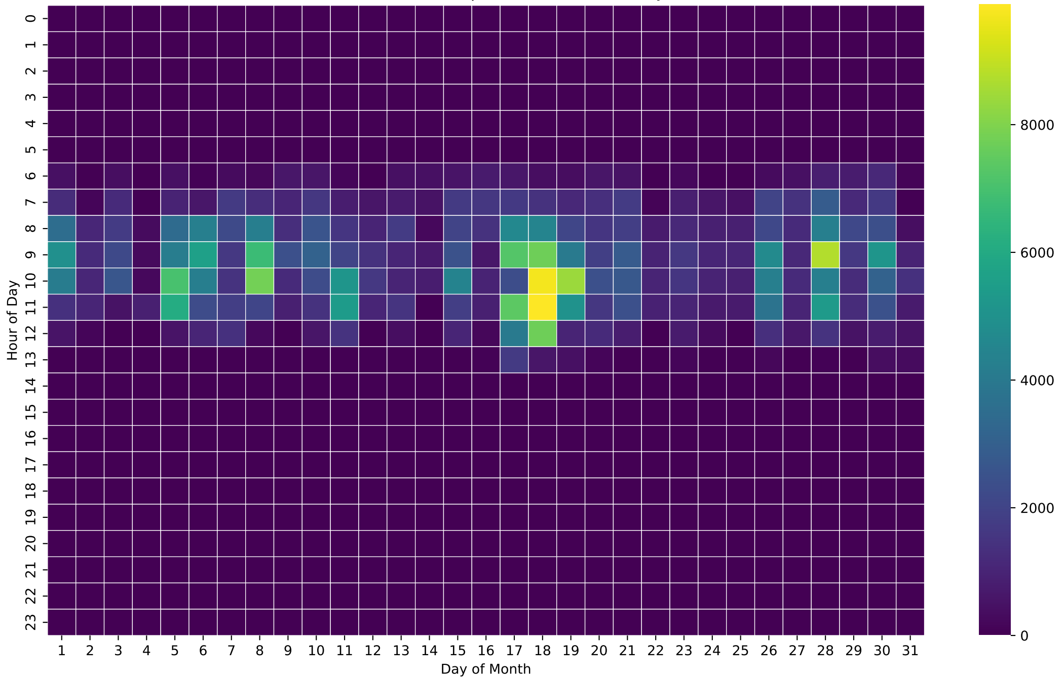
PV Production Heatmap (Wh/Hour) - 26kWh - Jan
