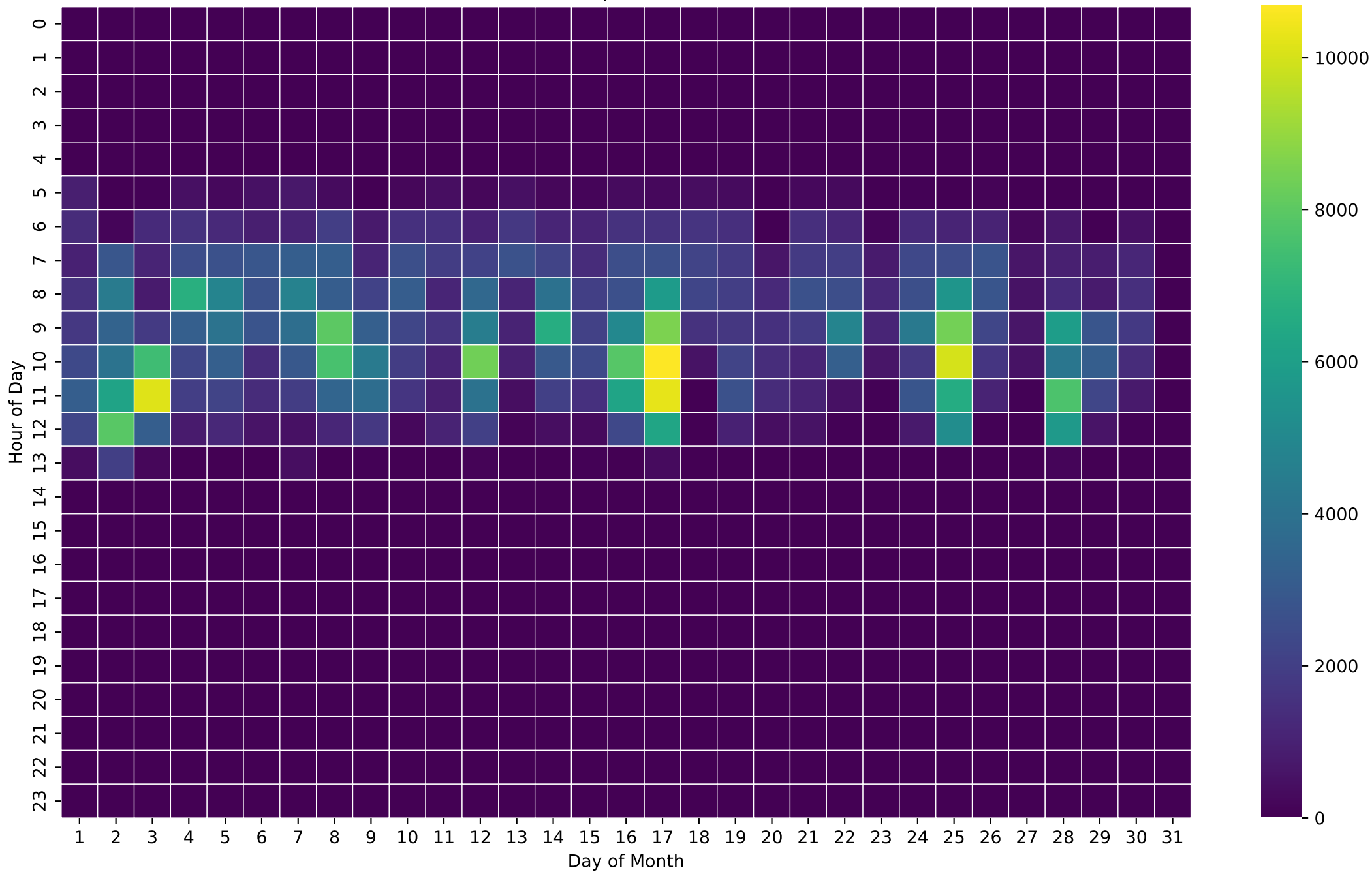
PV Production Heatmap (Wh/Hour) - 26kWh - Nov
