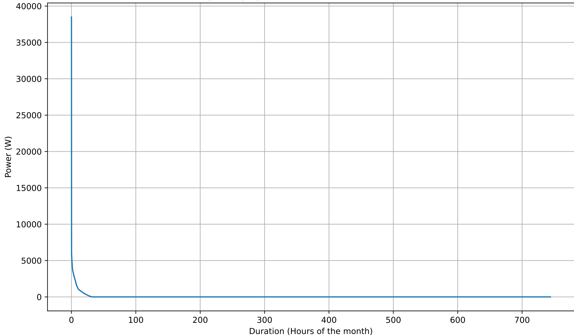
Battery Charging Power Duration Curve - 50kWh - Dec
