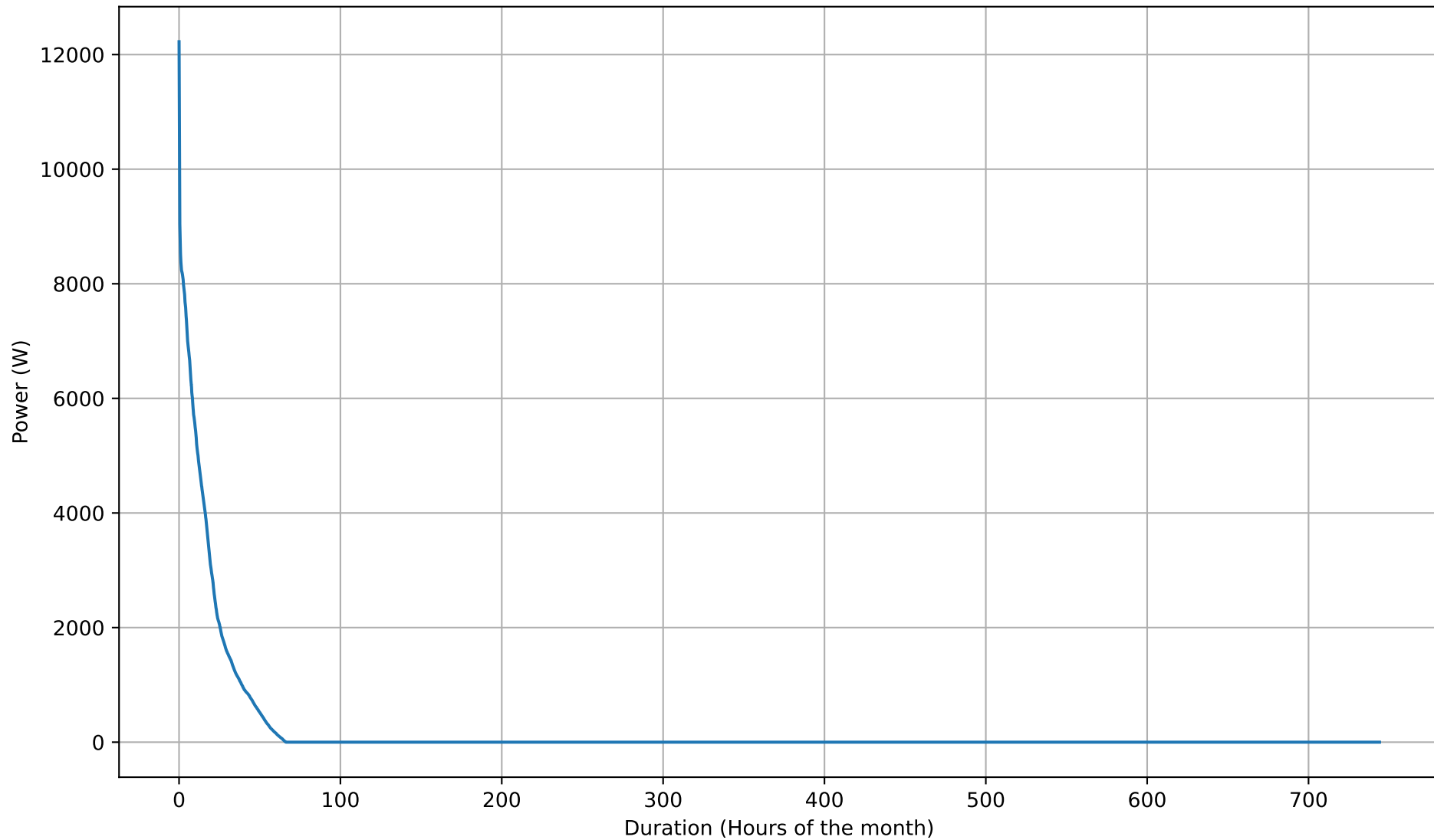
Battery Charging Power Duration Curve - 50kWh - Jan
