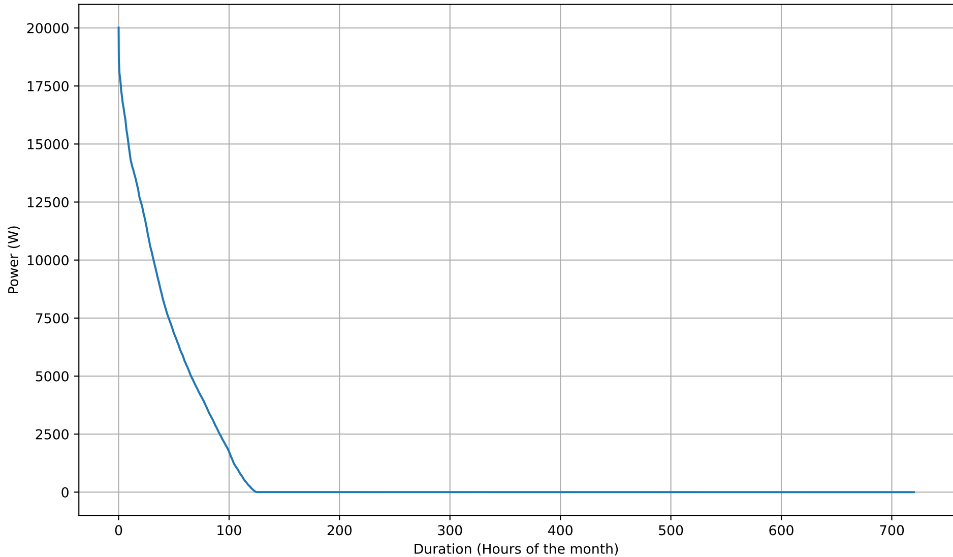
Battery Charging Power Duration Curve - 50kWh - Sep
