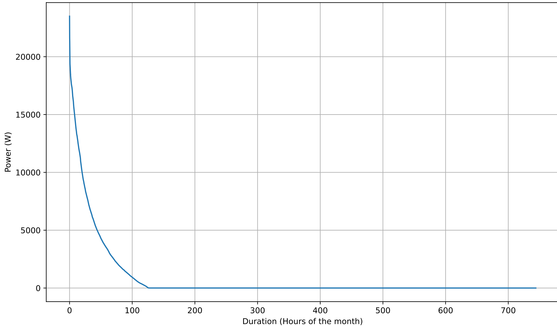
Battery Charging Power Duration Curve - 50kWh - Aug
