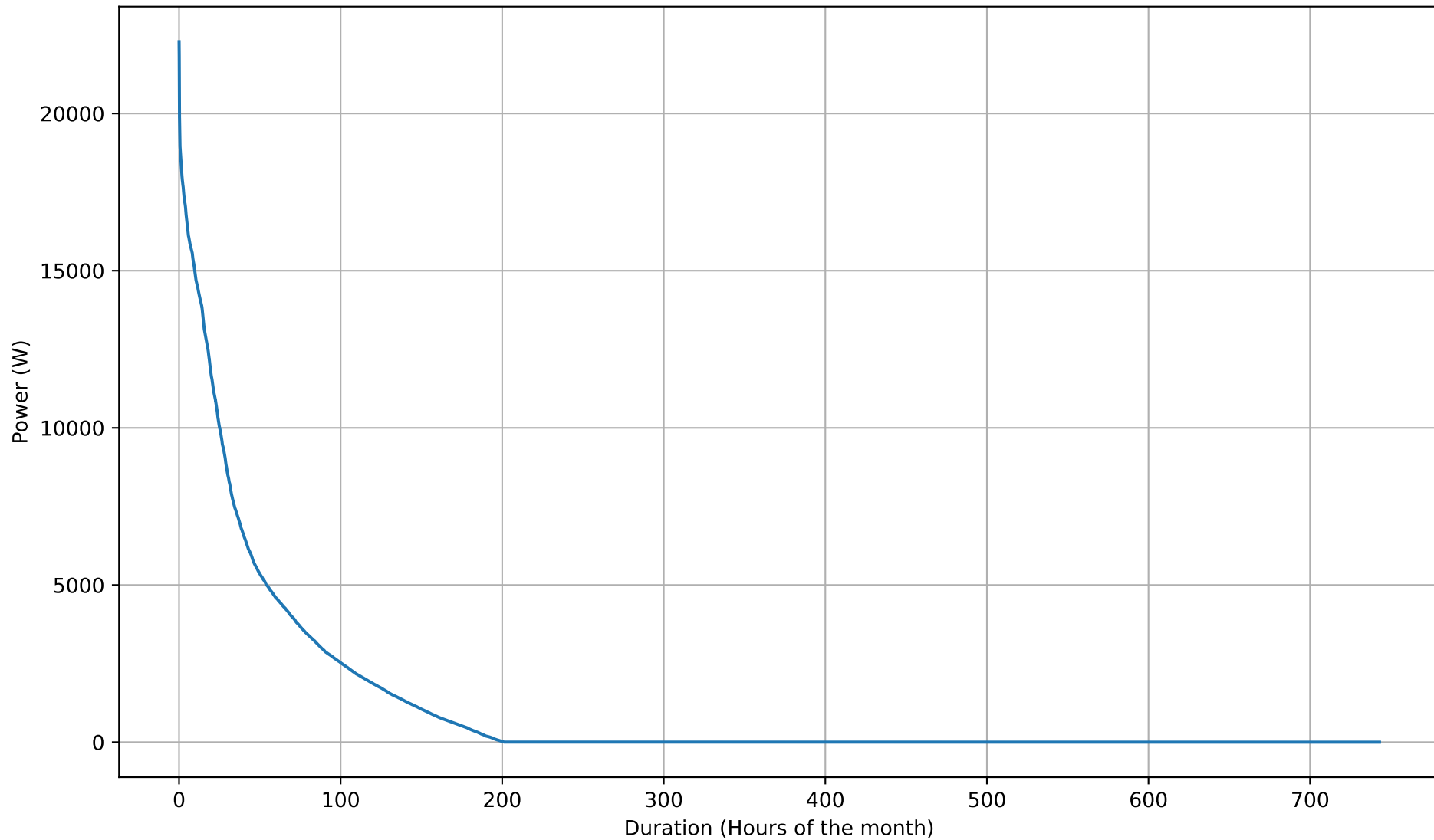
Battery Charging Power Duration Curve - 50kWh - Mar
