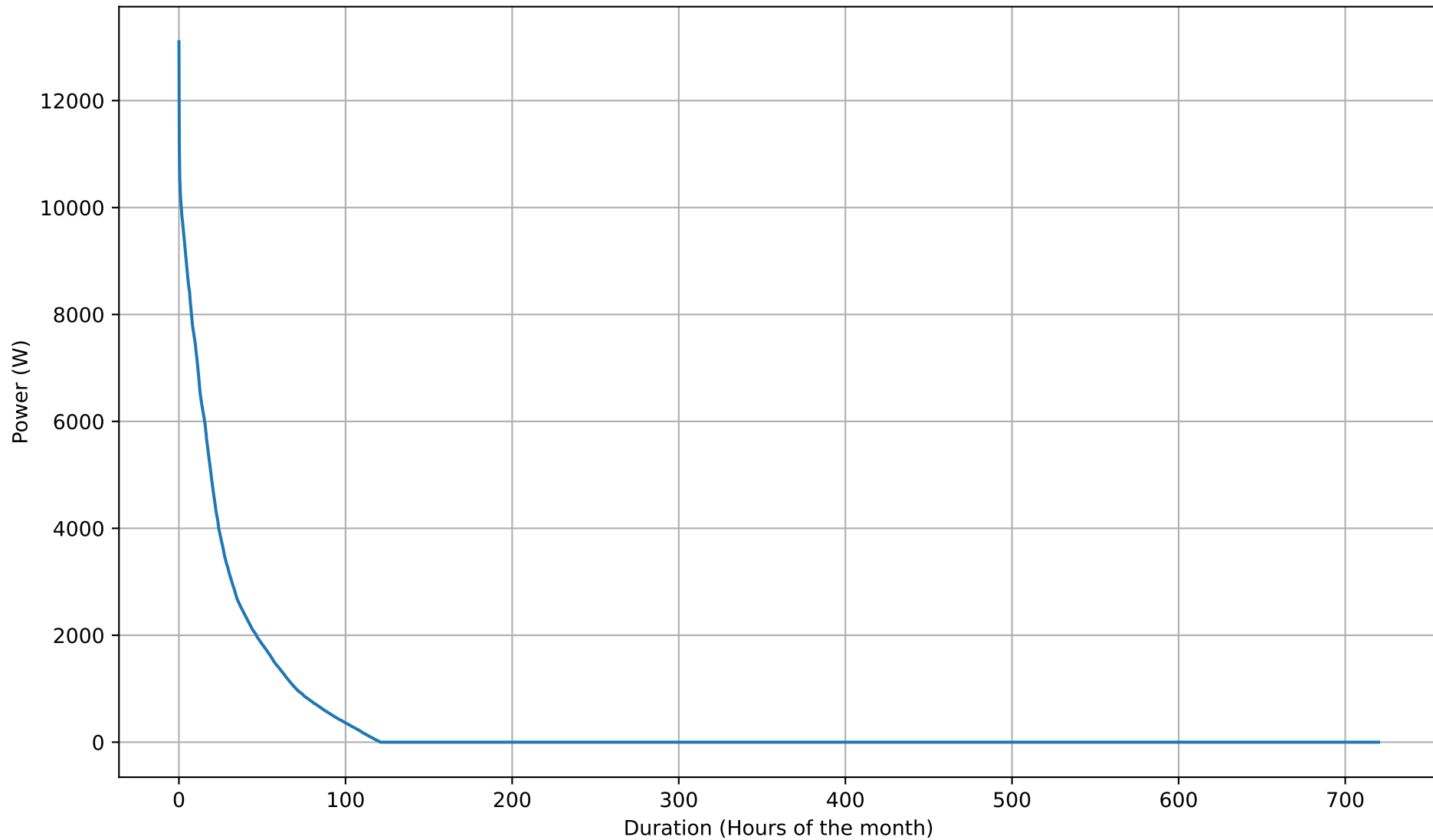
Battery Charging Power Duration Curve - 50kWh - Nov
