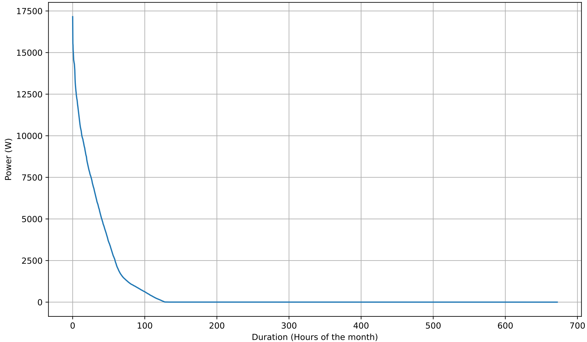
Battery Charging Power Duration Curve - 50kWh - Feb
