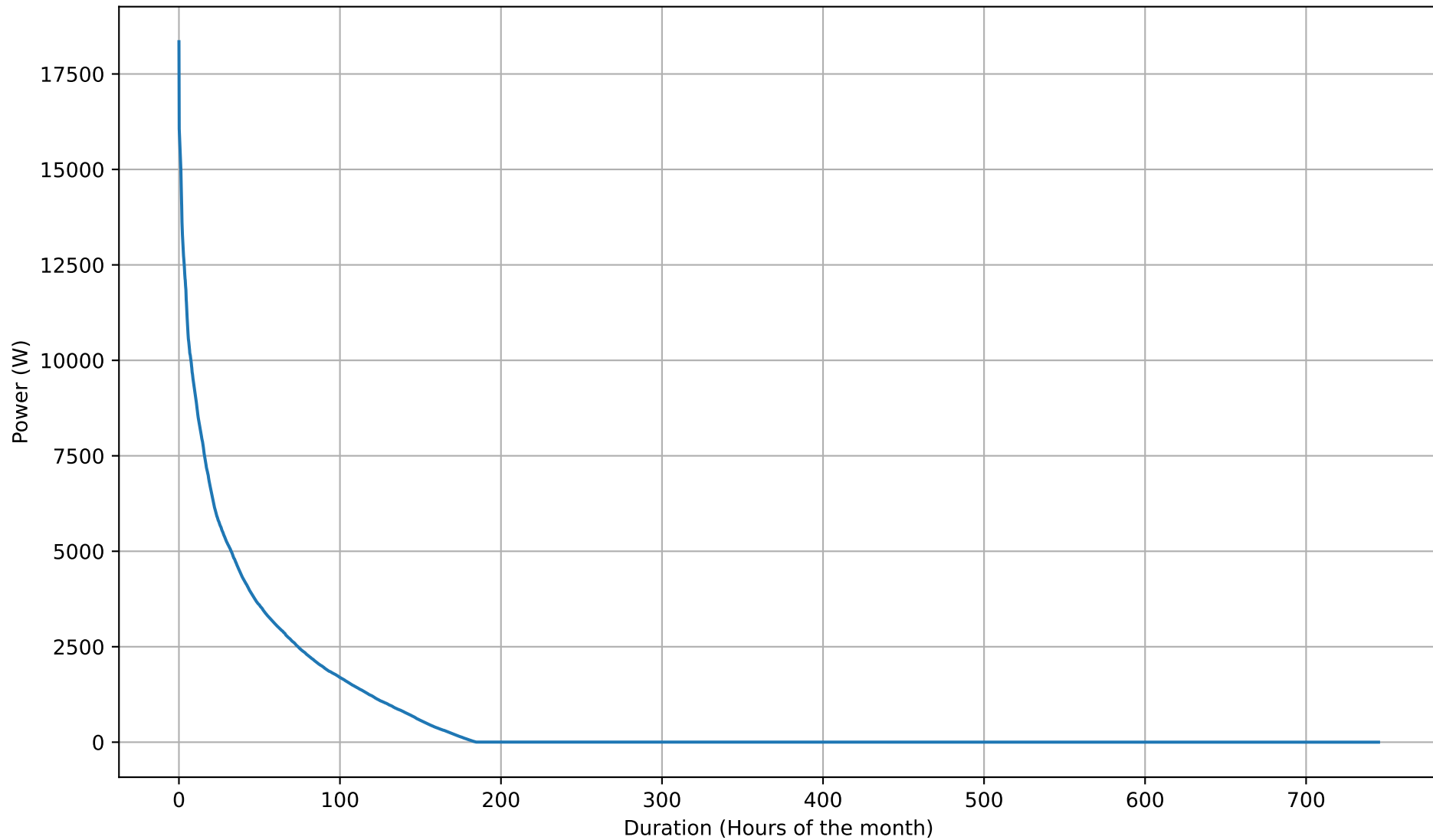
Battery Charging Power Duration Curve - 50kWh - Oct
