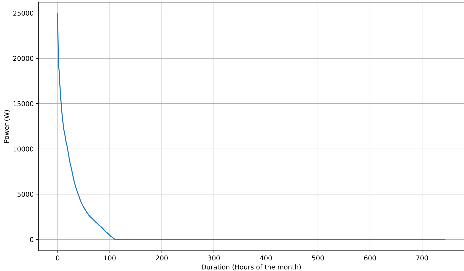
Battery Charging Power Duration Curve - 50kWh - Jul
