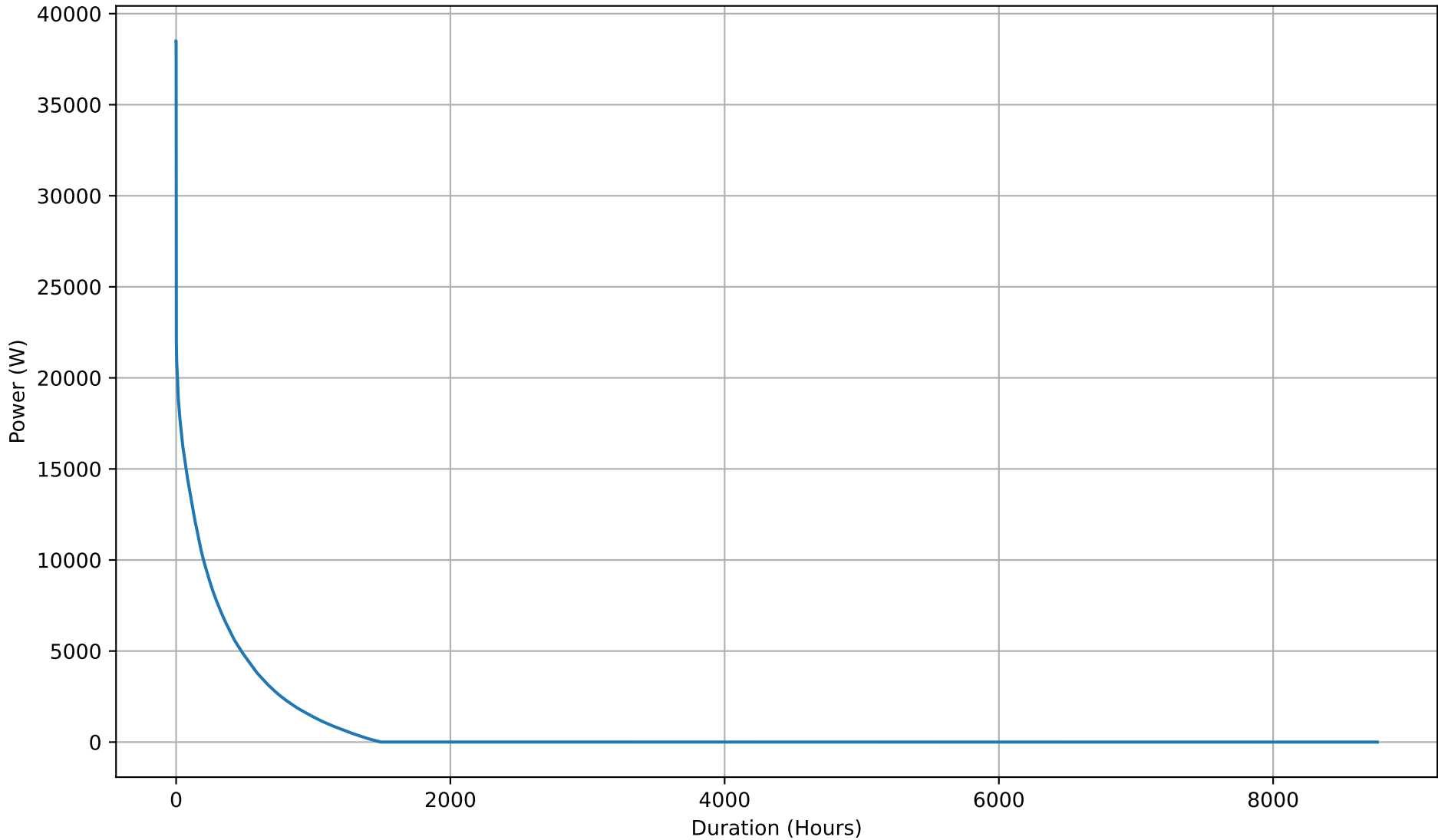
Yearly Battery Charging Power Duration Curve - 50kWh
