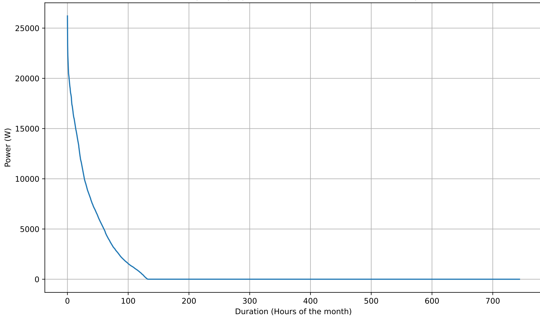
Battery Charging Power Duration Curve - 50kWh - May
