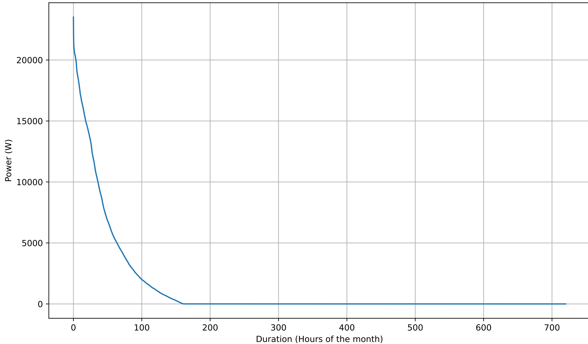
Battery Charging Power Duration Curve - 50kWh - Apr
