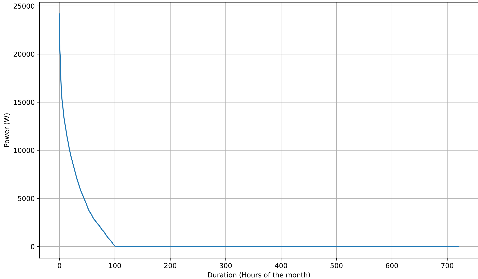
Battery Charging Power Duration Curve - 50kWh - Jun
