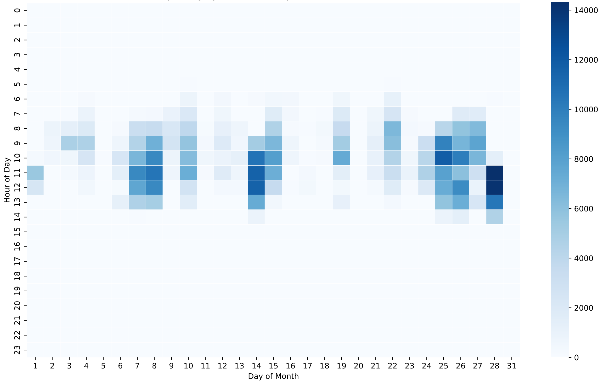
Battery Charging Power Heatmap (Wh/Hour) - 50kWh - Feb
