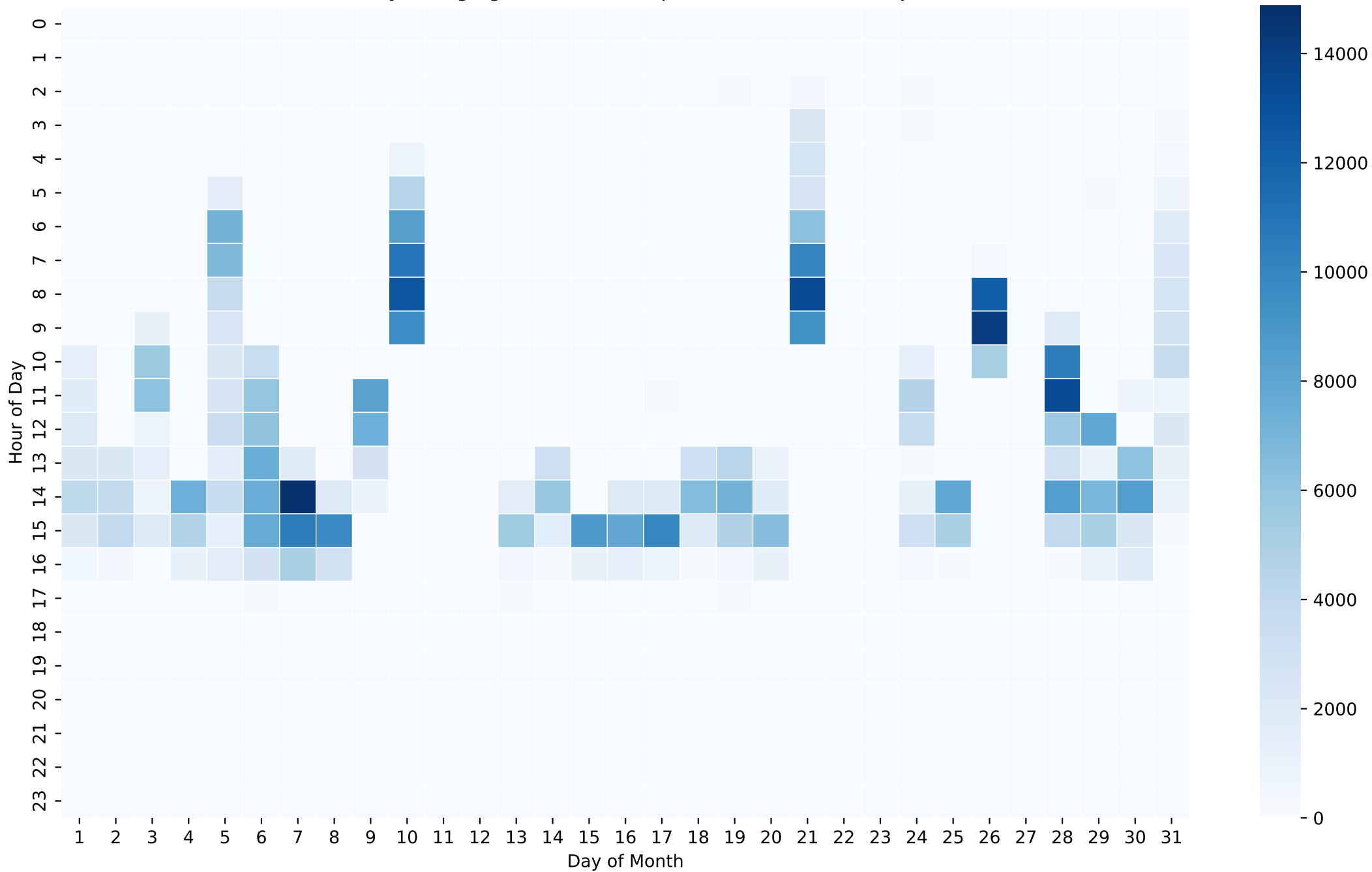
Battery Charging Power Heatmap (Wh/Hour) - 50kWh - Jul
