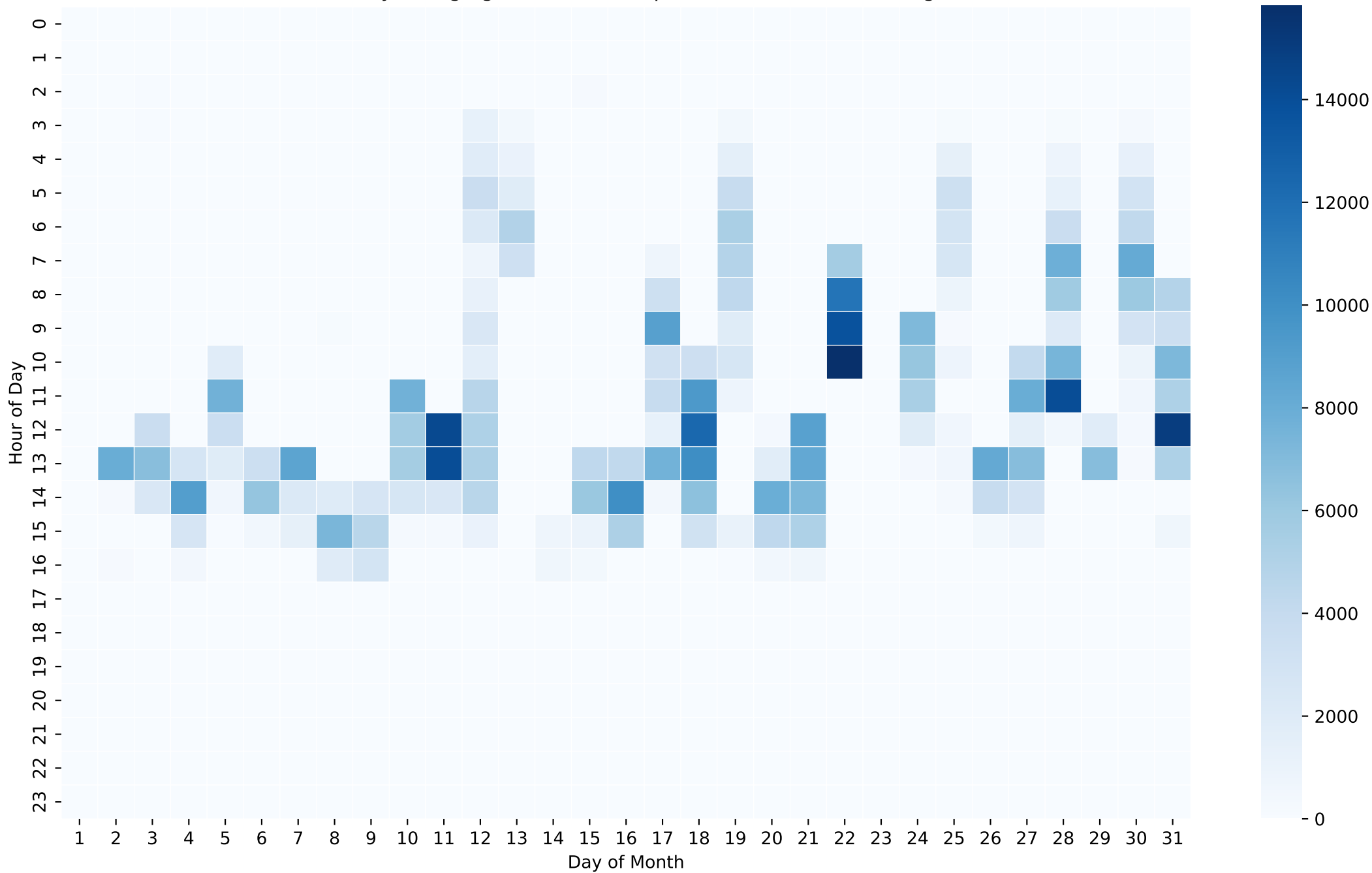
Battery Charging Power Heatmap (Wh/Hour) - 50kWh - Aug
