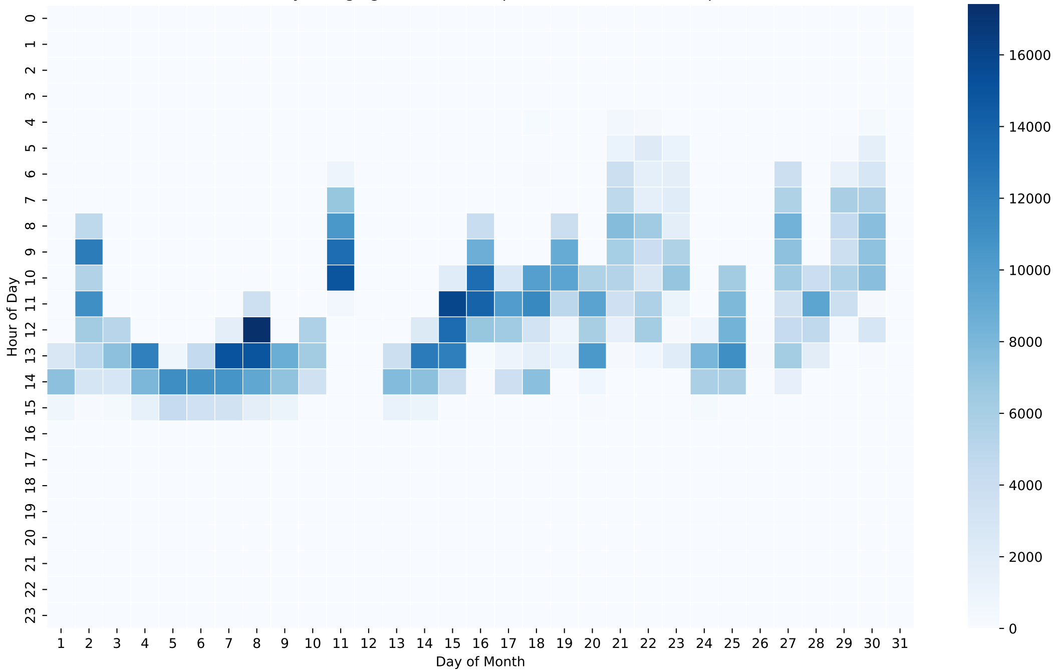
Battery Charging Power Heatmap (Wh/Hour) - 50kWh - Sep
