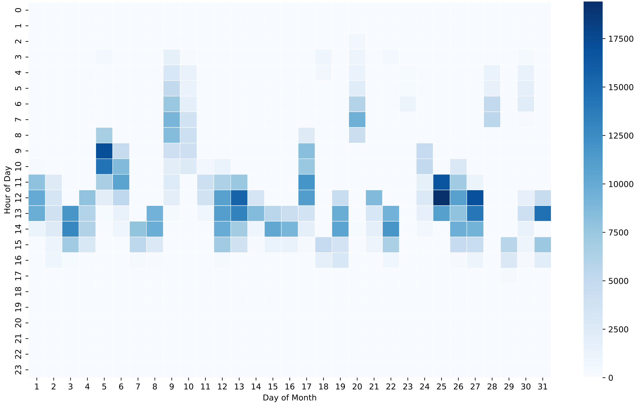
Battery Charging Power Heatmap (Wh/Hour) - 50kWh - May
