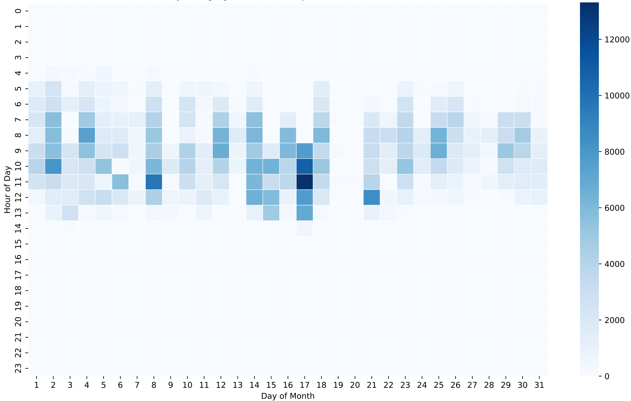
Battery Charging Power Heatmap (Wh/Hour) - 50kWh - Oct
