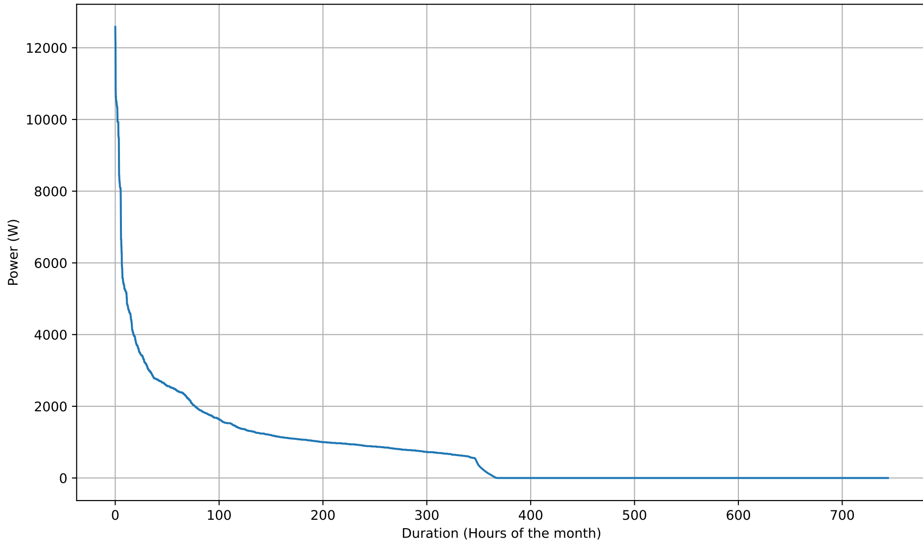
Battery Discharging Power Duration Curve - 50kWh - Aug
