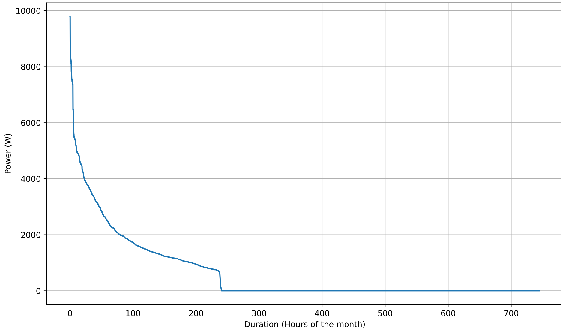
Battery Discharging Power Duration Curve - 50kWh - Oct
