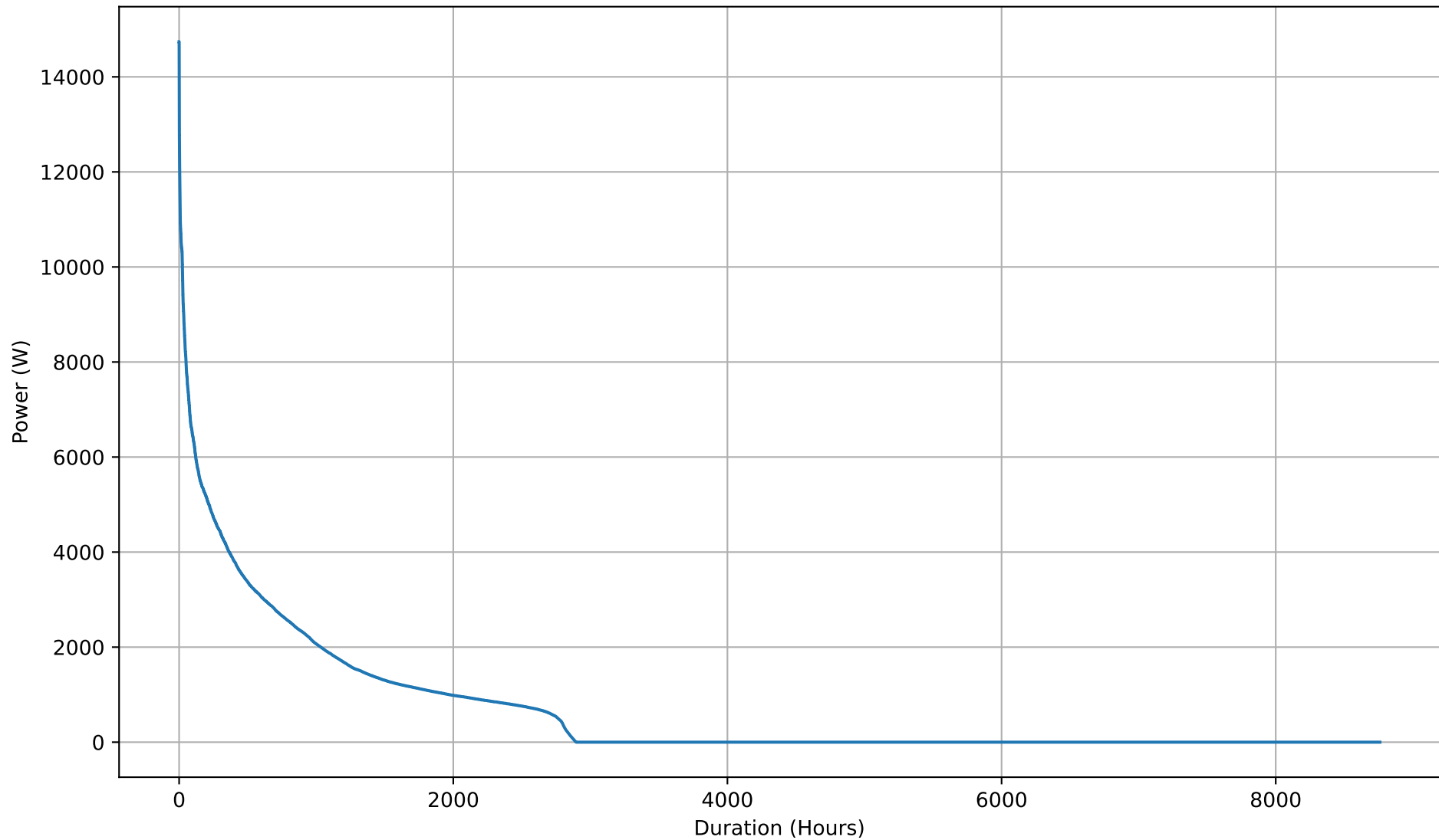
Yearly Battery Discharging Power Duration Curve - 50kWh
