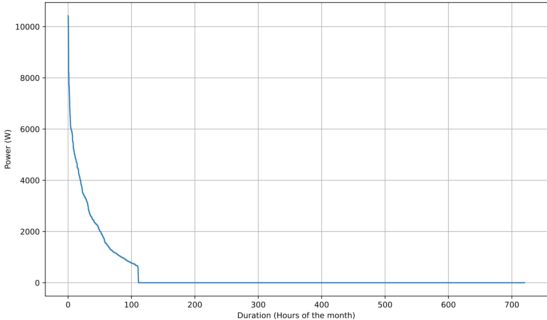
Battery Discharging Power Duration Curve - 50kWh - Nov
