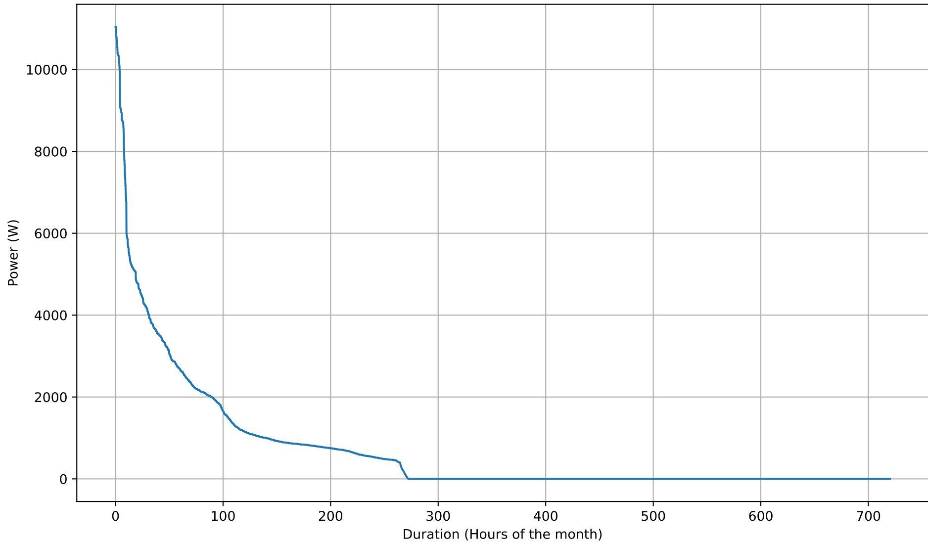
Battery Discharging Power Duration Curve - 50kWh - Jun
