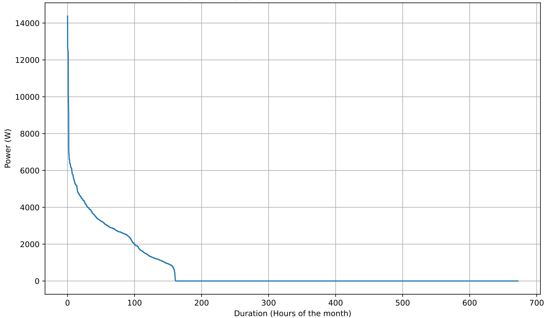
Battery Discharging Power Duration Curve - 50kWh - Feb
