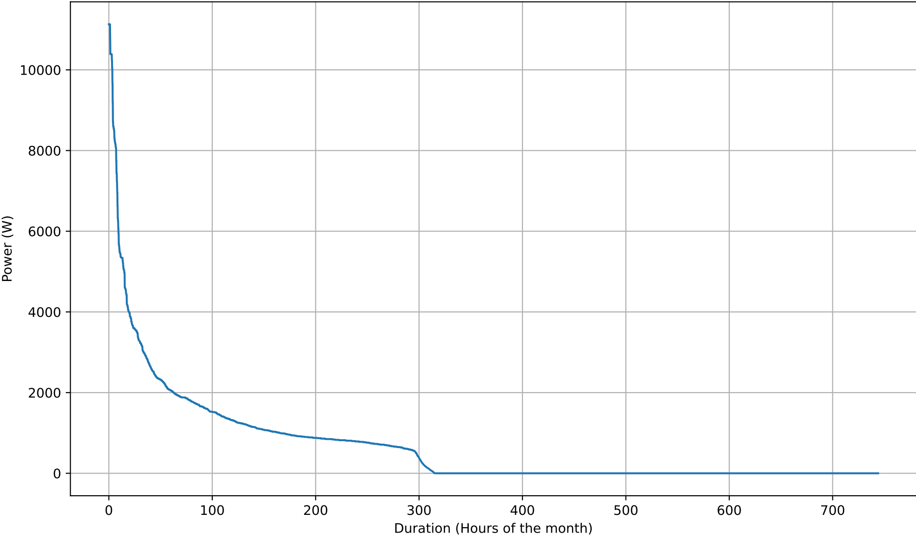
Battery Discharging Power Duration Curve - 50kWh - Jul
