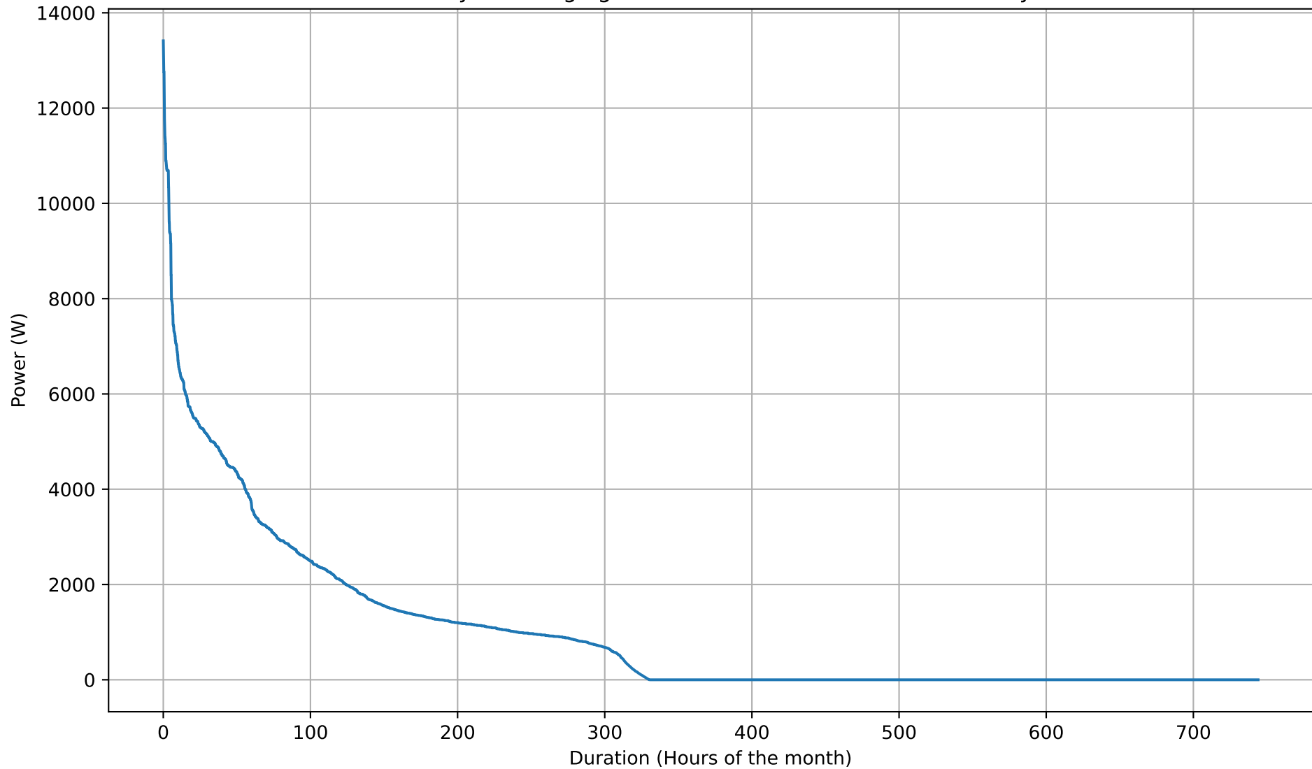
Battery Discharging Power Duration Curve - 50kWh - May
