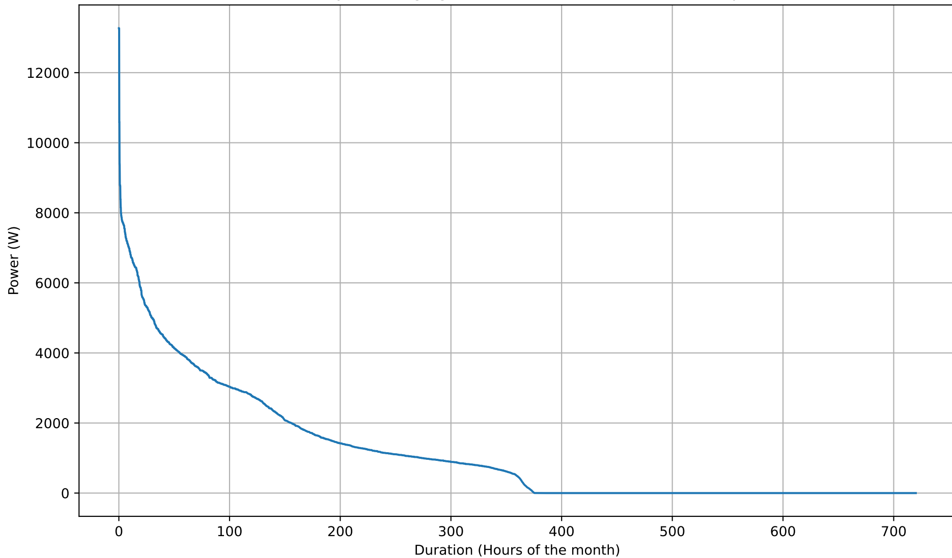
Battery Discharging Power Duration Curve - 50kWh - Apr
