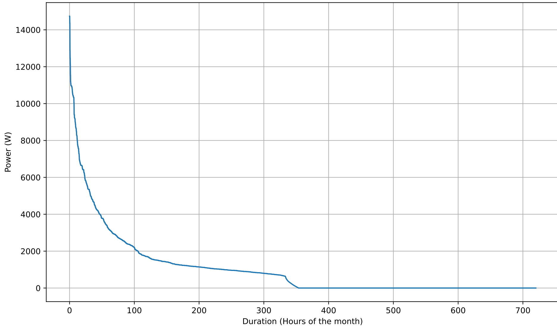
Battery Discharging Power Duration Curve - 50kWh - Sep
