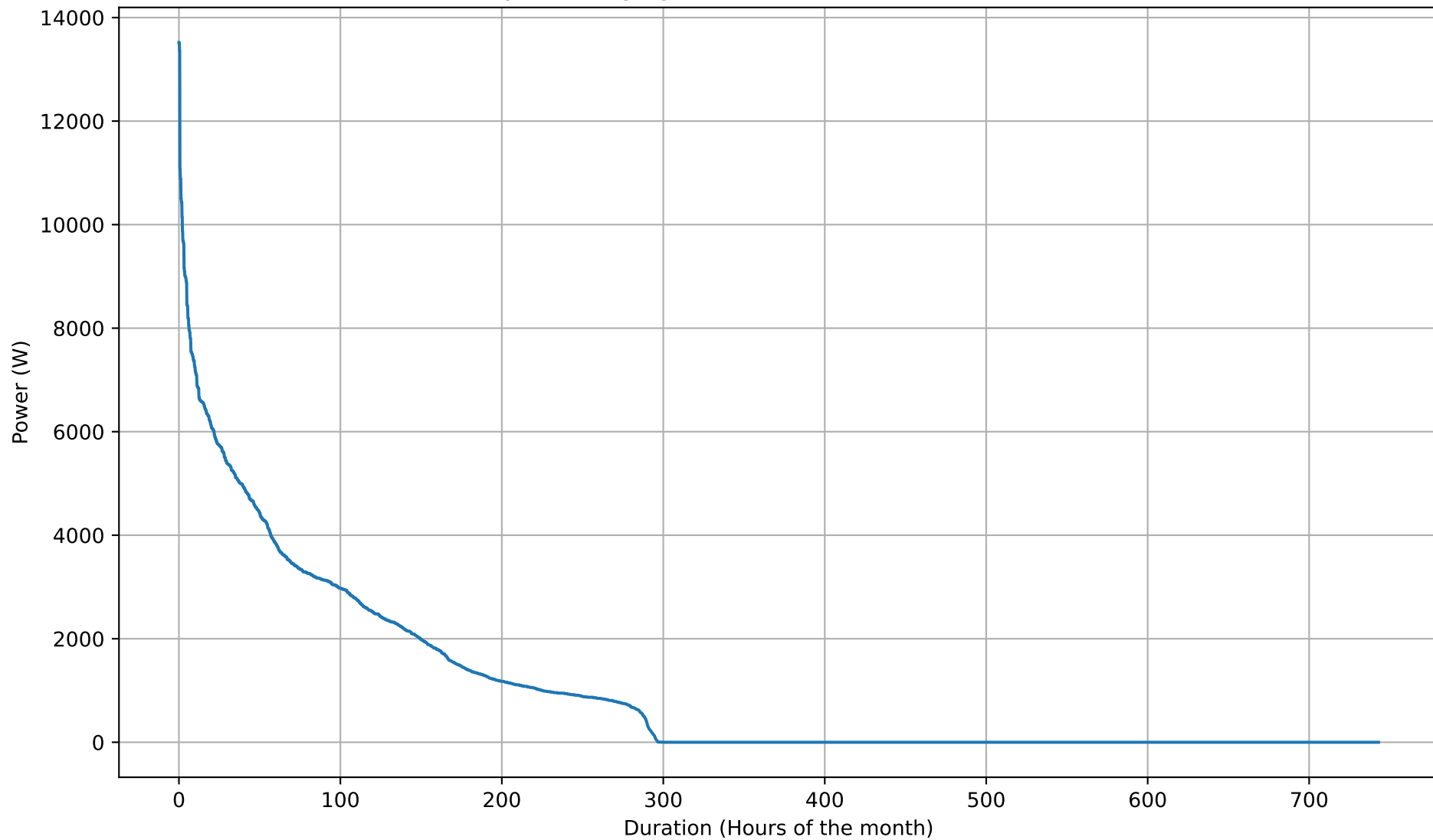
Battery Discharging Power Duration Curve - 50kWh - Mar
