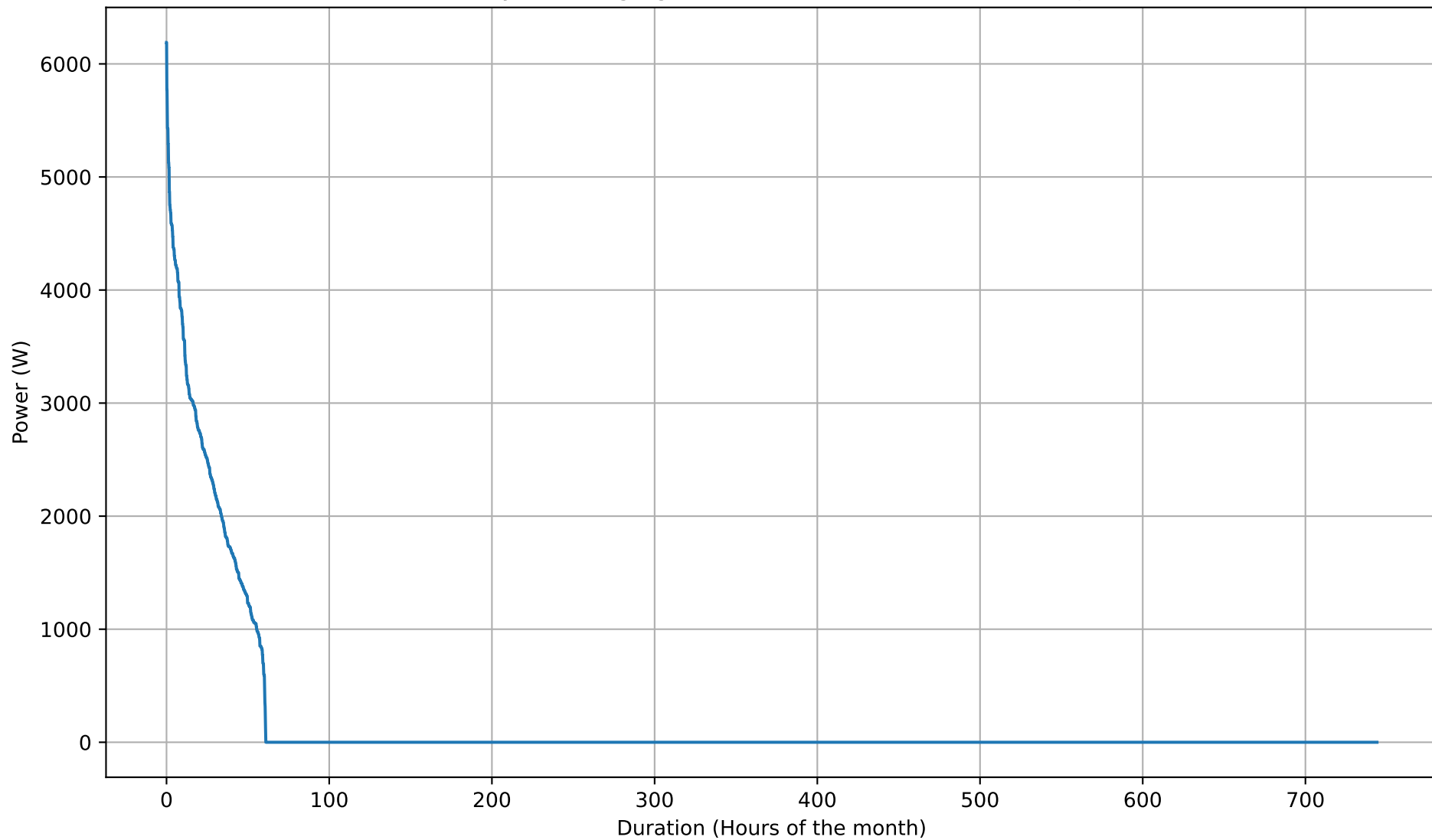
Battery Discharging Power Duration Curve - 50kWh - Jan
