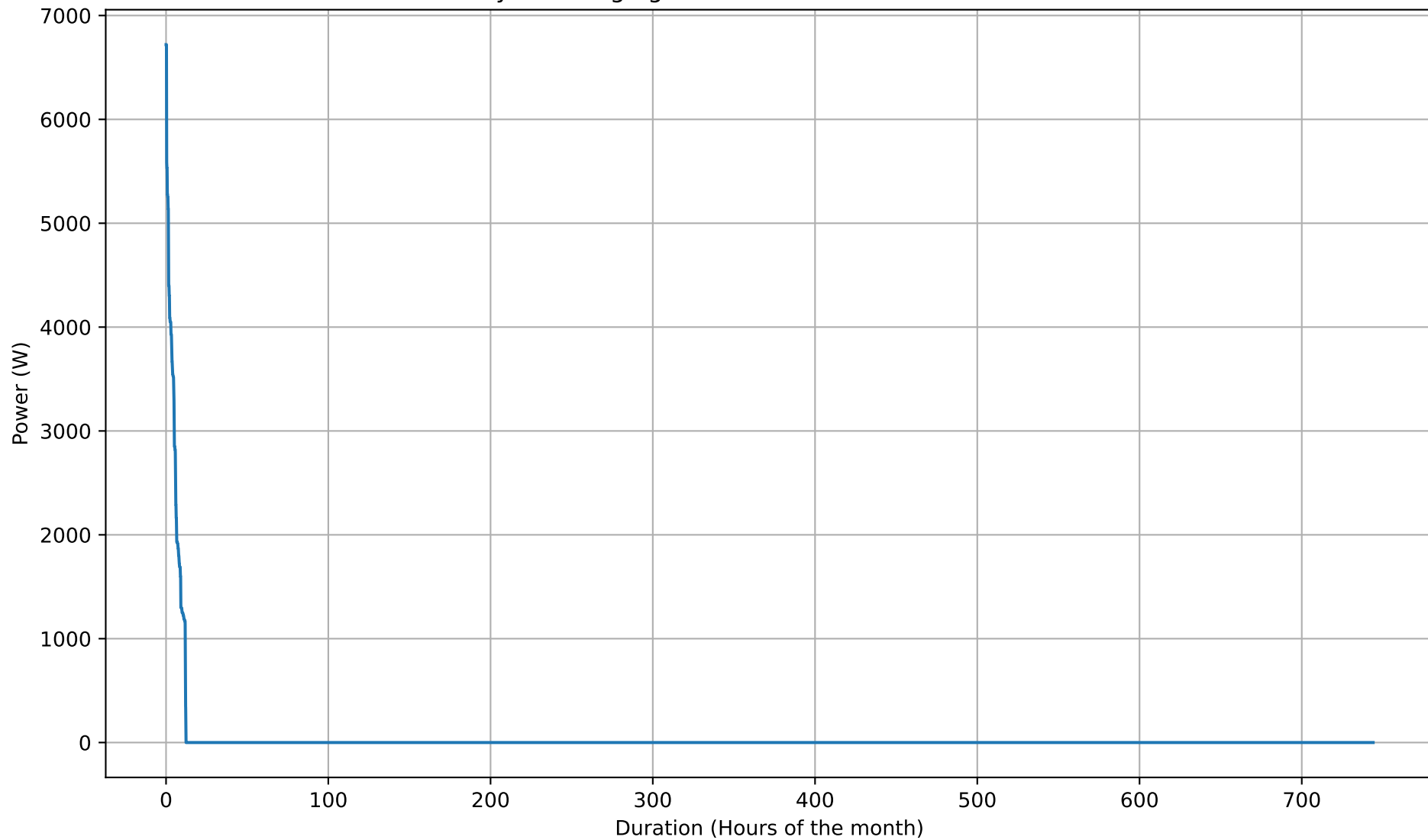
Battery Discharging Power Duration Curve - 50kWh - Dec
