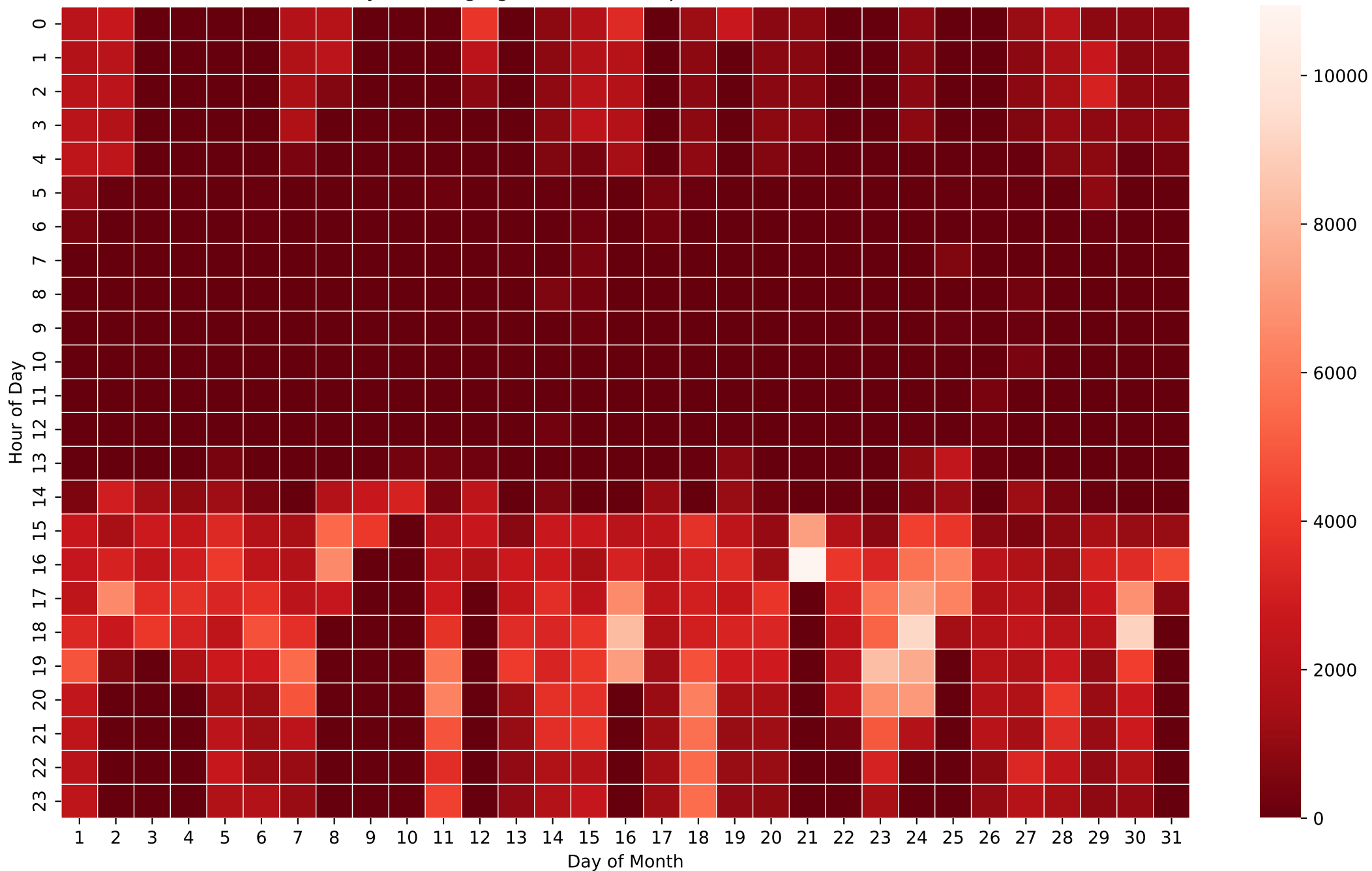
Battery Discharging Power Heatmap (Wh/Hour) - 50kWh - Mar
