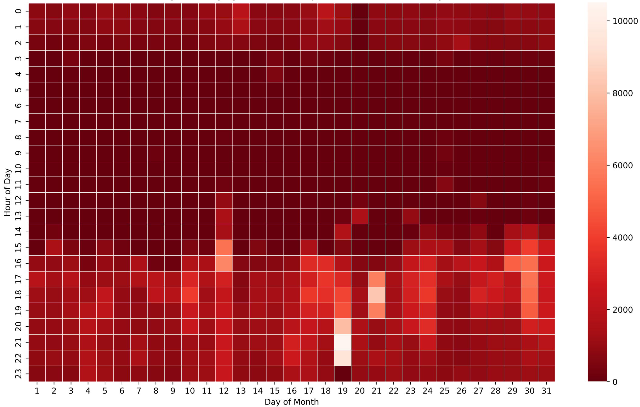
Battery Discharging Power Heatmap (Wh/Hour) - 50kWh - Aug
