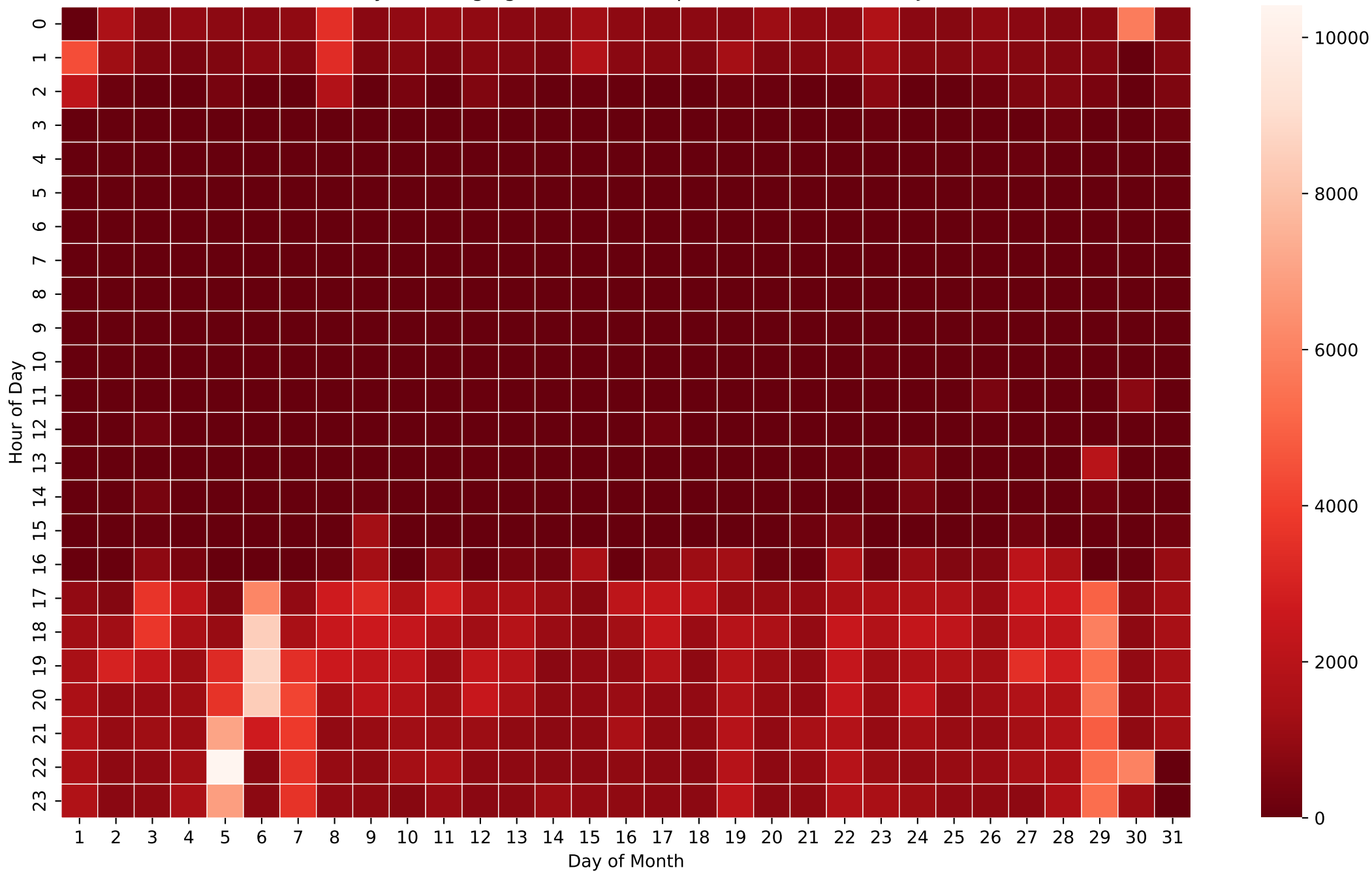
Battery Discharging Power Heatmap (Wh/Hour) - 50kWh - Jul
