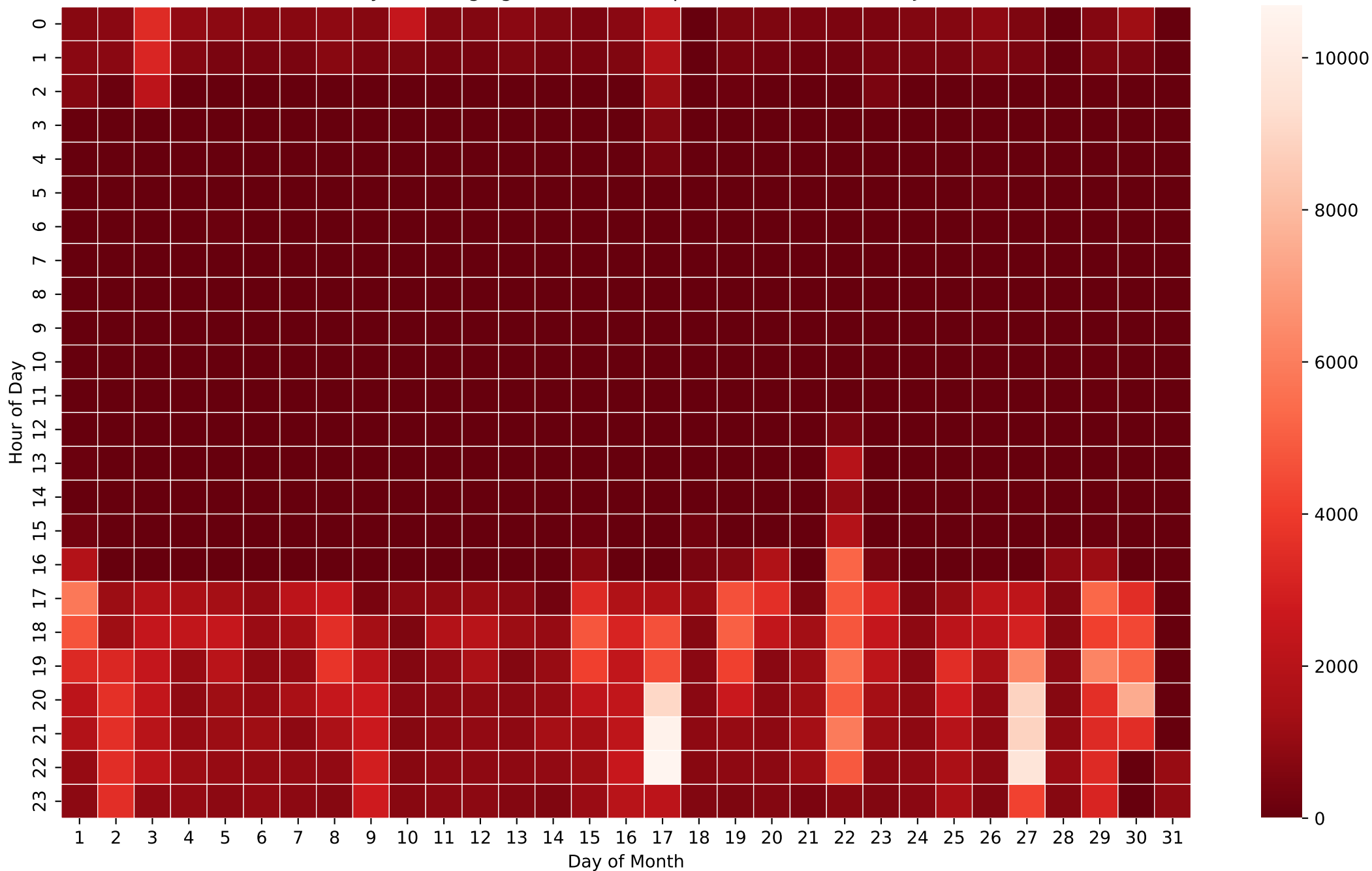
Battery Discharging Power Heatmap (Wh/Hour) - 50kWh - Jun
