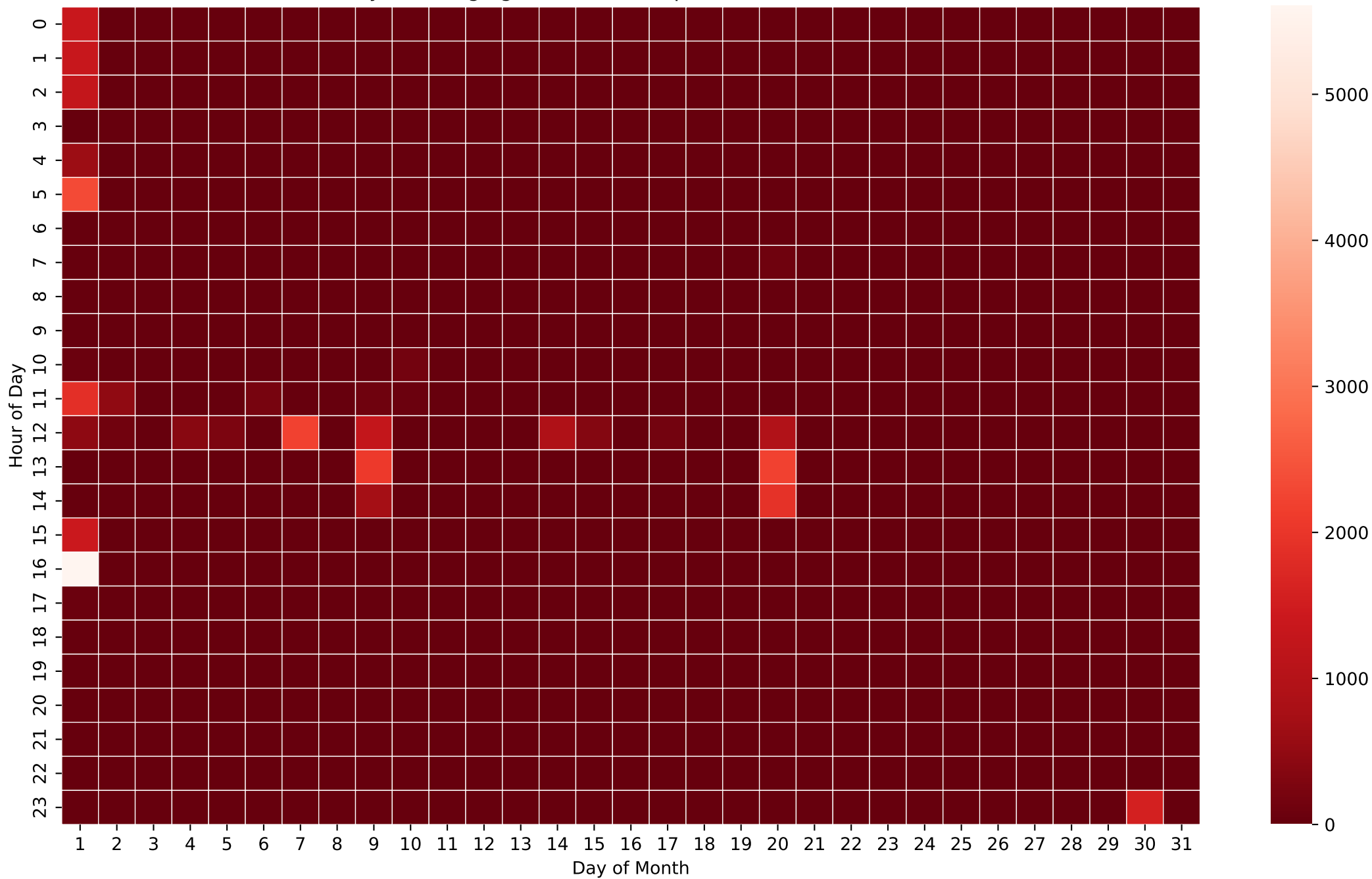
Battery Discharging Power Heatmap (Wh/Hour) - 50kWh - Dec
