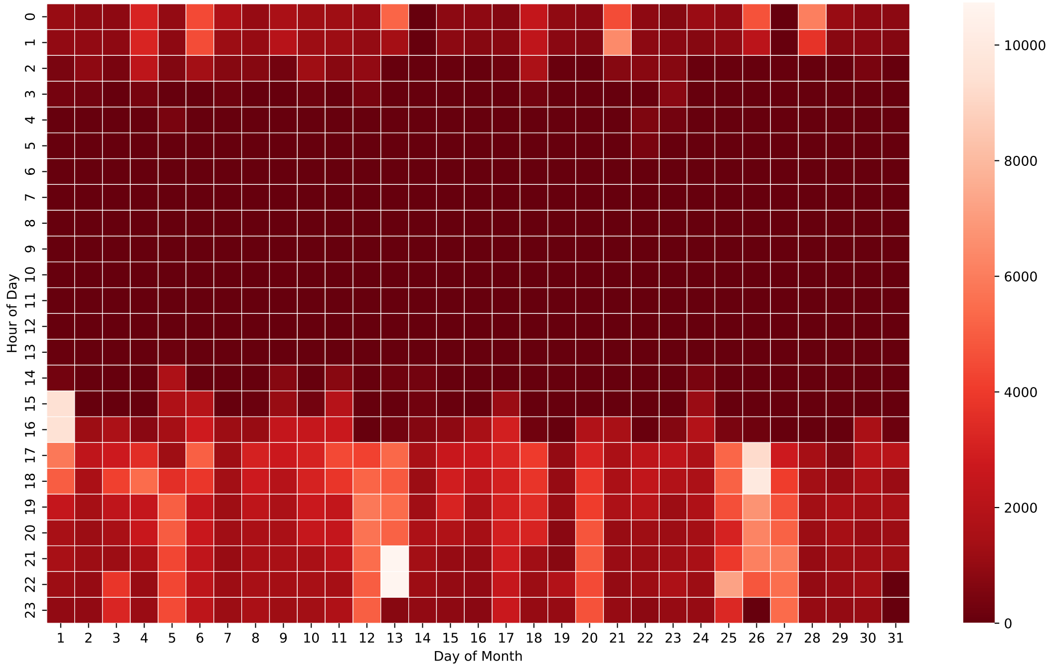
Battery Discharging Power Heatmap (Wh/Hour) - 50kWh - May
