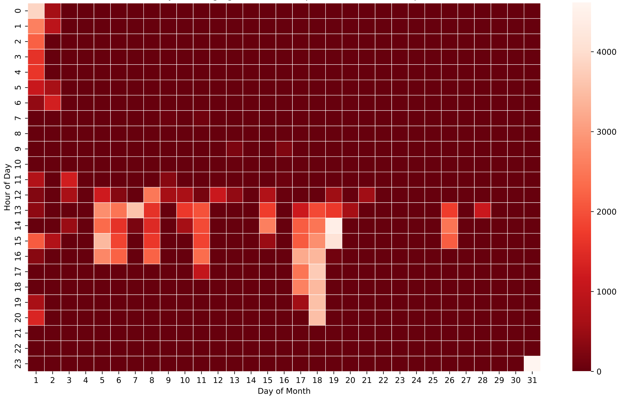
Battery Discharging Power Heatmap (Wh/Hour) - 50kWh - Jan
