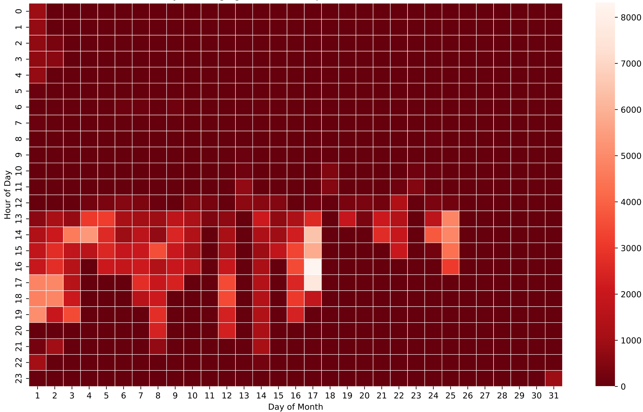
Battery Discharging Power Heatmap (Wh/Hour) - 50kWh - Nov
