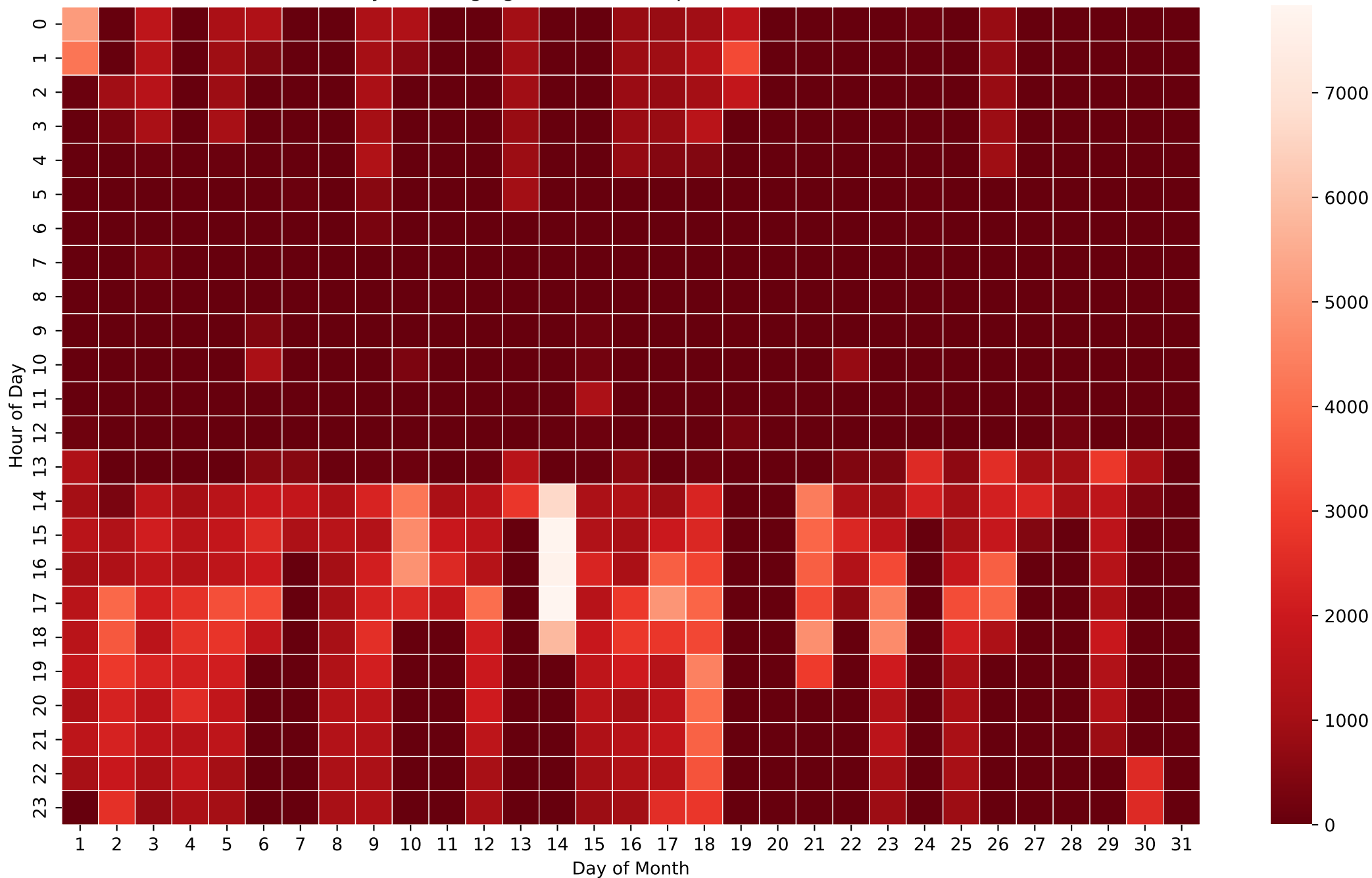
Battery Discharging Power Heatmap (Wh/Hour) - 50kWh - Oct
