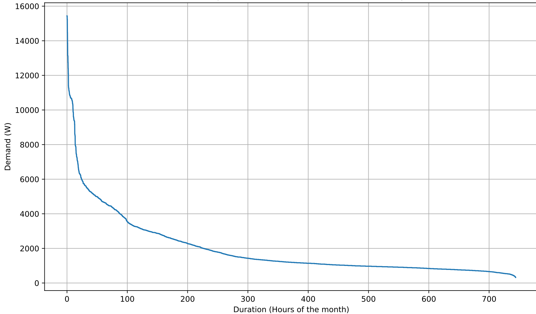
Electricity Demand Duration Curve - 50kWh - May
