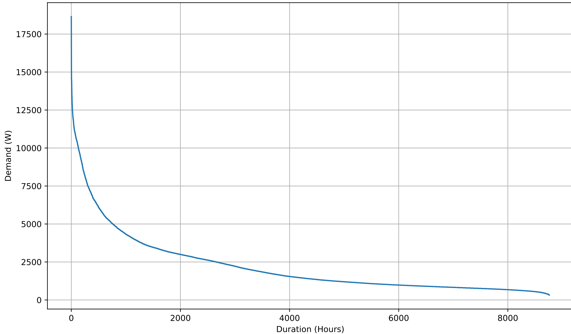
Yearly Electricity Demand Duration Curve - 50kWh
