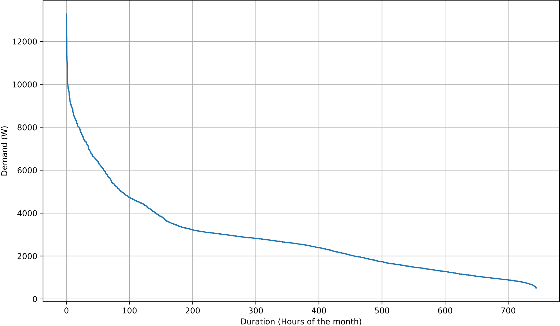
Electricity Demand Duration Curve - 50kWh - Jan
