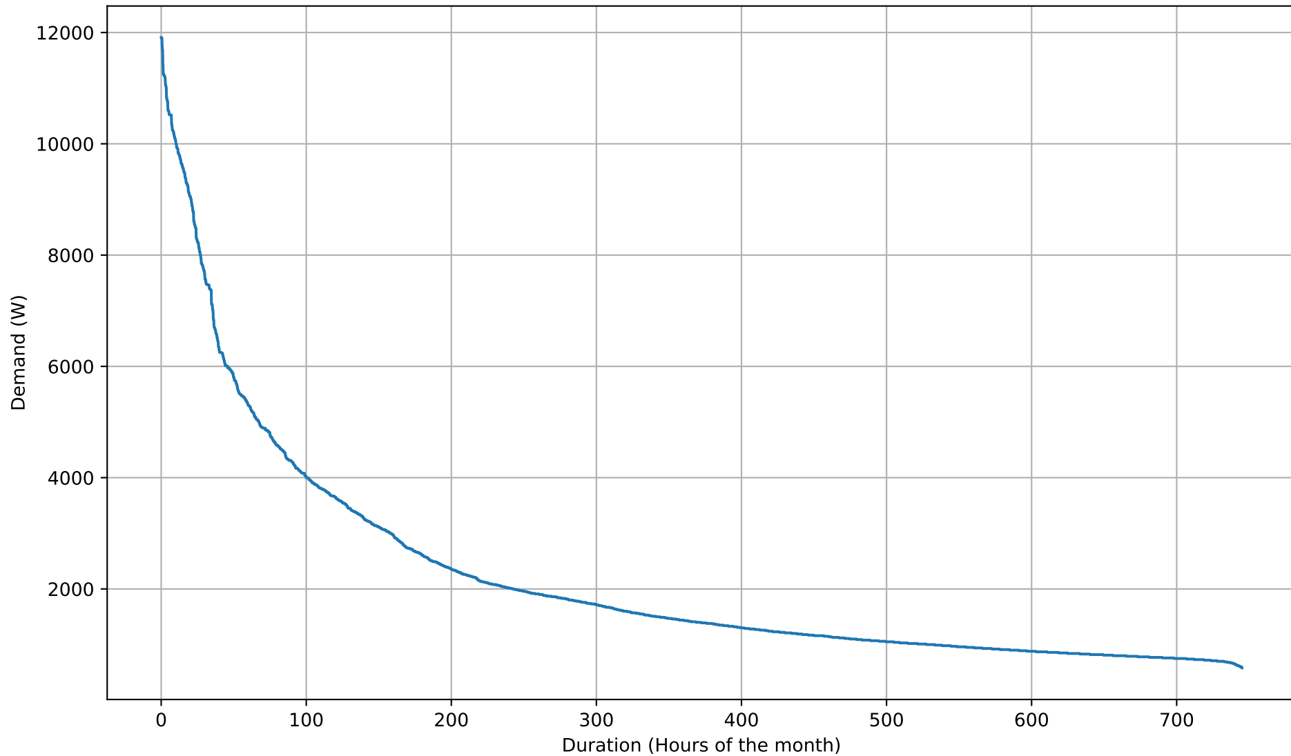
Electricity Demand Duration Curve - 50kWh - Oct
