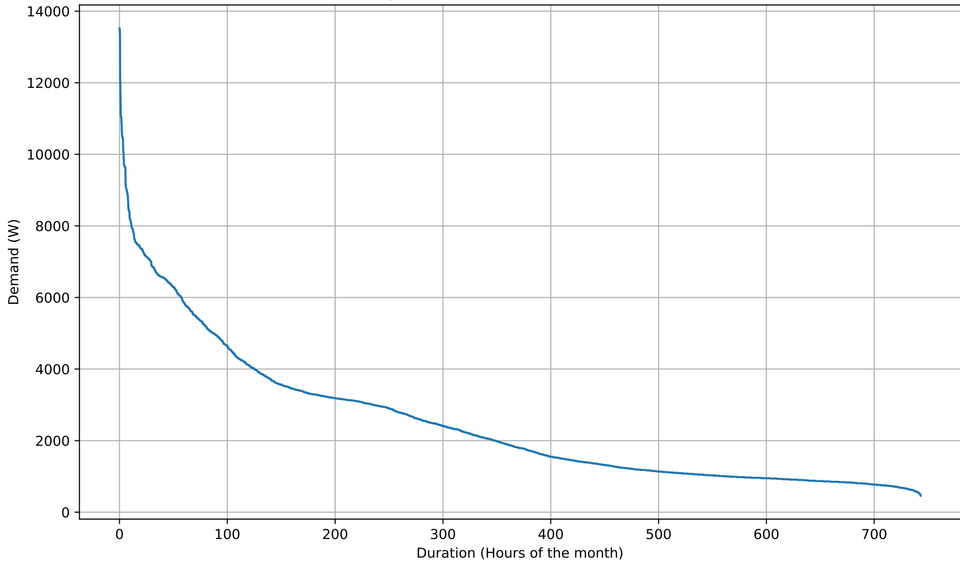
Electricity Demand Duration Curve - 50kWh - Mar
