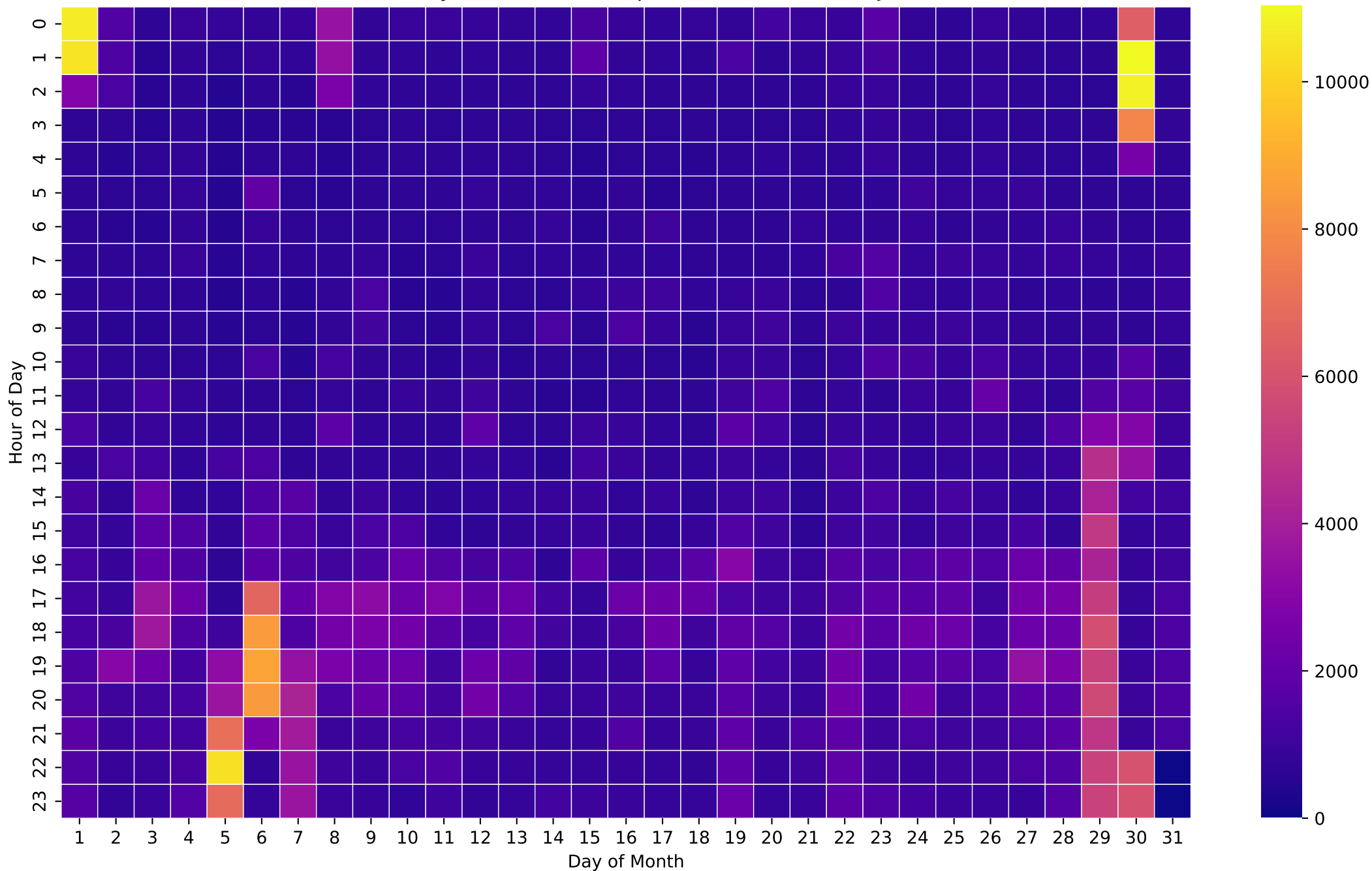
Electricity Demand Heatmap (Wh/Hour) - 50kWh - Jul
