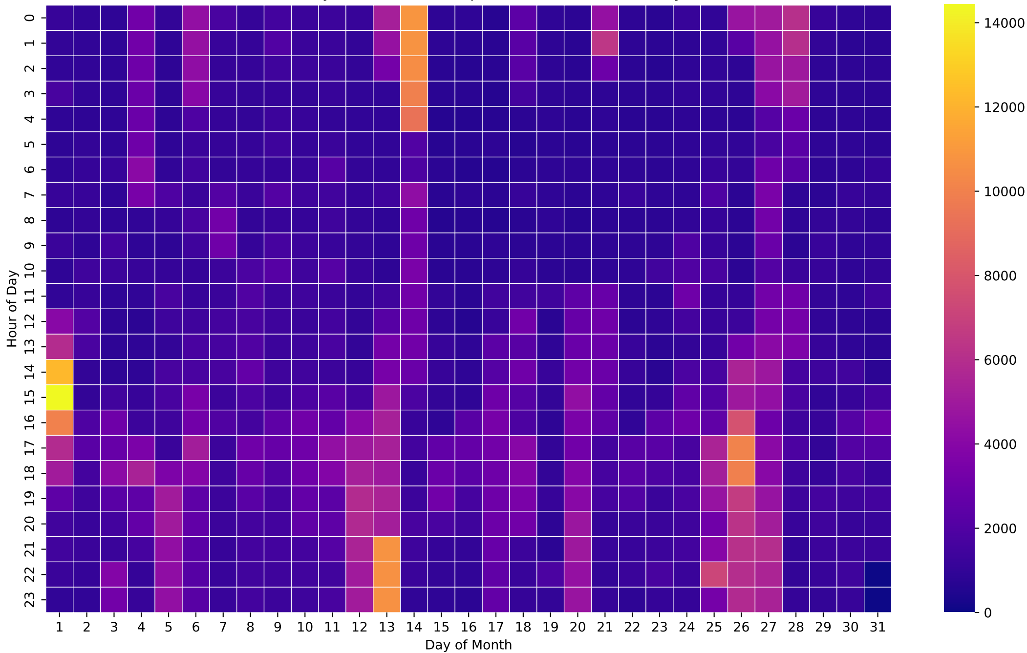
Electricity Demand Heatmap (Wh/Hour) - 50kWh - May
