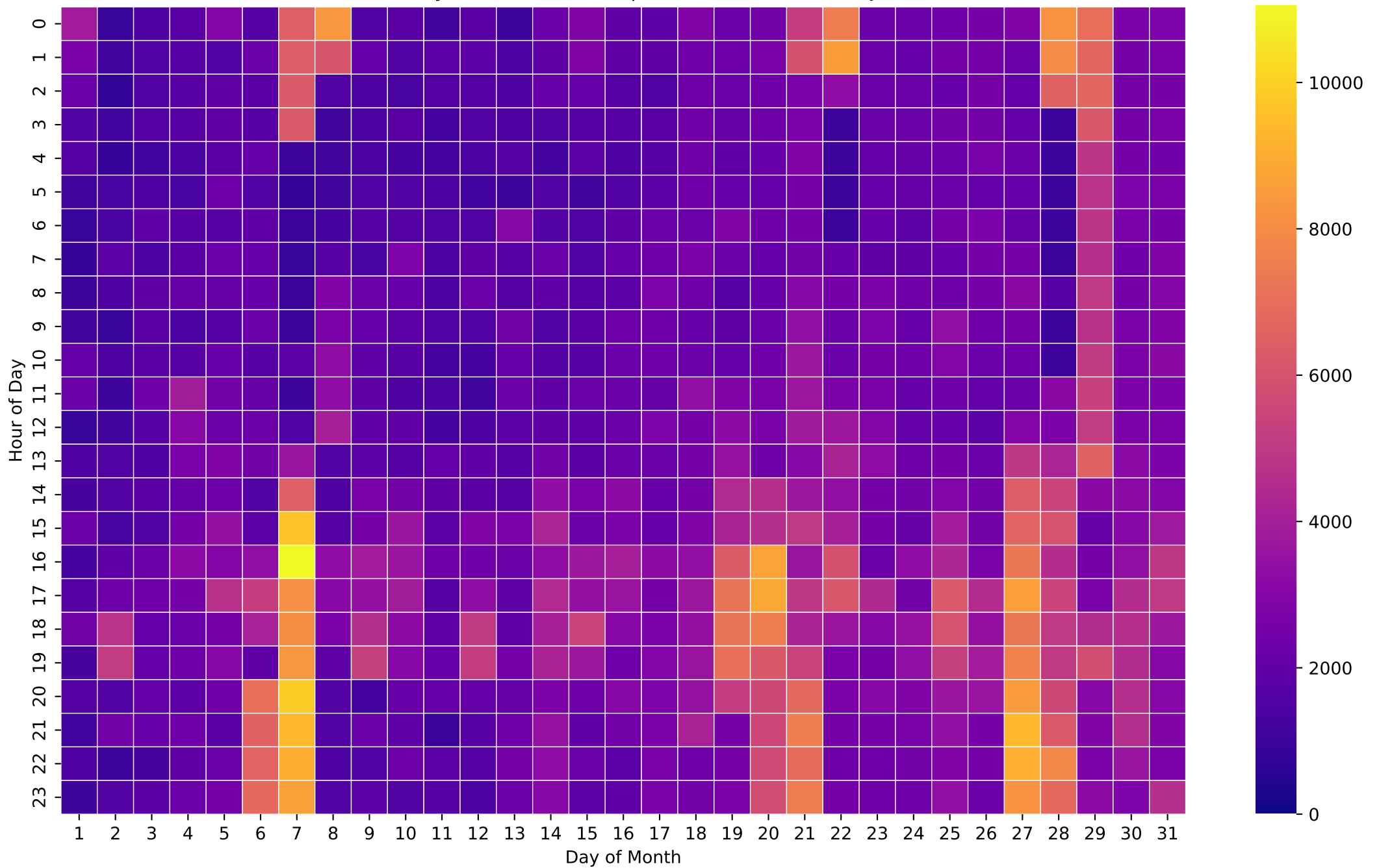
Electricity Demand Heatmap (Wh/Hour) - 50kWh - Jan
