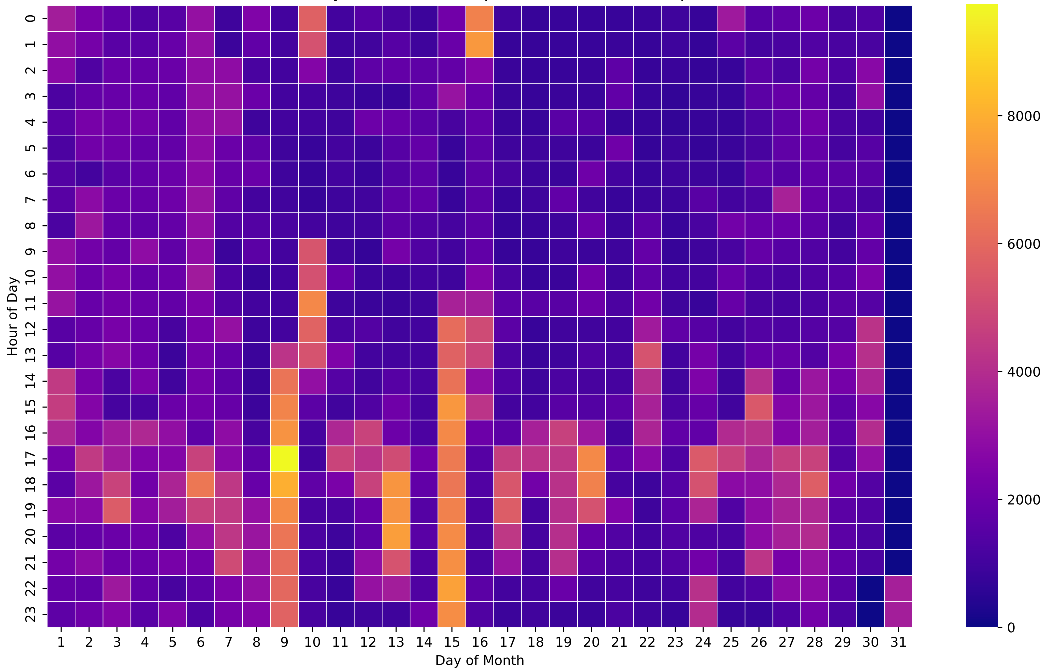
Electricity Demand Heatmap (Wh/Hour) - 50kWh - Apr
