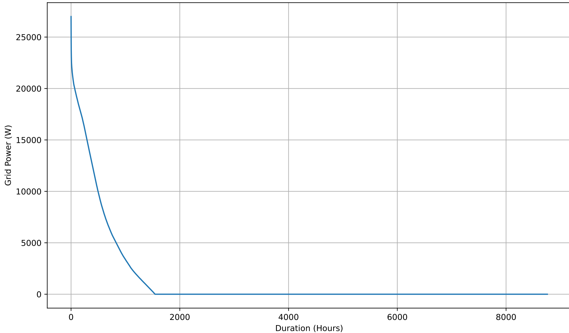
Yearly Grid Export Duration Curve - 50kWh
