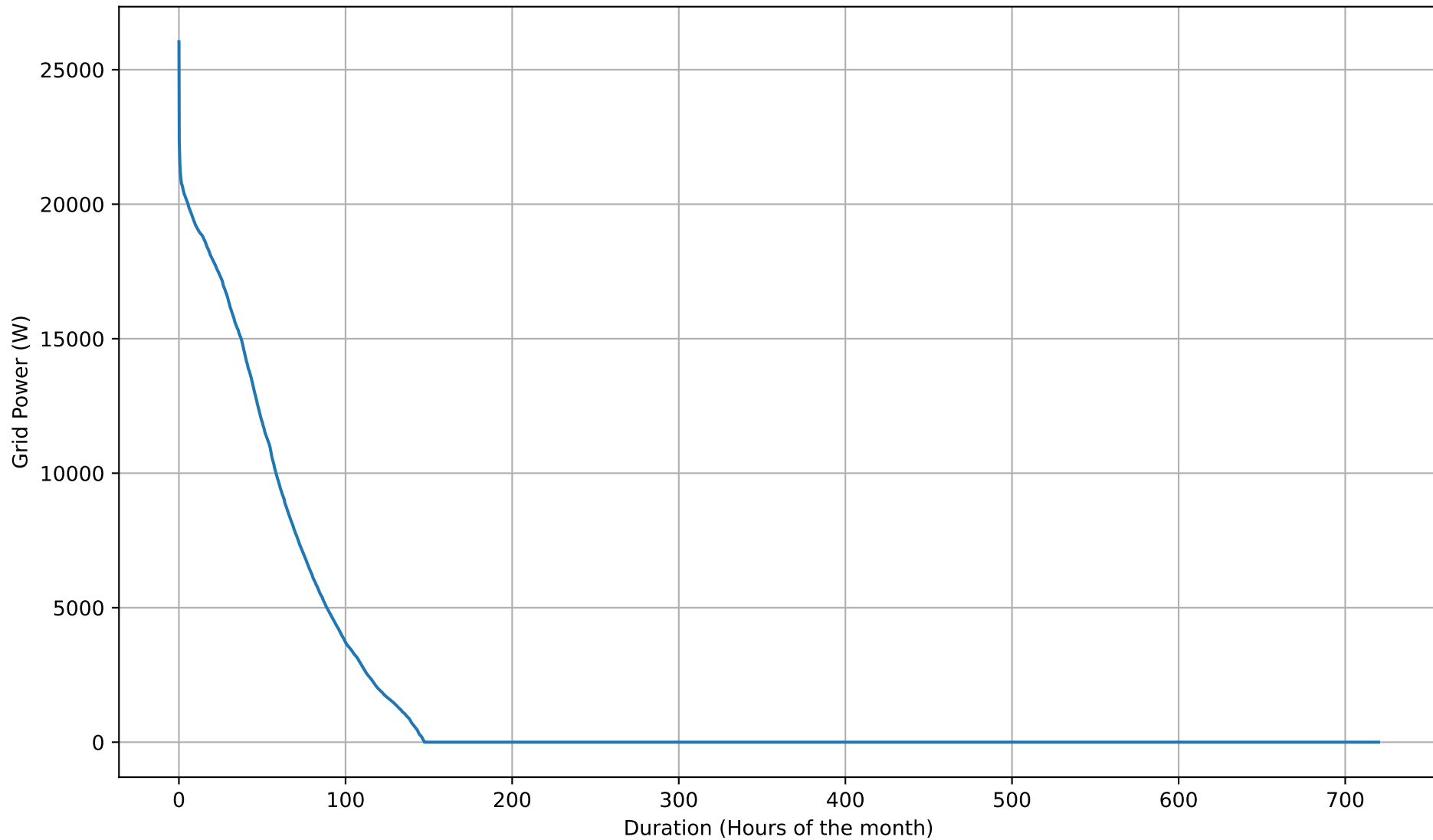
Grid Export Duration Curve - 50kWh - Apr
