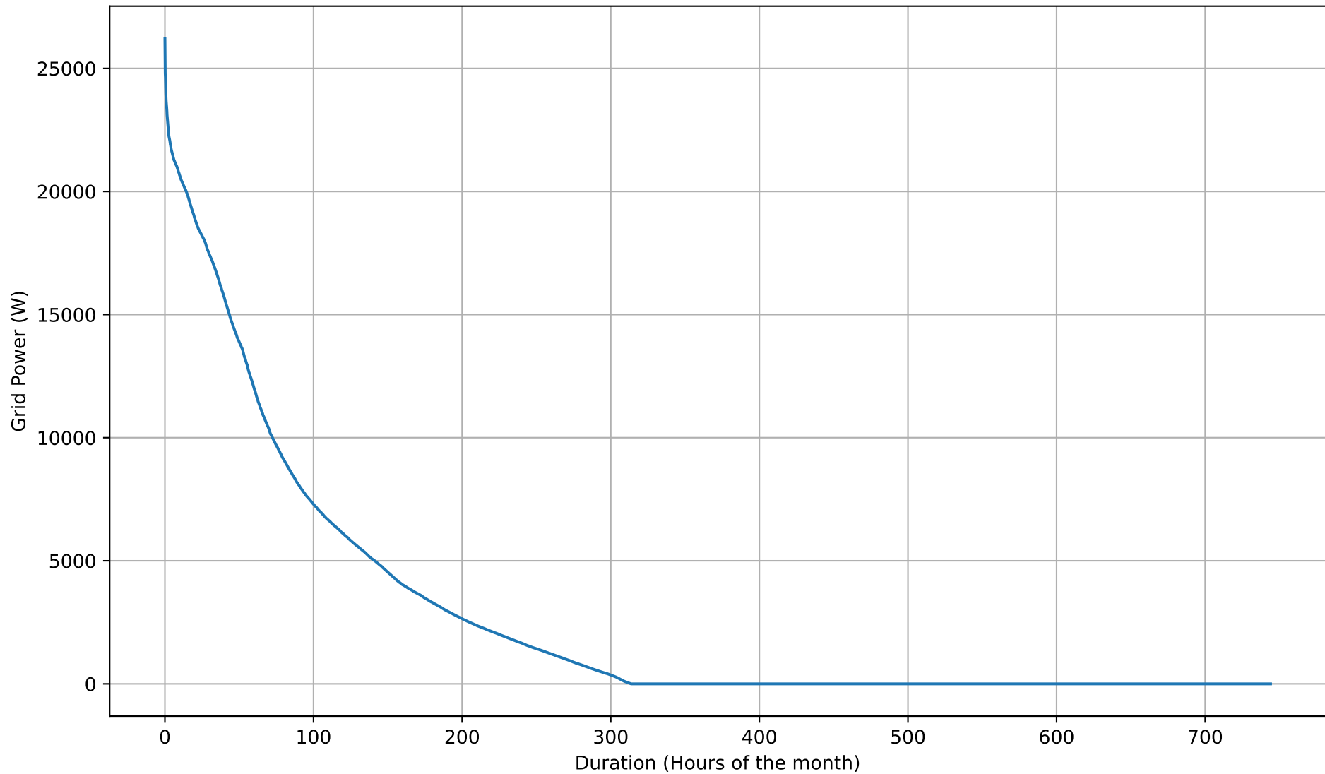
Grid Export Duration Curve - 50kWh - Jul
