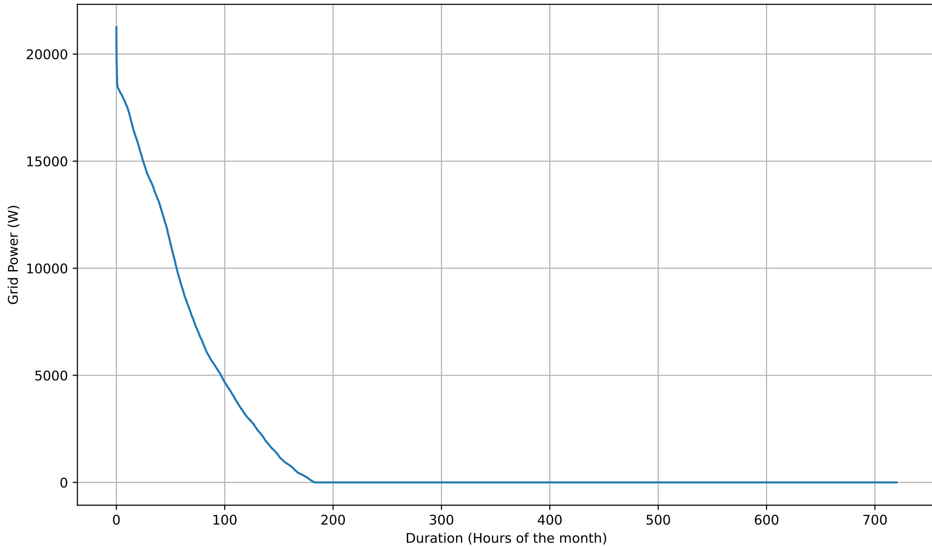
Grid Export Duration Curve - 50kWh - Sep
