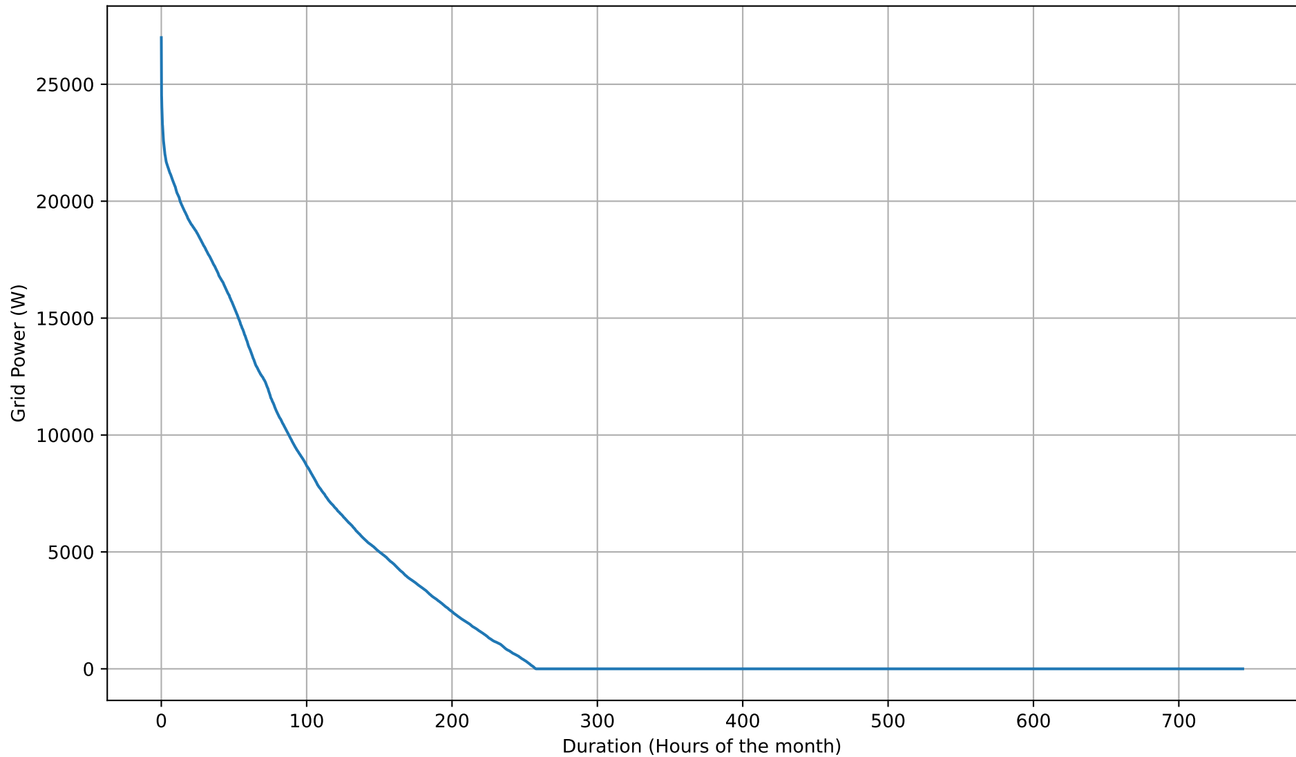
Grid Export Duration Curve - 50kWh - May
