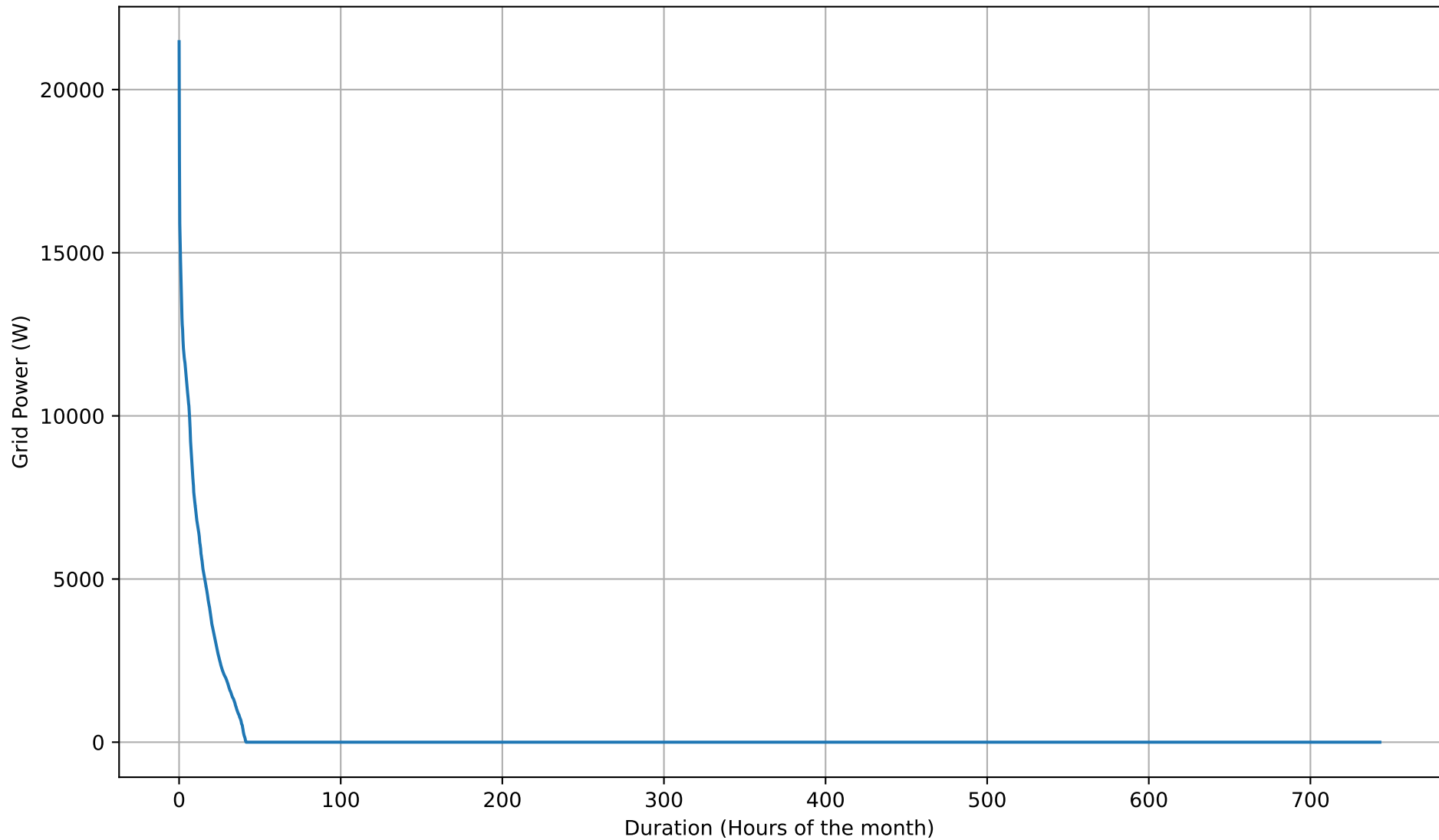
Grid Export Duration Curve - 50kWh - Mar
