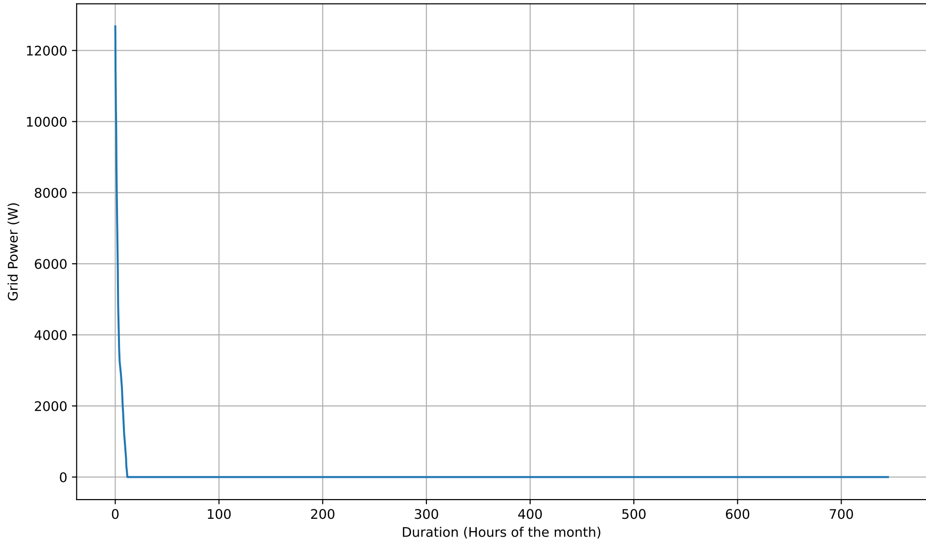
Grid Export Duration Curve - 50kWh - Oct
