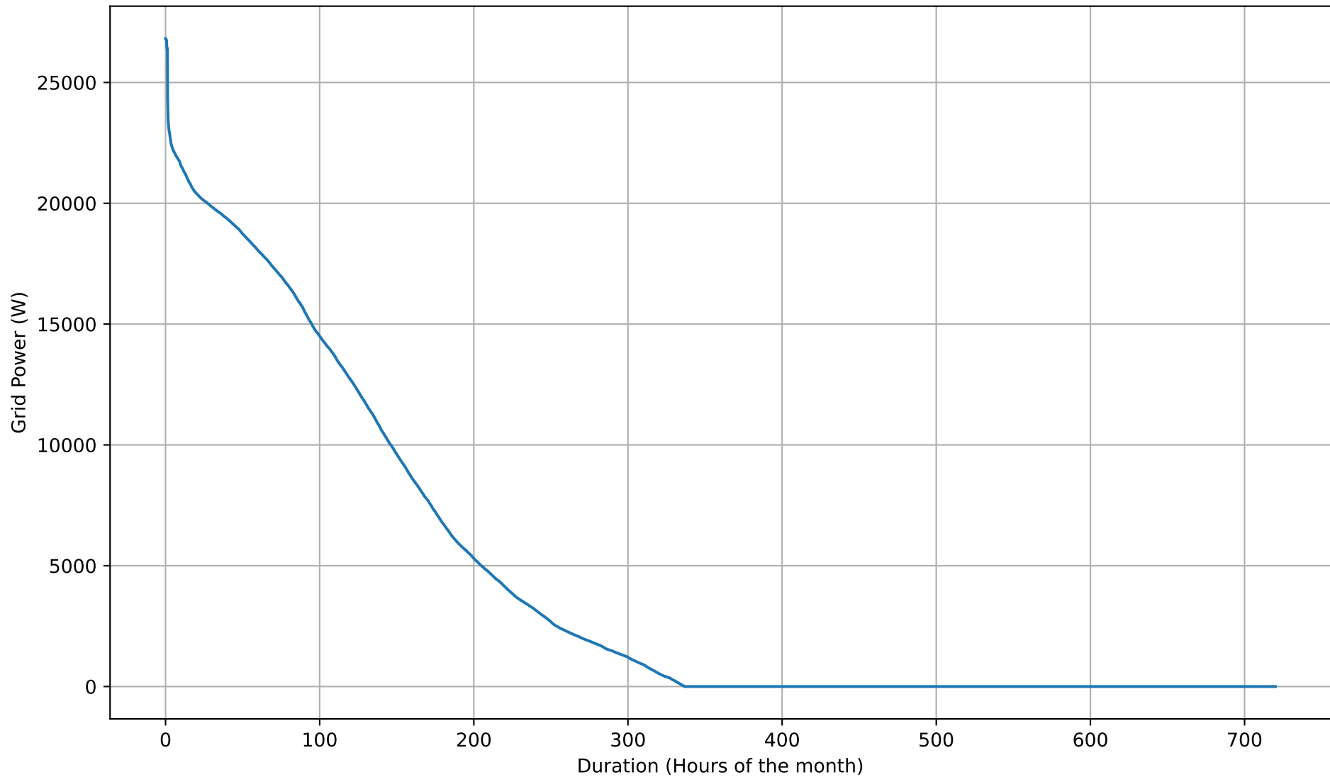
Grid Export Duration Curve - 50kWh - Jun
