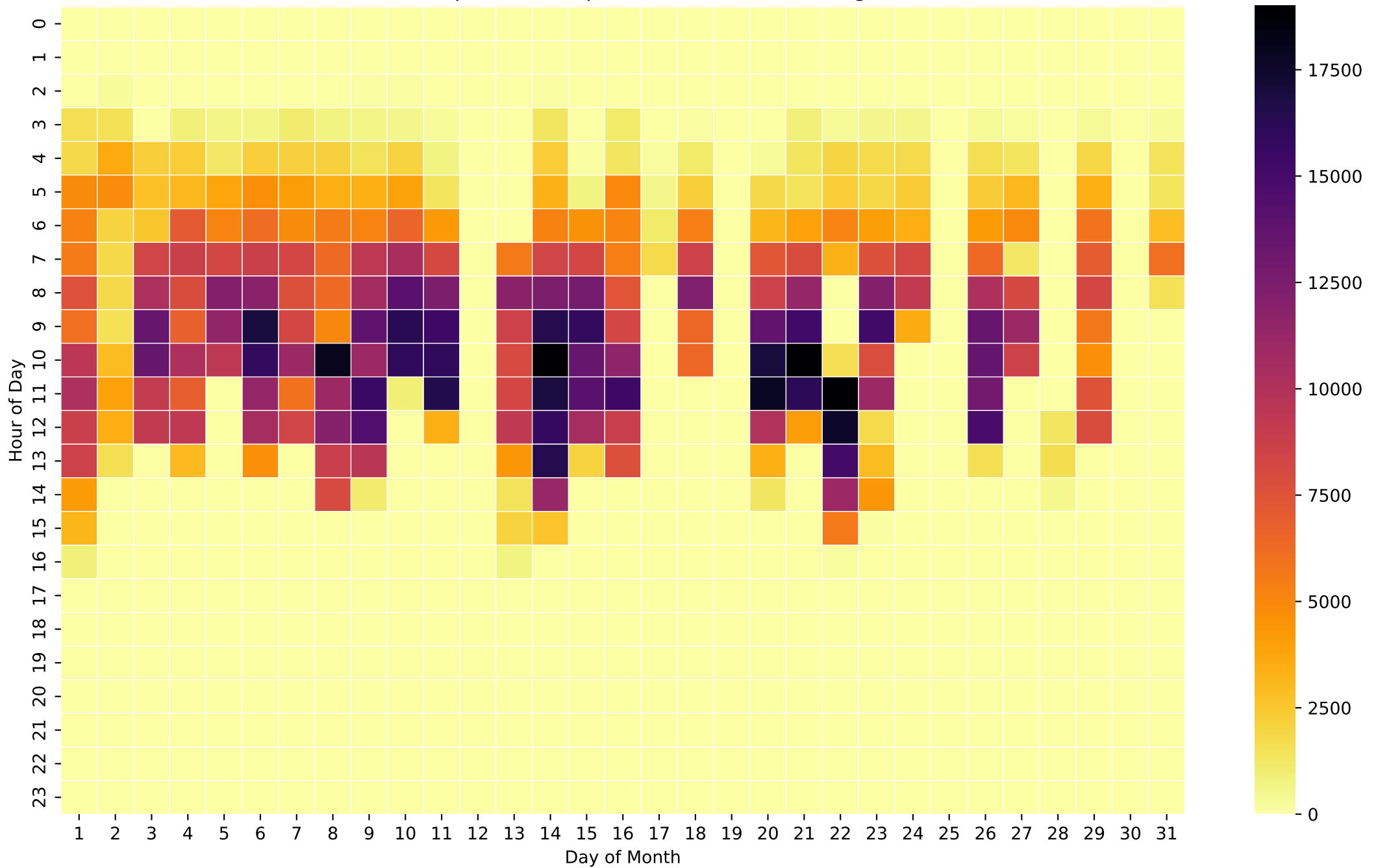
Grid Export Heatmap (Wh/Hour) - 50kWh - Aug
