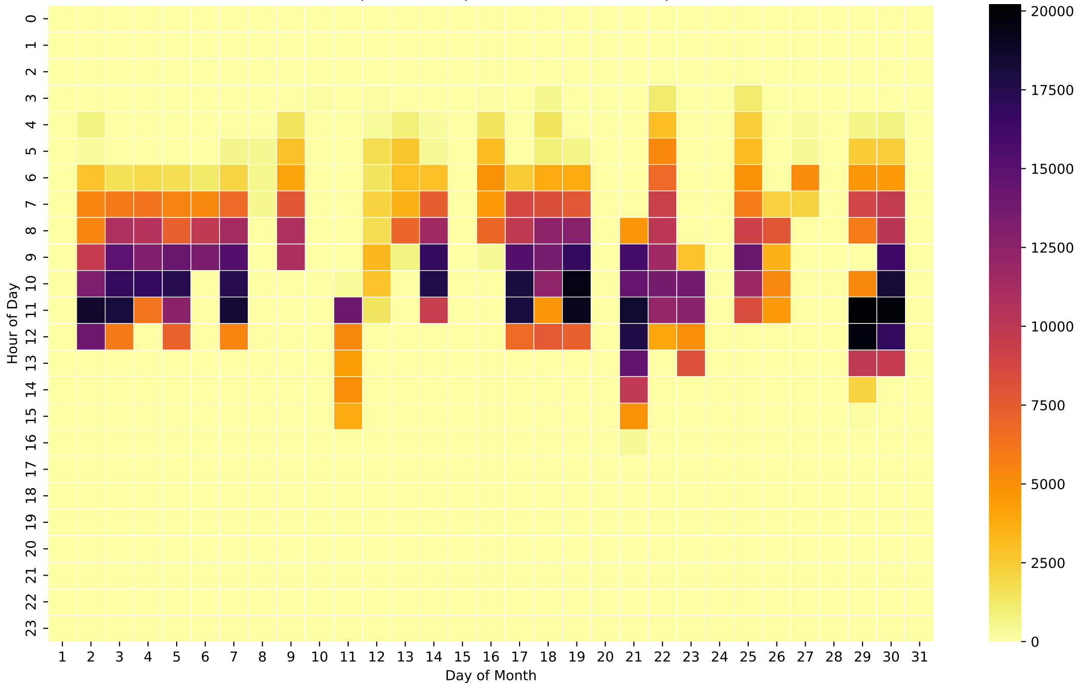
Grid Export Heatmap (Wh/Hour) - 50kWh - Apr
