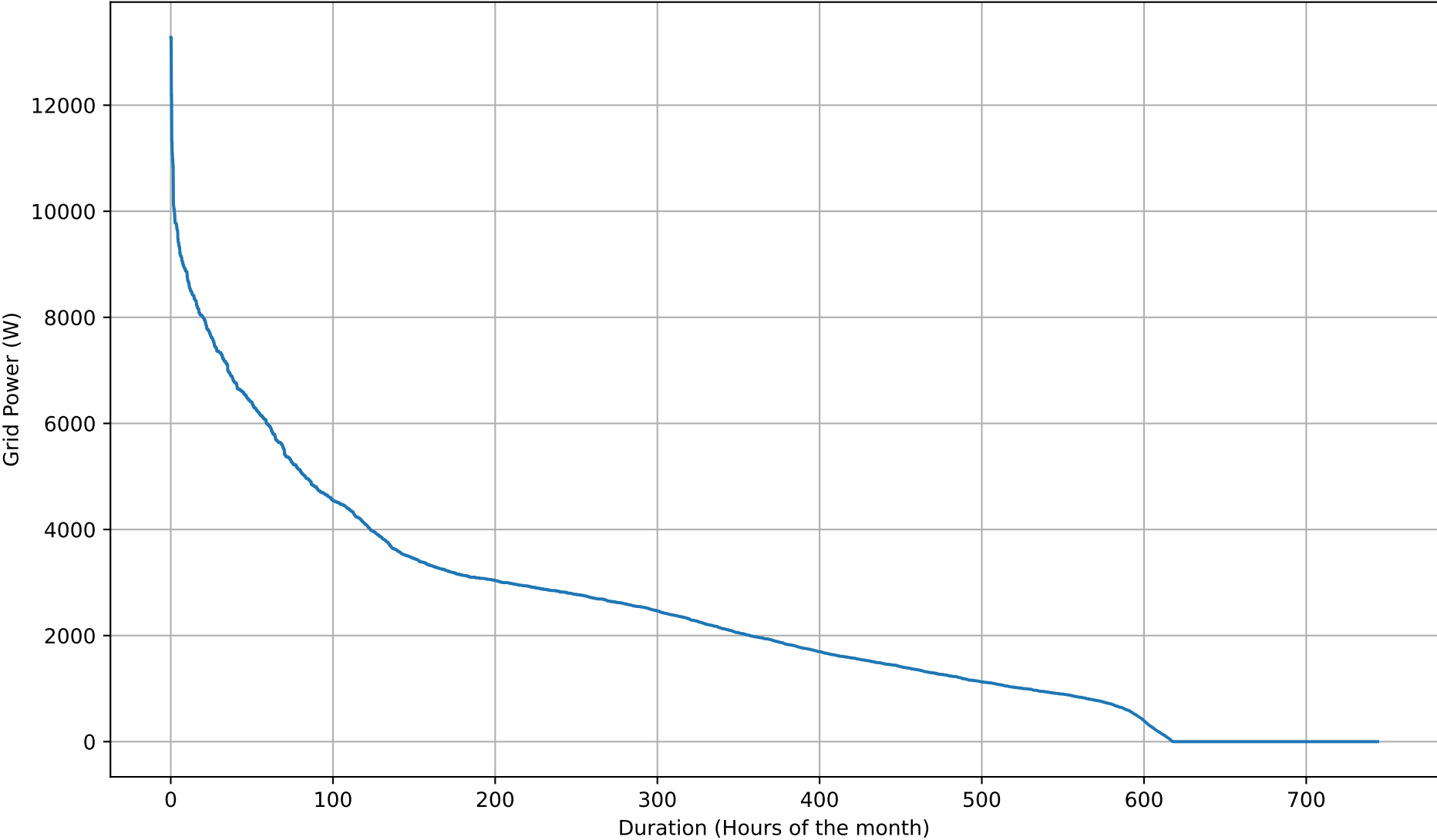
Grid Import Duration Curve - 50kWh - Jan
