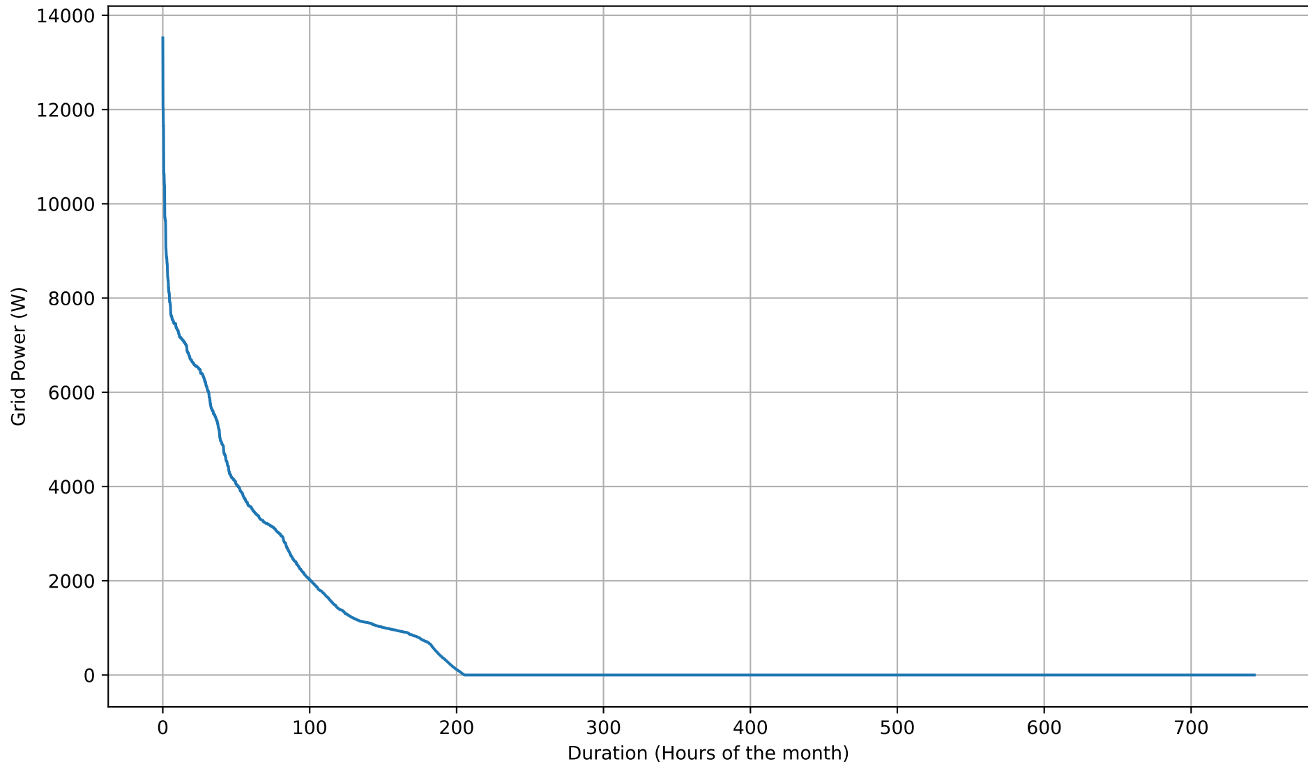
Grid Import Duration Curve - 50kWh - Mar
