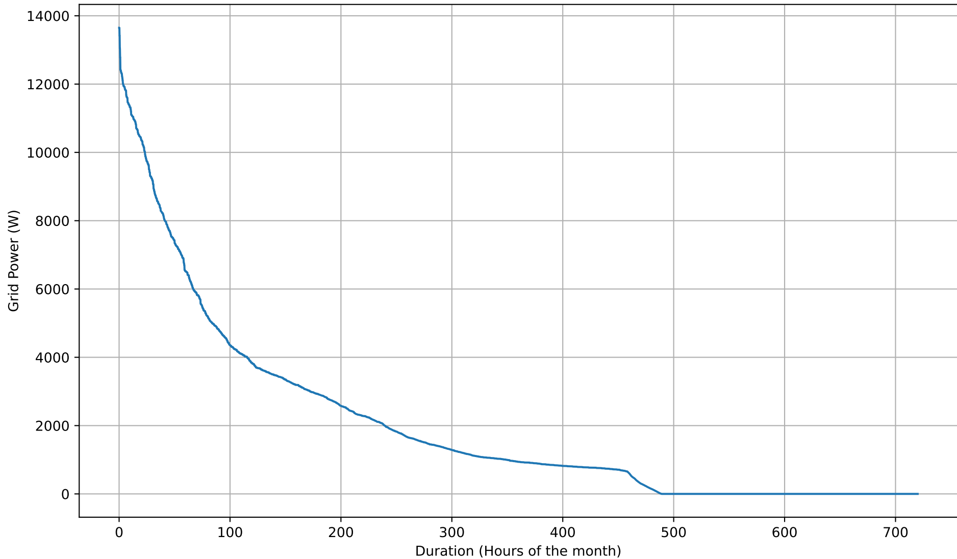
Grid Import Duration Curve - 50kWh - Nov
