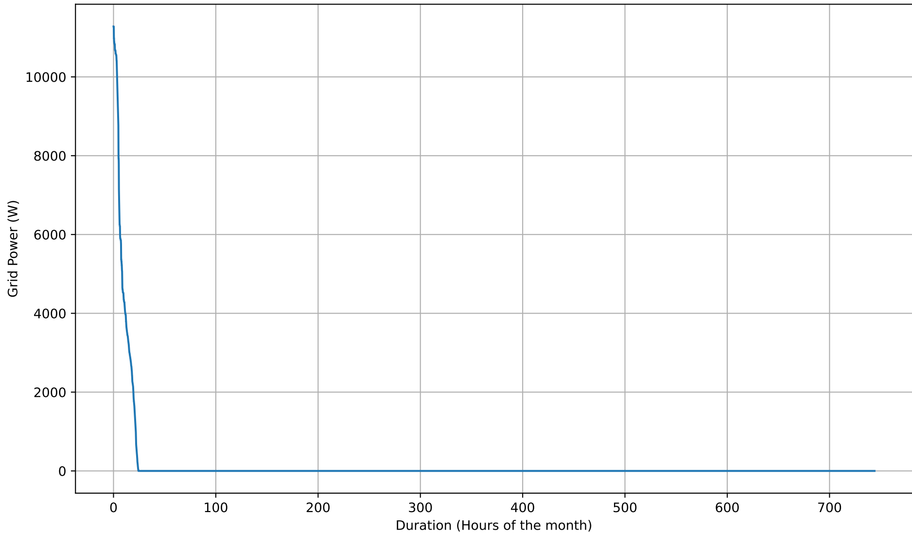
Grid Import Duration Curve - 50kWh - May
