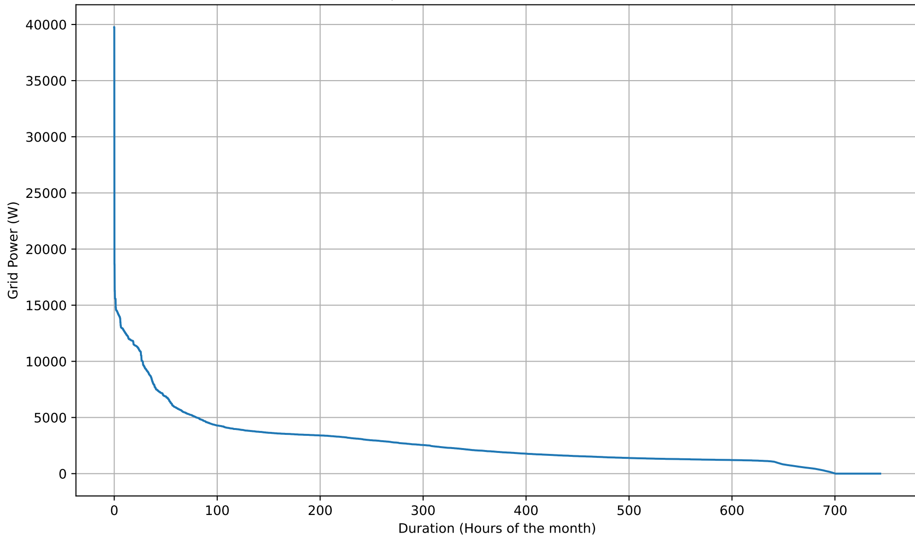
Grid Import Duration Curve - 50kWh - Dec
