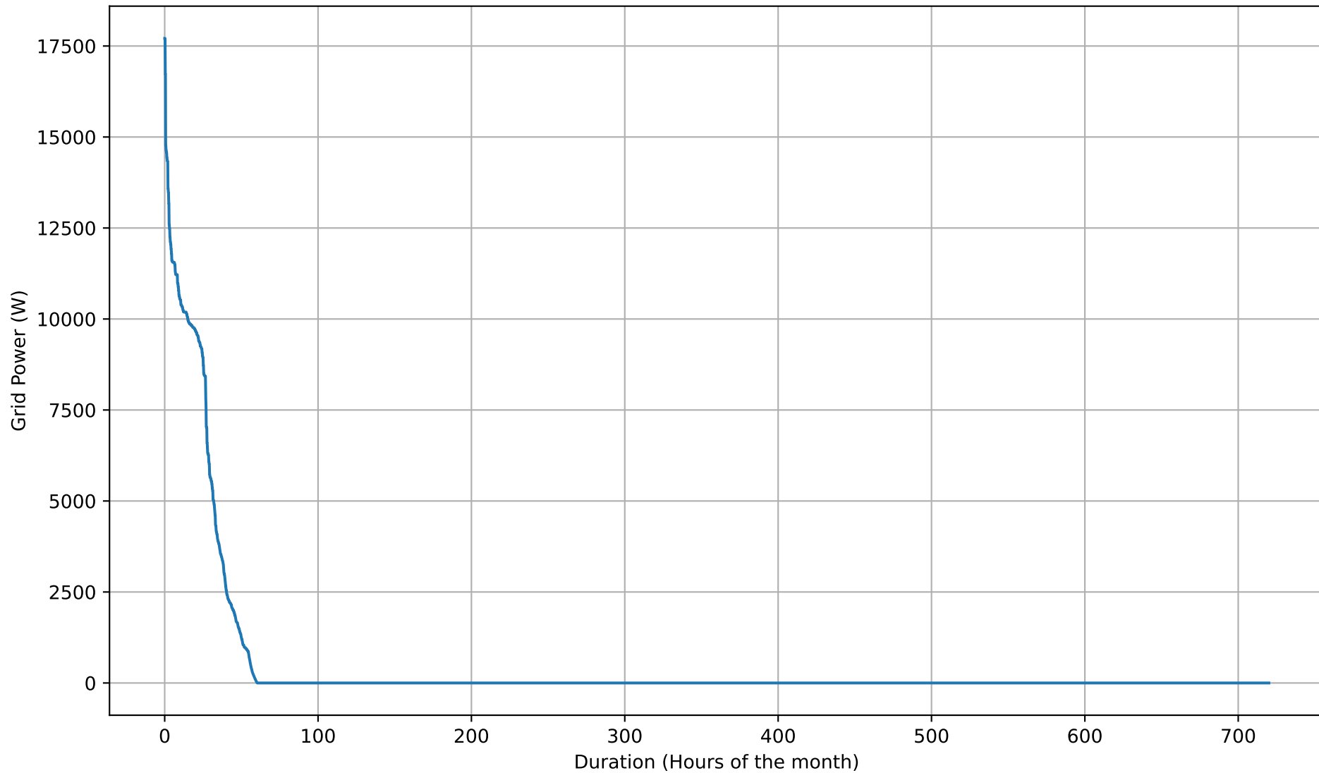
Grid Import Duration Curve - 50kWh - Sep
