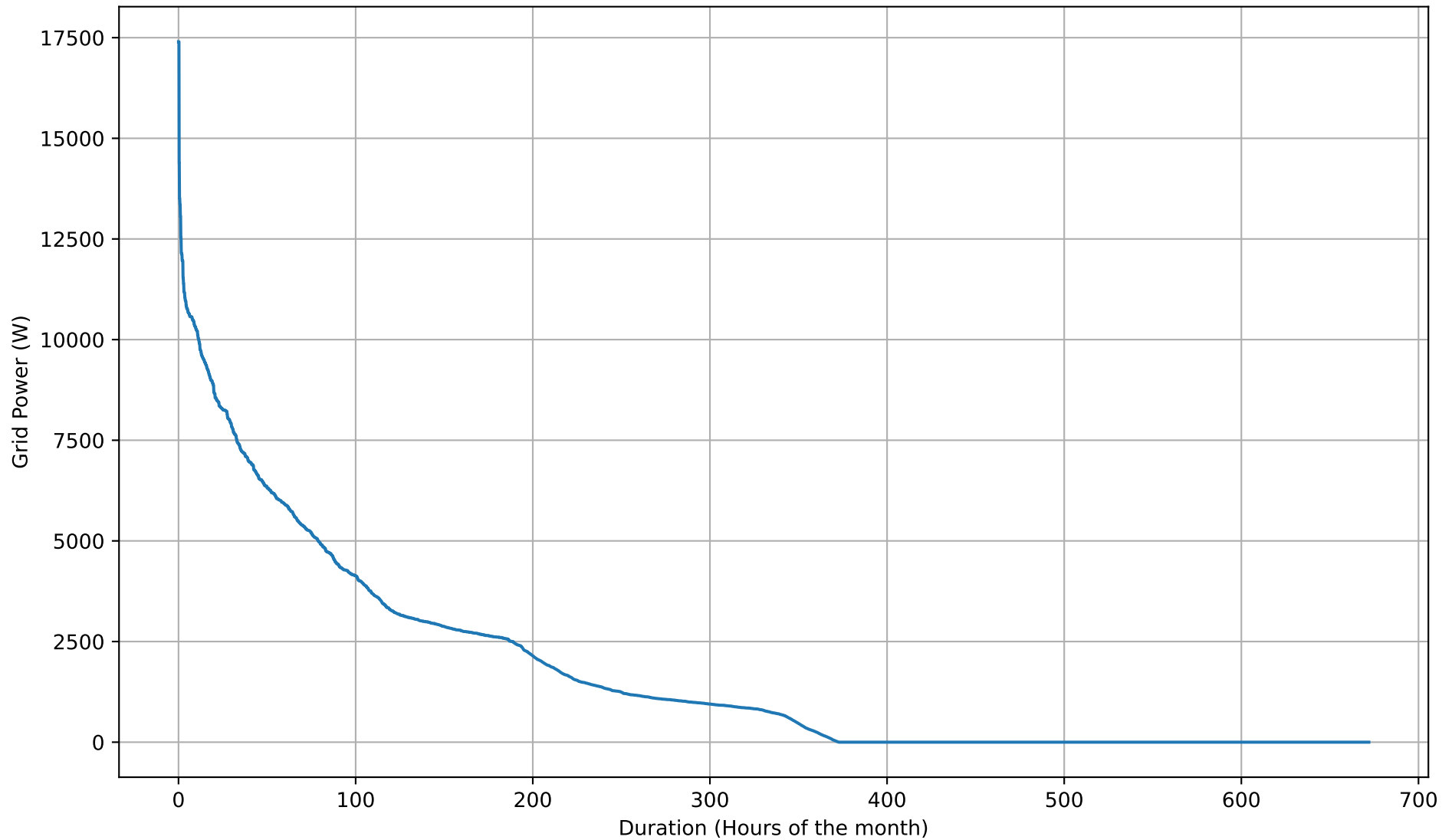
Grid Import Duration Curve - 50kWh - Feb
