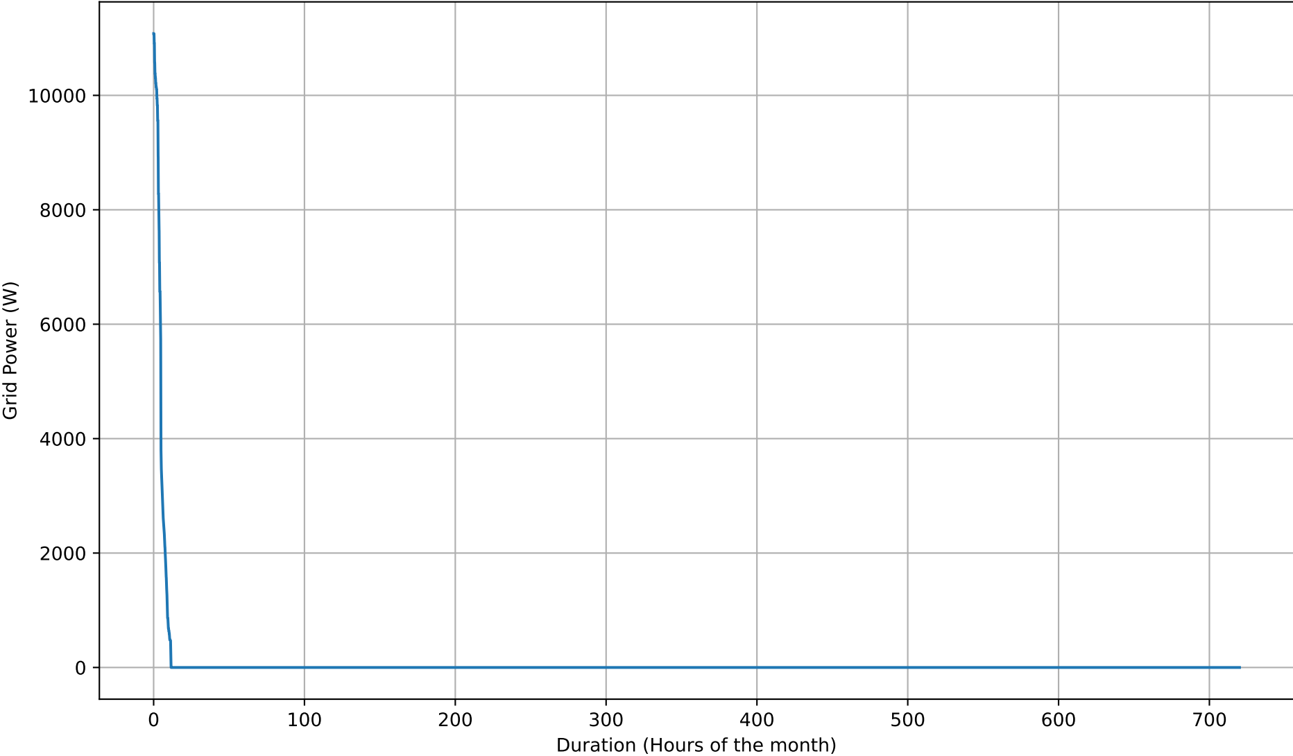
Grid Import Duration Curve - 50kWh - Jun
