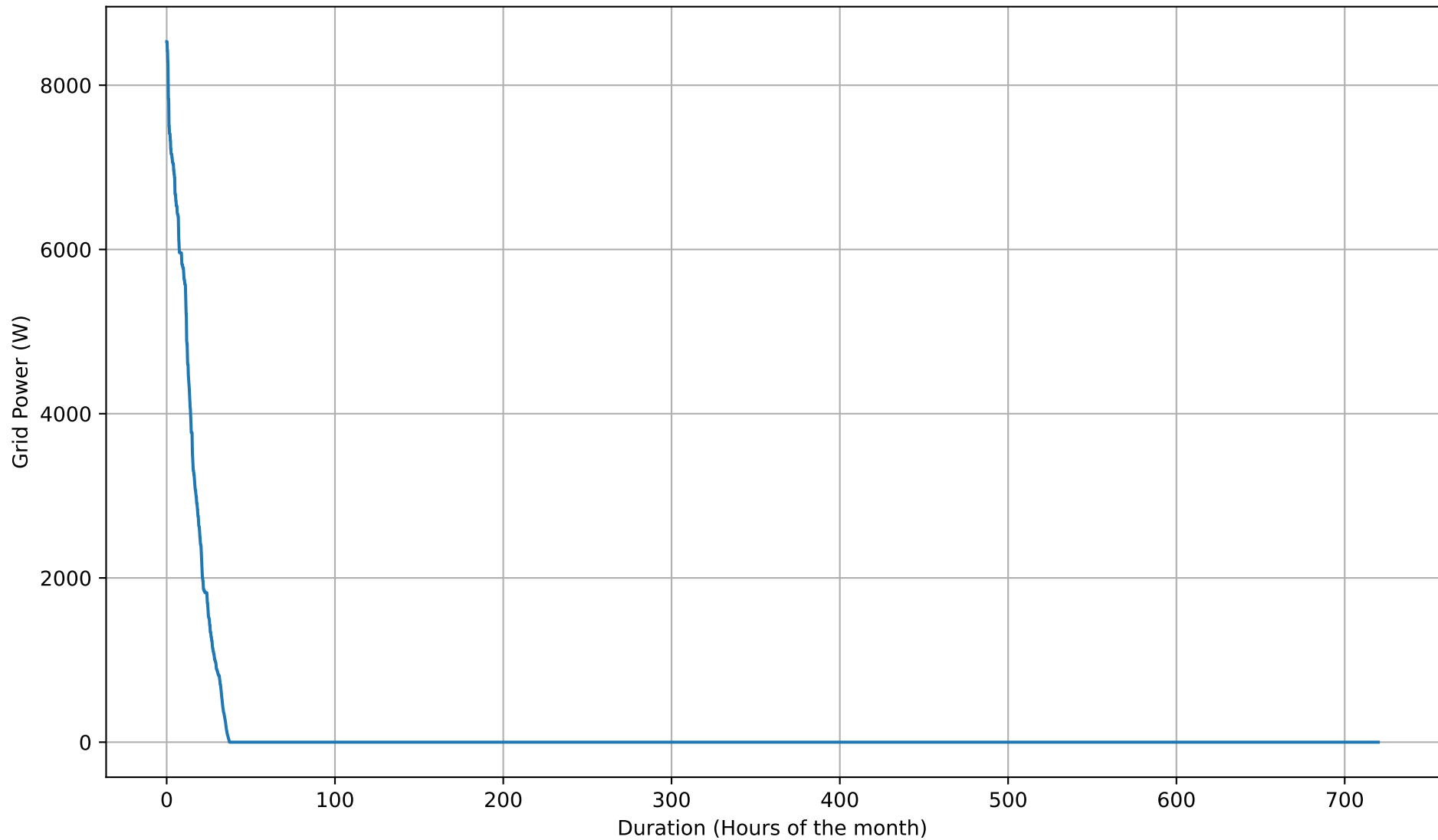
Grid Import Duration Curve - 50kWh - Apr
