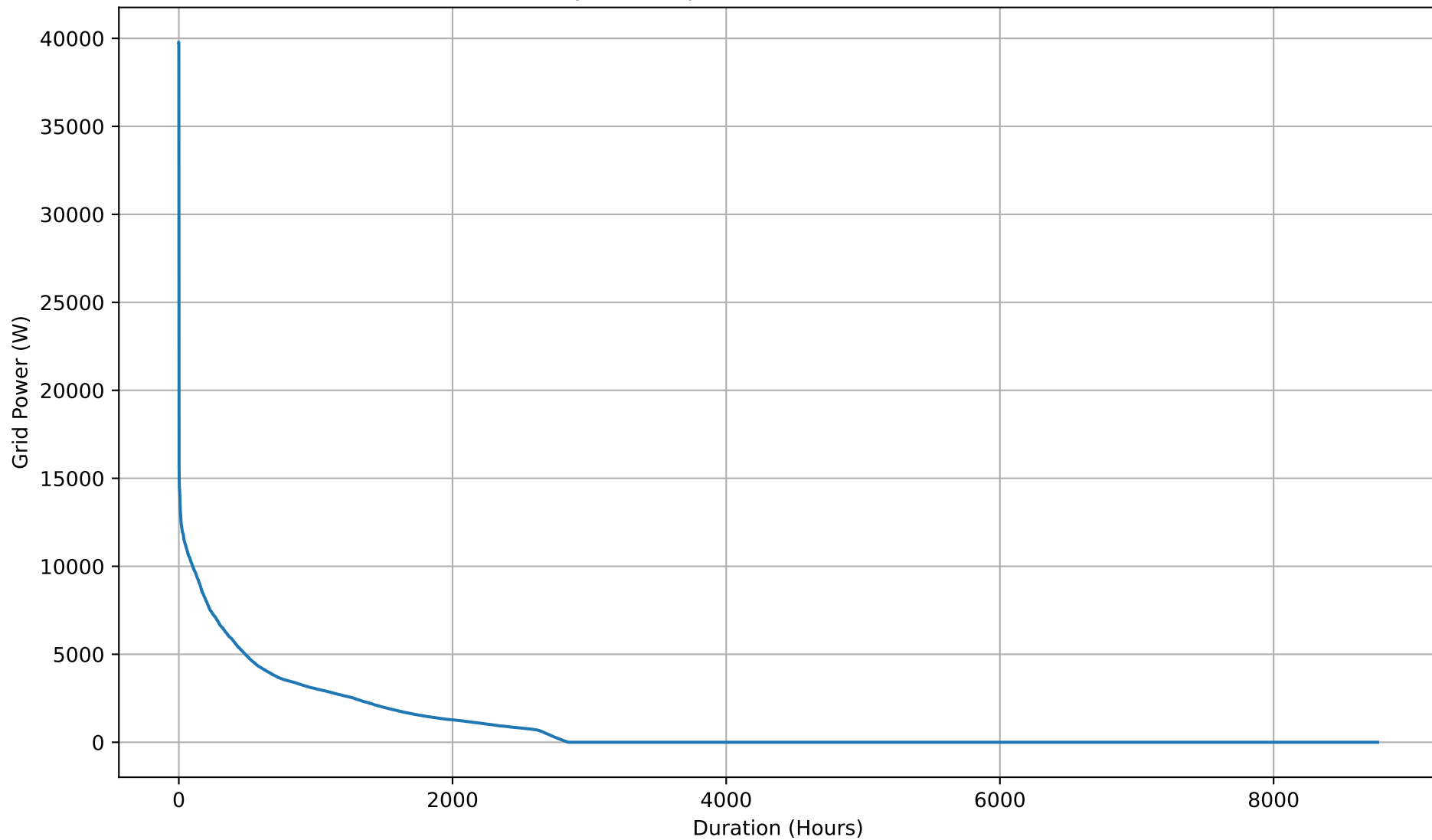
Yearly Grid Import Duration Curve - 50kWh
