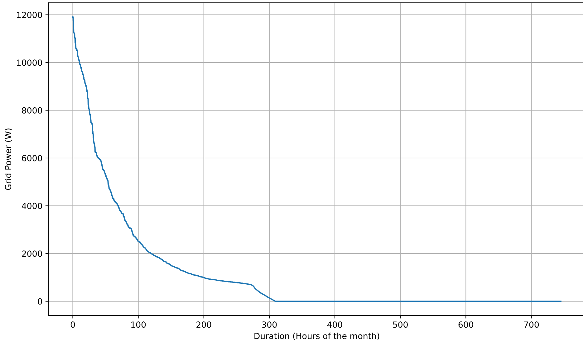
Grid Import Duration Curve - 50kWh - Oct
