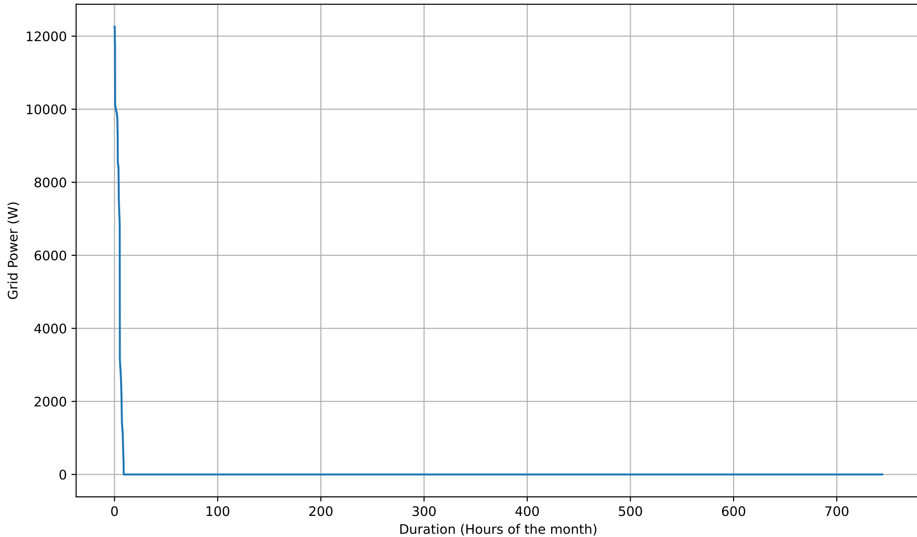
Grid Import Duration Curve - 50kWh - Aug
