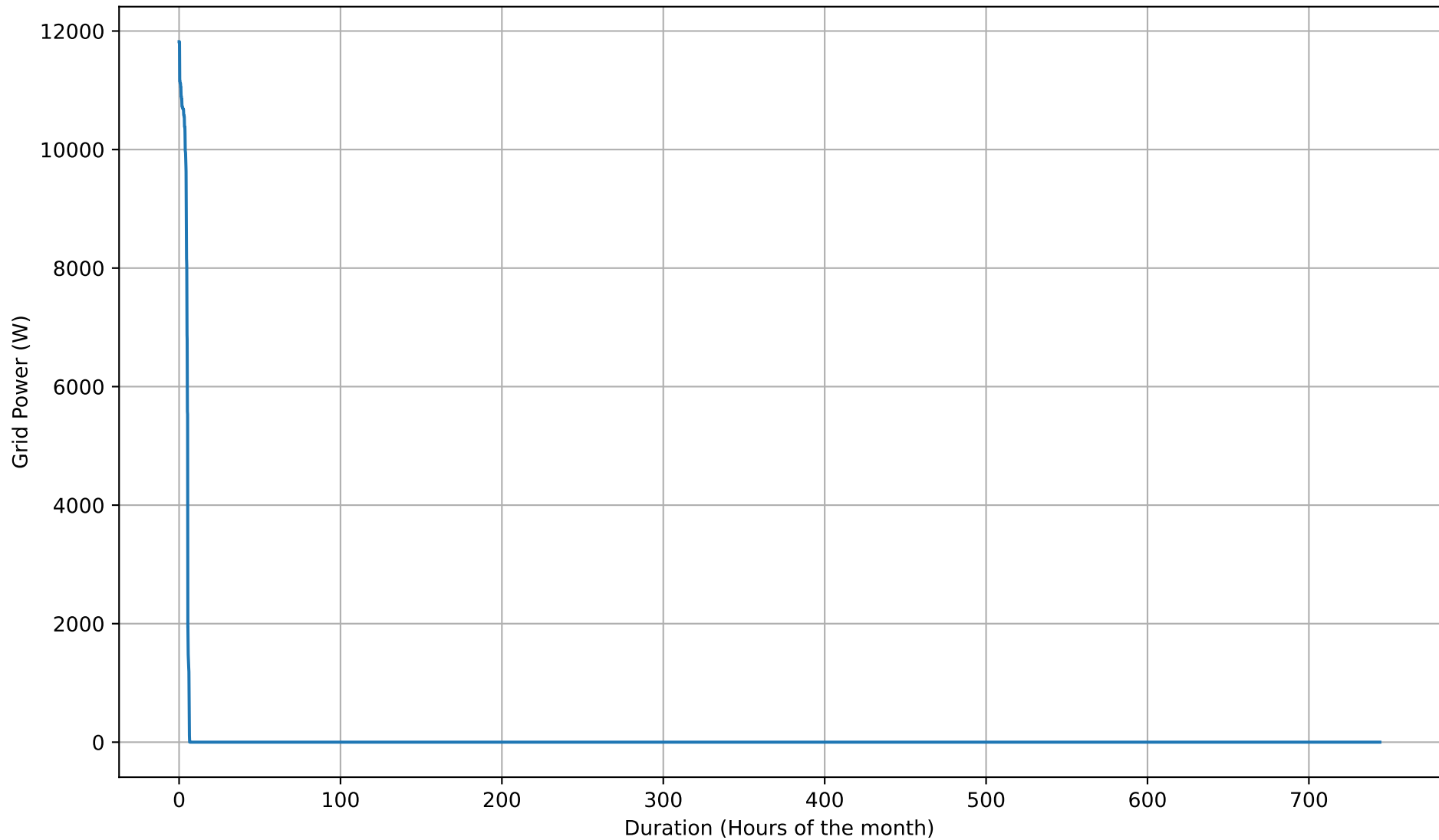
Grid Import Duration Curve - 50kWh - Jul
