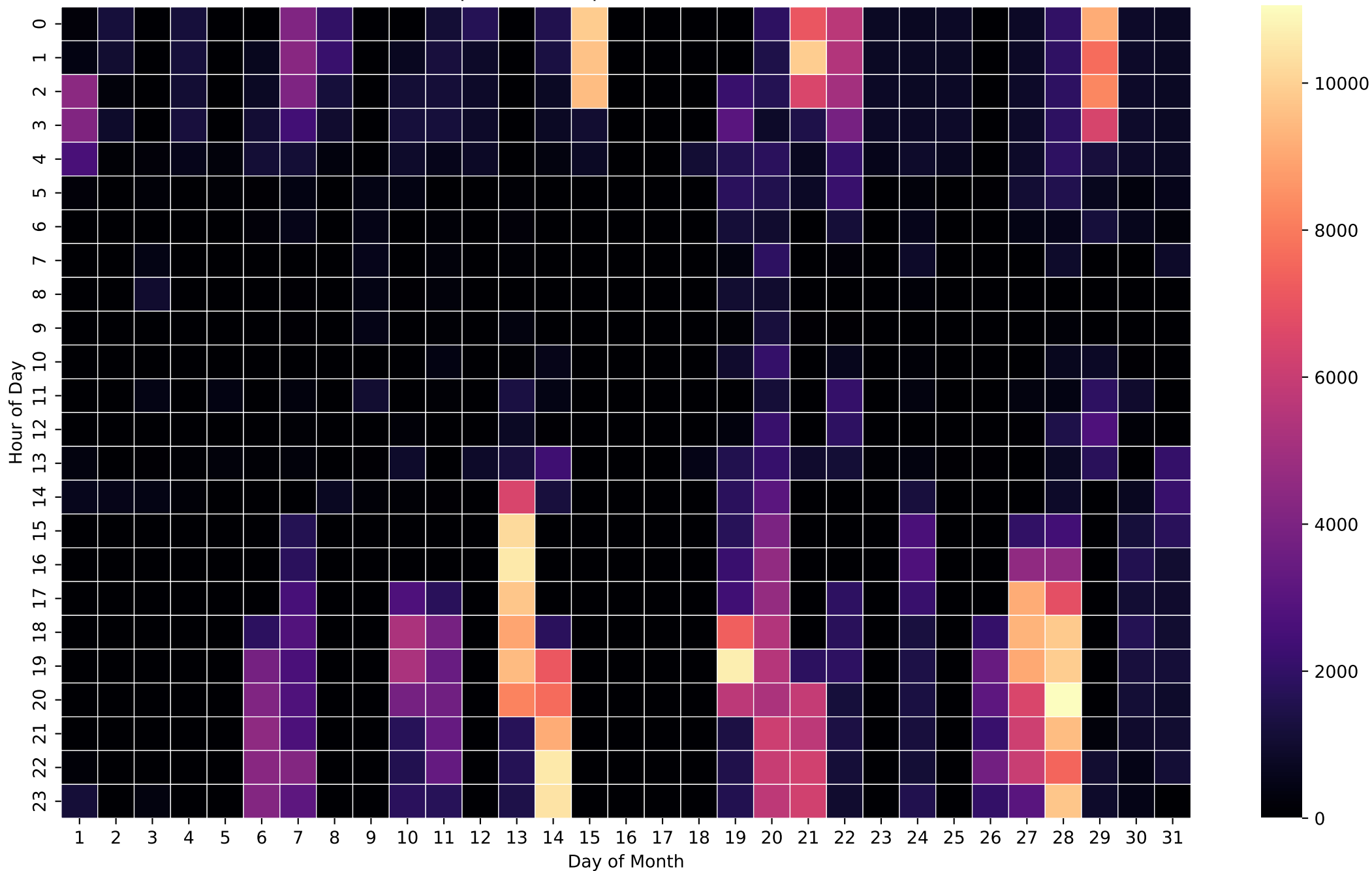
Grid Import Heatmap (Wh/Hour) - 50kWh - Oct
