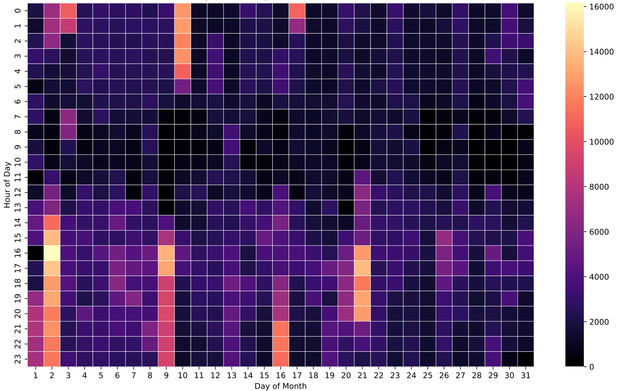
Grid Import Heatmap (Wh/Hour) - 50kWh - Dec
