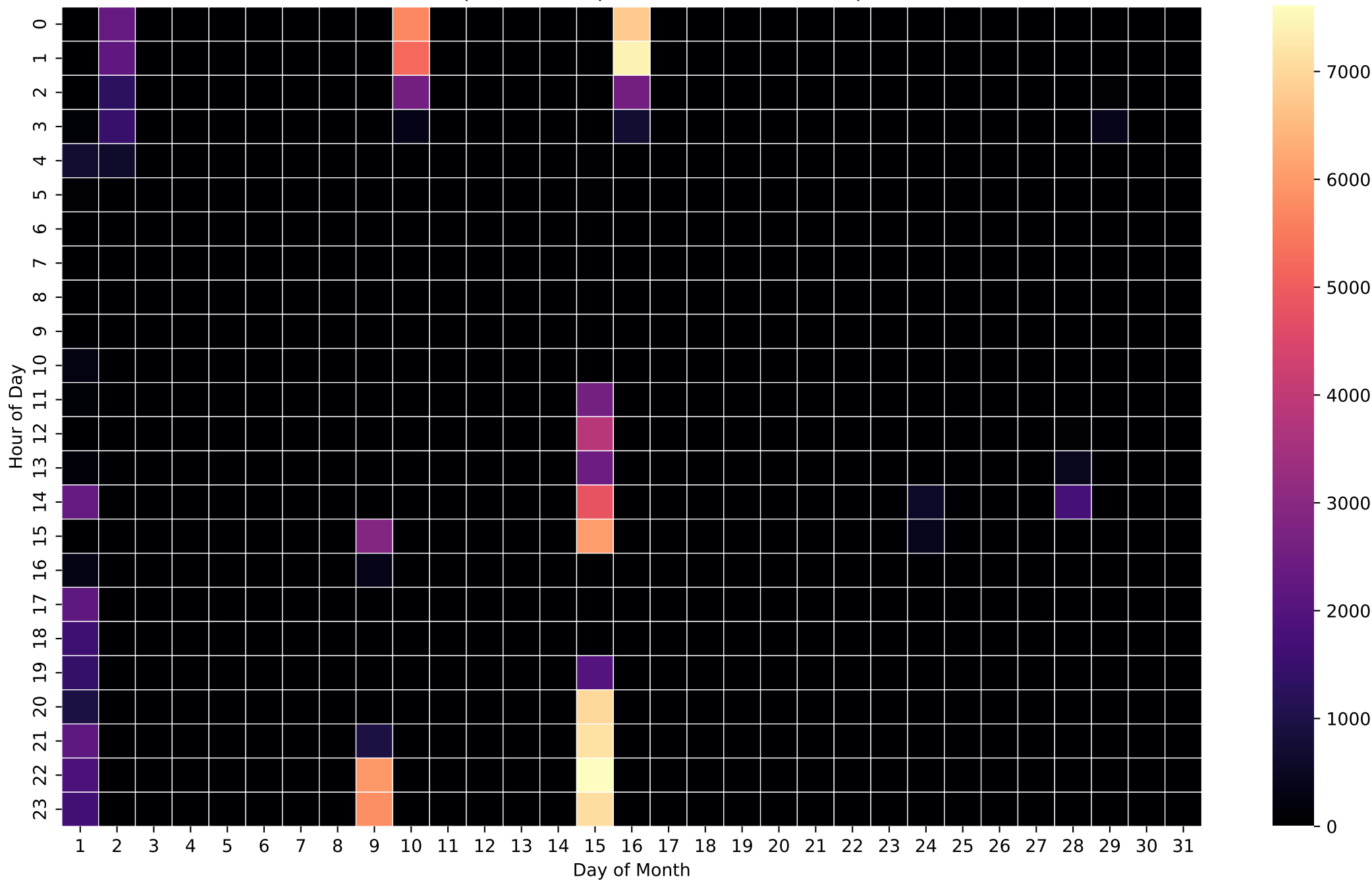
Grid Import Heatmap (Wh/Hour) - 50kWh - Apr
