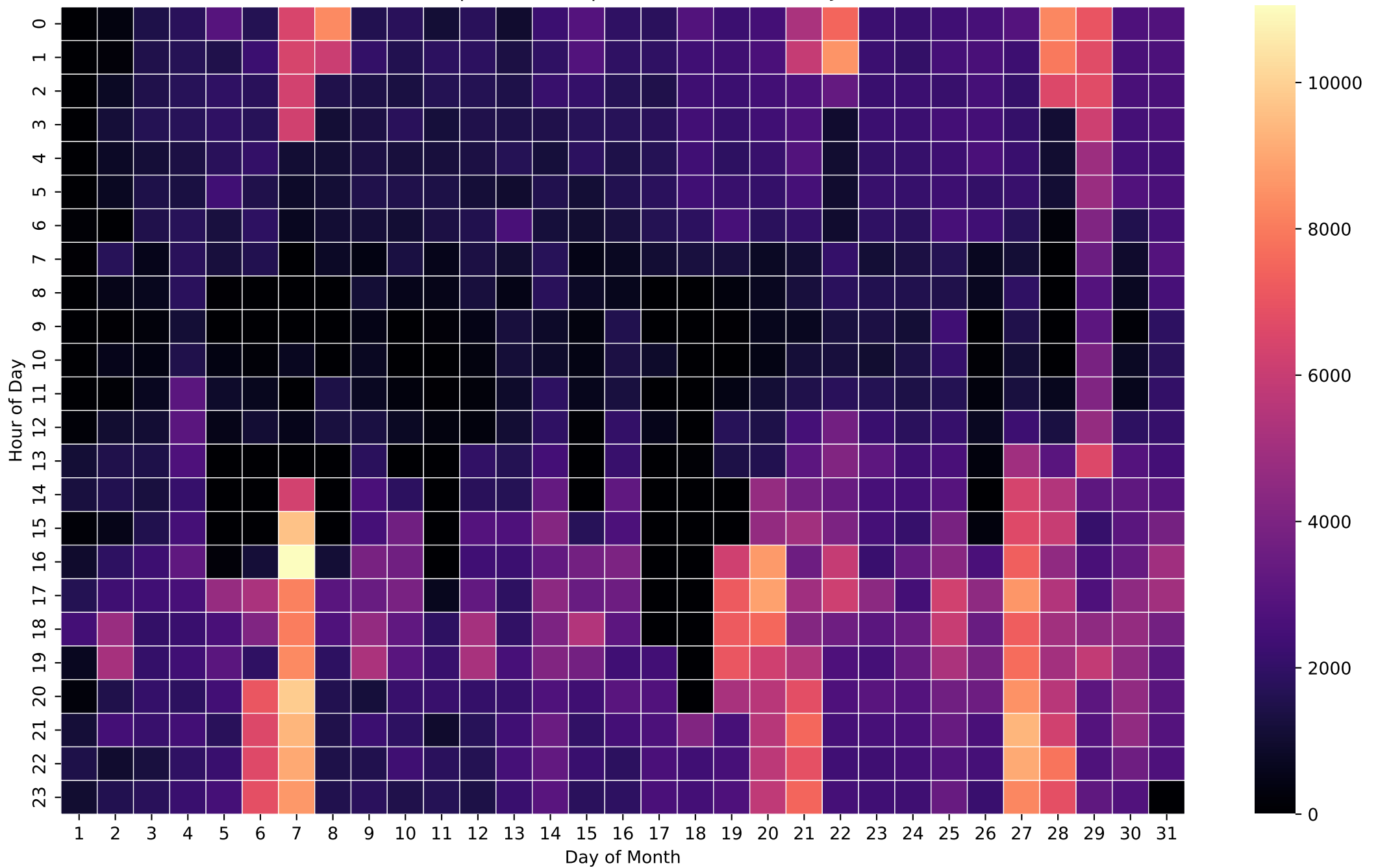
Grid Import Heatmap (Wh/Hour) - 50kWh - Jan
