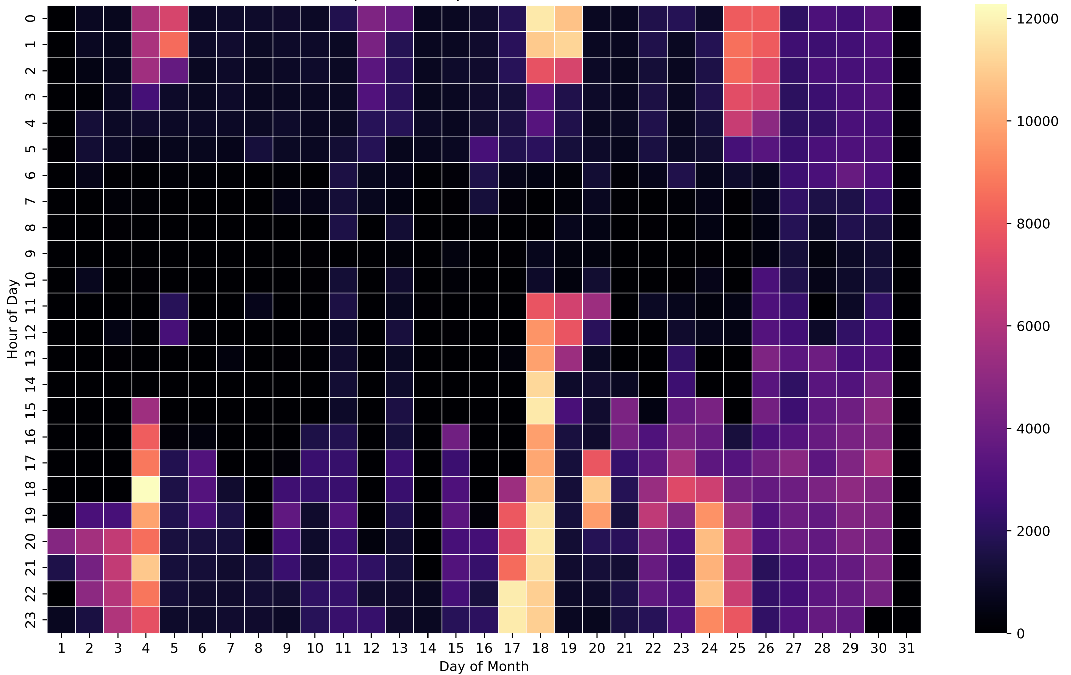
Grid Import Heatmap (Wh/Hour) - 50kWh - Nov
