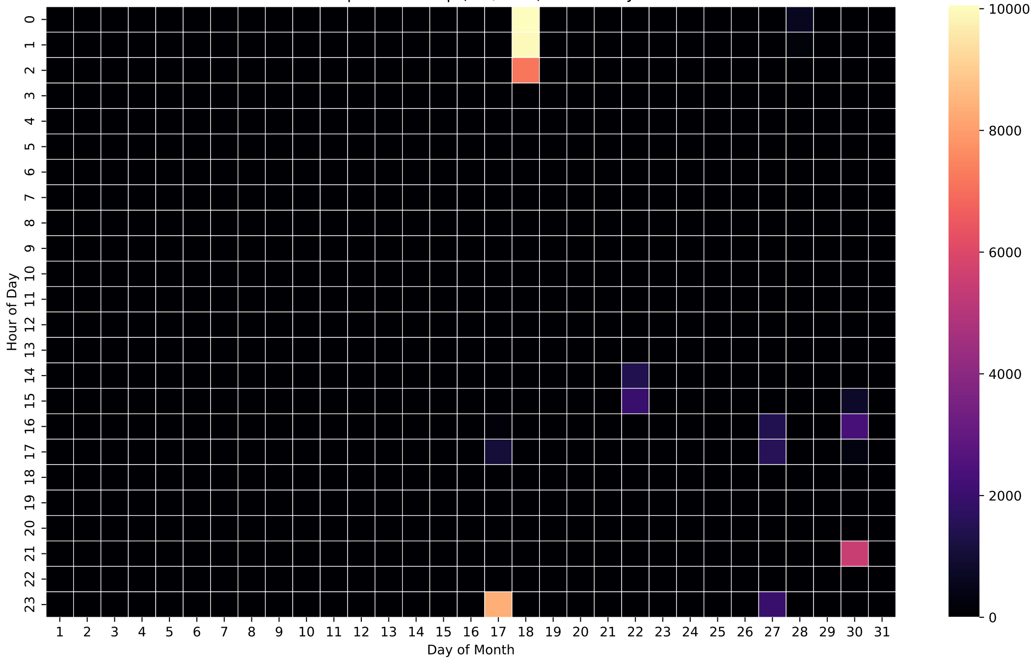
Grid Import Heatmap (Wh/Hour) - 50kWh - Jun
