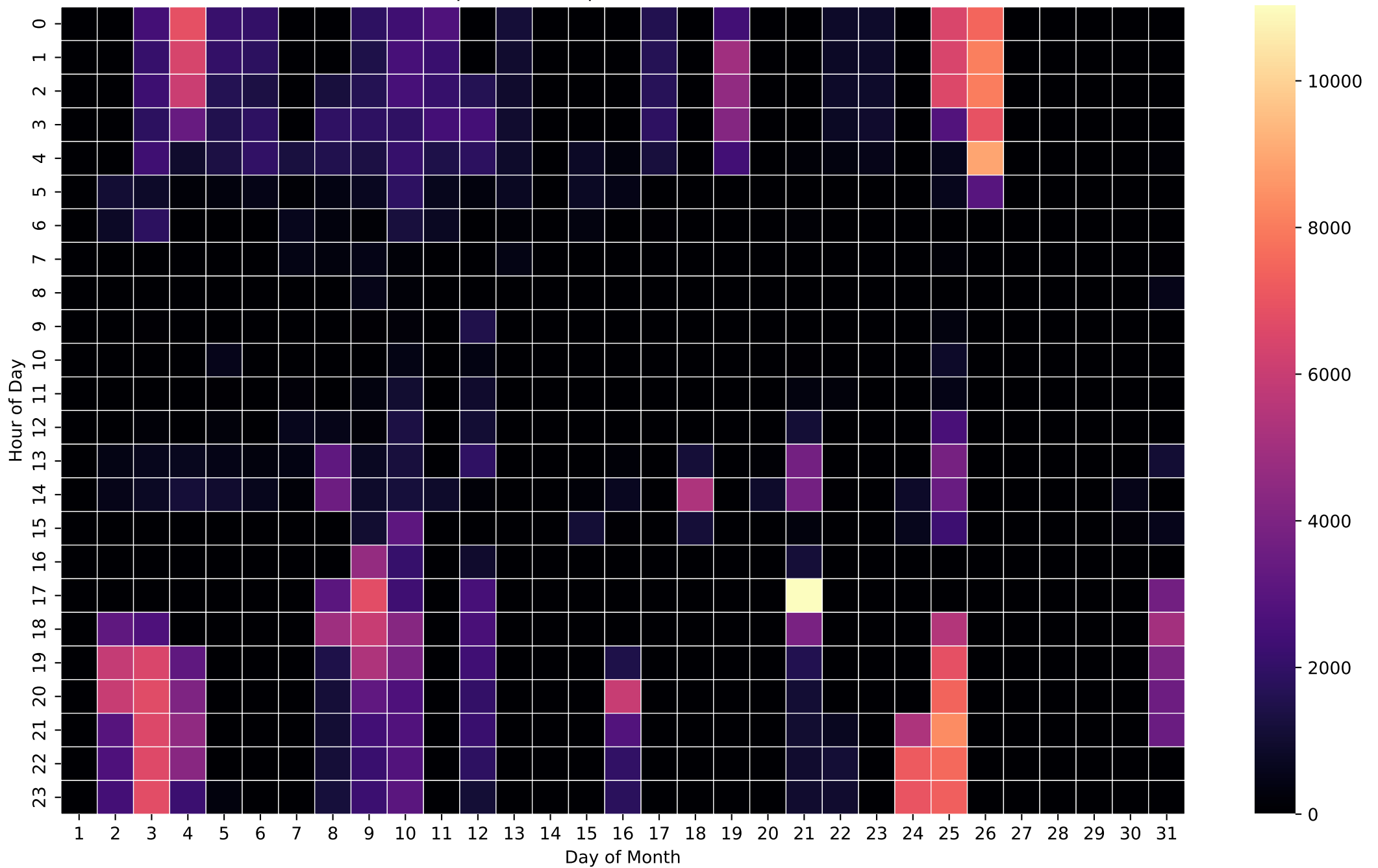
Grid Import Heatmap (Wh/Hour) - 50kWh - Mar
