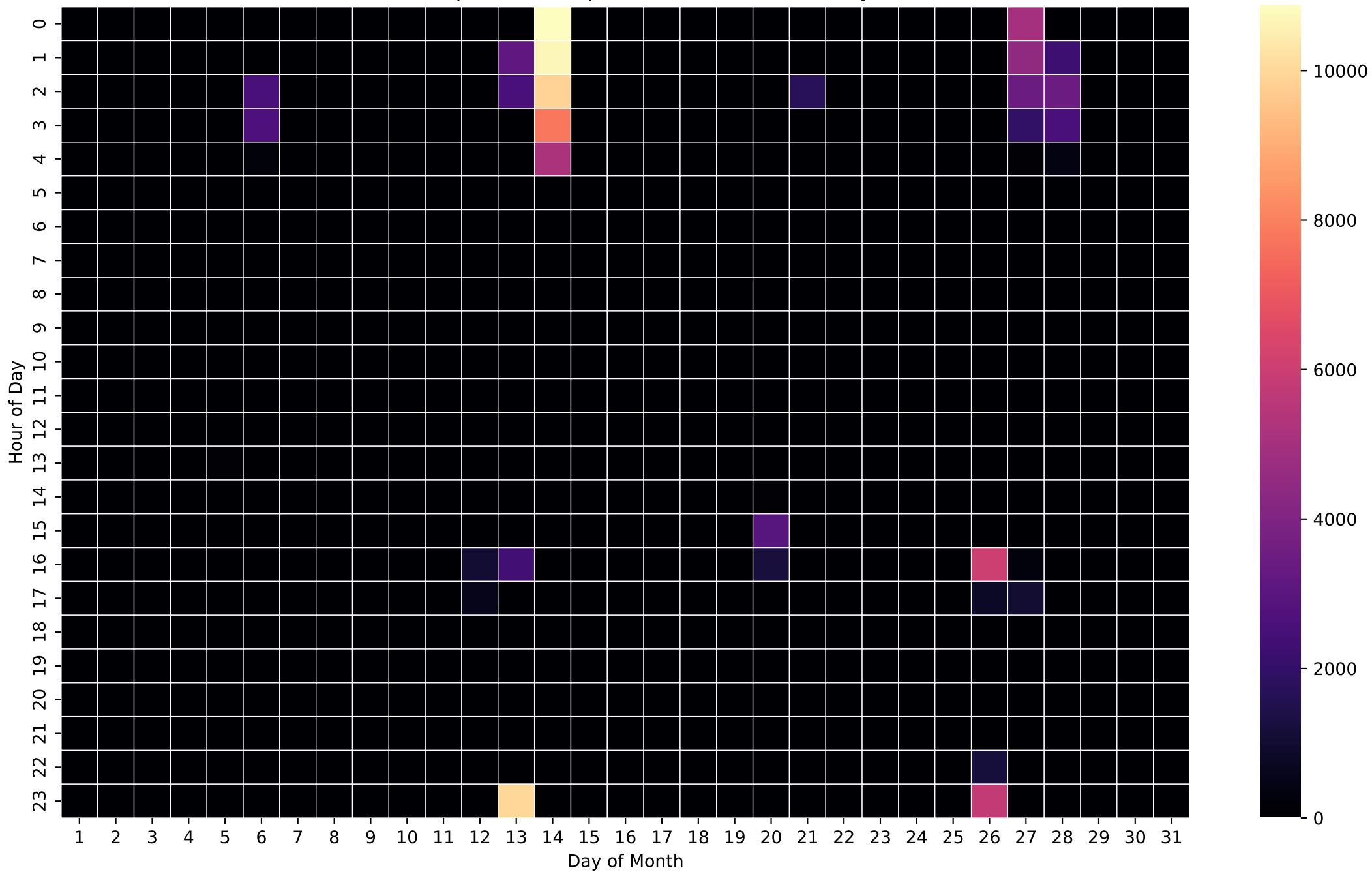
Grid Import Heatmap (Wh/Hour) - 50kWh - May
