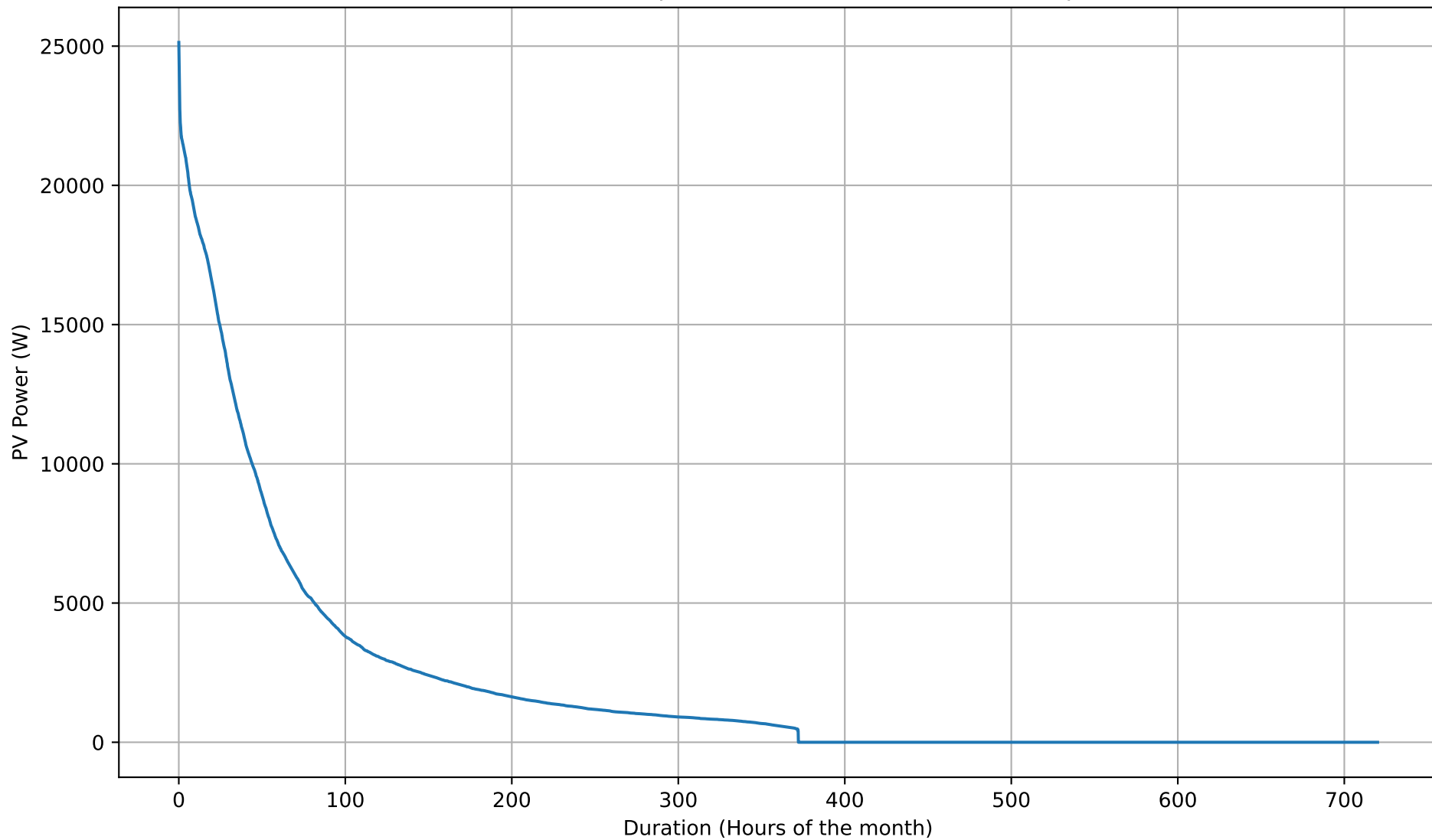
PV Self-Consumption Duration Curve - 50kWh - Apr
