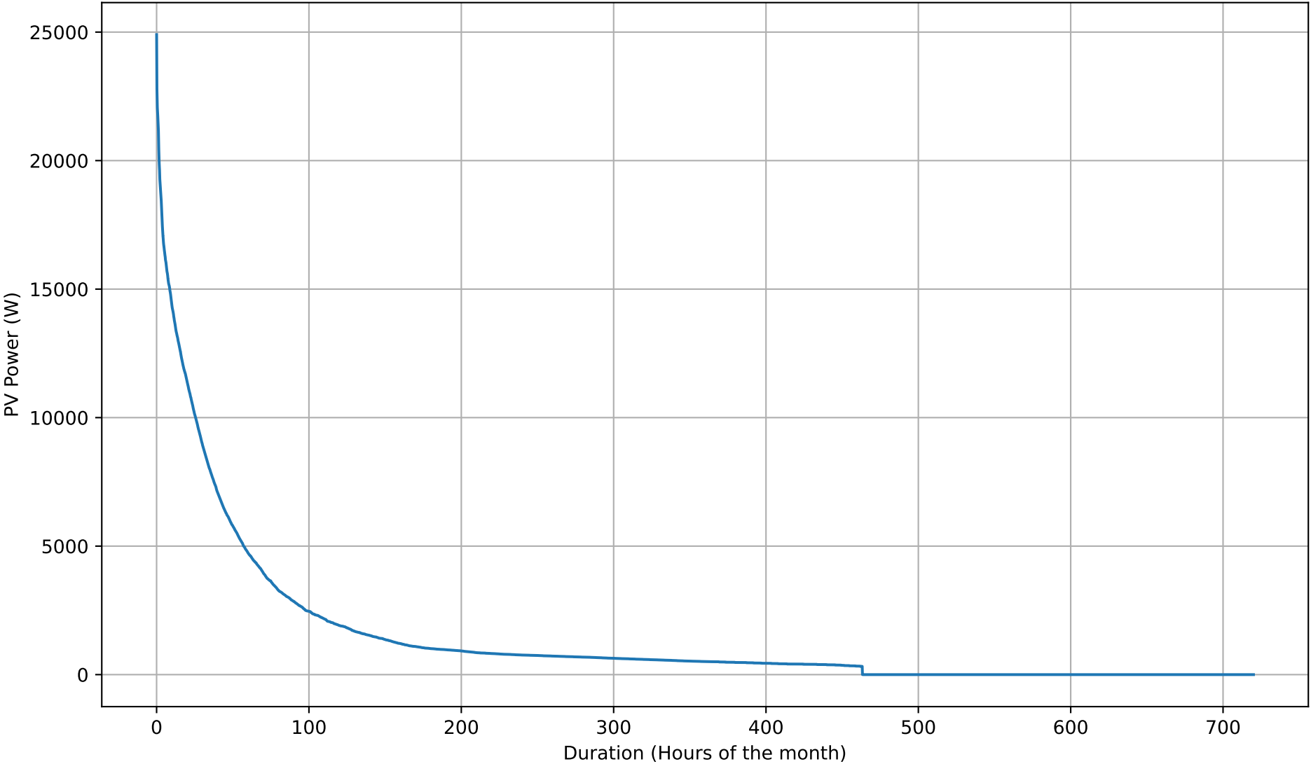
PV Self-Consumption Duration Curve - 50kWh - Jun
