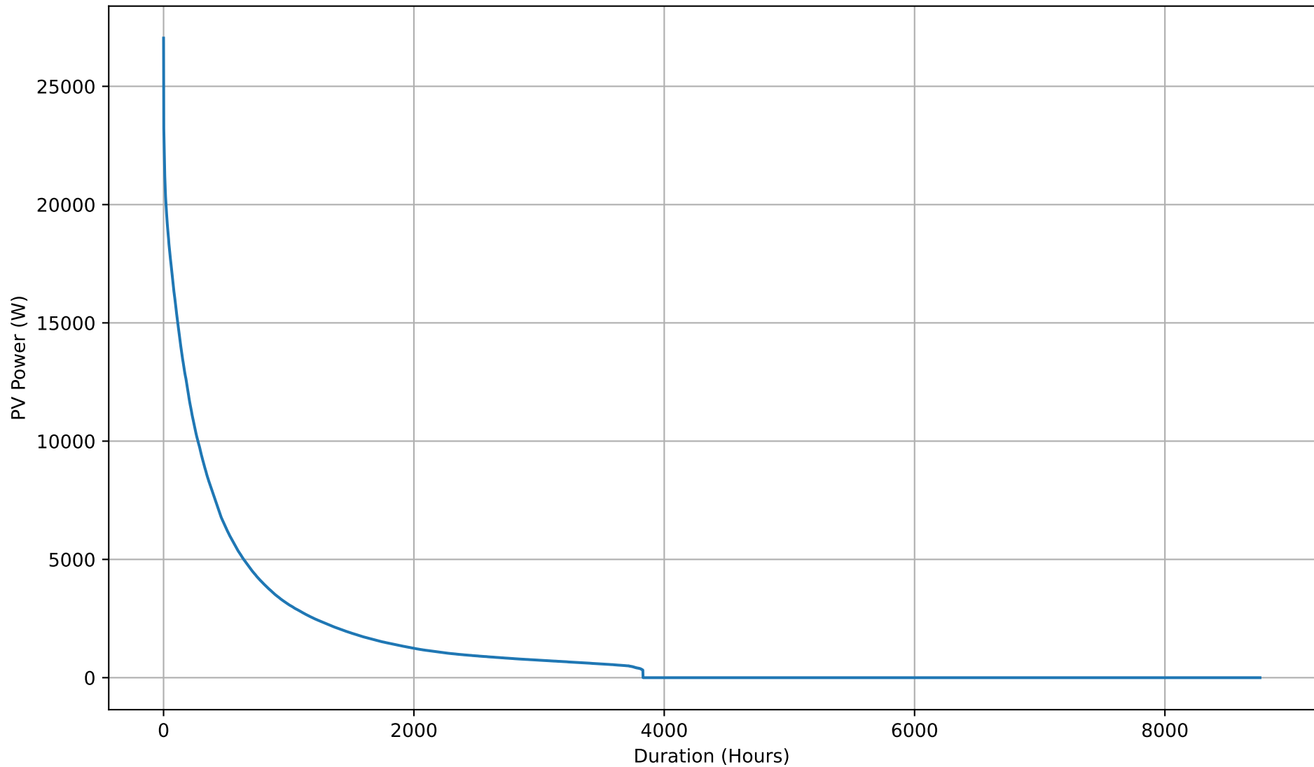
Yearly PV Self-Consumption Duration Curve - 50kWh
