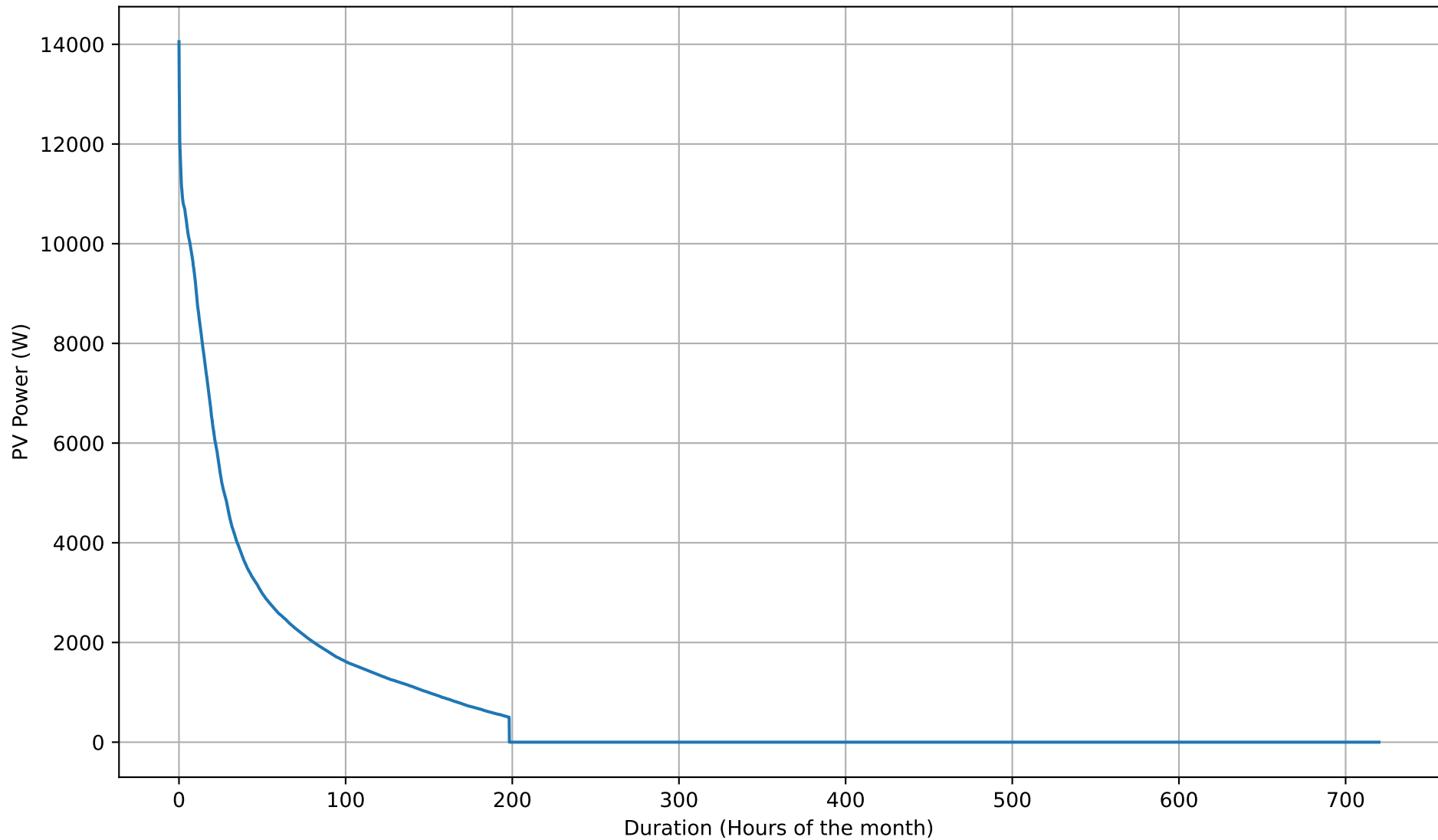
PV Self-Consumption Duration Curve - 50kWh - Nov
