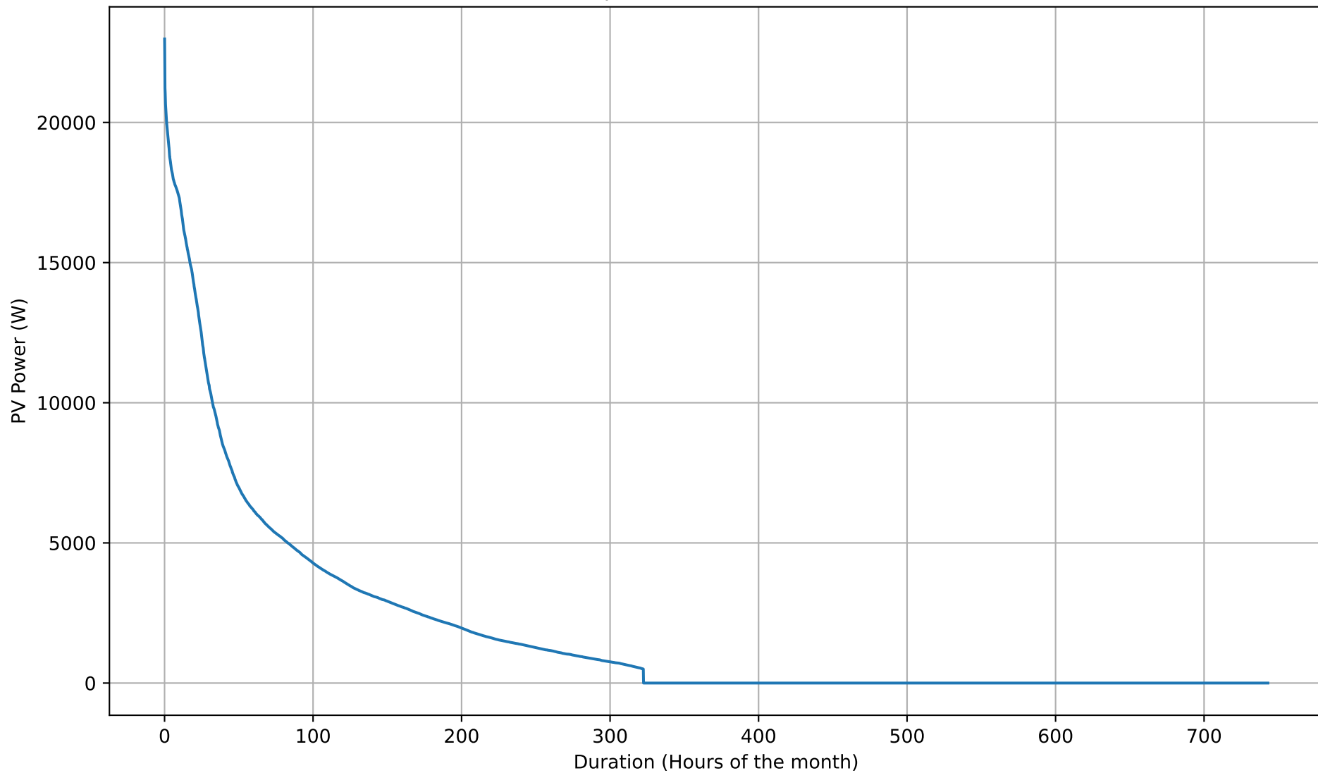
PV Self-Consumption Duration Curve - 50kWh - Mar
