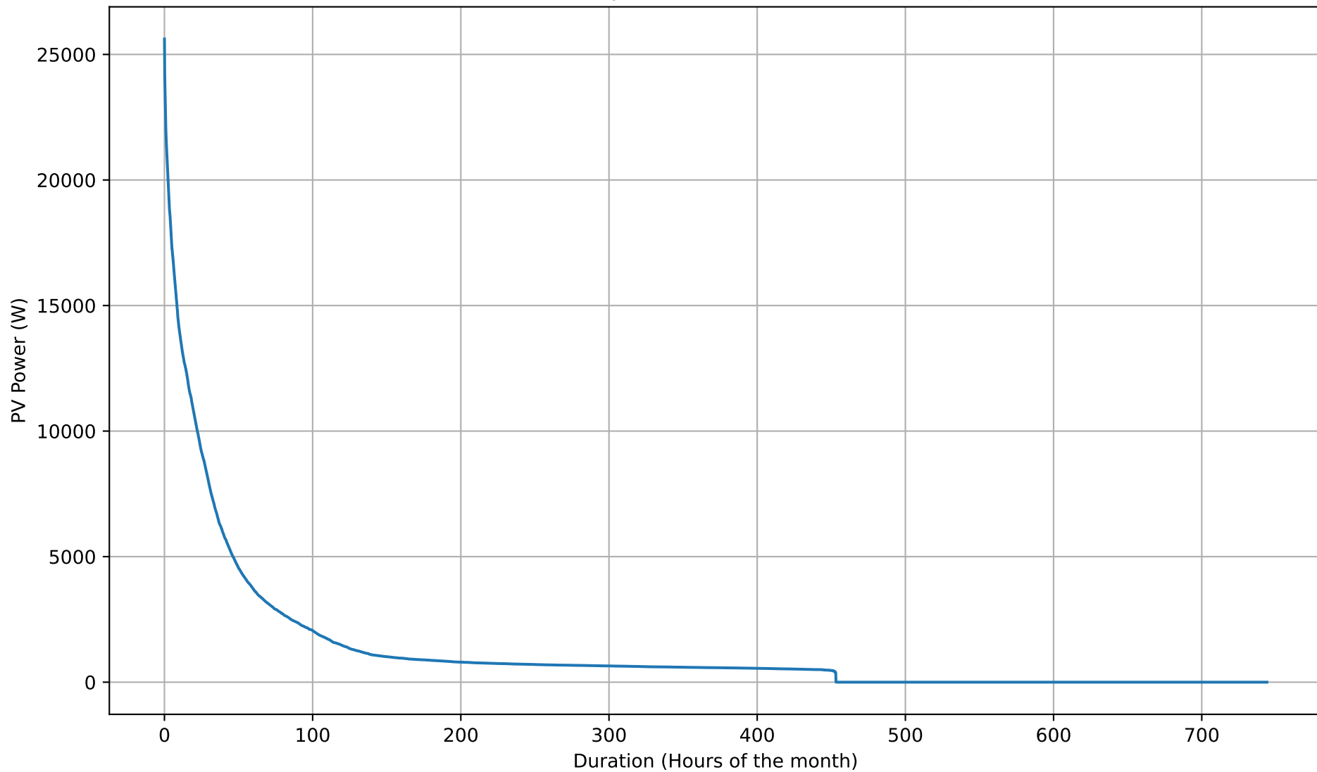
PV Self-Consumption Duration Curve - 50kWh - Jul
