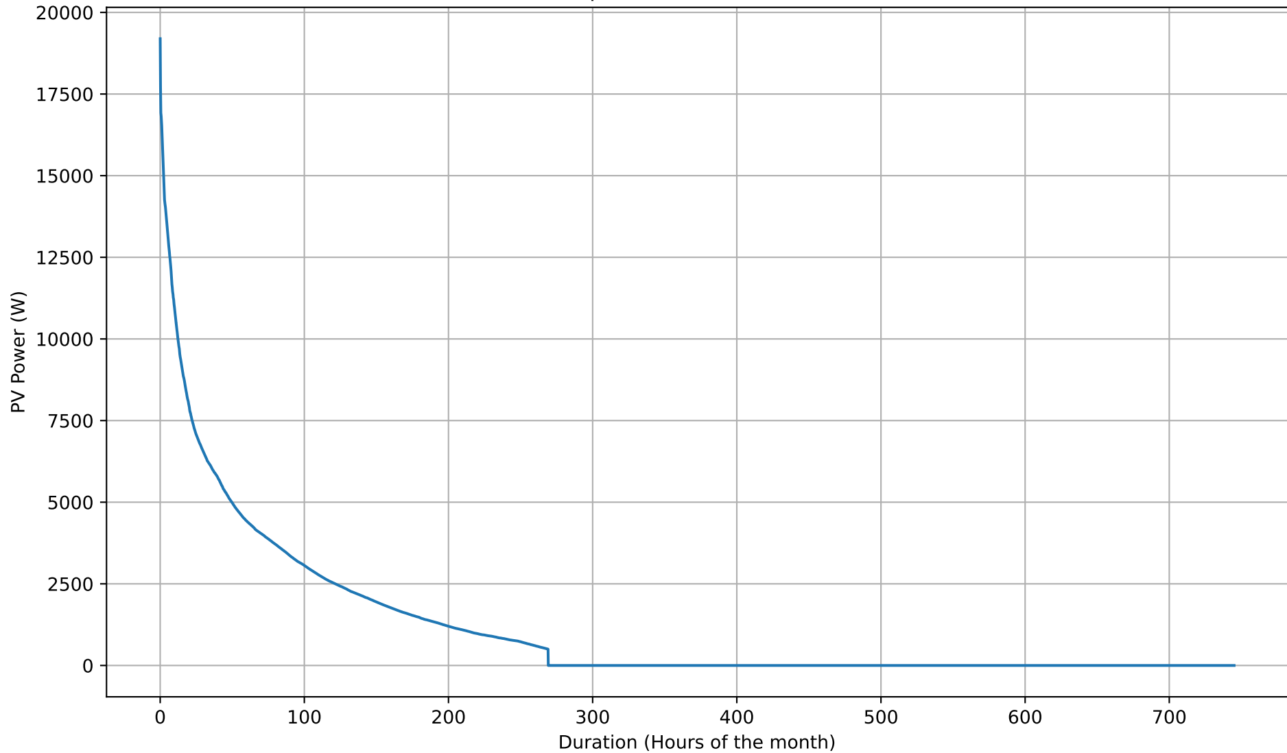
PV Self-Consumption Duration Curve - 50kWh - Oct
