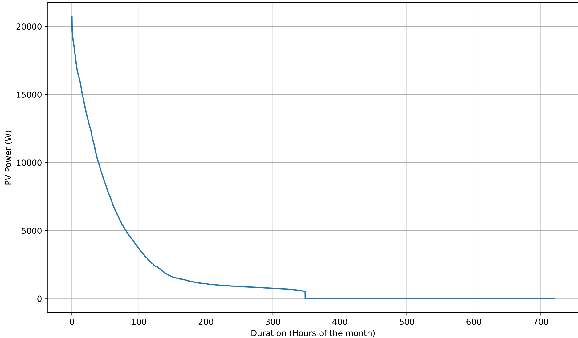
PV Self-Consumption Duration Curve - 50kWh - Sep
