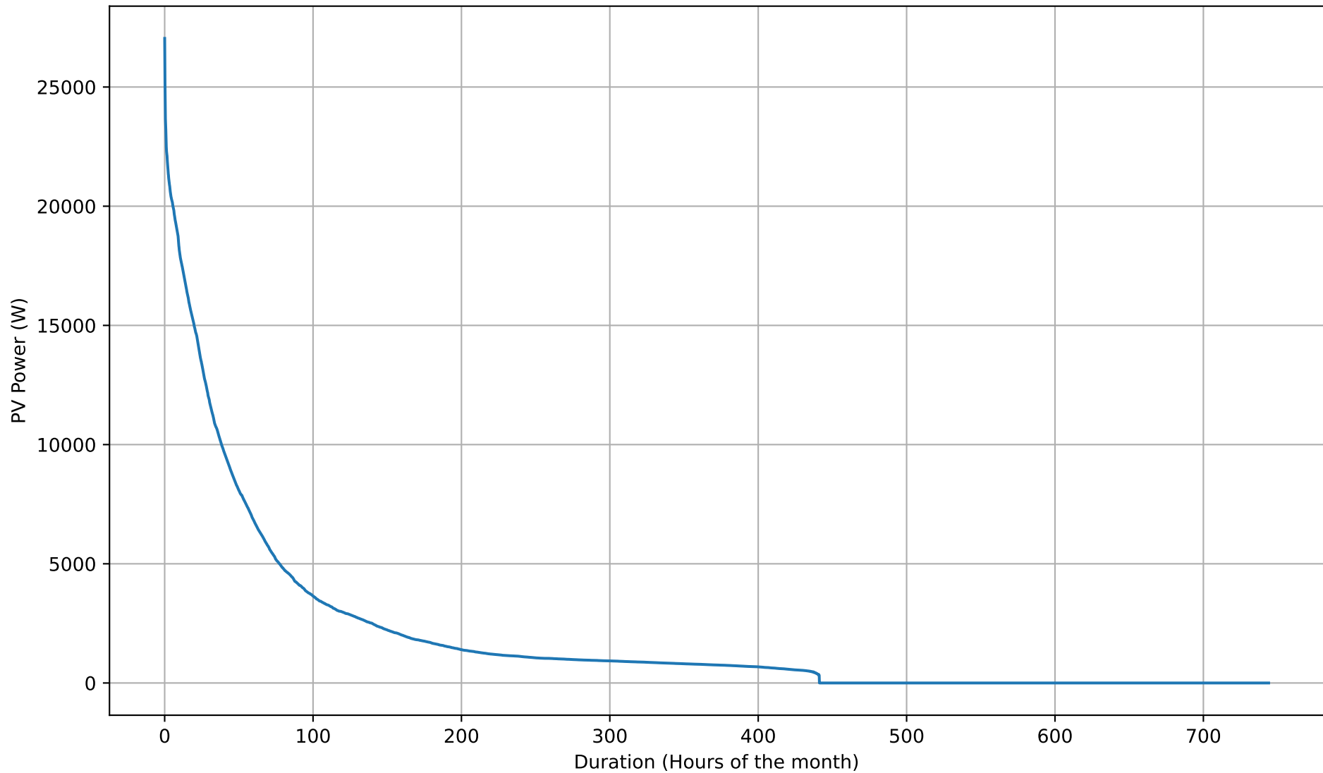
PV Self-Consumption Duration Curve - 50kWh - May
