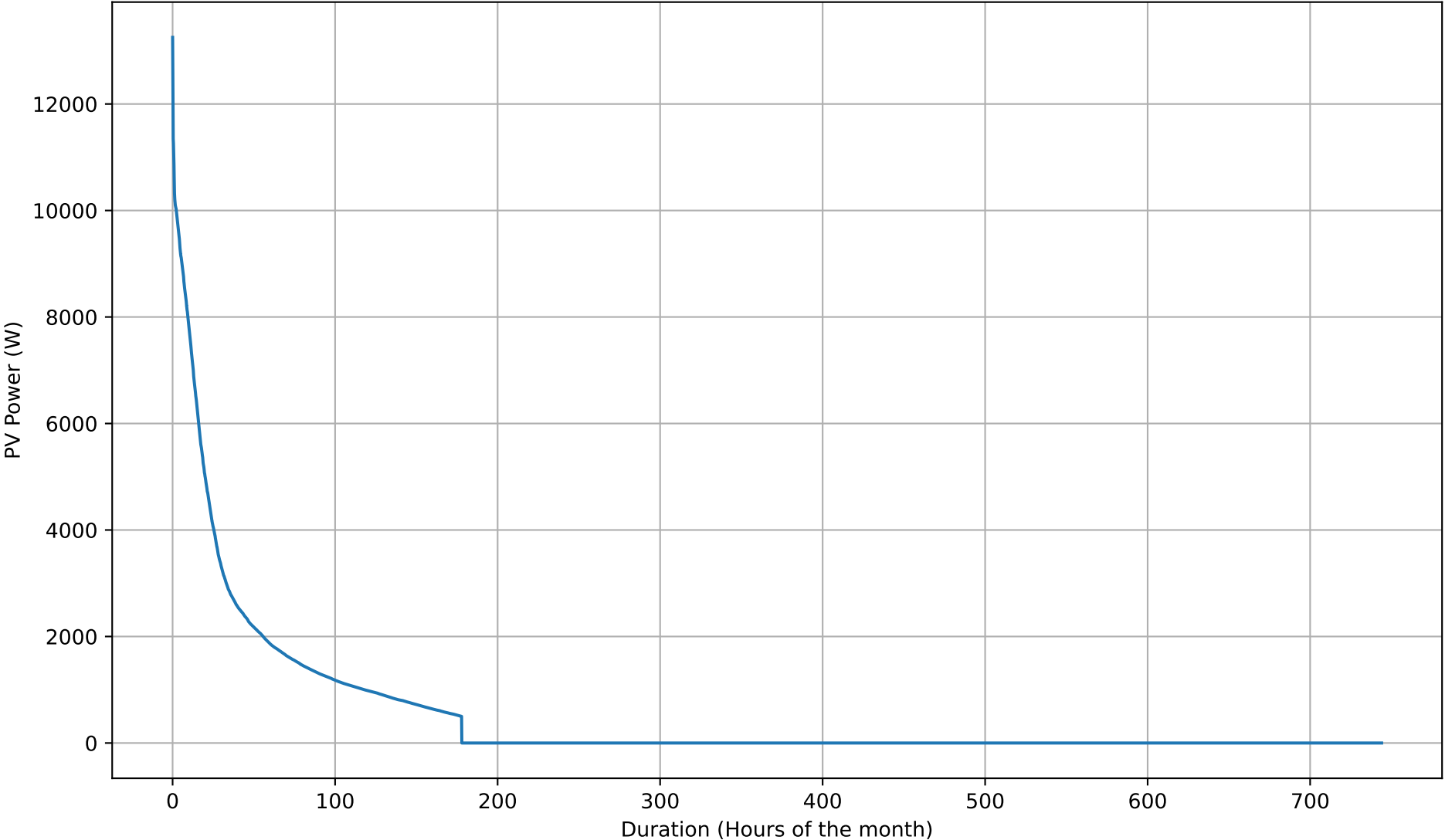
PV Self-Consumption Duration Curve - 50kWh - Jan
