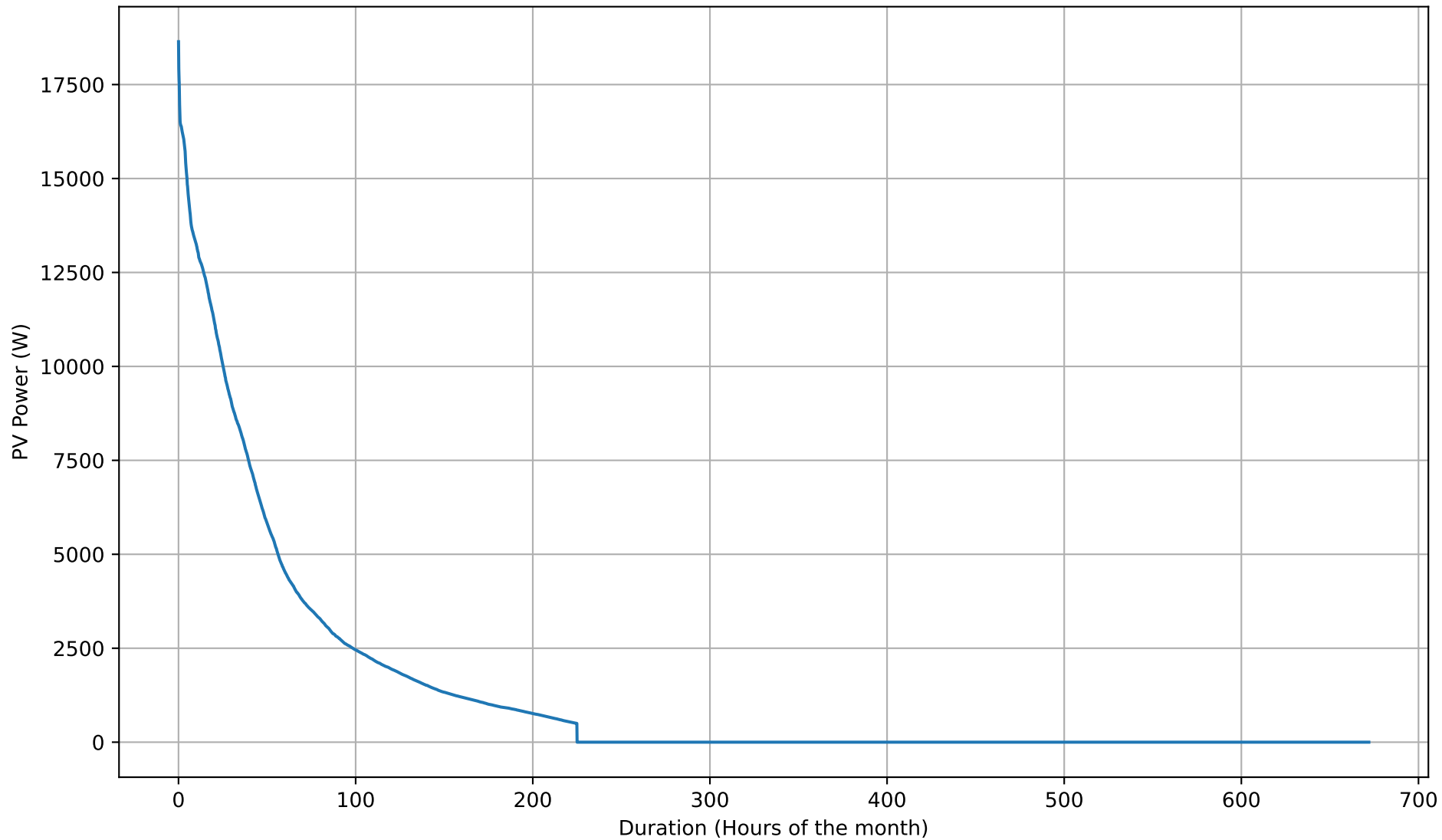
PV Self-Consumption Duration Curve - 50kWh - Feb
