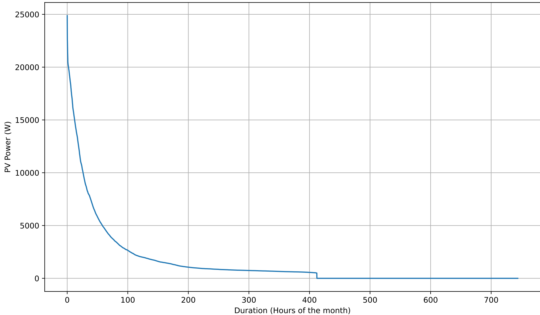
PV Self-Consumption Duration Curve - 50kWh - Aug
