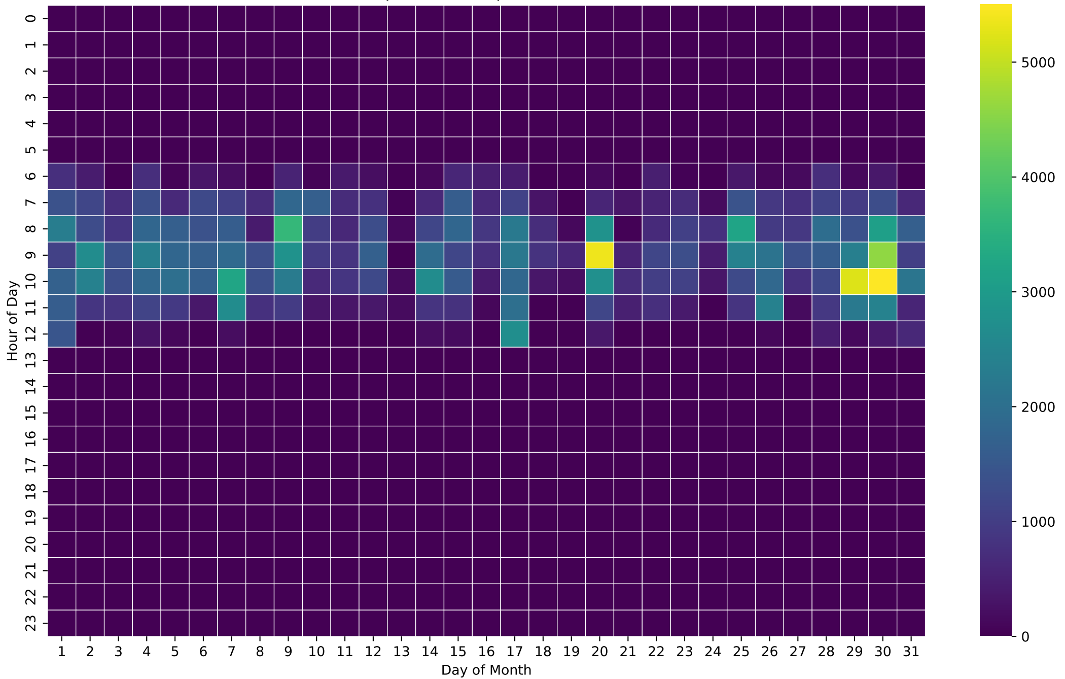
PV Self-Consumption Heatmap (Wh/Hour) - 50kWh - Dec
