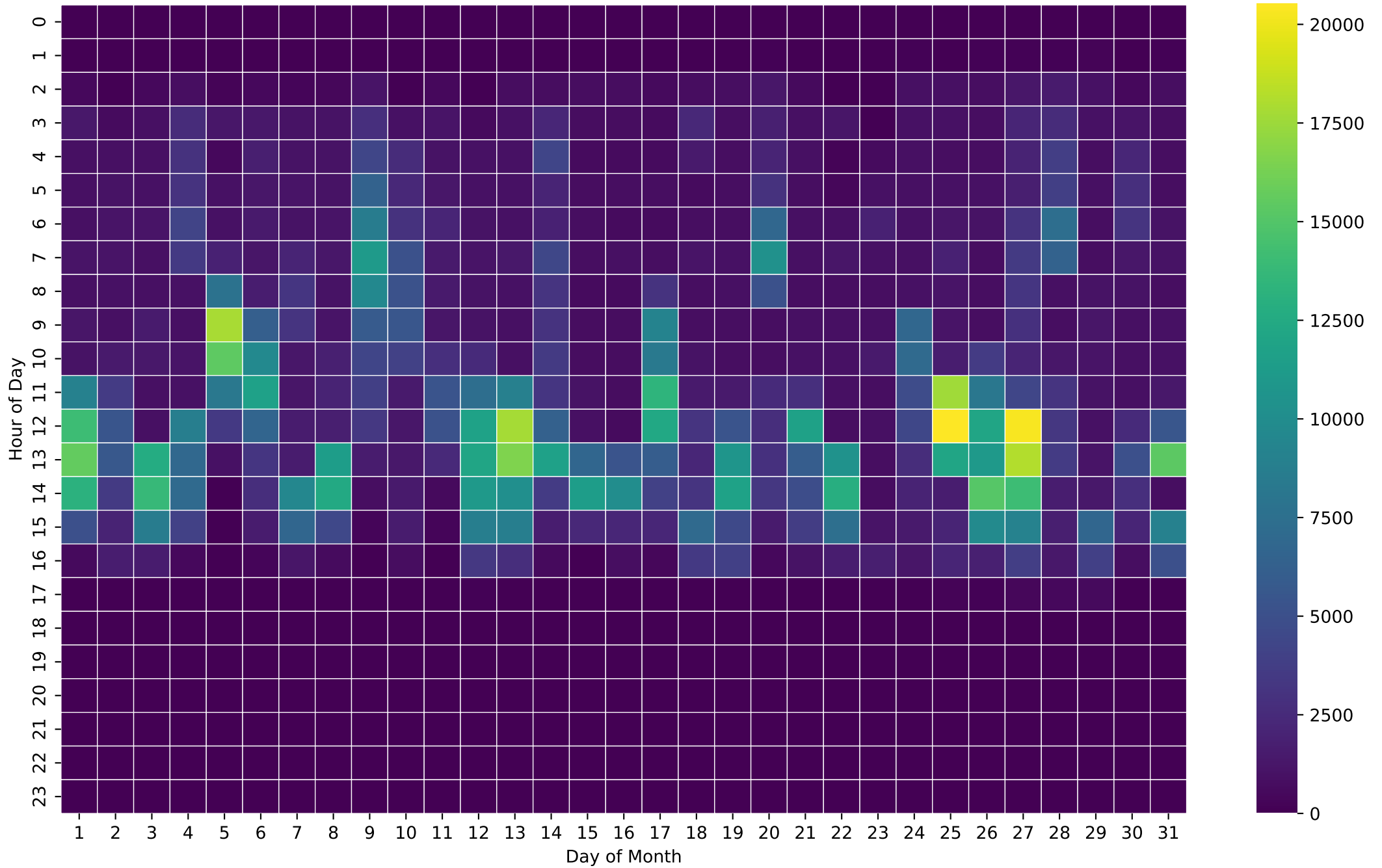
PV Self-Consumption Heatmap (Wh/Hour) - 50kWh - May
