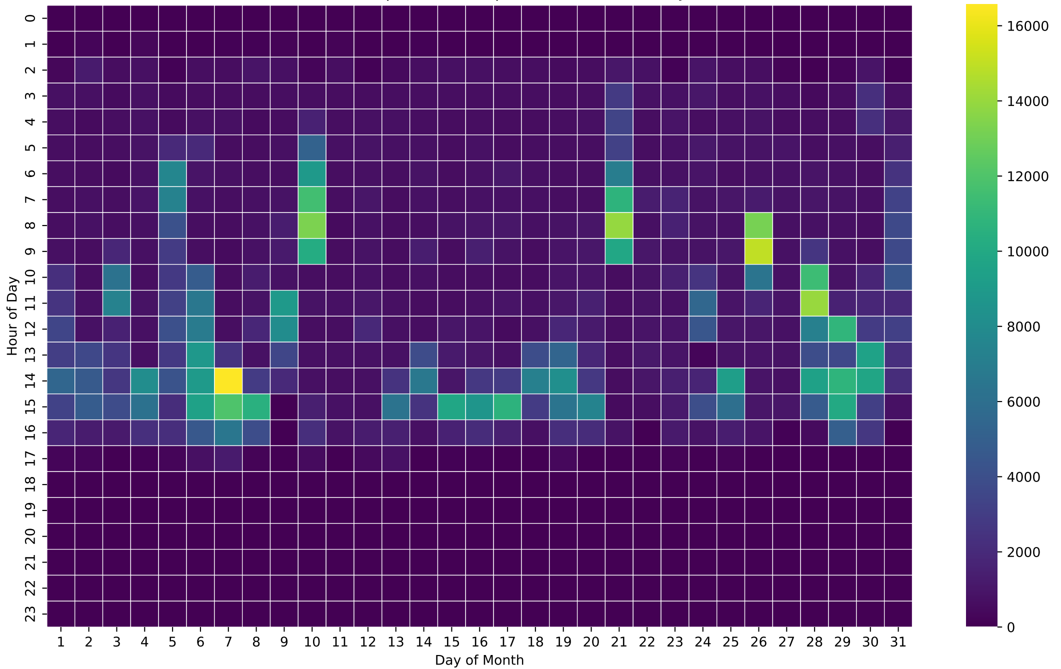
PV Self-Consumption Heatmap (Wh/Hour) - 50kWh - Jul
