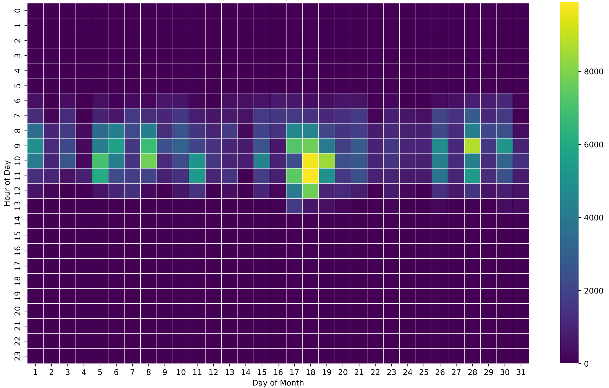
PV Self-Consumption Heatmap (Wh/Hour) - 50kWh - Jan
