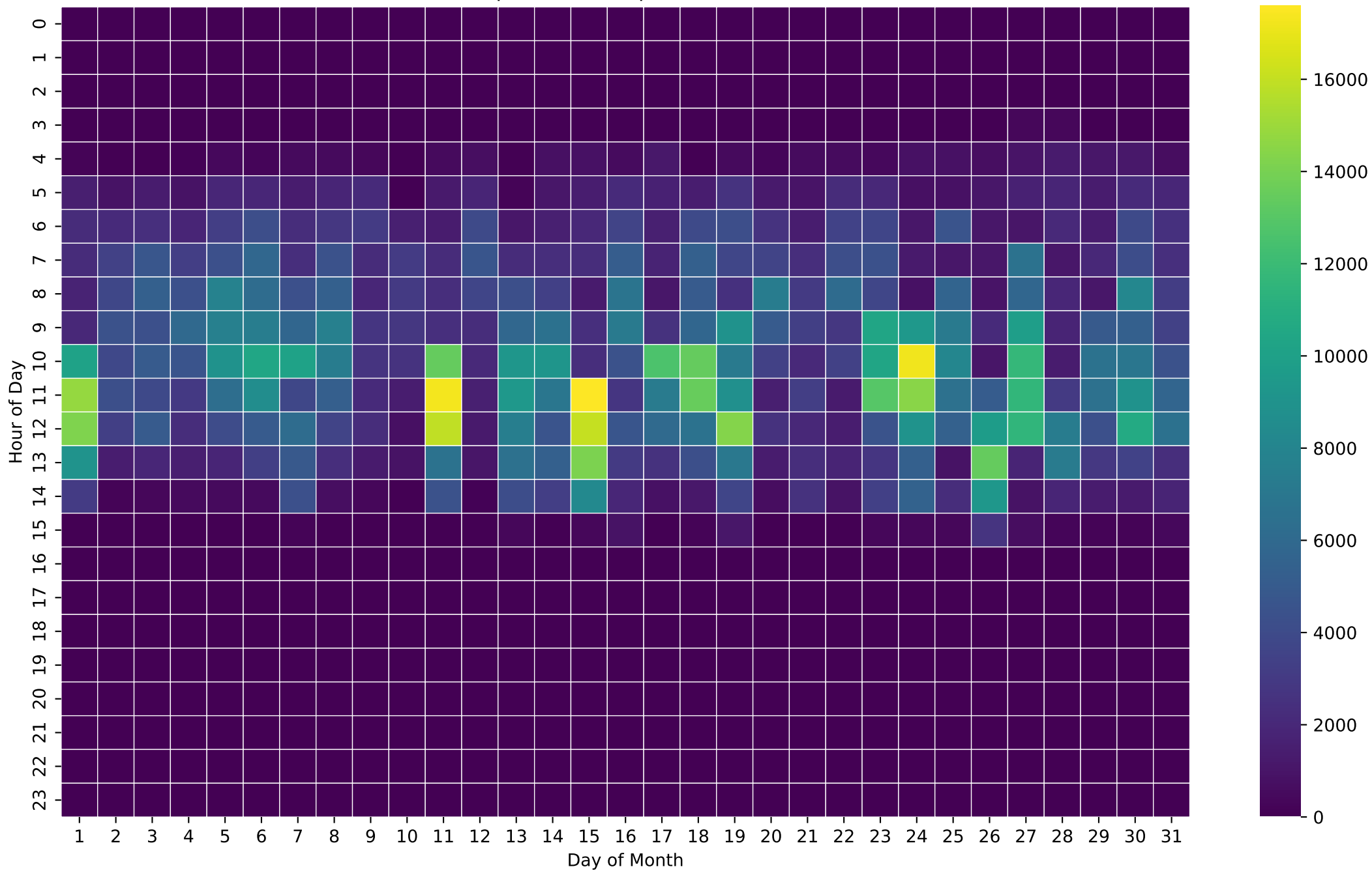
PV Self-Consumption Heatmap (Wh/Hour) - 50kWh - Mar
