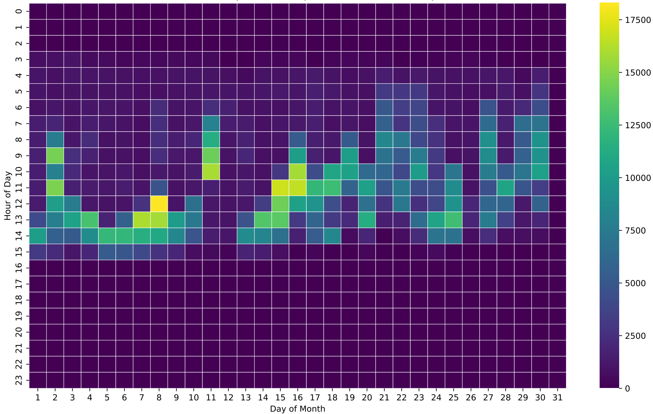
PV Self-Consumption Heatmap (Wh/Hour) - 50kWh - Sep
