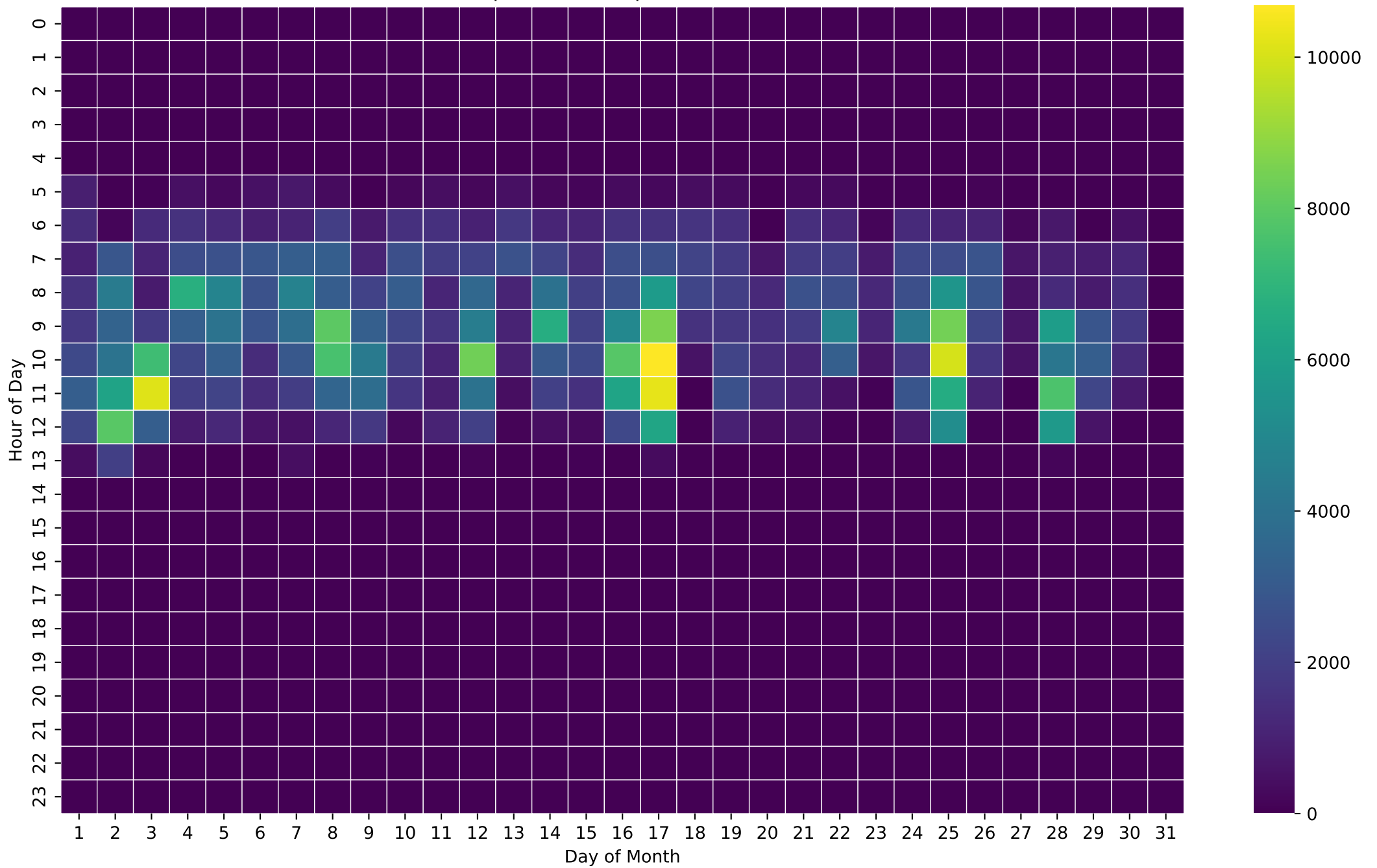
PV Self-Consumption Heatmap (Wh/Hour) - 50kWh - Nov
