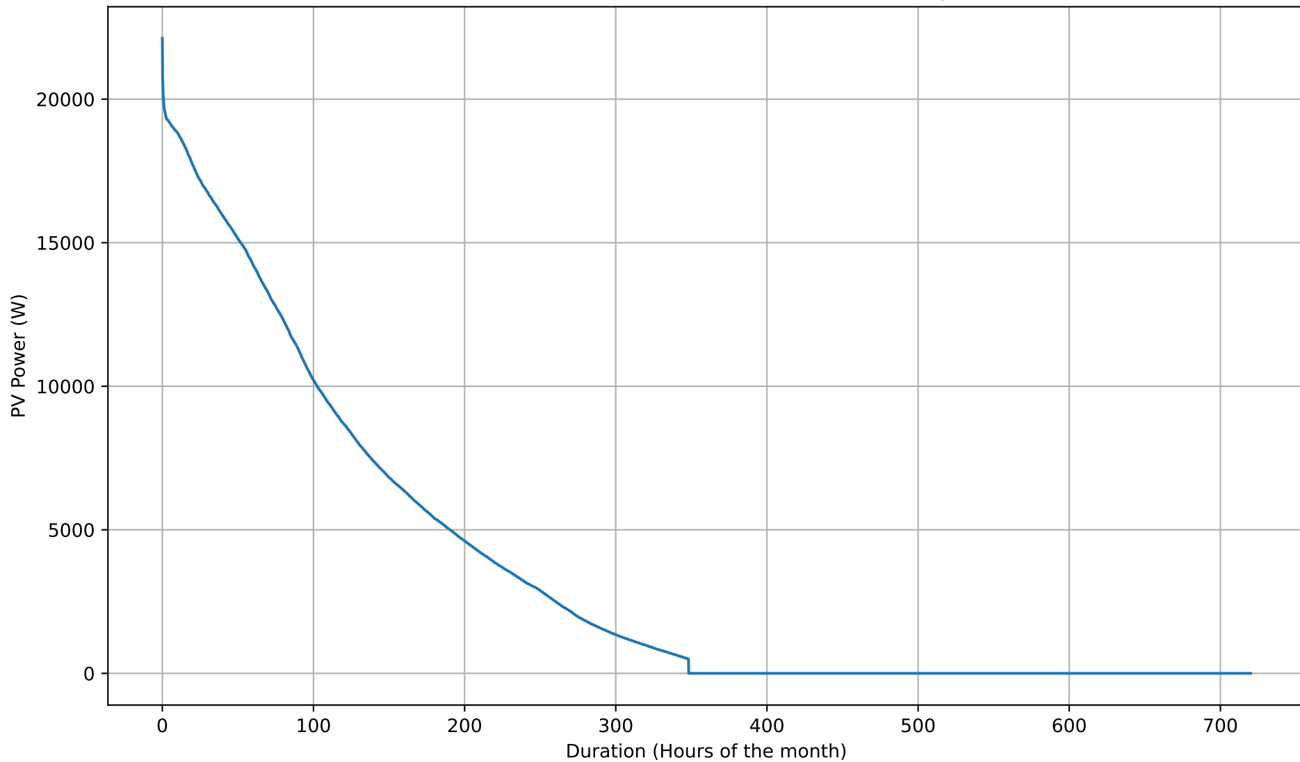
PV Production Duration Curve - 50kWh - Sep
