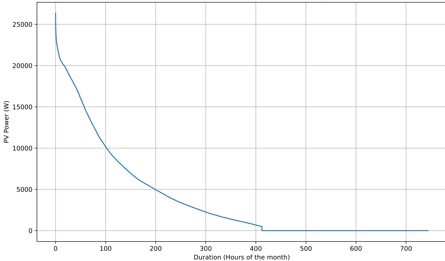
PV Production Duration Curve - 50kWh - Aug
