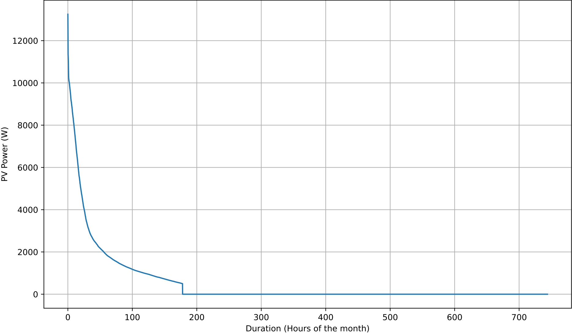
PV Production Duration Curve - 50kWh - Jan
