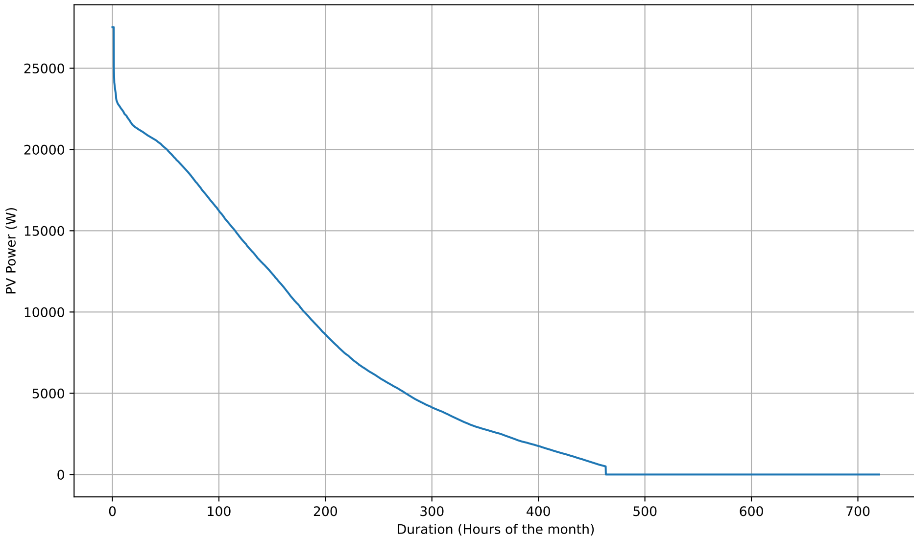
PV Production Duration Curve - 50kWh - Jun
