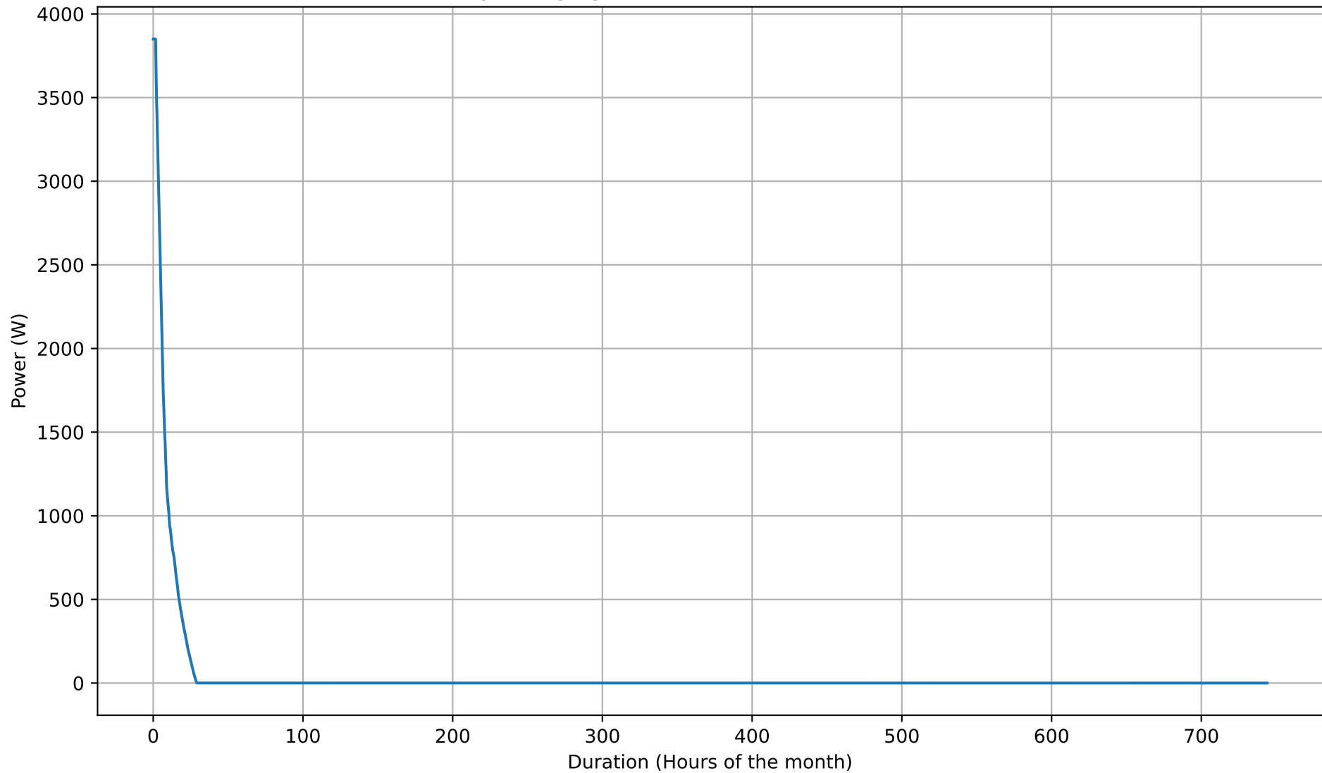
Battery Charging Power Duration Curve - 5kWh - Dec
