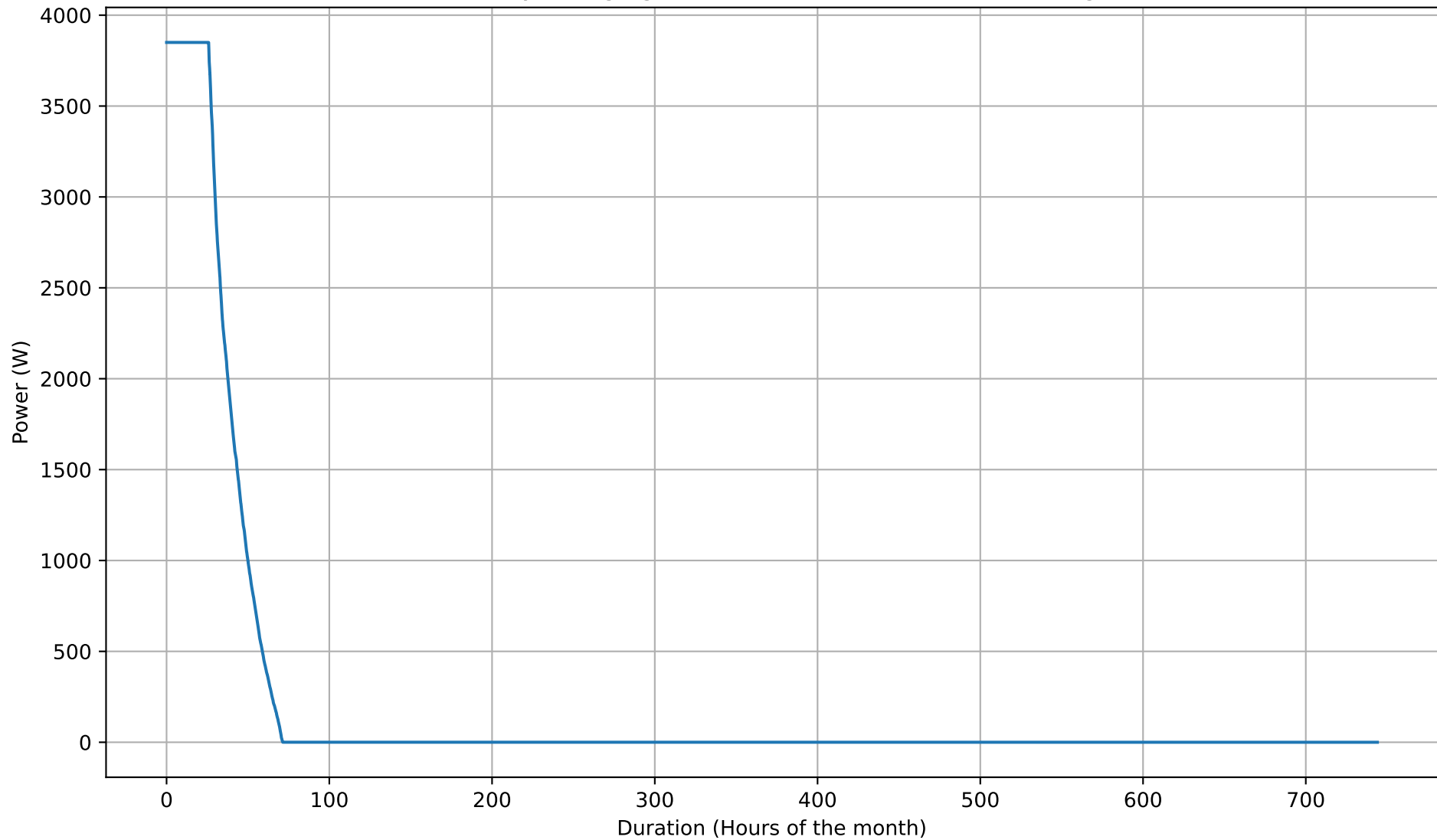
Battery Charging Power Duration Curve - 5kWh - Aug
