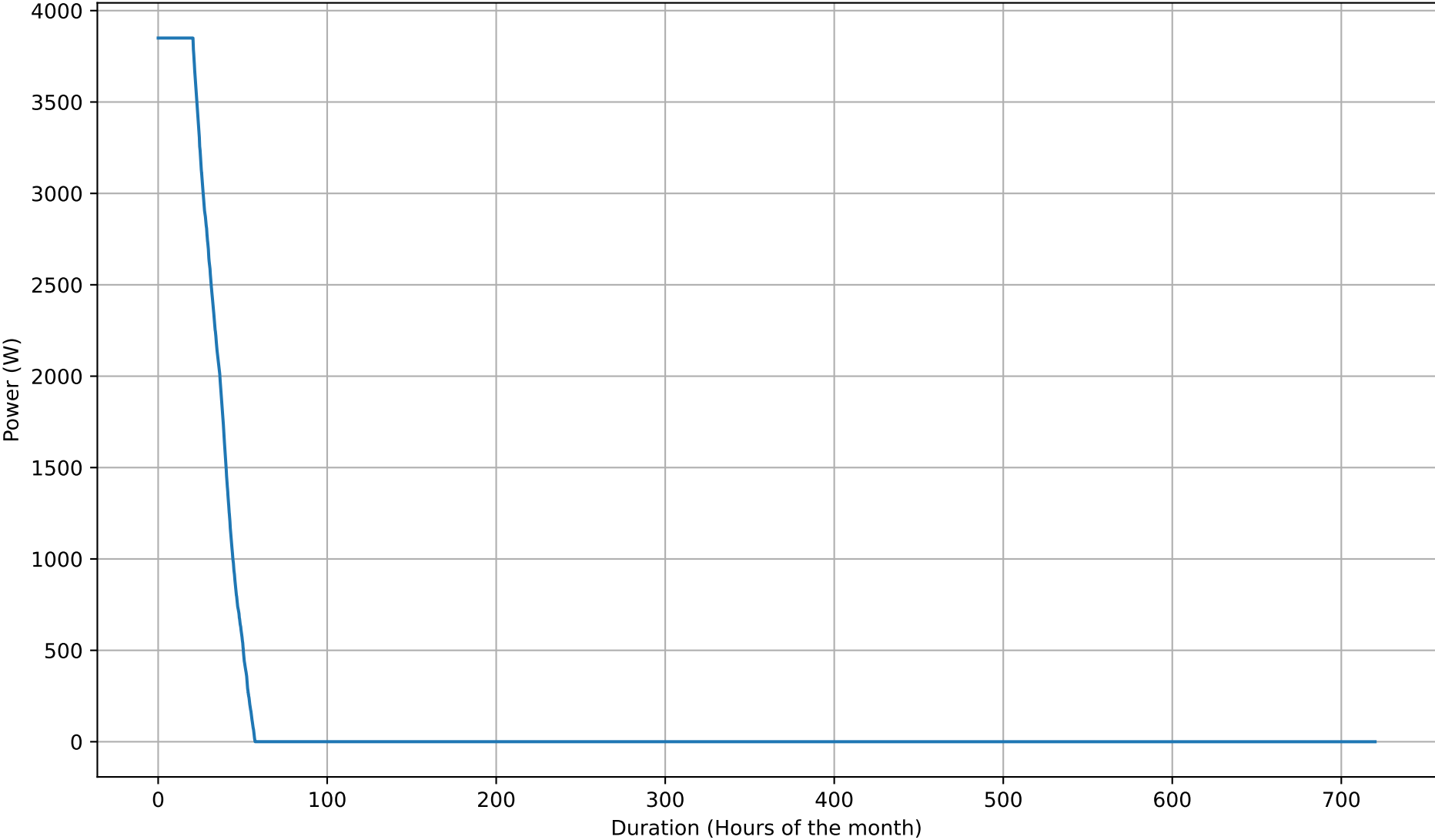
Battery Charging Power Duration Curve - 5kWh - Jun
