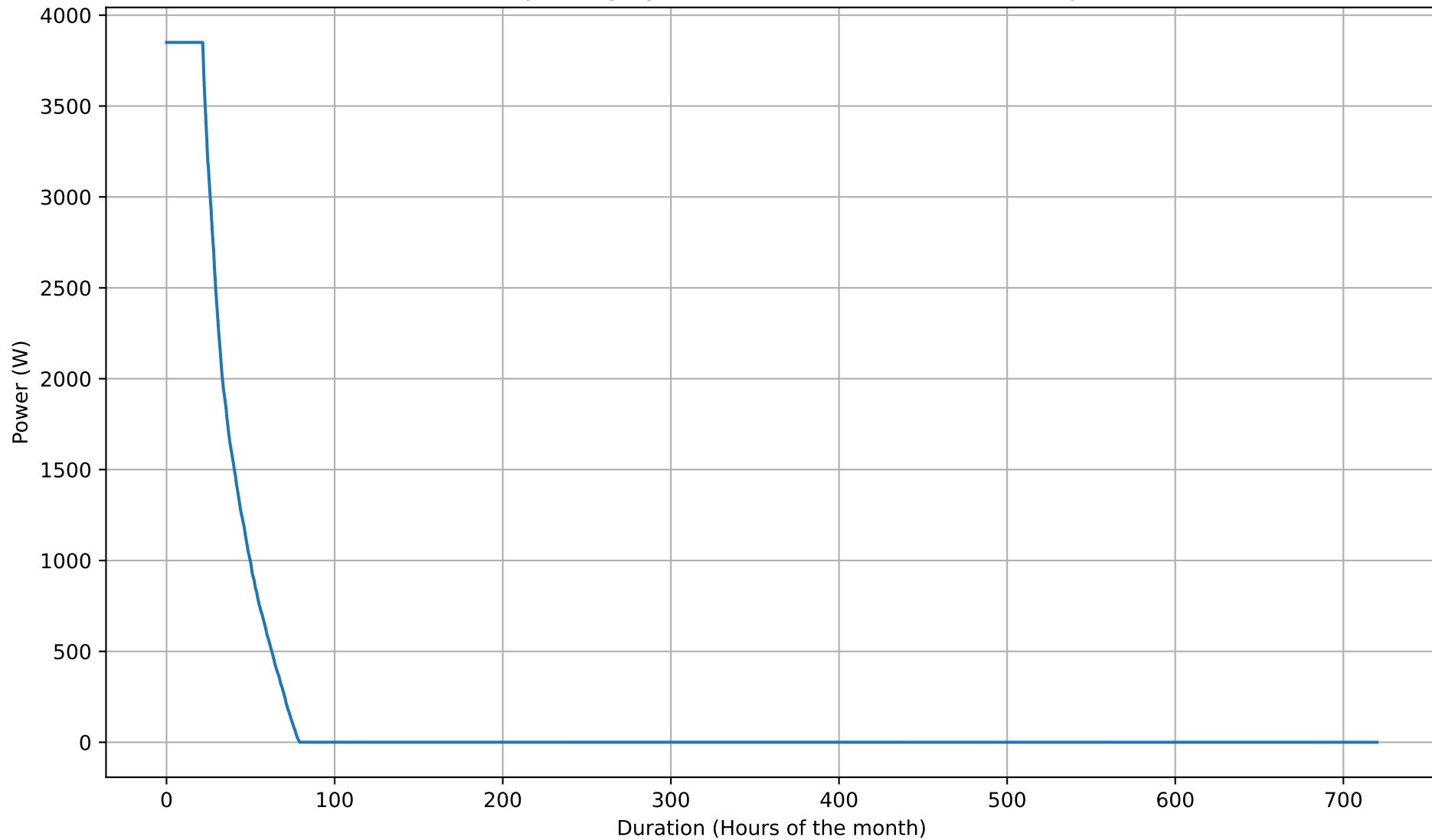
Battery Charging Power Duration Curve - 5kWh - Apr
