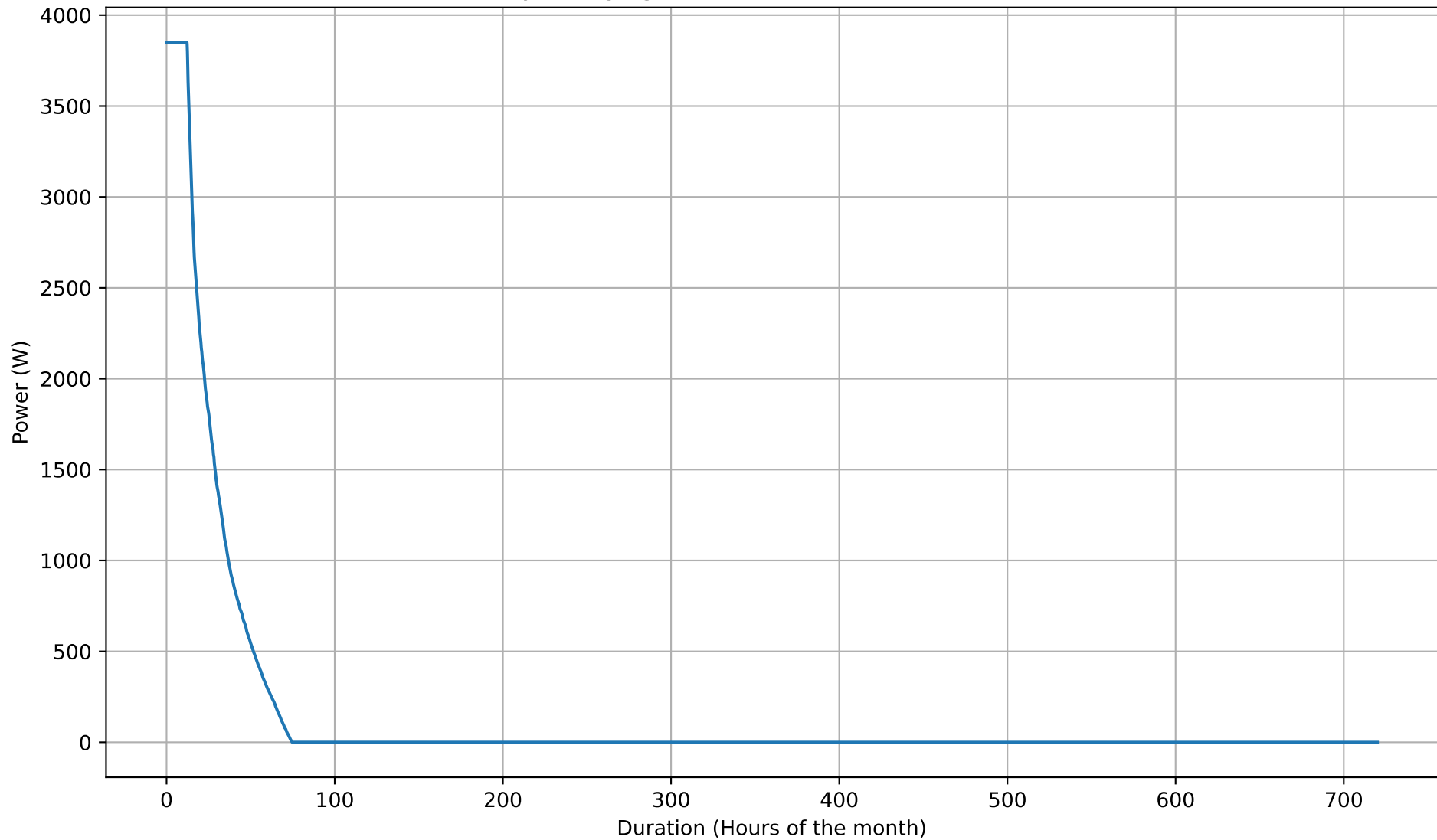
Battery Charging Power Duration Curve - 5kWh - Nov
