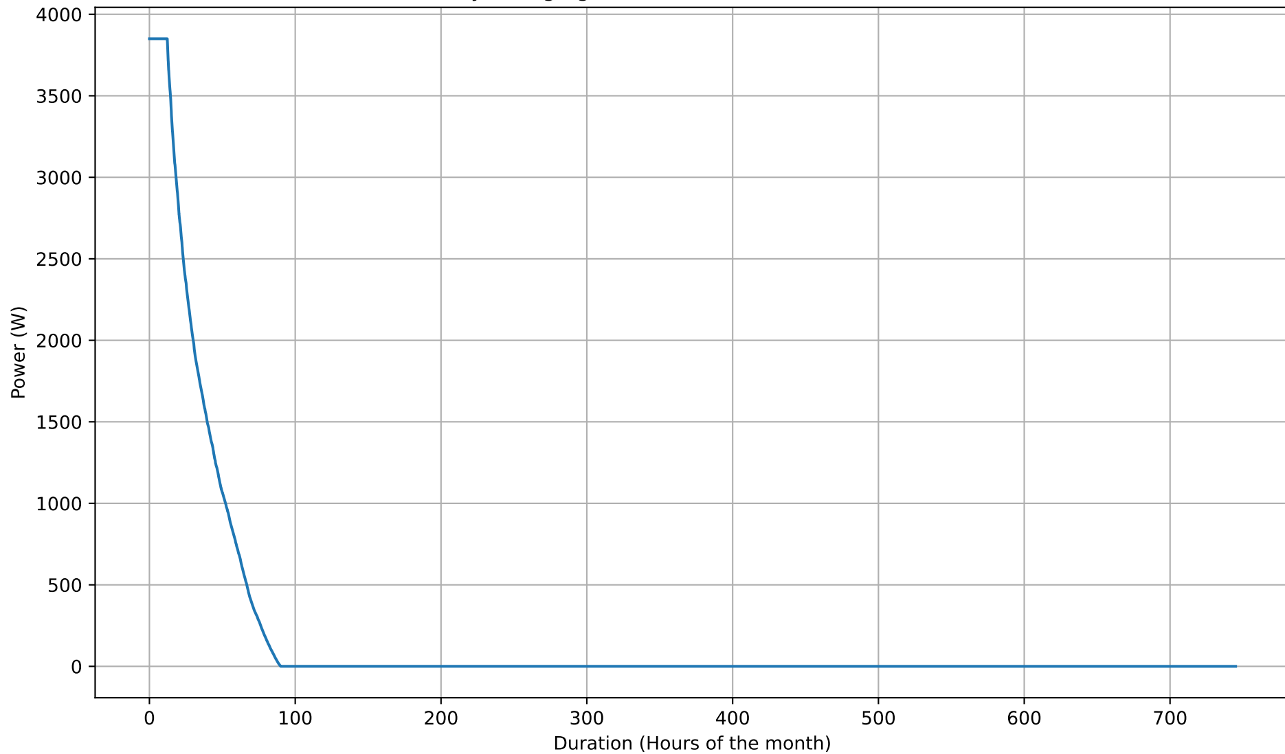
Battery Charging Power Duration Curve - 5kWh - Oct
