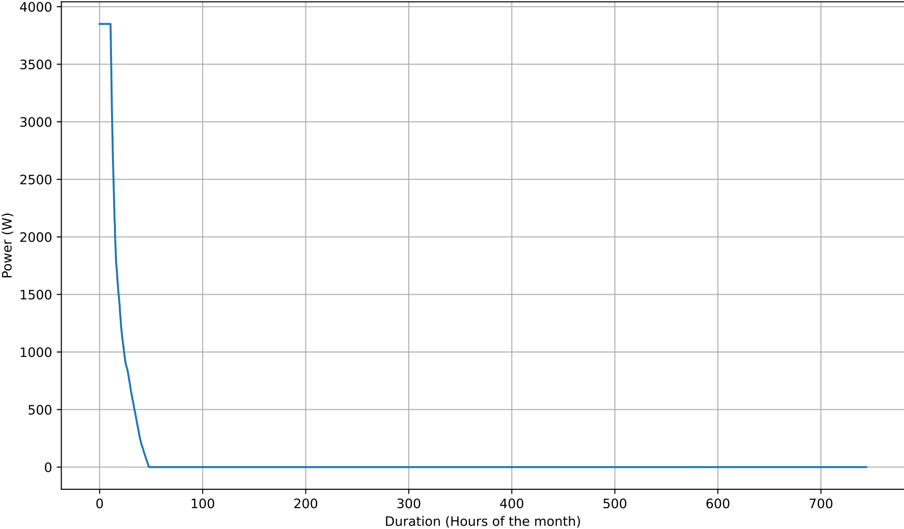
Battery Charging Power Duration Curve - 5kWh - Jan
