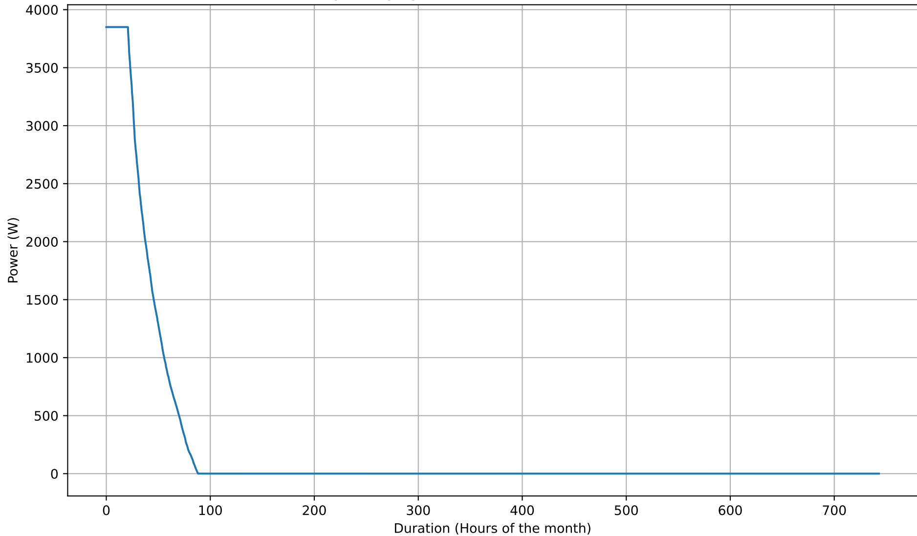
Battery Charging Power Duration Curve - 5kWh - Mar
