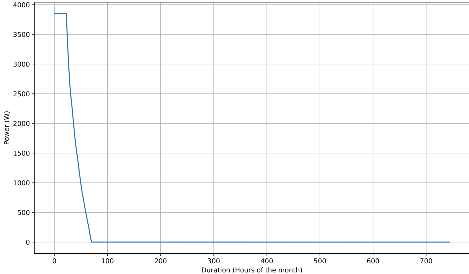
Battery Charging Power Duration Curve - 5kWh - Jul
