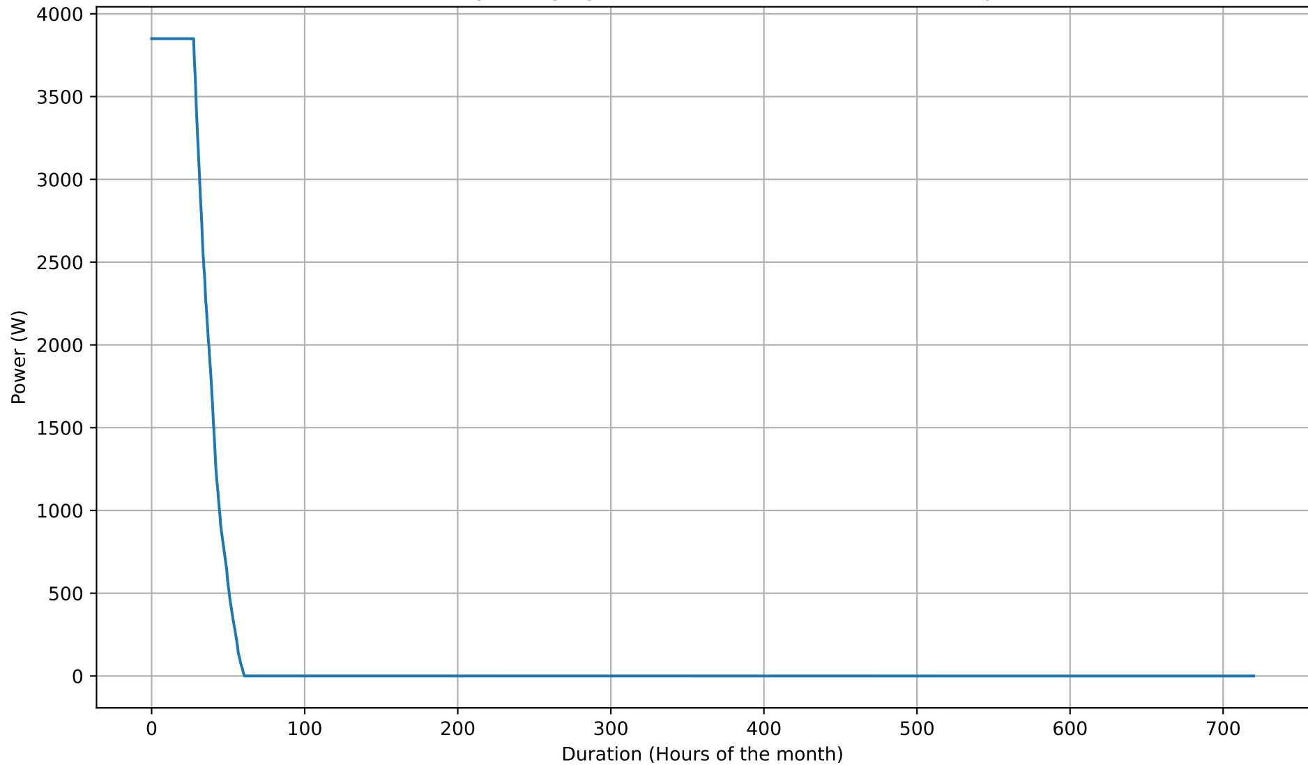
Battery Charging Power Duration Curve - 5kWh - Sep
