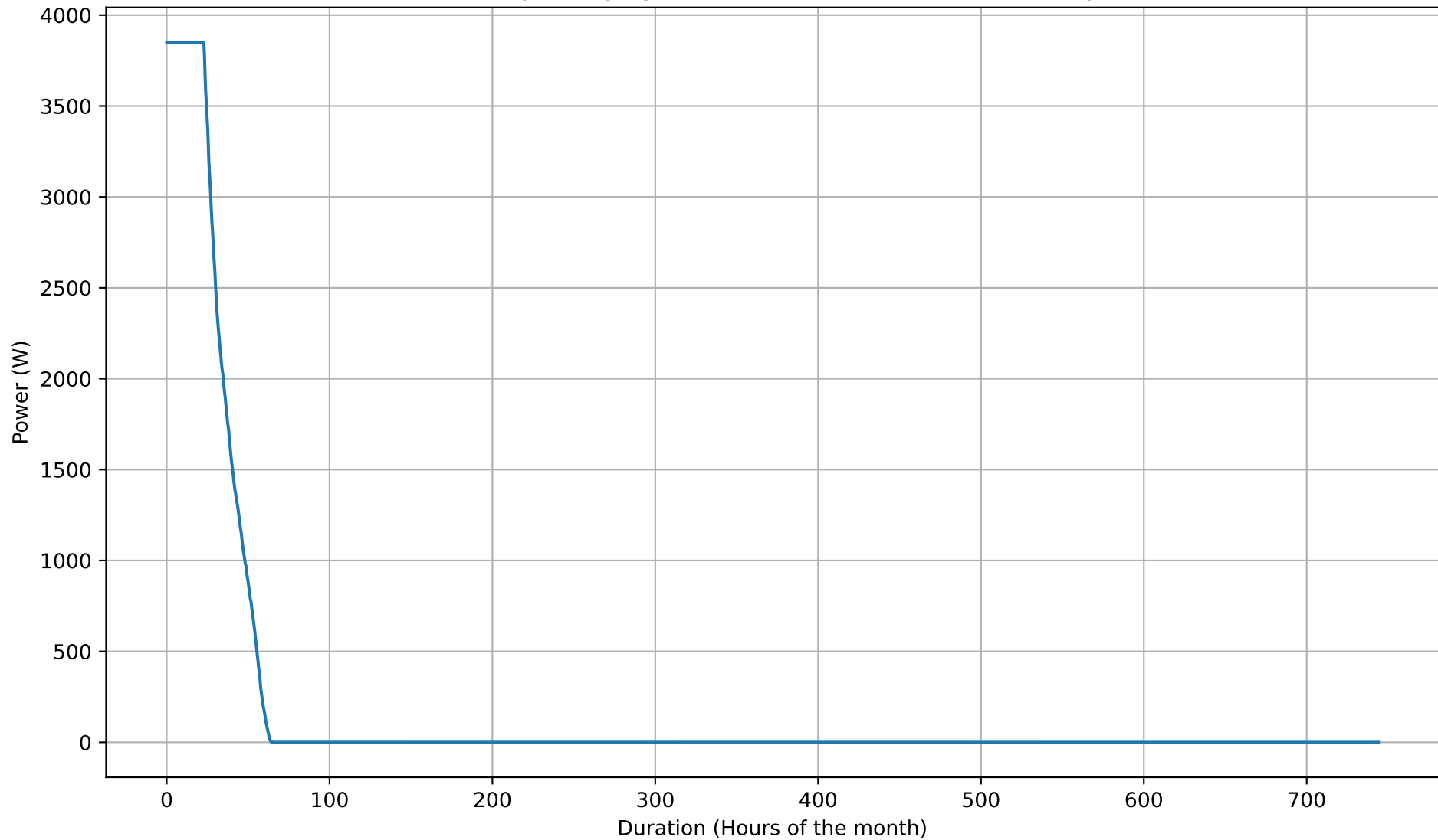
Battery Charging Power Duration Curve - 5kWh - May
