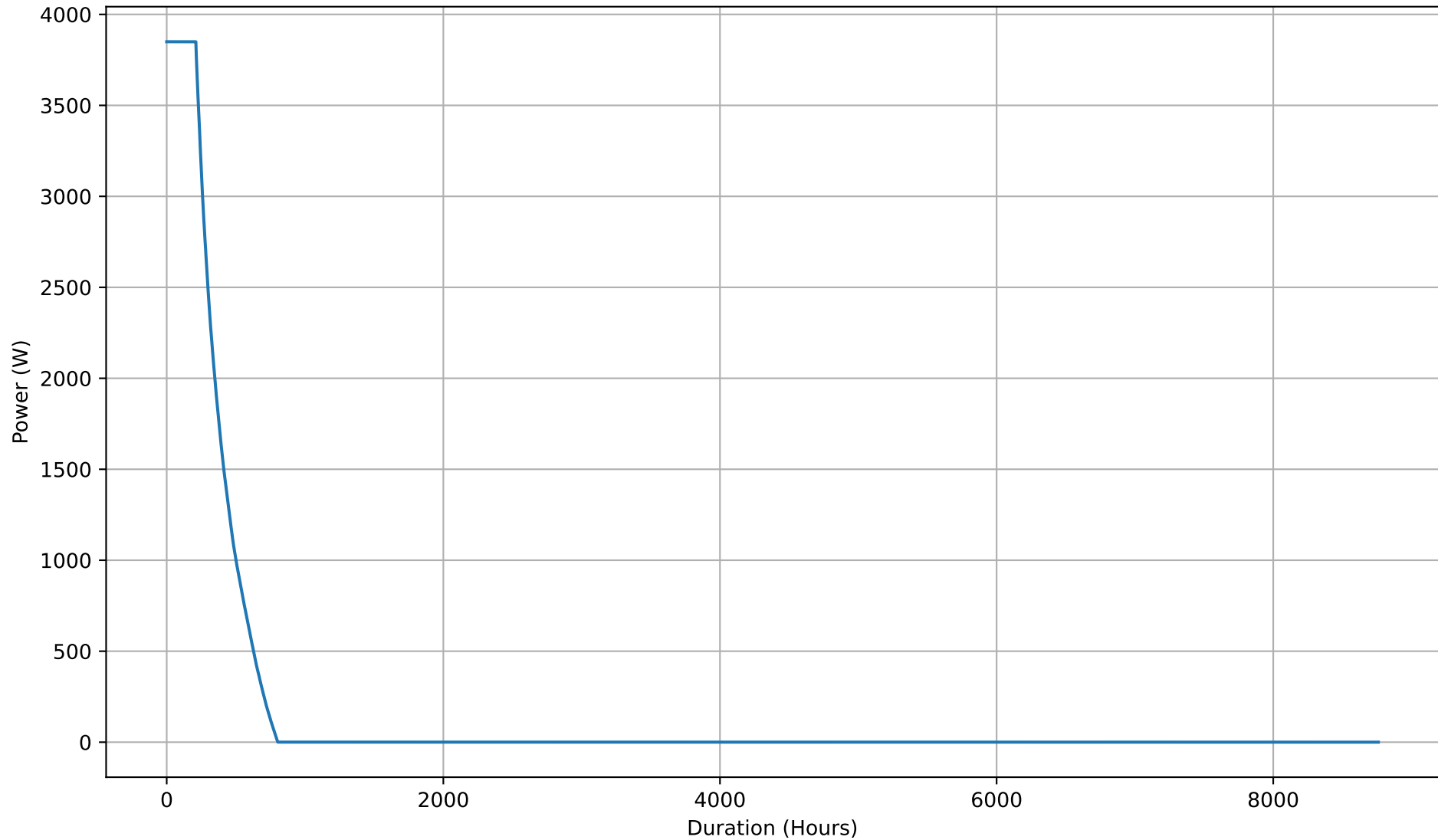
Yearly Battery Charging Power Duration Curve - 5kWh
