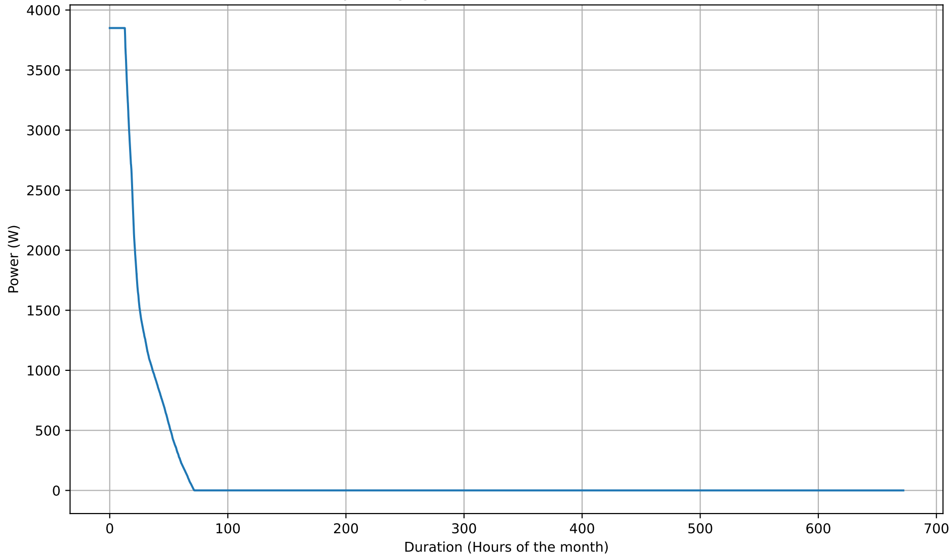
Battery Charging Power Duration Curve - 5kWh - Feb
